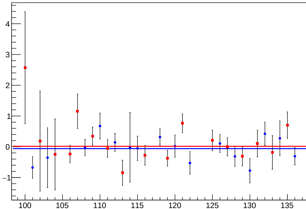
asym_us_avg_atlr_avg_avg_dit_vs_slug_sign_corrected
