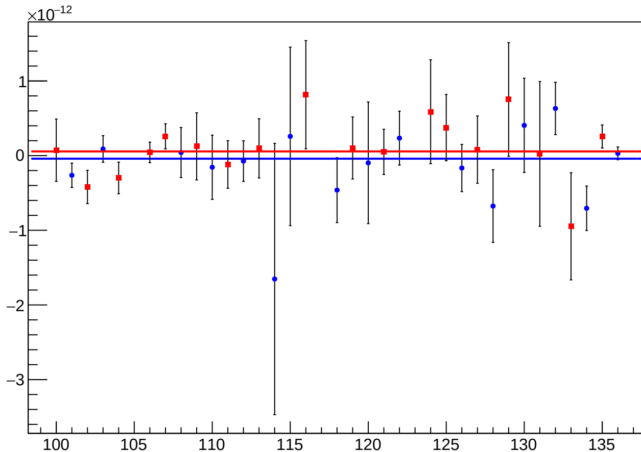
asym_at1_avg_at2_avg_dd_reg_vs_slug_sign_corrected
