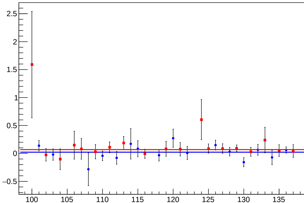
asym_sam3_eigen_dit_vs_cor_diff_mean vs Slug
