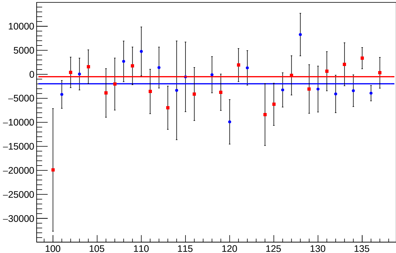
asym_sam_26_dd_dit_correction_mean vs Slug
