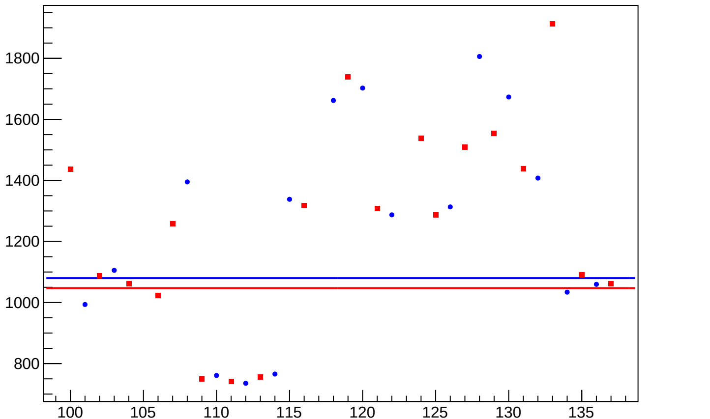
asym_sam_3748_avg_reg_correction_rms vs Slug
