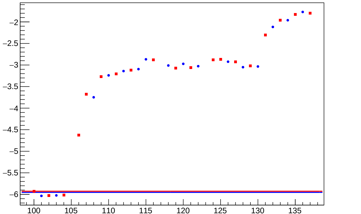
yield_bpm0l03X_mean vs Slug
