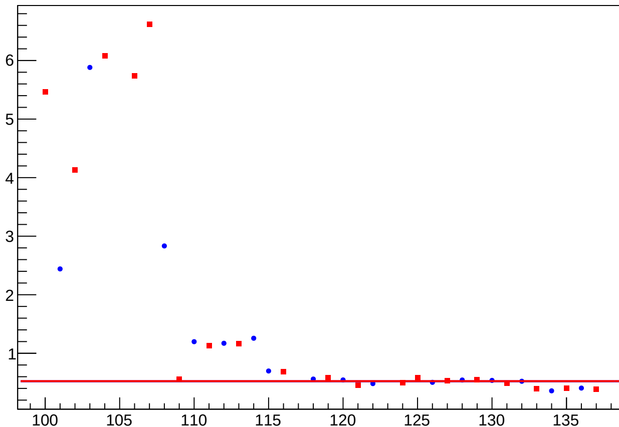
yield_cav4cY_rms vs Slug
