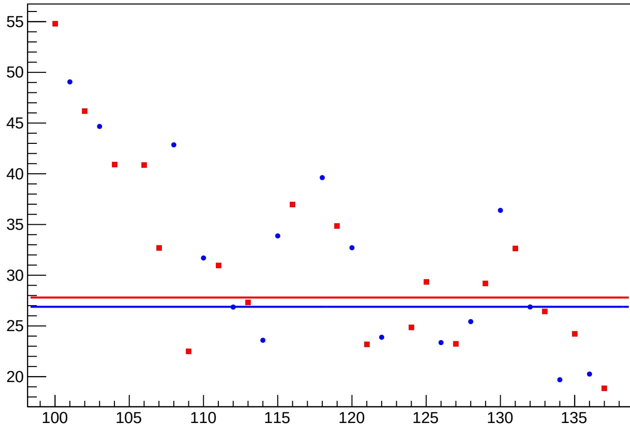
asym_sam_15_dd_dit_vs_cor_diff_rms vs Slug
