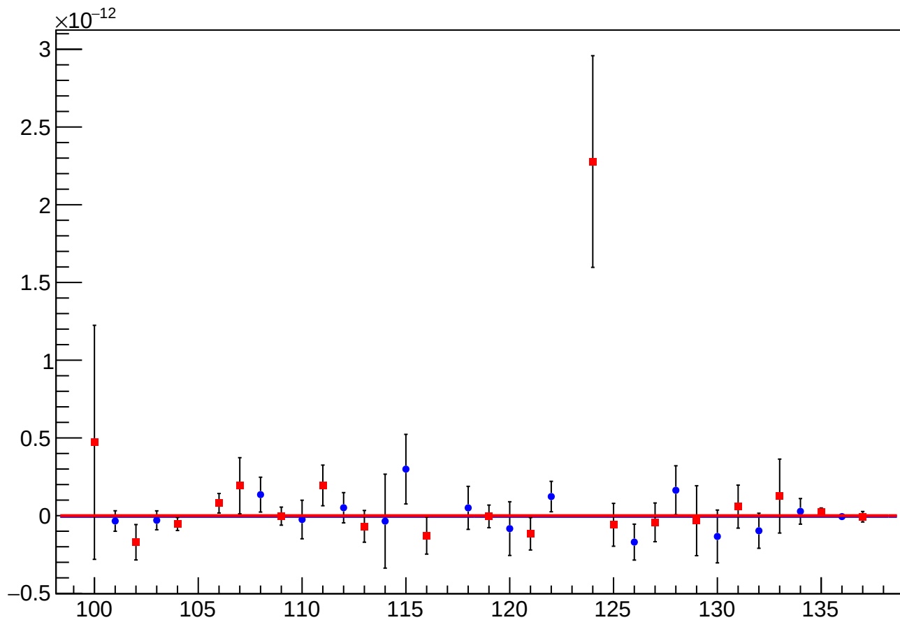
asym_at2_dd_eigen_cor_vs_cor_diff_mean vs Slug
