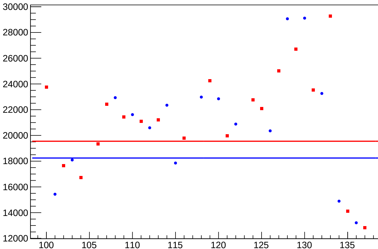
diff_bpmtargetsumX_rms vs Slug
