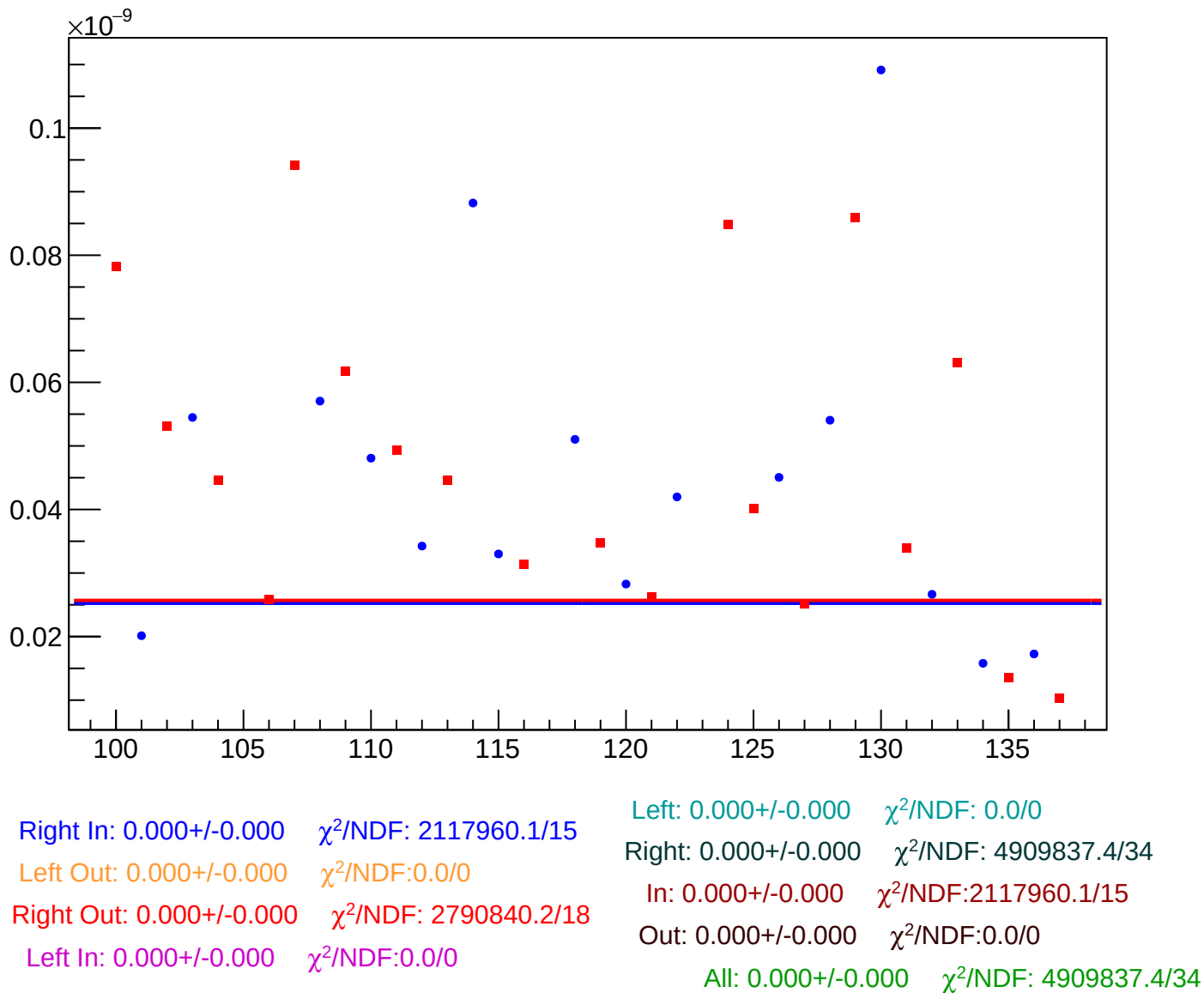
asym_sam_24_68_dd_eigen_cor_vs_cor_diff_rms vs Slug, Sign Corrected
