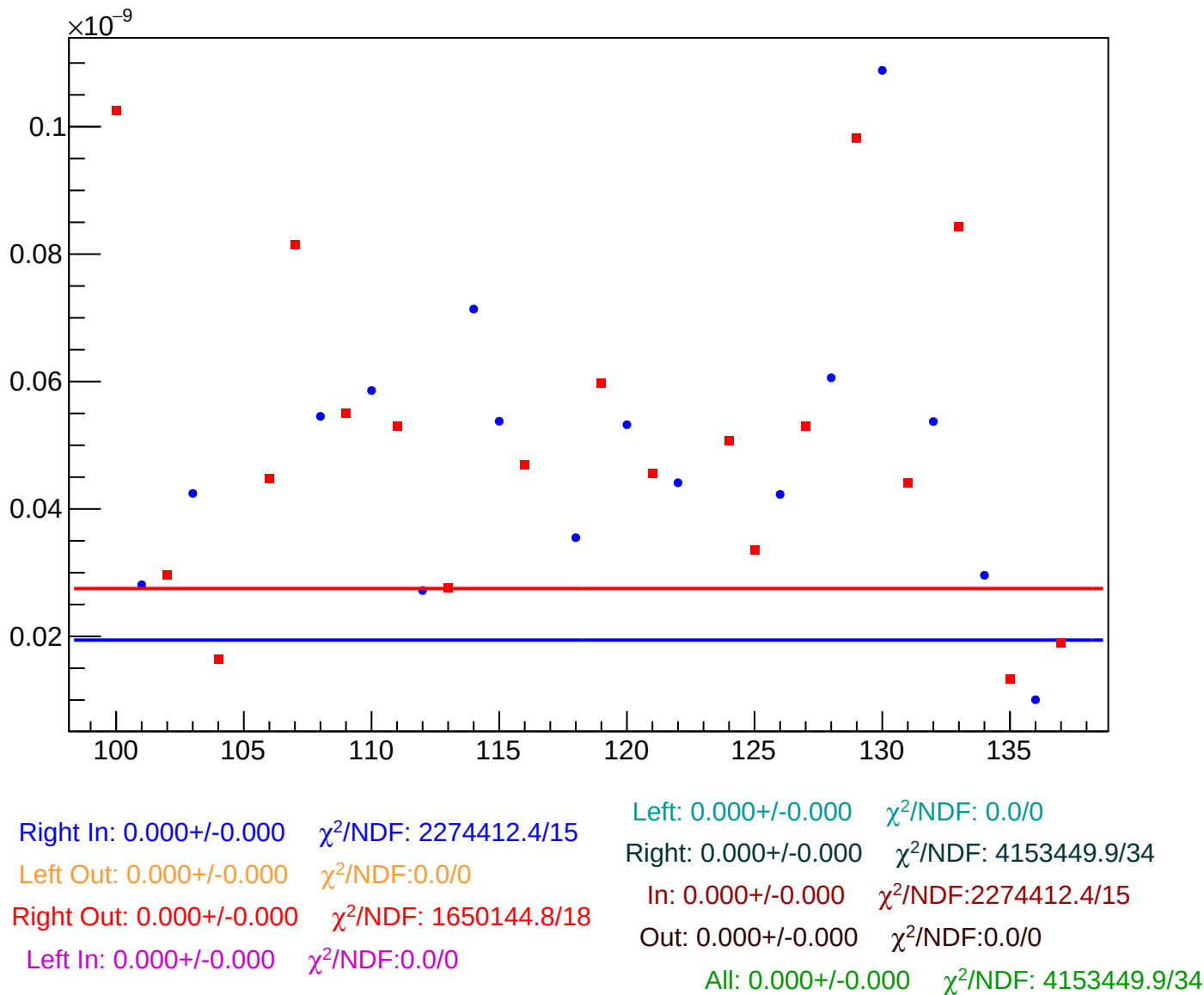
asym_usr_atr1_dd_reg_vs_cor_diff_rms vs Slug, Sign Corrected
