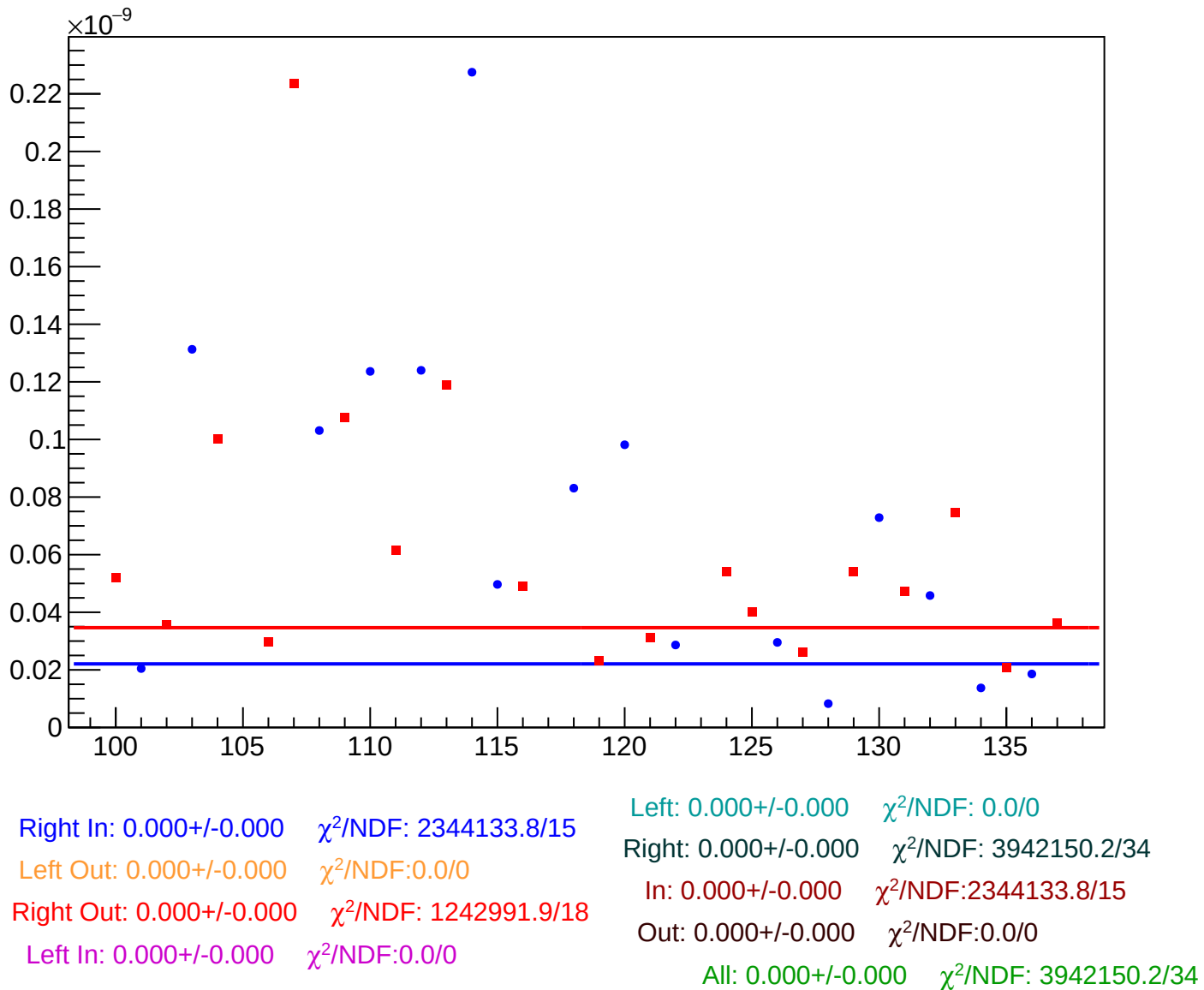
asym_atl1_reg_vs_cor_diff_rms vs Slug, Sign Corrected
