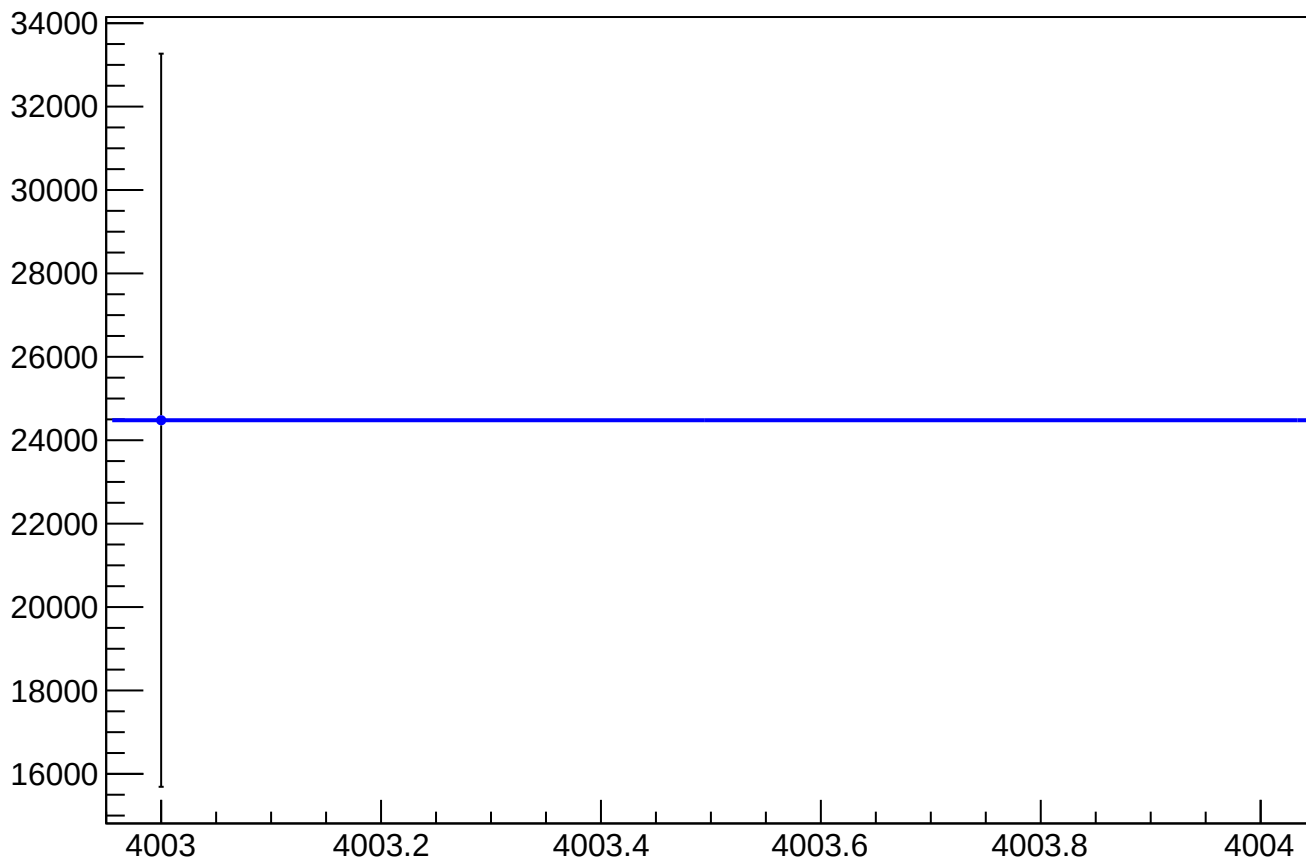
reg_asym_atr2_mean vs Slug, Sign Corrected
