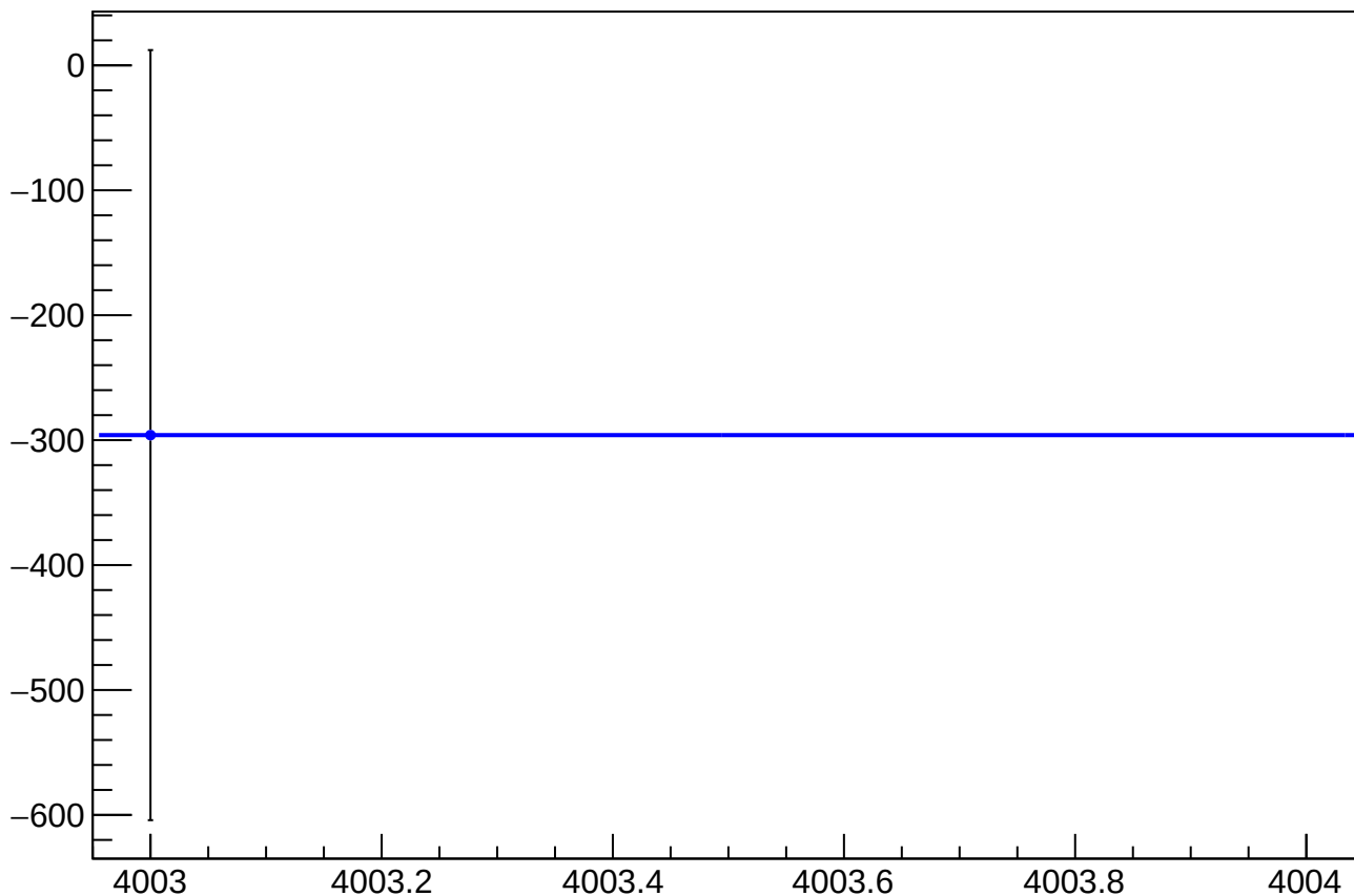
eigen_cor_asym_sam_15_dd_mean vs Slug, Sign Corrected
