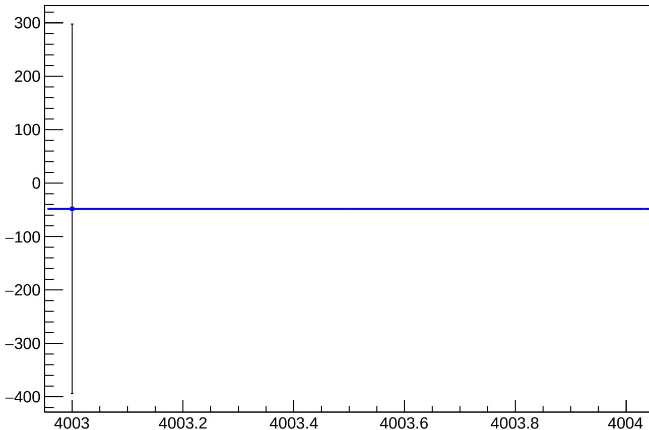
eigen_dit_asym_sam_26_48_dd_mean vs Slug, Sign Corrected
