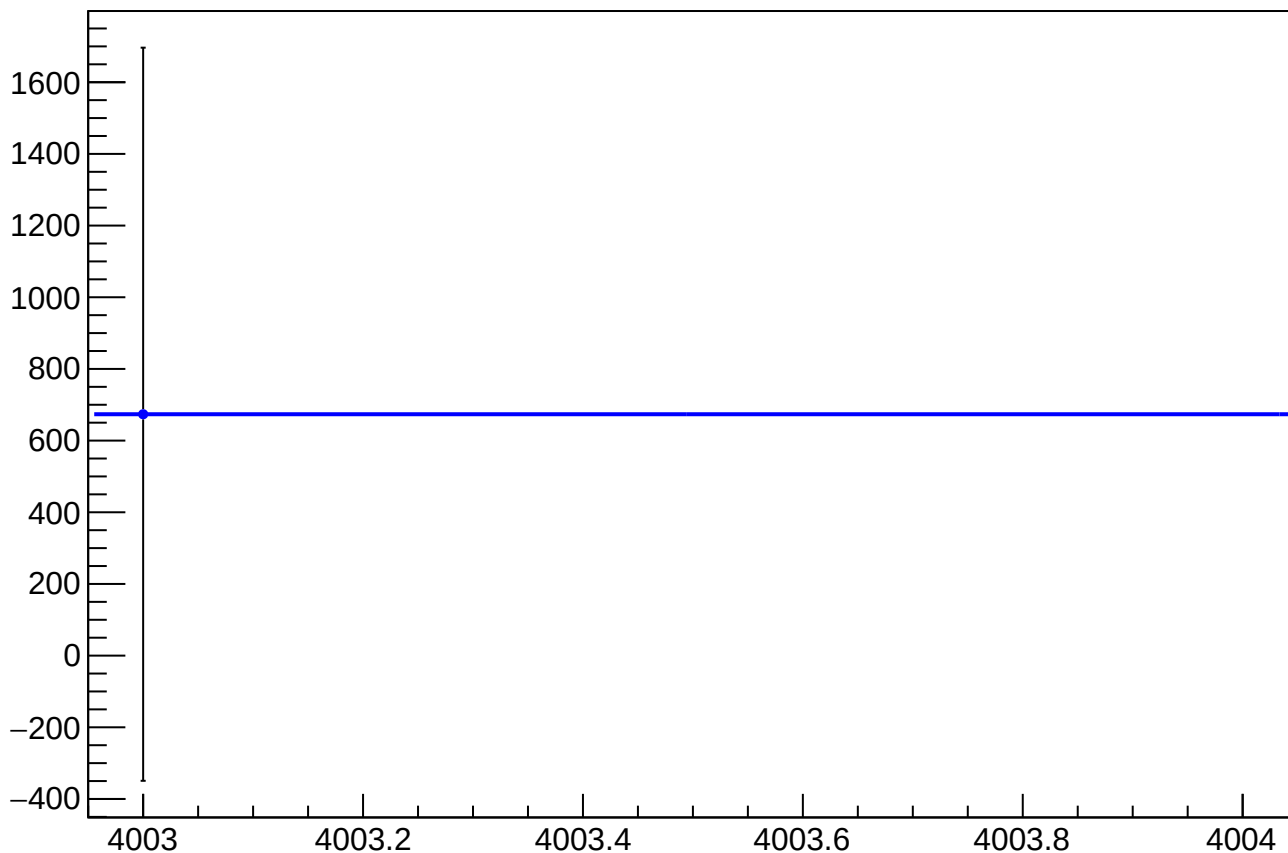
asym_sam_1357_avg_eigen_dit_correction_mean vs Slug, Sign Corrected
