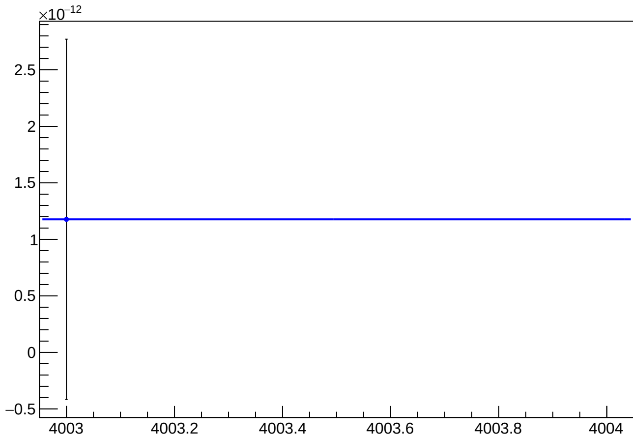
asym_us_avg_at2lr_avg_avg_reg_vs_cor_diff_mean vs Slug, Sign Corrected
