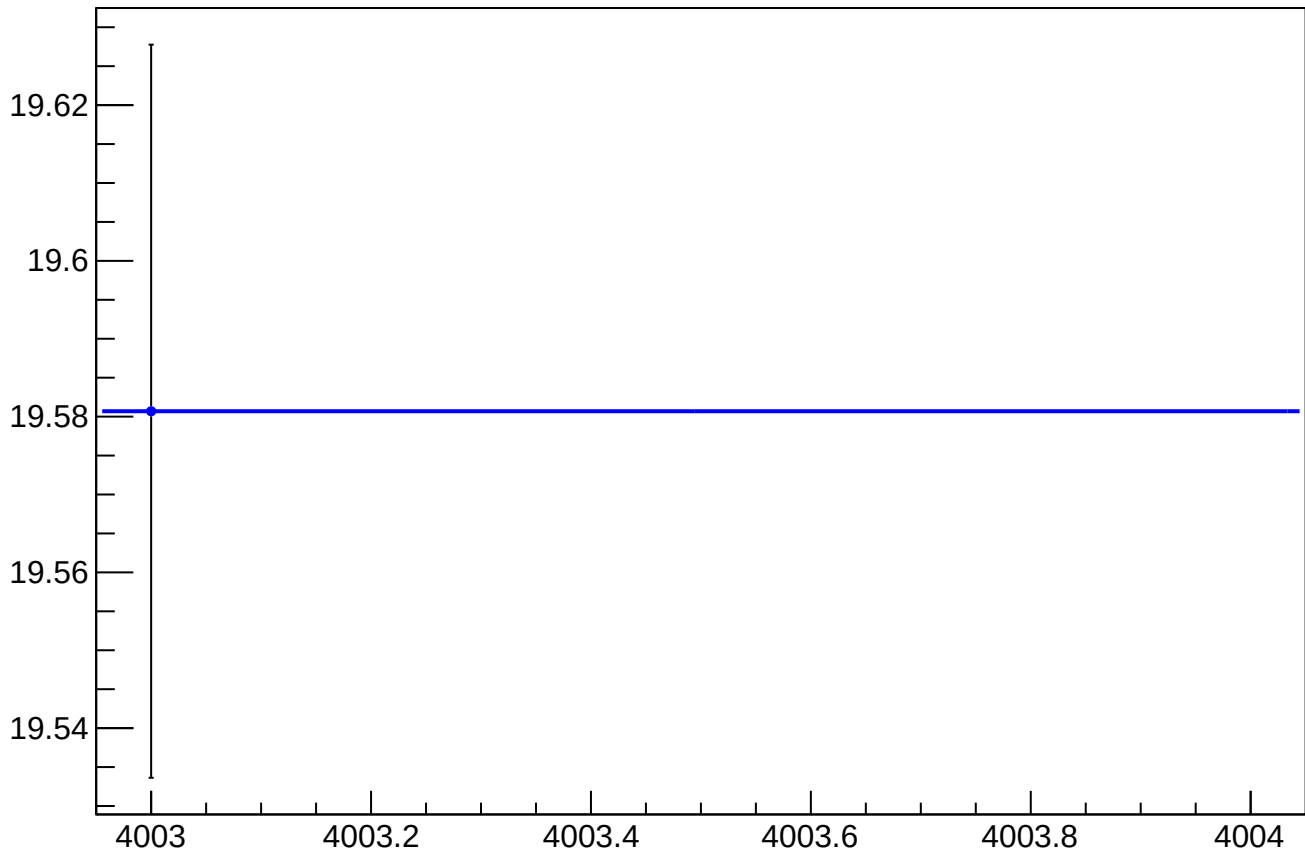
asym_sam8_eigen_dit_vs_eigen_cor_diff_rms vs Slug, Sign Corrected
