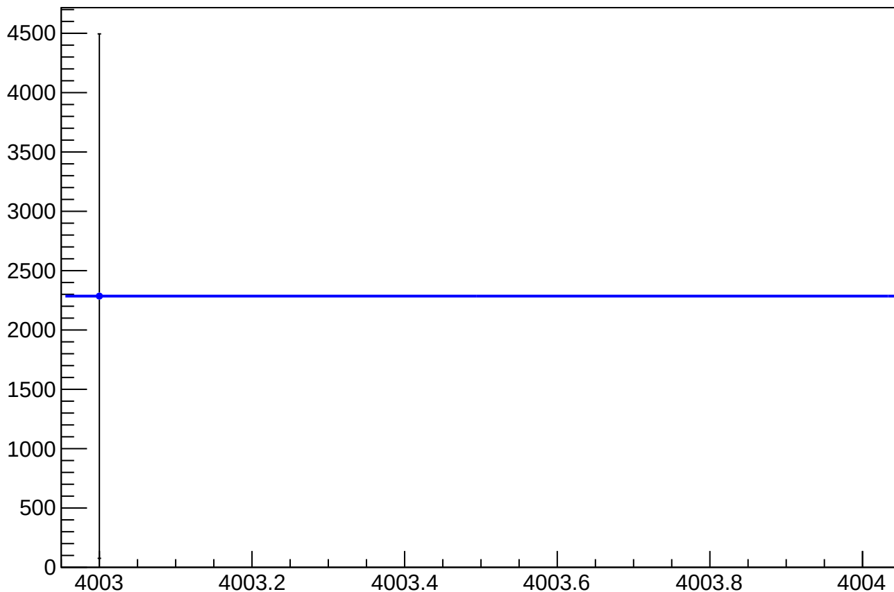
asym_usl_atl1_dd_dit_correction_mean vs Slug, Sign Corrected
