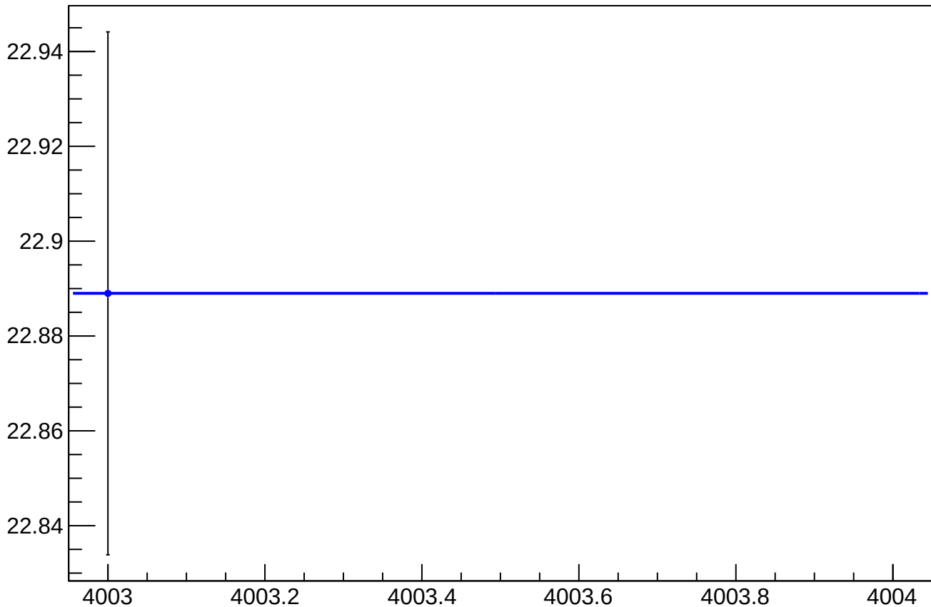
asym_sam_13_57_dd_eigen_dit_vs_eigen_cor_diff_rms vs Slug, Sign Corrected
