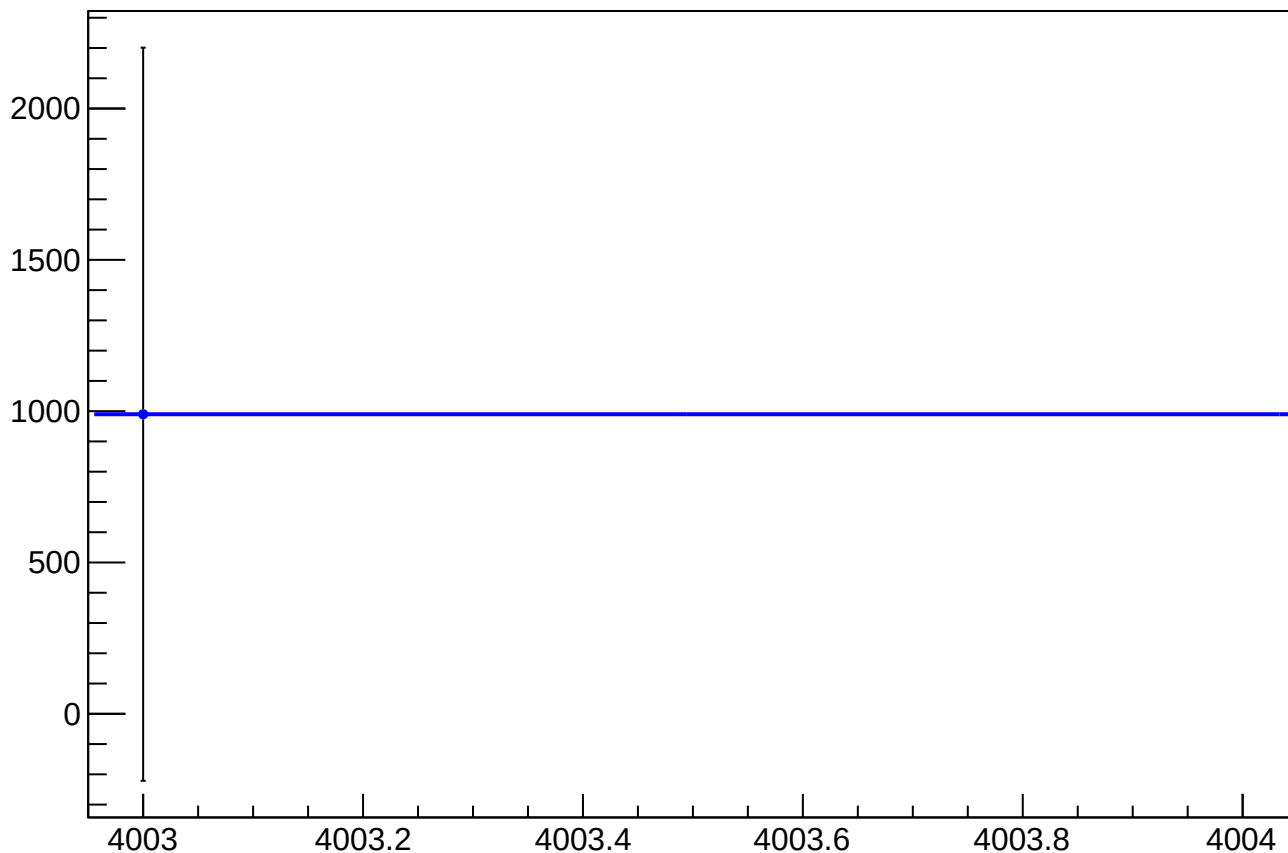
asym_sam_13_57_dd_dit_correction_mean vs Slug, Sign Corrected
