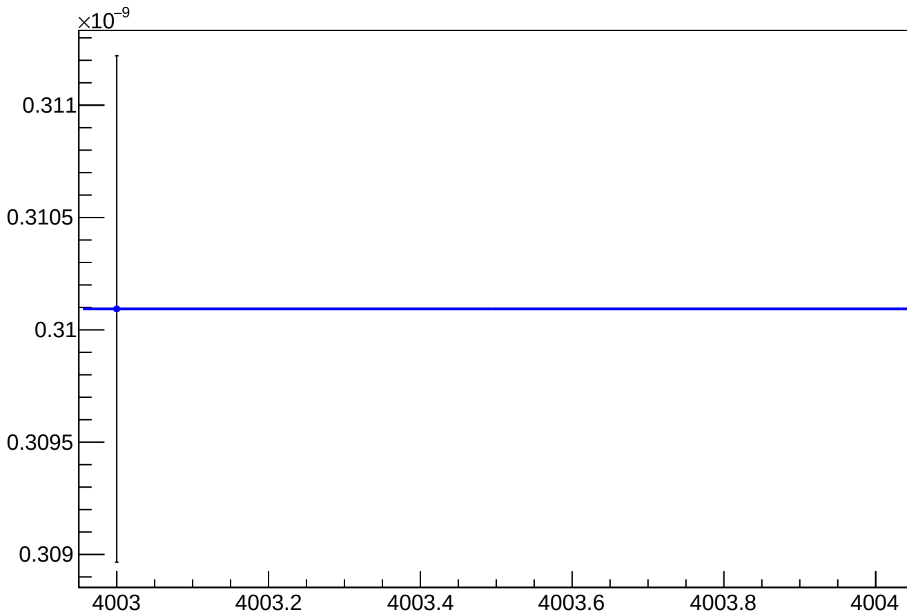
asym_us_avg_at2lr_avg_avg_reg_vs_cor_diff_rms vs Slug, Sign Corrected
