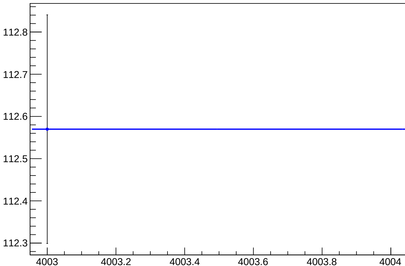
asym_usr_overload_cor_vs_eigen_cor_diff_rms vs Slug, Sign Corrected
