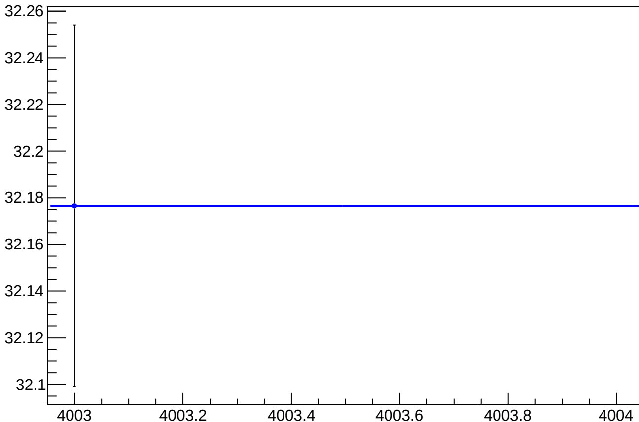
asym_sam_15_26_dd_eigen_dit_vs_cor_diff_rms vs Slug, Sign Corrected
