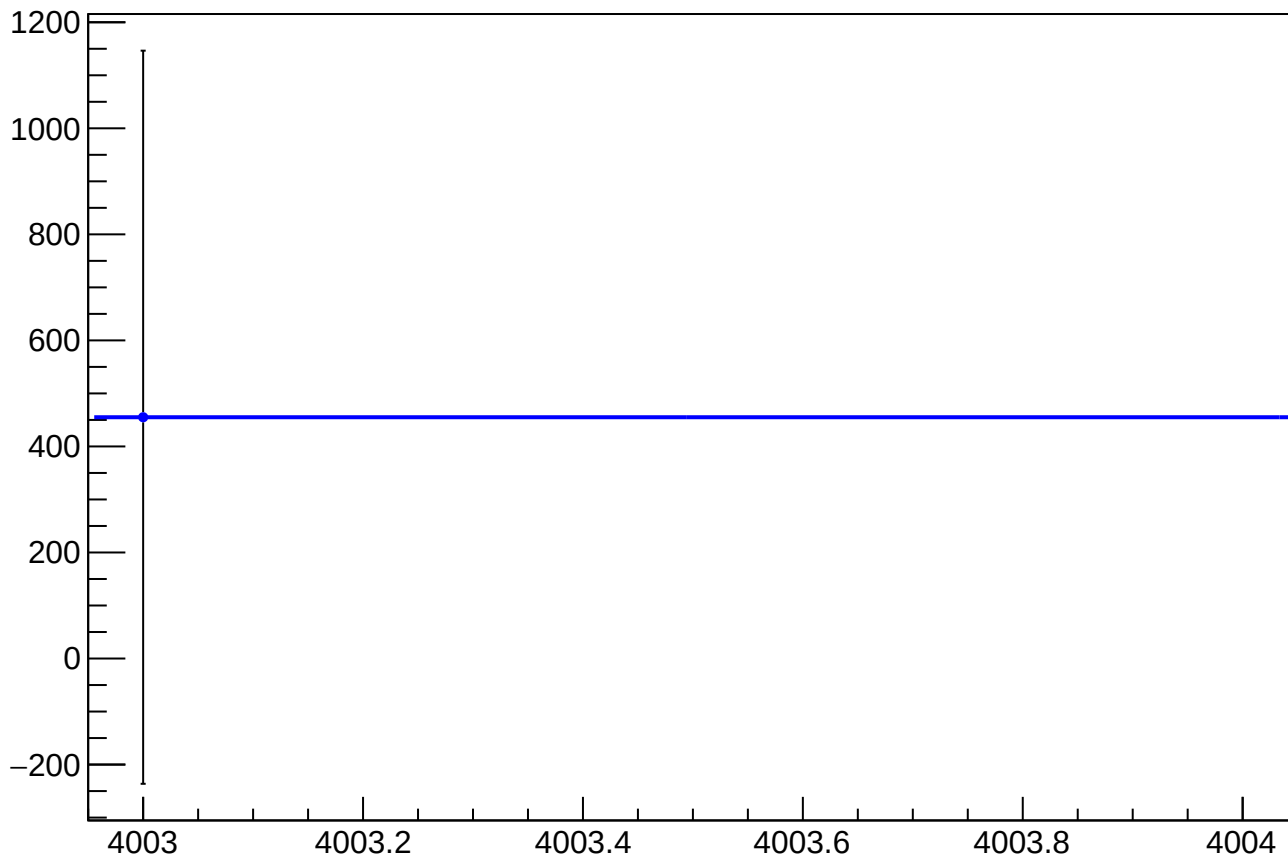
asym_sam8_dit_correction_mean vs Slug, Sign Corrected
