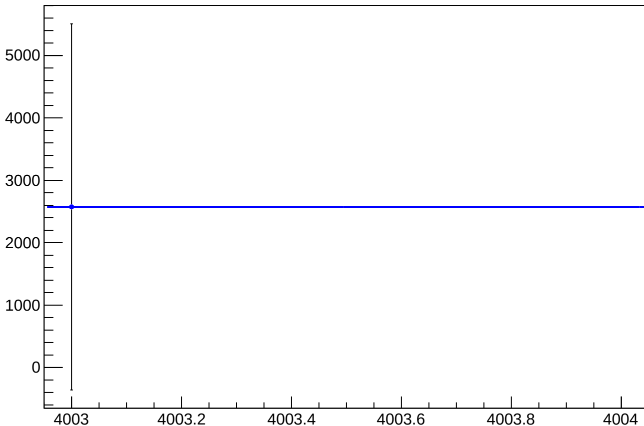
asym_sam_3748_avg_eigen_dit_correction_mean vs Slug, Sign Corrected
