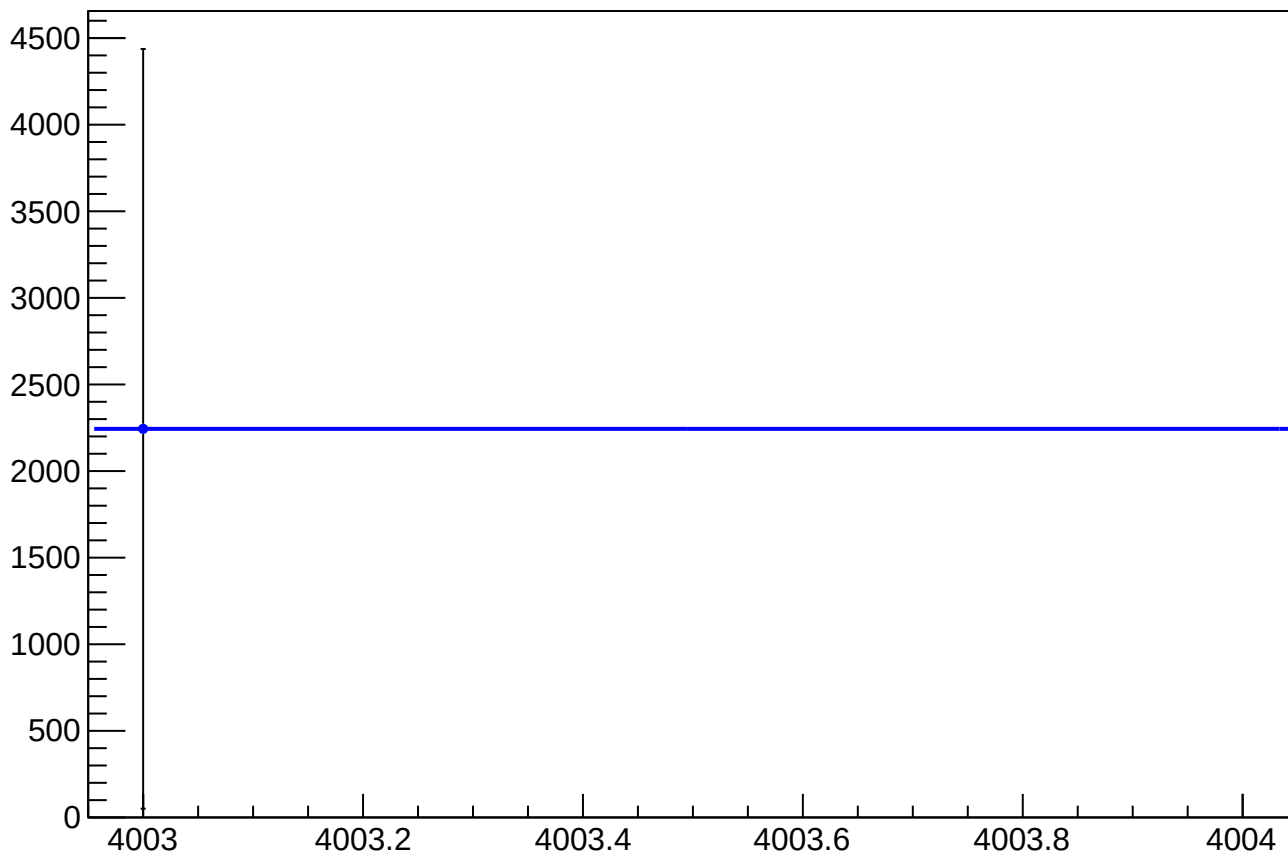
asym_usl_atl1_dd_reg_correction_mean vs Slug, Sign Corrected
