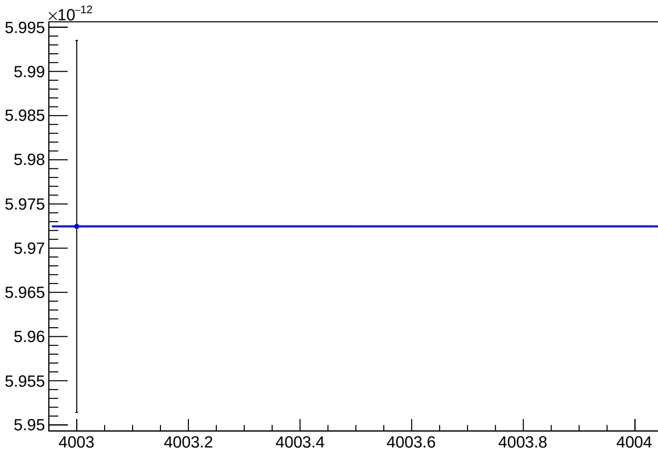
asym_sam_1357_avg_reg_vs_cor_diff_rms vs Slug, Sign Corrected
