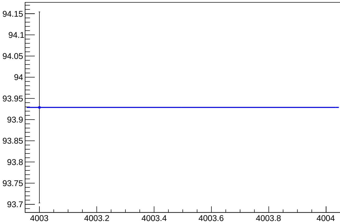
eigen_dit_asym_sam_15_dd_rms vs Slug, Sign Corrected
