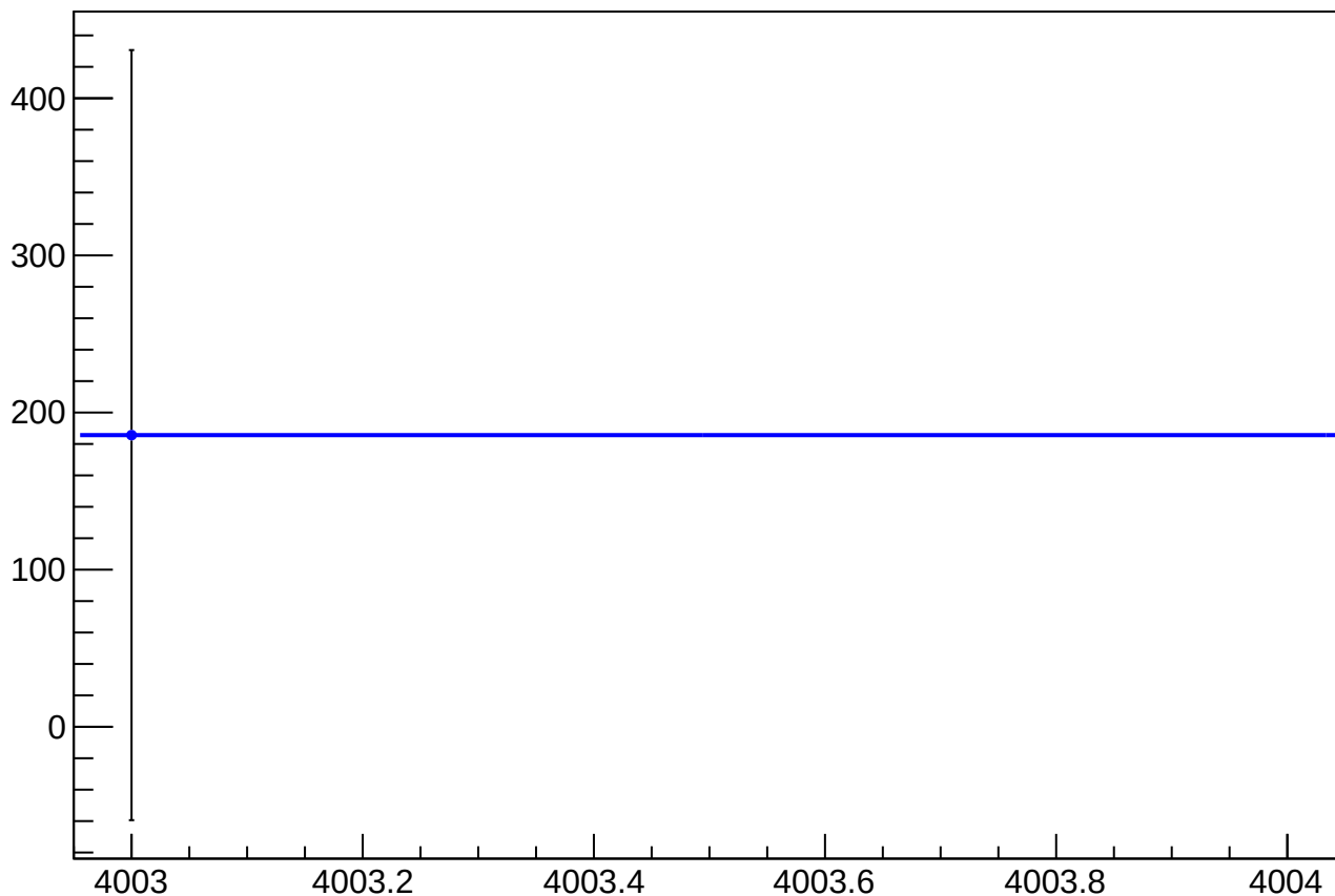
reg_asym_sam_37_avg_mean vs Slug, Sign Corrected
