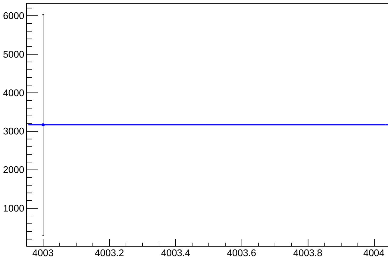
asym_sam_2468_avg_dit_correction_mean vs Slug, Sign Corrected
