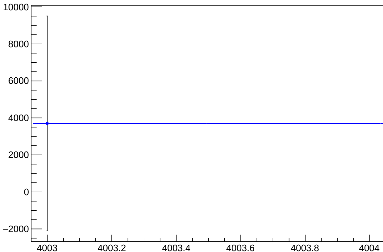
asym_us_dd_at2lr_dd_dd_mean vs Slug, Sign Corrected
