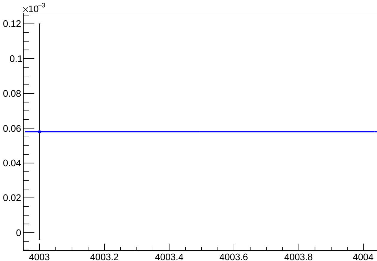
asym_atl2_eigen_dit_vs_dit_diff_mean vs Slug, Sign Corrected
