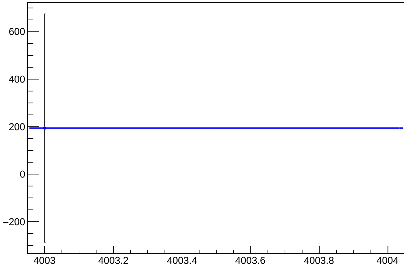
dit_asym_sam5_mean vs Slug, Sign Corrected
