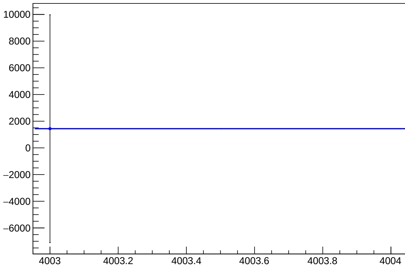
eigen_cor_asym_atr1_mean vs Slug, Sign Corrected
