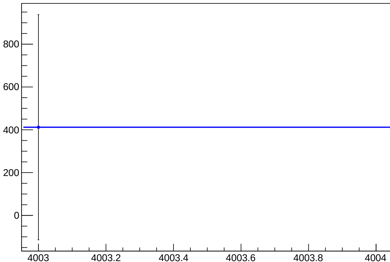
eigen_dit_asym_sam_48_avg_mean vs Slug, Sign Corrected
