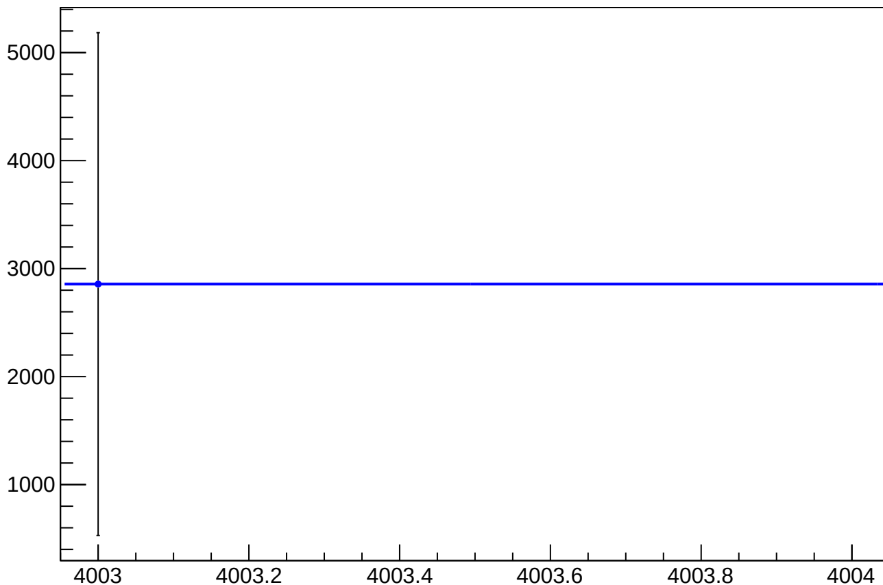
asym_us_dd_atlr_dd_avg_reg_correction_mean vs Slug, Sign Corrected
