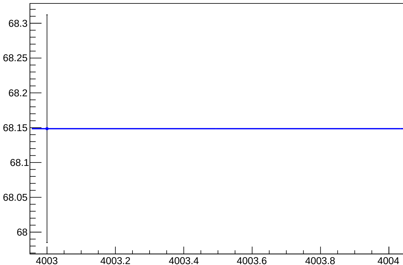
eigen_cor_asym_sam_37_48_dd_rms vs Slug, Sign Corrected
