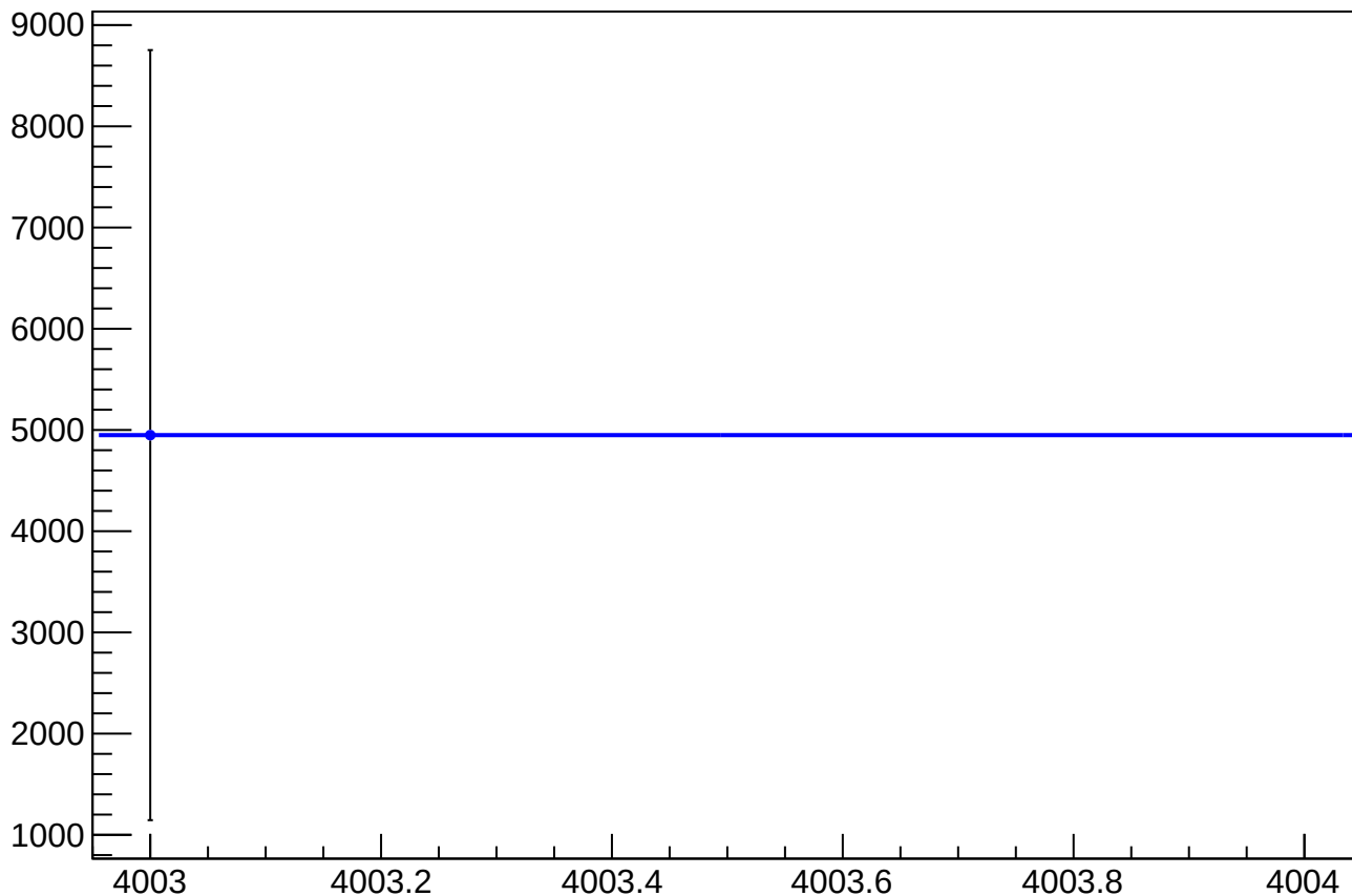
asym_us_dd_at1lr_dd_dd_dit_correction_mean vs Slug, Sign Corrected
