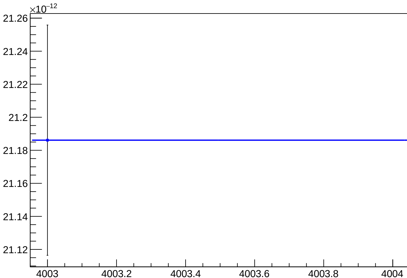
asym_sam_1526_avg_reg_vs_cor_diff_rms vs Slug, Sign Corrected
