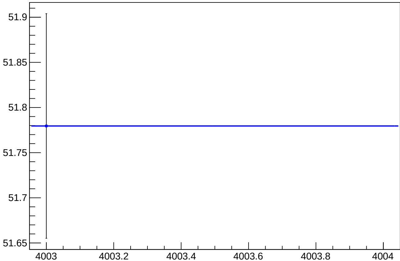
cor_asym_sam_37_26_dd_rms vs Slug, Sign Corrected
