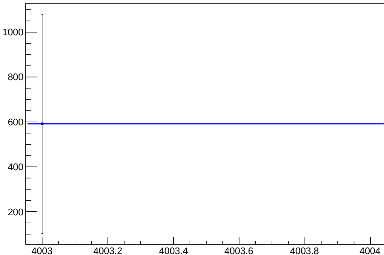
asym_atl_avg_atr_avg_dd_dit_correction_mean vs Slug, Sign Corrected
