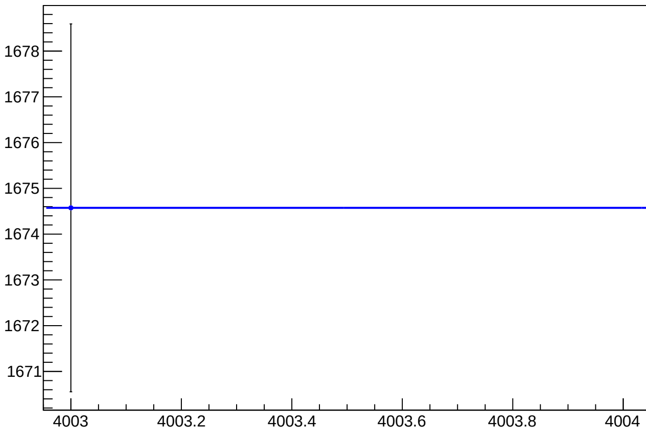
reg_asym_us_dd_atlr_dd_avg_rms vs Slug, Sign Corrected
