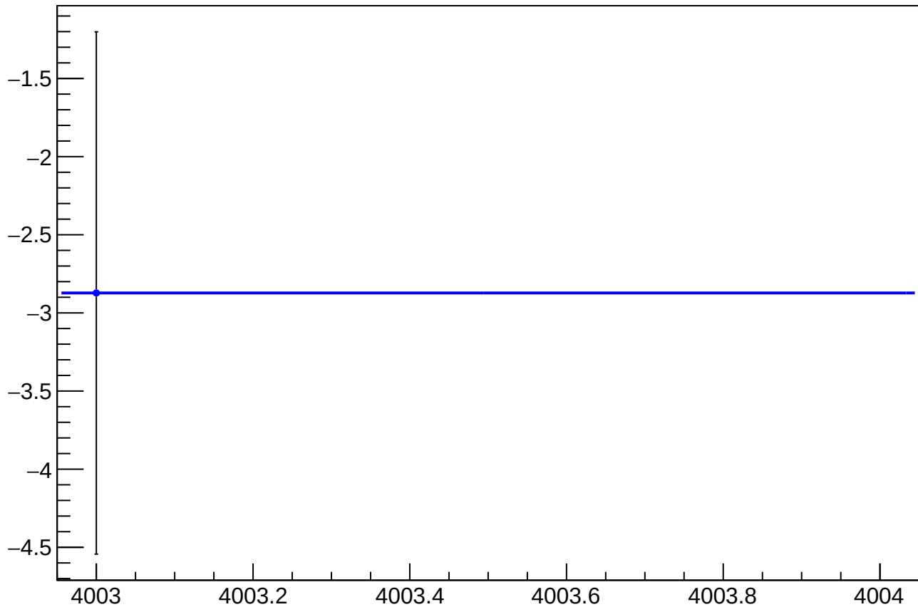
asym_us_avg_at2lr_avg_avg_eigen_dit_vs_cor_diff_mean vs Slug, Sign Corrected
