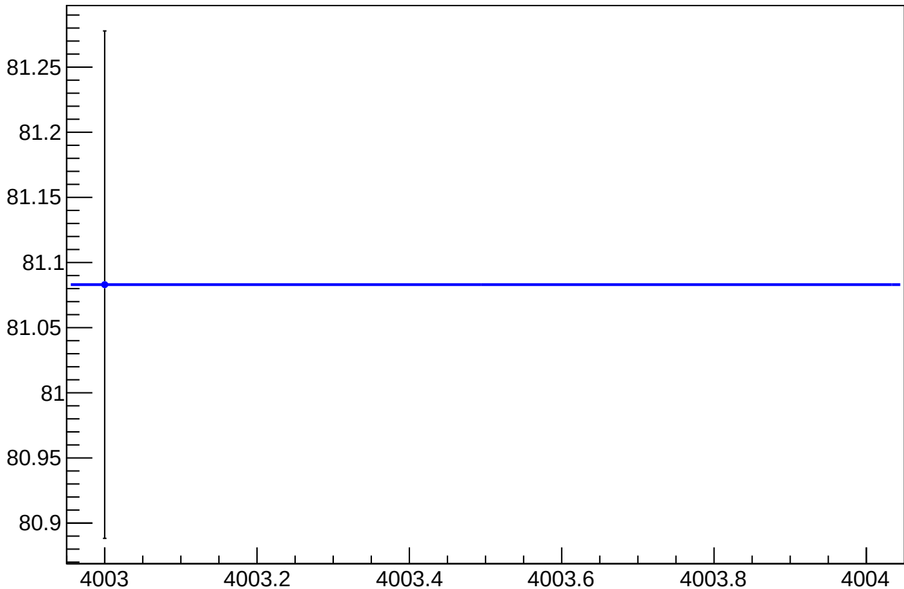
asym_sam_26_dd_dit_vs_eigen_cor_diff_rms vs Slug, Sign Corrected
