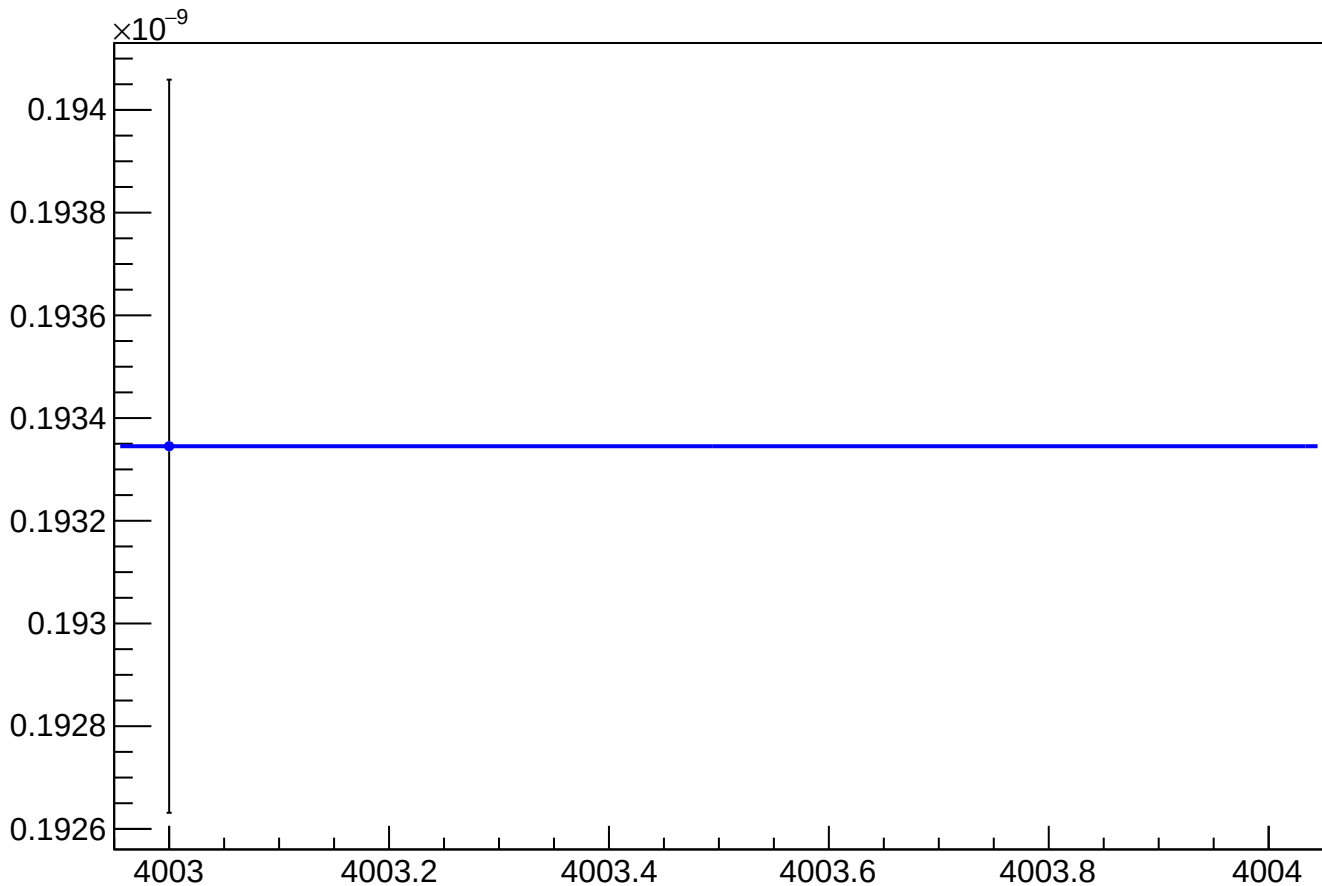
asym_atr2_reg_vs_cor_diff_rms vs Slug, Sign Corrected
