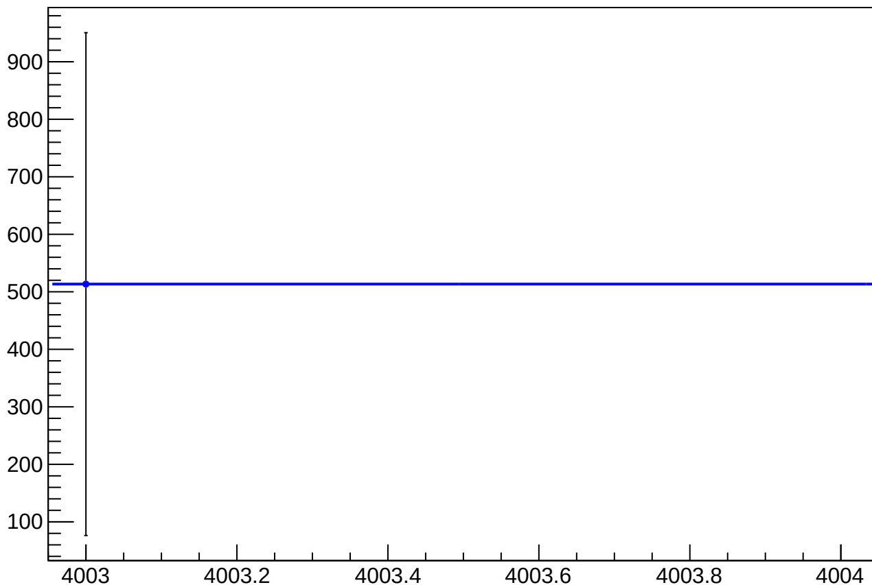
asym_atl1r2_dd_atl2r1_dd_avg_reg_correction_mean vs Slug, Sign Corrected
