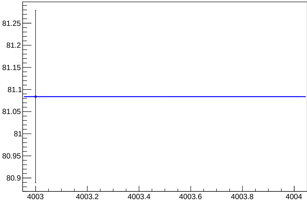
asym_sam_26_dd_eigen_dit_vs_cor_diff_rms vs Slug, Sign Corrected
