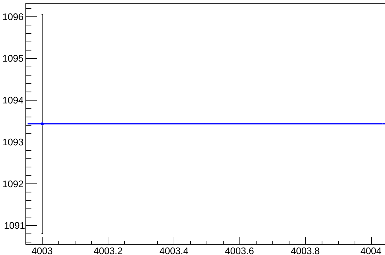
asym_sam_48_dd_reg_correction_rms vs Slug, Sign Corrected
