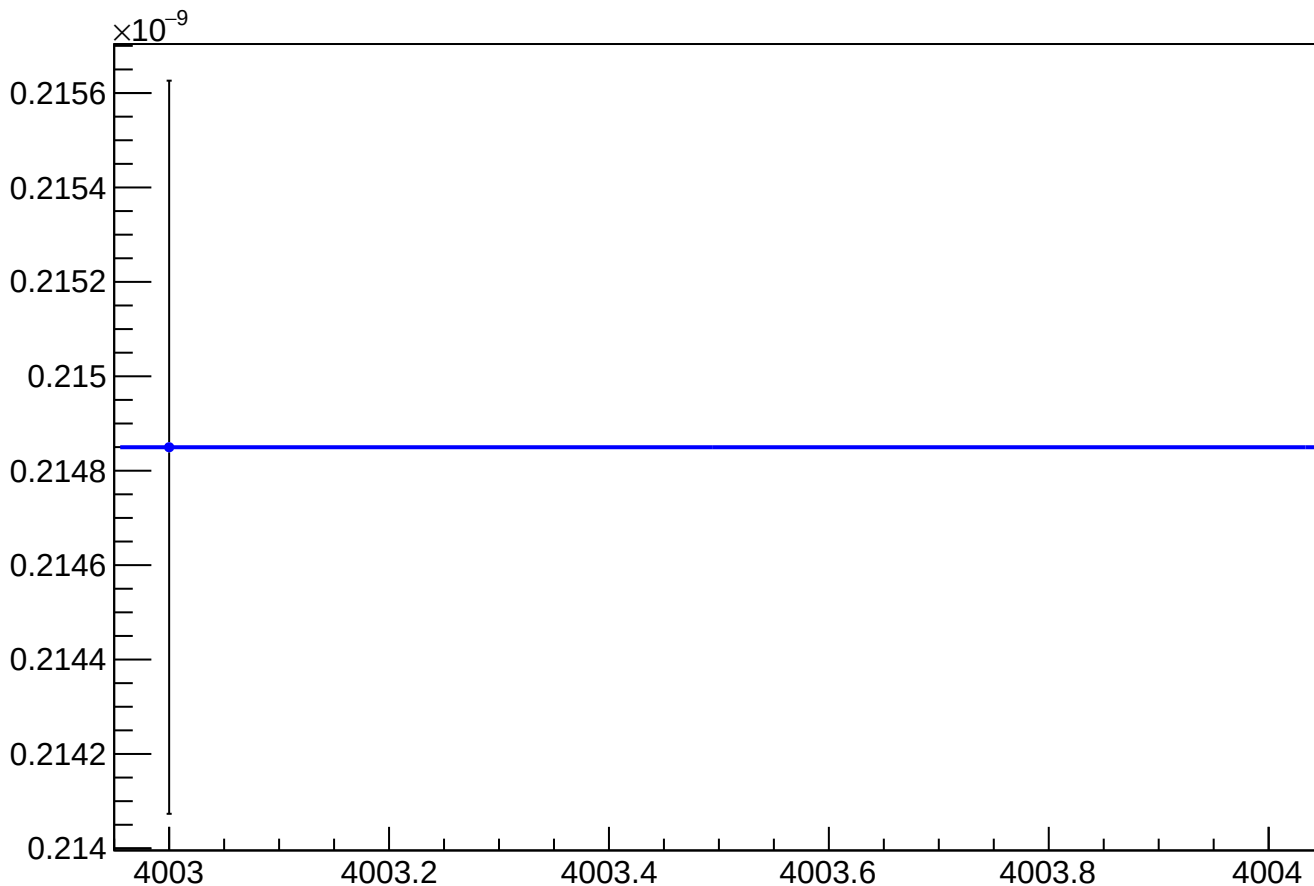
asym_at2_avg_reg_vs_cor_diff_rms vs Slug, Sign Corrected
