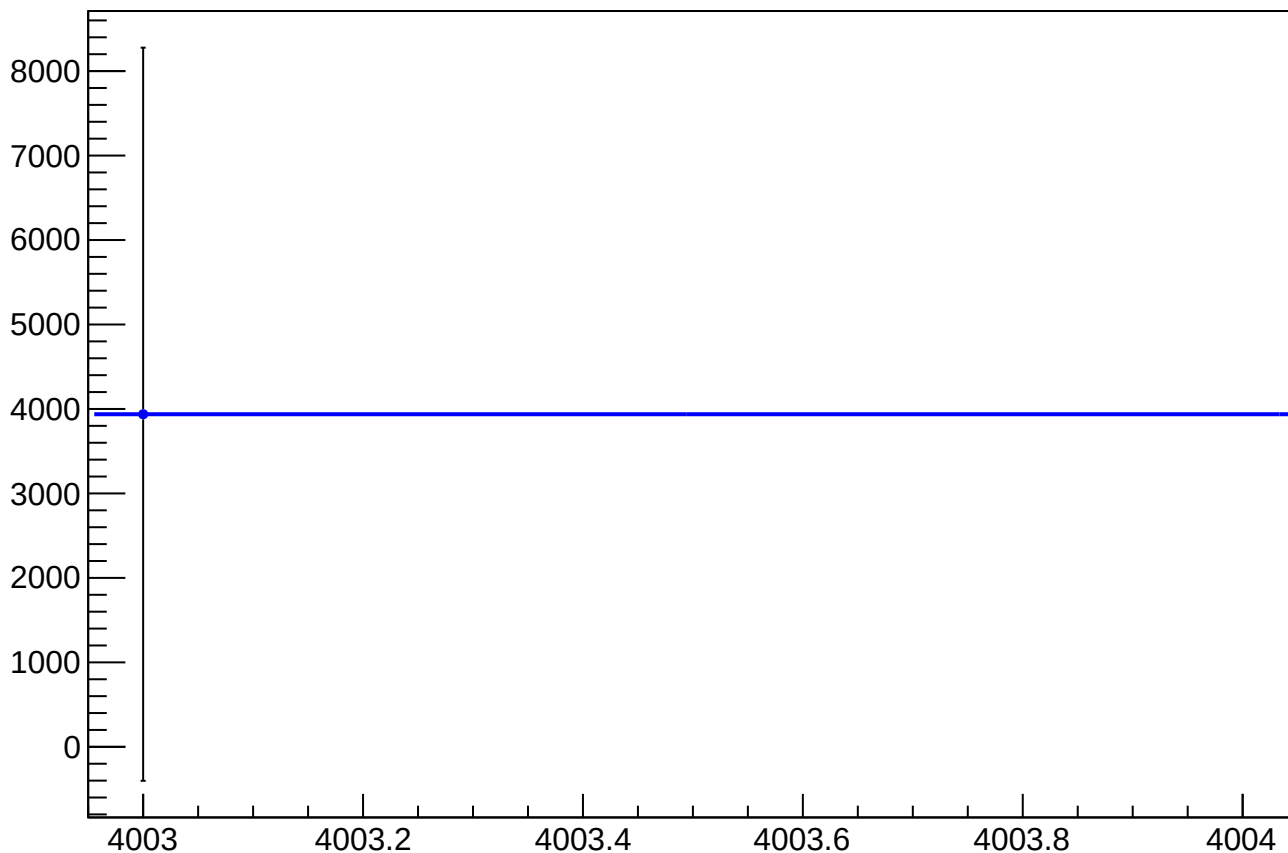
eigen_dit_asym_atl_avg_atr_avg_avg_mean vs Slug, Sign Corrected
