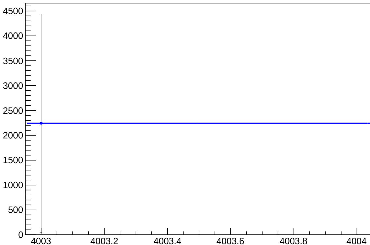
asym_usl_atl1_dd_eigen_cor_correction_mean vs Slug, Sign Corrected
