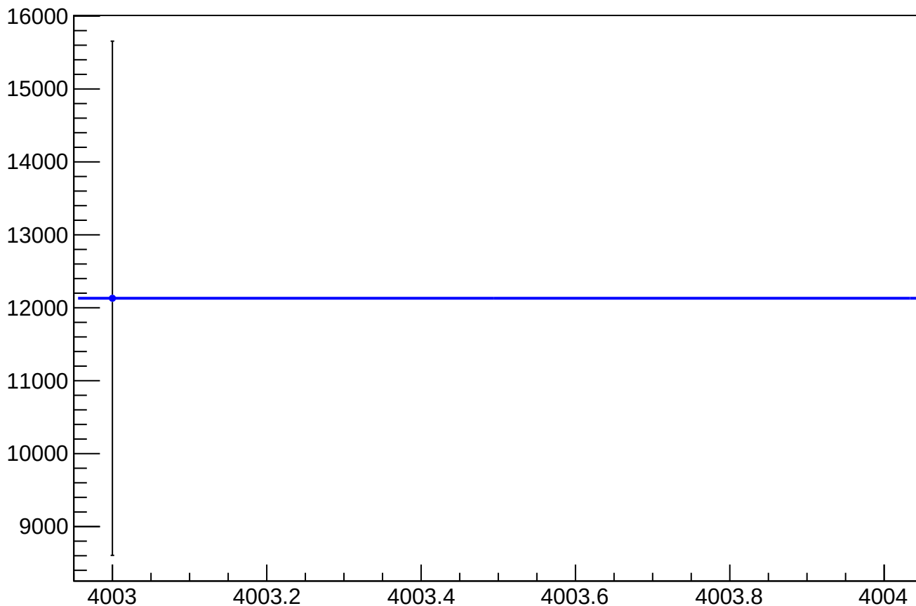
eigen_dit_asym_usr_mean vs Slug, Sign Corrected
