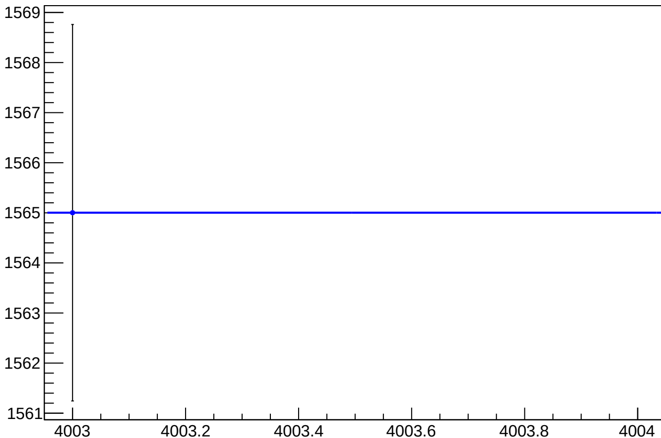
asym_atl1_dit_correction_rms vs Slug, Sign Corrected
