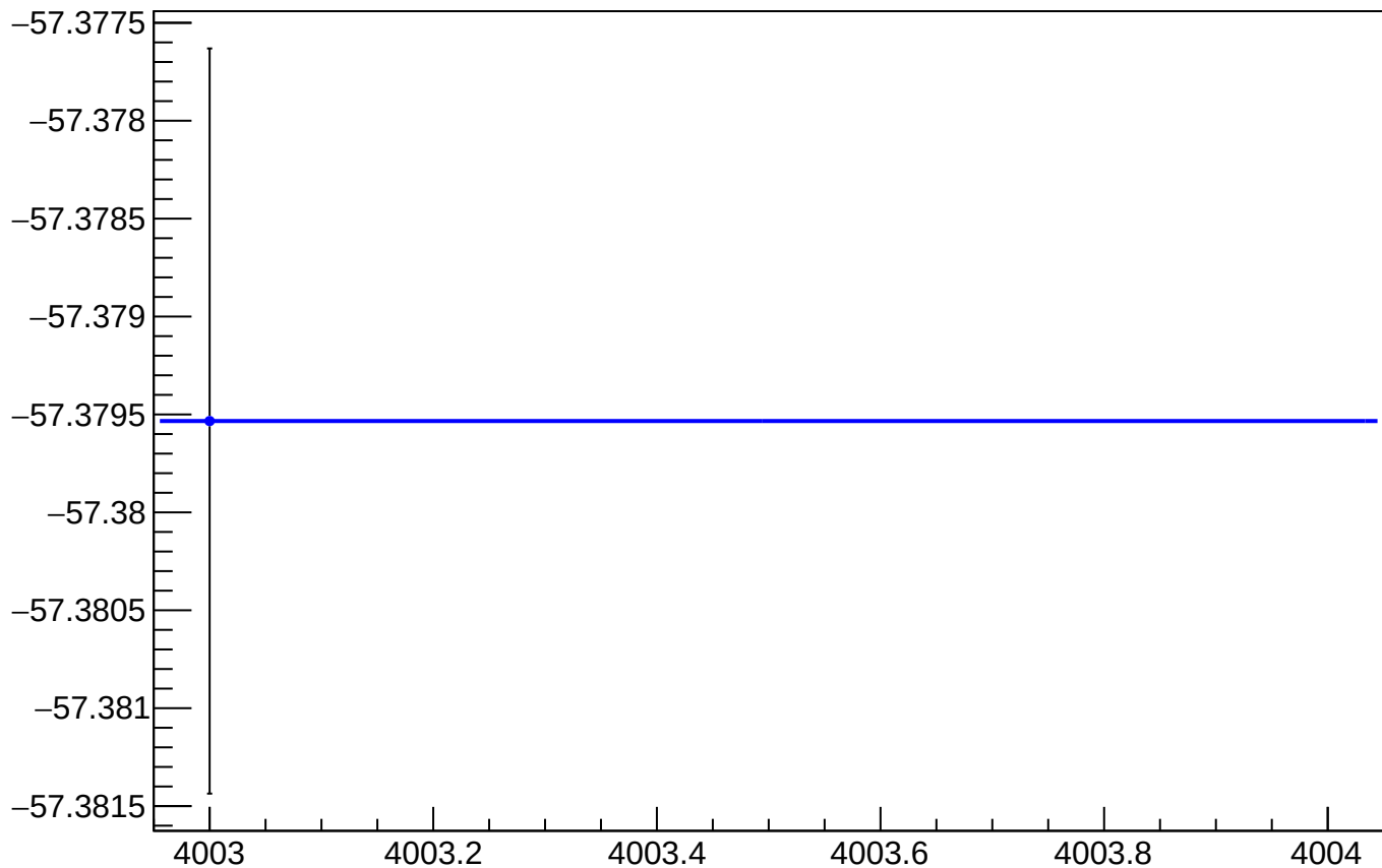
yield_cav4bY_mean vs Slug, Sign Corrected
