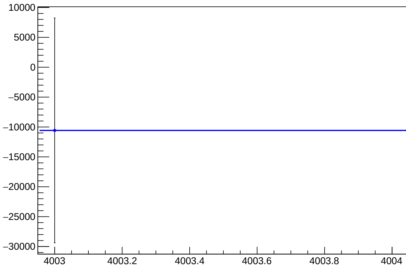
asym_atl1r2_dd_mean vs Slug, Sign Corrected
