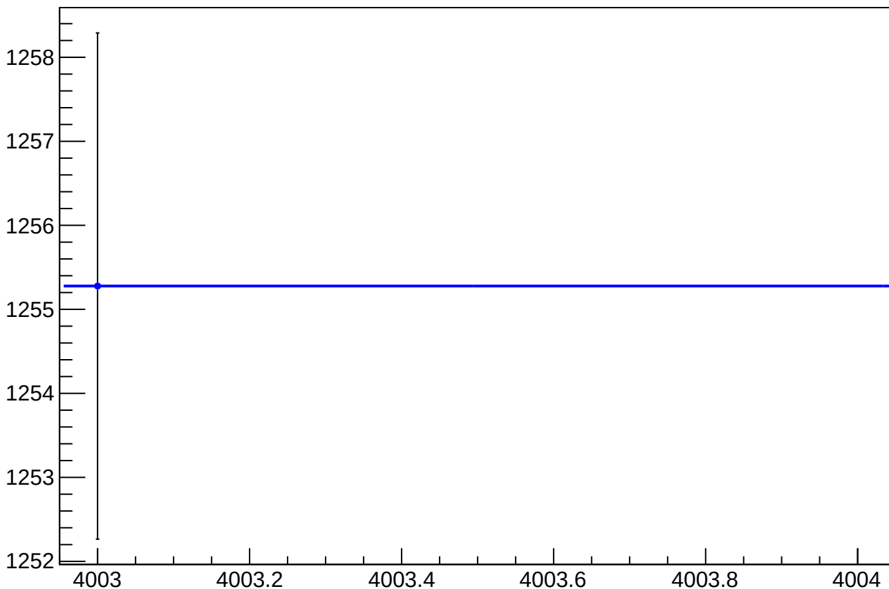
eigen_dit_asym_at1_avg_at2_avg_dd_rms vs Slug, Sign Corrected
