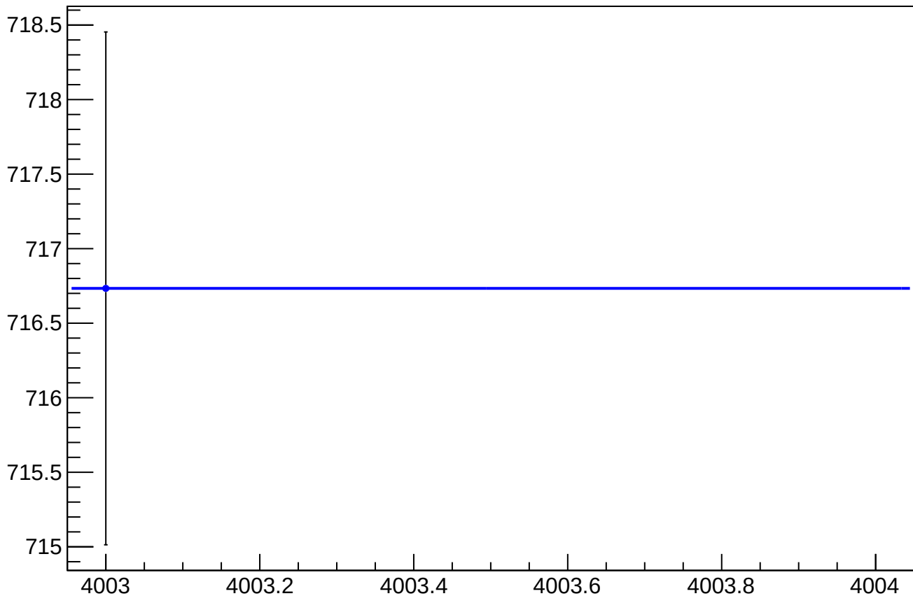
eigen_cor_asym_us_dd_rms vs Slug, Sign Corrected
