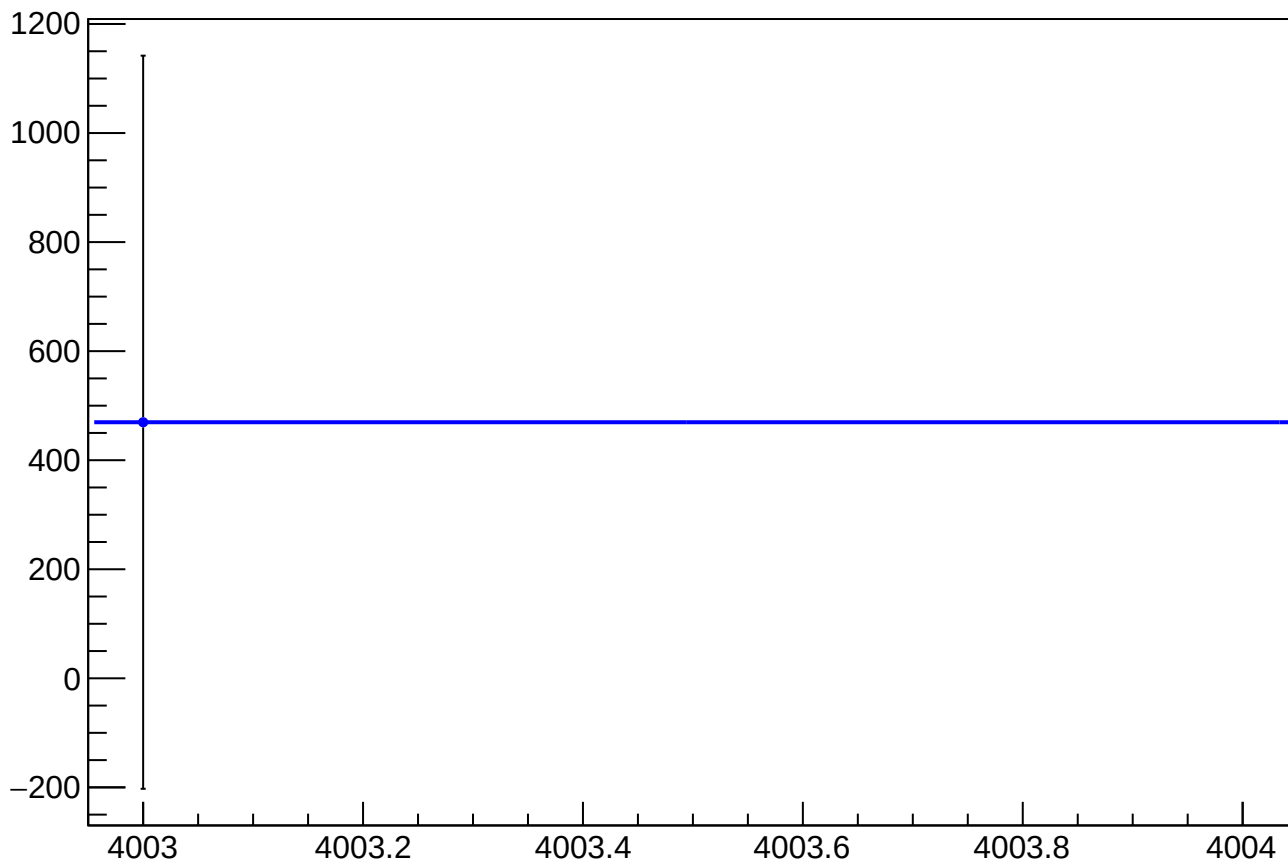
asym_sam8_reg_correction_mean vs Slug, Sign Corrected
