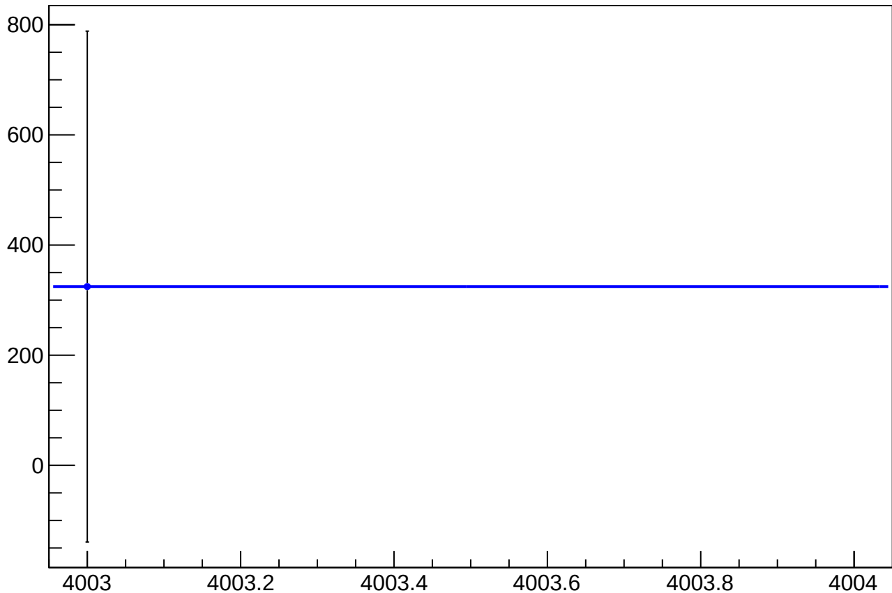
eigen_cor_asym_sam5_mean vs Slug, Sign Corrected
