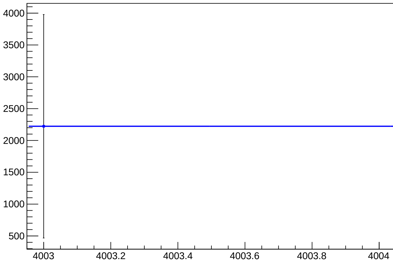
asym_sam_37_avg_eigen_dit_correction_mean vs Slug, Sign Corrected
