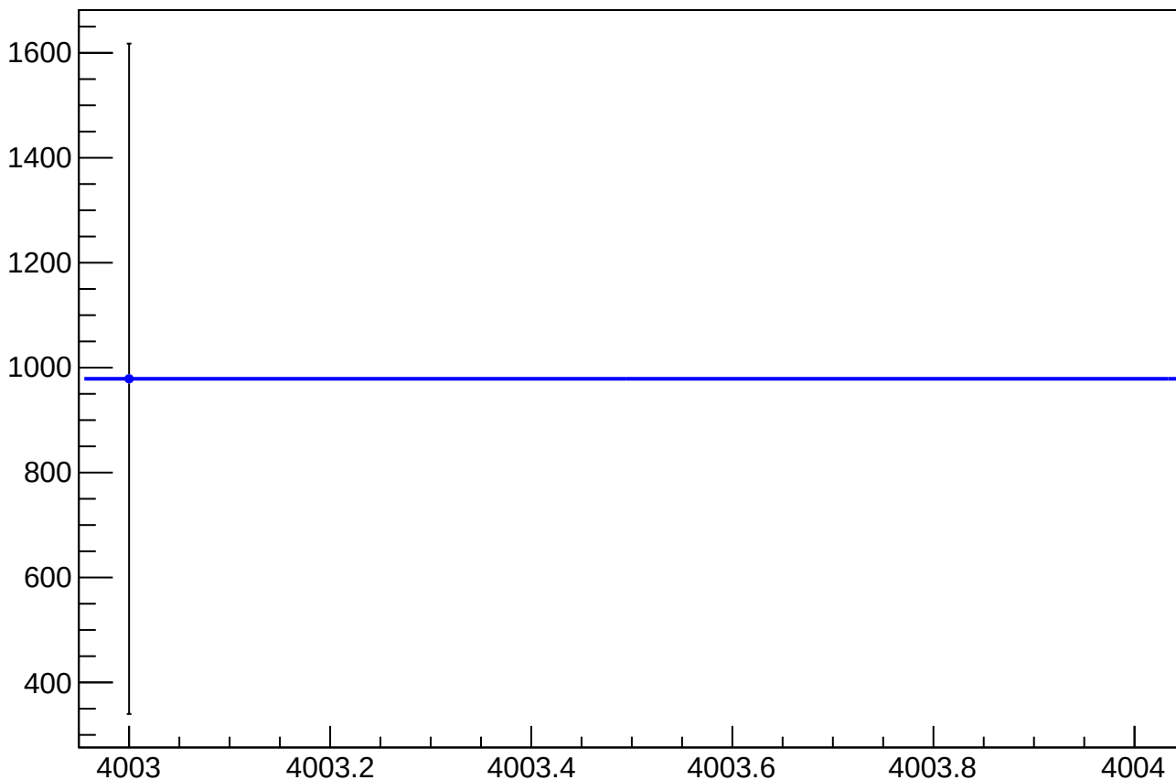
asym_sam7_dit_correction_mean vs Slug, Sign Corrected
