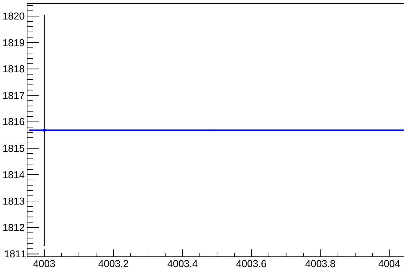
eigen_cor_asym_atr_avg_rms vs Slug, Sign Corrected
