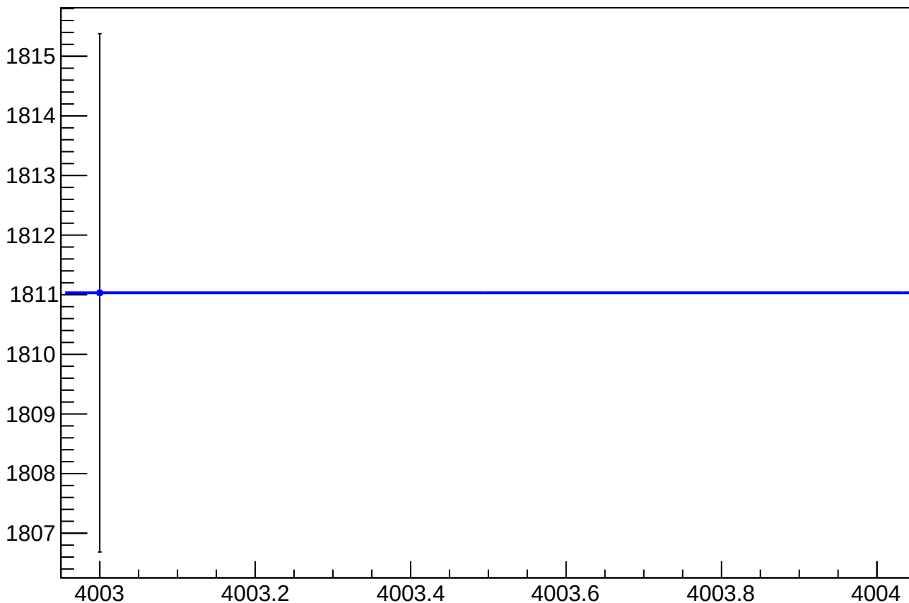
asym_us_dd_atlr_dd_avg_rms vs Slug, Sign Corrected
