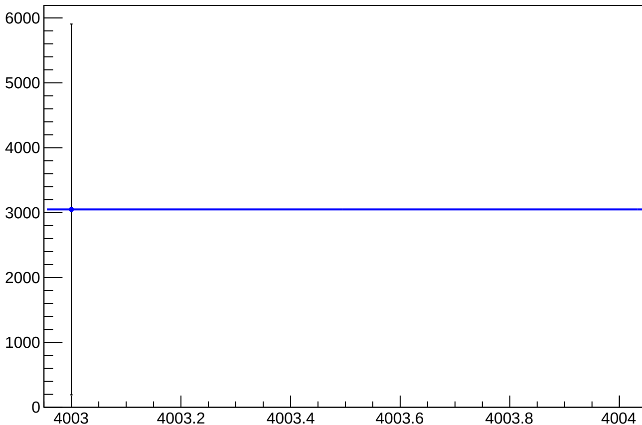
asym_sam_2468_avg_eigen_cor_correction_mean vs Slug, Sign Corrected
