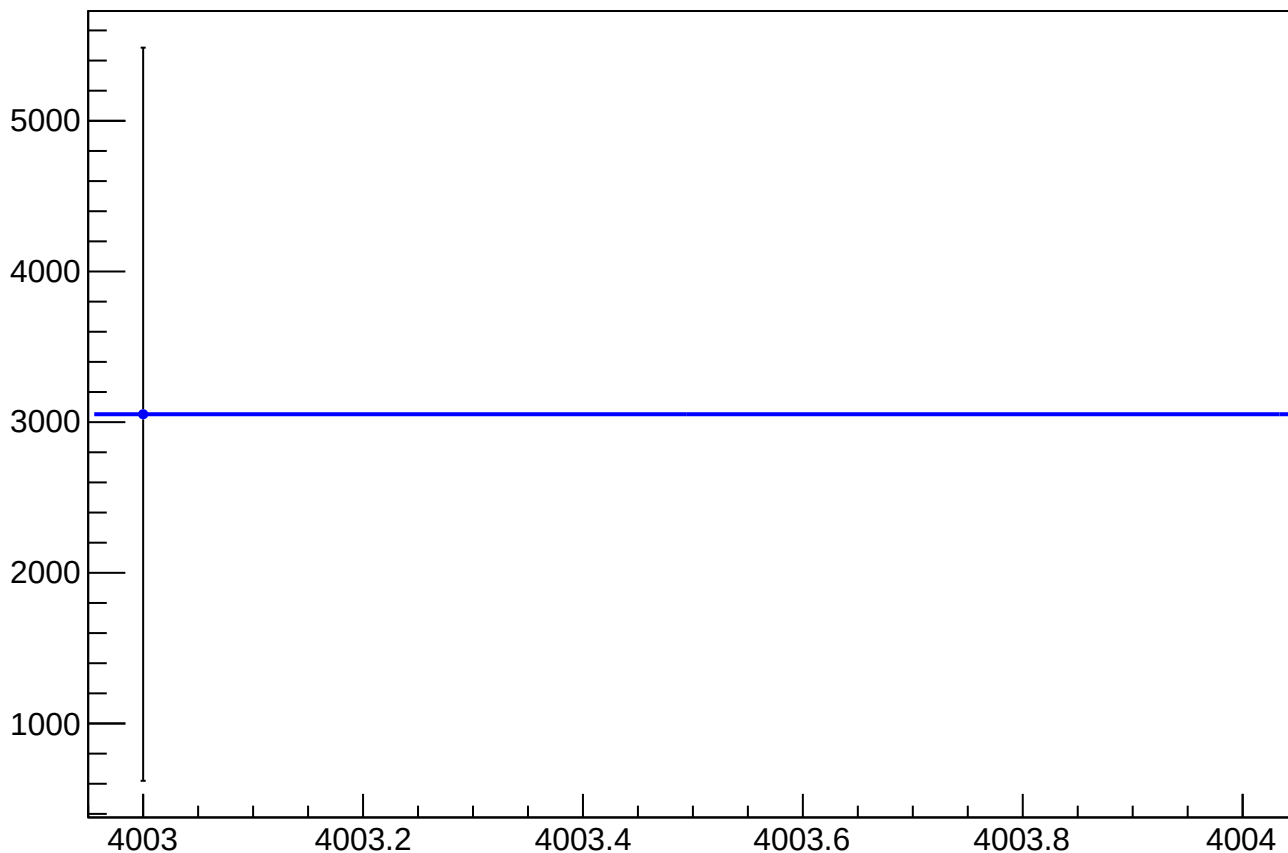
asym_sam_26_avg_reg_correction_mean vs Slug, Sign Corrected
