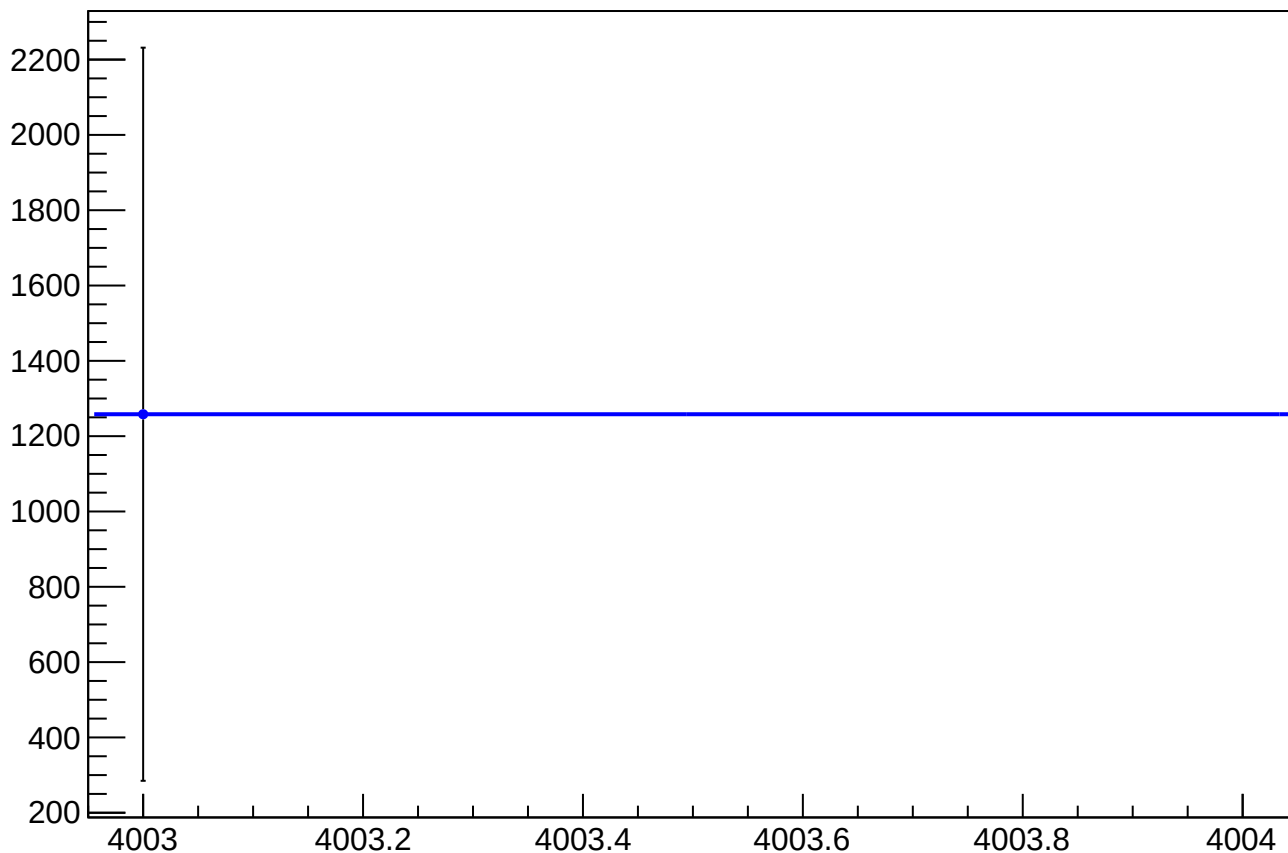
asym_sam_1526_avg_dit_correction_mean vs Slug, Sign Corrected
