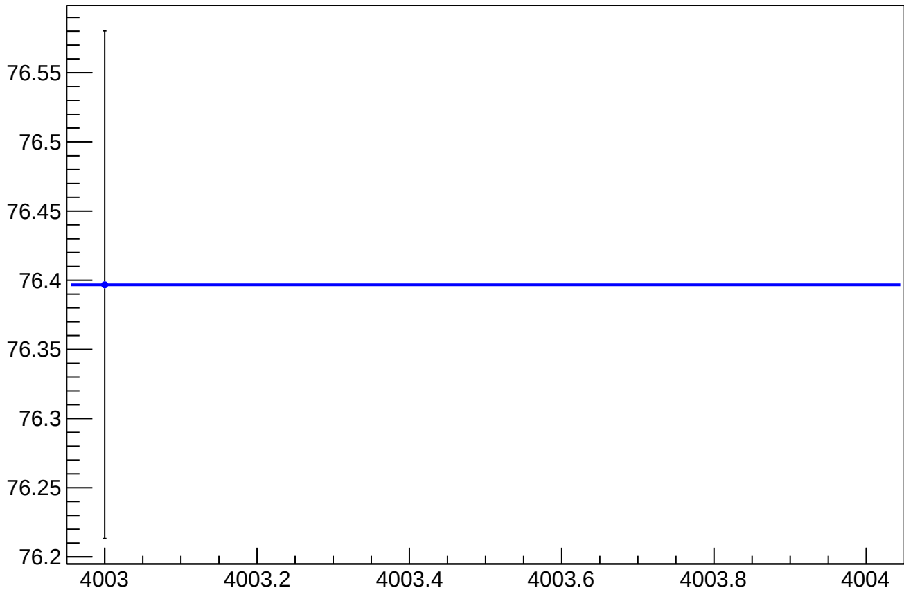
eigen_dit_asym_sam_3726_avg_rms vs Slug, Sign Corrected
