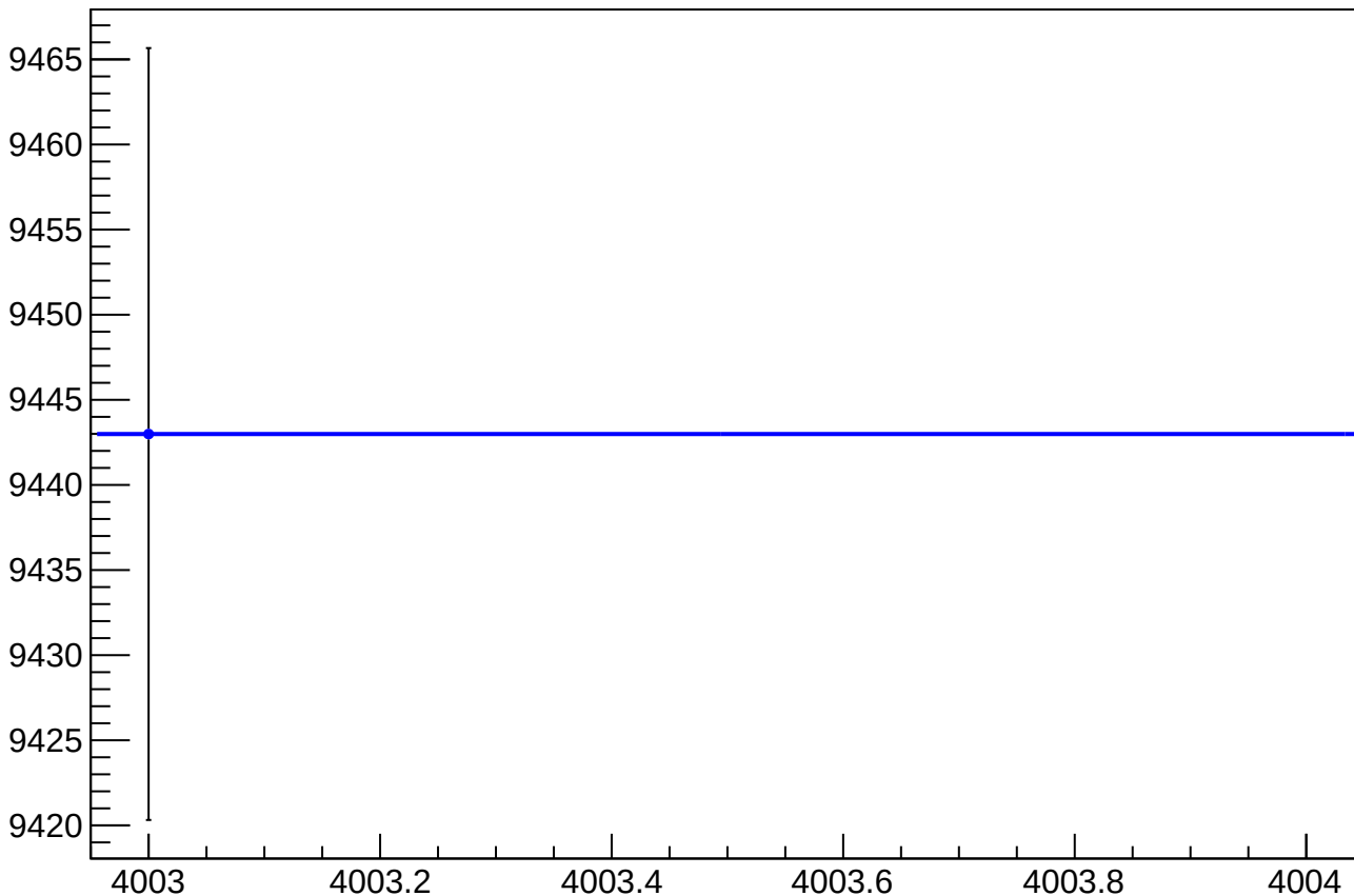
asym_us_avg_atlr_avg_avg_eigen_cor_correction_rms vs Slug, Sign Corrected
