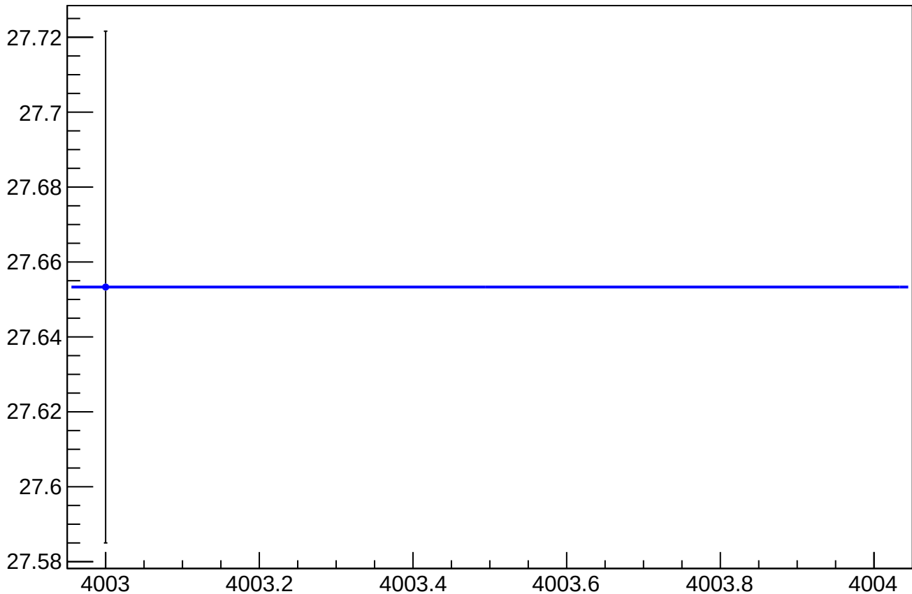
asym_us_dd_eigen_dit_vs_cor_diff_rms vs Slug, Sign Corrected
