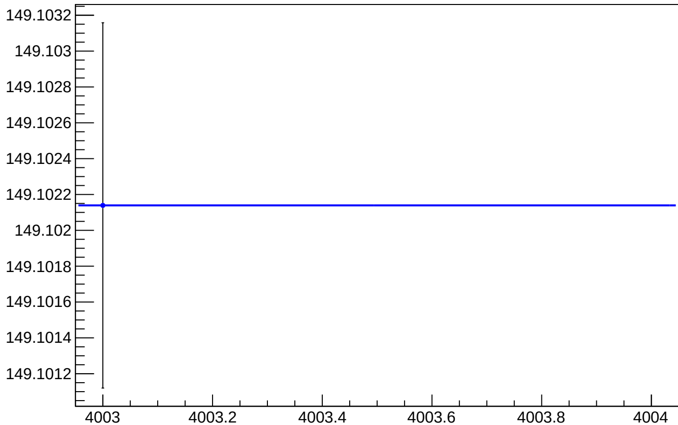
yield_bcm_an_ds3_mean vs Slug, Sign Corrected
