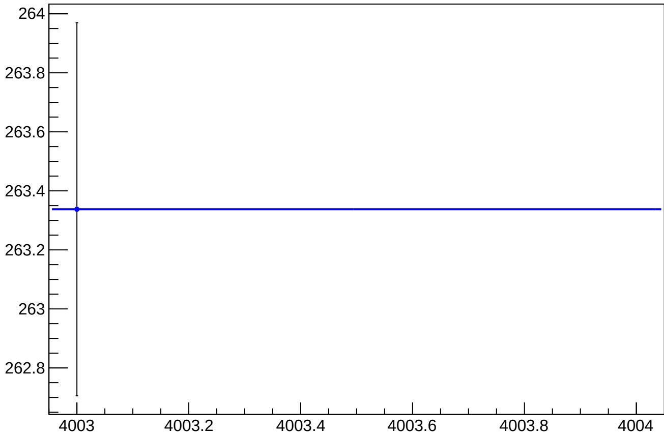
eigen_cor_asym_sam4_rms vs Slug, Sign Corrected
