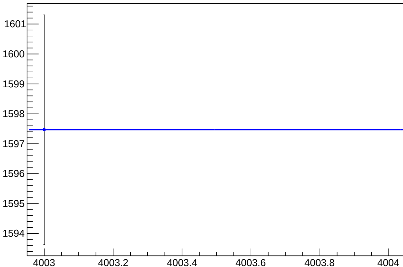
dit_asym_us_avg_at1lr_avg_dd_rms vs Slug, Sign Corrected
