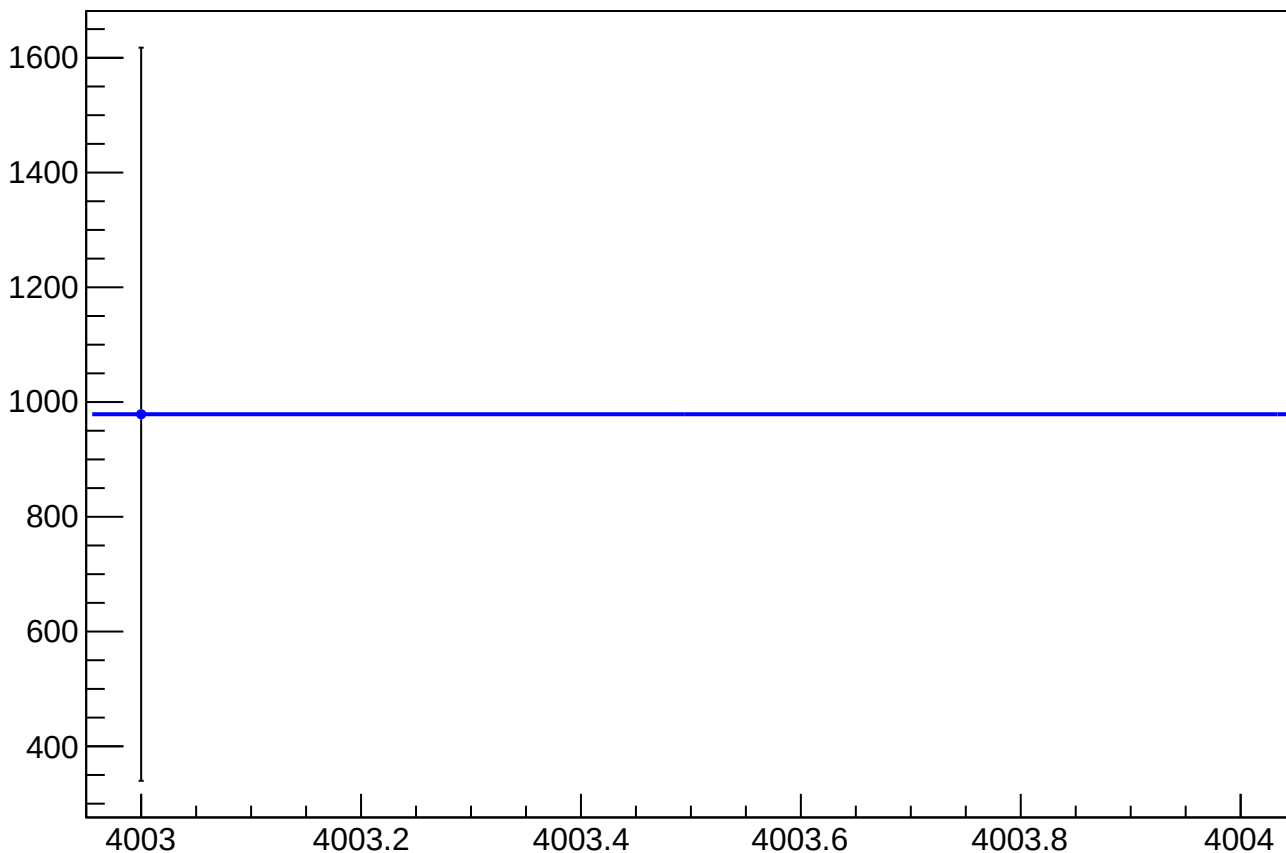
asym_sam7_eigen_dit_correction_mean vs Slug, Sign Corrected
