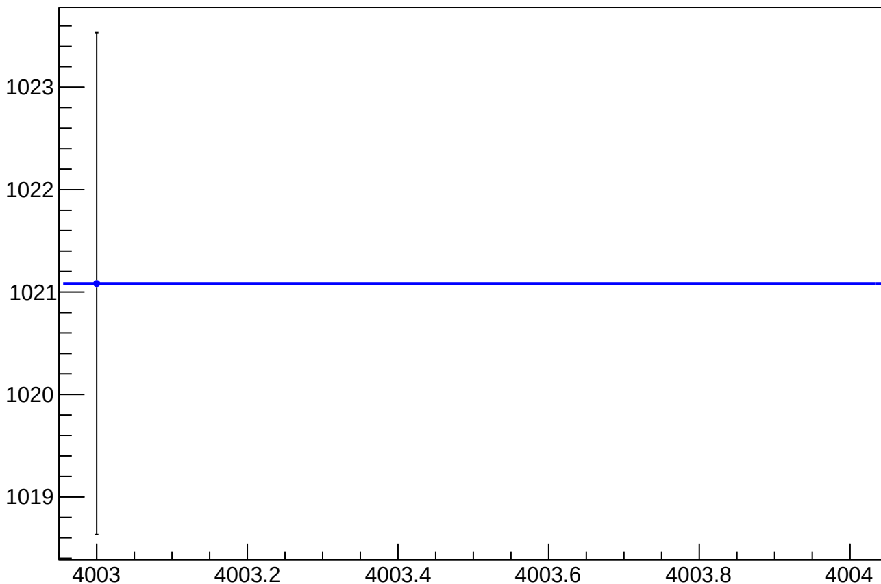
reg_asym_usl_atl1_dd_rms vs Slug, Sign Corrected
