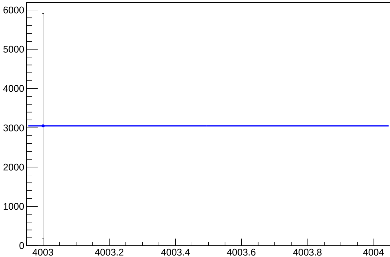
asym_sam_2468_avg_reg_correction_mean vs Slug, Sign Corrected
