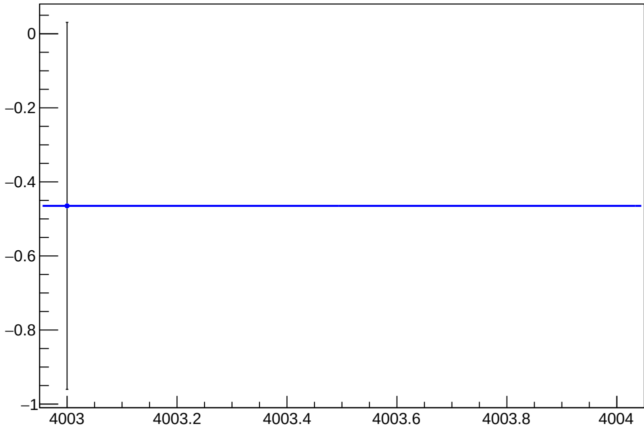
asym_usr_atr1_avg_dit_vs_cor_diff_mean vs Slug, Sign Corrected
