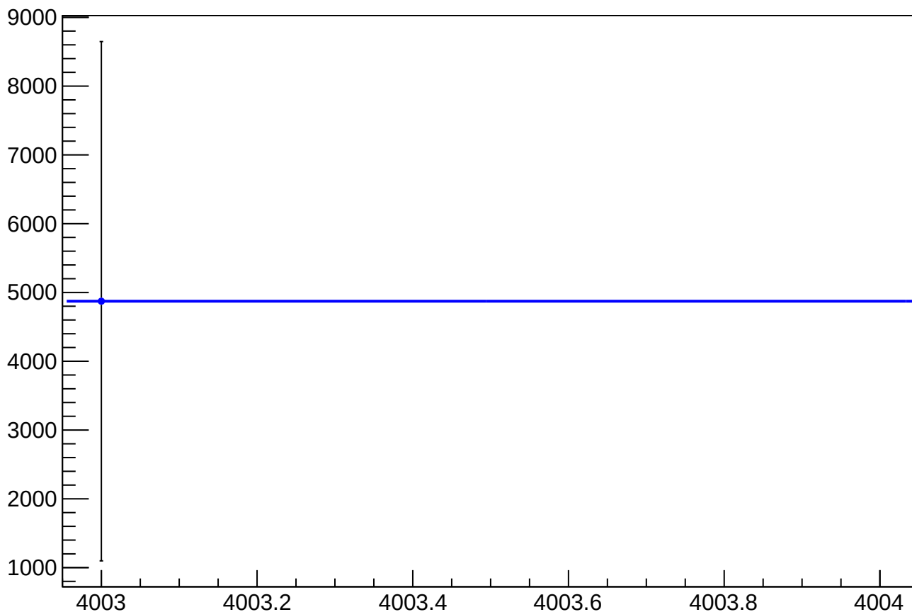
asym_us_dd_at1lr_dd_dd_reg_correction_mean vs Slug, Sign Corrected
