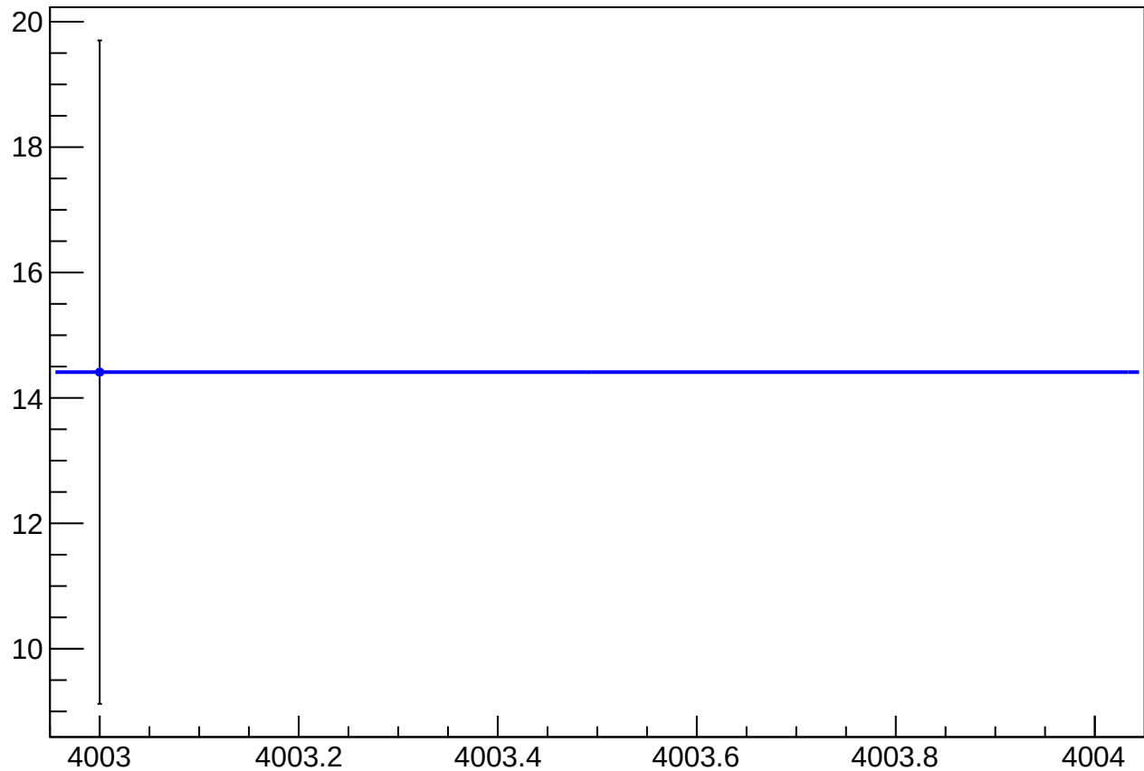
reg_asym_us_dd_at1lr_dd_avg_diff_bpm4eY_slope vs Slug, Sign Corrected
