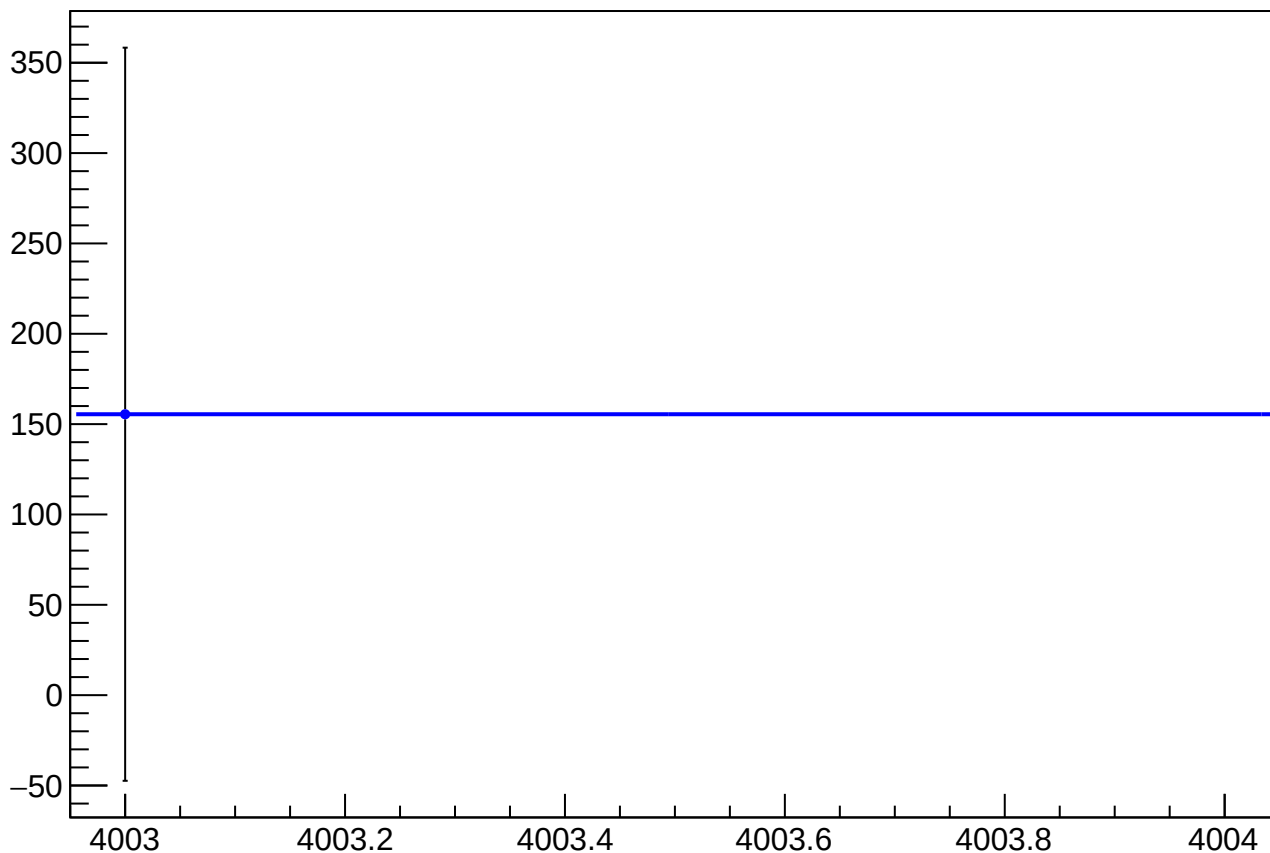
eigen_cor_asym_sam_12345678_avg_mean vs Slug, Sign Corrected
