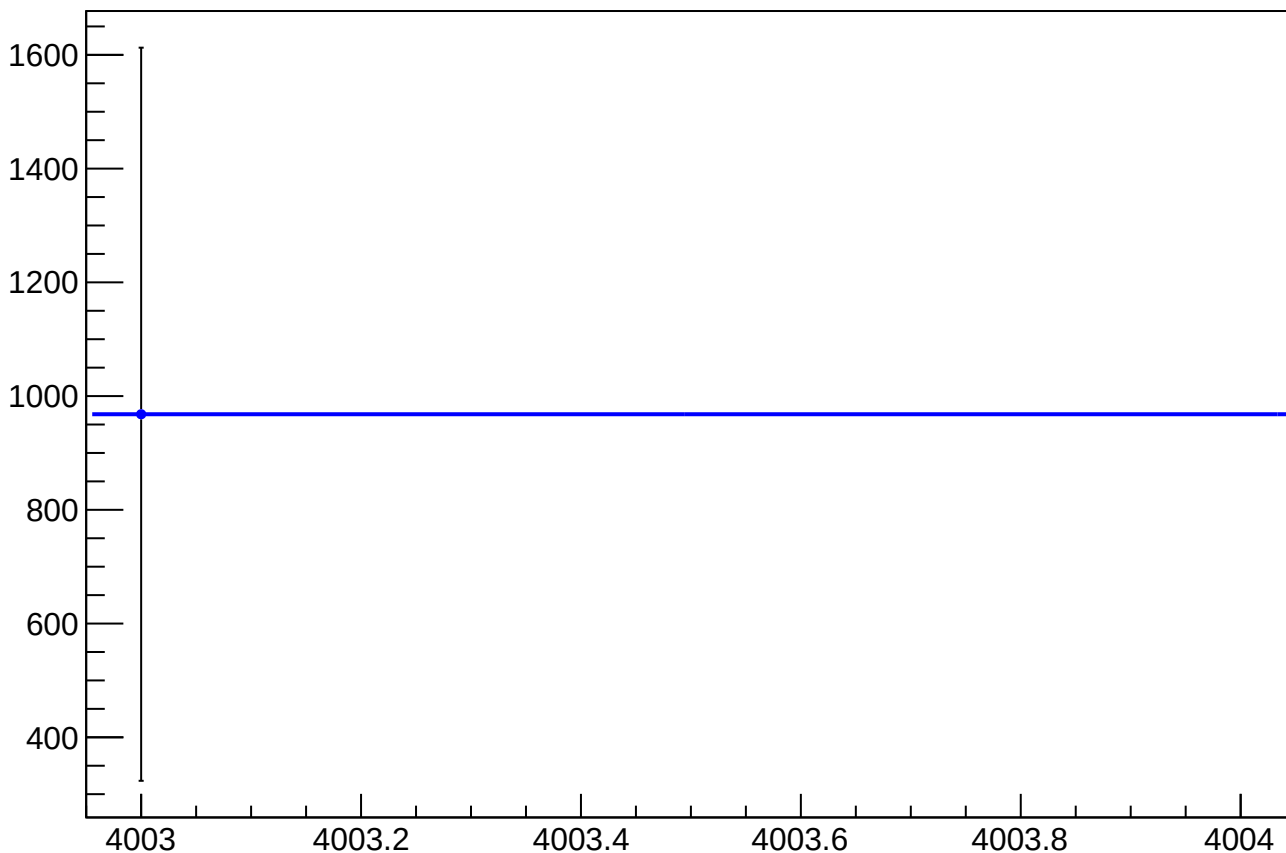
asym_sam7_eigen_cor_correction_mean vs Slug, Sign Corrected
