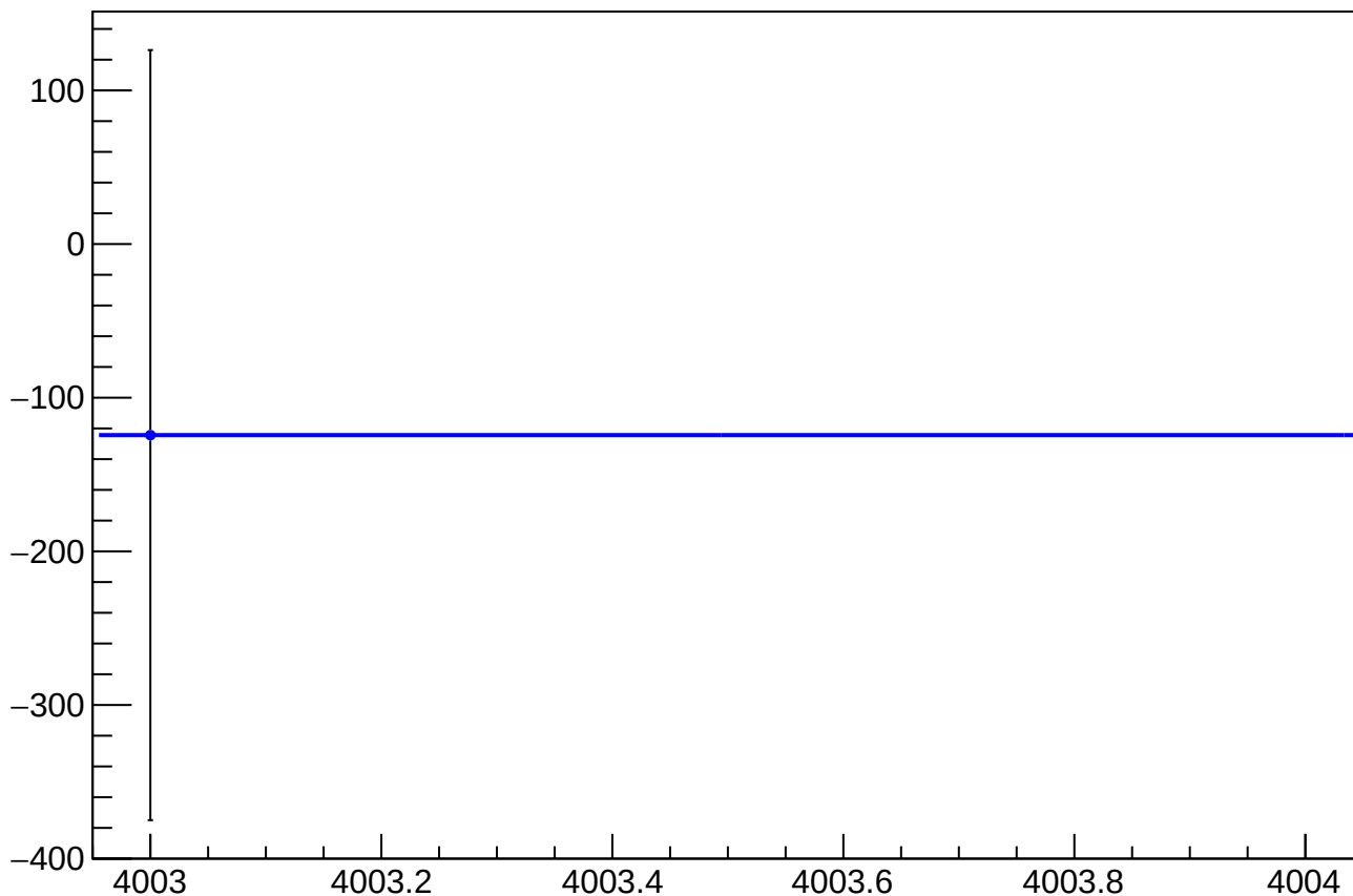
eigen_dit_asym_sam_37_48_dd_mean vs Slug, Sign Corrected
