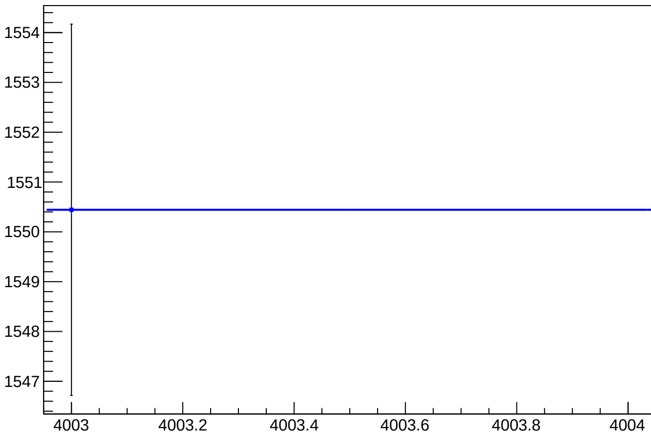
asym_atl1_eigen_cor_correction_rms vs Slug, Sign Corrected
