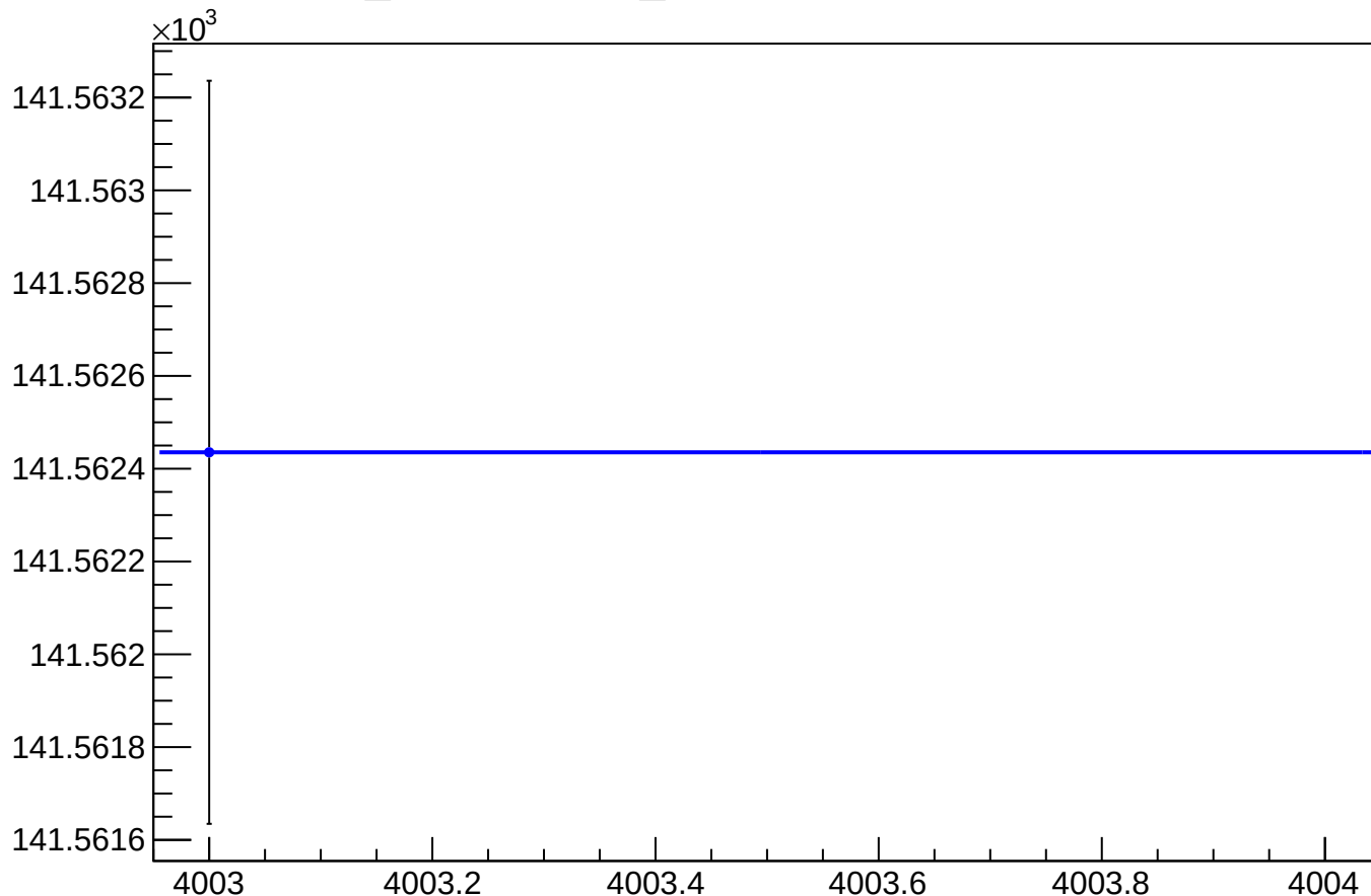
yield_bpm0r03WS_mean vs Slug, Sign Corrected
