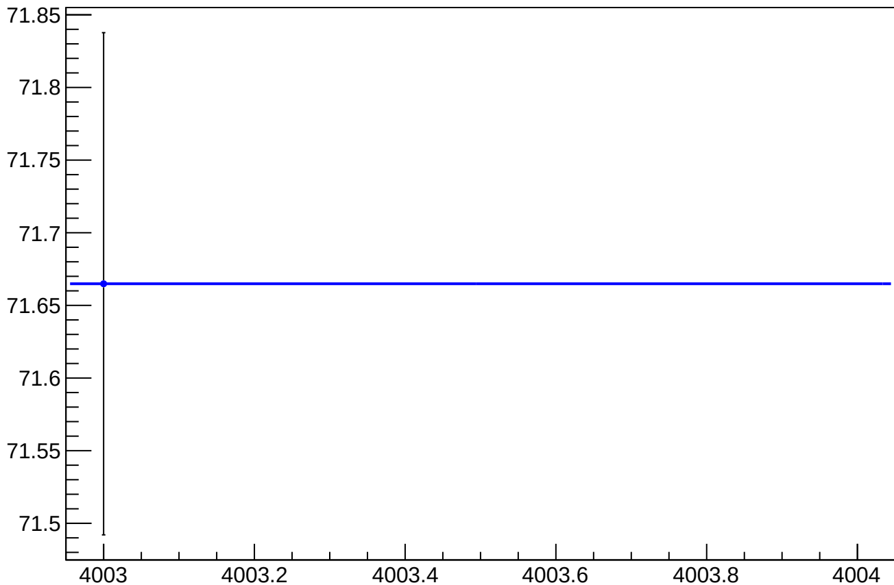
asym_sam4_eigen_dit_vs_cor_diff_rms vs Slug, Sign Corrected
