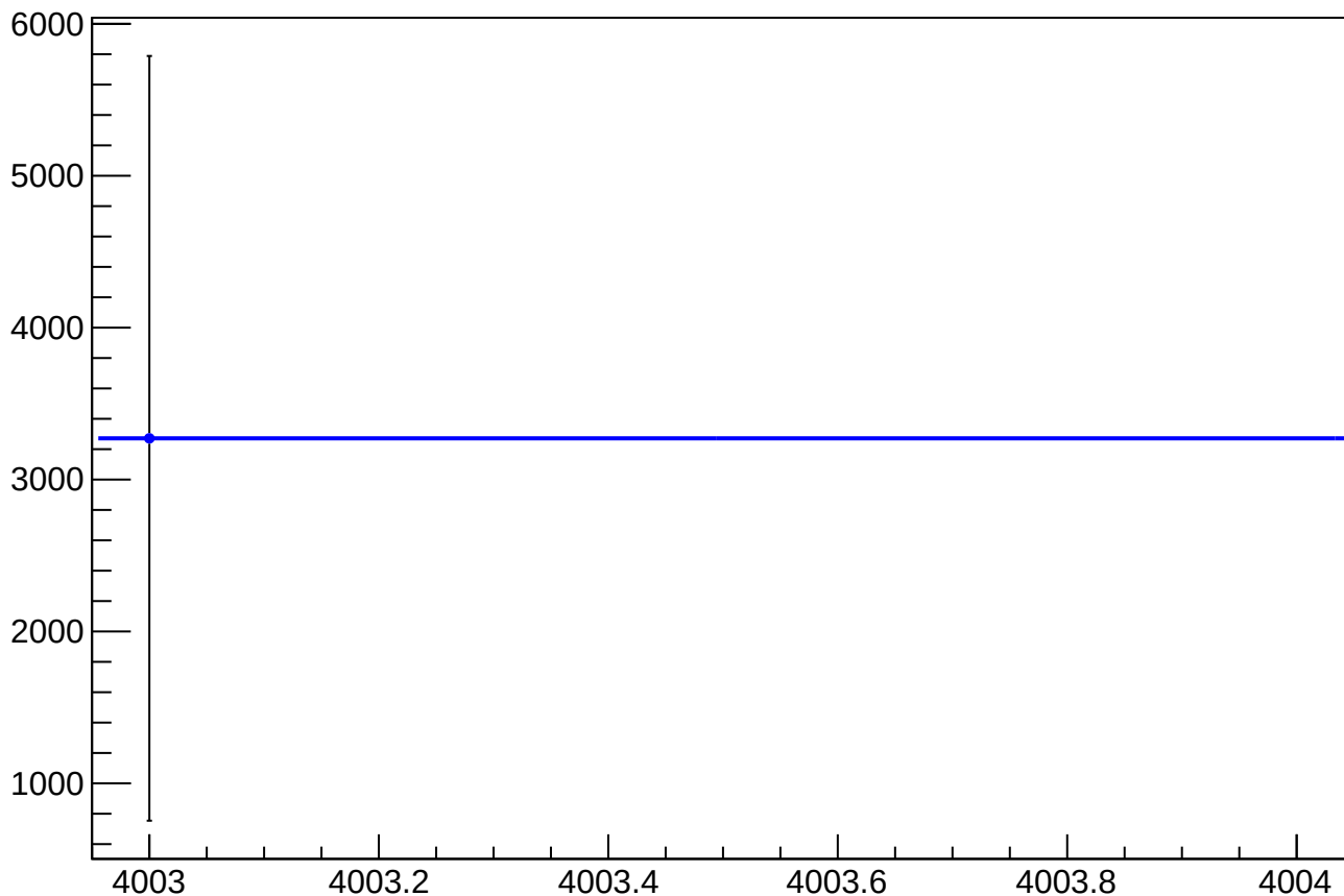
asym_sam_26_avg_dit_correction_mean vs Slug, Sign Corrected
