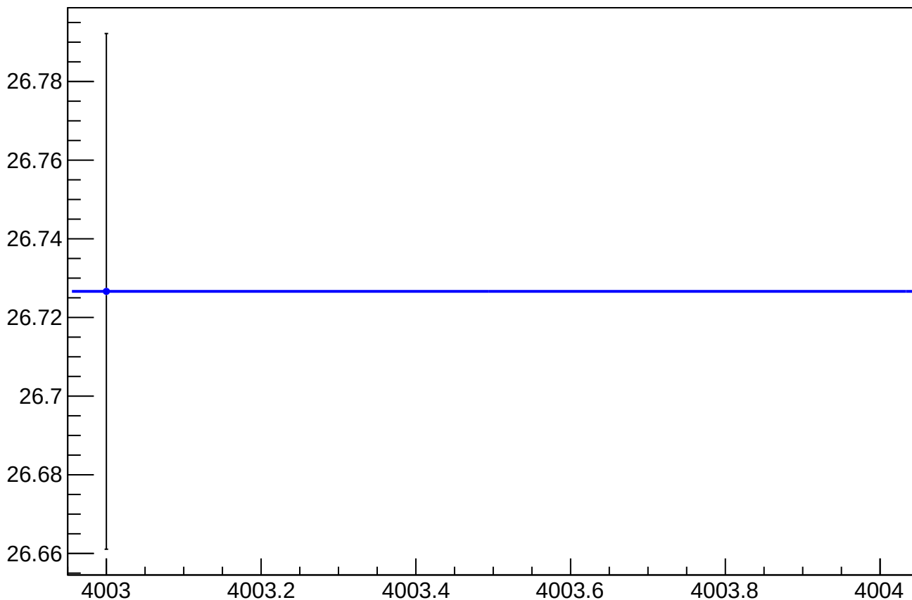
asym_sam_37_dd_dit_vs_slug, Sign Corrected
