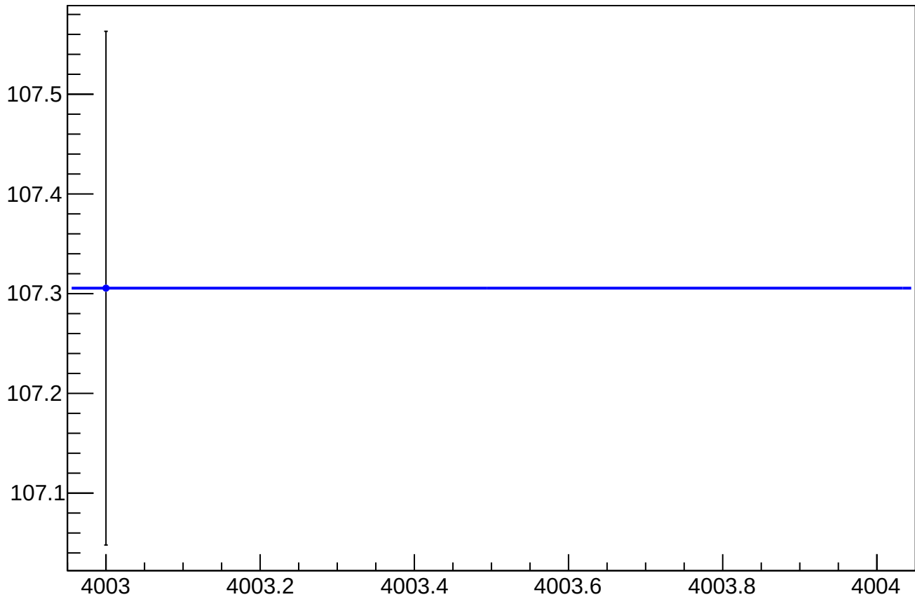
eigen_dit_asym_sam_26_avg_rms vs Slug, Sign Corrected
