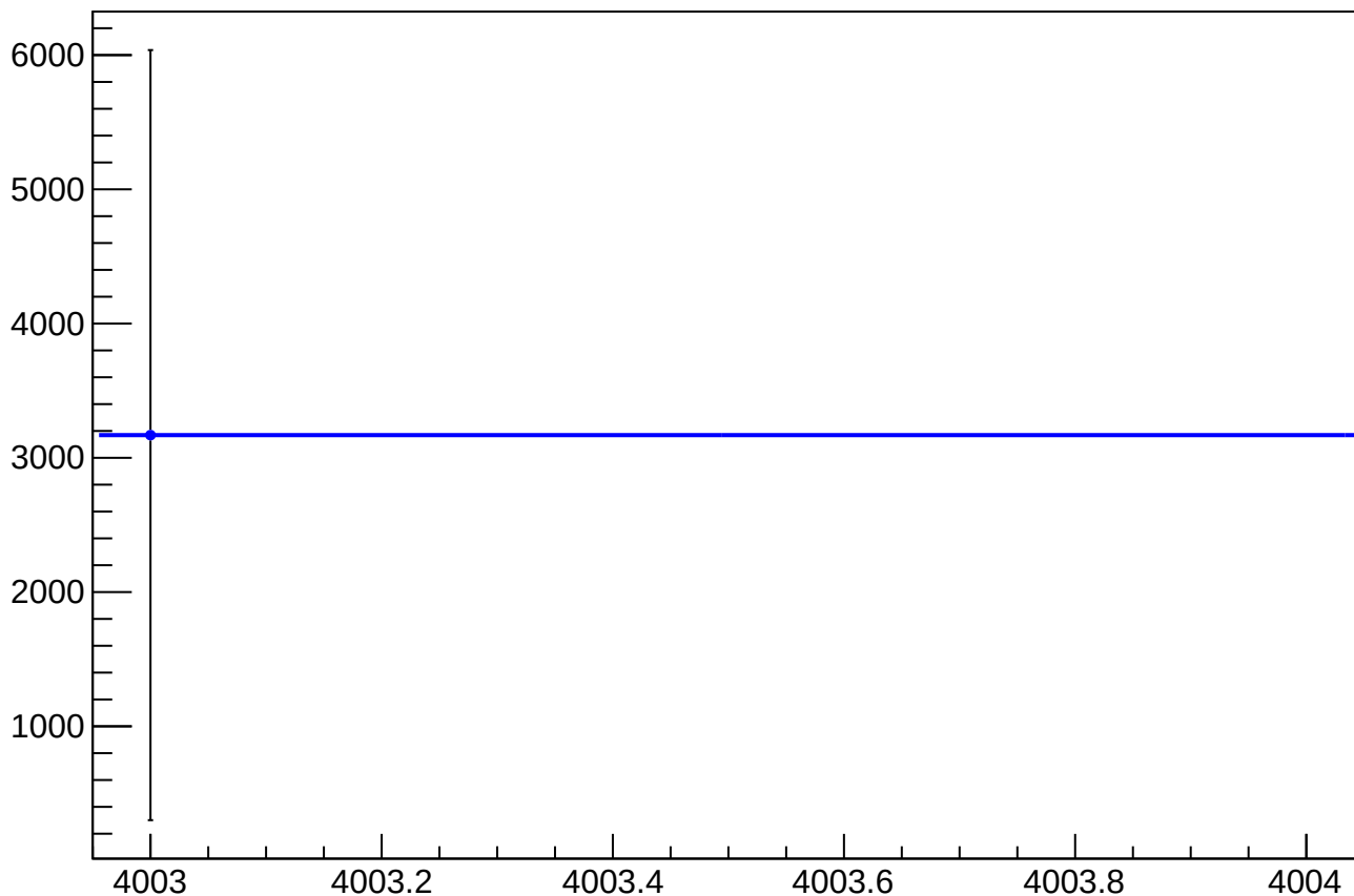
asym_sam_2468_avg_eigen_dit_correction_mean vs Slug, Sign Corrected
