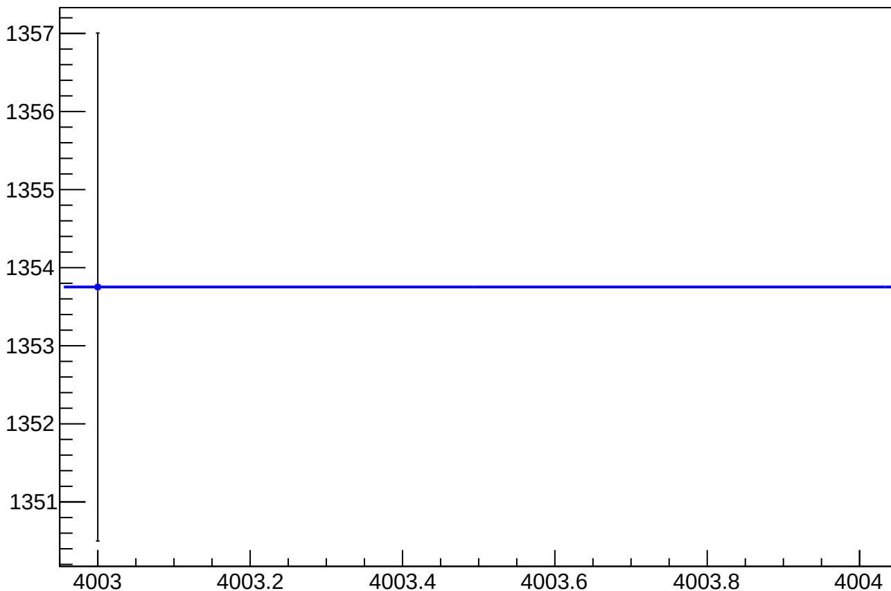
asym_us_dd_at2lr_dd_avg_eigen_dit_correction_rms vs Slug, Sign Corrected
