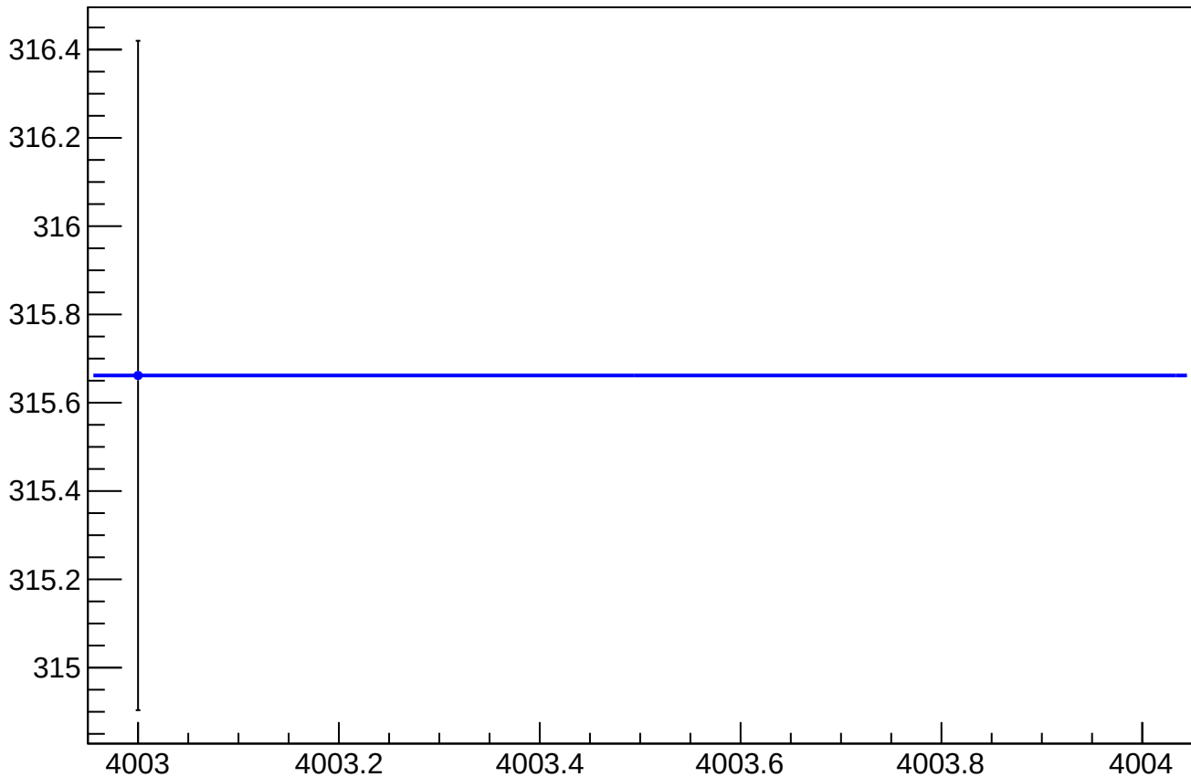
asym_sam_1357_avg_cor_correction_rms vs Slug, Sign Corrected
