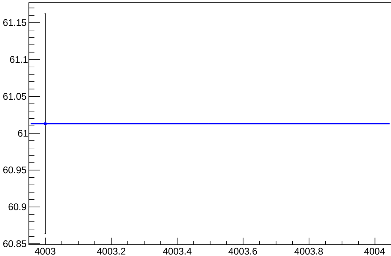
asym_sam3_dit_vs_eigen_cor_diff_rms vs Slug, Sign Corrected
