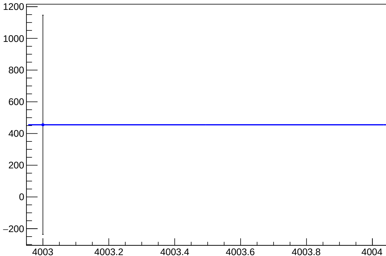
asym_sam8_eigen_dit_correction_mean vs Slug, Sign Corrected
