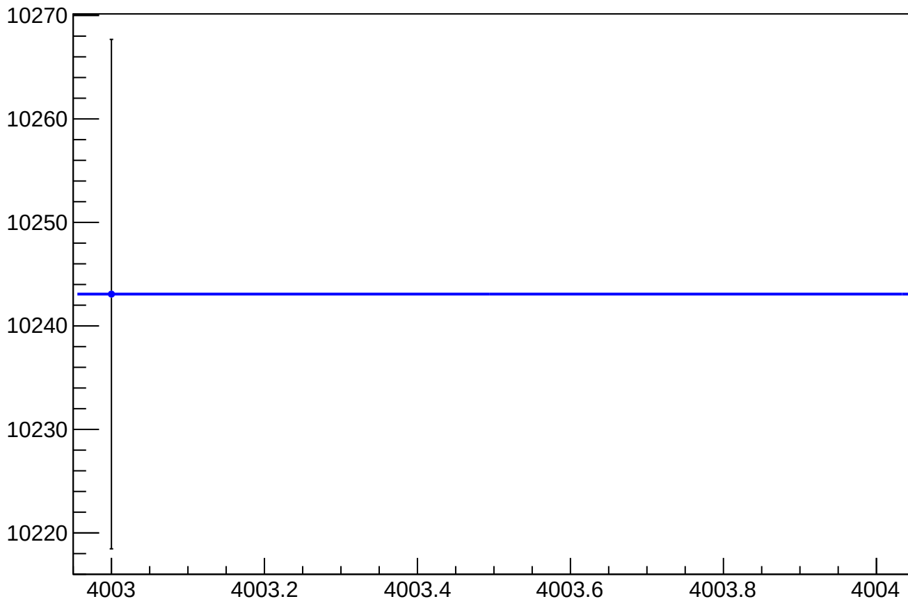
diff_bpm_4aX_4acX_avg_rms vs Slug, Sign Corrected
