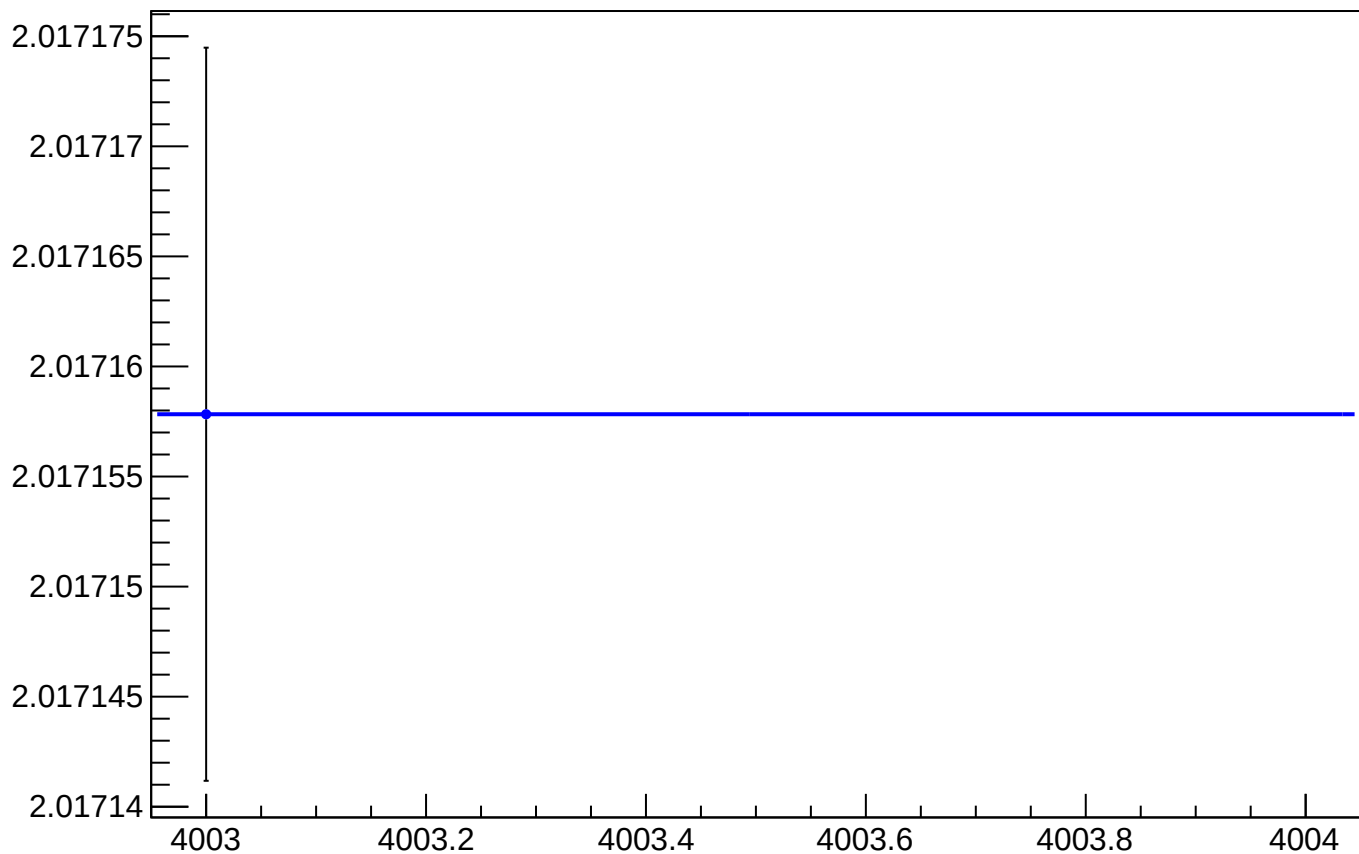
yield_bpm0i01aY_mean vs Slug, Sign Corrected
