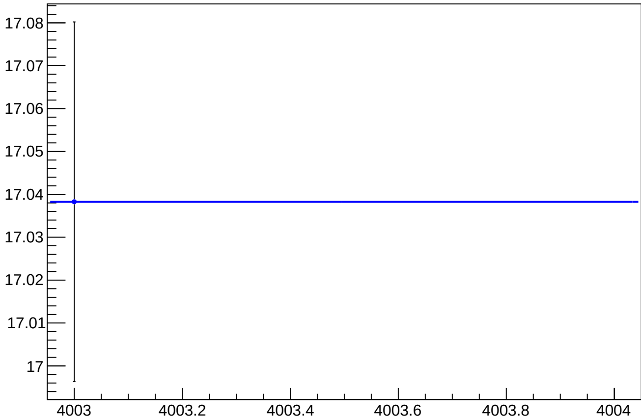
asym_sam_1357_avg_eigen_dit_vs_cor_diff_rms vs Slug, Sign Corrected
