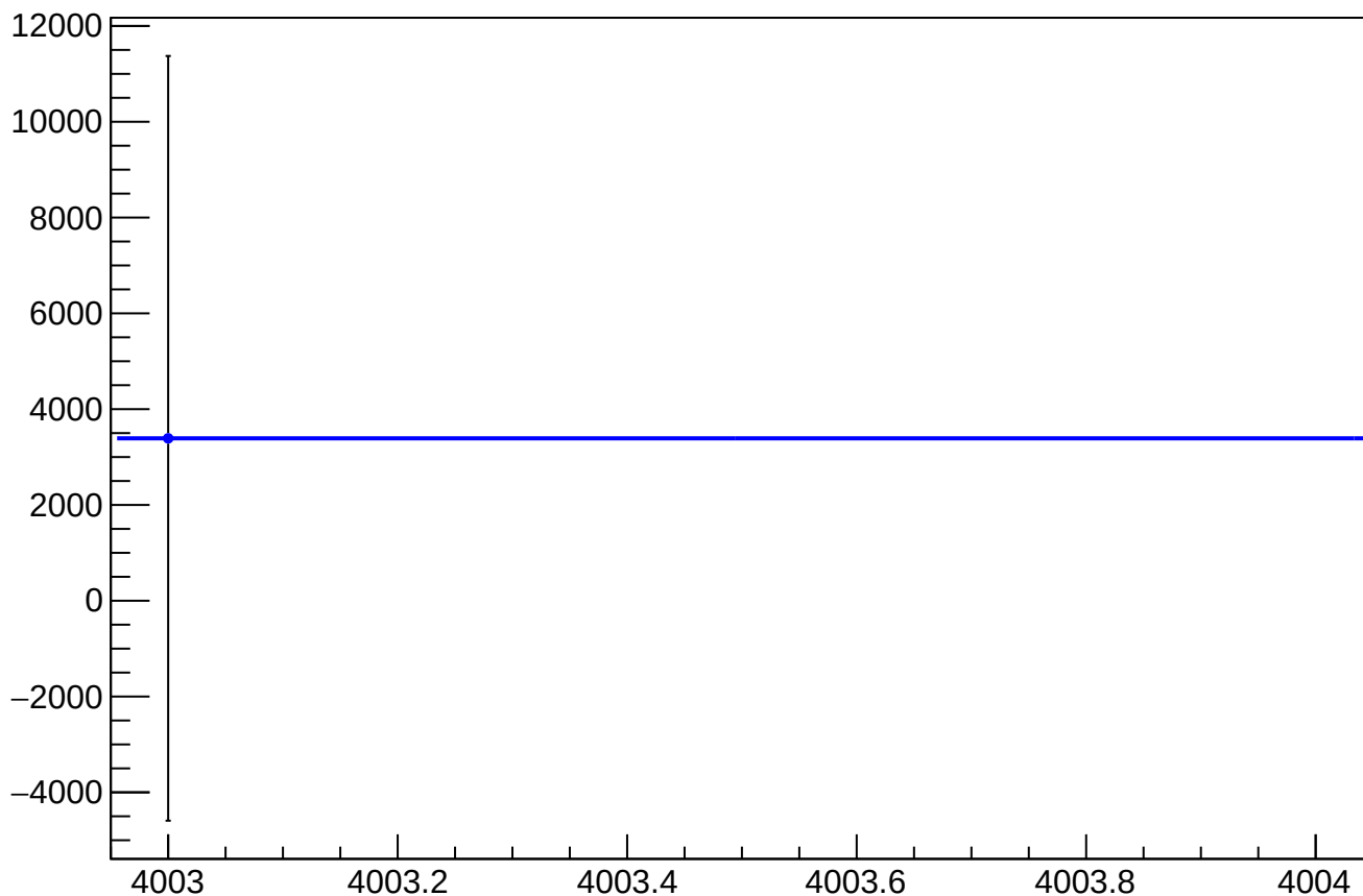
asym_usl_dit_correction_mean vs Slug, Sign Corrected
