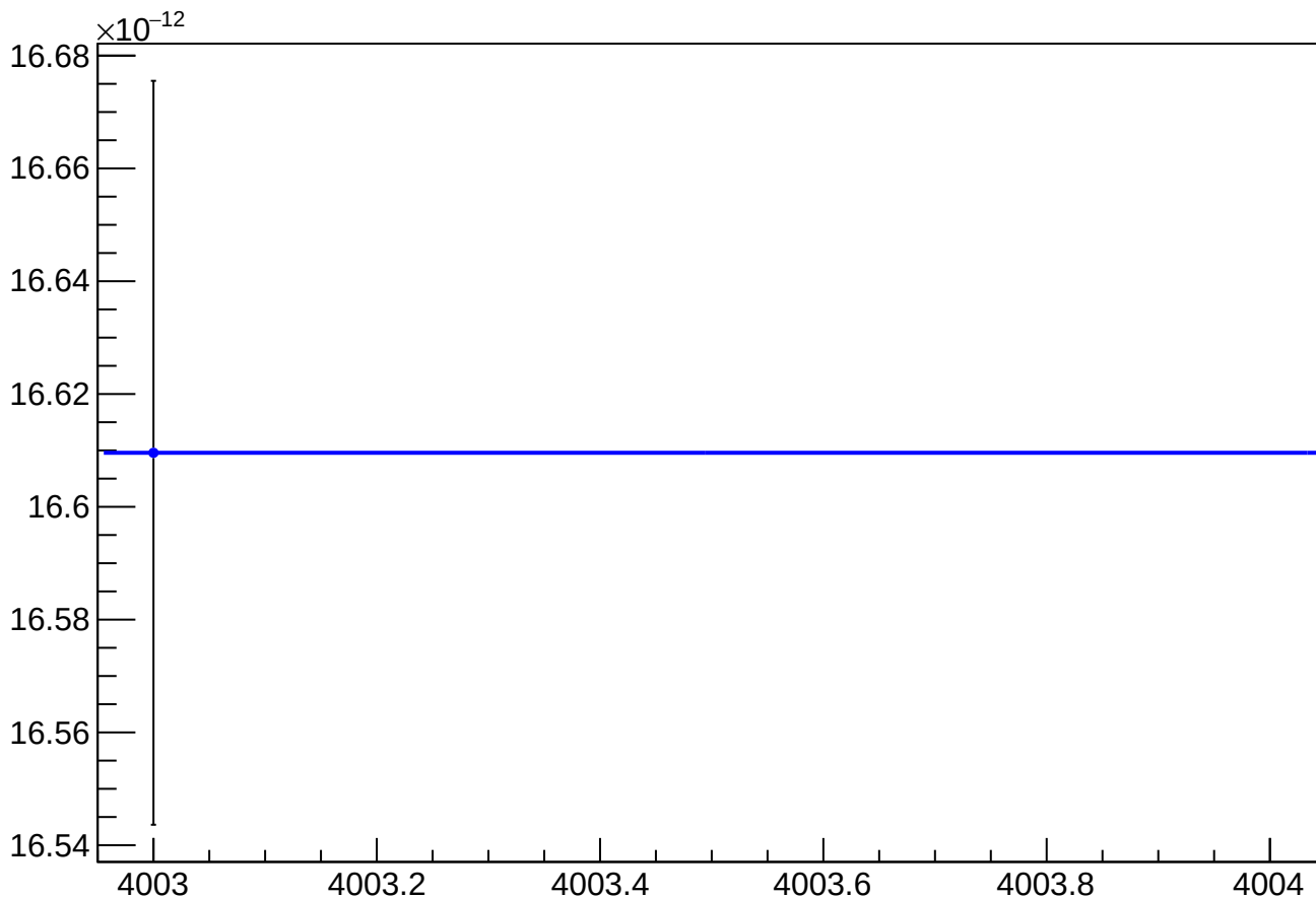
asym_sam8_reg_vs_cor_diff_rms vs Slug, Sign Corrected
