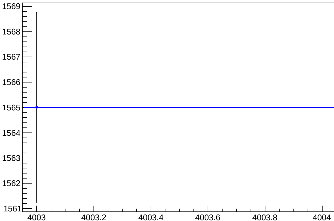
asym_atl1_eigen_dit_correction_rms vs Slug, Sign Corrected
