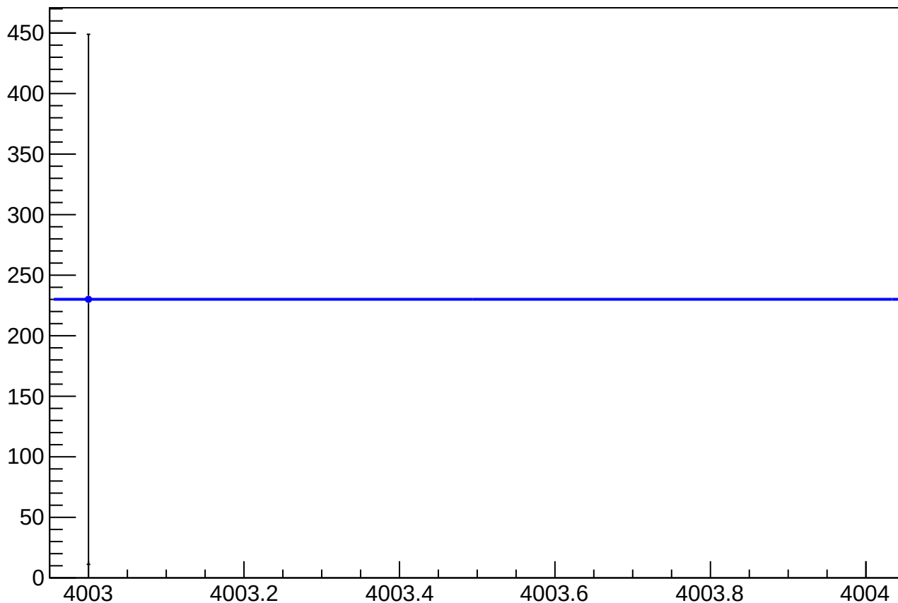
eigen_dit_asym_sam_12345678_avg_mean vs Slug, Sign Corrected
