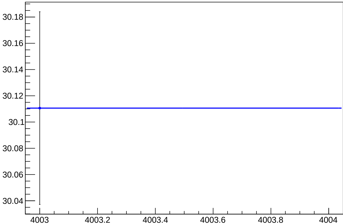
asym_us_dd_overload_cor_vs_cor_diff_rms vs Slug, Sign Corrected
