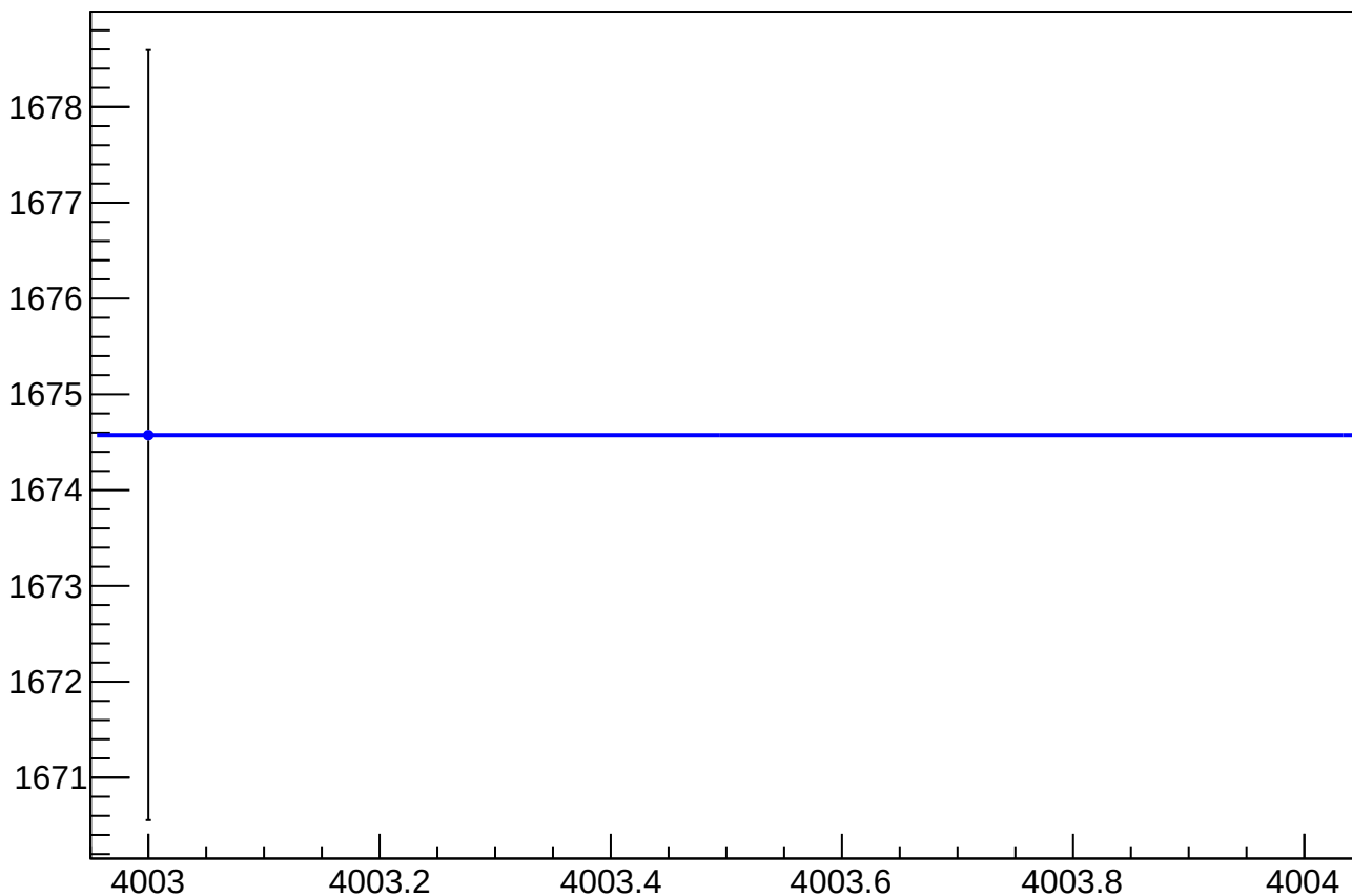
eigen_cor_asym_us_dd_atlr_dd_avg_rms vs Slug, Sign Corrected
