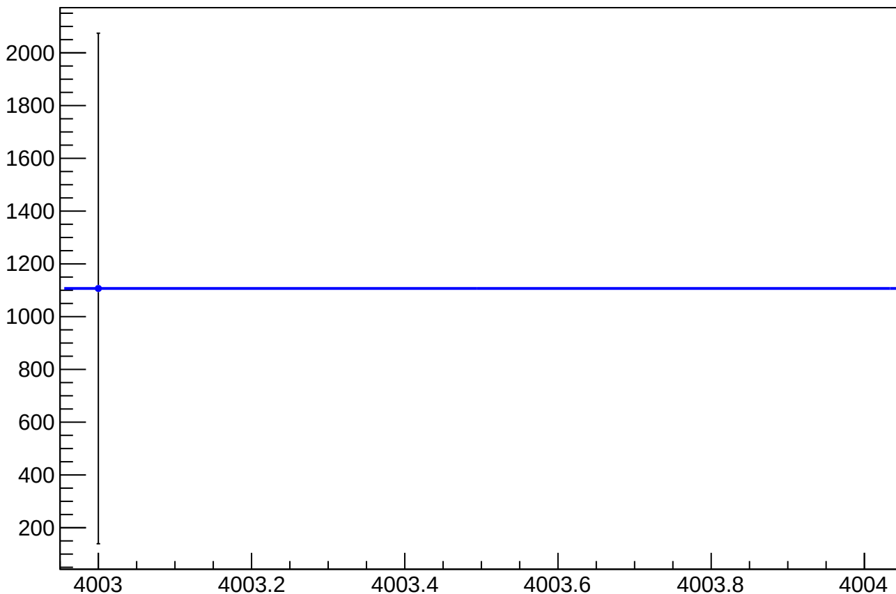
asym_sam_1357_2468_dd_mean vs Slug, Sign Corrected
