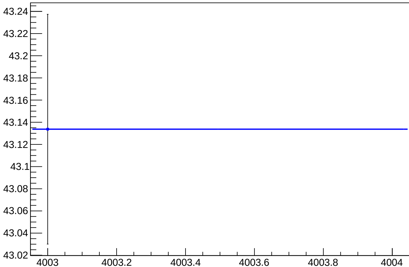
asym_sam_24_68_dd_eigen_dit_vs_eigen_cor_diff_rms vs Slug, Sign Corrected
