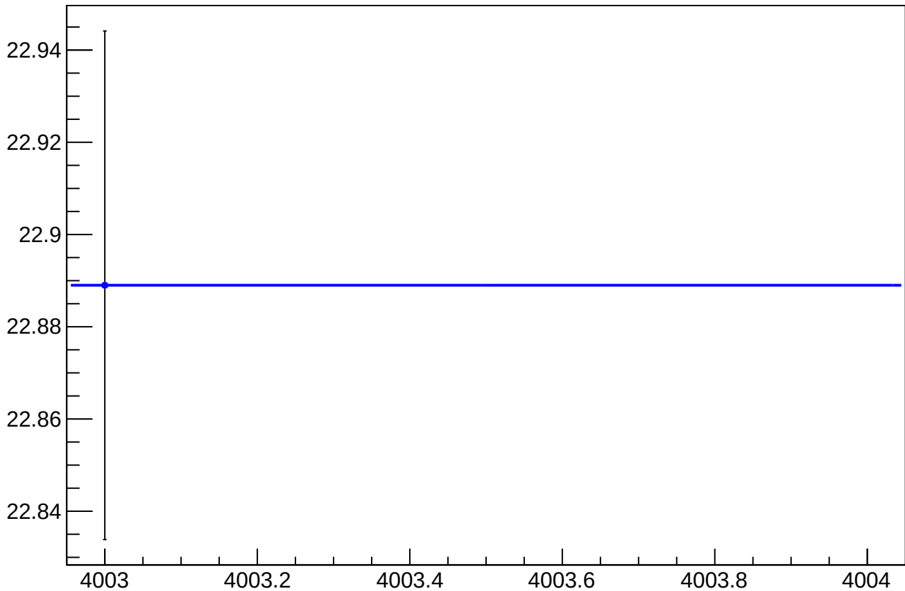
asym_sam_13_57_dd_eigen_dit_vs_cor_diff_rms vs Slug, Sign Corrected
