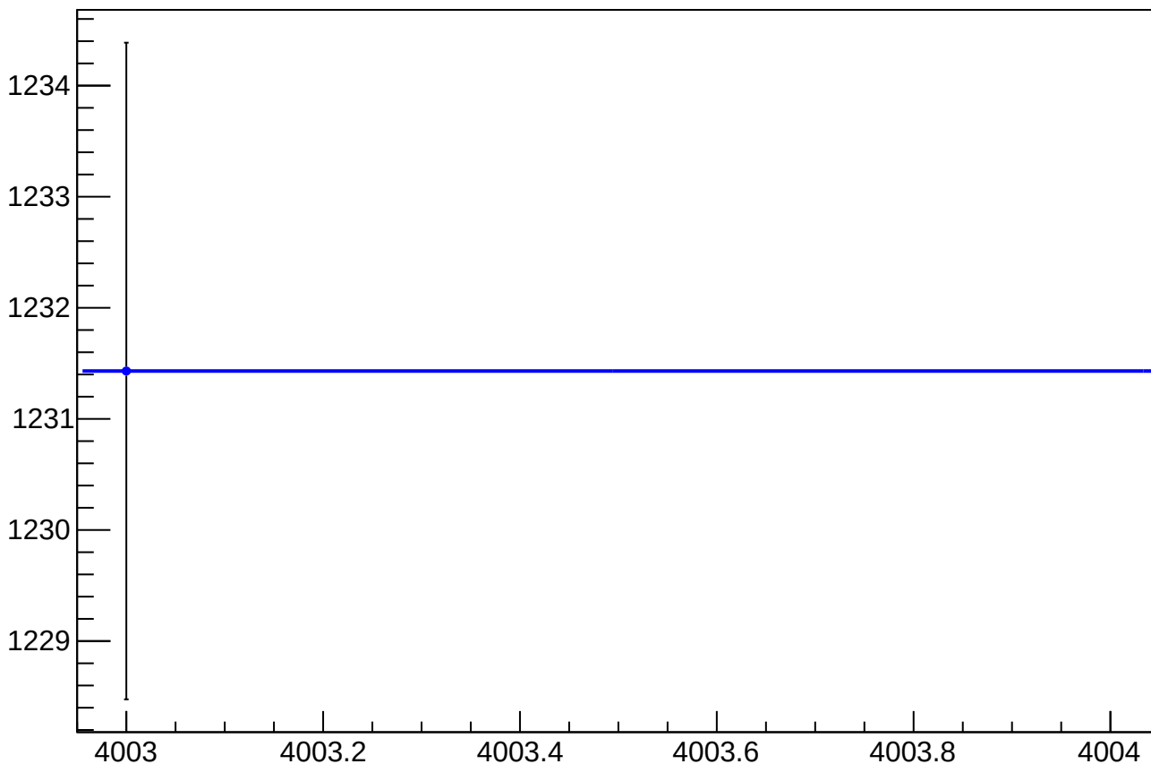
reg_asym_at1_avg_at2_avg_dd_rms vs Slug, Sign Corrected
