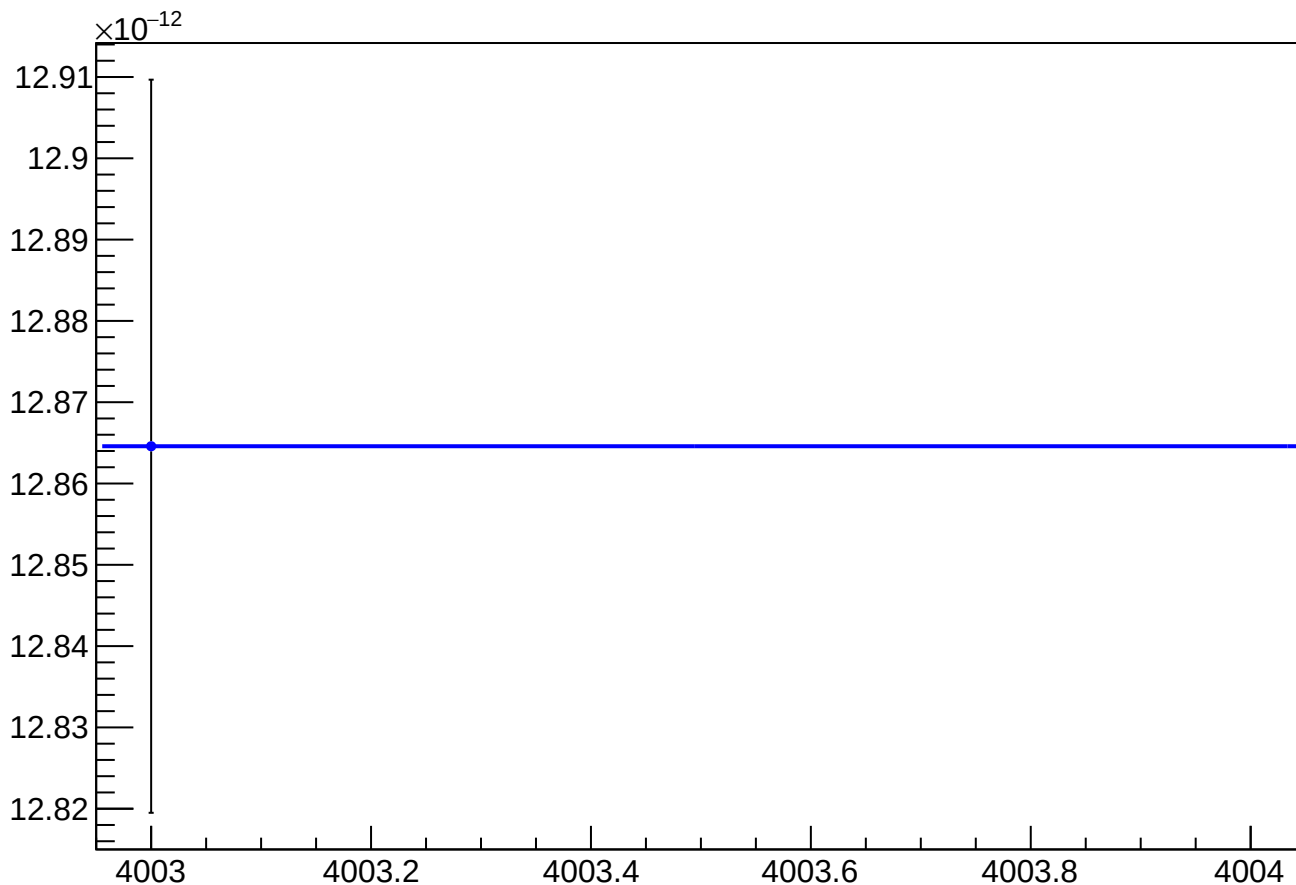
asym_sam_13_57_dd_reg_vs_cor_diff_rms vs Slug, Sign Corrected
