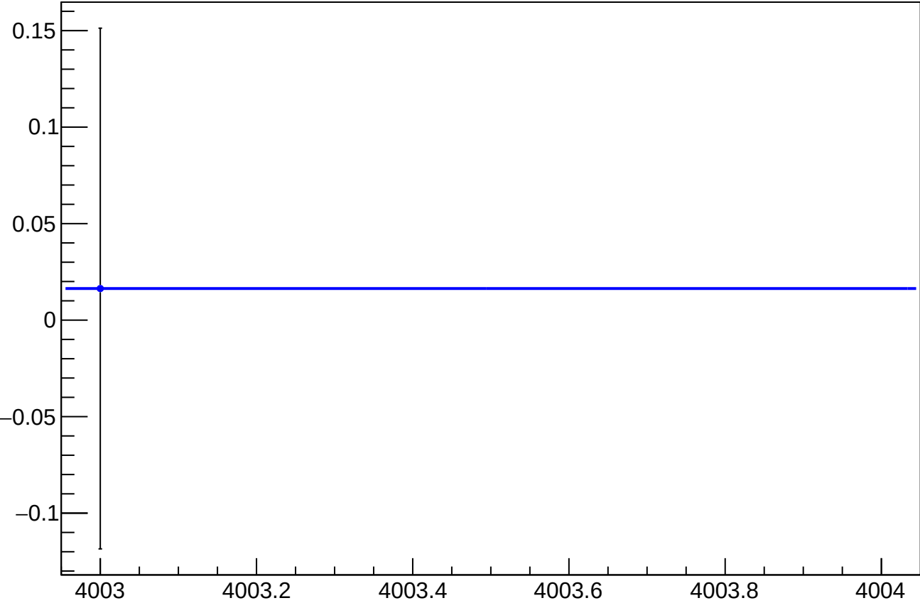
asym_us_dd_at2lr_dd_dd_dit_vs_eigen_cor_diff_mean vs Slug, Sign Corrected
