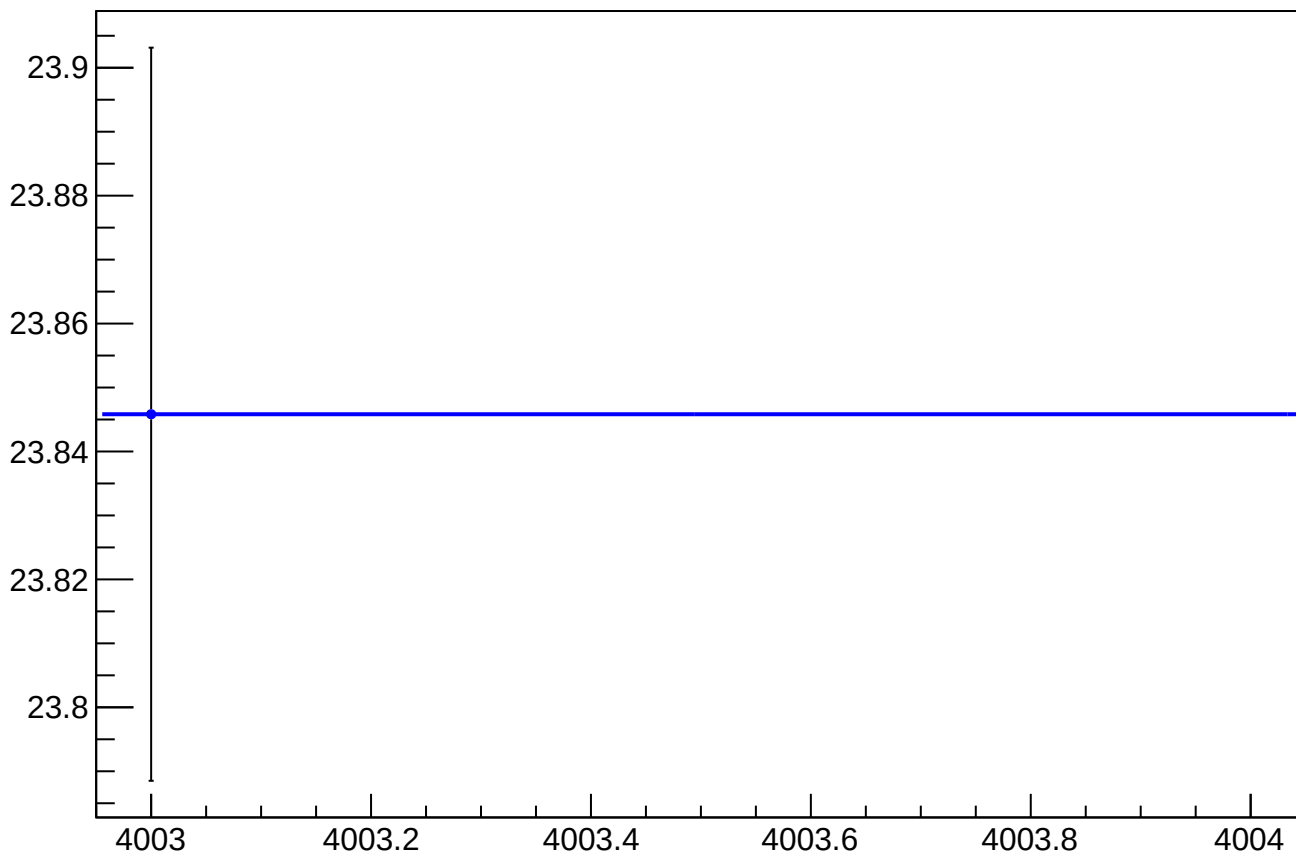
asym_sam_15_dd_eigen_dit_vs_cor_diff_rms vs Slug, Sign Corrected
