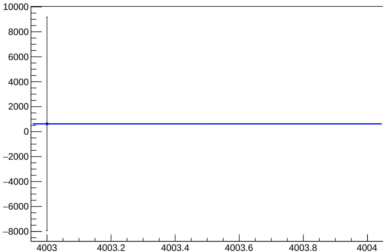
eigen_dit_asym_atr1_mean vs Slug, Sign Corrected
