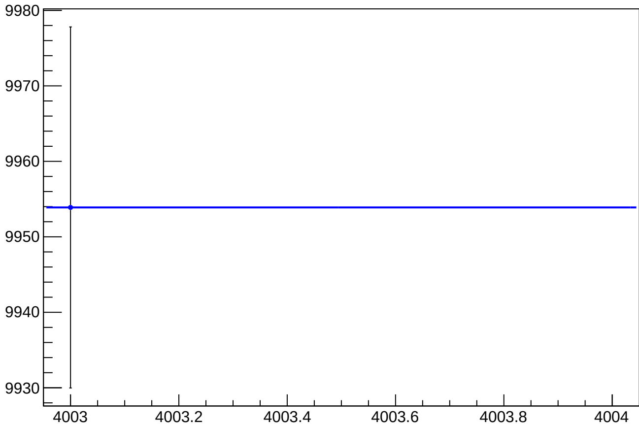
diff_bpm_4aX_4eX_avg_rms vs Slug, Sign Corrected
