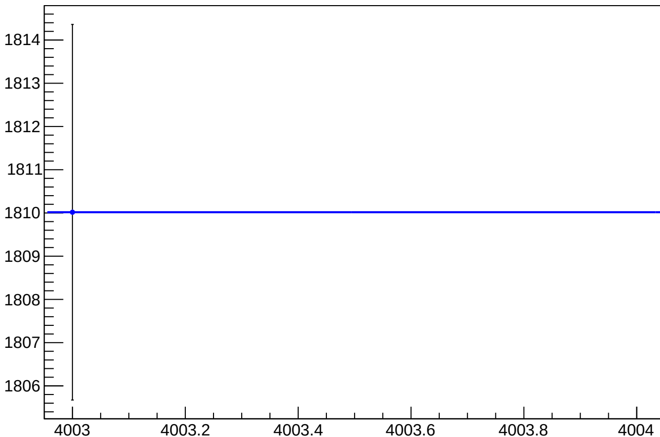
eigen_dit_asym_atr1l2_avg_rms vs Slug, Sign Corrected
