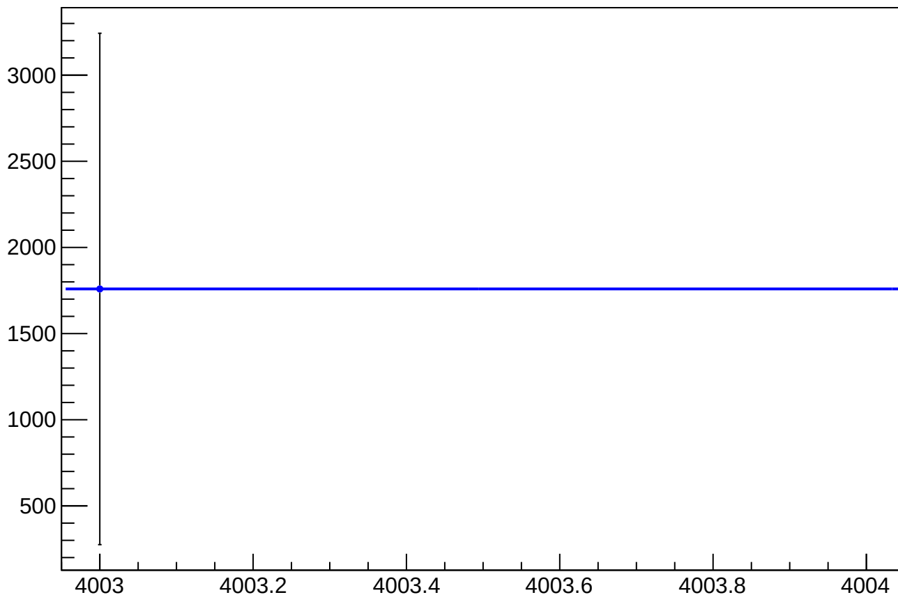
asym_us_dd_atlr_dd_dd_reg_correction_mean vs Slug, Sign Corrected
