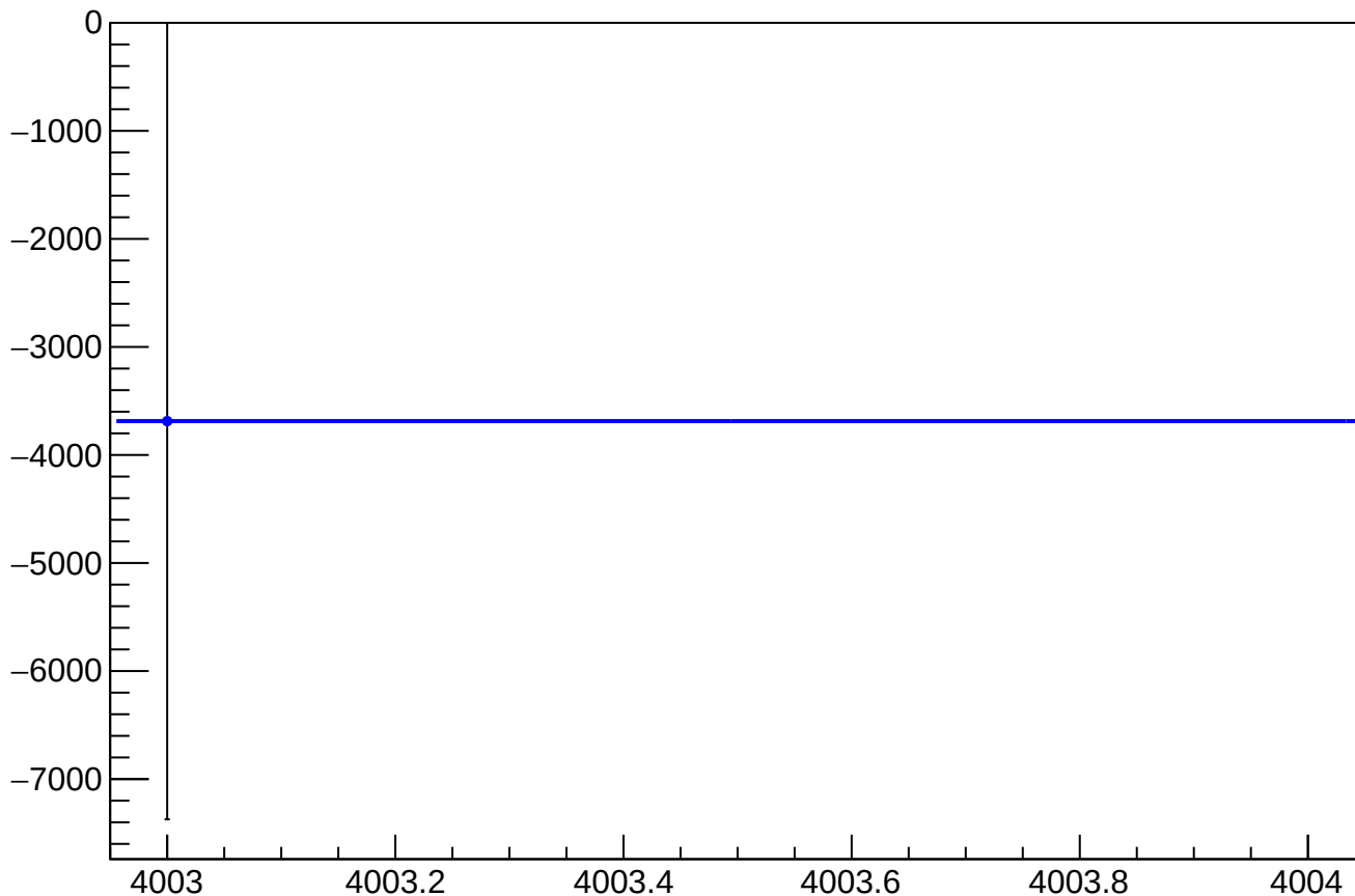
eigen_dit_asym_us_dd_atlr_dd_dd_mean vs Slug, Sign Corrected
