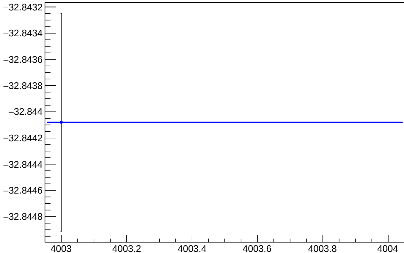
yield_cav4dY_mean vs Slug, Sign Corrected
