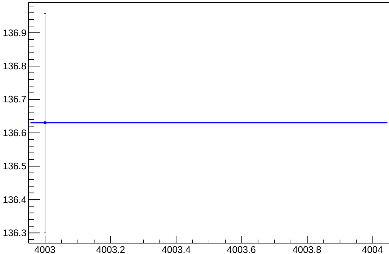
eigen_cor_asym_sam5_rms vs Slug, Sign Corrected
