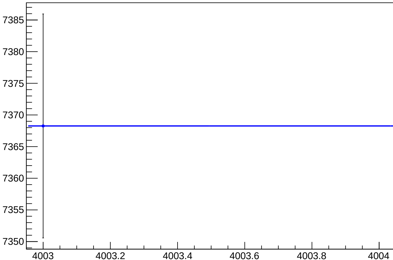
asym_usl_atl2_avg_eigen_dit_correction_rms vs Slug, Sign Corrected
