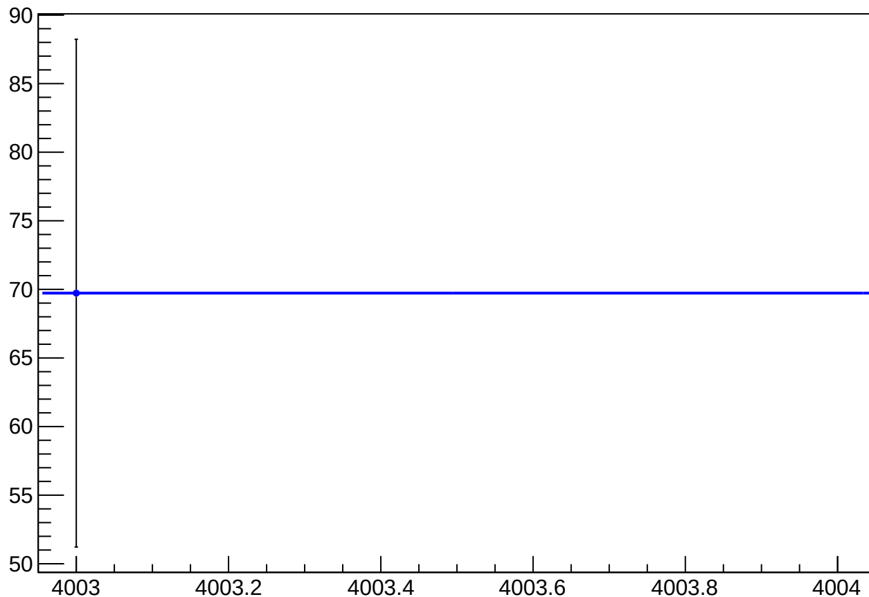
reg_asym_atl_avg_atr_avg_avg_diff_bpm4eY_slope vs Slug, Sign Corrected
