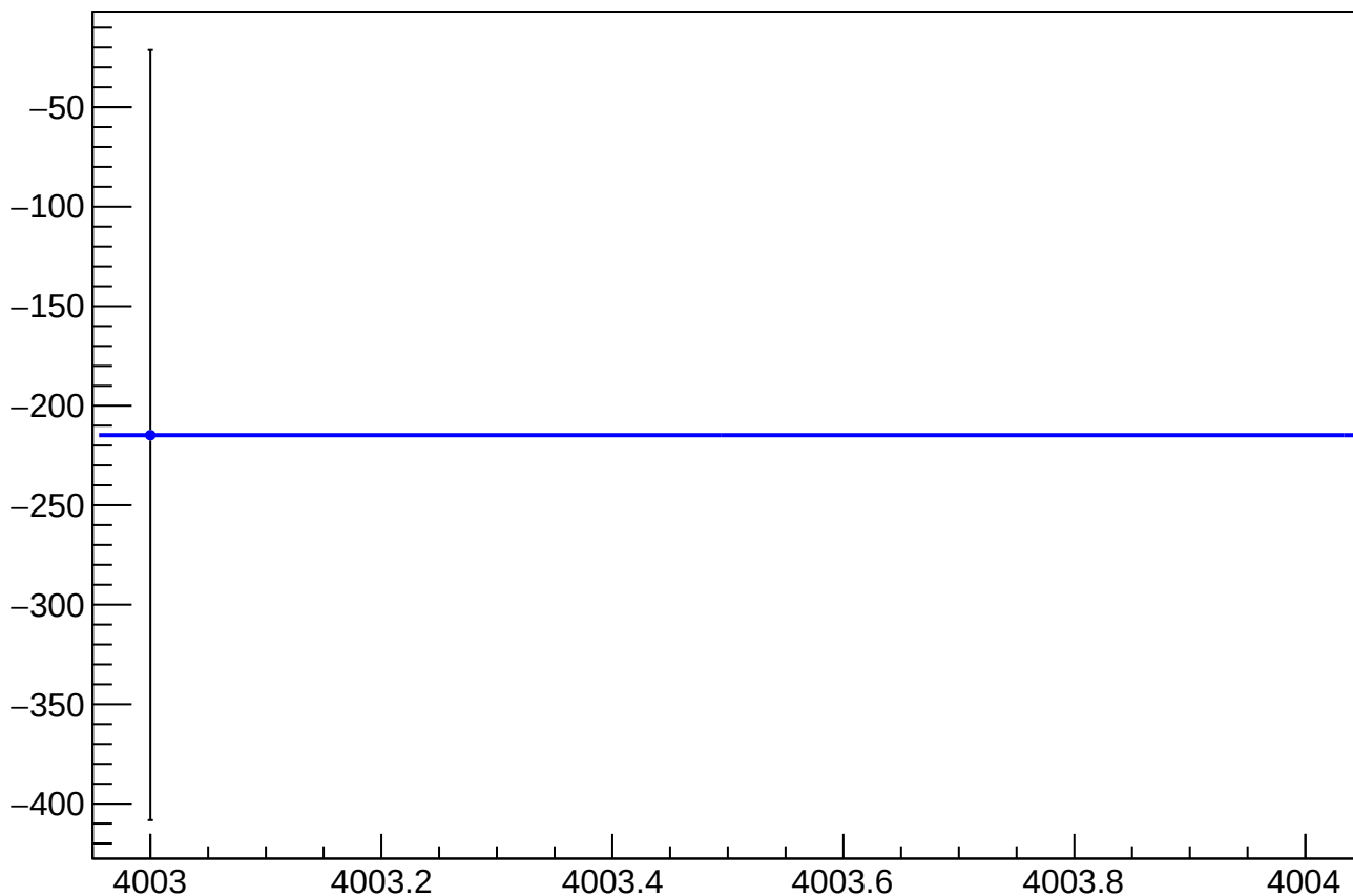
eigen_dit_asym_sam_15_48_dd_mean vs Slug, Sign Corrected
