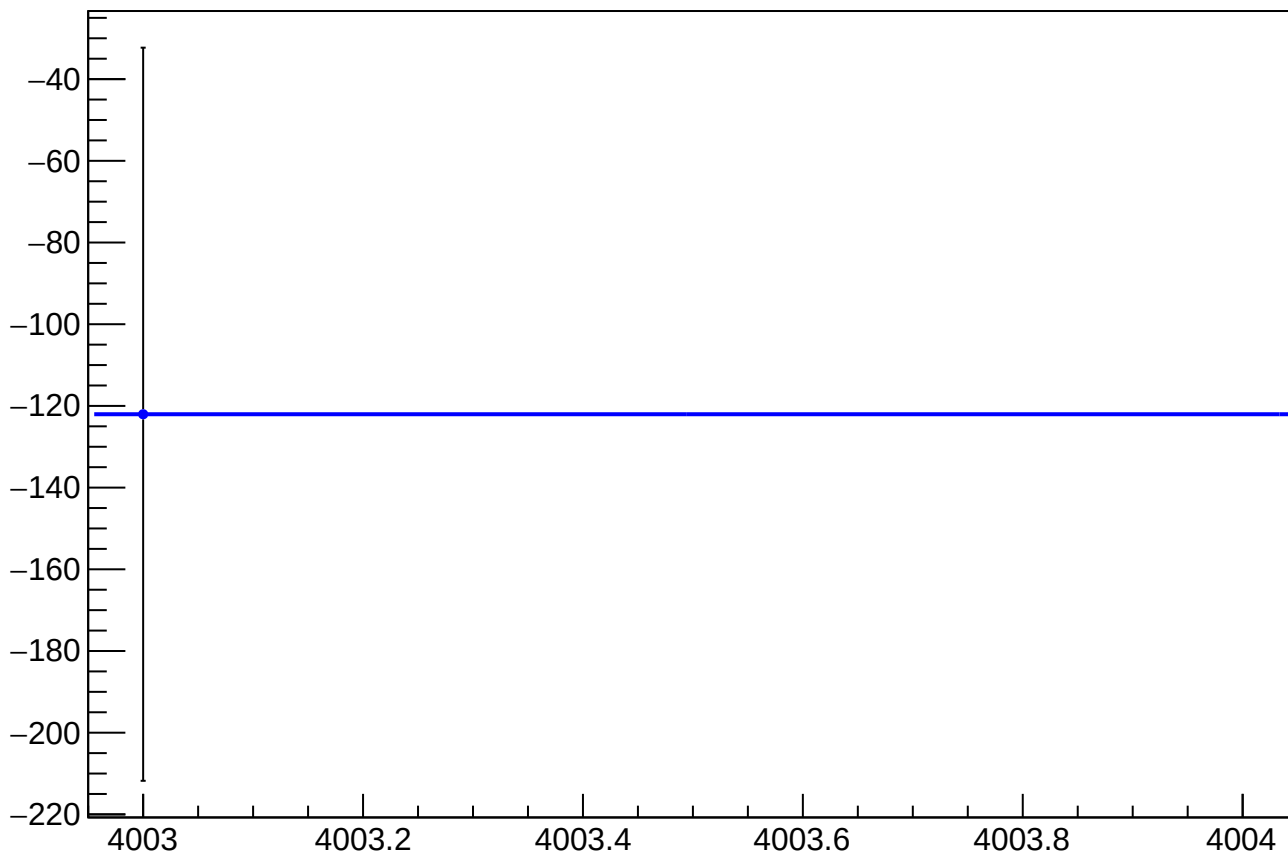
asym_bcm_cav4cQ_an_ds_dd_mean vs Slug, Sign Corrected
