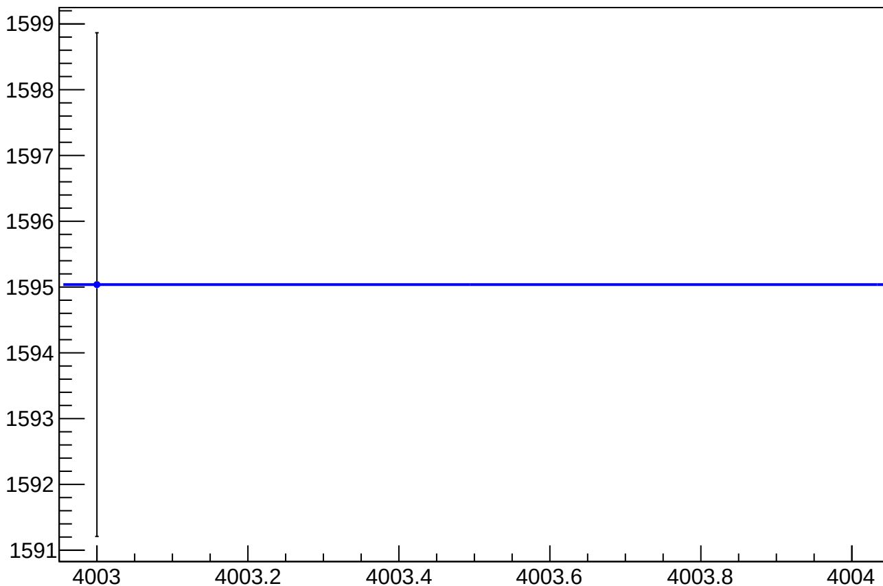
eigen_dit_asym_us_dd_at1lr_dd_dd_rms vs Slug, Sign Corrected
