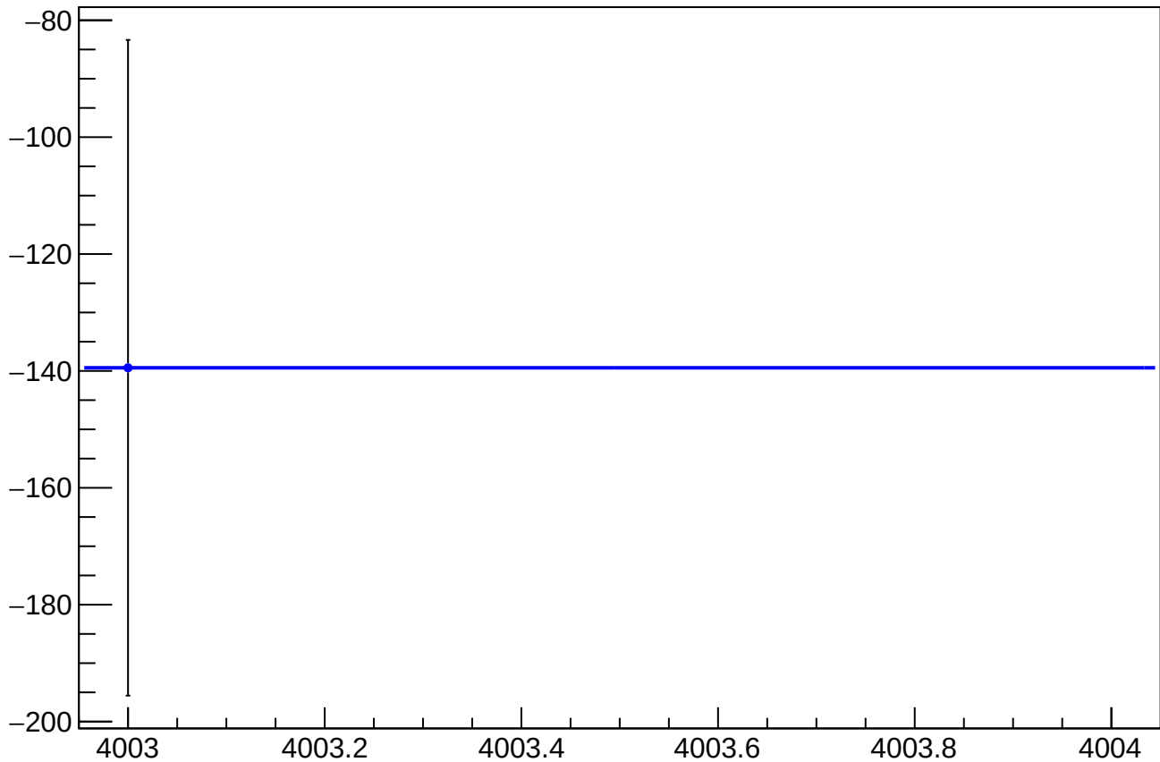
asym_bcm_dg_ds_an_us_dd_mean vs Slug, Sign Corrected
