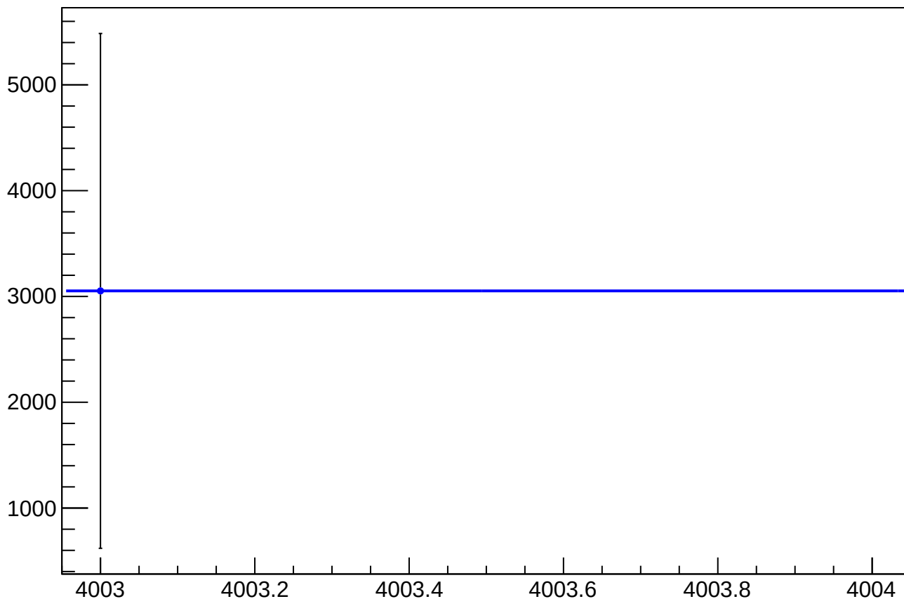
asym_sam_26_avg_eigen_cor_correction_mean vs Slug, Sign Corrected
