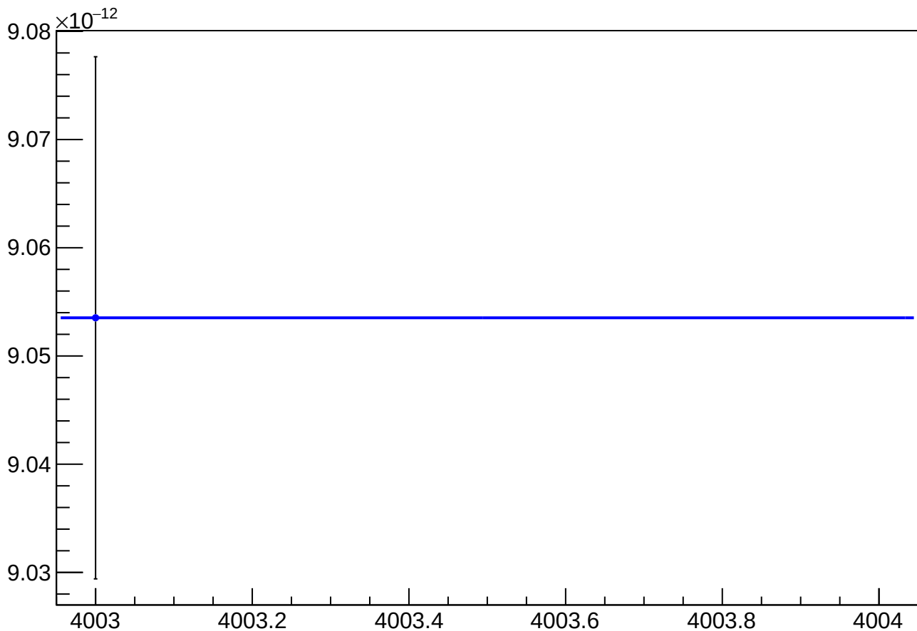
asym_sam_15_26_dd_eigen_cor_vs_cor_diff_rms vs Slug, Sign Corrected
