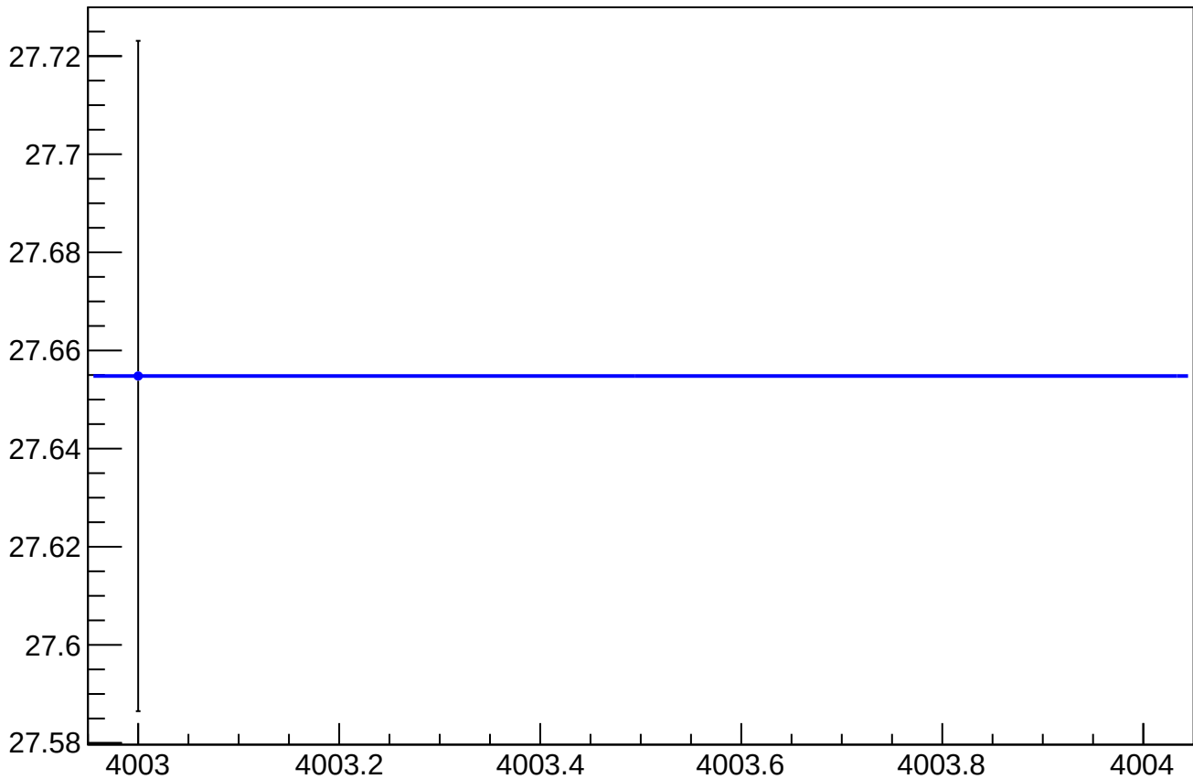
asym_us_dd_dit_vs_eigen_cor_diff_rms vs Slug, Sign Corrected
