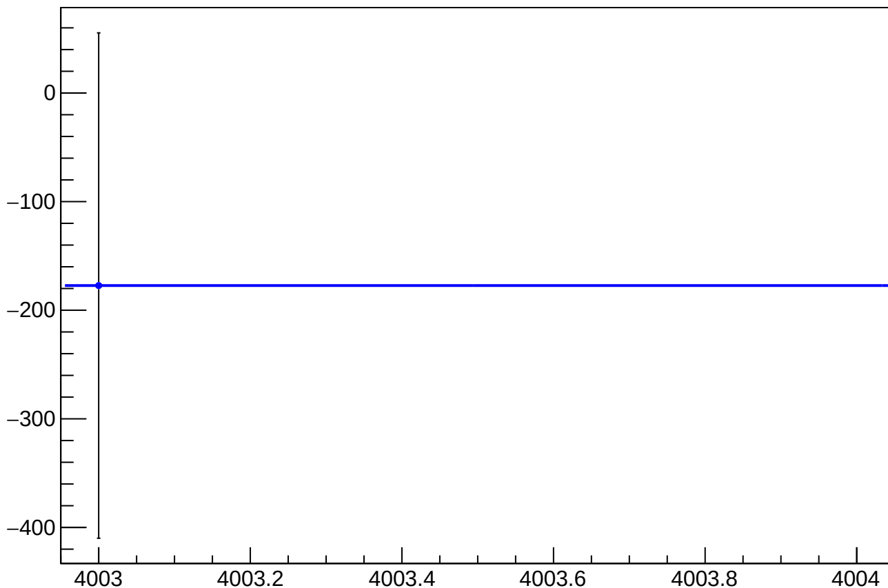
eigen_dit_asym_sam_15_26_dd_mean vs Slug, Sign Corrected
