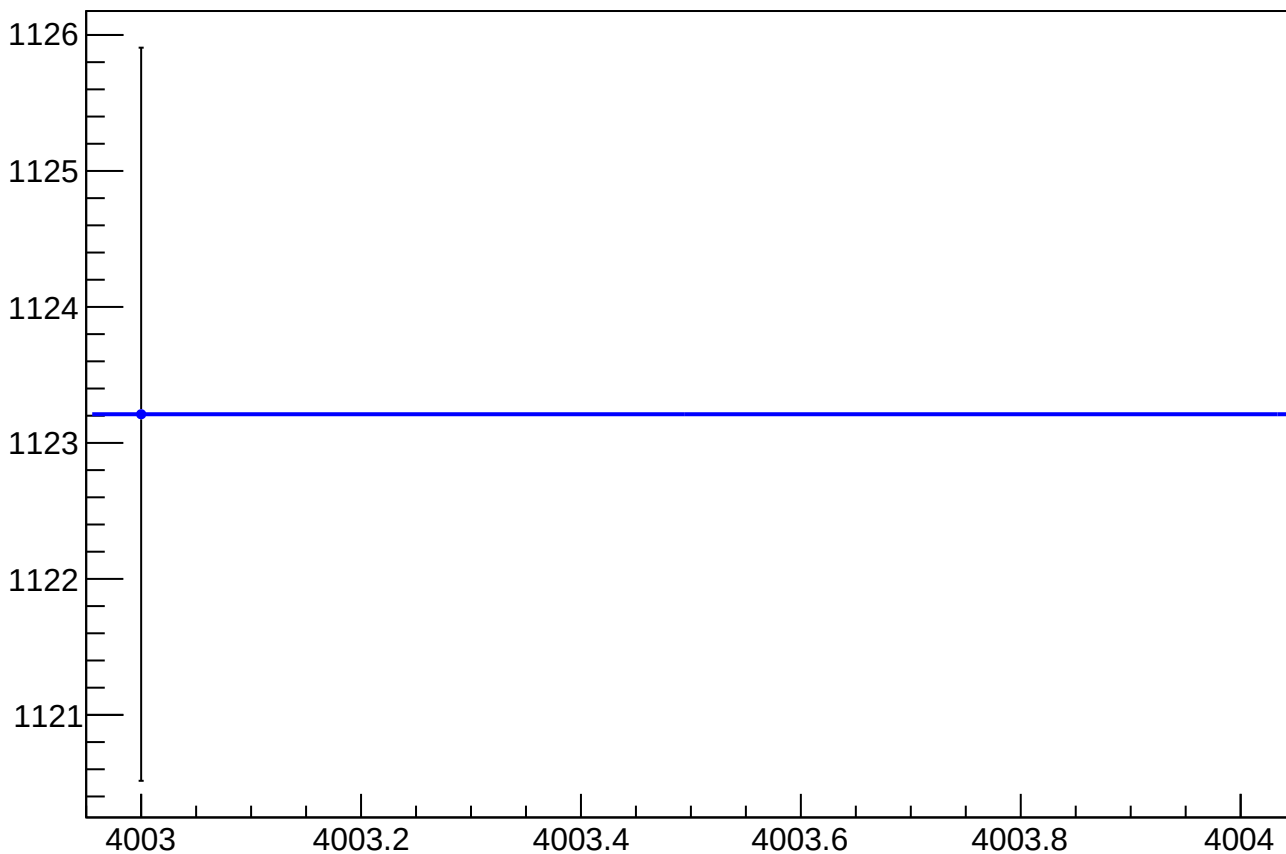
eigen_dit_asym_us_avg_atlr_avg_dd_rms vs Slug, Sign Corrected
