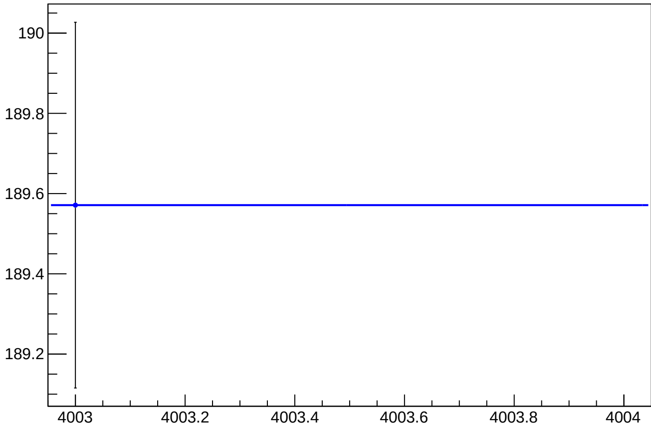
asym_sam7_cor_correction_rms vs Slug, Sign Corrected
