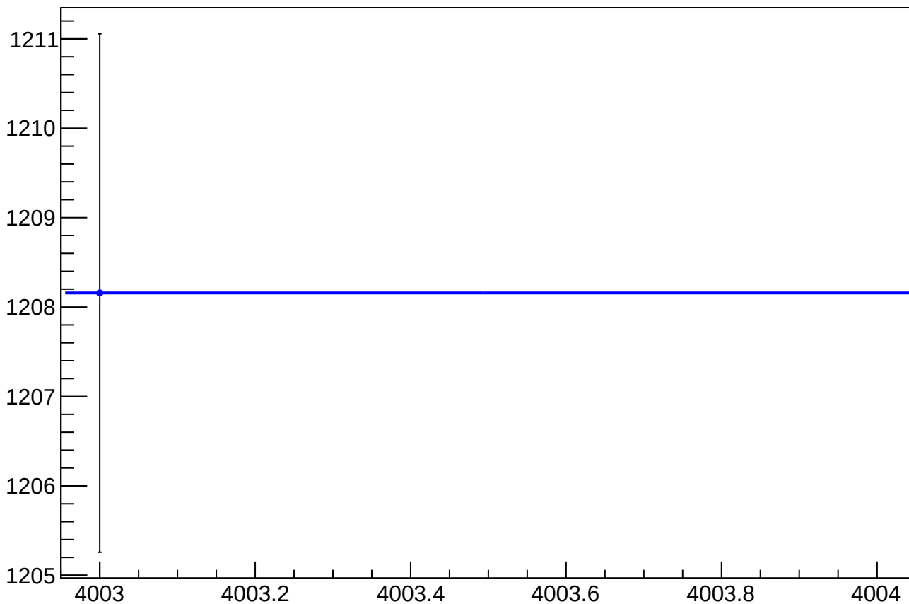
eigen_dit_asym_at1_dd_at2_dd_avg_rms vs Slug, Sign Corrected
