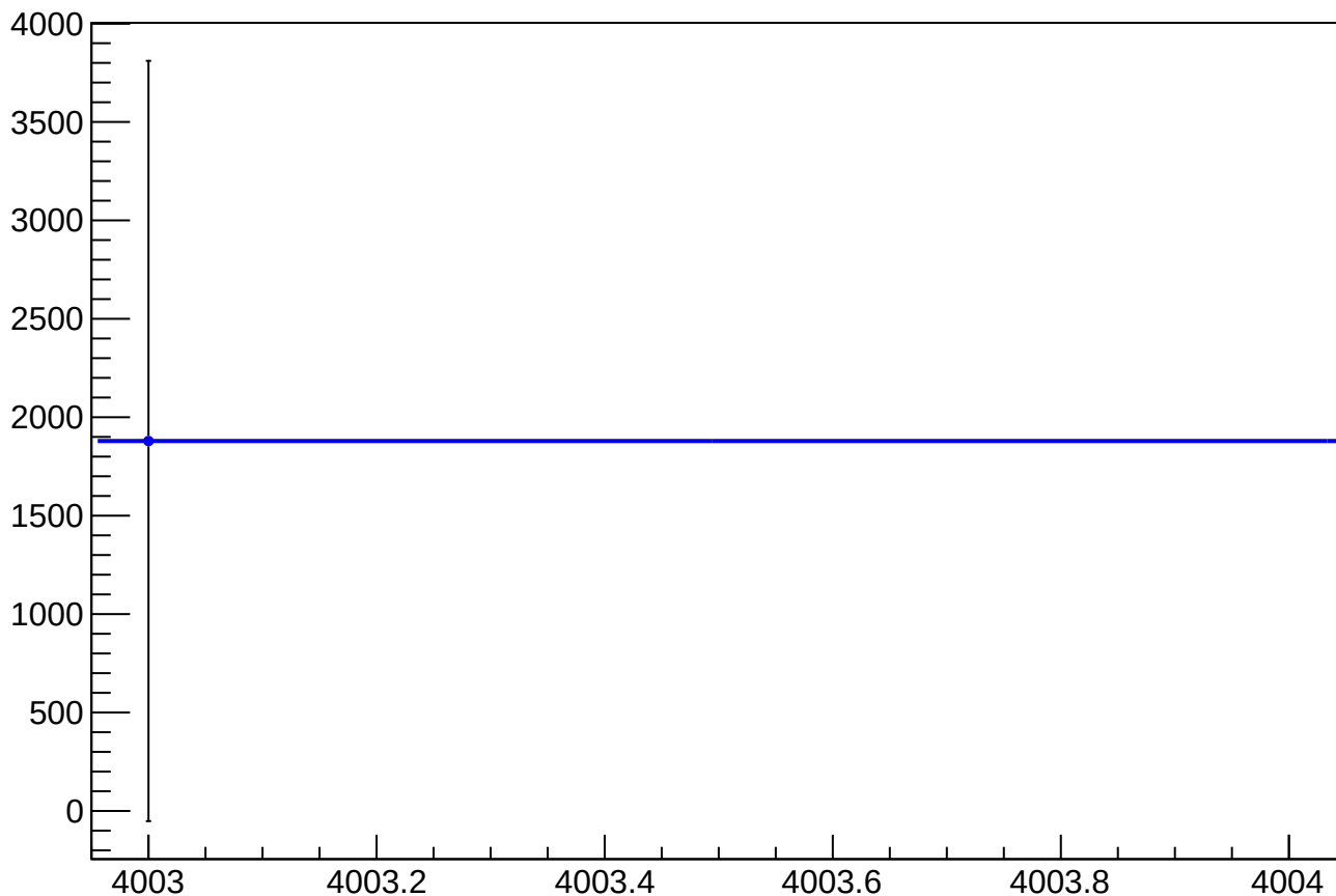
asym_sam_12345678_avg_reg_correction_mean vs Slug, Sign Corrected
