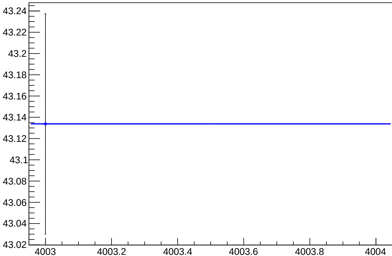
asym_sam_24_68_dd_dit_vs_eigen_cor_diff_rms vs Slug, Sign Corrected
