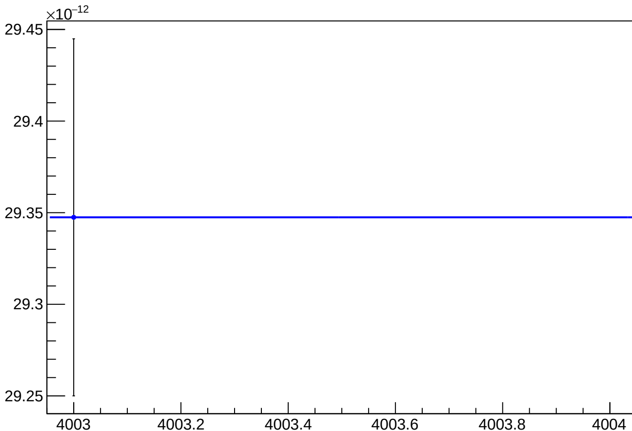
asym_sam_37_48_dd_reg_vs_cor_diff_rms vs Slug, Sign Corrected
