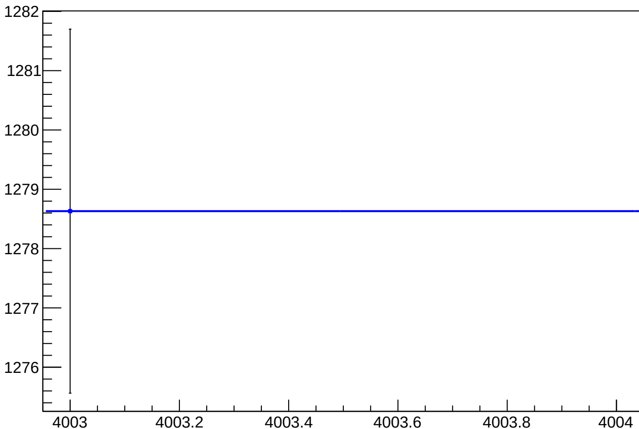
eigen_dit_asym_atl_avg_atr_avg_avg_rms vs Slug, Sign Corrected
