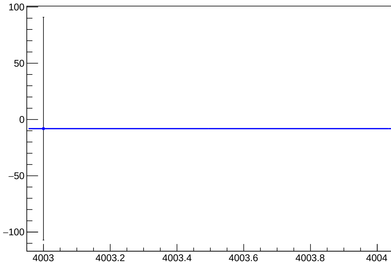
asym_bcm_cav4cQ_dg_ds_dd_mean vs Slug, Sign Corrected
