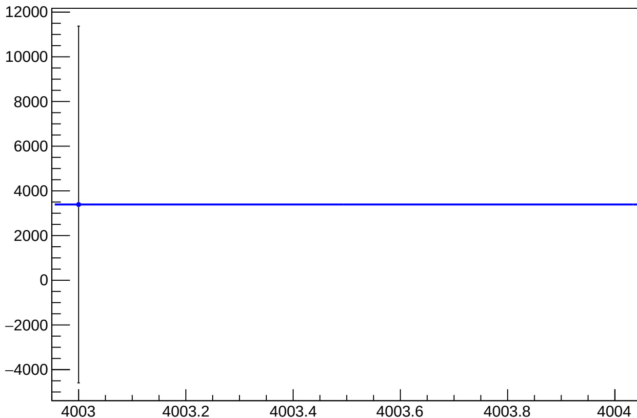
asym_usl_eigen_dit_correction_mean vs Slug, Sign Corrected
