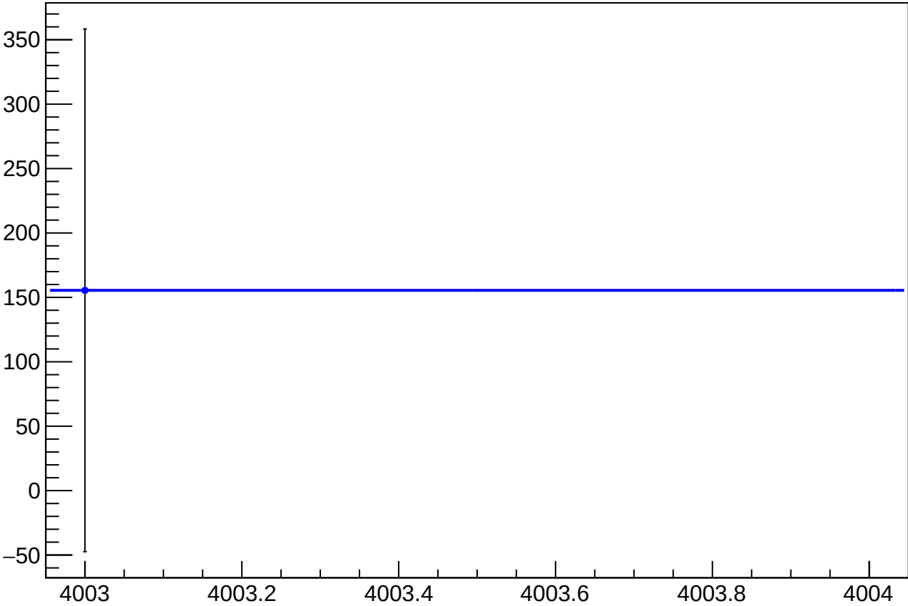
cor_asym_sam_12345678_avg_mean vs Slug, Sign Corrected
