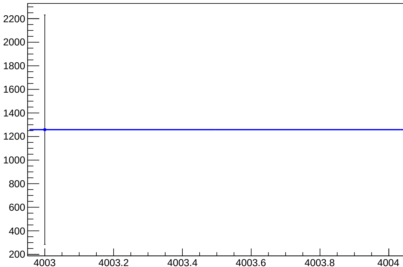
asym_sam_1526_avg_eigen_dit_correction_mean vs Slug, Sign Corrected
