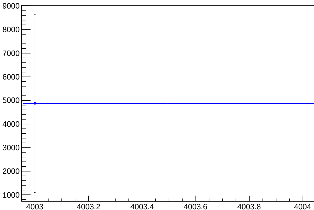
asym_us_dd_at1lr_dd_dd_eigen_cor_correction_mean vs Slug, Sign Corrected
