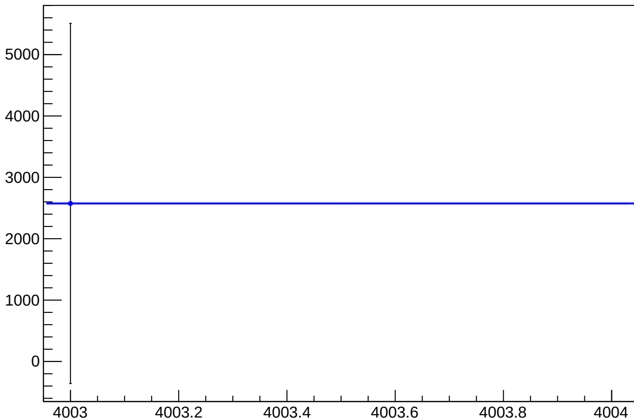
asym_sam_3748_avg_dit_correction_mean vs Slug, Sign Corrected
