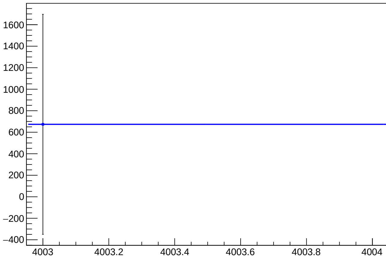
asym_sam_1357_avg_dit_correction_mean vs Slug, Sign Corrected
