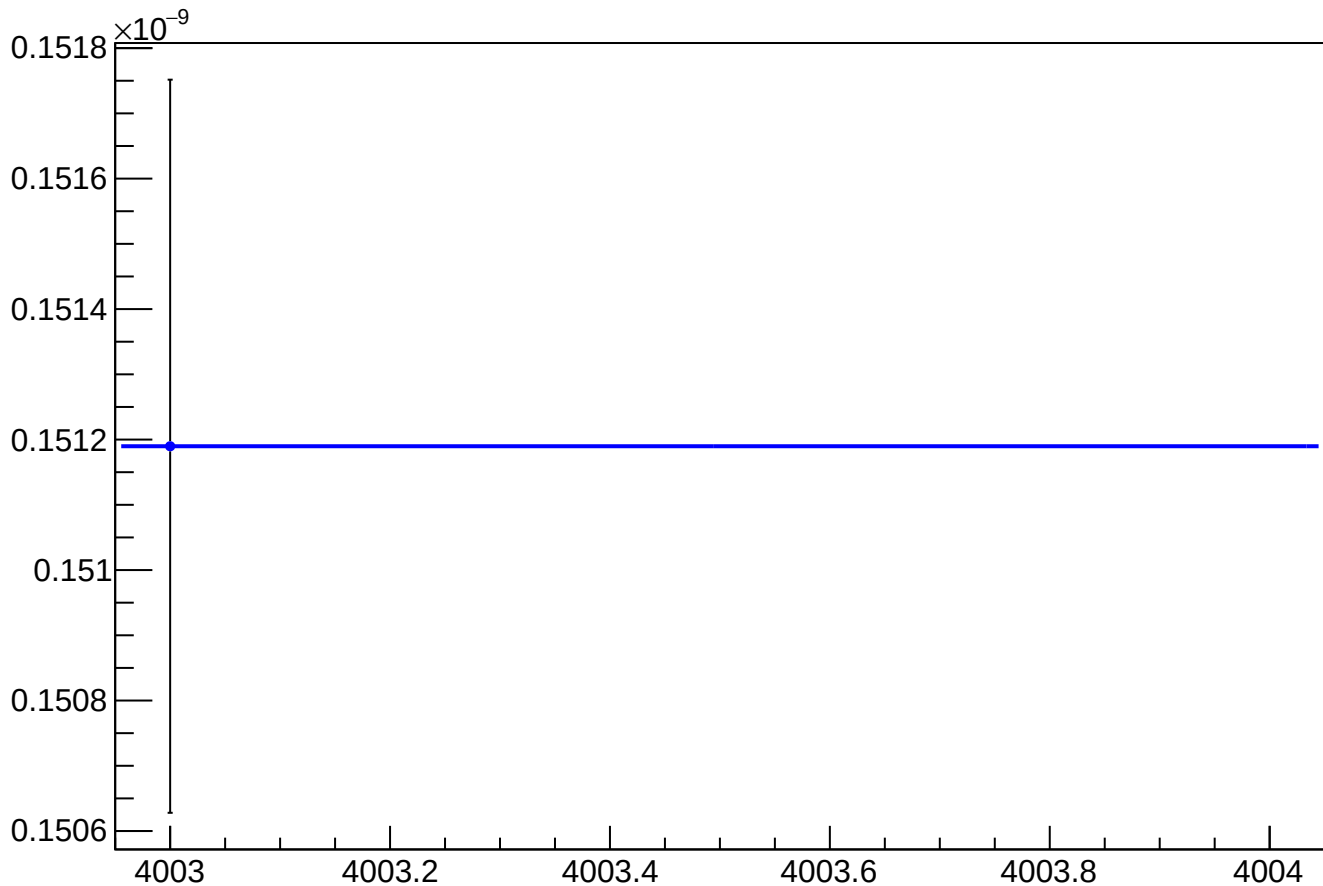
asym_us_avg_at2lr_avg_dd_reg_vs_cor_diff_rms vs Slug, Sign Corrected
