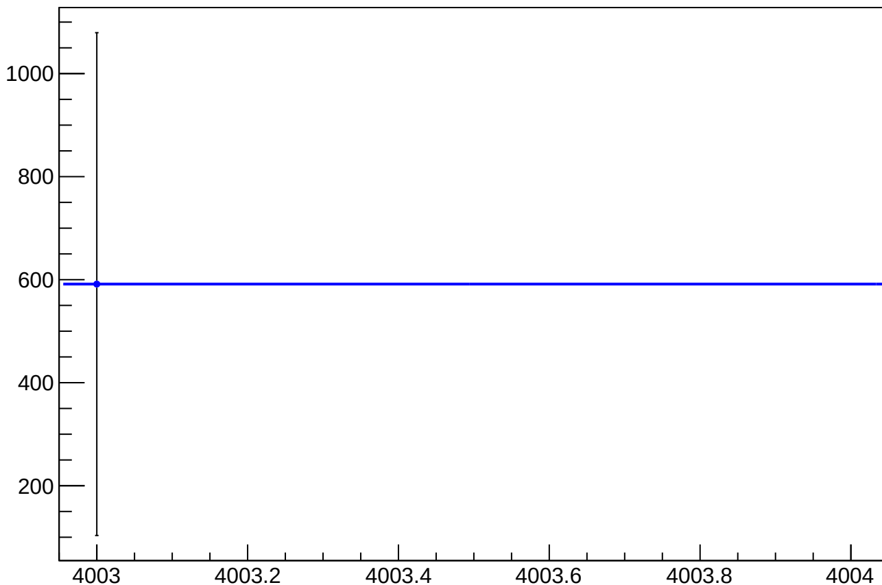
asym_atl1r2_dd_atl2r1_dd_avg_eigen_dit_correction_mean vs Slug, Sign Corrected
