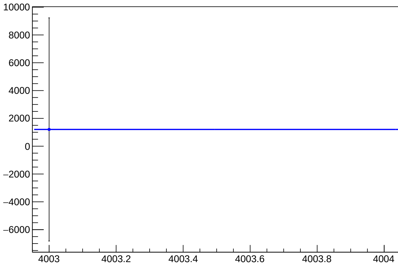
asym_usr_atr1_avg_eigen_dit_correction_mean vs Slug, Sign Corrected
