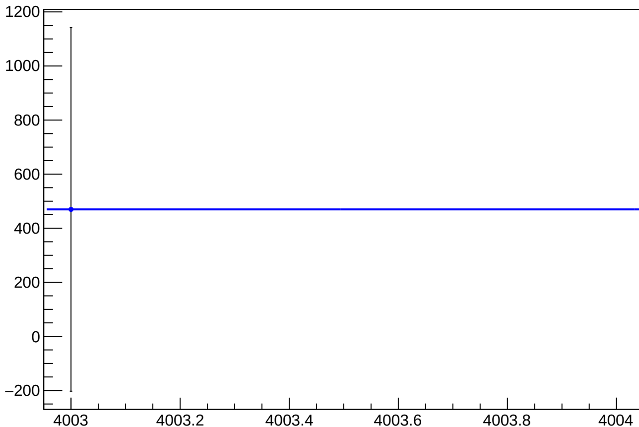
asym_sam8_eigen_cor_correction_mean vs Slug, Sign Corrected
