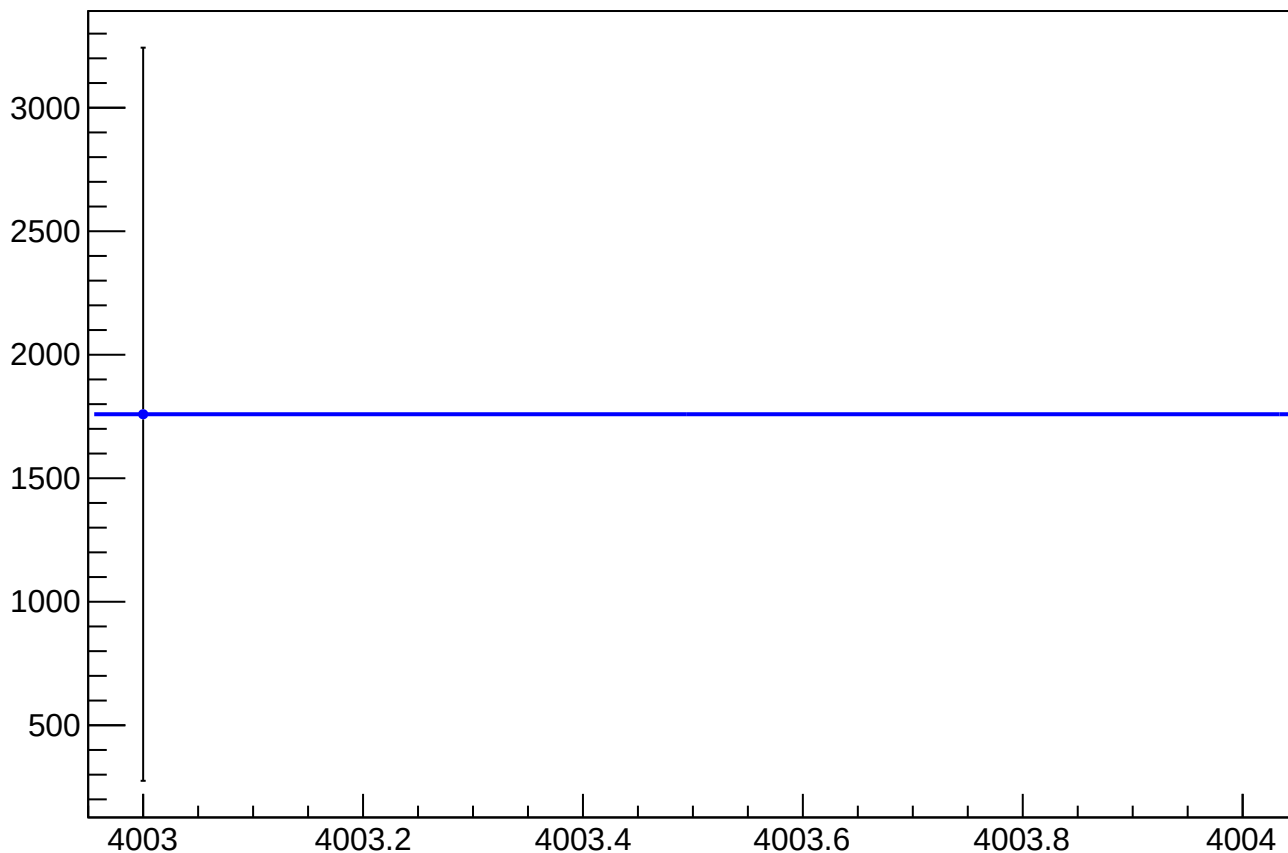
asym_us_dd_atlr_dd_dd_cor_correction_mean vs Slug, Sign Corrected
