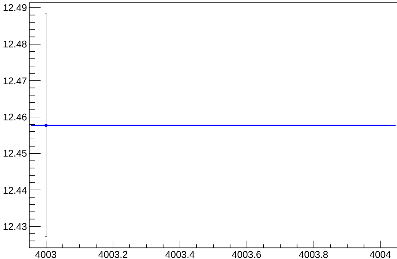
asym_sam_15_avg_dit_vs_cor_diff_rms vs Slug, Sign Corrected
