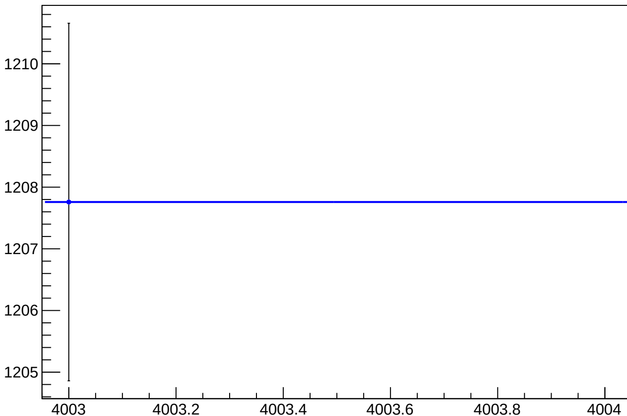
reg_asym_at1_dd_at2_dd_avg_rms vs Slug, Sign Corrected
