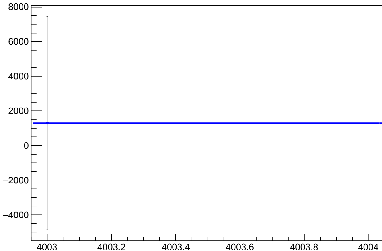
asym_at1_avg_eigen_dit_correction_mean vs Slug, Sign Corrected
