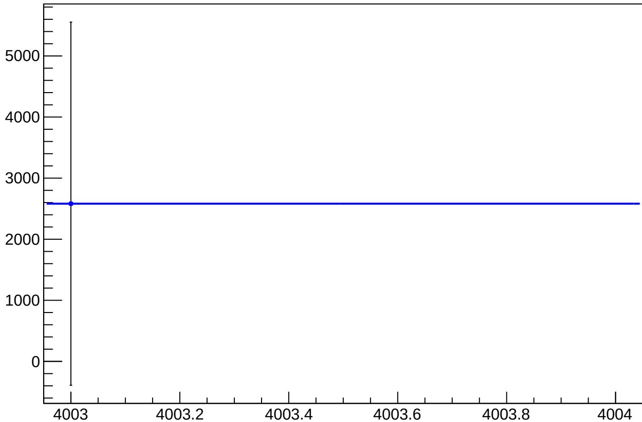
asym_sam_3748_avg_reg_correction_mean vs Slug, Sign Corrected
