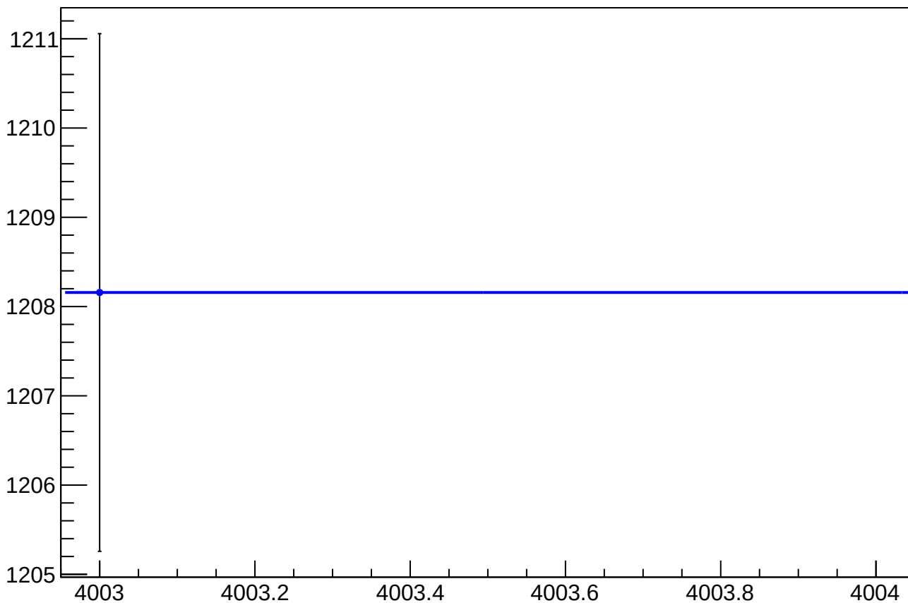
dit_asym_at1_dd_at2_dd_avg_rms vs Slug, Sign Corrected
