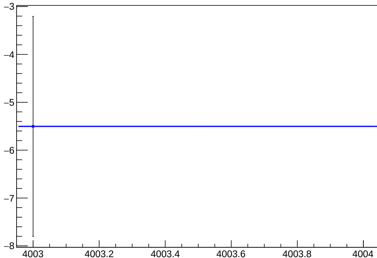
reg_asym_us_dd_diff_bpm4aY_slope vs Slug, Sign Corrected
