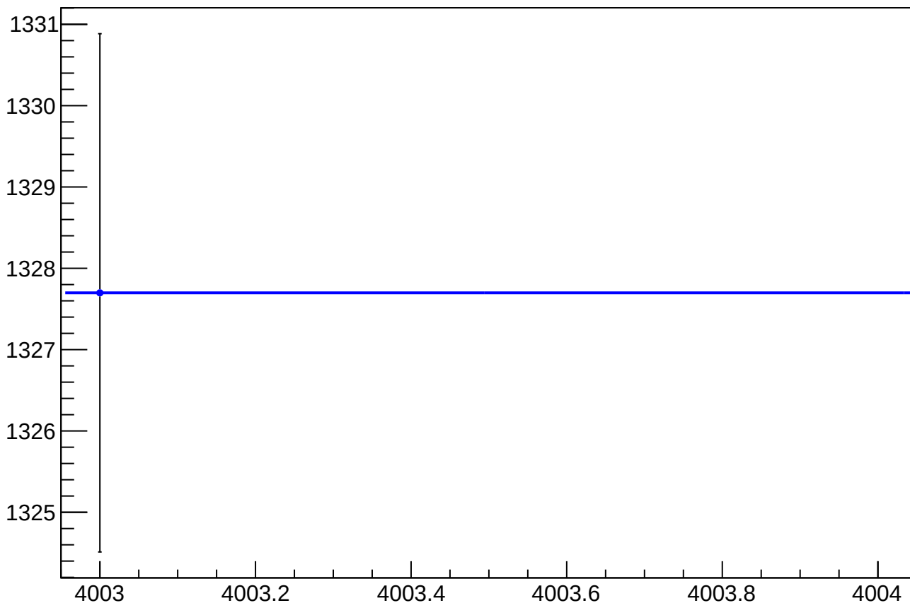
reg_asym_usl_atl1_avg_rms vs Slug, Sign Corrected
