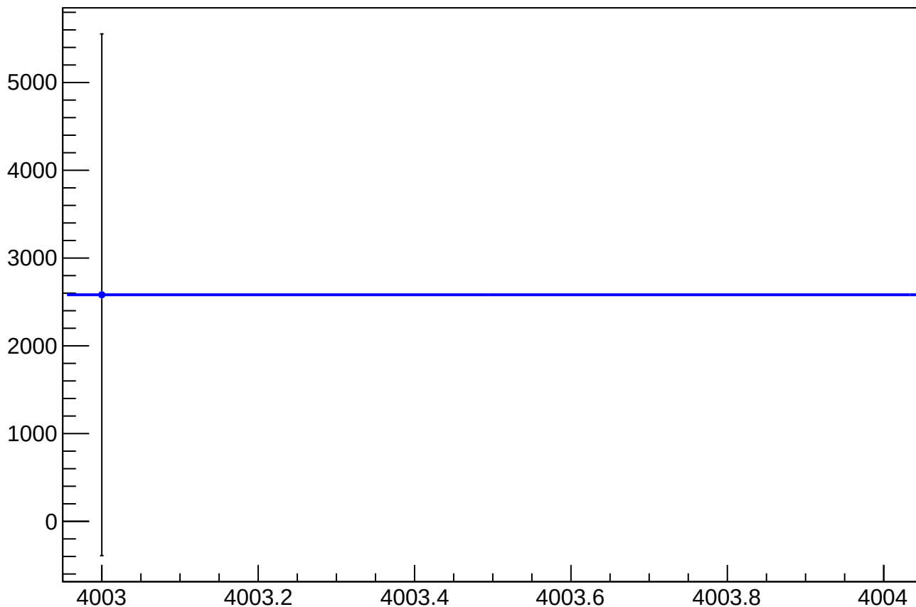
asym_sam_3748_avg_eigen_cor_correction_mean vs Slug, Sign Corrected
