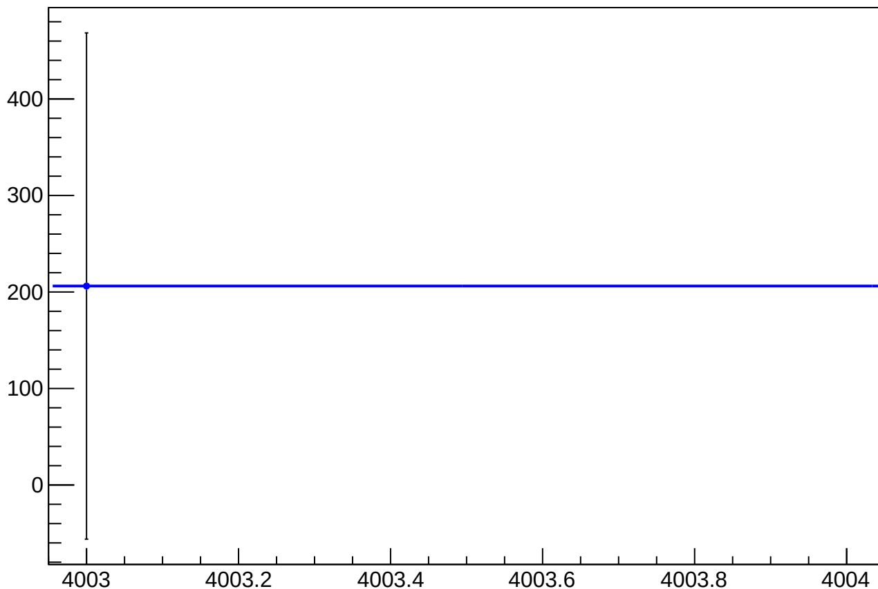
reg_asym_sam_2468_avg_mean vs Slug, Sign Corrected
