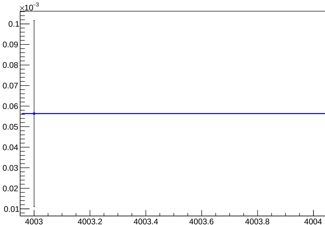
asym_atl_avg_atr_avg_avg_eigen_dit_vs_dit_diff_mean vs Slug, Sign Corrected
