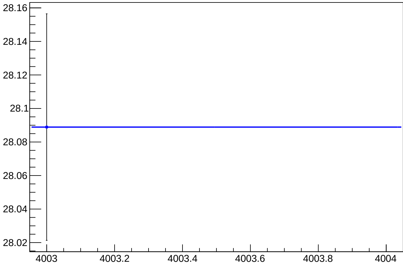
asym_sam_37_48_dd_dit_vs_eigen_cor_diff_rms vs Slug, Sign Corrected
