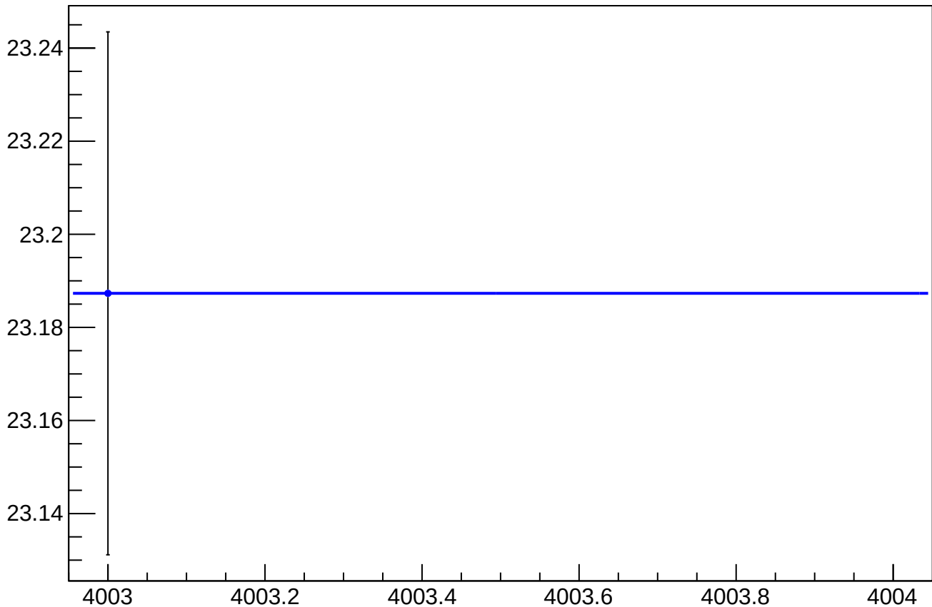
asym_sam_37_26_dd_eigen_dit_vs_cor_diff_rms vs Slug, Sign Corrected
