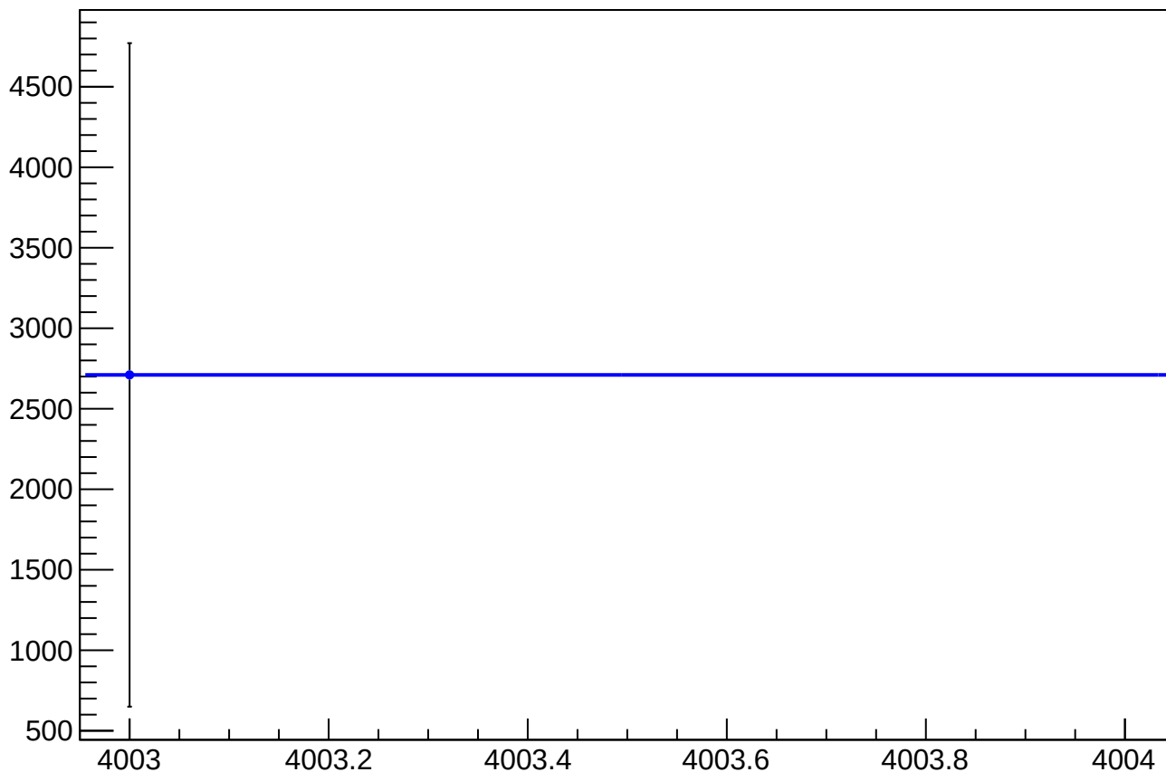
asym_sam_3726_avg_reg_correction_mean vs Slug, Sign Corrected
