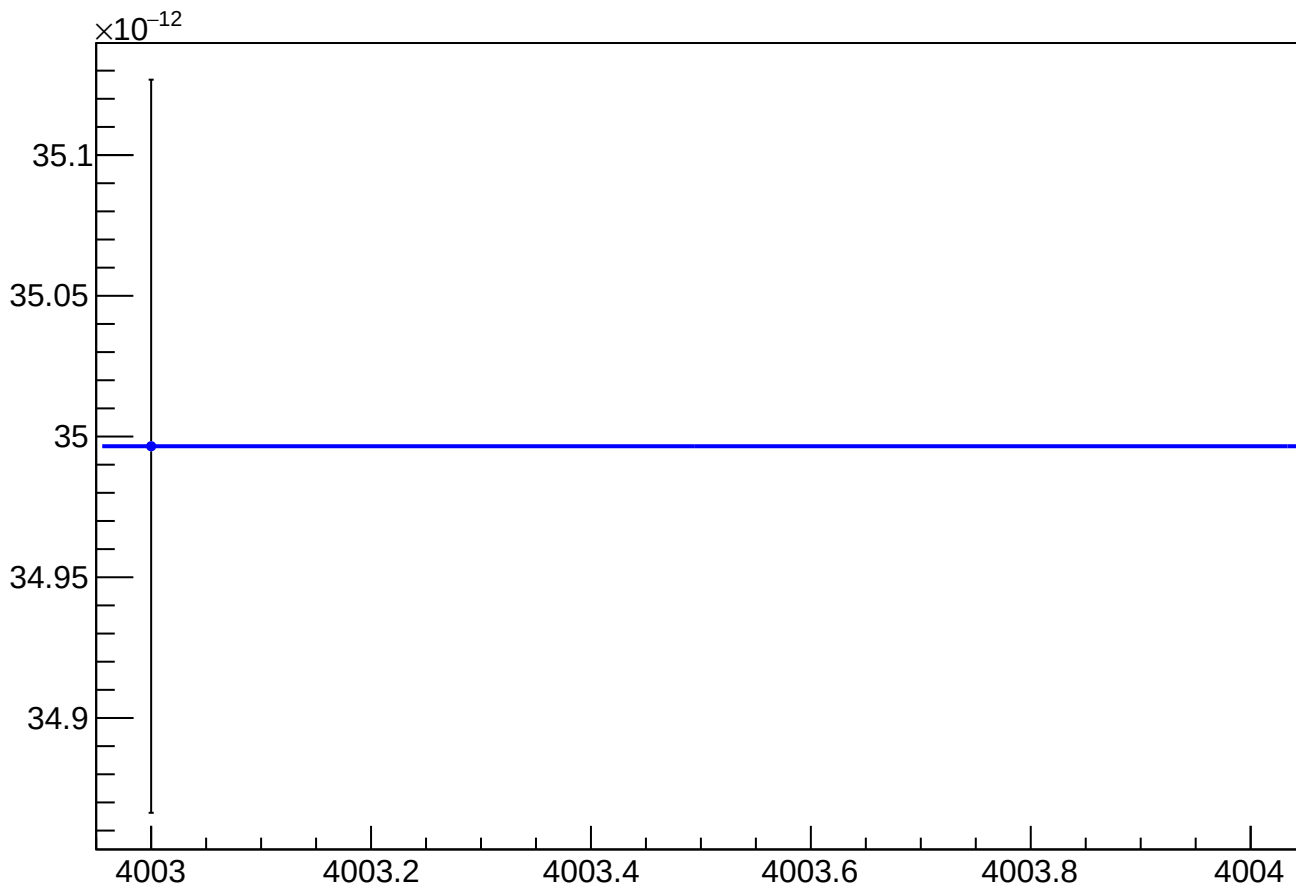
asym_at1_avg_reg_vs_cor_diff_rms vs Slug, Sign Corrected
