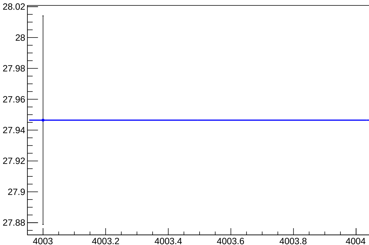
asym_sam_48_dd_dit_vs_eigen_cor_diff_rms vs Slug, Sign Corrected
