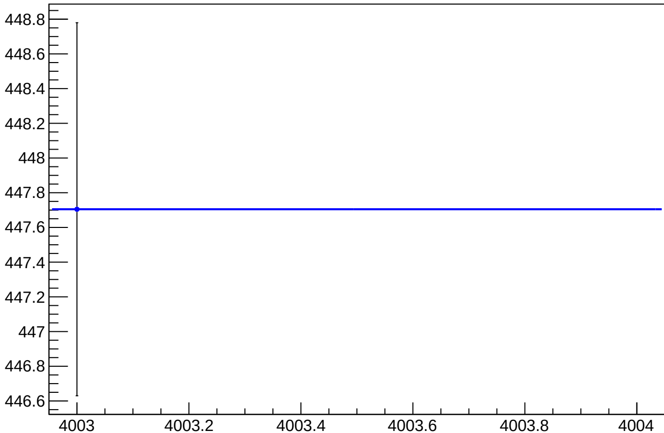
asym_sam_37_48_dd_reg_correction_rms vs Slug, Sign Corrected
