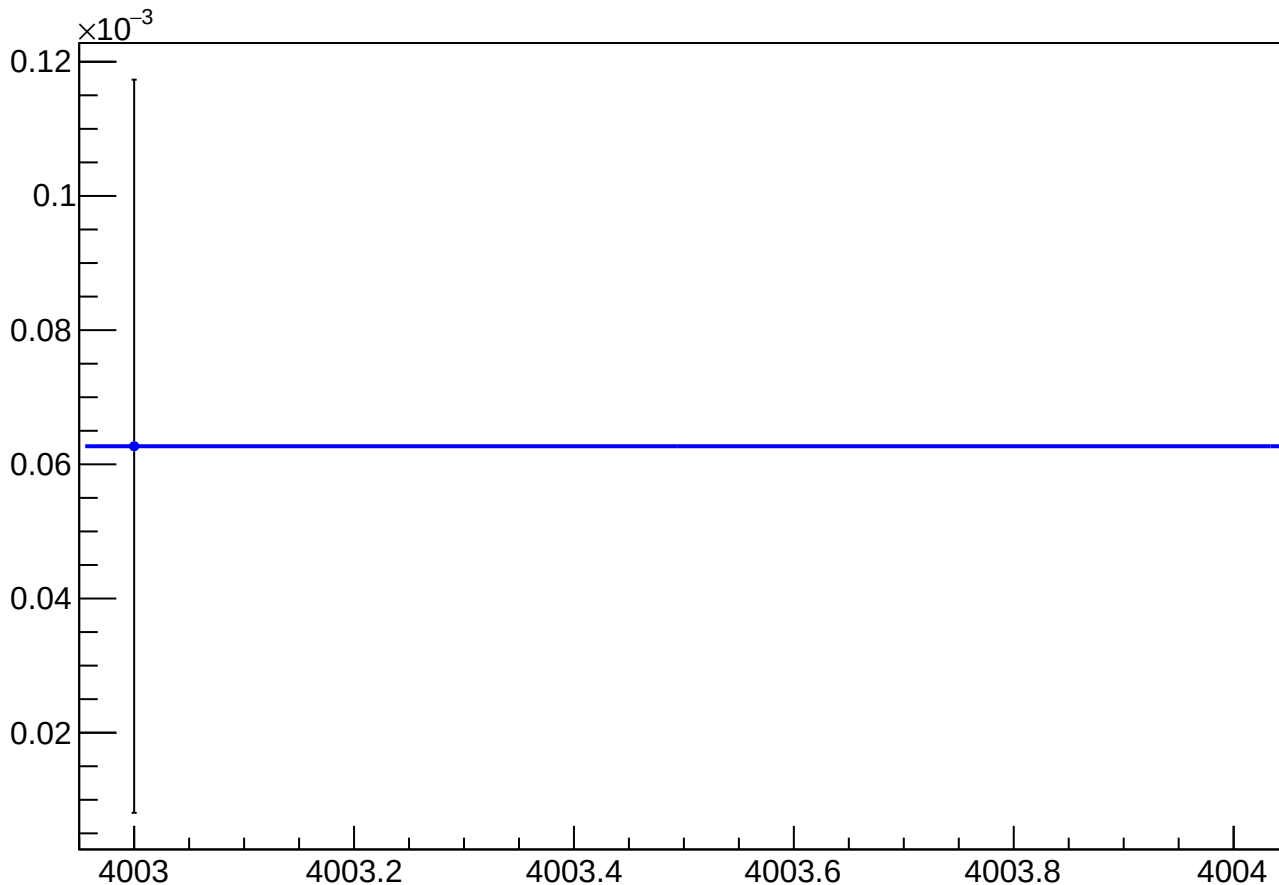
asym_us_avg_atlr_avg_avg_eigen_dit_vs_dit_diff_mean vs Slug, Sign Corrected
