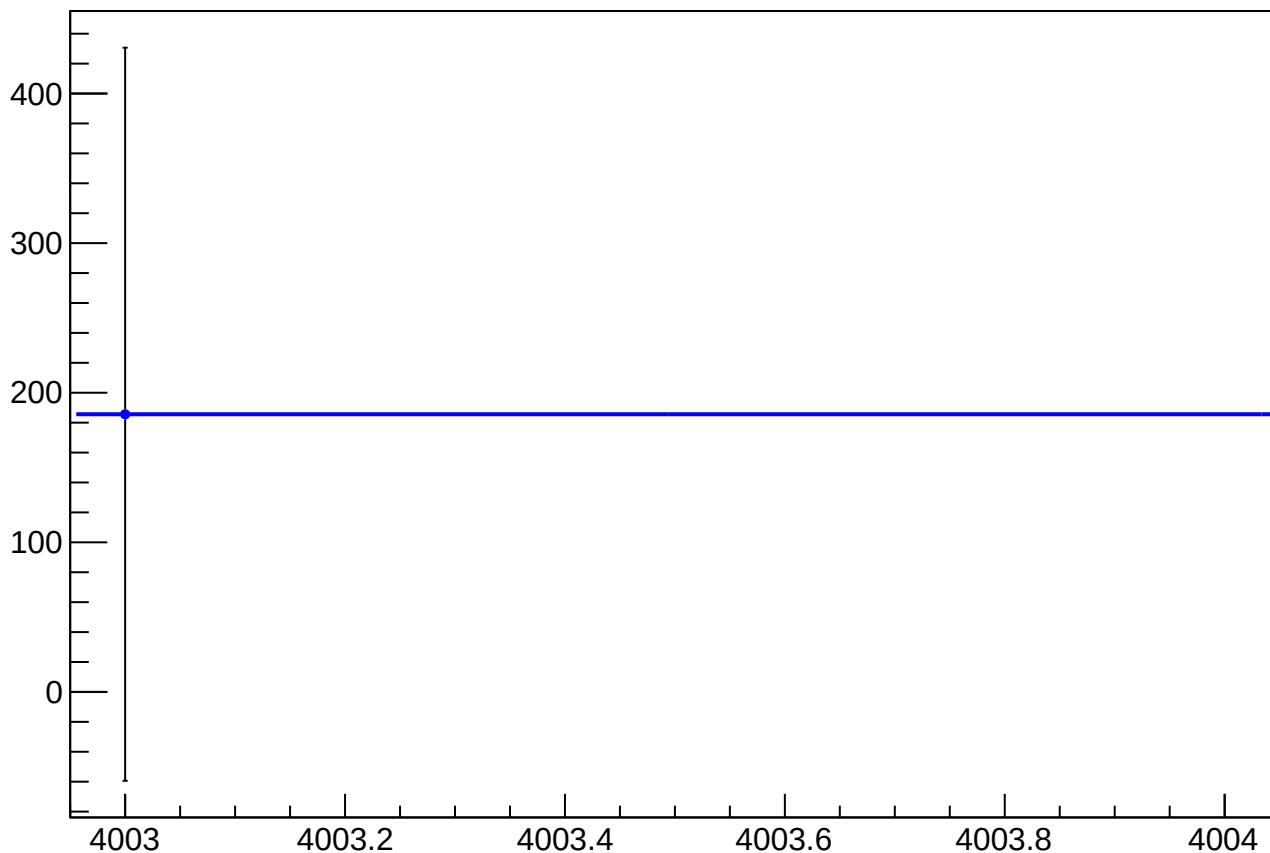
cor_asym_sam_37_avg_mean vs Slug, Sign Corrected
