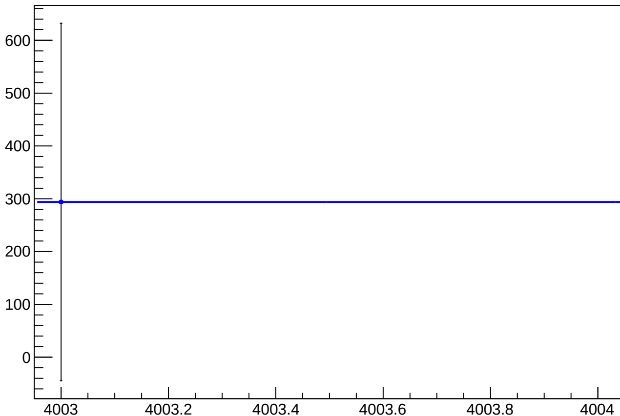
eigen_dit_asym_sam_3748_avg_mean vs Slug, Sign Corrected
