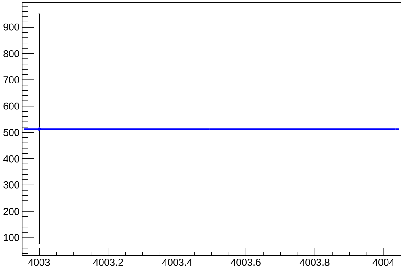
asym_atl_avg_atr_avg_dd_eigen_cor_correction_mean vs Slug, Sign Corrected
