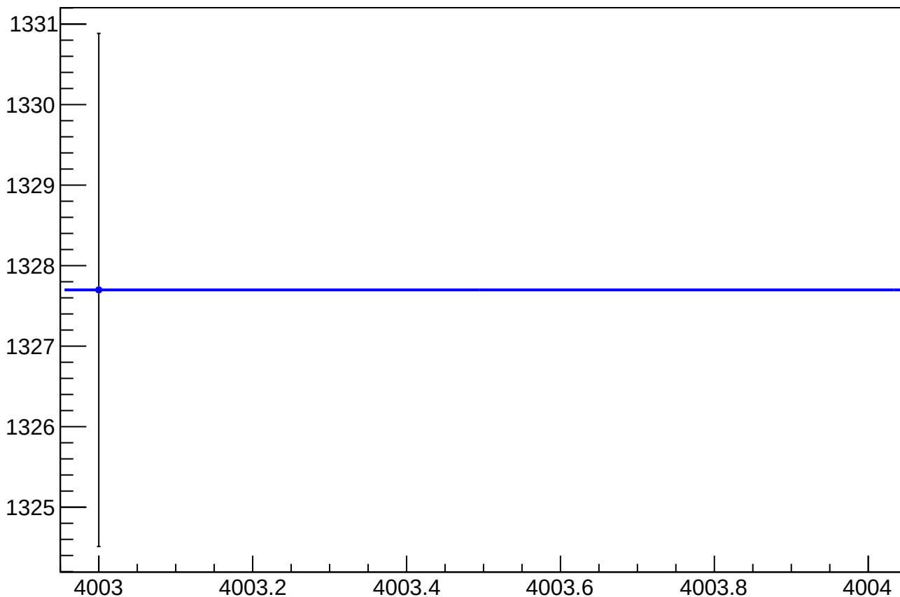
eigen_cor_asym_usl_atl1_avg_rms vs Slug, Sign Corrected
