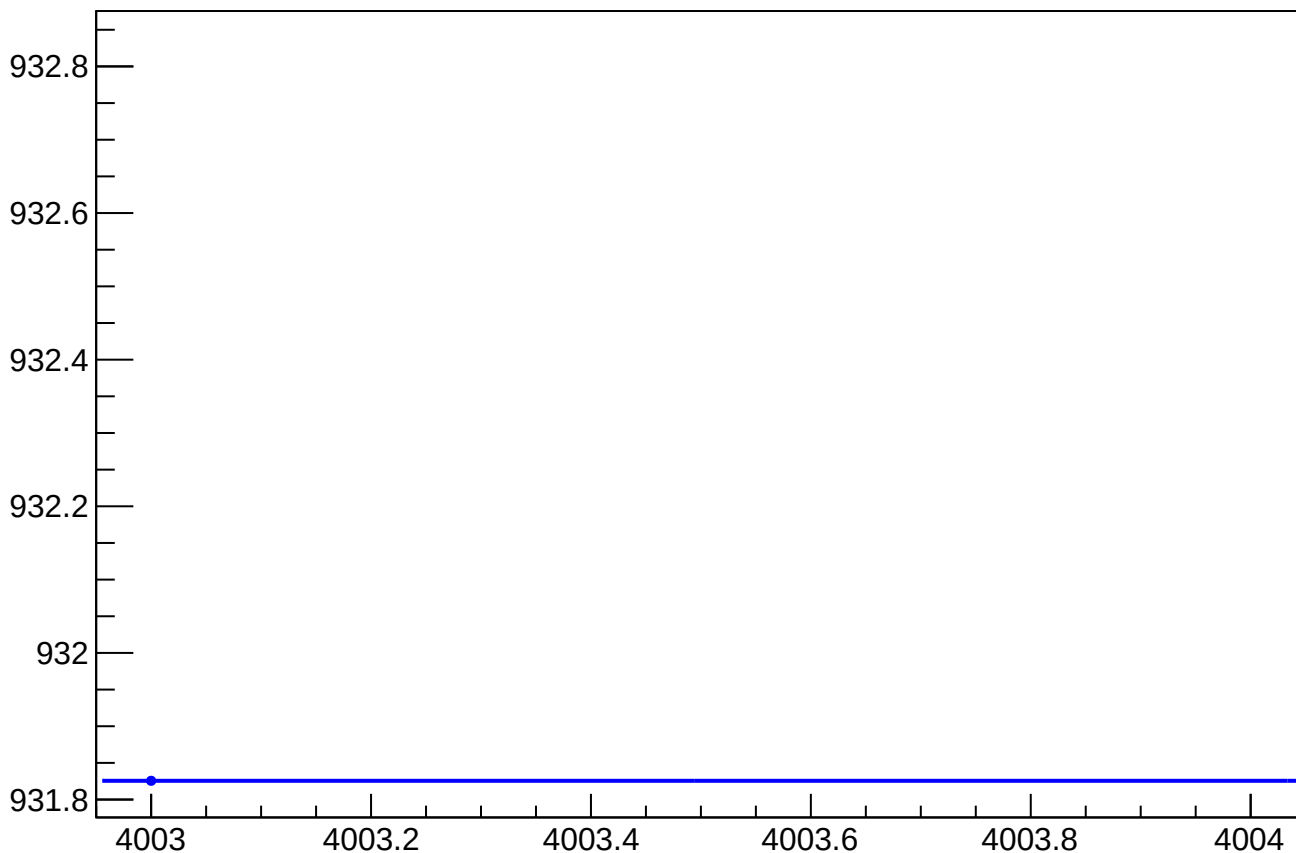
HacL_Q2_HP3458A_IOUT_mean vs Slug, Sign Corrected
