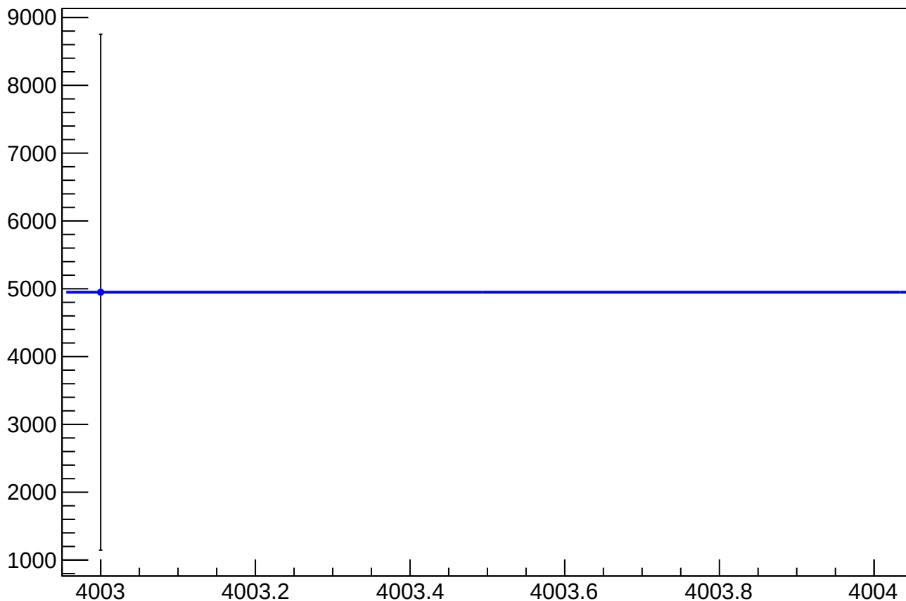
asym_us_dd_at1lr_dd_dd_eigen_dit_correction_mean vs Slug, Sign Corrected
