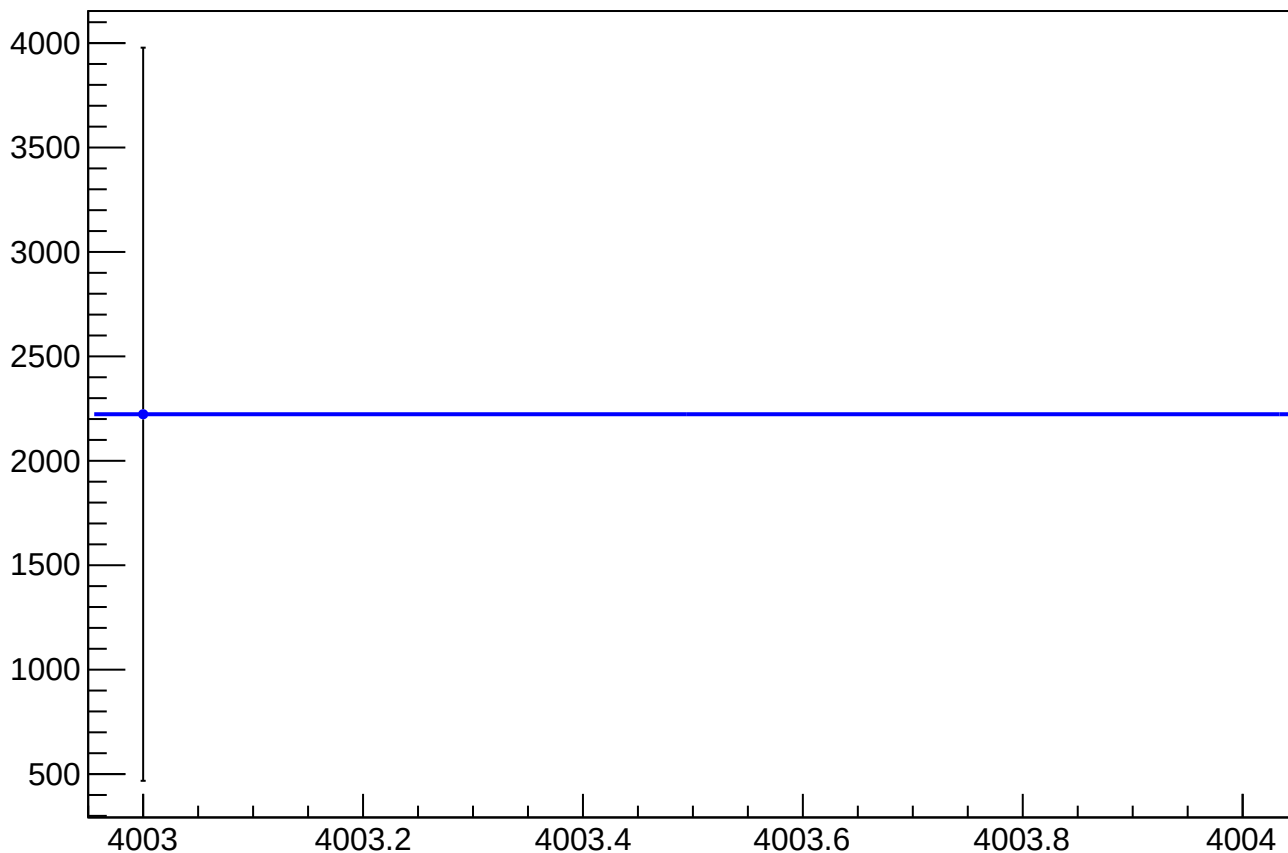
asym_sam_37_avg_dit_correction_mean vs Slug, Sign Corrected
