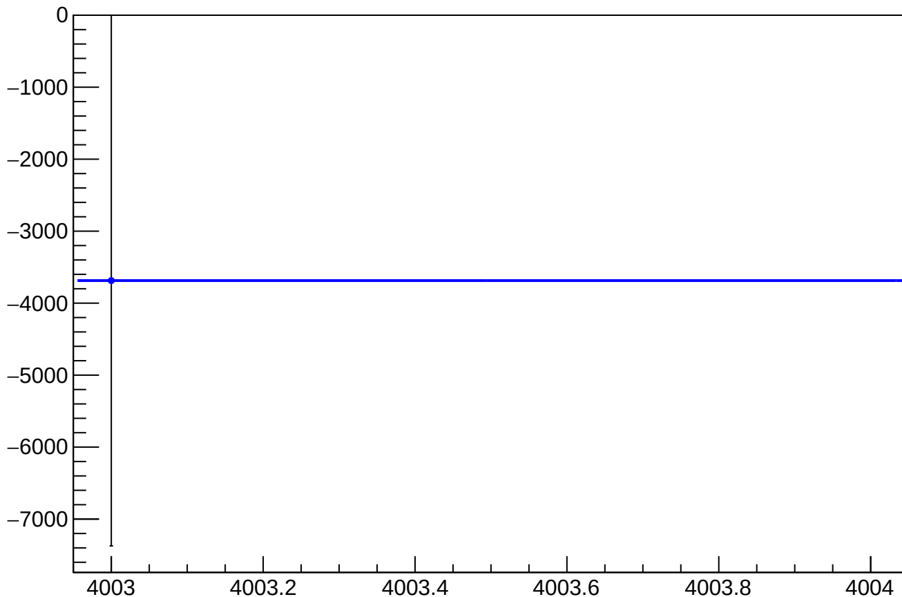
dit_asym_us_dd_atlr_dd_dd_mean vs Slug, Sign Corrected
