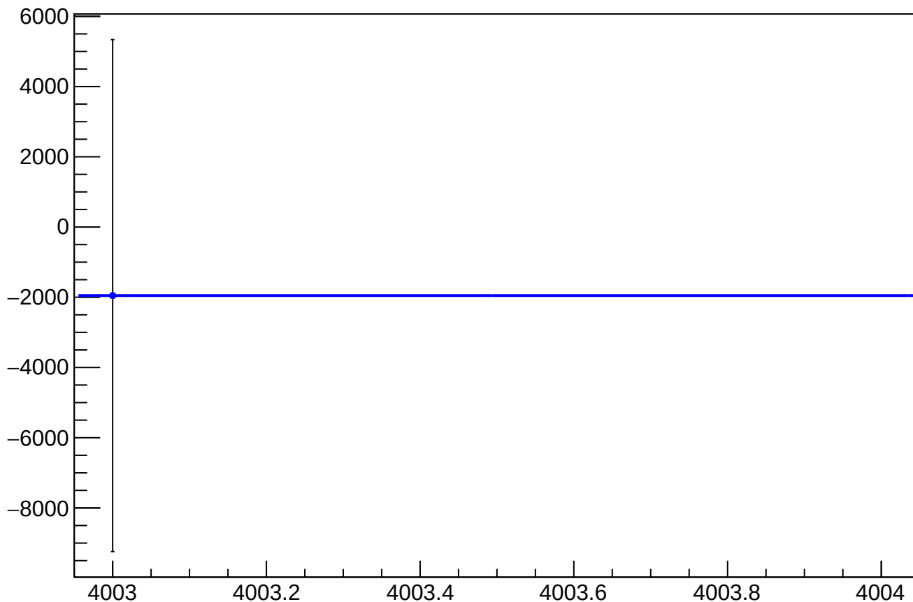
eigen_dit_asym_atl1_mean vs Slug, Sign Corrected
