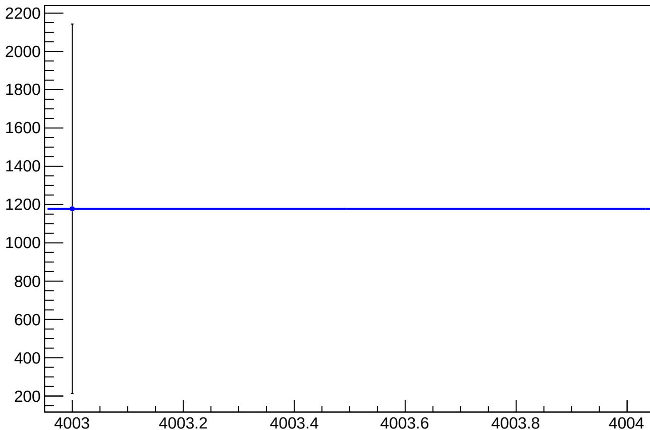
asym_sam_1526_avg_eigen_cor_correction_mean vs Slug, Sign Corrected
