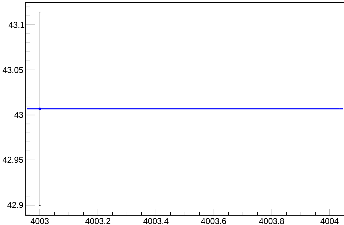
asym_us_dd_at1lr_dd_avg_eigen_dit_vs_cor_diff_rms vs Slug, Sign Corrected
