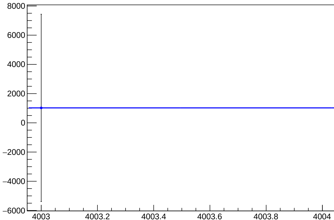
asym_usl_atl1_avg_eigen_dit_correction_mean vs Slug, Sign Corrected
