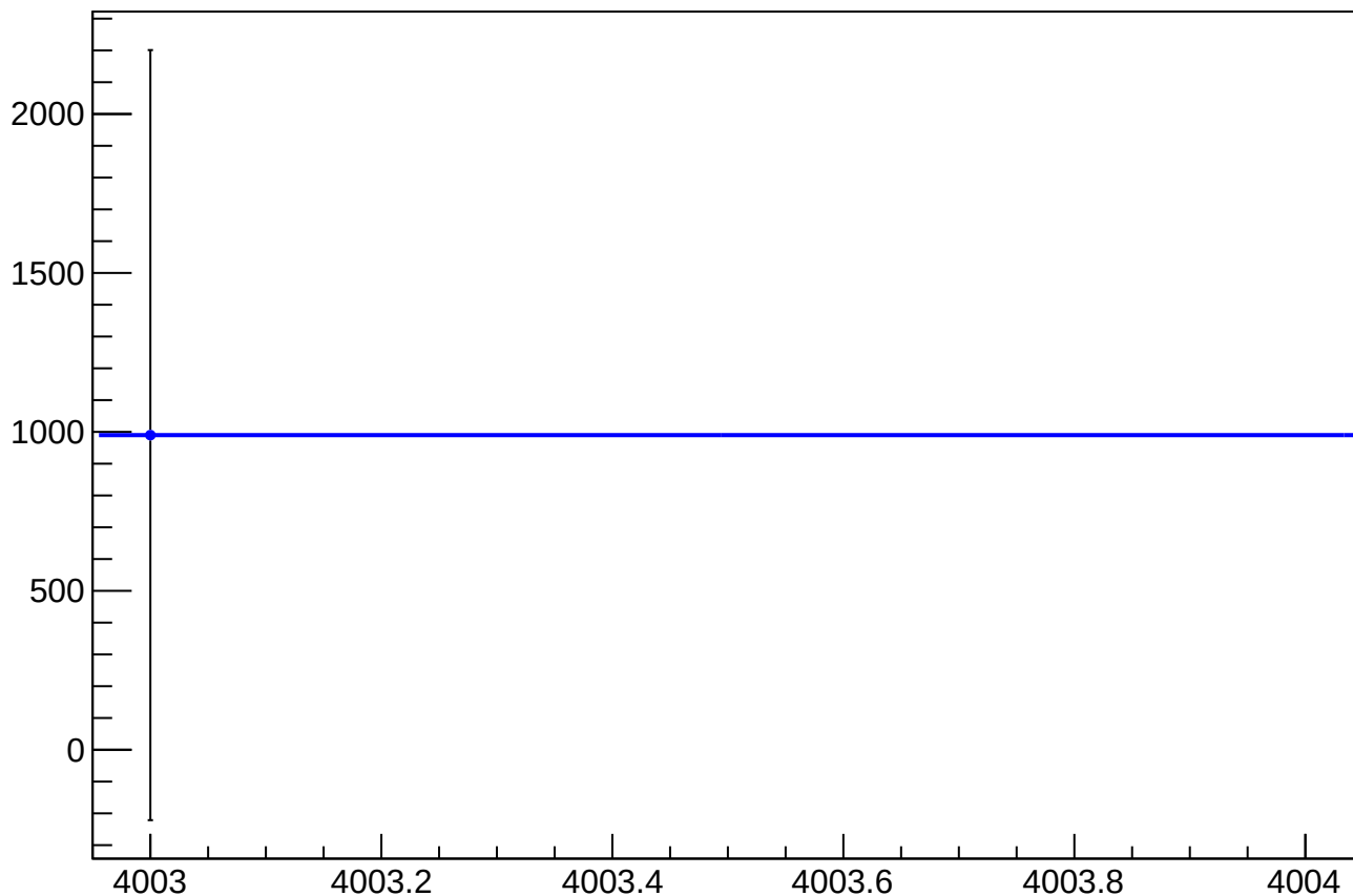
asym_sam_13_57_dd_eigen_dit_correction_mean vs Slug, Sign Corrected
