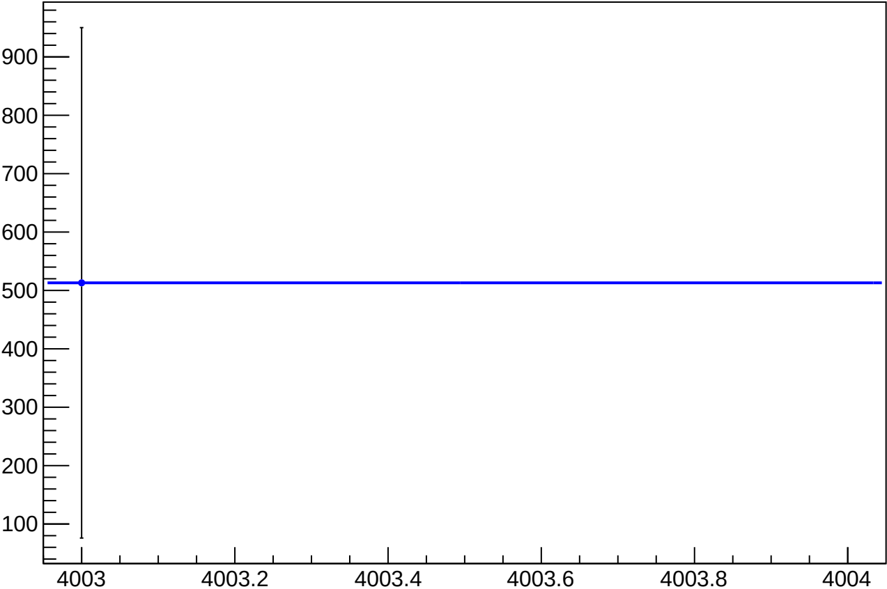
asym_atl_avg_atr_avg_dd_cor_correction_mean vs Slug, Sign Corrected
