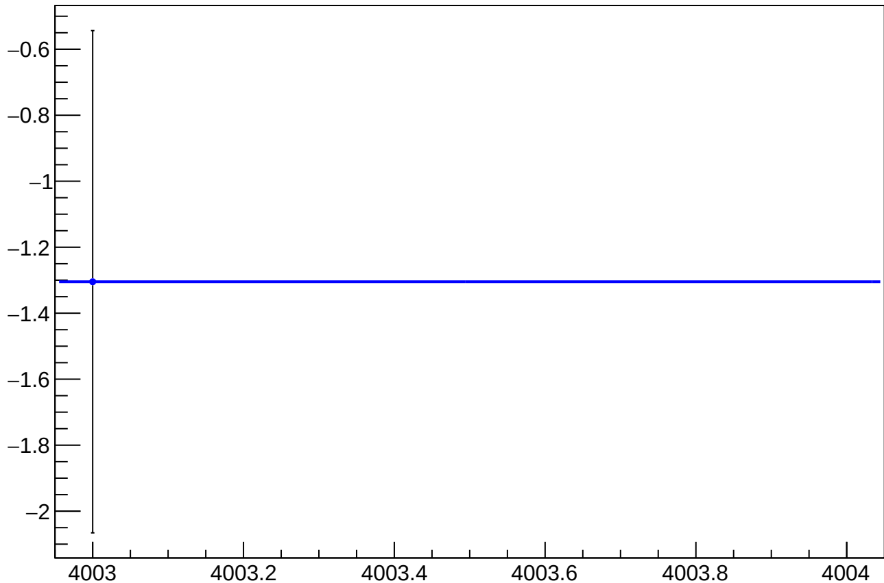
asym_atl_avg_dit_vs_eigen_cor_diff_mean vs Slug, Sign Corrected
