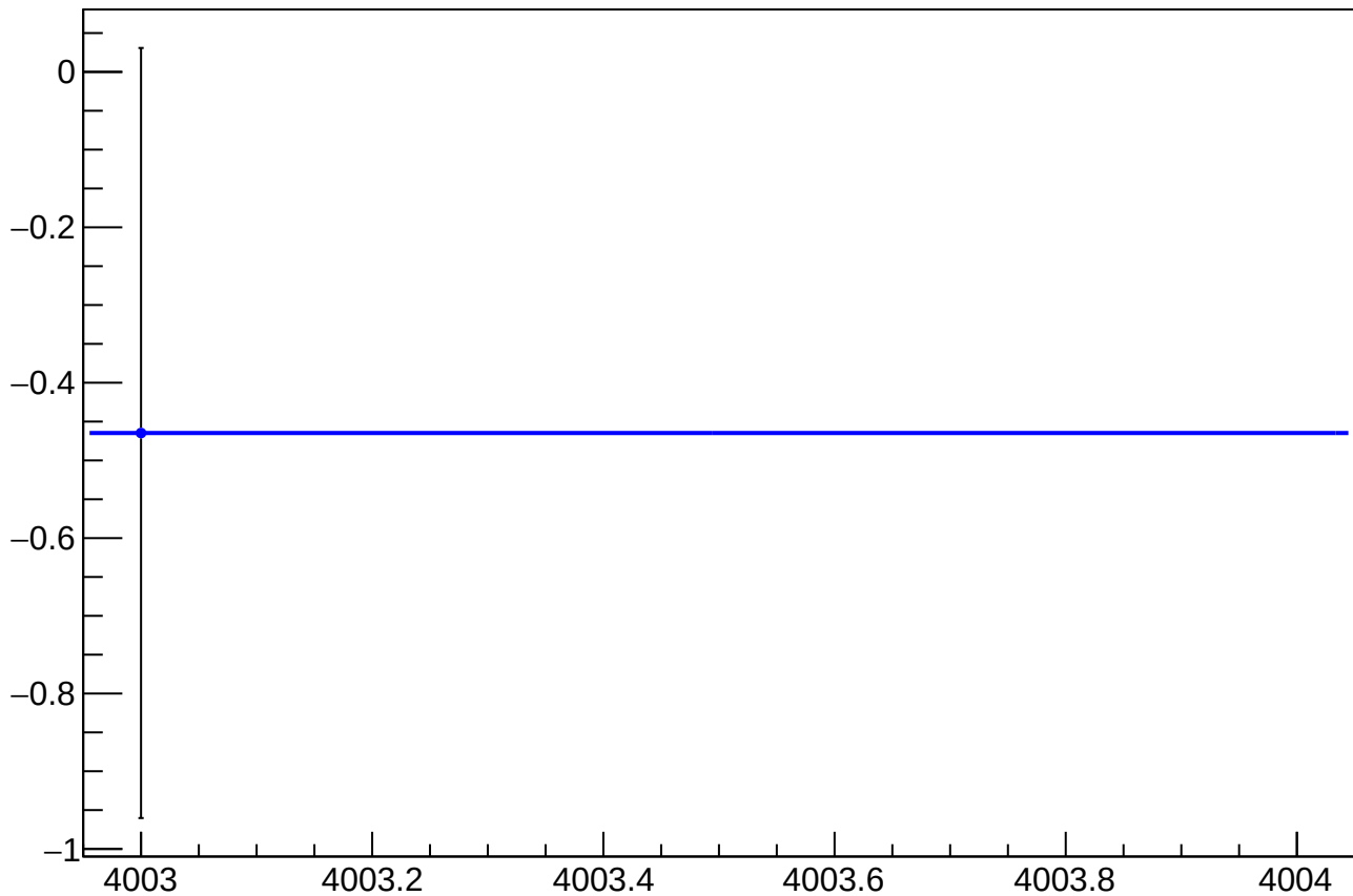
asym_usr_atr1_avg_dit_vs_eigen_cor_diff_mean vs Slug, Sign Corrected
