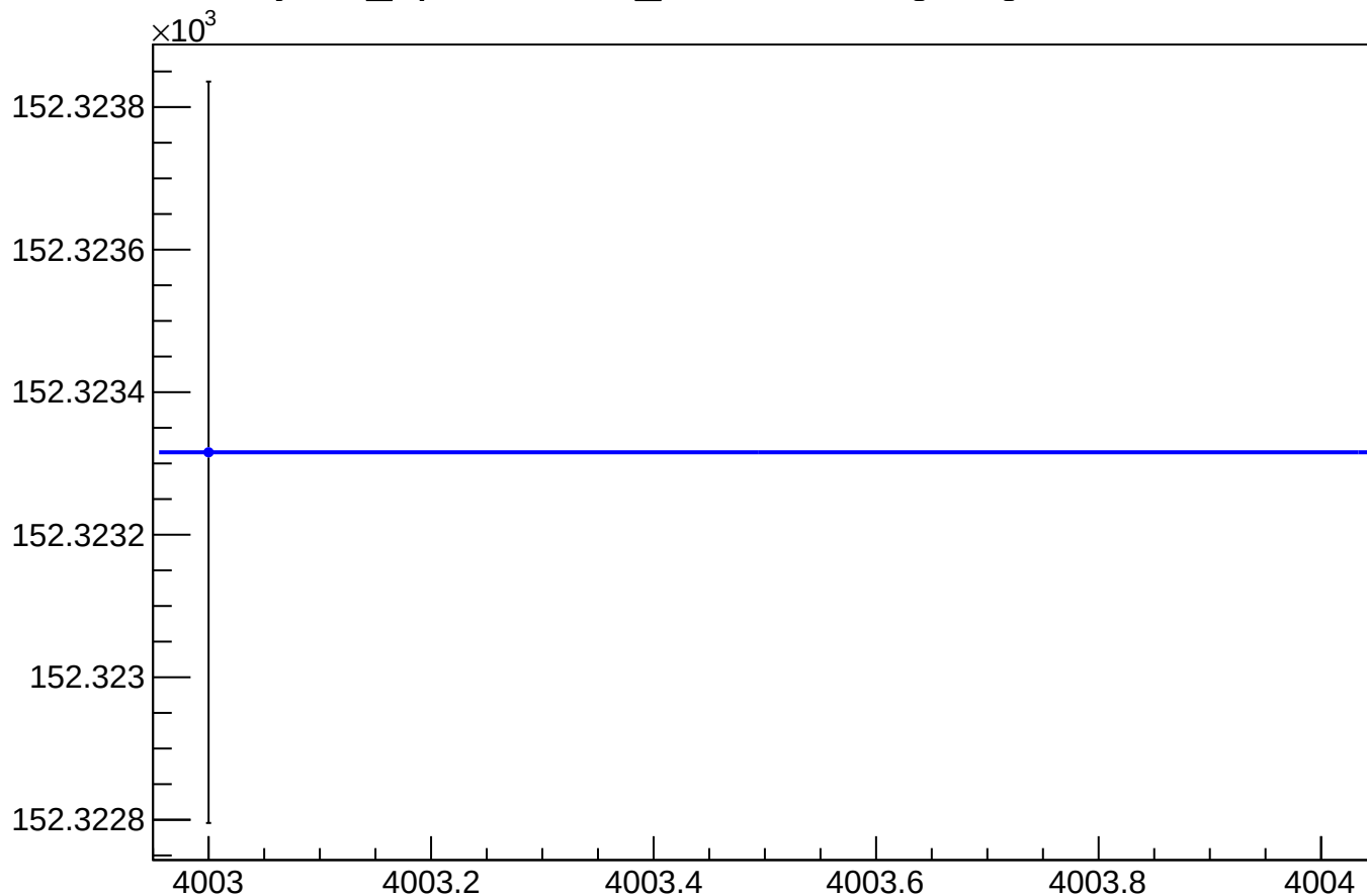
yield_bpm2i01WS_mean vs Slug, Sign Corrected
