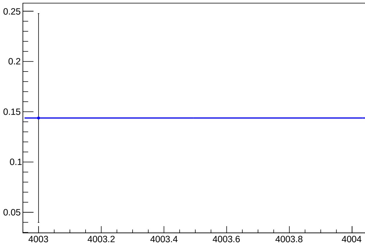
asym_us_dd_overload_cor_vs_eigen_cor_diff_mean vs Slug, Sign Corrected
