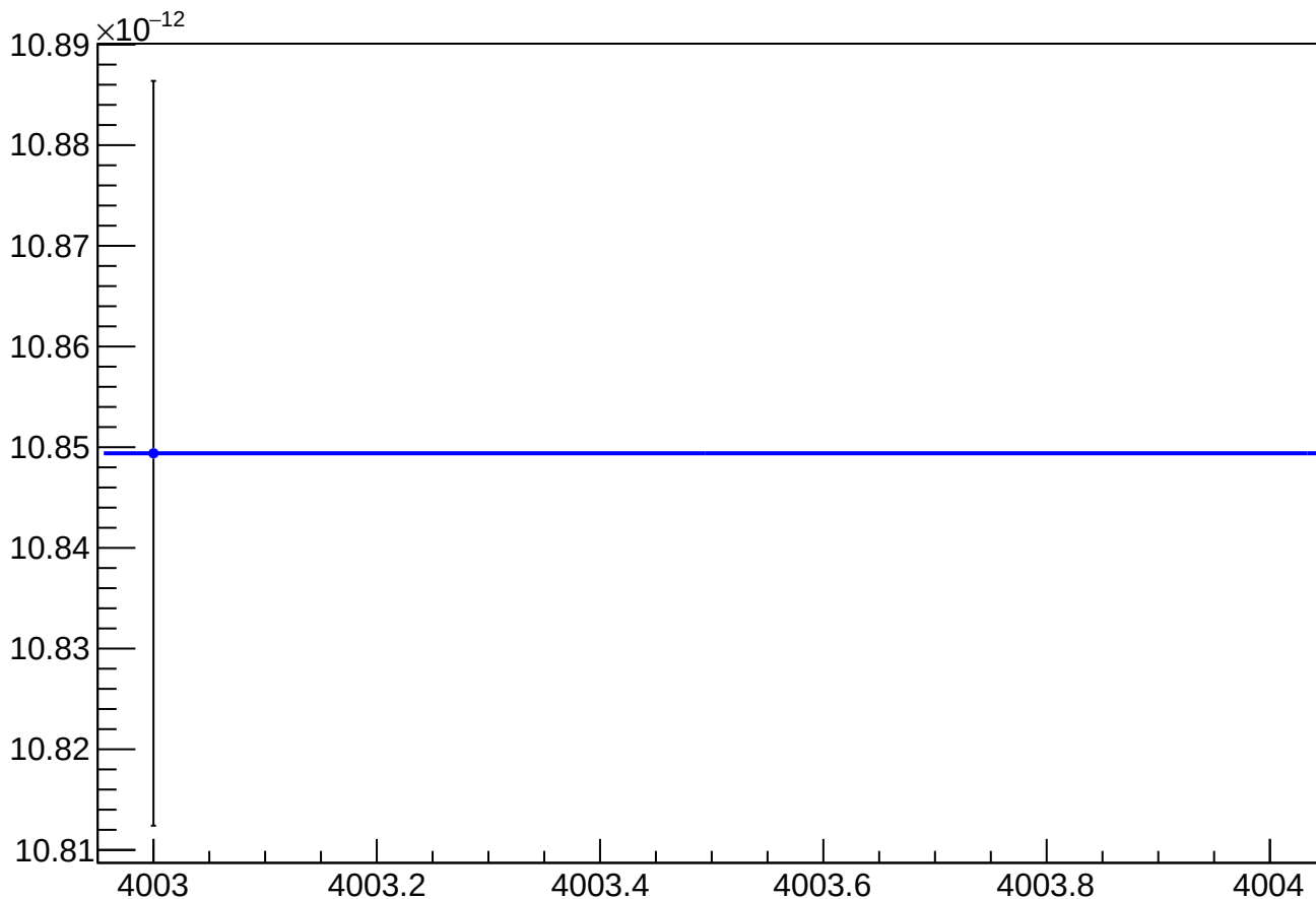
asym_sam_37_26_dd_reg_vs_cor_diff_rms vs Slug, Sign Corrected
