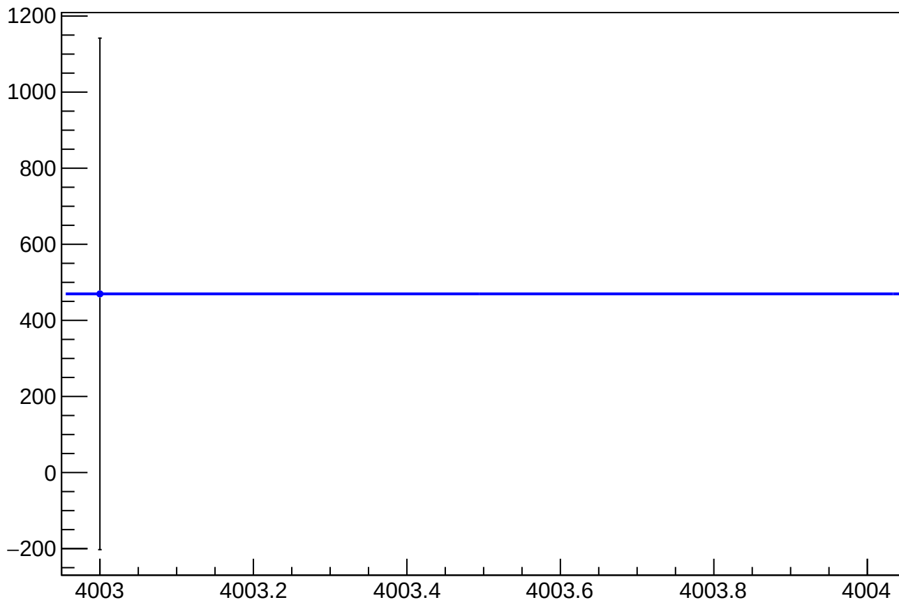
asym_sam8_cor_correction_mean vs Slug, Sign Corrected
