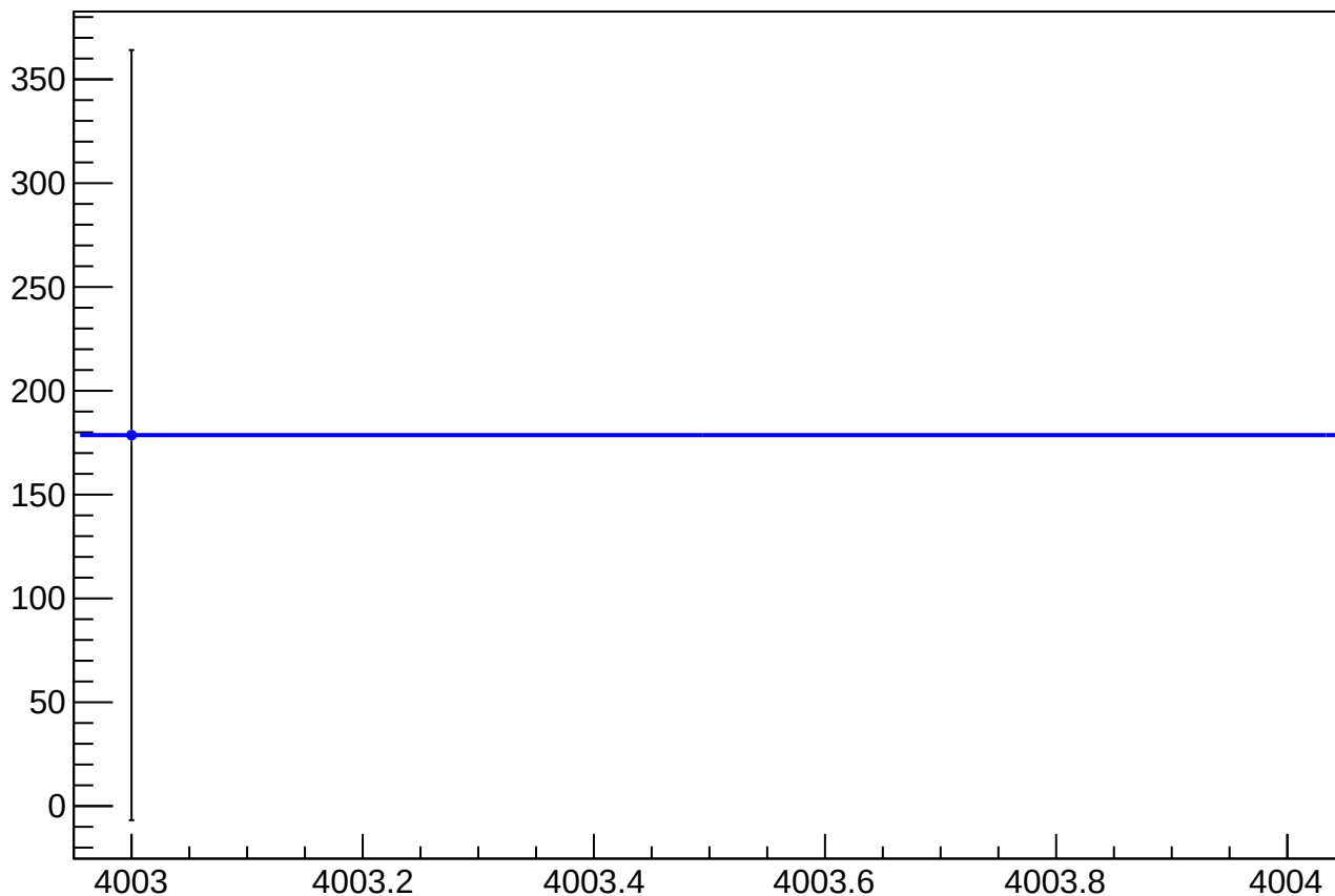
eigen_dit_asym_sam_1526_avg_mean vs Slug, Sign Corrected
