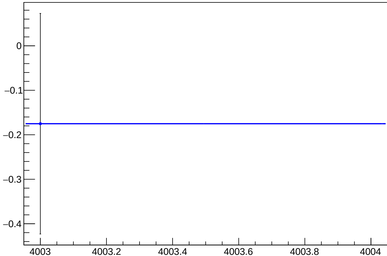
asym_us_avg_at1lr_avg_dd_eigen_dit_vs_cor_diff_mean vs Slug, Sign Corrected
