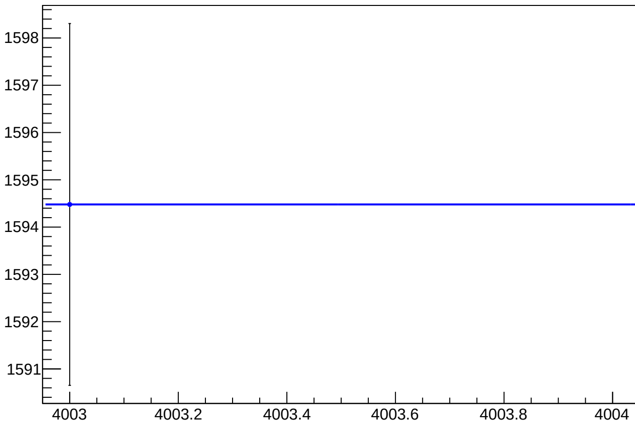
cor_asym_us_dd_at1lr_dd_dd_rms vs Slug, Sign Corrected
