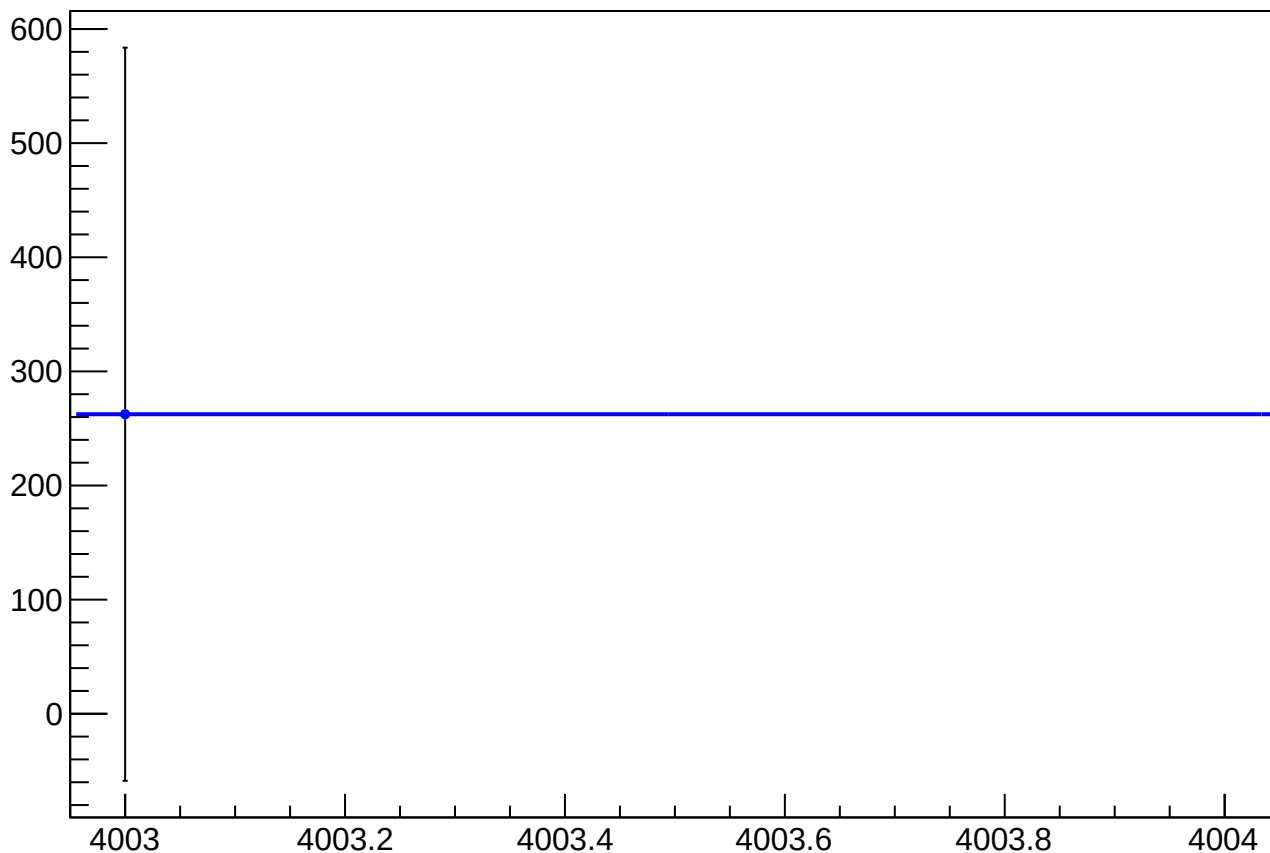
eigen_cor_asym_sam_3748_avg_mean vs Slug, Sign Corrected
