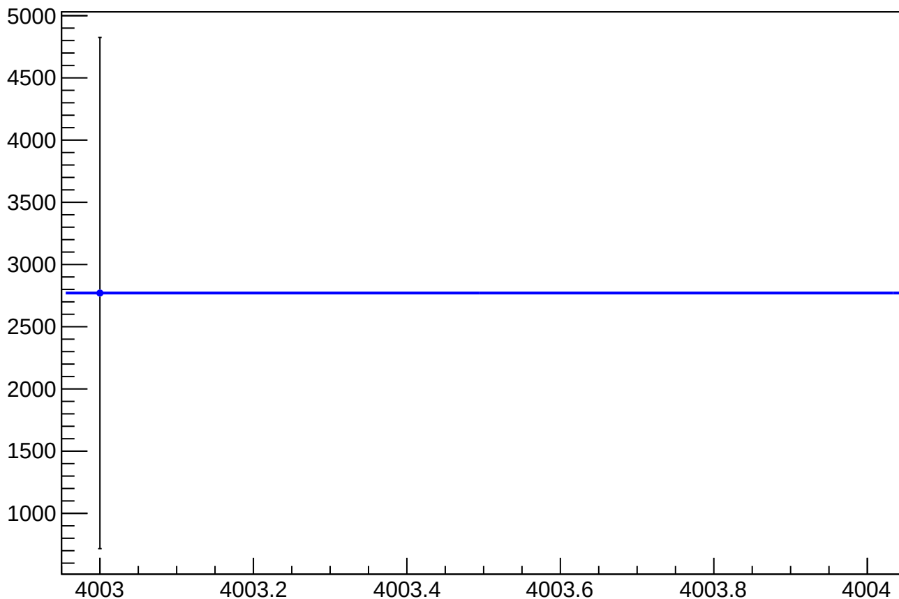
asym_sam_3726_avg_eigen_dit_correction_mean vs Slug, Sign Corrected
