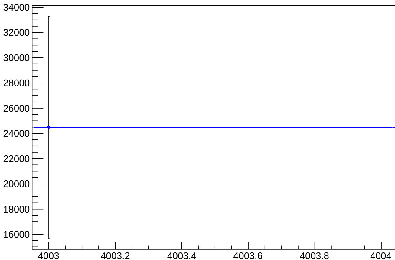
eigen_cor_asym_atr2_mean vs Slug, Sign Corrected
