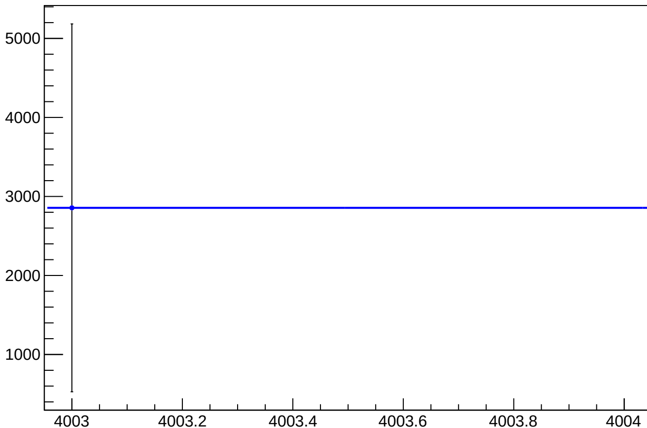
asym_us_dd_atlr_dd_avg_cor_correction_mean vs Slug, Sign Corrected
