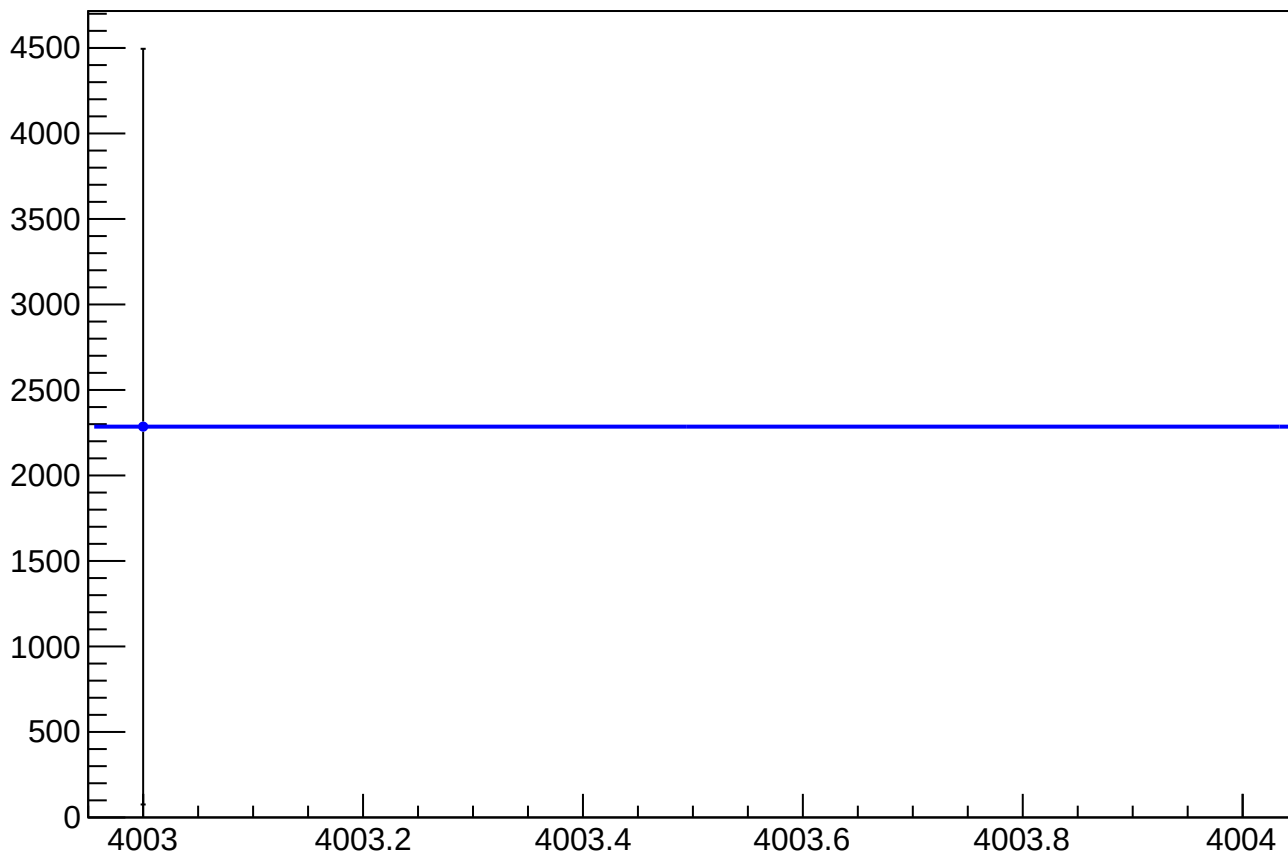
asym_usl_atl1_dd_eigen_dit_correction_mean vs Slug, Sign Corrected
