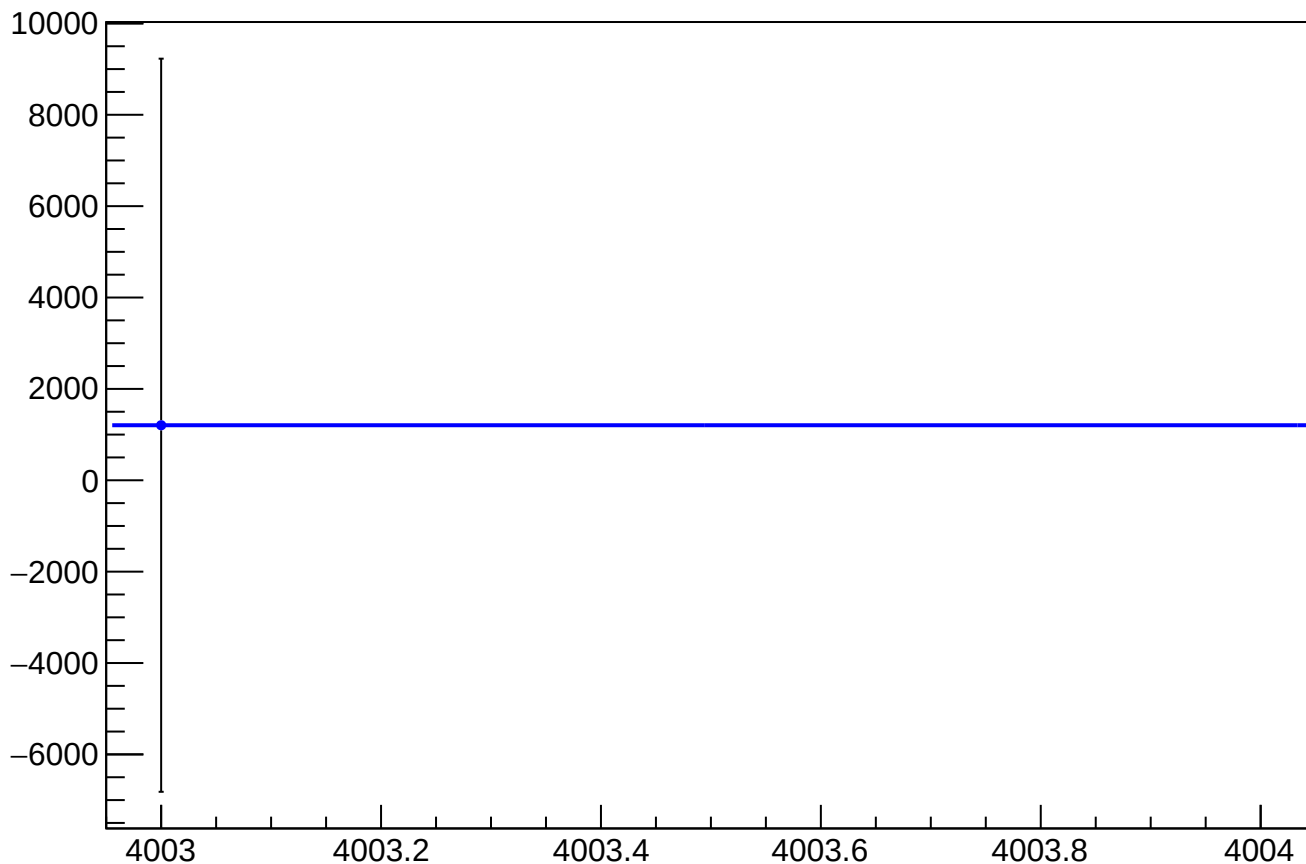
asym_usr_atr1_avg_dit_correction_mean vs Slug, Sign Corrected
