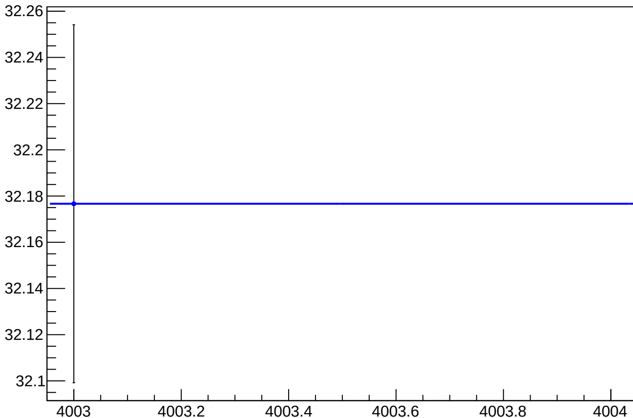
asym_sam_15_26_dd_dit_vs_eigen_cor_diff_rms vs Slug, Sign Corrected
