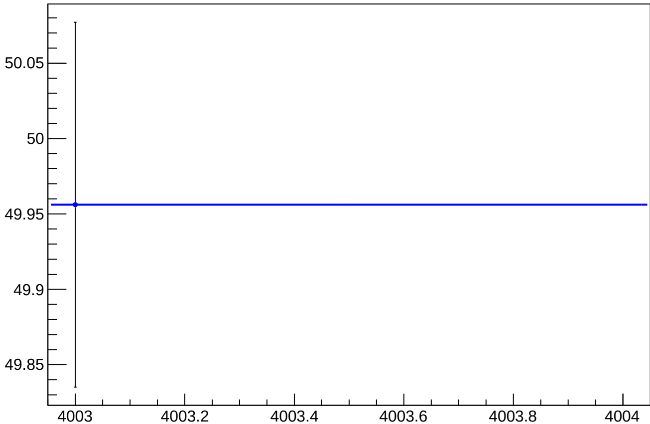
asym_usr_atr1_dd_dit_vs_eigen_cor_diff_rms vs Slug, Sign Corrected
