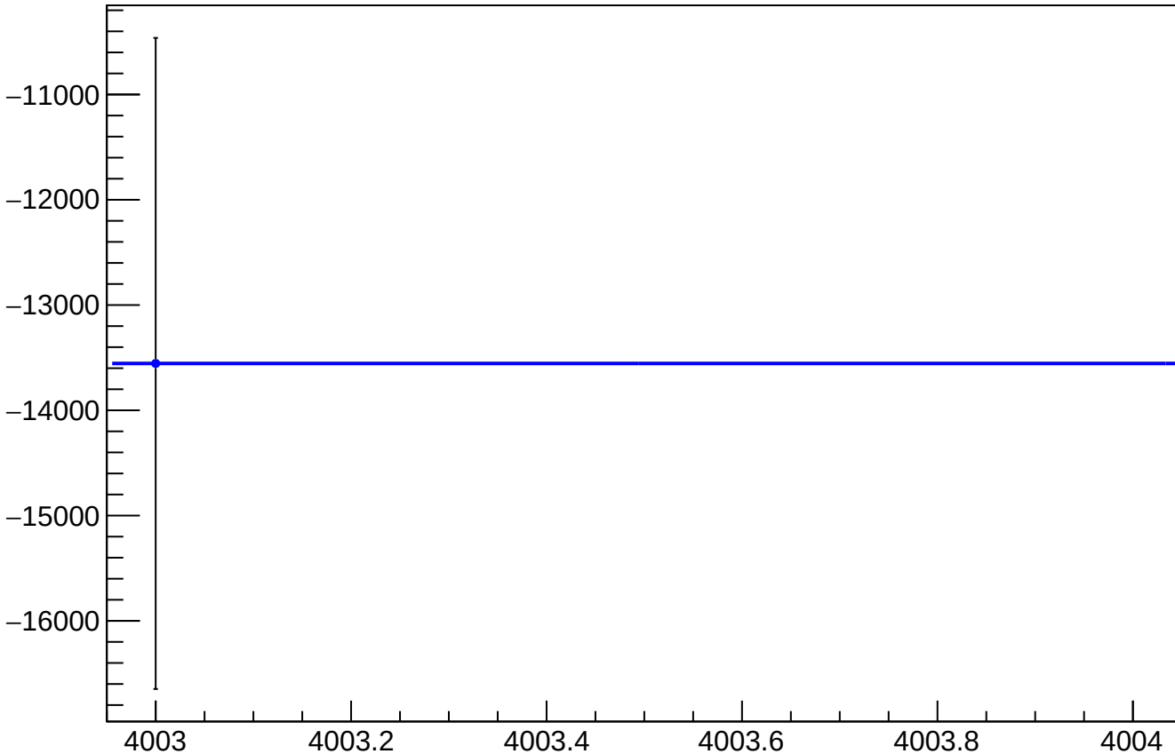
asym us dd mean vs Slug, Sign Corrected
