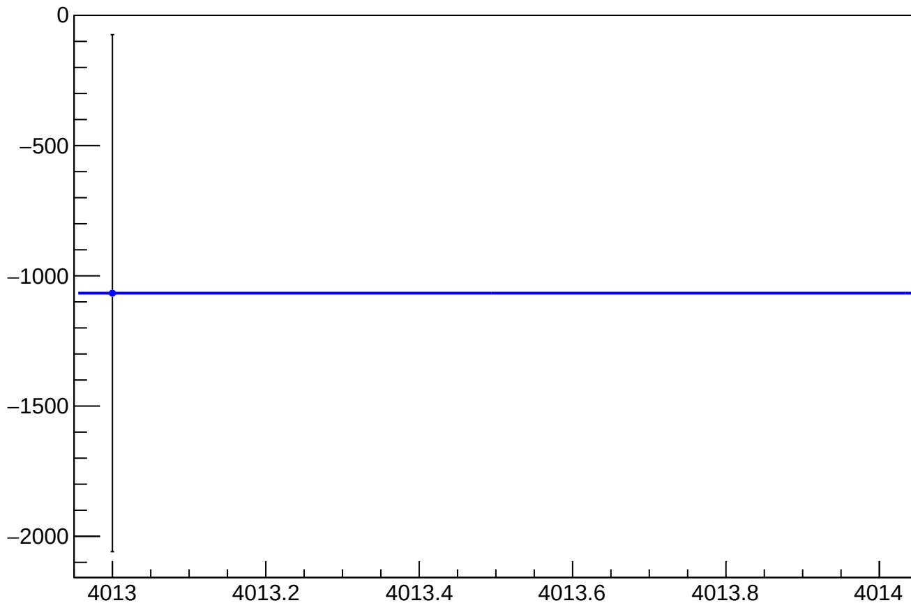
asym_sam7_cor_correction_mean vs Slug
