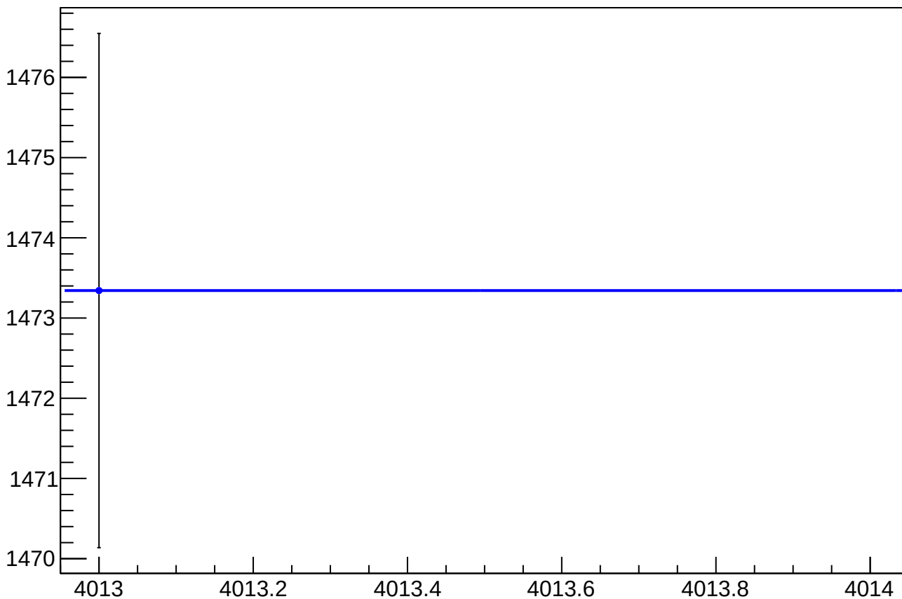
eigen_dit_asym_us_avg_atlr_avg_avg_rms vs Slug
