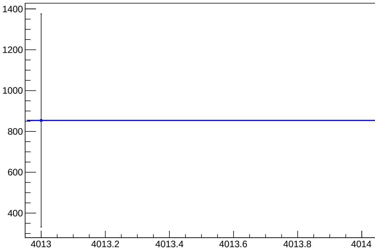
reg_asym_sam_3726_avg_mean vs Slug
