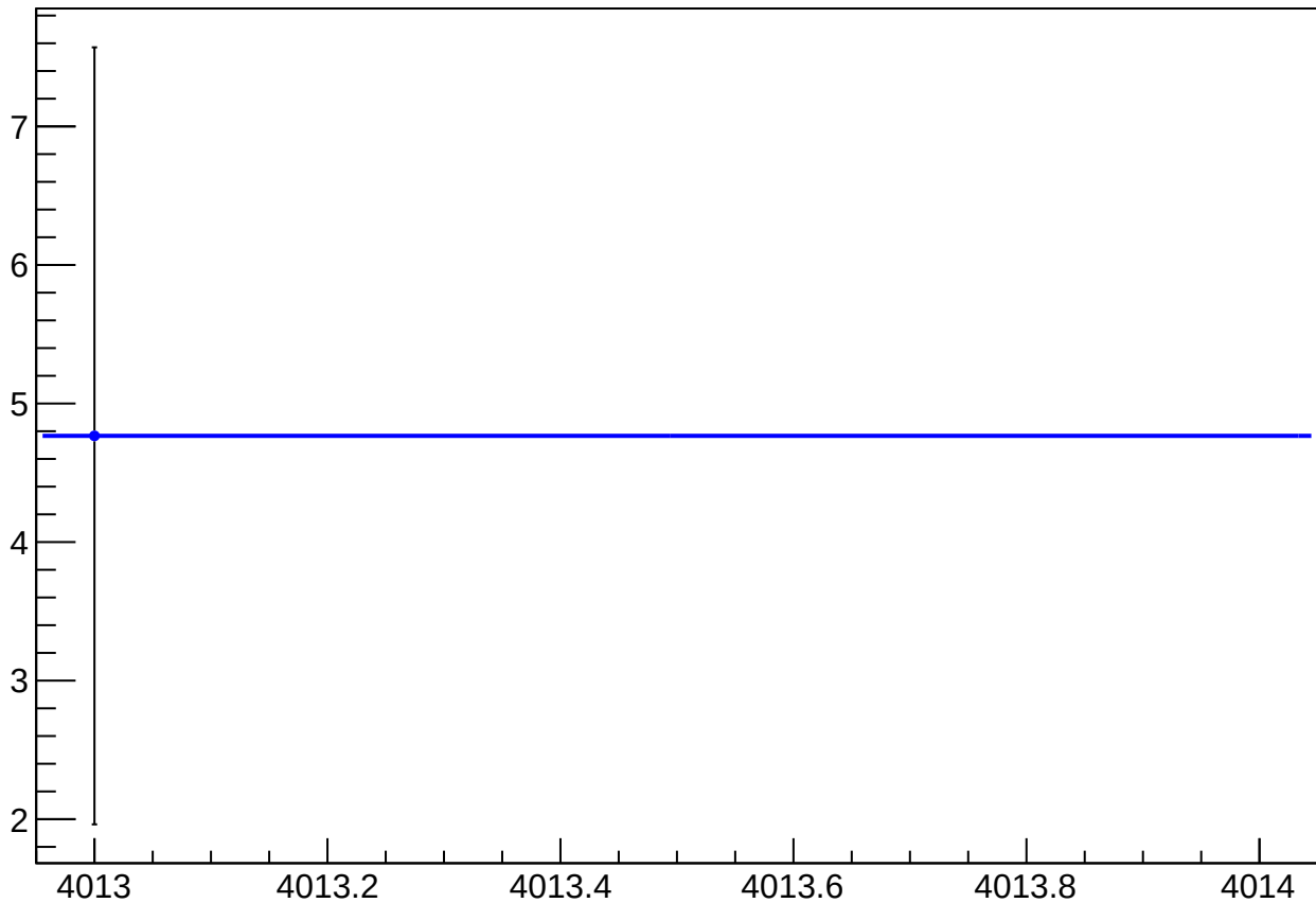
reg_asym_atl_avg_atr_avg_dd_diff_bpm1X_slope vs Slug
