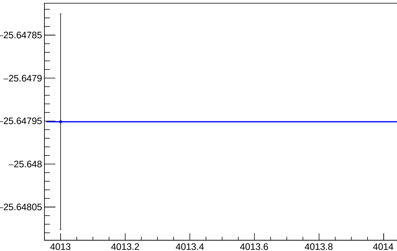
yield_dsl_mean vs Slug
