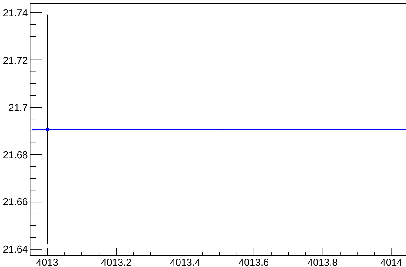
asym_us_dd_overload_cor_vs_eigen_cor_diff_rms vs Slug
