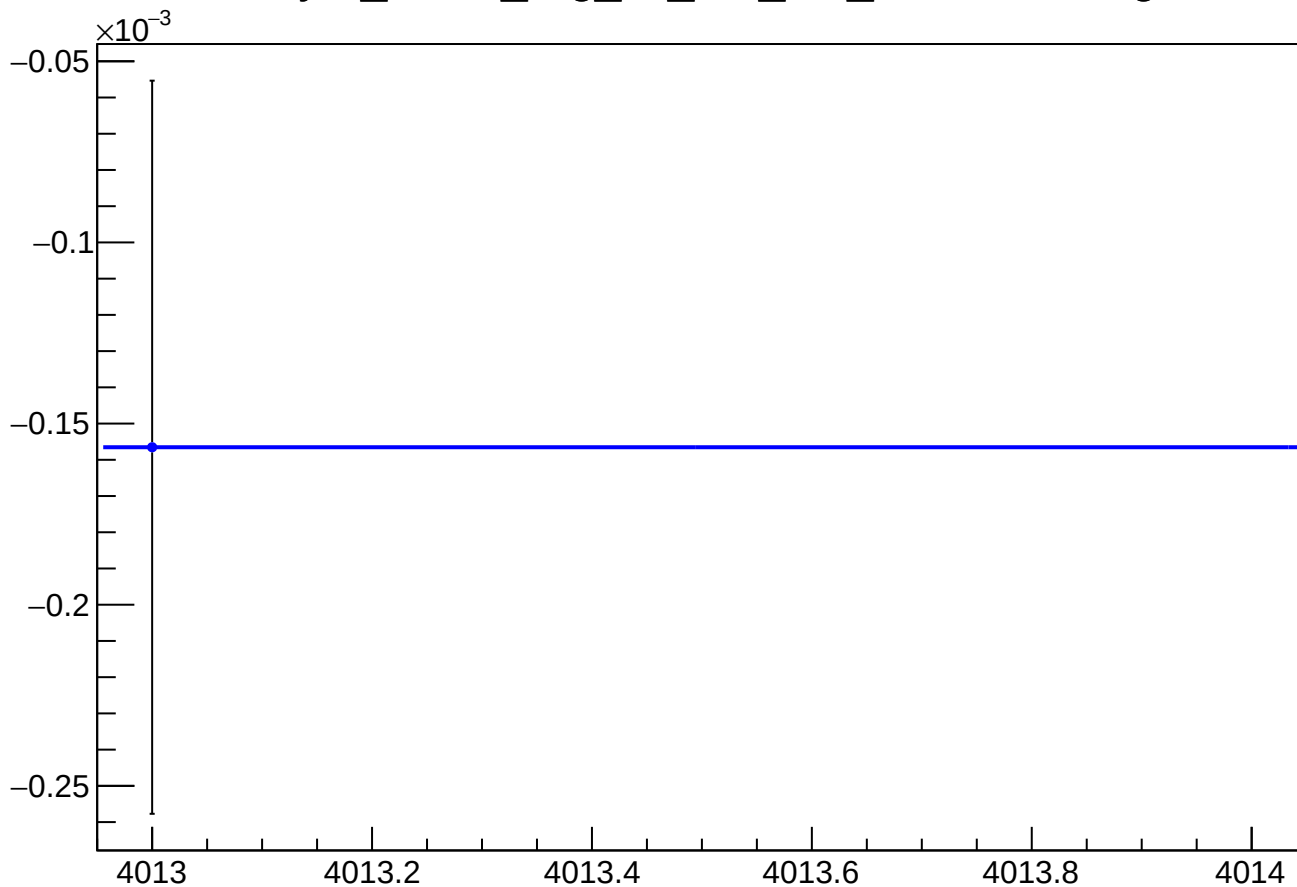
asym_sam6_reg_vs_cor_diff_mean vs Slug
