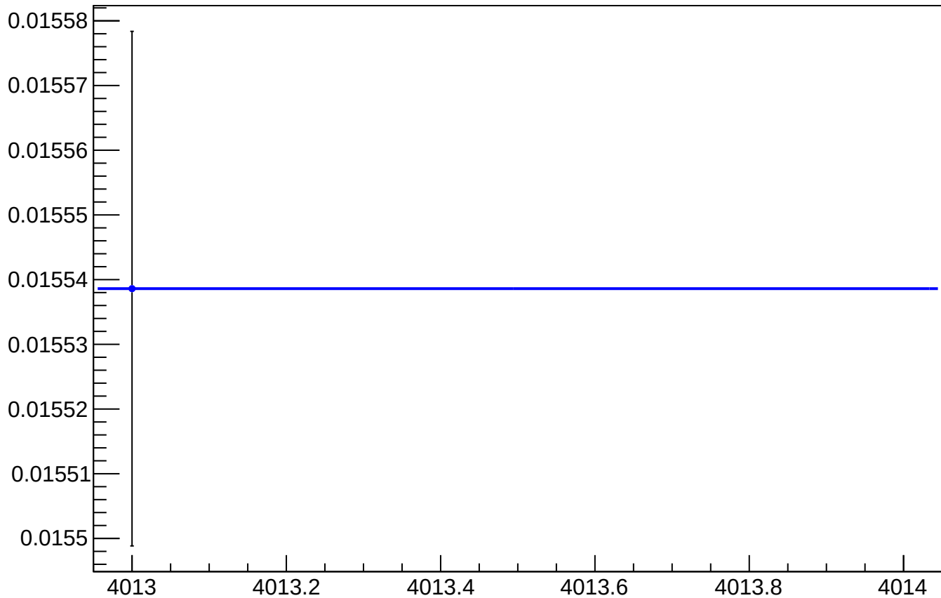
asym_sam_13_57_dd_reg_vs_cor_diff_rms vs Slug
