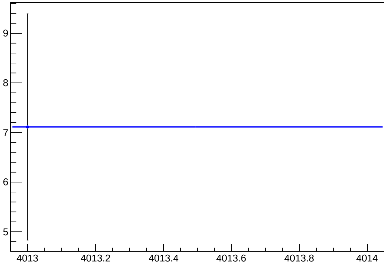
reg_asym_atl_avg_atr_avg_dd_diff_bpm4eY_slope vs Slug
