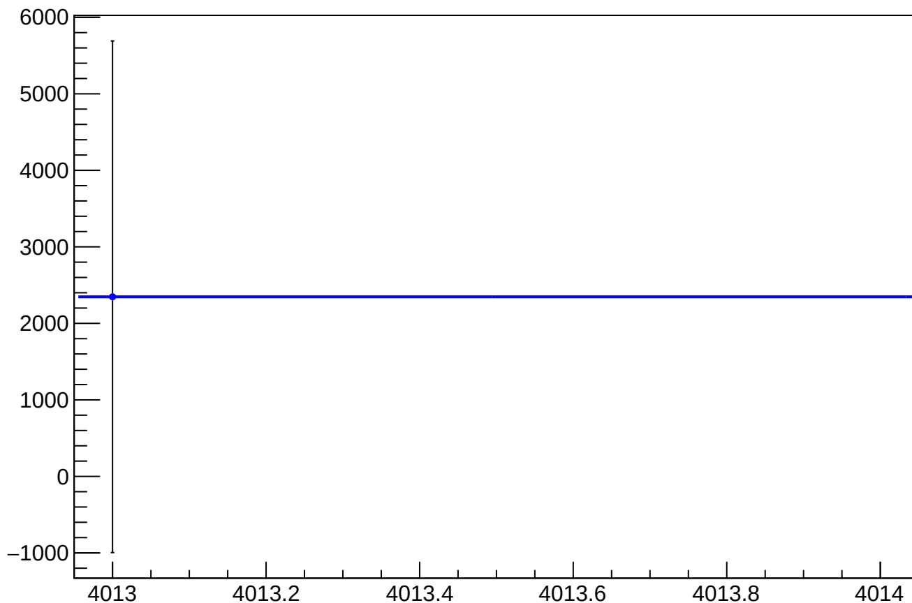
asym_sam5_cor_correction_mean vs Slug
