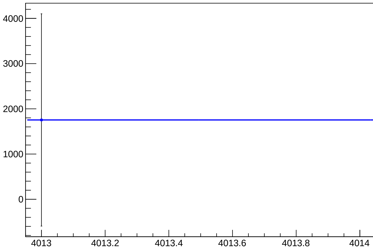
asym_at1_dd_at2_dd_avg_reg_correction_mean vs Slug
