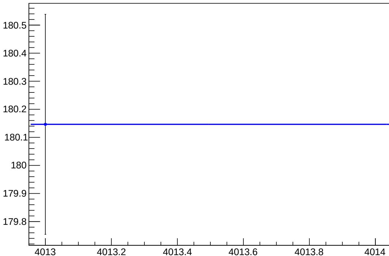
eigen_cor_asym_sam_2468_avg_rms vs Slug
