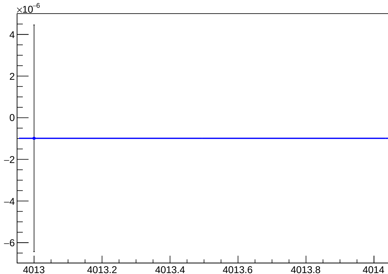
asym_sam_1526_avg_eigen_dit_vs_dit_diff_mean vs Slug
