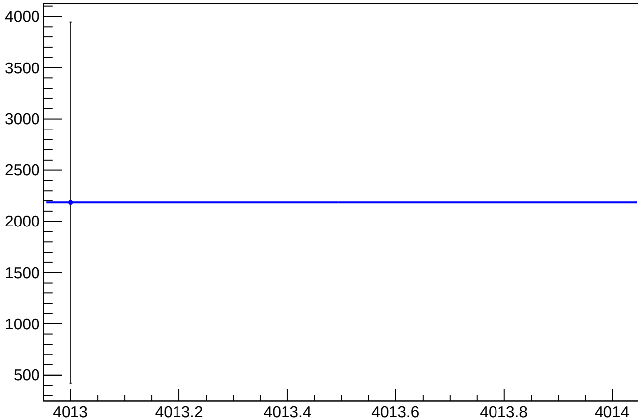
asym_sam_15_26_dd_eigen_dit_correction_mean vs Slug
