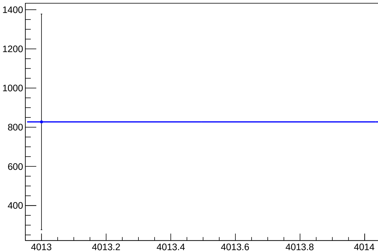
dit_asym_sam_3726_avg_mean vs Slug
