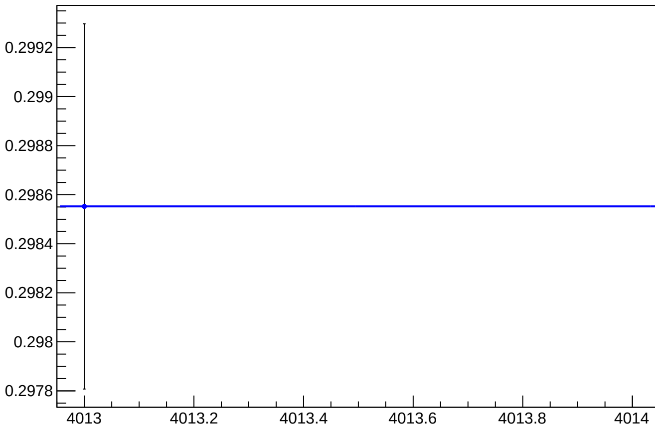
asym_us_avg_at2lr_avg_dd_reg_vs_cor_diff_rms vs Slug
