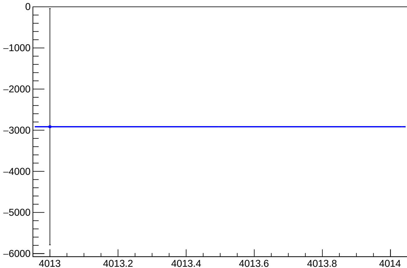
reg_asym_us_avg_atlr_avg_dd_mean vs Slug
