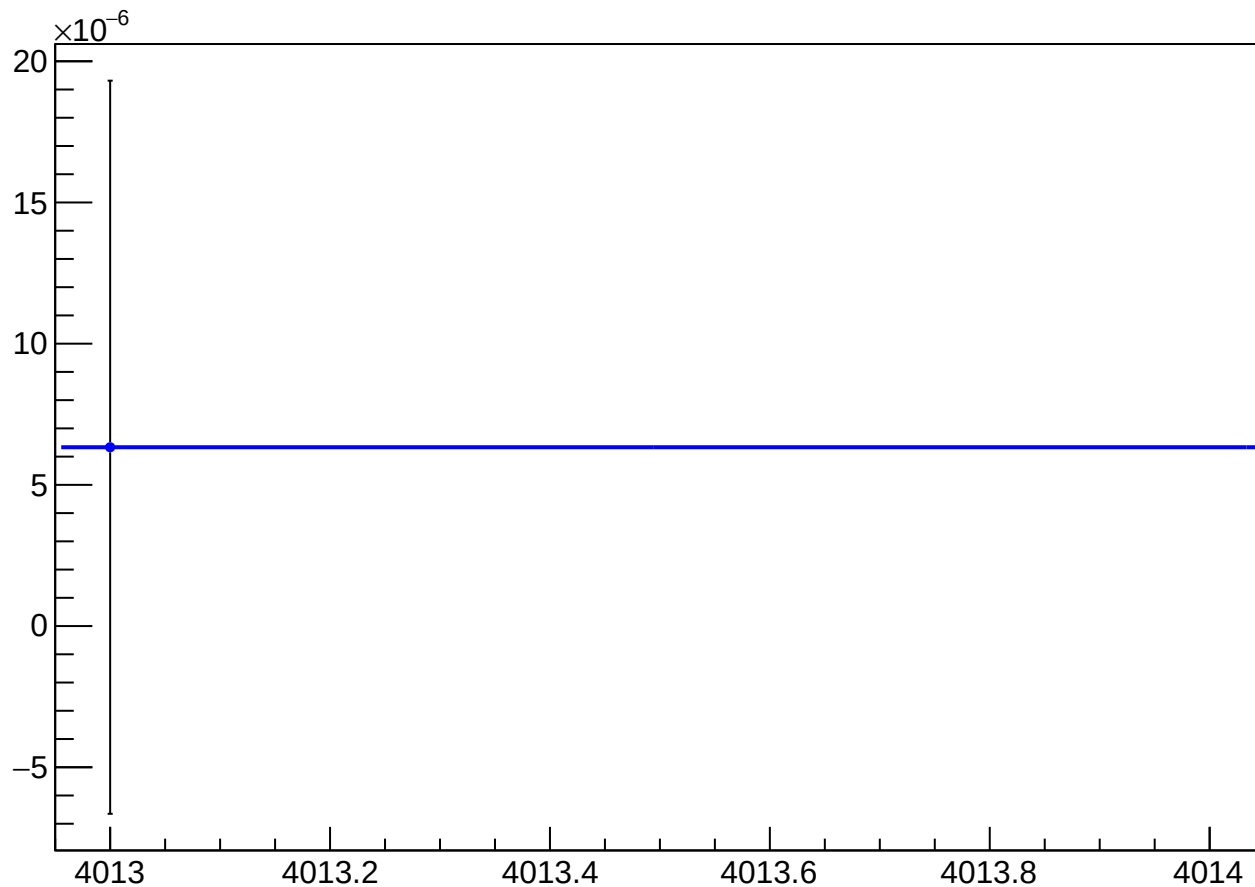
asym_usl_atl1_dd_eigen_dit_vs_dit_diff_mean vs Slug
