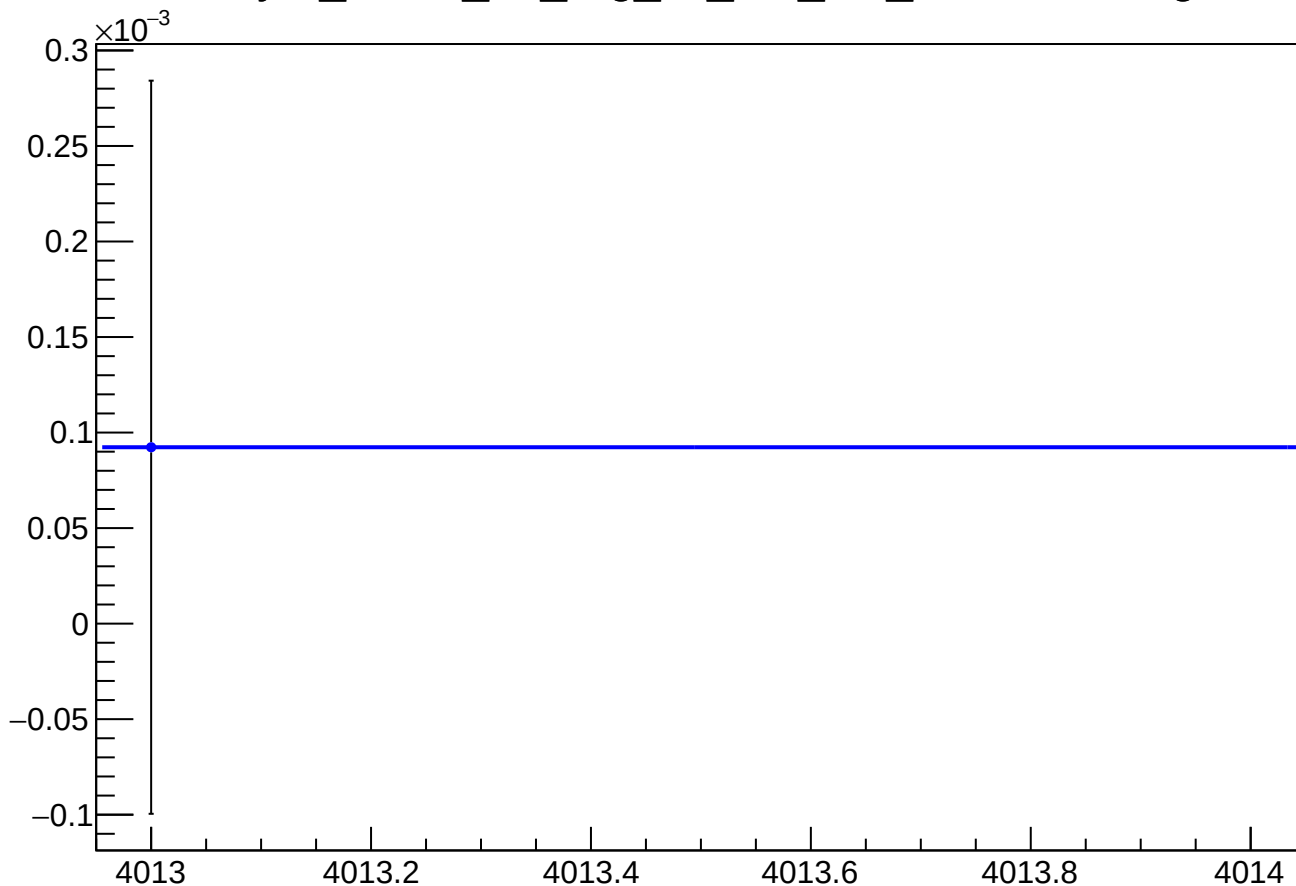
asym_atl1r2_dd_reg_vs_cor_diff_mean vs Slug
