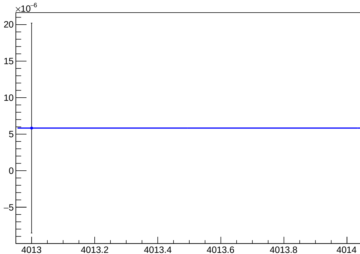
asym_atl_dd_atr_dd_dd_eigen_dit_vs_dit_diff_mean vs Slug
