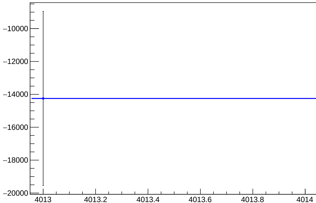
asym_us_dd_at1lr_dd_avg_mean vs Slug
