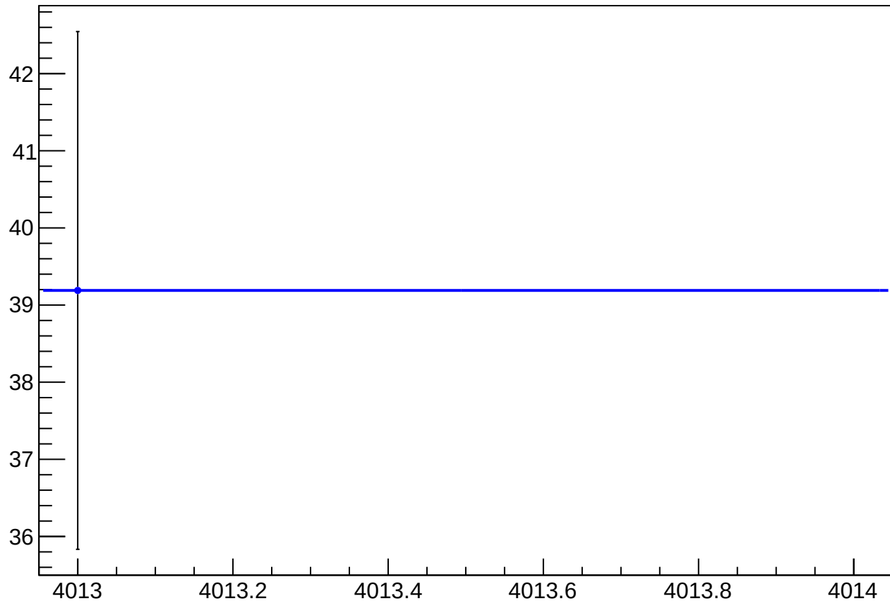
reg_asym_usr_atr1_dd_diff_bpm4eX_slope vs Slug
