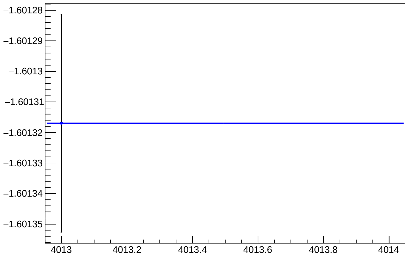
yield_bpm0i05Y_mean vs Slug
