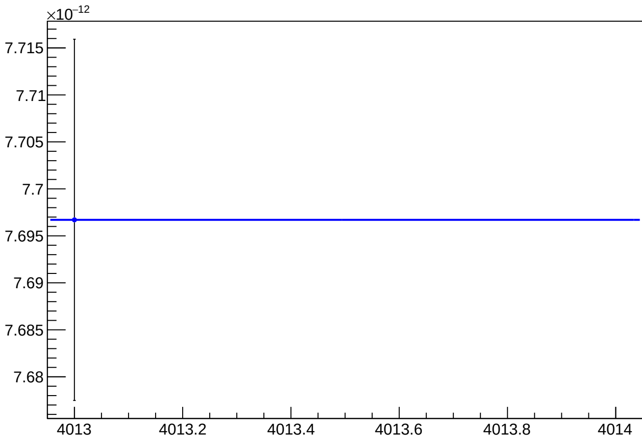
asym_sam_15_avg_eigen_cor_vs_cor_diff_rms vs Slug
