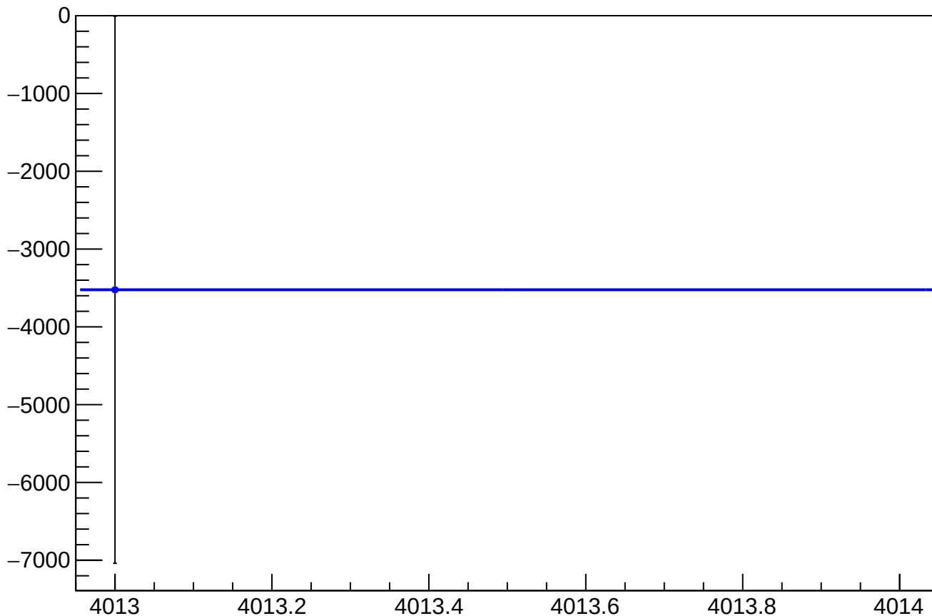
eigen_dit_asym_usl_atl1_avg_mean vs Slug
