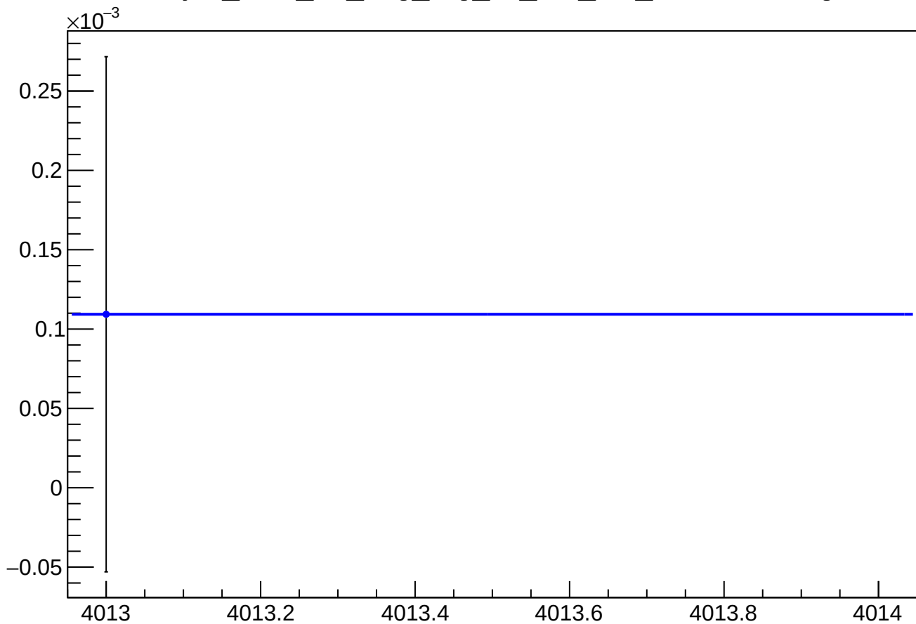
asym_sam_26_avg_reg_vs_cor_diff_mean vs Slug
