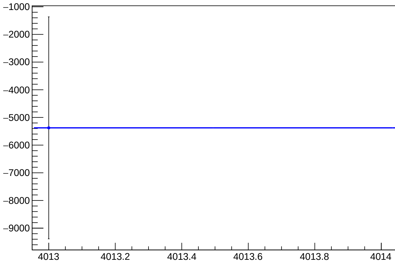
eigen_dit_asym_usl_atl2_avg_mean vs Slug
