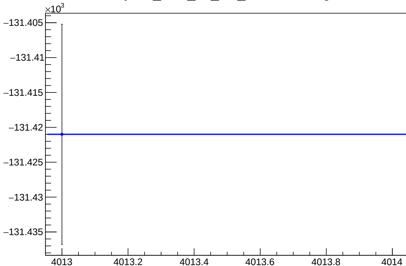
yield_bcm_an_diff_mean vs Slug
