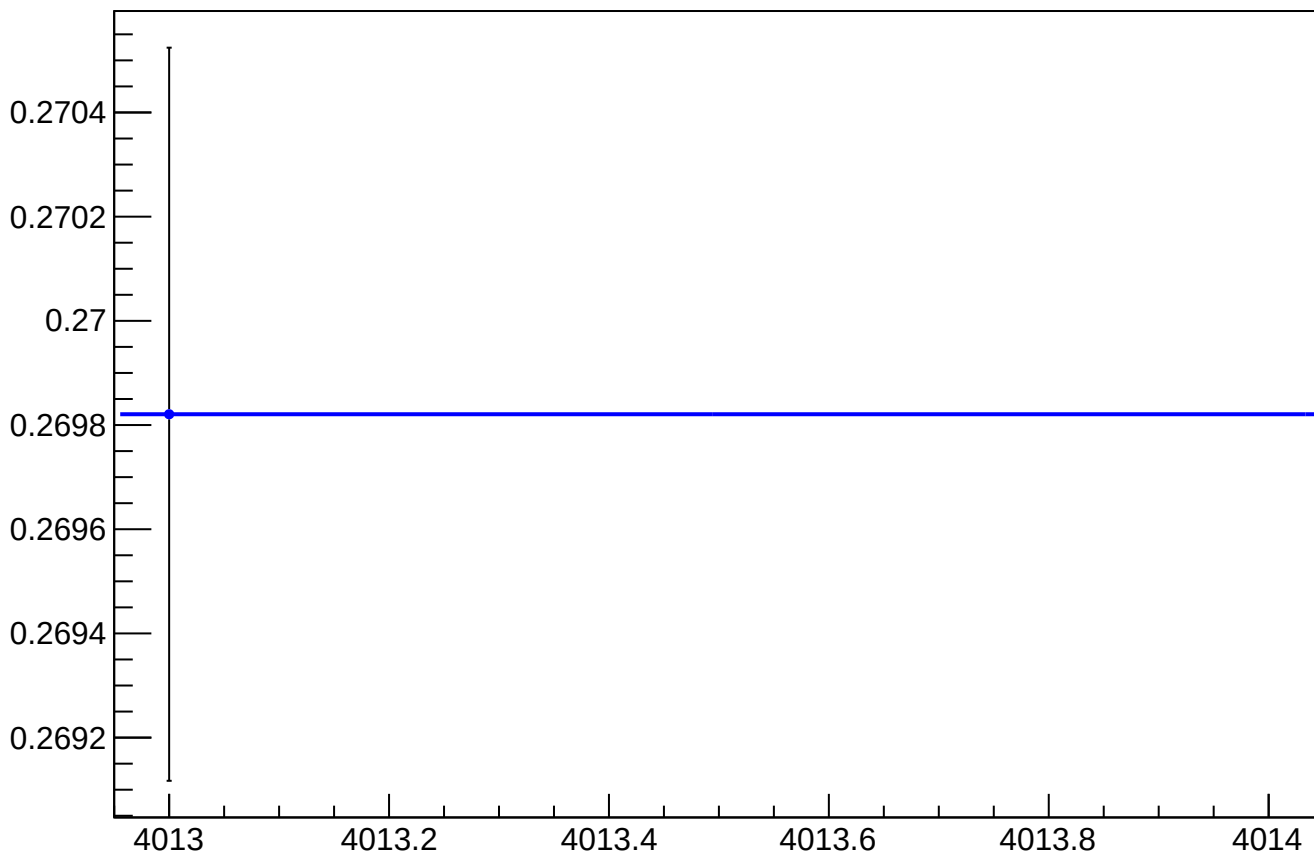
asym_us_avg_at1lr_avg_avg_reg_vs_cor_diff_rms vs Slug
