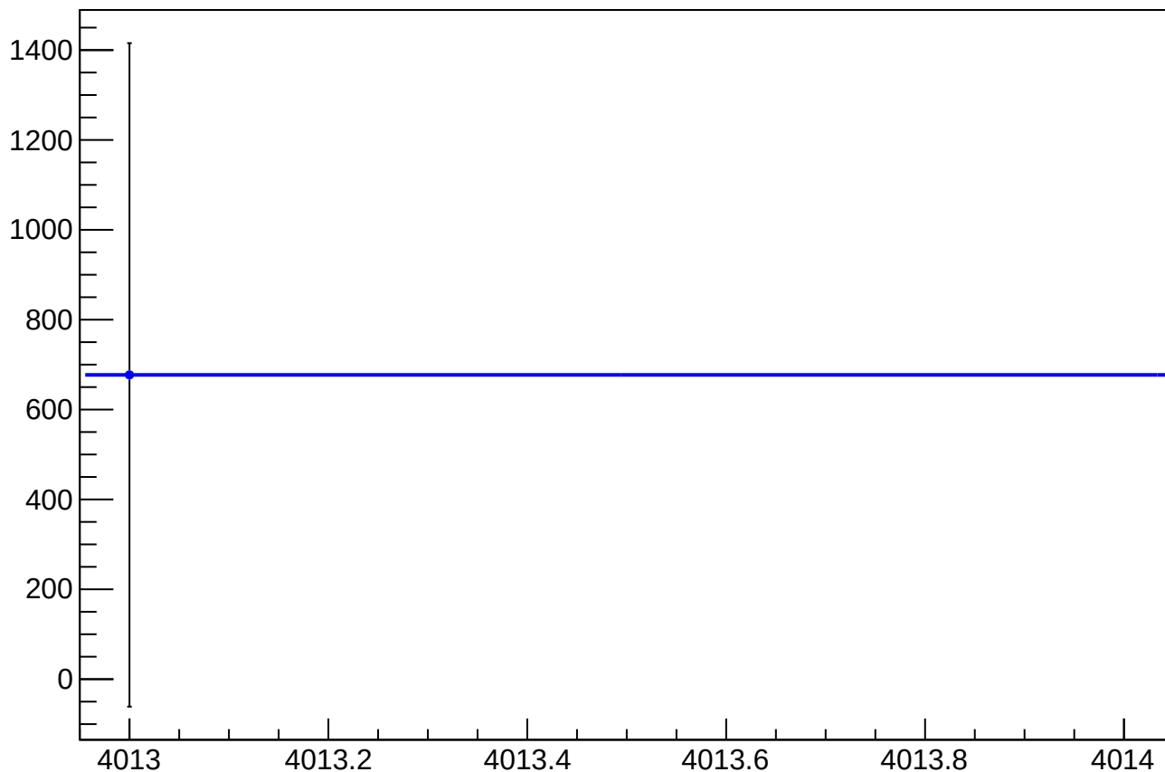
asym_sam_37_26_dd_cor_correction_mean vs Slug
