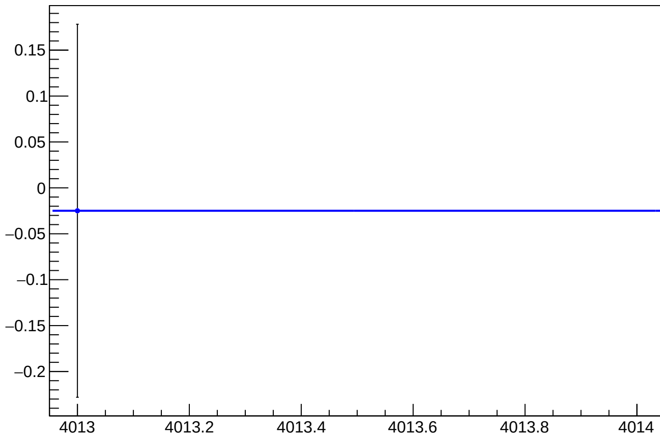
asym_sam_26_avg_eigen_dit_vs_eigen_cor_diff_mean vs Slug
