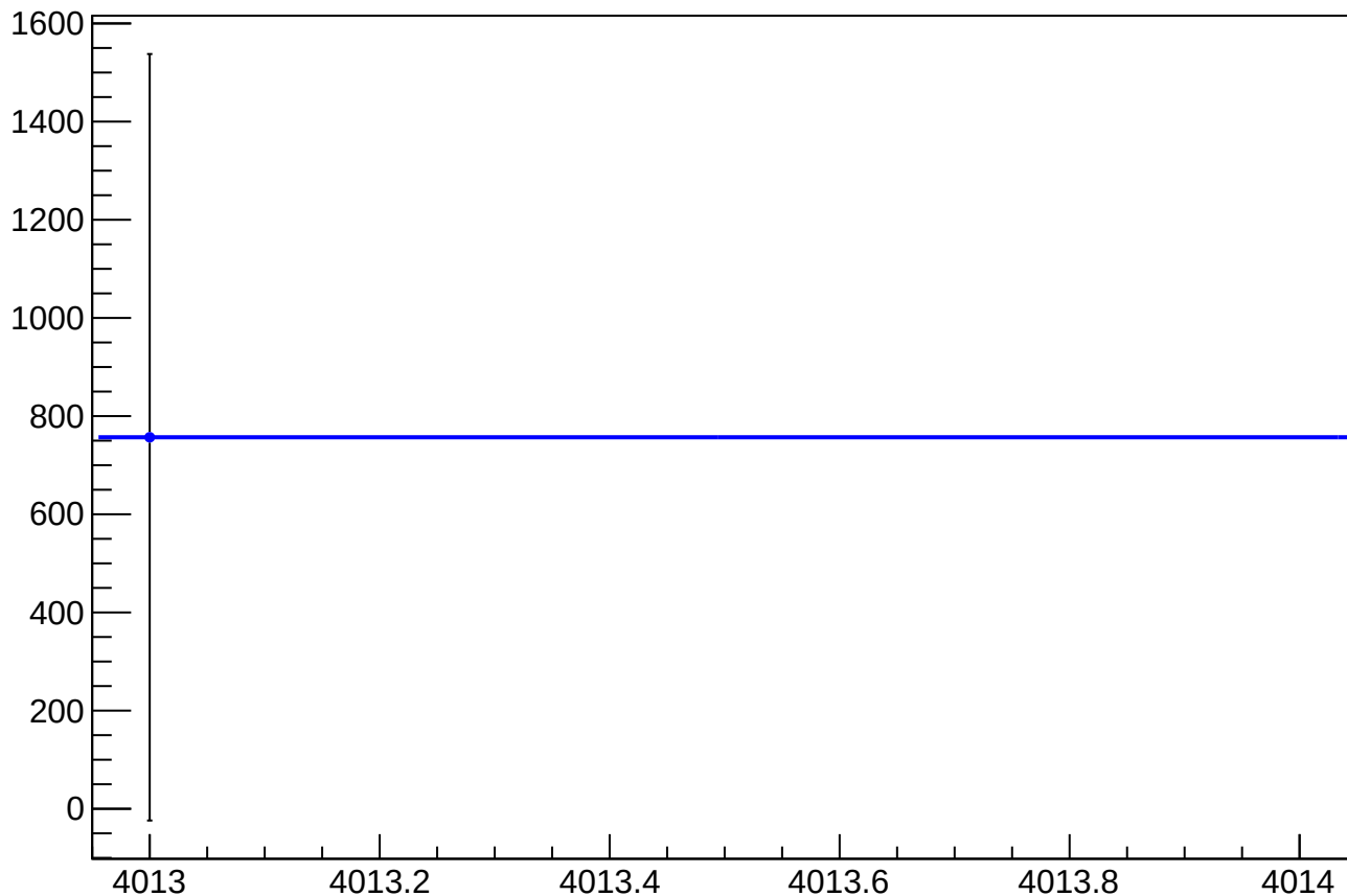
asym_sam_37_26_dd_eigen_dit_correction_mean vs Slug
