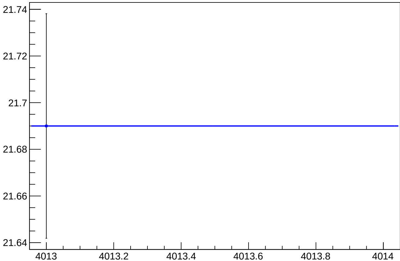
asym_sam_15_avg_eigen_dit_vs_cor_diff_rms vs Slug
