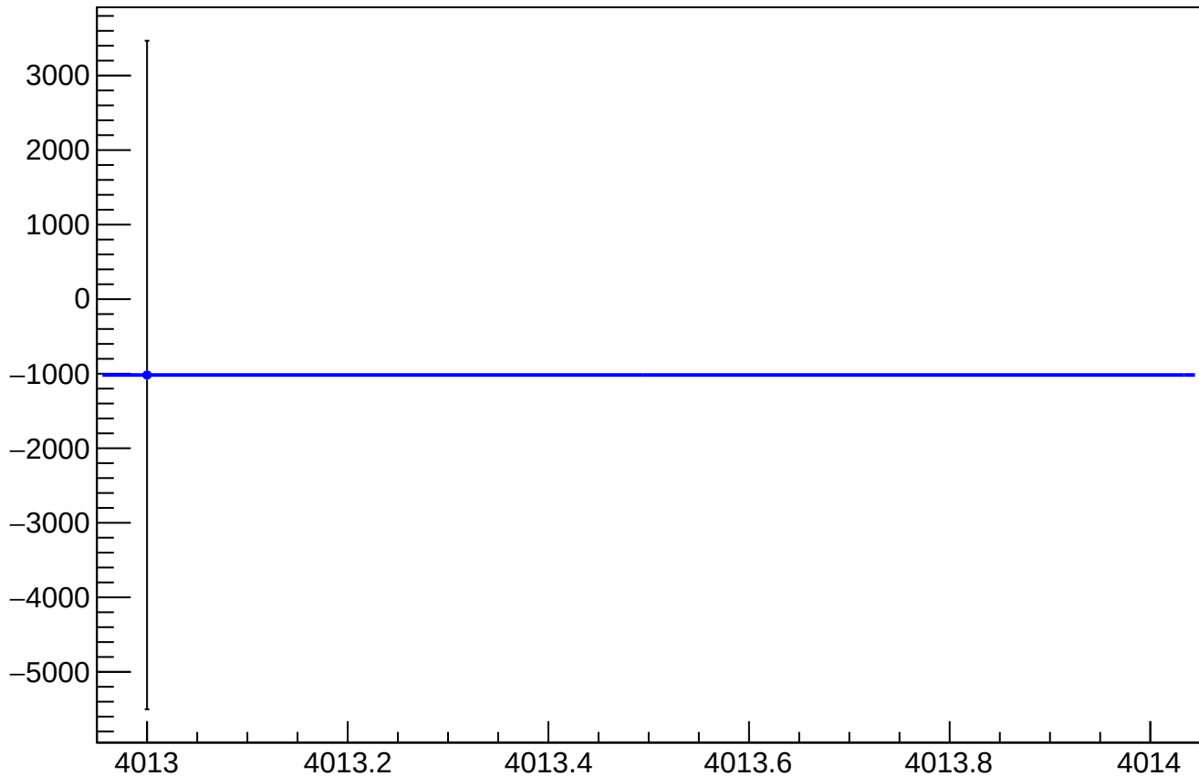
asym_us_dd_at2lr_dd_dd_mean vs Slug
