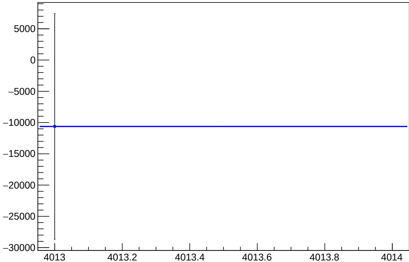
asym_atl_dd_reg_correction_mean vs Slug
