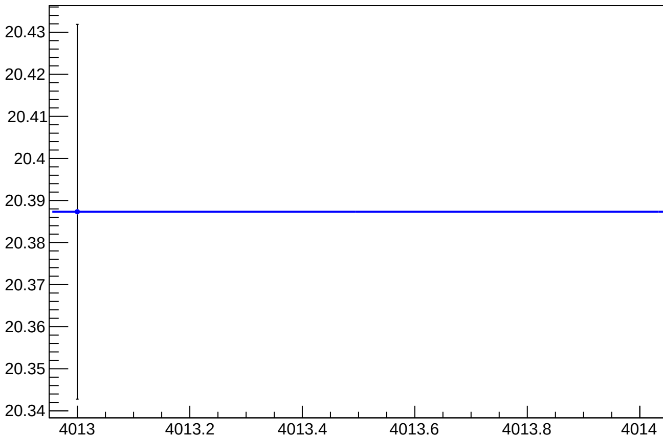
asym_sam_15_dd_eigen_dit_vs_eigen_cor_diff_rms vs Slug
