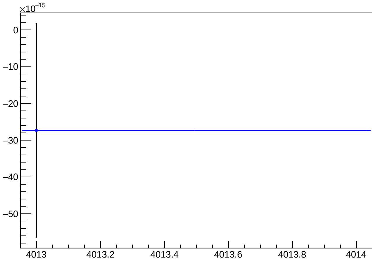
asym_us_dd_at2lr_dd_eigen_cor_vs_cor_diff_mean vs Slug
