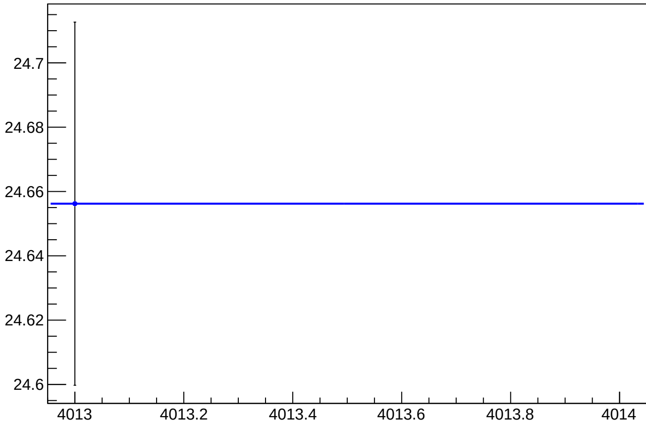
asym_sam_1357_avg_dit_vs_cor_diff_rms vs Slug
