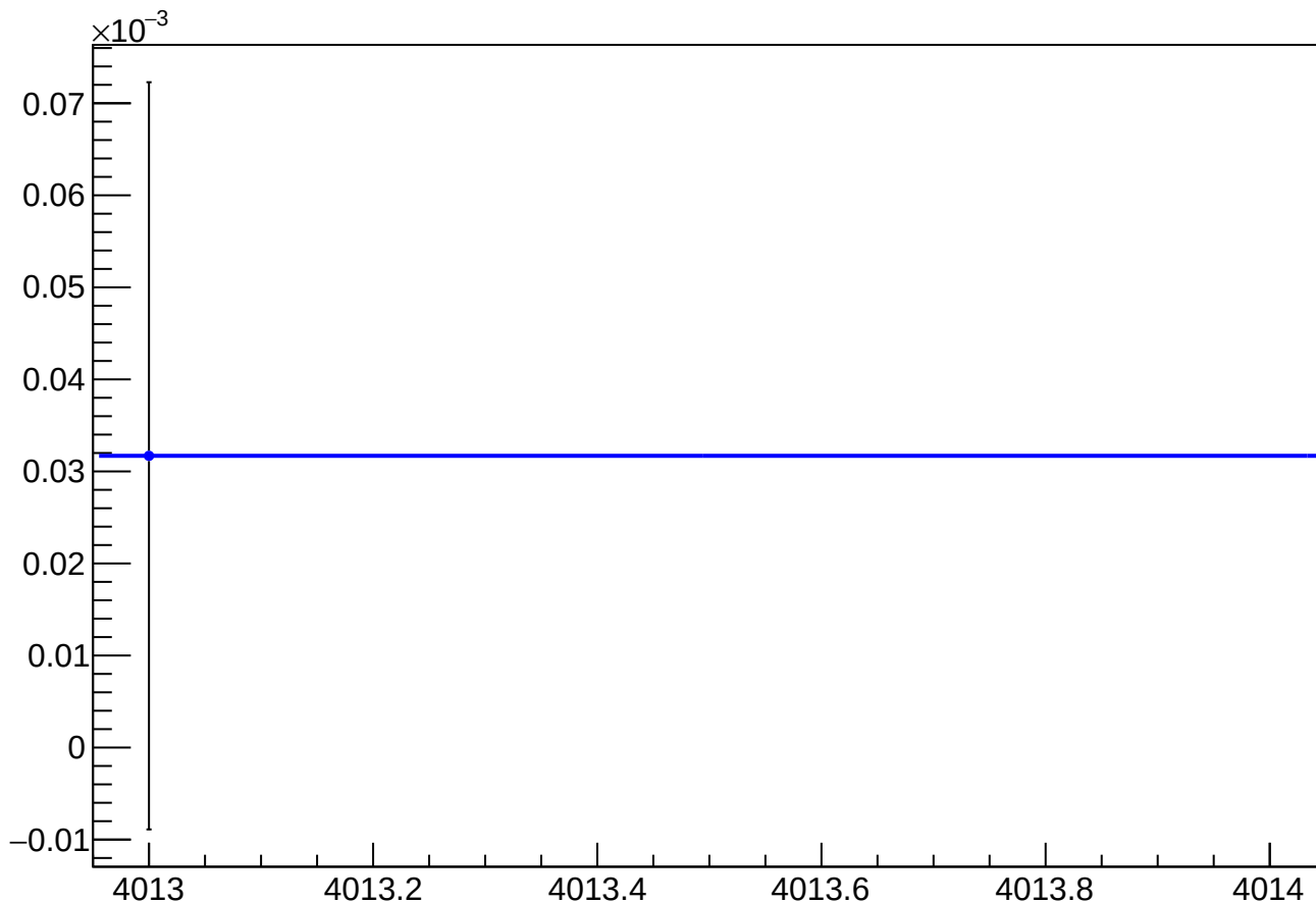
asym_atl_avg_atr_avg_avg_eigen_dit_vs_dit_diff_mean vs Slug
