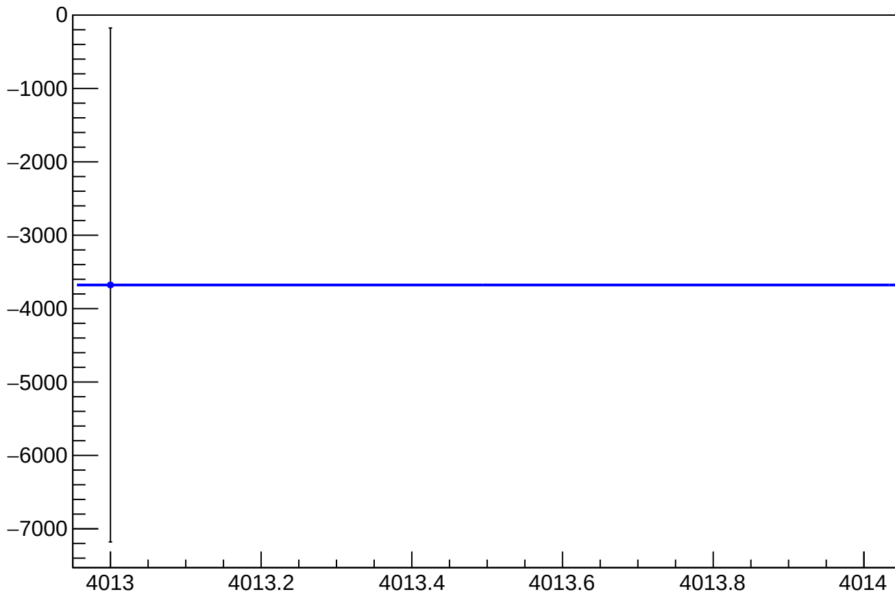
eigen_cor_asym_usl_atl1_avg_mean vs Slug
