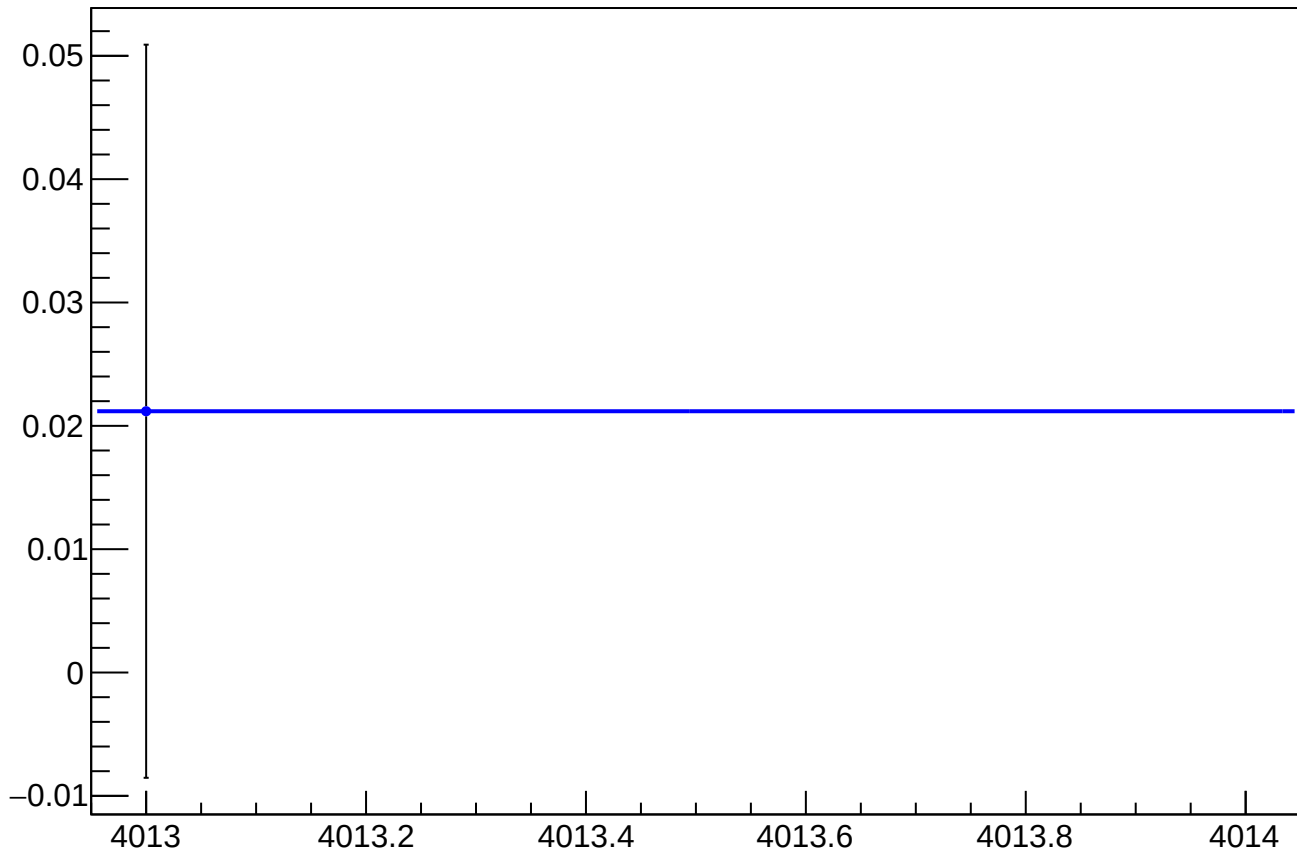
asym_sam1_dit_vs_cor_diff_mean vs Slug
