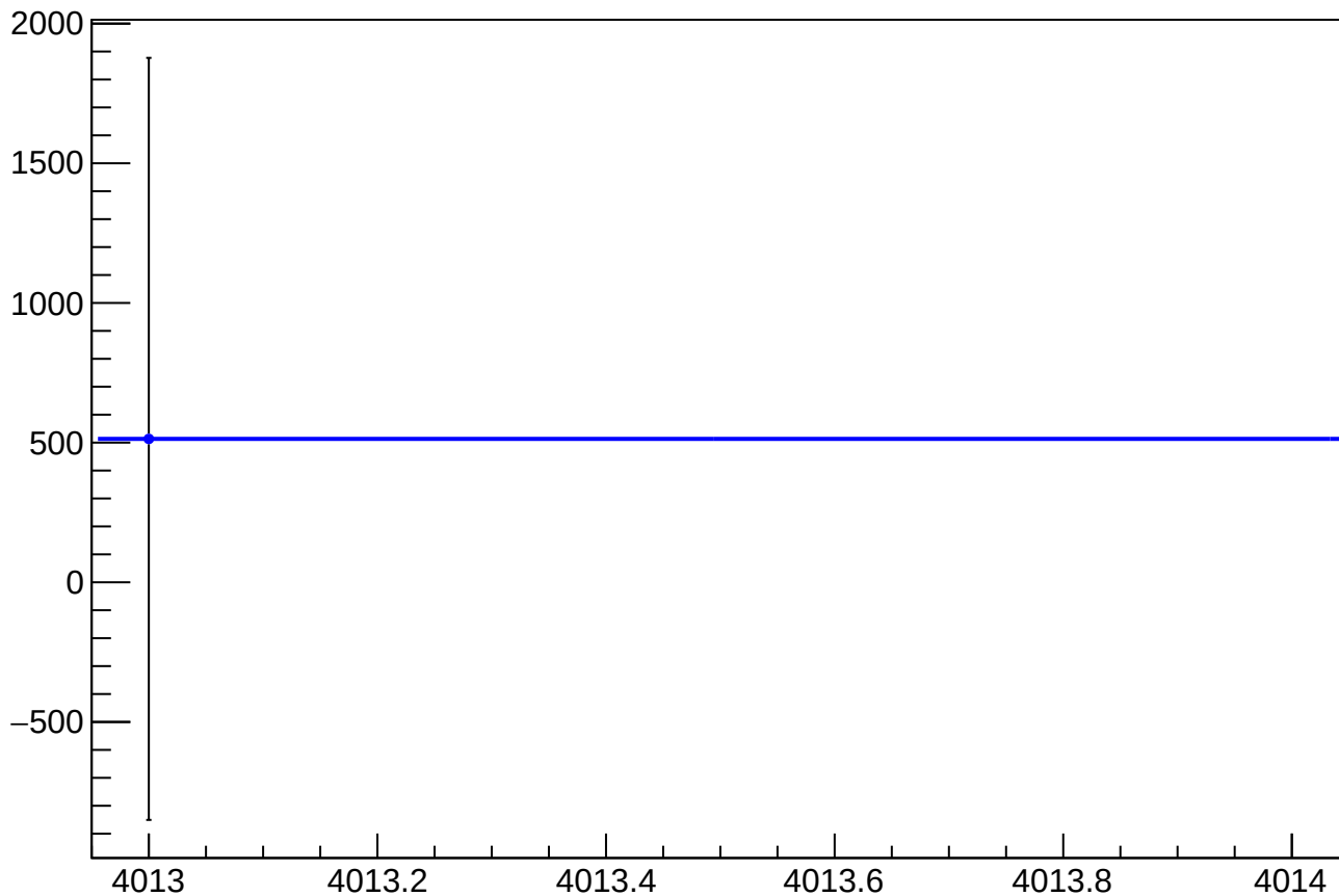
asym_us_dd_at1lr_dd_avg_eigen_dit_correction_mean vs Slug
