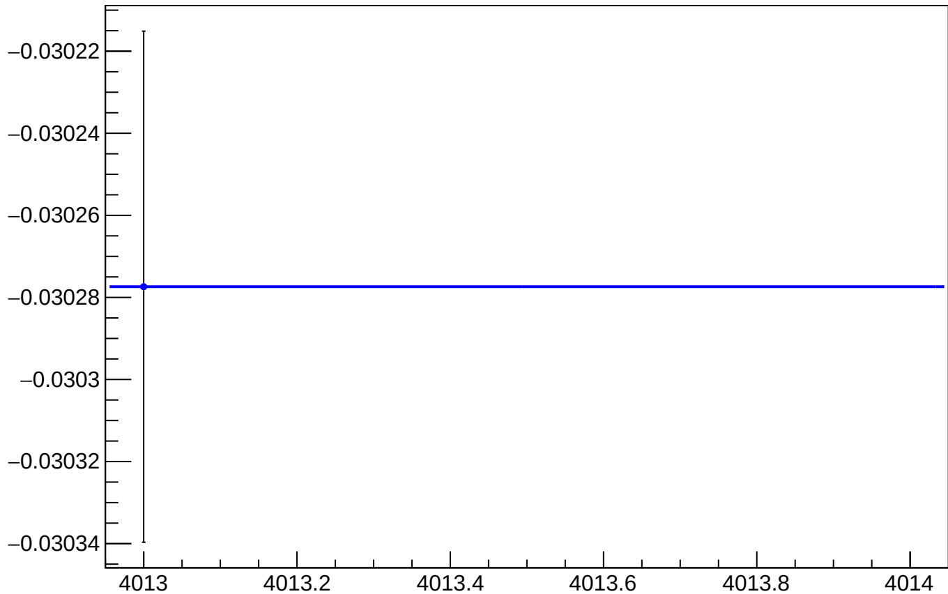
yield_bpm4ecX_mean vs Slug
