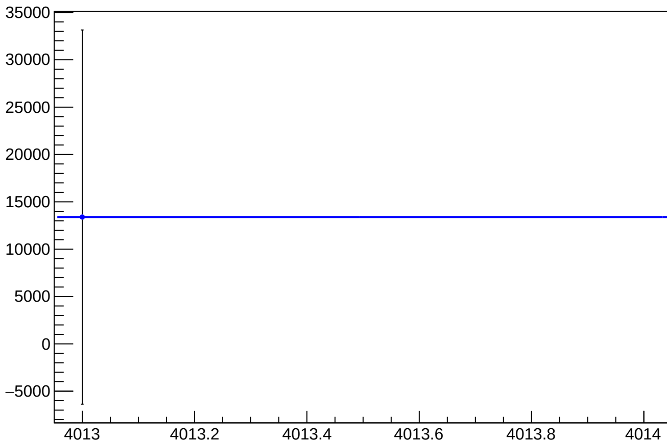
asym_atl_avg_atr_avg_avg_reg_correction_mean vs Slug
