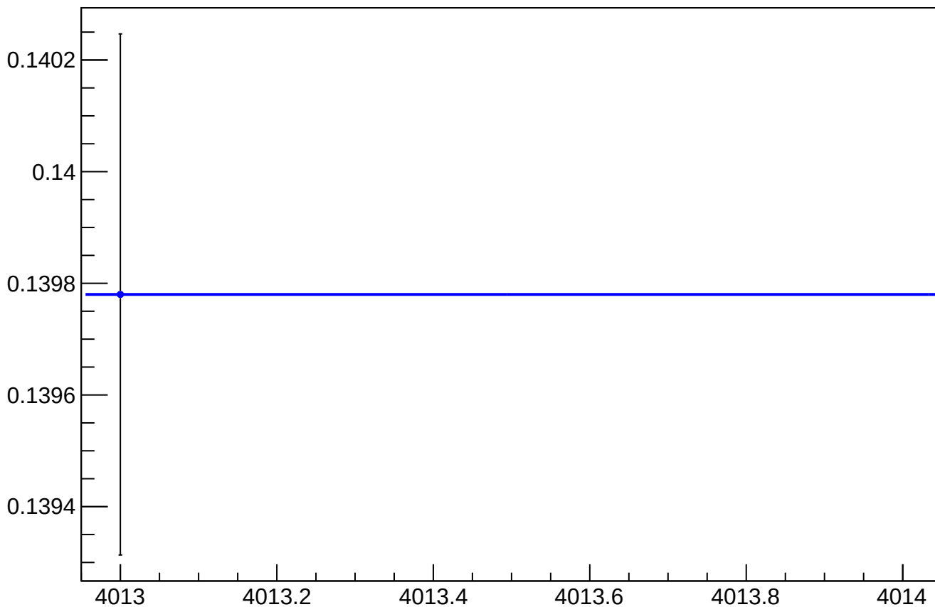
asym_us_dd_at1lr_dd_avg_reg_vs_cor_diff_rms vs Slug
