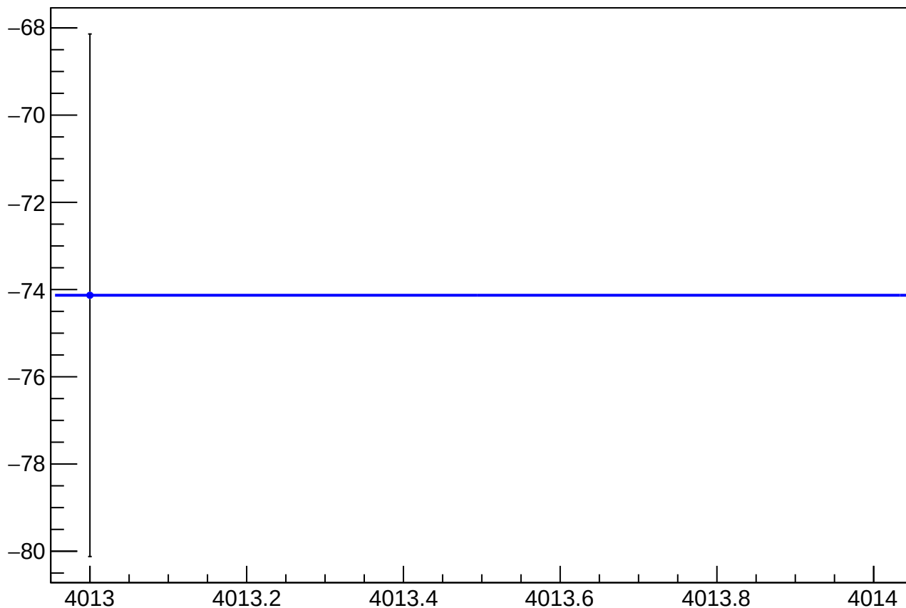
reg_asym_us_dd_at2lr_dd_avg_diff_bpm4eX_slope vs Slug
