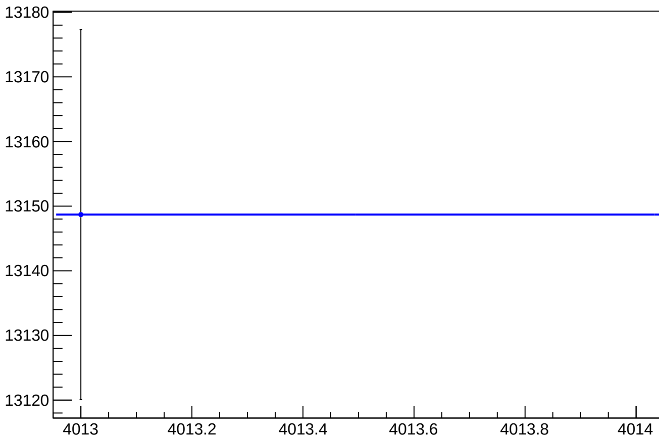
asym_us_avg_at2lr_avg_avg_reg_correction_rms vs Slug
