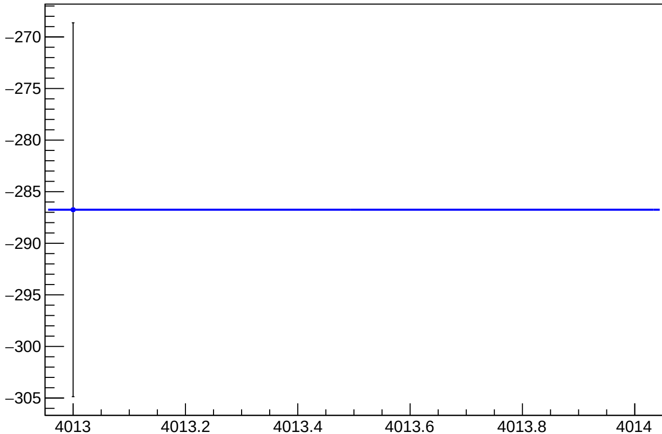
reg_asym_usr_atr2_avg_diff_bpm1X_slope vs Slug
