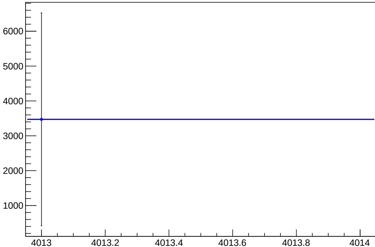
asym_sam6_eigen_dit_correction_mean vs Slug
