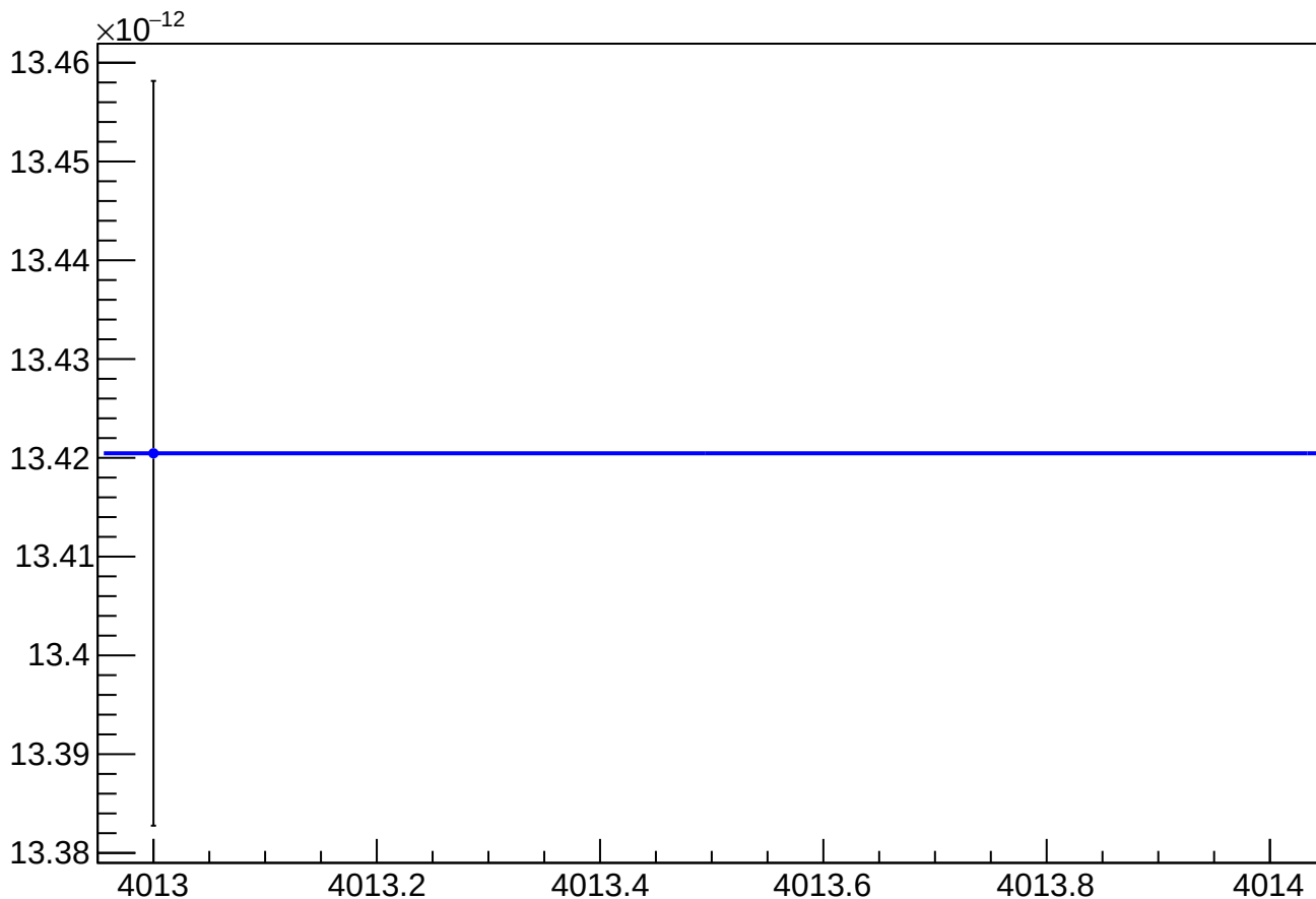
asym_sam_1548_avg_eigen_cor_vs_cor_diff_rms vs Slug
