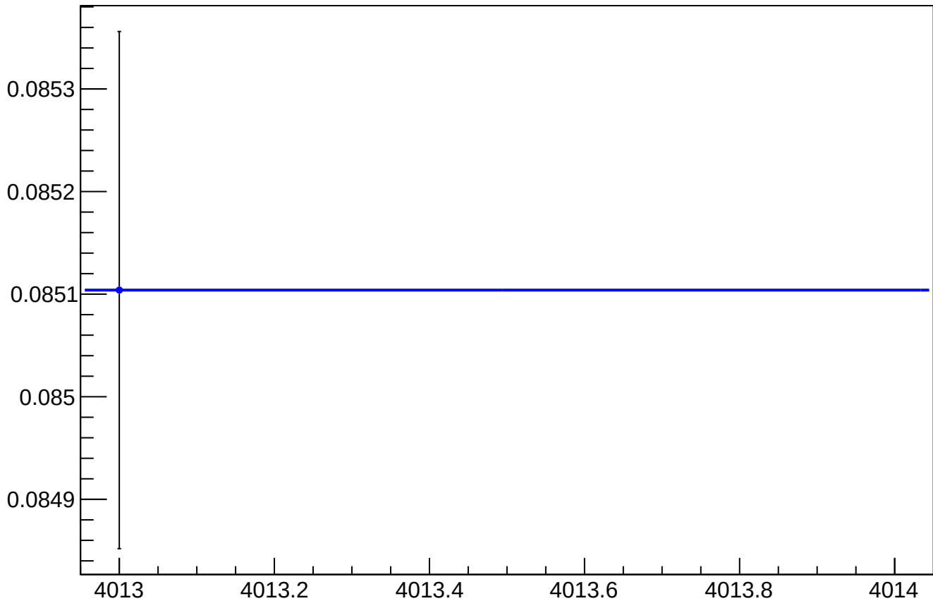
asym_atl_dd_atr_dd_avg_reg_vs_cor_diff_rms vs Slug
