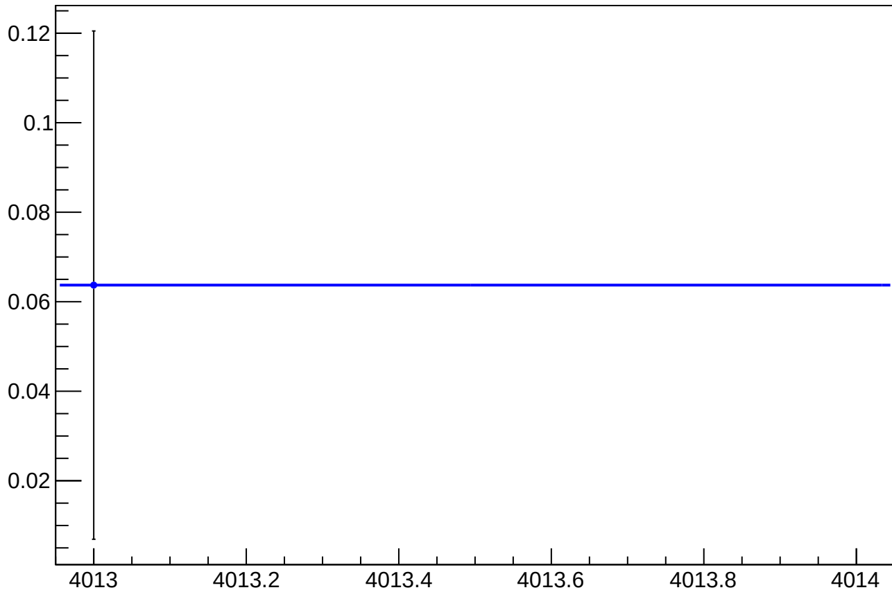
asym_us_dd_dit_vs_eigen_cor_diff_mean vs Slug
