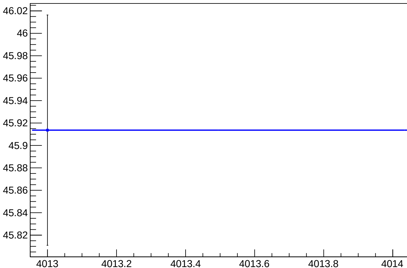
asym_sam_37_avg_eigen_dit_vs_eigen_cor_diff_rms vs Slug
