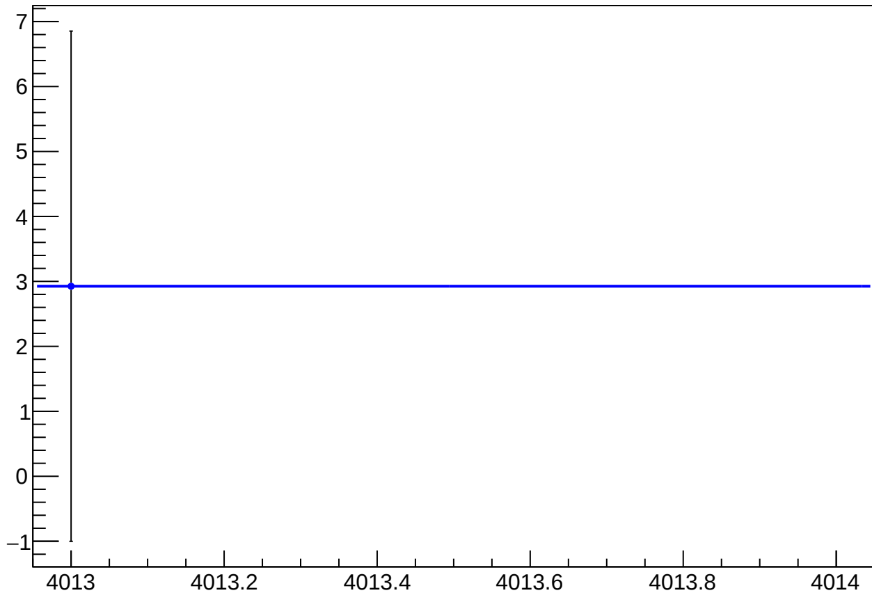
reg_asym_us_dd_atlr_dd_avg_diff_bpm1X_slope vs Slug
