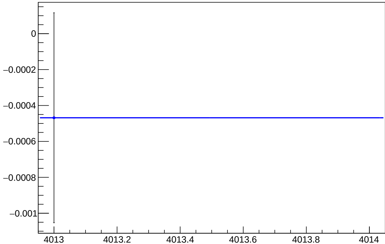
asym_usr_atr1_dd_reg_vs_cor_diff_mean vs Slug
