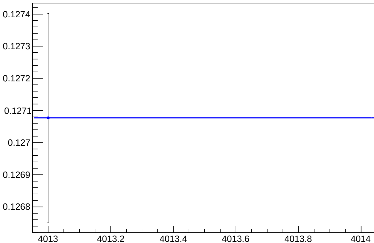
asym_at1_dd_at2_dd_avg_reg_vs_cor_diff_rms vs Slug
