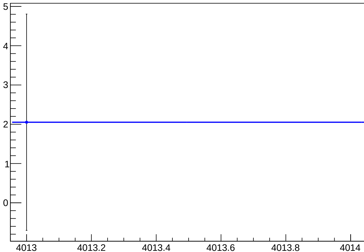
diff_bpm1i02X_mean vs Slug
