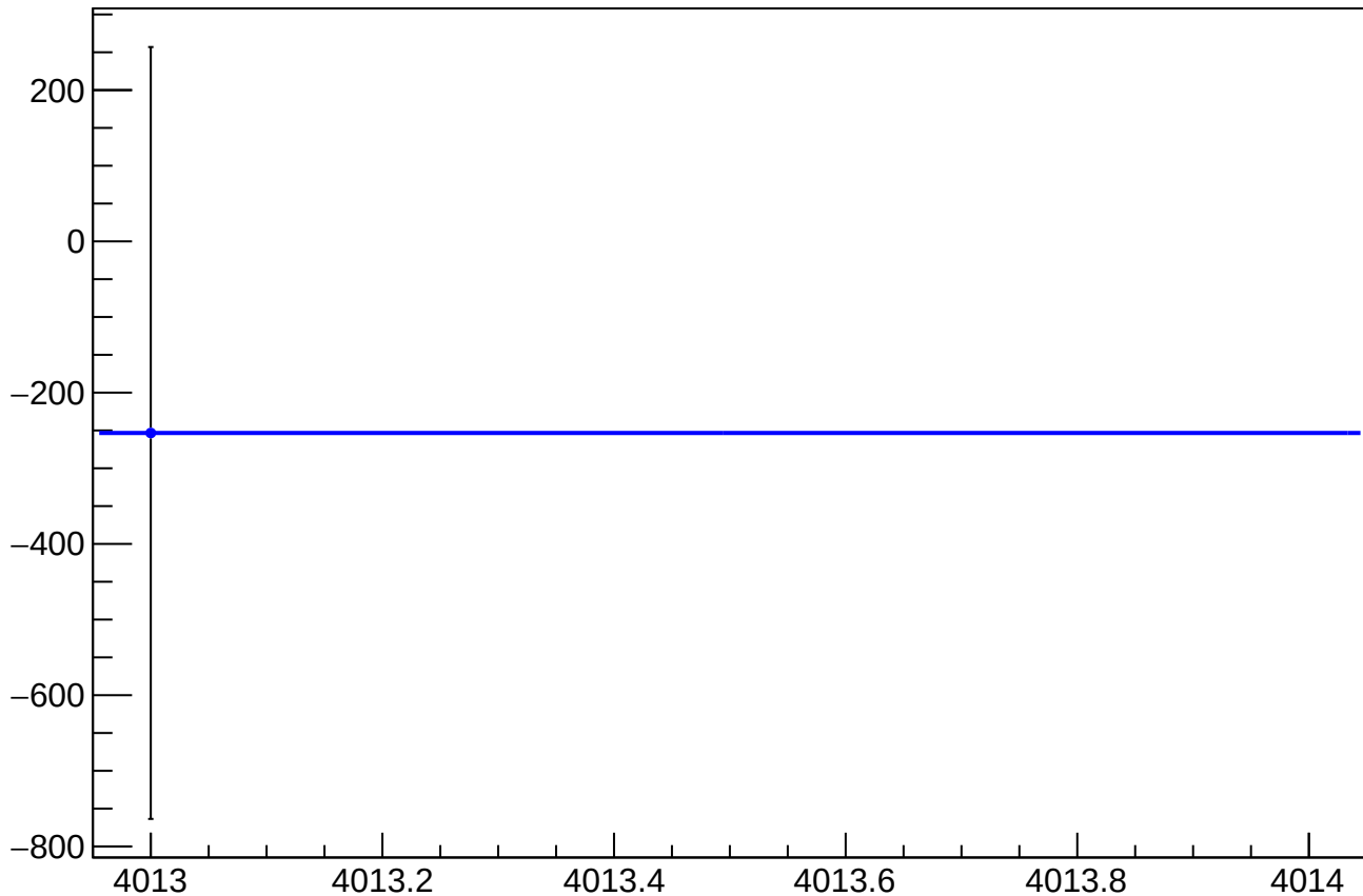
asym_bcm_cav4cQ_dg_ds_avg_mean vs Slug
