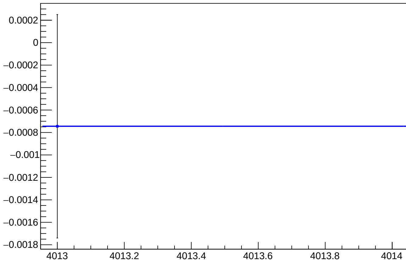
asym_us_avg_at1lr_avg_avg_reg_vs_cor_diff_mean vs Slug
