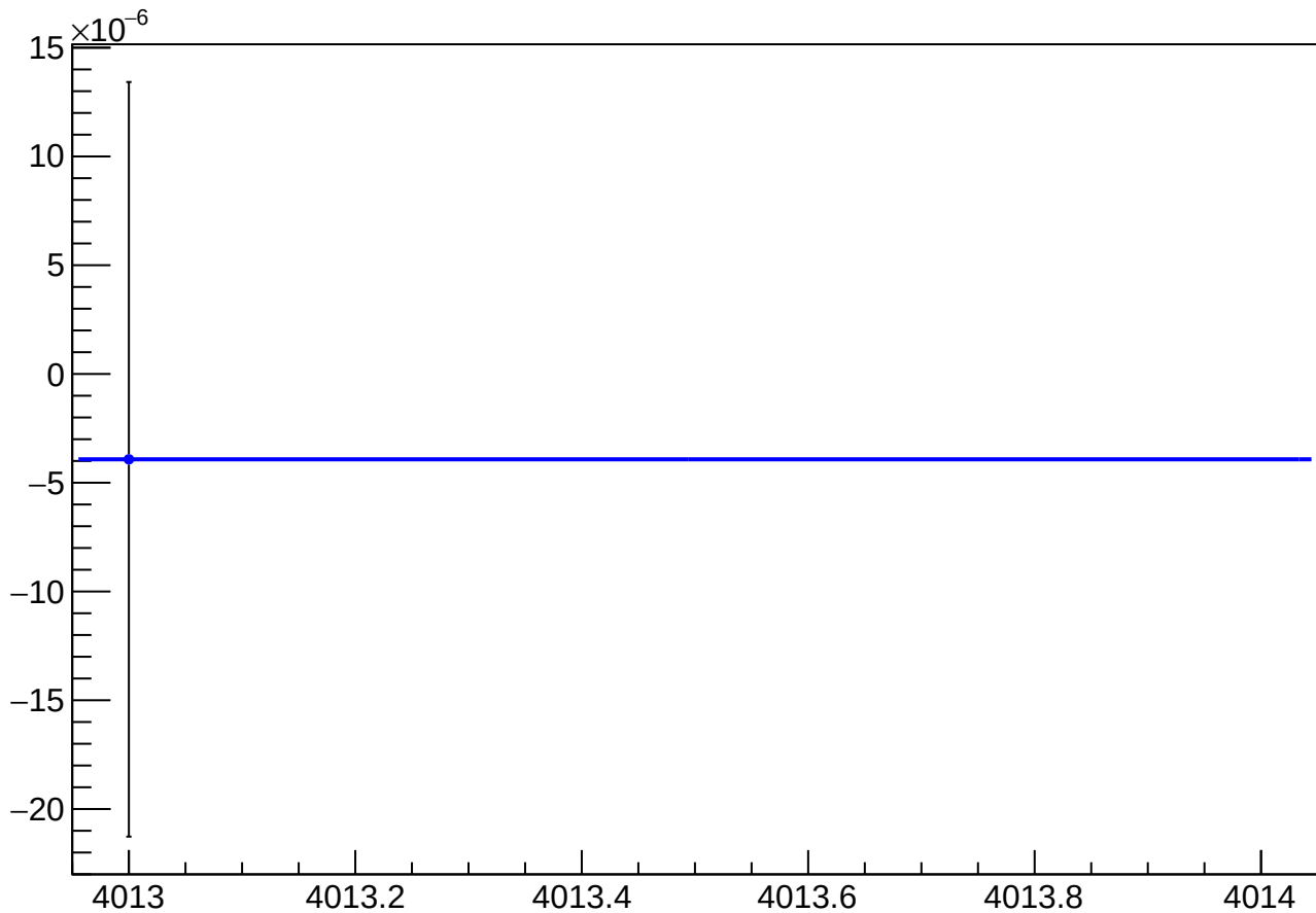
asym_sam_26_dd_eigen_dit_vs_dit_diff_mean vs Slug
