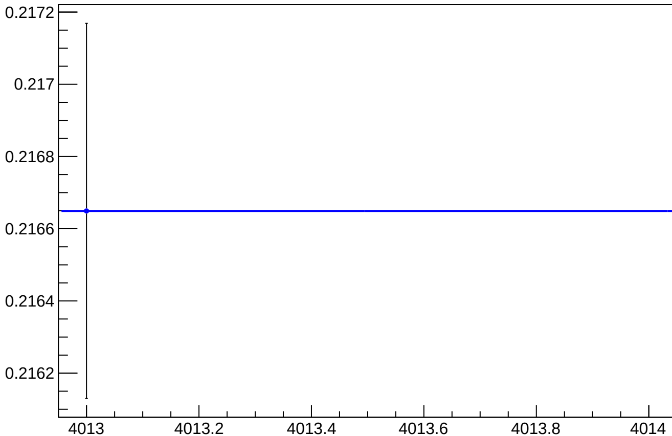
asym_us_avg_atlr_avg_dd_reg_vs_cor_diff_rms vs Slug
