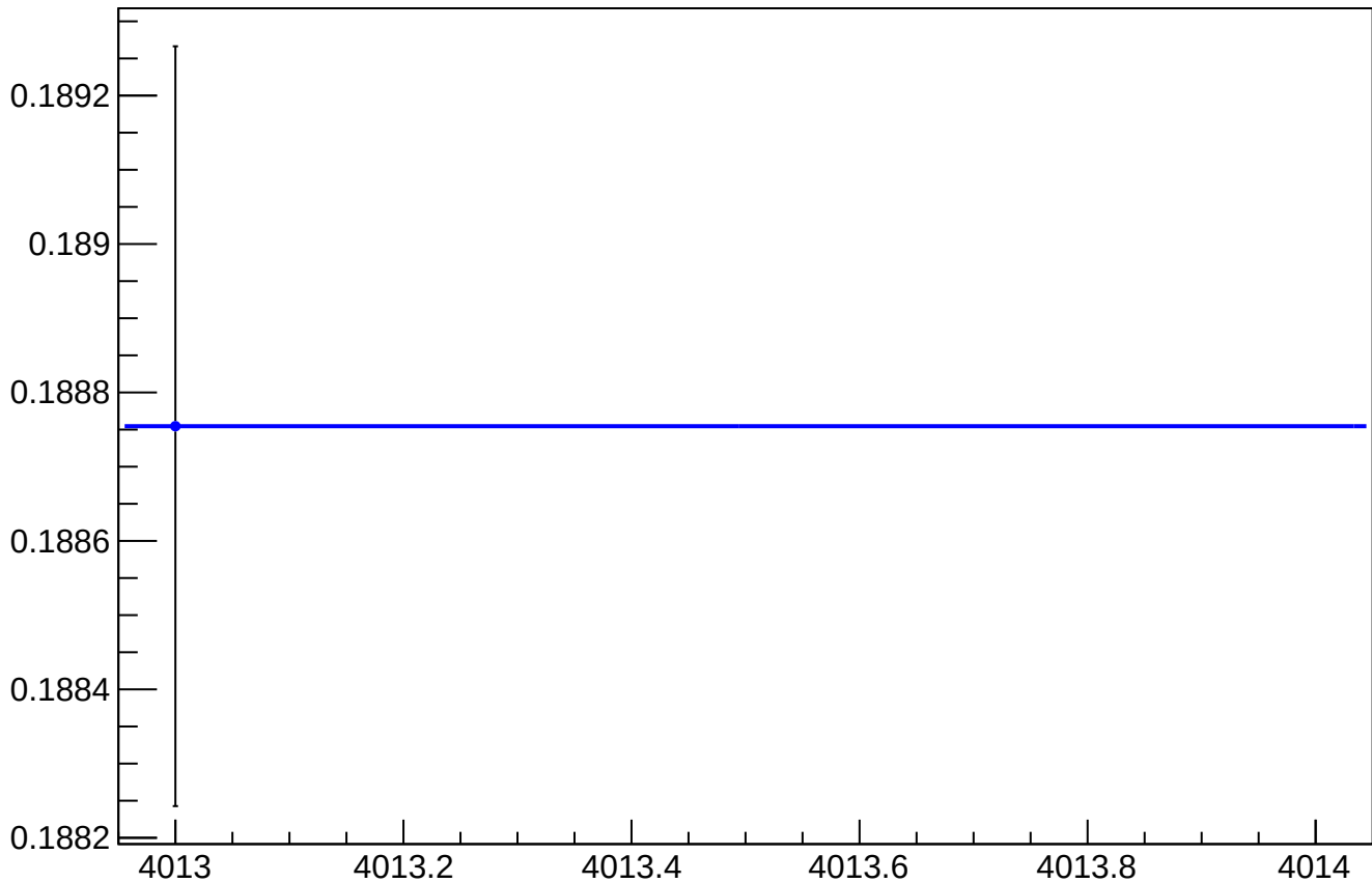
asym_atl_avg_atr_avg_dd_reg_vs_cor_diff_rms vs Slug
