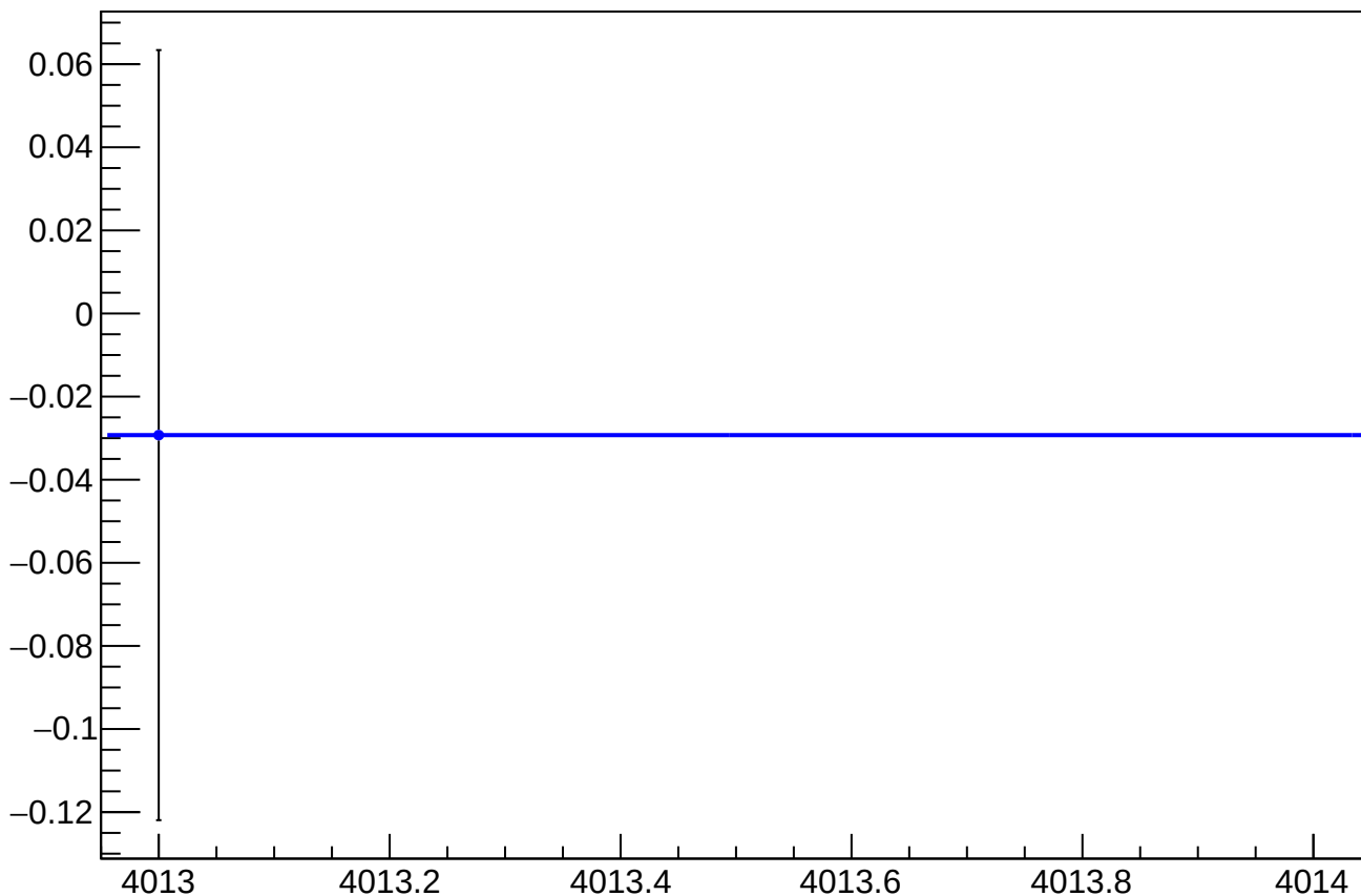
asym_us_dd_at2lr_dd_dd_dit_vs_cor_diff_mean vs Slug
