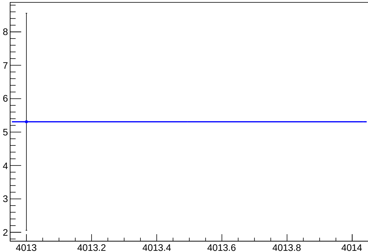
reg_asym_usl_atl1_avg_diff_bpm4eY_slope vs Slug
