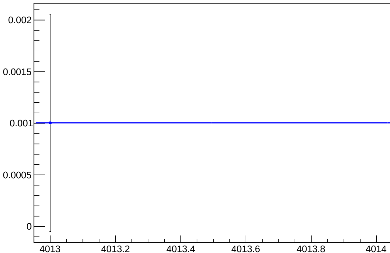
asym_us_avg_at2lr_avg_dd_reg_vs_cor_diff_mean vs Slug
