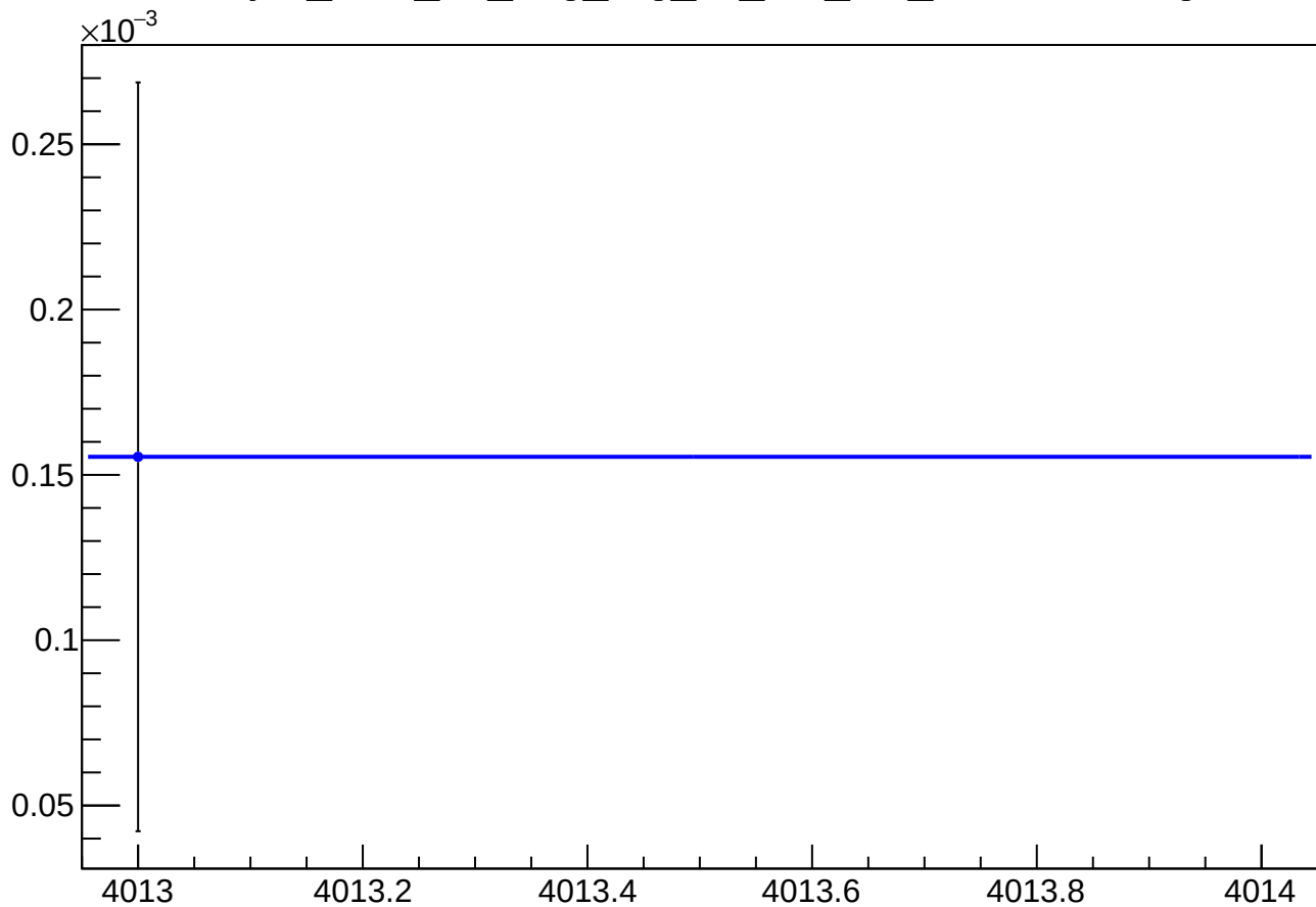
asym_sam_37_avg_reg_vs_cor_diff_mean vs Slug
