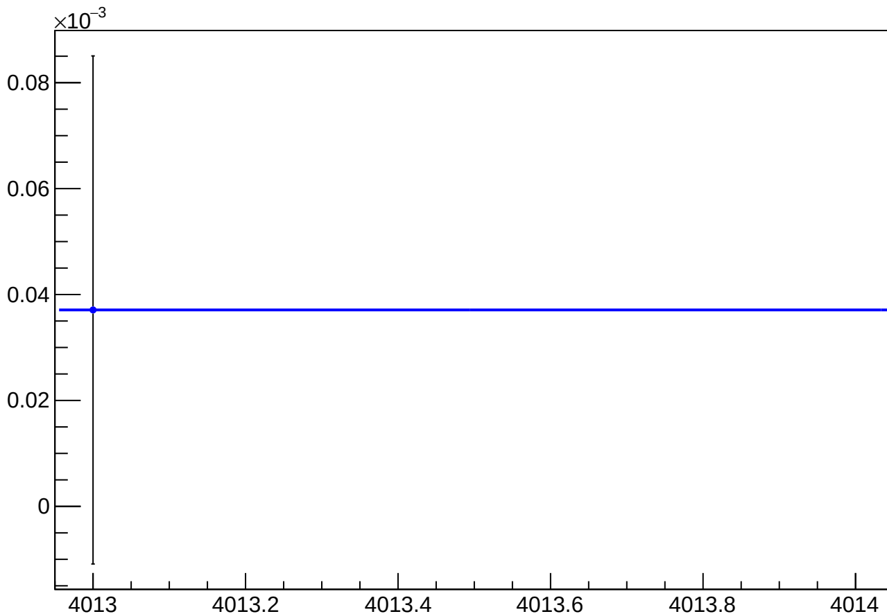
asym_atl1r2_avg_eigen_dit_vs_dit_diff_mean vs Slug
