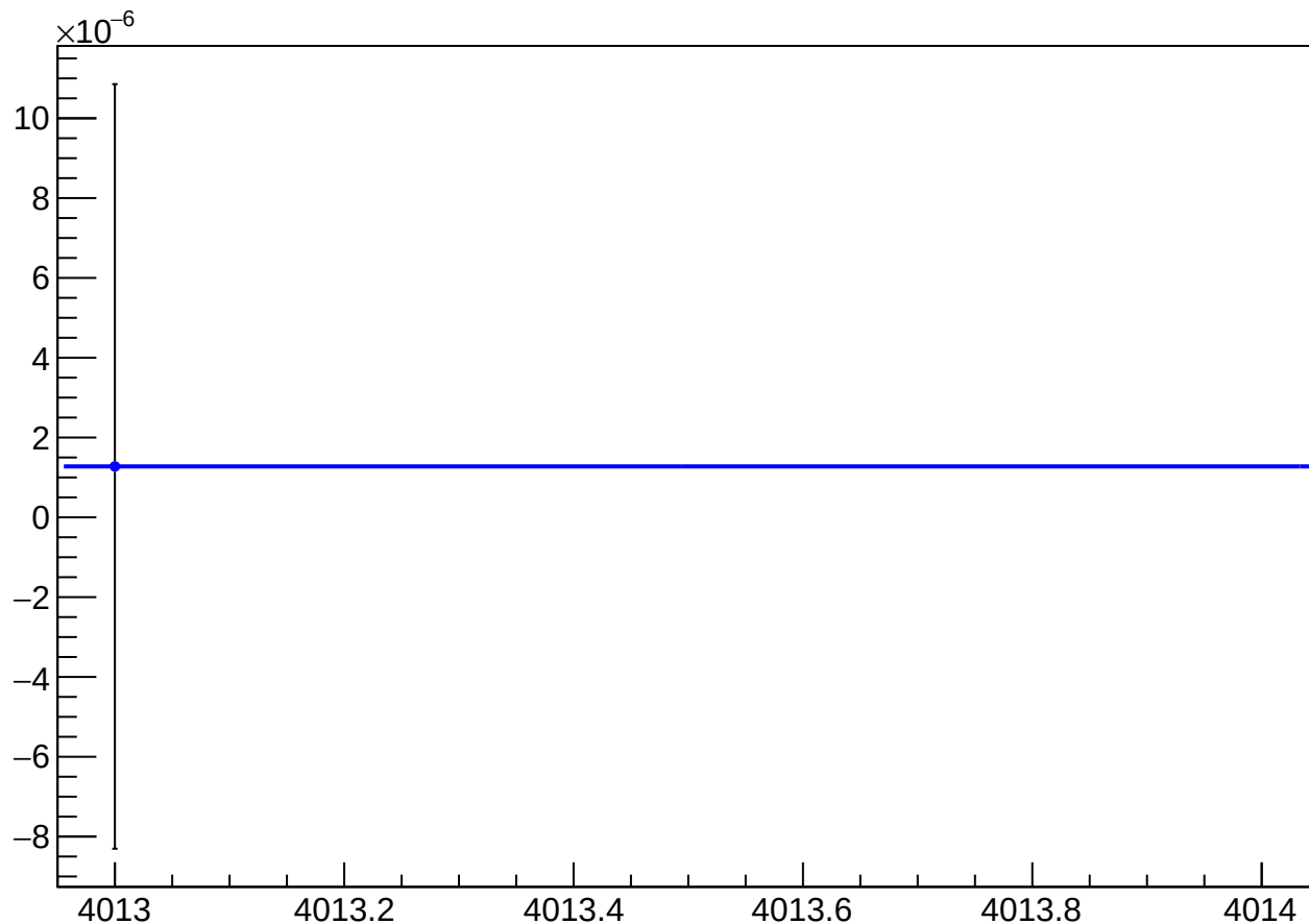
asym_sam_3726_avg_eigen_dit_vs_dit_diff_mean vs Slug
