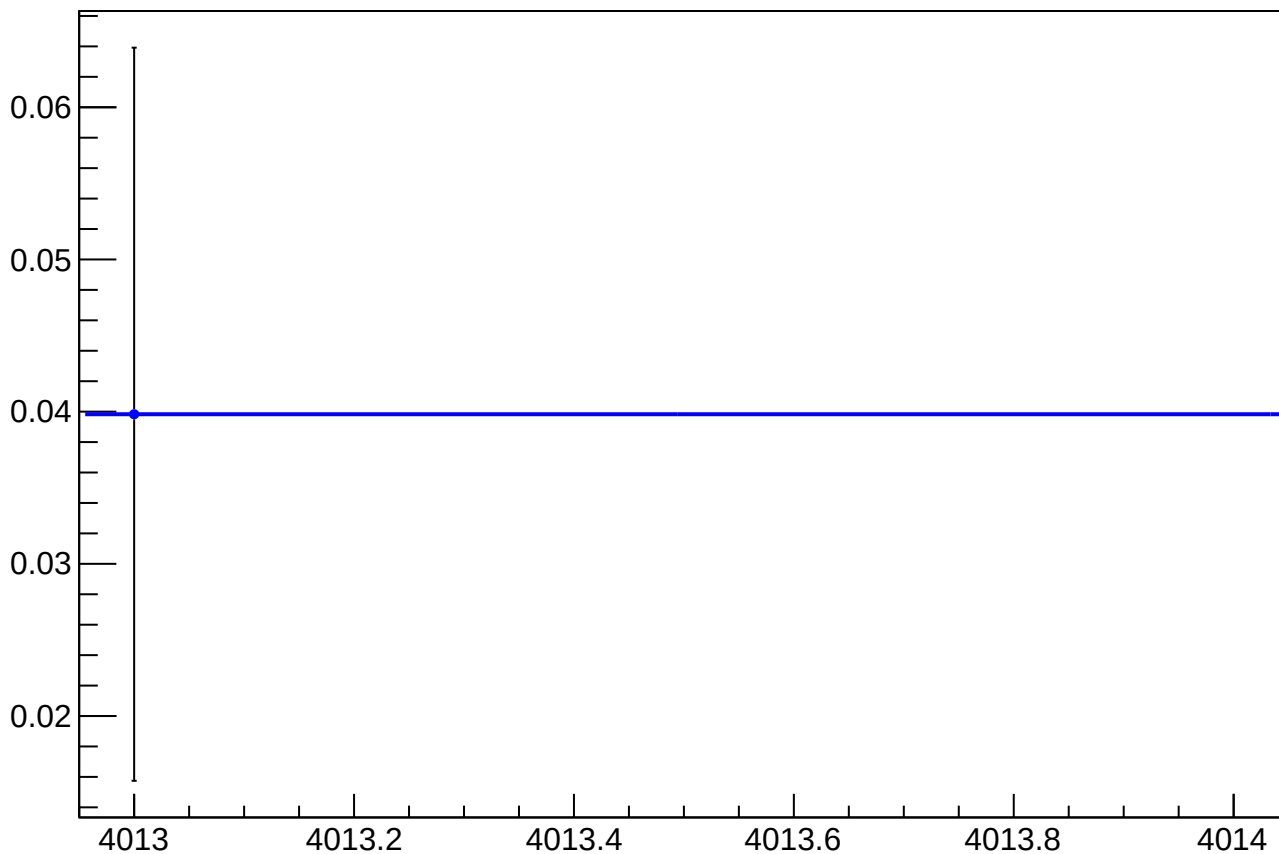
reg_asym_bcm_an_us_an_ds_dd_diff_bpm4eY_slope vs Slug
