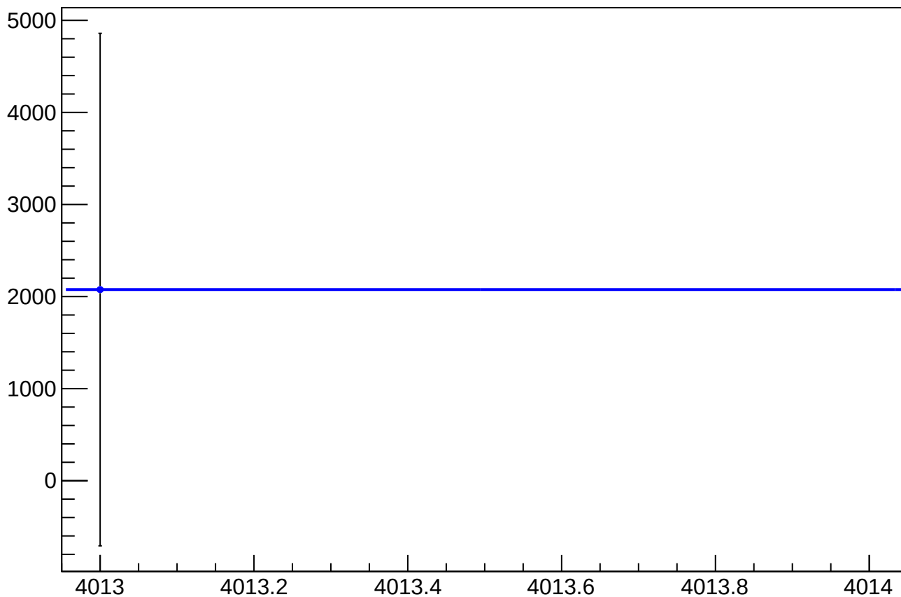
asym_usl_atl1_avg_eigen_cor_correction_mean vs Slug
