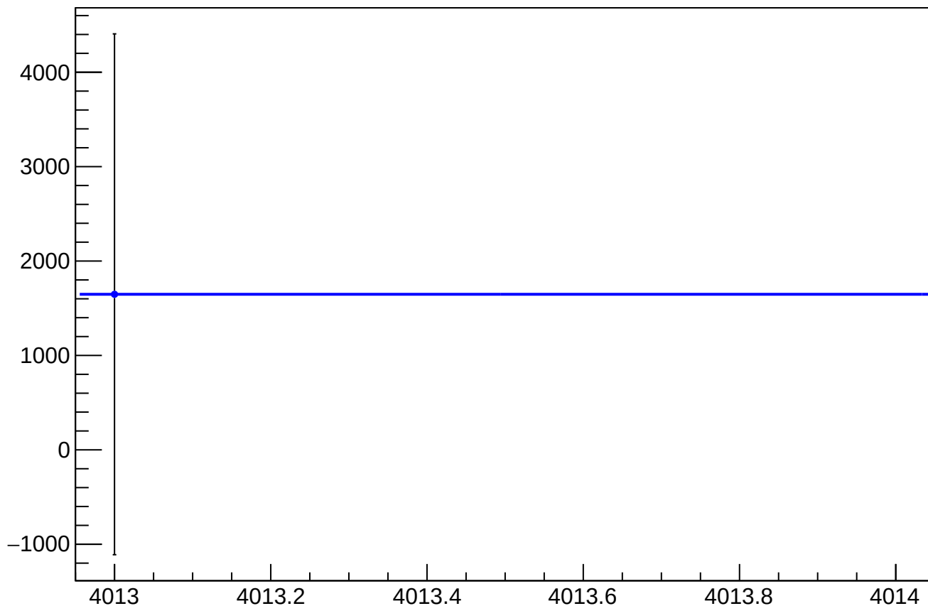
reg_asym_us_dd_atlr_dd_dd_mean vs Slug
