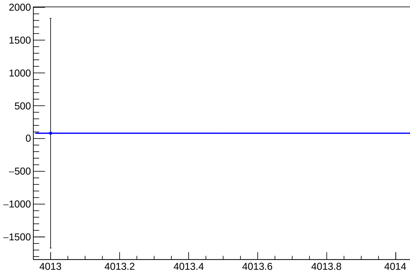
dit_asym_us_avg_mean vs Slug
