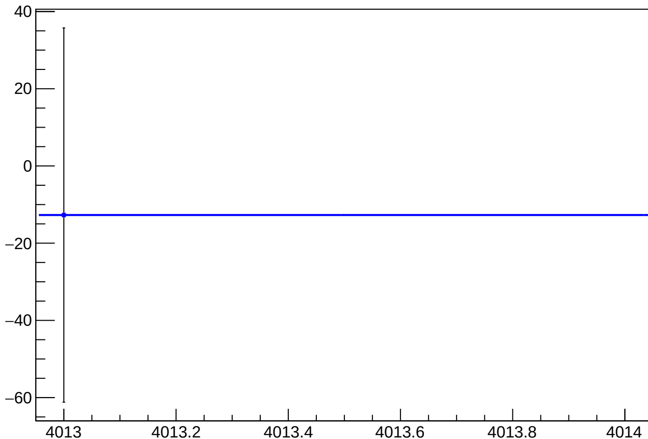
asym_bcm_an_avg_bcm_dg_ds_agg_dd_mean vs Slug
