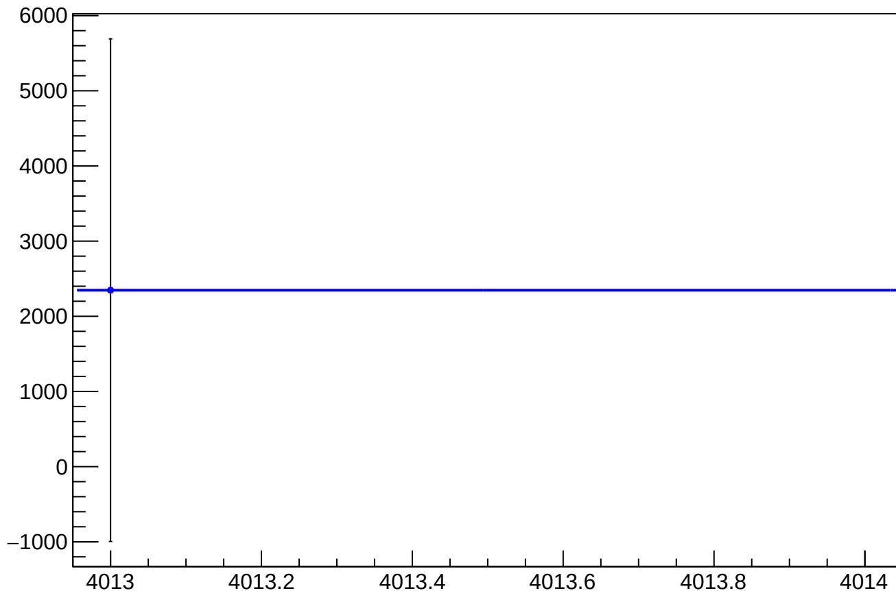
asym_sam5_eigen_cor_correction_mean vs Slug
