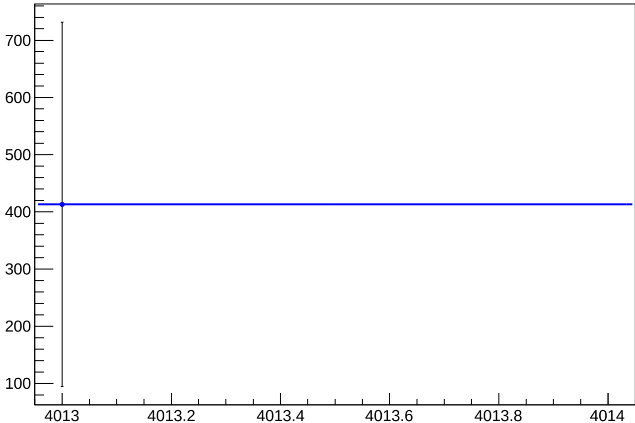
eigen_dit_asym_sam_37_48_dd_mean vs Slug
