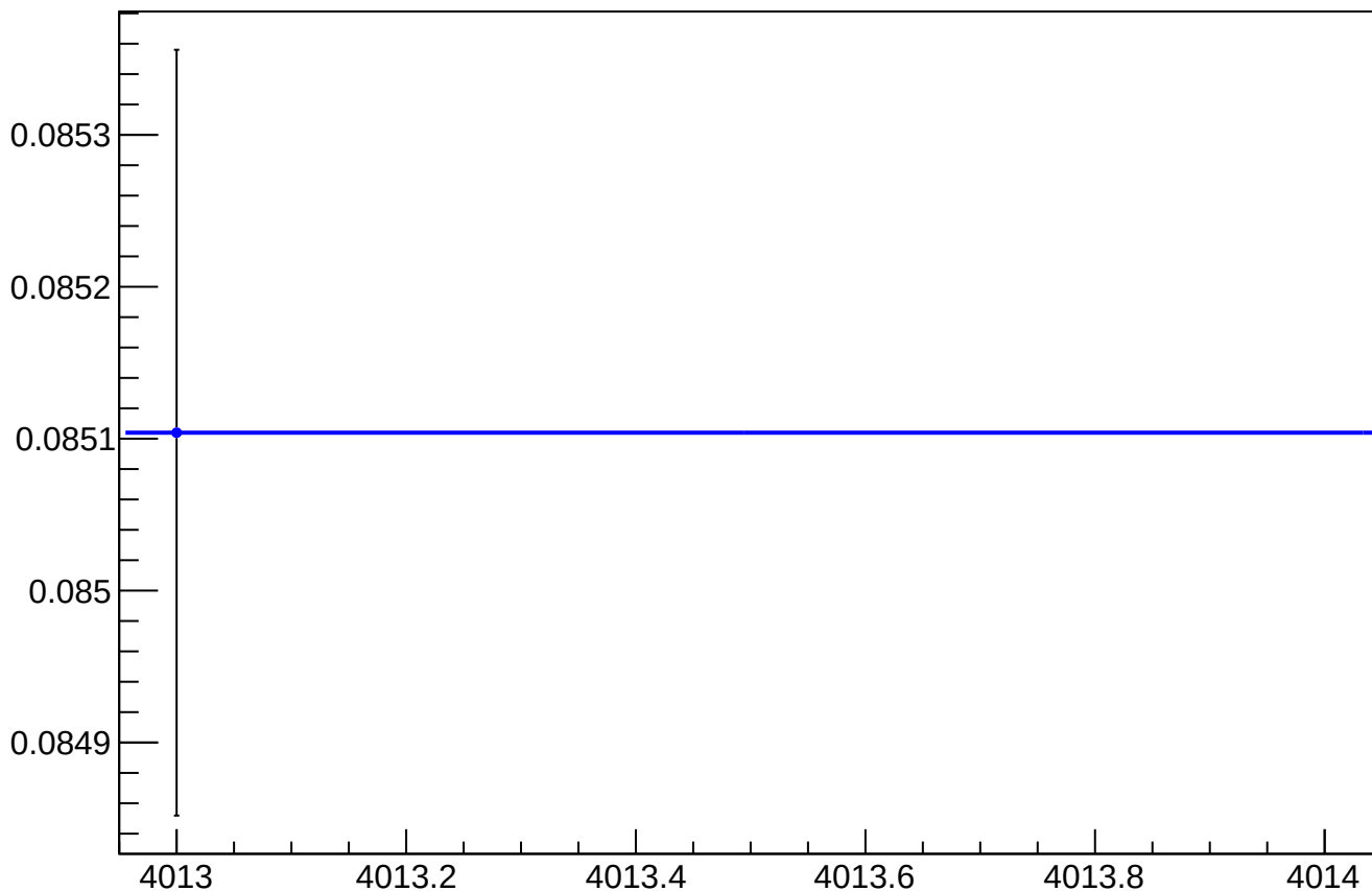
asym_atl1r2_dd_atl2r1_dd_dd_reg_vs_cor_diff_rms vs Slug
