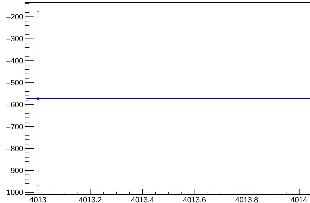
cor_asym_sam_1548_avg_mean vs Slug
