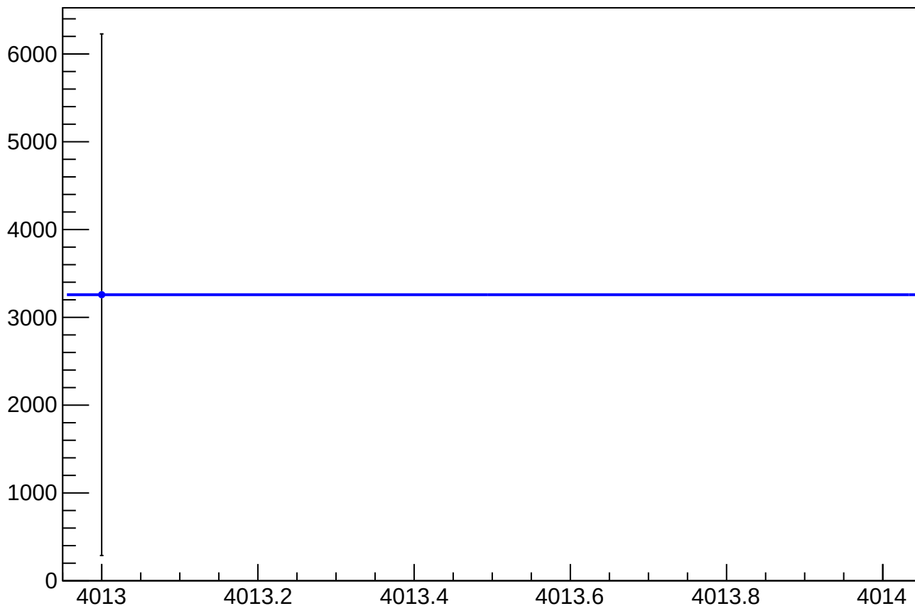
asym_sam6_eigen_cor_correction_mean vs Slug
