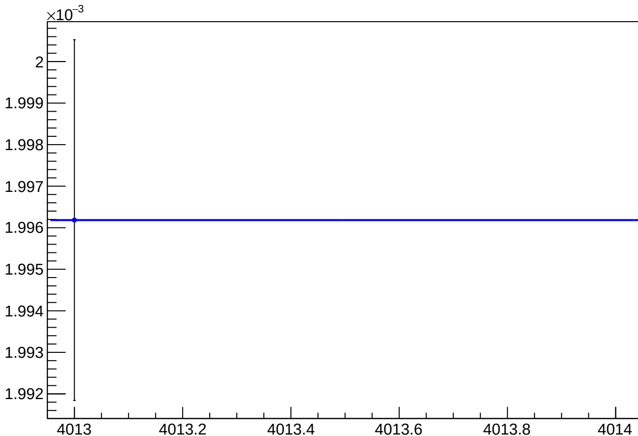
asym_sam_1357_2468_dd_eigen_dit_vs_dit_diff_rms vs Slug
