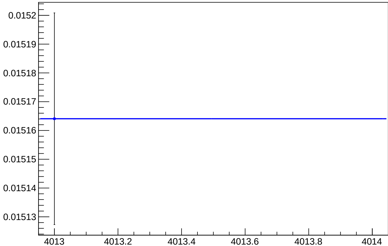
asym_sam_1357_avg_reg_vs_cor_diff_rms vs Slug
