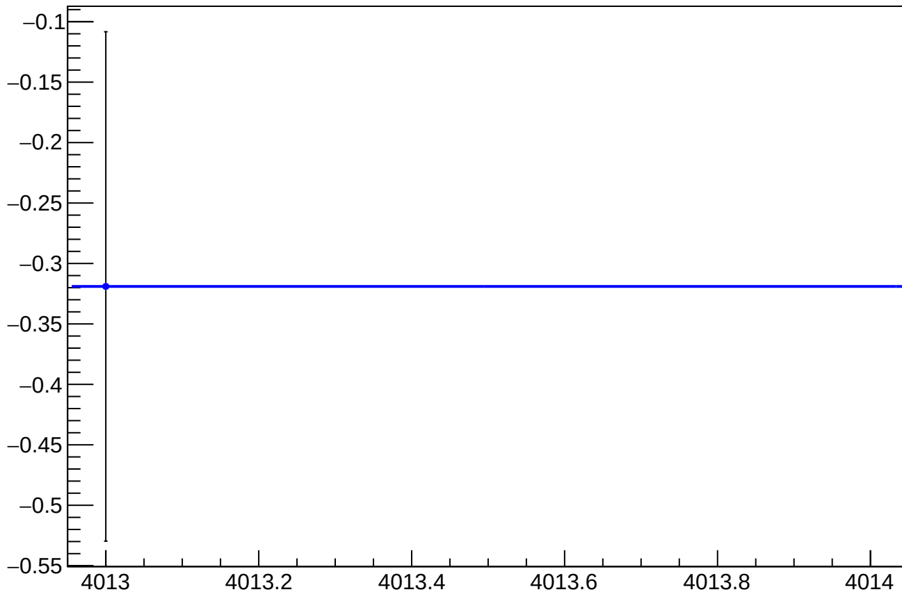
asym_us_avg_at1lr_avg_dd_eigen_dit_vs_cor_diff_mean vs Slug
