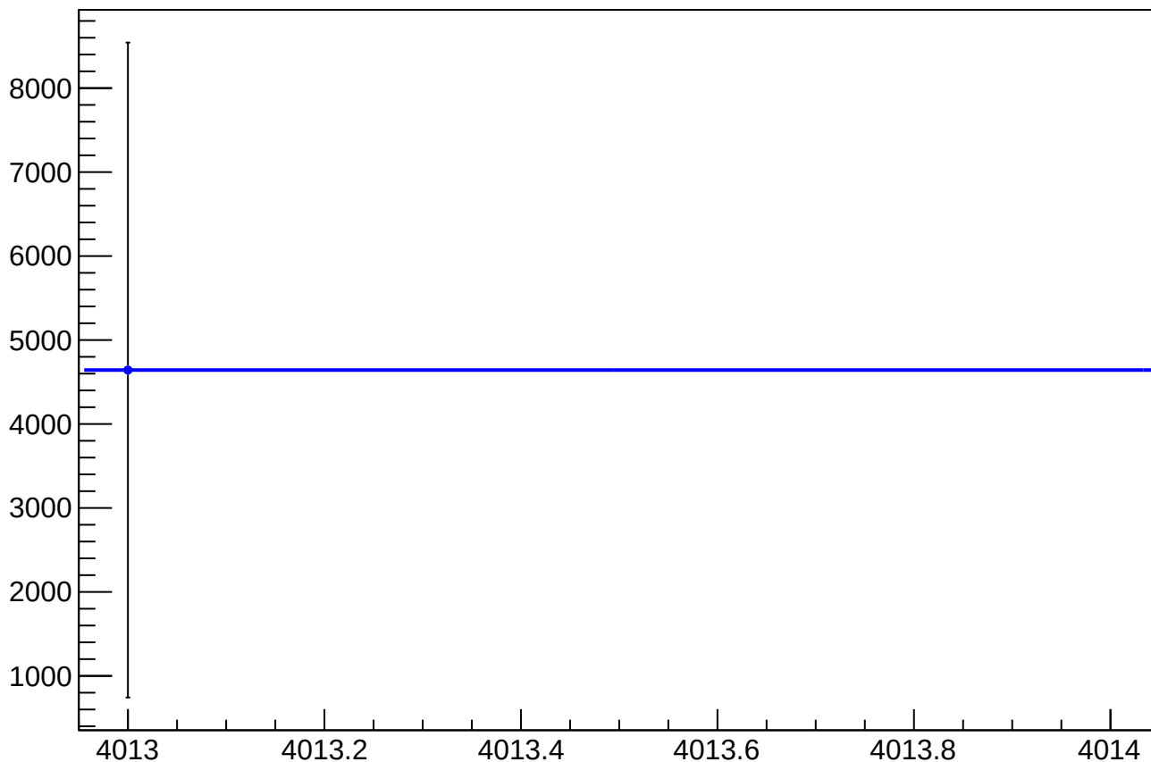
eigen_cor_asym_usr_atr2_avg_mean vs Slug
