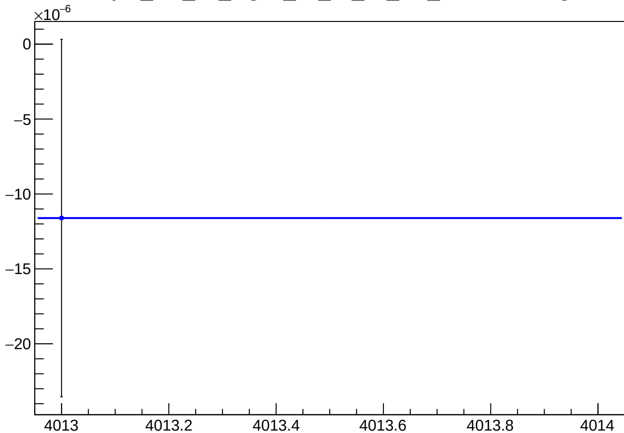
asym_at1_dd_eigen_dit_vs_dit_diff_mean vs Slug
