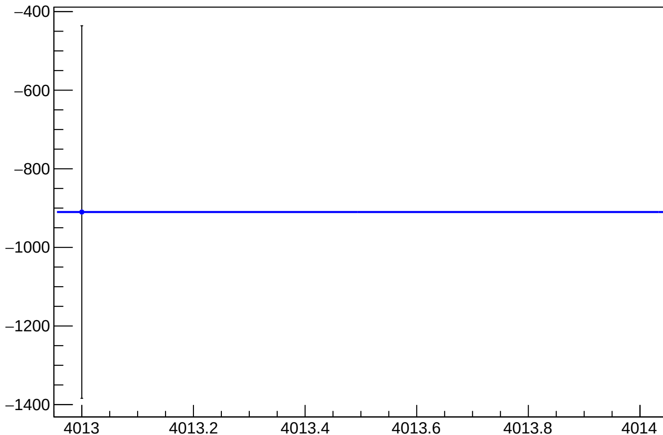
reg_asym_sam_15_26_dd_mean vs Slug
