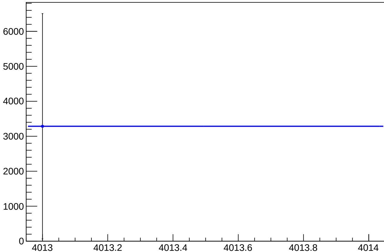
reg_asym_at1_avg_at2_avg_dd_mean vs Slug
