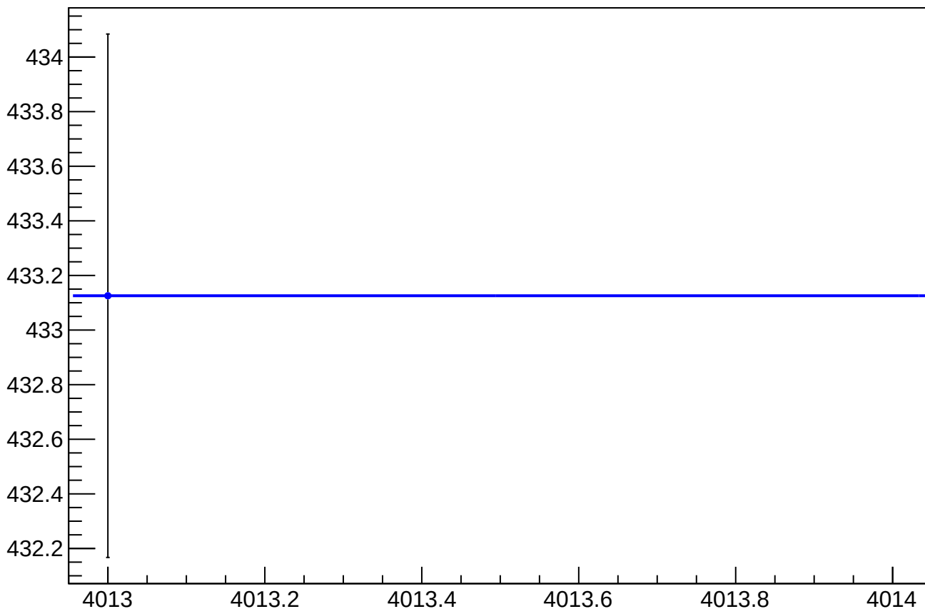
asym_us_avg_at2lr_avg_dd_dit_vs_cor_diff_rms vs Slug
