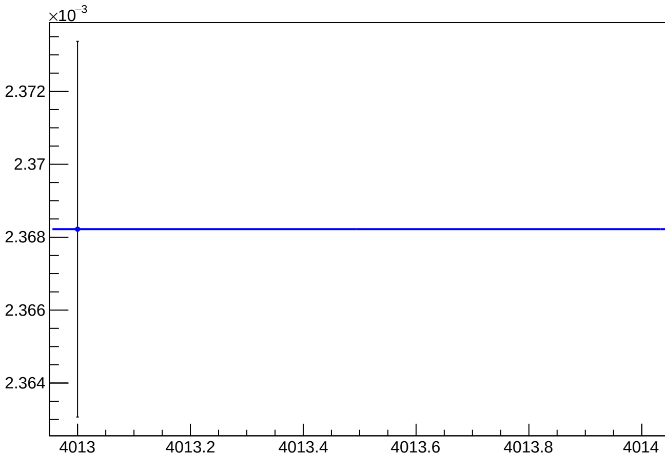
asym_sam_15_37_dd_eigen_dit_vs_dit_diff_rms vs Slug
