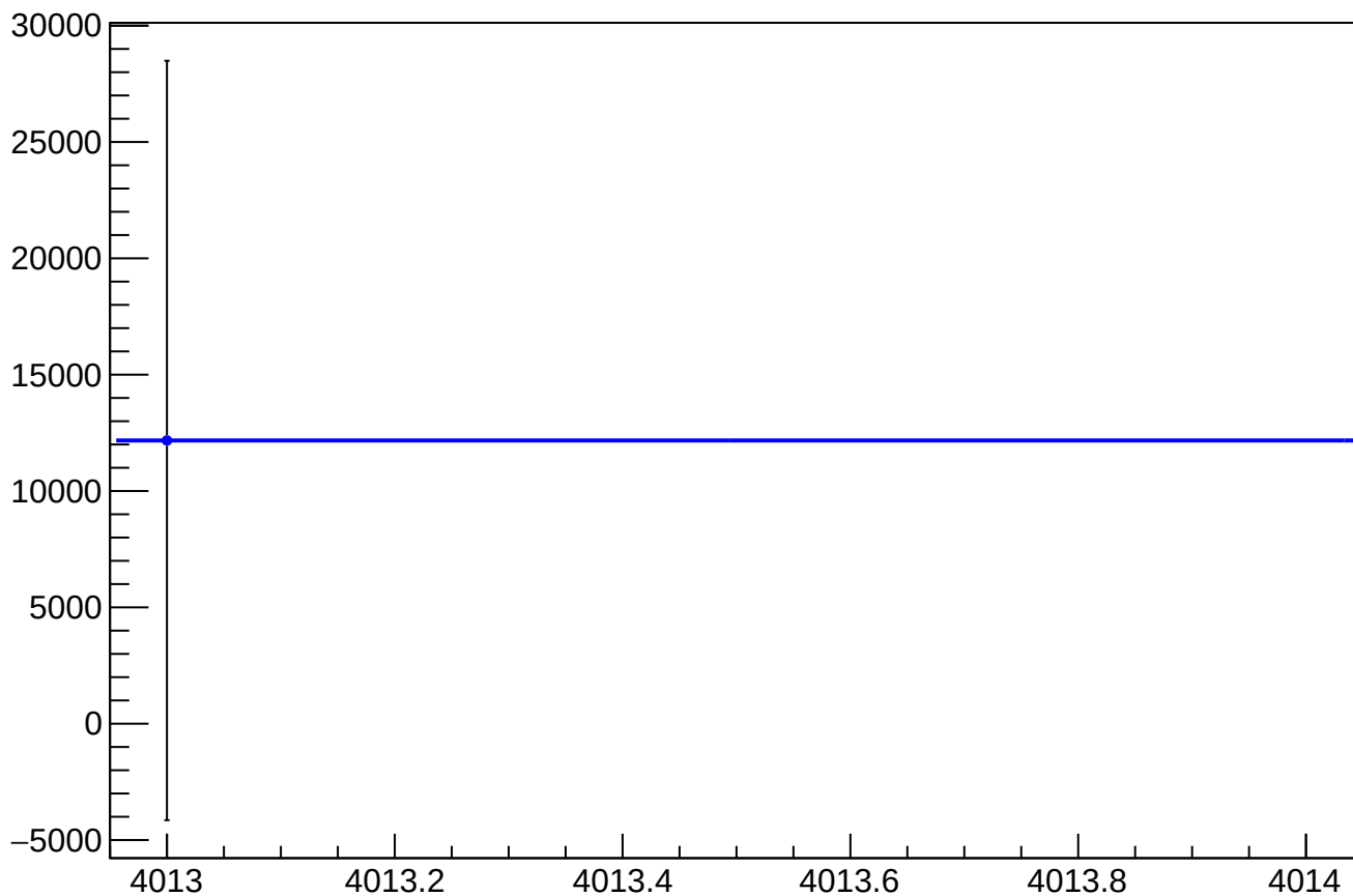
asym_usr_atr2_dd_mean vs Slug
