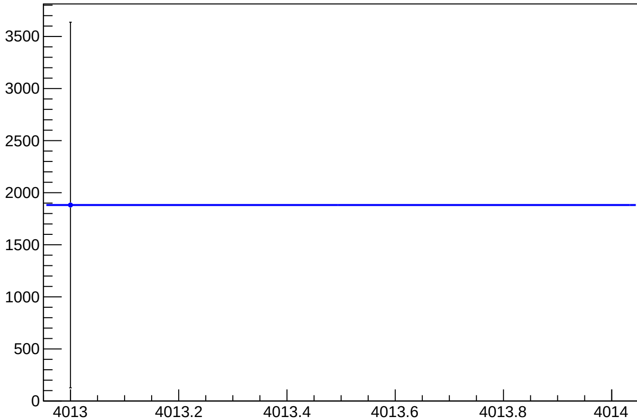
asym_usr_atr1_dd_dit_correction_mean vs Slug
