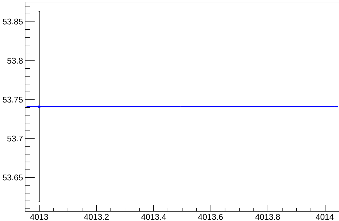
asym_sam_2468_avg_eigen_dit_vs_cor_diff_rms vs Slug
