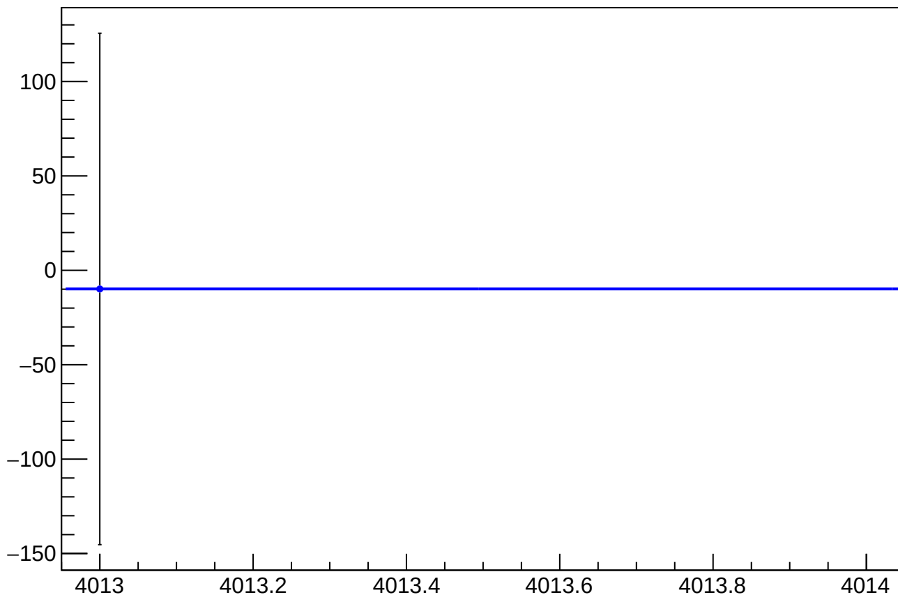
asym_atl1r2_dd_atl2r1_dd_avg_dit_correction_mean vs Slug
