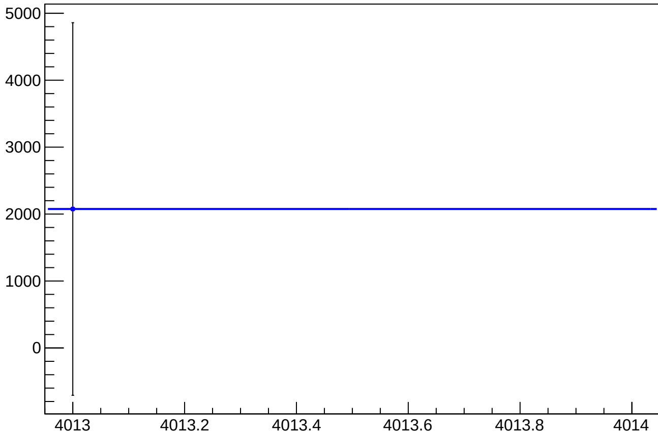
asym_usl_atl1_avg_cor_correction_mean vs Slug
