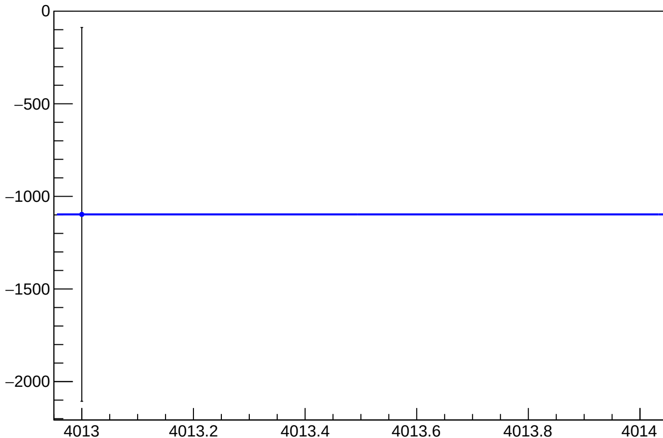
asym_us_dd_atlr_dd_dd_eigen_dit_correction_mean vs Slug
