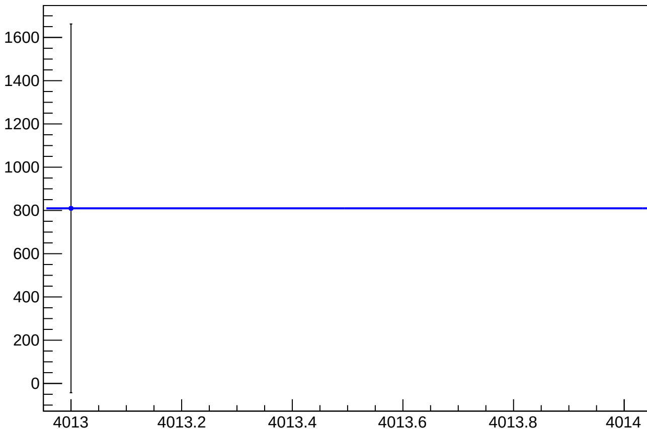
asym_sam_1357_2468_dd_dit_correction_mean vs Slug
