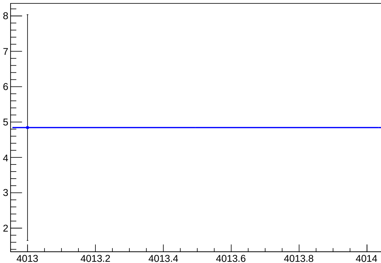
reg_asym_us_dd_atlr_dd_avg_diff_bpm4eY_slope vs Slug
