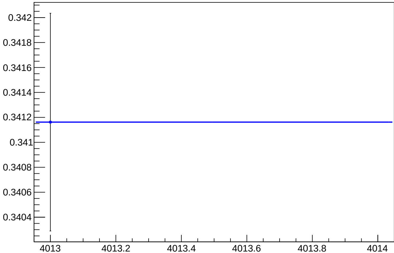
asym_us_dd_at2lr_dd_avg_reg_vs_cor_diff_rms vs Slug
