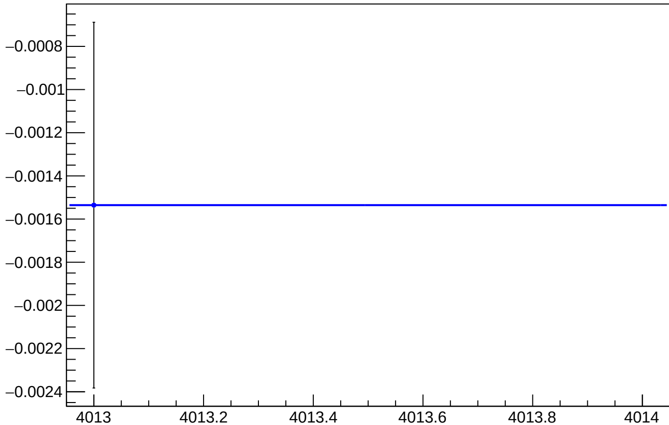
asym_at2_avg_reg_vs_cor_diff_mean vs Slug
