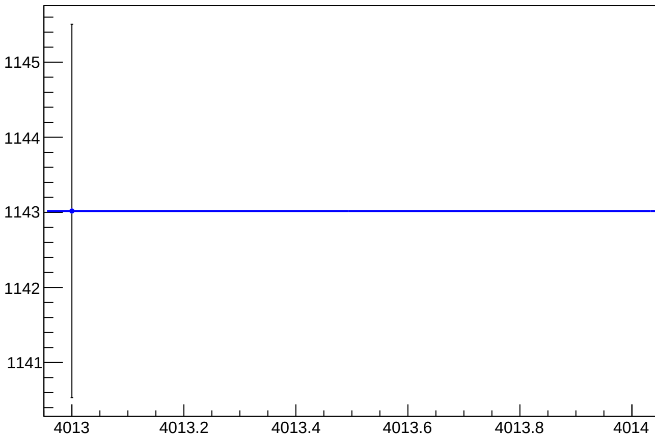
eigen_dit_asym_usl_atl1_avg_rms vs Slug
