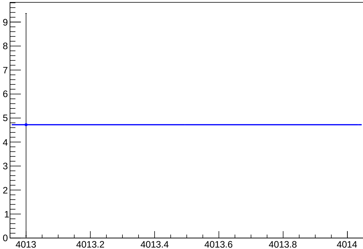
reg_asym_us_dd_at2lr_dd_avg_diff_bpm4eY_slope vs Slug
