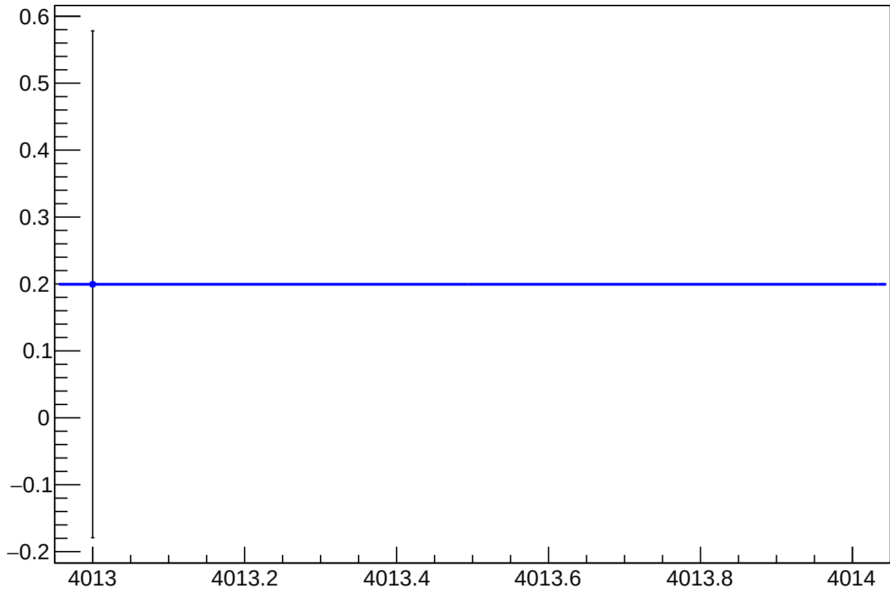
asym_usr_atr1_avg_eigen_dit_vs_cor_diff_mean vs Slug
