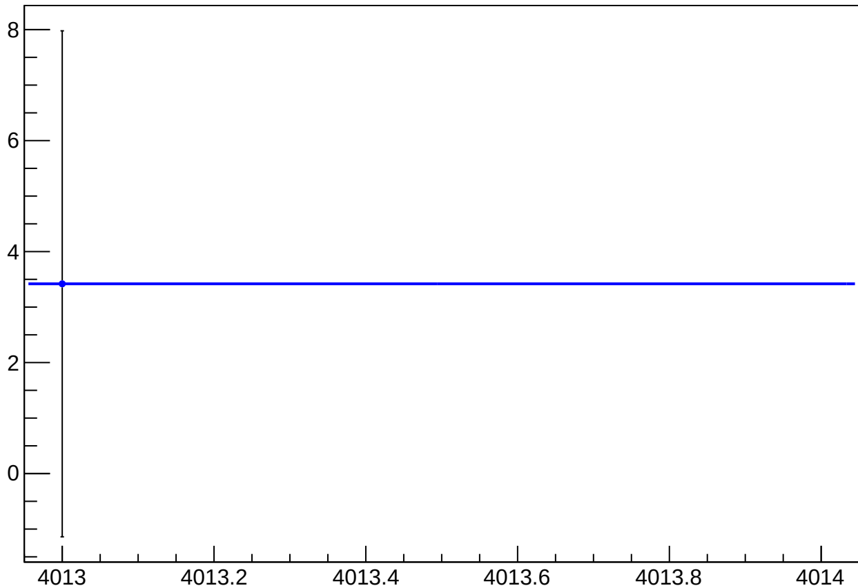
reg_asym_us_dd_at2lr_dd_avg_diff_bpm4aY_slope vs Slug, Sign Corrected
