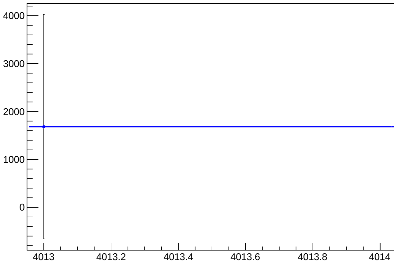
asym_at1_dd_at2_dd_avg_dit_correction_mean vs Slug, Sign Corrected
