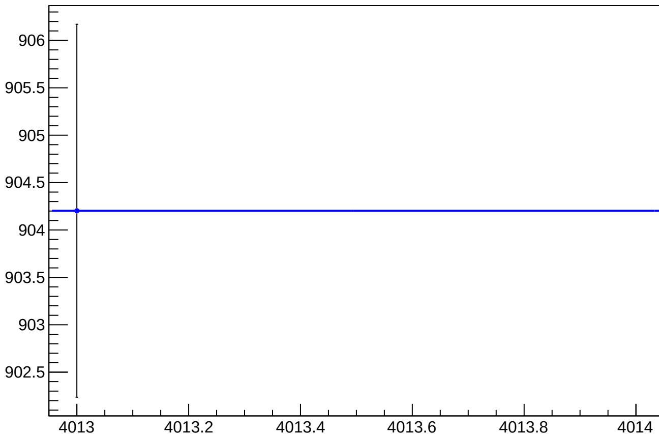
asym_sam_1548_avg_eigen_dit_correction_rms vs Slug, Sign Corrected
