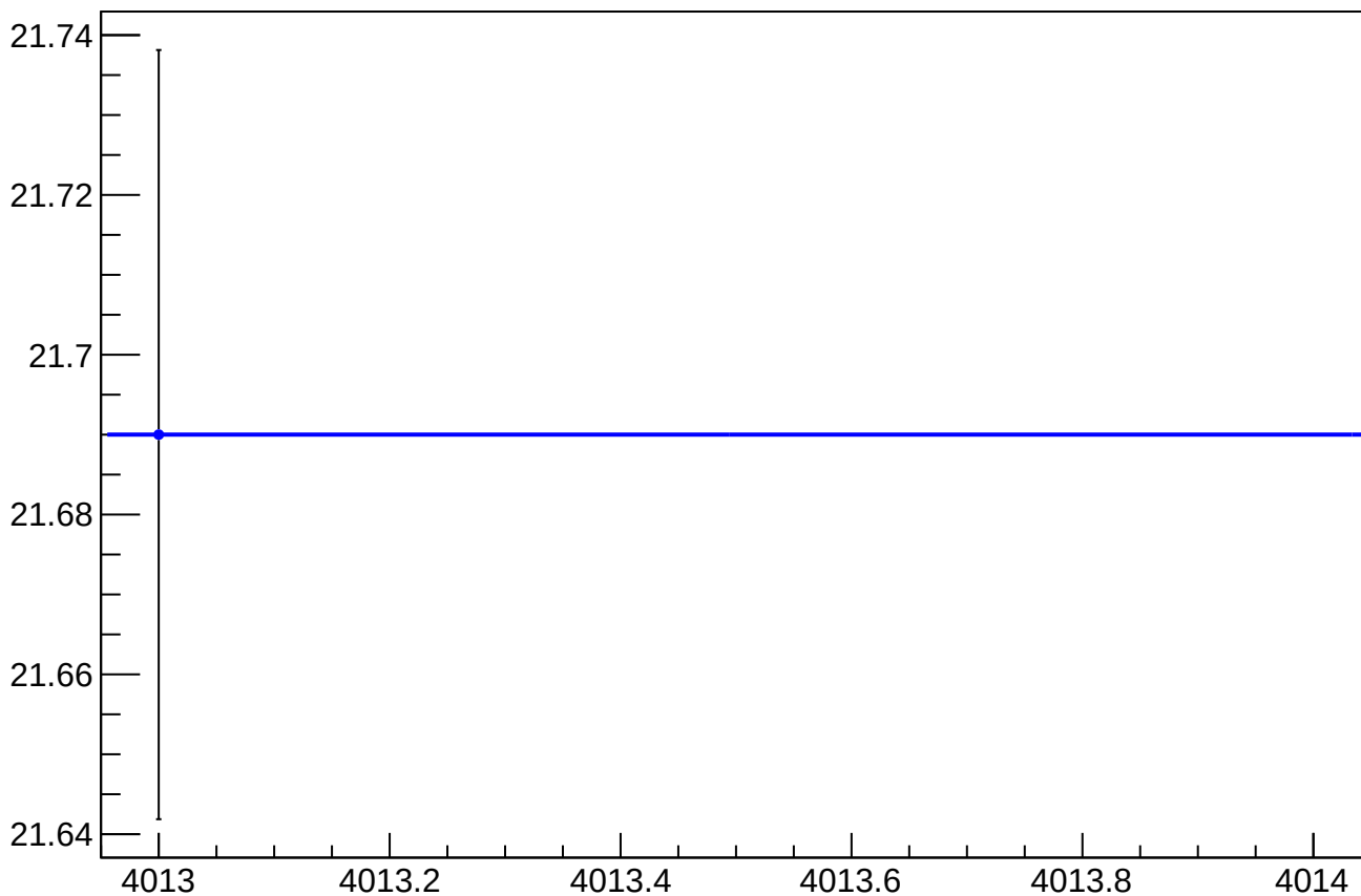
asym_sam_15_avg_eigen_dit_vs_eigen_cor_diff_rms vs Slug, Sign Corrected
