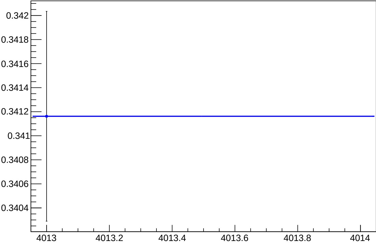
asym_us_dd_at2lr_dd_avg_reg_vs_cor_diff_rms vs Slug, Sign Corrected
