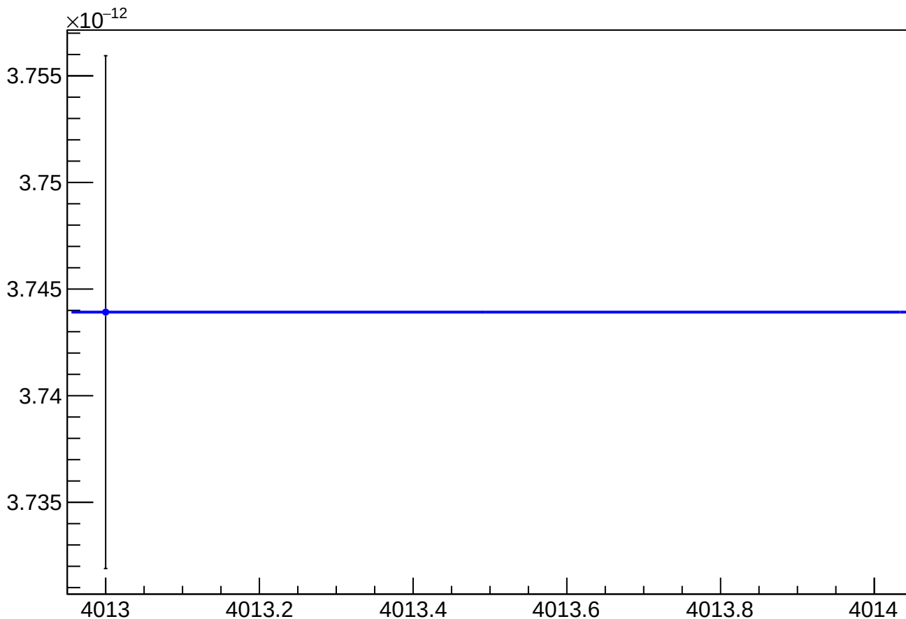
asym_sam1_eigen_cor_vs_cor_diff_rms vs Slug, Sign Corrected
