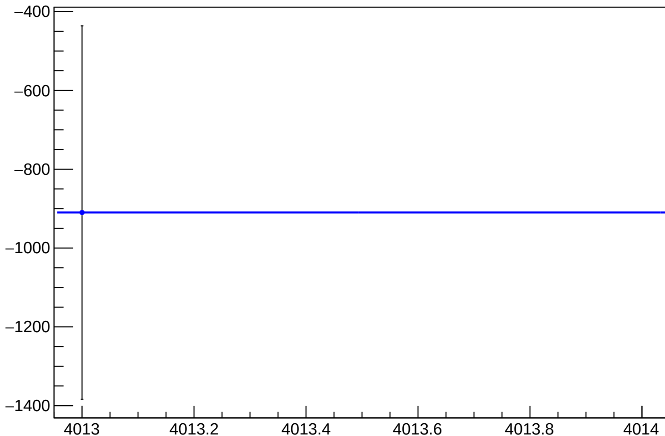
cor_asym_sam_15_26_dd_mean vs Slug, Sign Corrected
