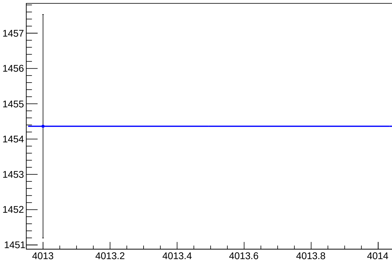
asym_sam_48_avg_dit_correction_rms vs Slug, Sign Corrected
