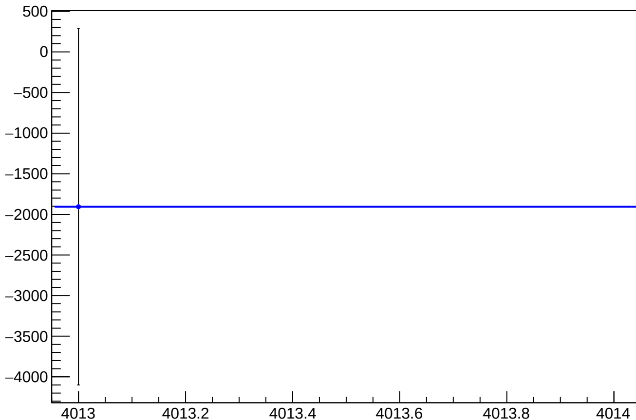
asym_sam_37_avg_eigen_cor_correction_mean vs Slug, Sign Corrected
