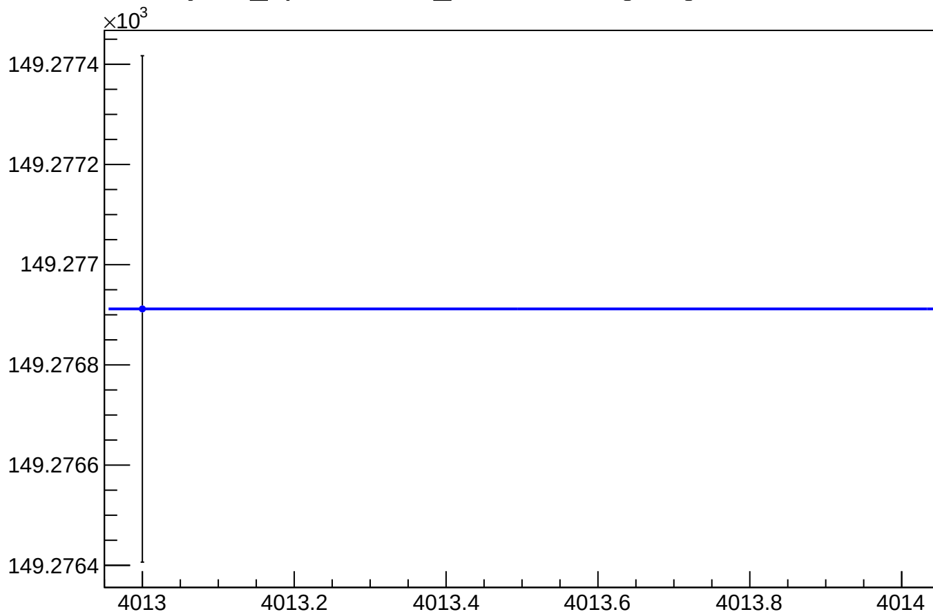
yield_bpm0l02WS_mean vs Slug, Sign Corrected
