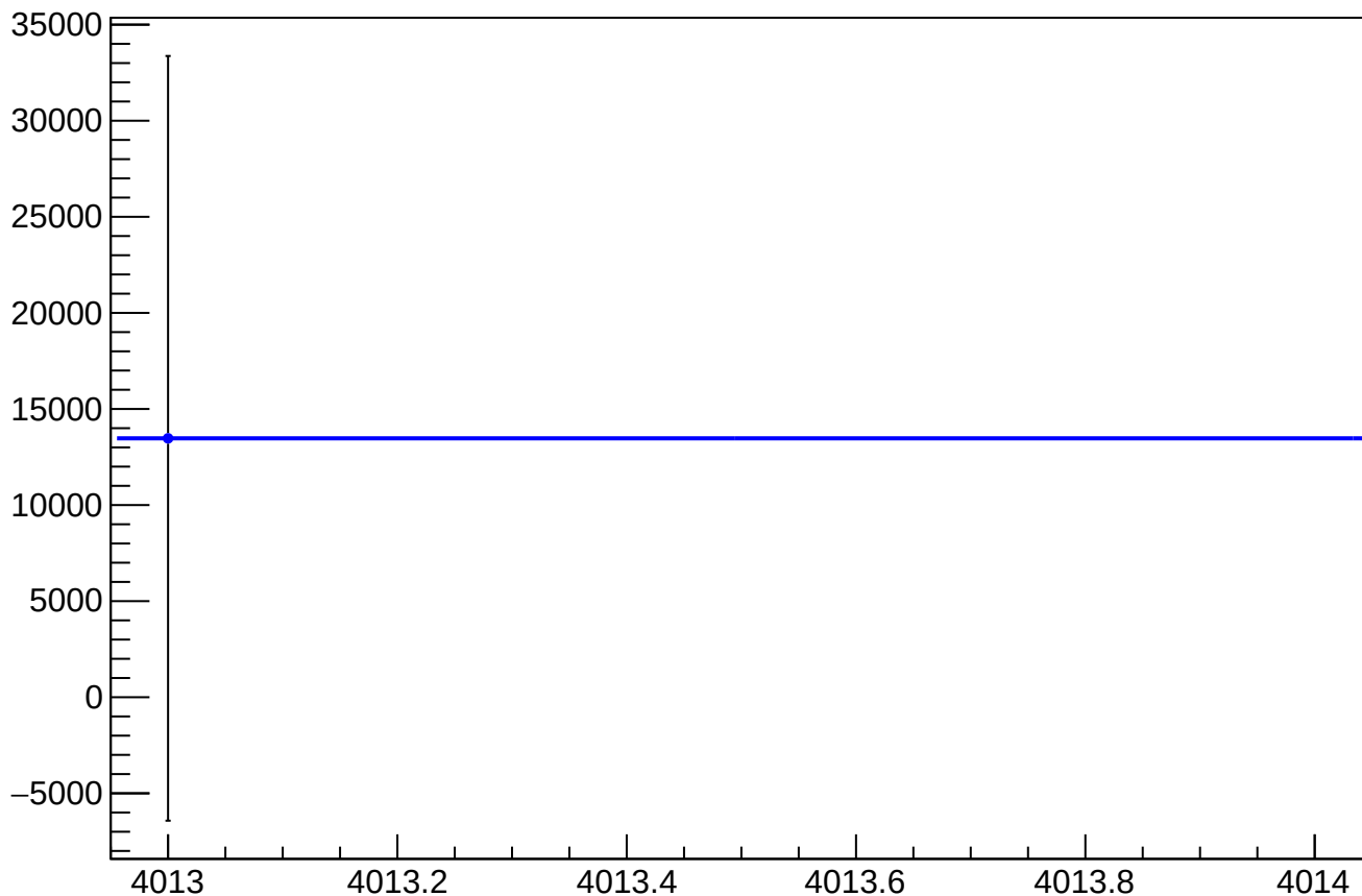
asym_atl_avg_cor_correction_mean vs Slug, Sign Corrected
