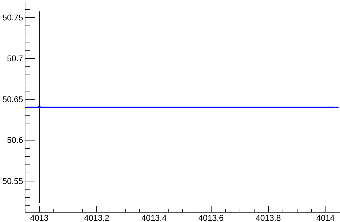
asym_sam_3748_avg_dit_vs_cor_diff_rms vs Slug, Sign Corrected
