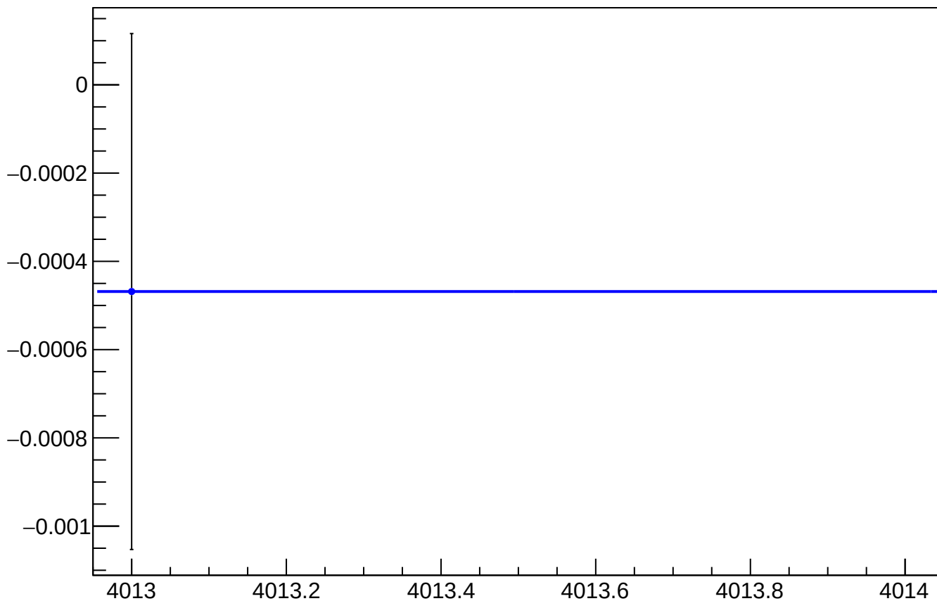
asym_usr_atr1_dd_reg_vs_cor_diff_mean vs Slug, Sign Corrected
