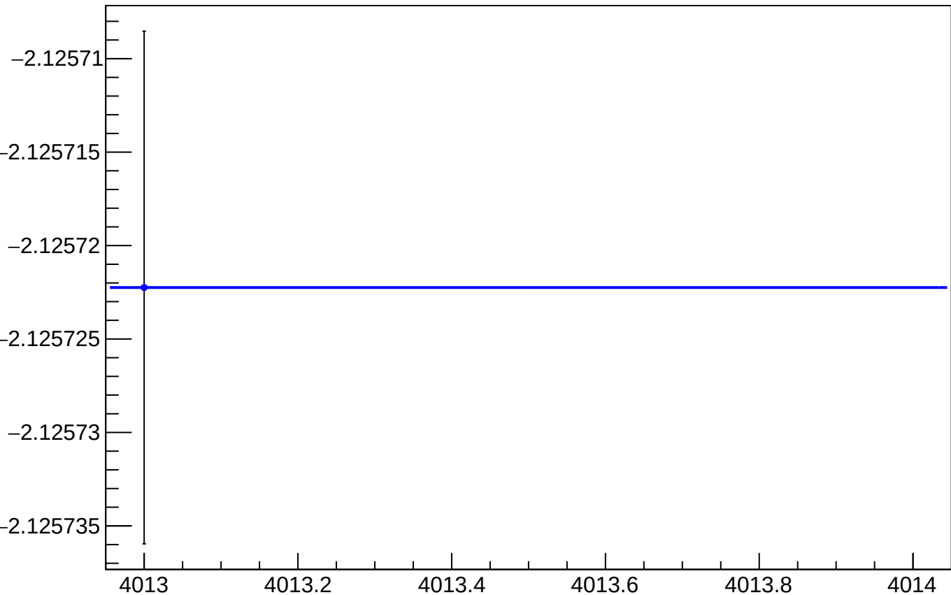
yield_bpm0i01aX_mean vs Slug, Sign Corrected
