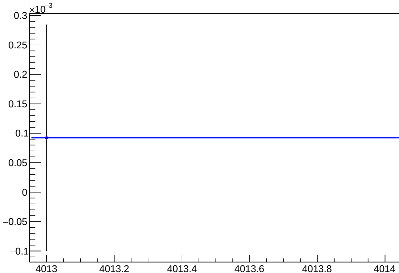
asym_atl1r2_dd_reg_vs_cor_diff_mean vs Slug, Sign Corrected
