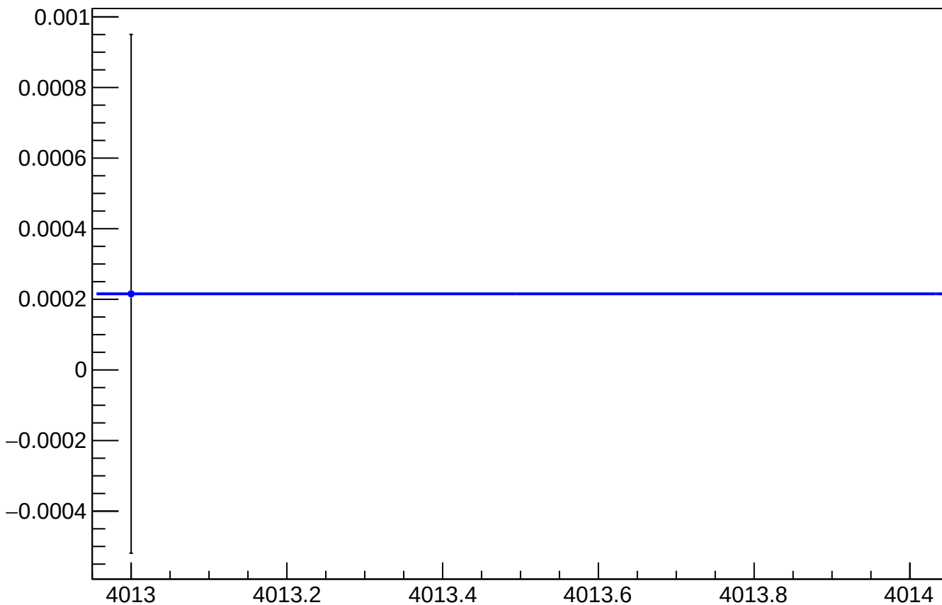
asym_us_avg_atlr_avg_dd_reg_vs_cor_diff_mean vs Slug, Sign Corrected
