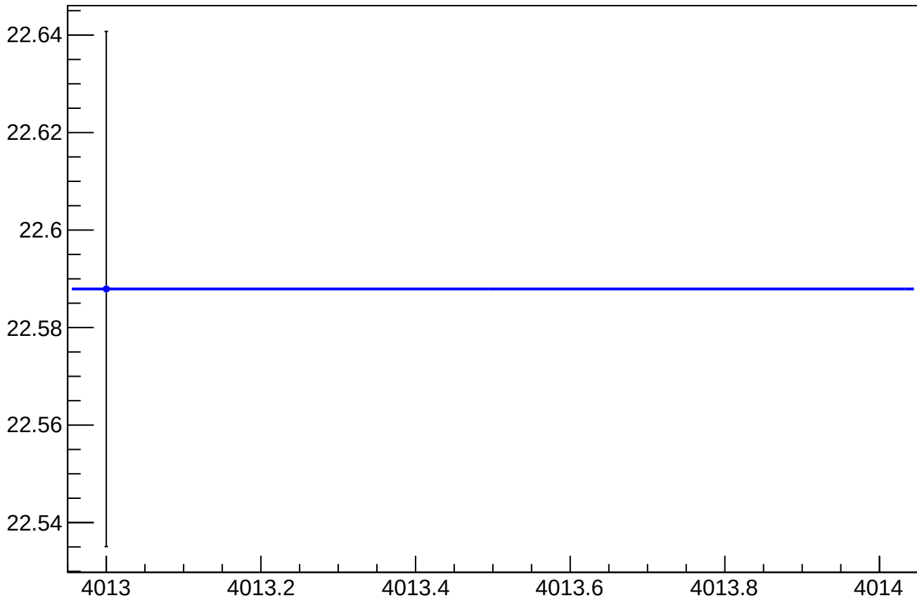
asym_us_dd_atlr_dd_dd_dit_vs_eigen_cor_diff_rms vs Slug, Sign Corrected
