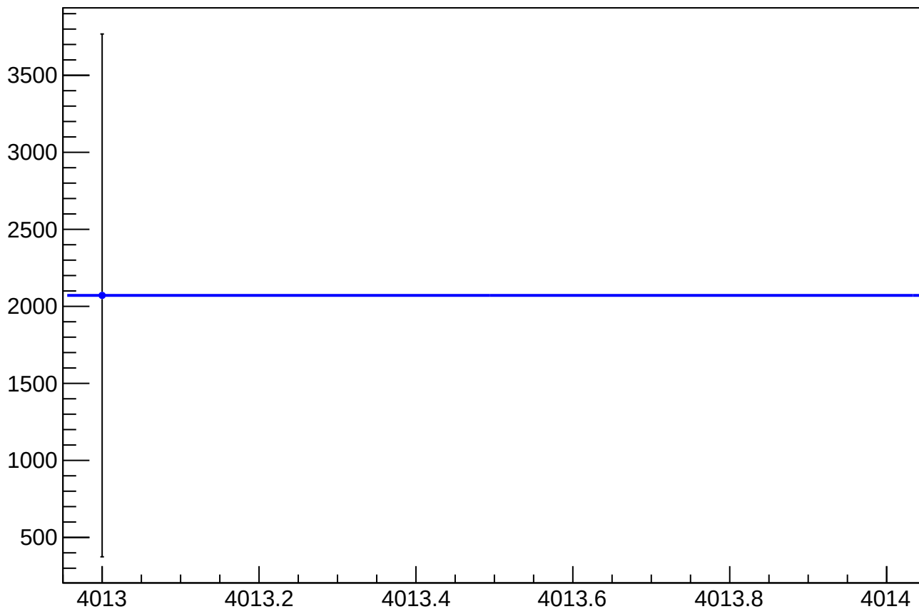
asym_sam_15_26_dd_reg_correction_mean vs Slug, Sign Corrected
