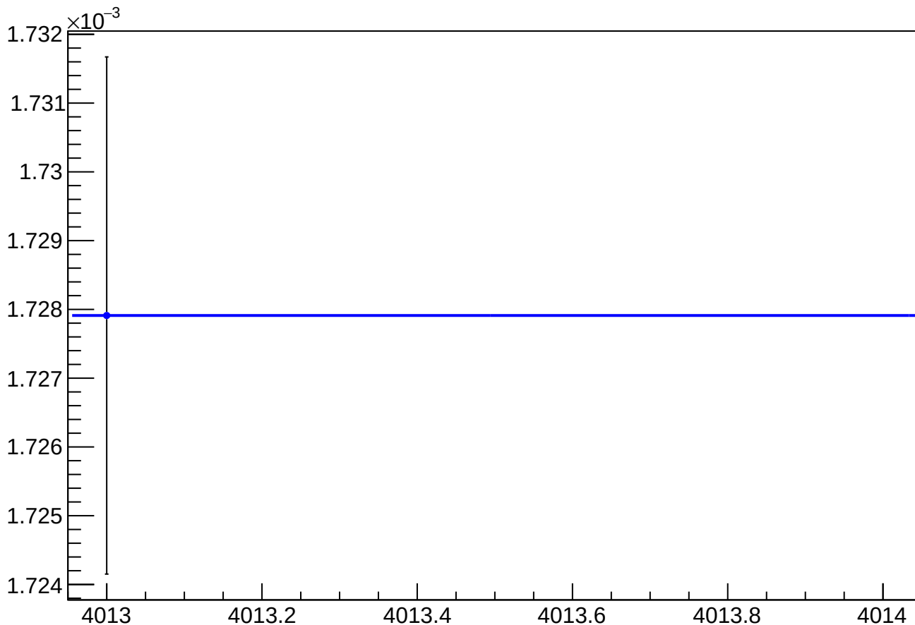
asym_sam8_eigen_dit_vs_dit_diff_rms vs Slug, Sign Corrected
