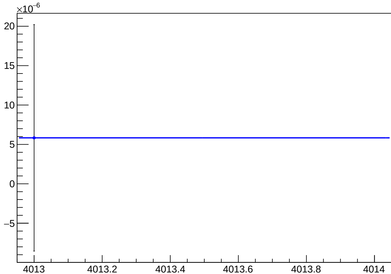
asym_atl_dd_atr_dd_dd_eigen_dit_vs_dit_diff_mean vs Slug, Sign Corrected
