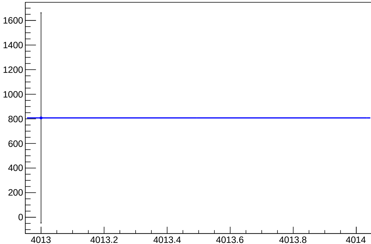
asym_sam_1357_2468_dd_reg_correction_mean vs Slug, Sign Corrected
