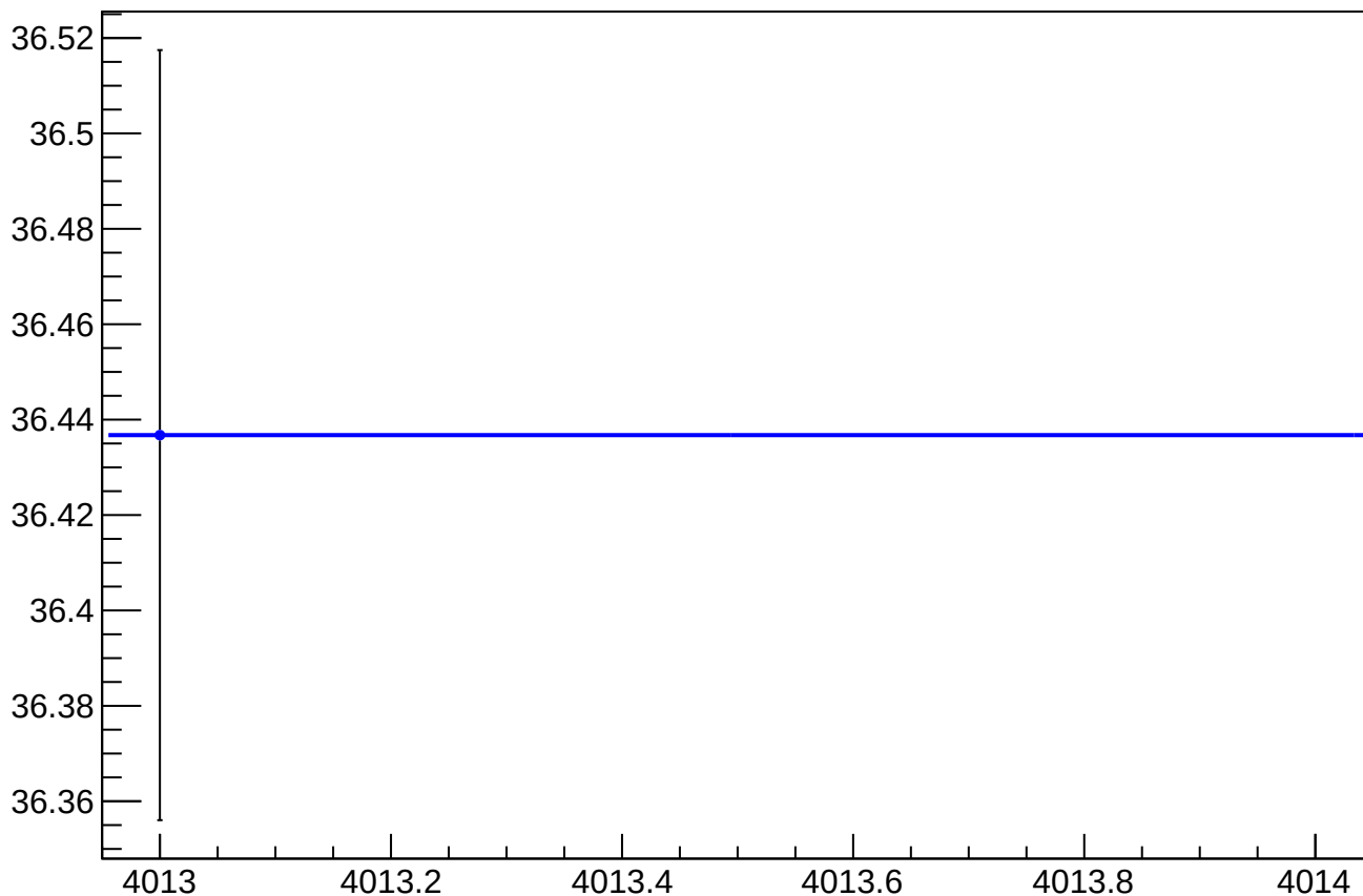
asym_usl_overload_cor_vs_eigen_cor_diff_rms vs Slug, Sign Corrected
