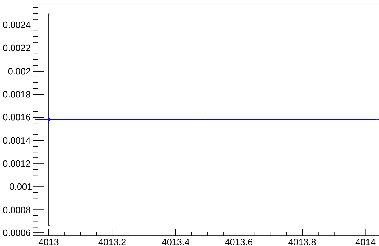
asym_atr1l2_dd_reg_vs_cor_diff_mean vs Slug, Sign Corrected
