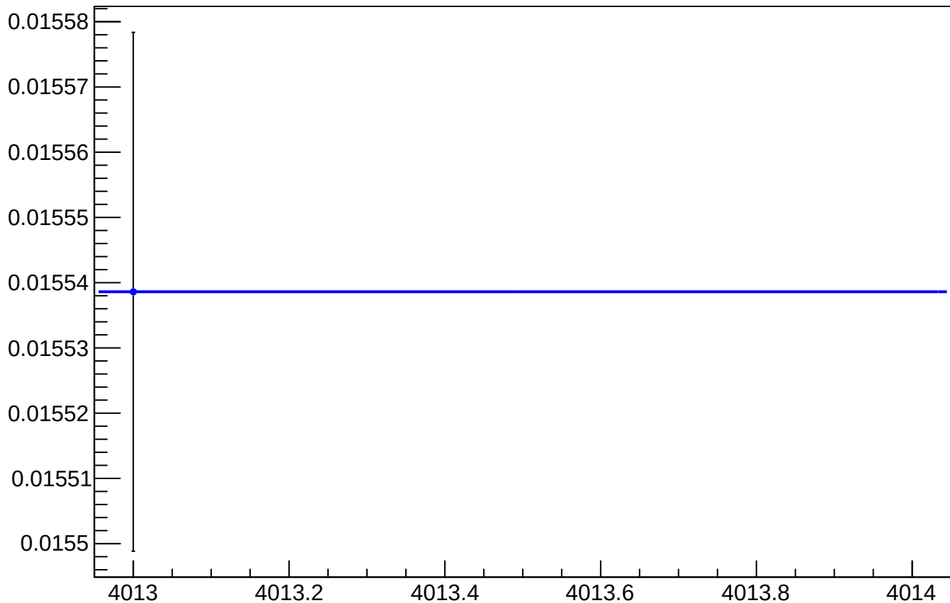
asym_sam_13_57_dd_reg_vs_cor_diff_rms vs Slug, Sign Corrected
