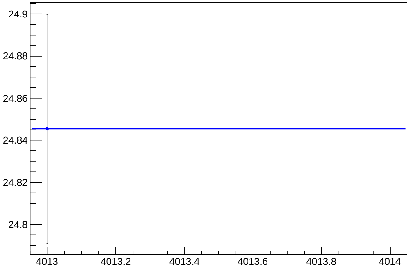
asym_sam_15_37_dd_eigen_dit_vs_eigen_cor_diff_rms vs Slug, Sign Corrected
