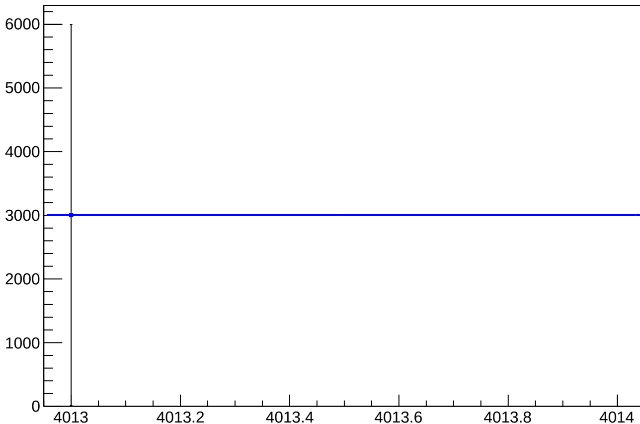
asym_atl1_dit_correction_mean vs Slug, Sign Corrected
