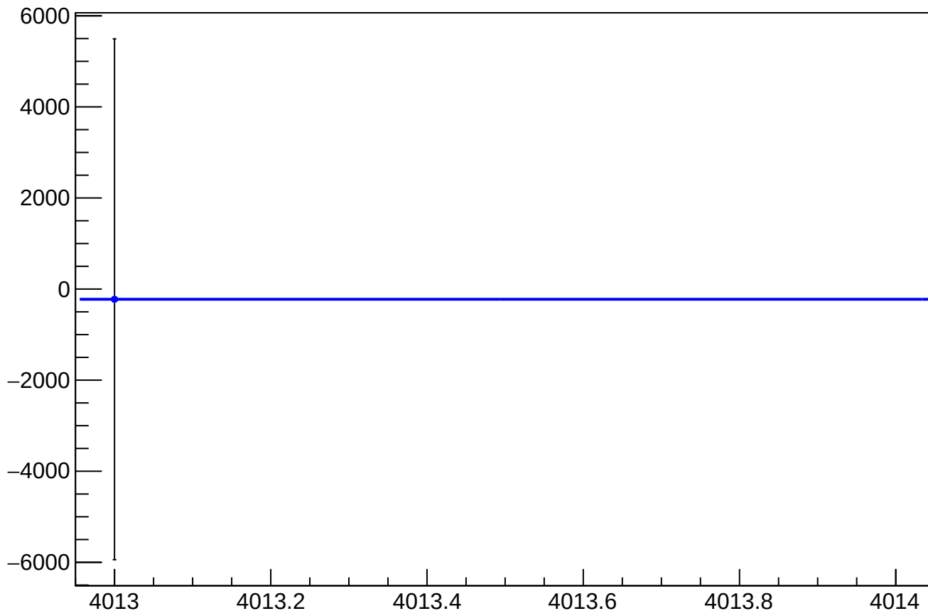
eigen_cor_asym_us_avg_at2lr_avg_avg_mean vs Slug, Sign Corrected
