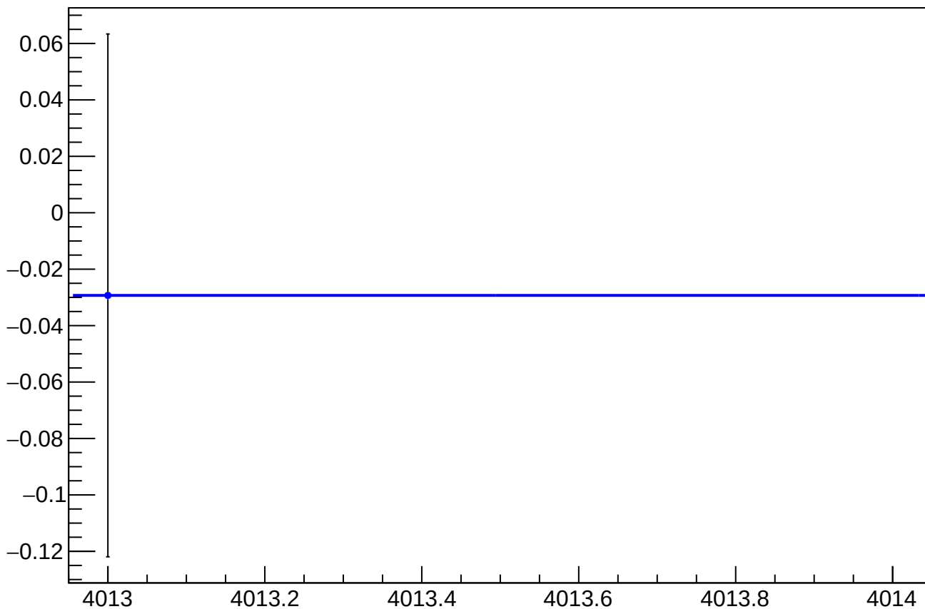
asym_us_dd_at2lr_dd_dd_eigen_dit_vs_cor_diff_mean vs Slug, Sign Corrected
