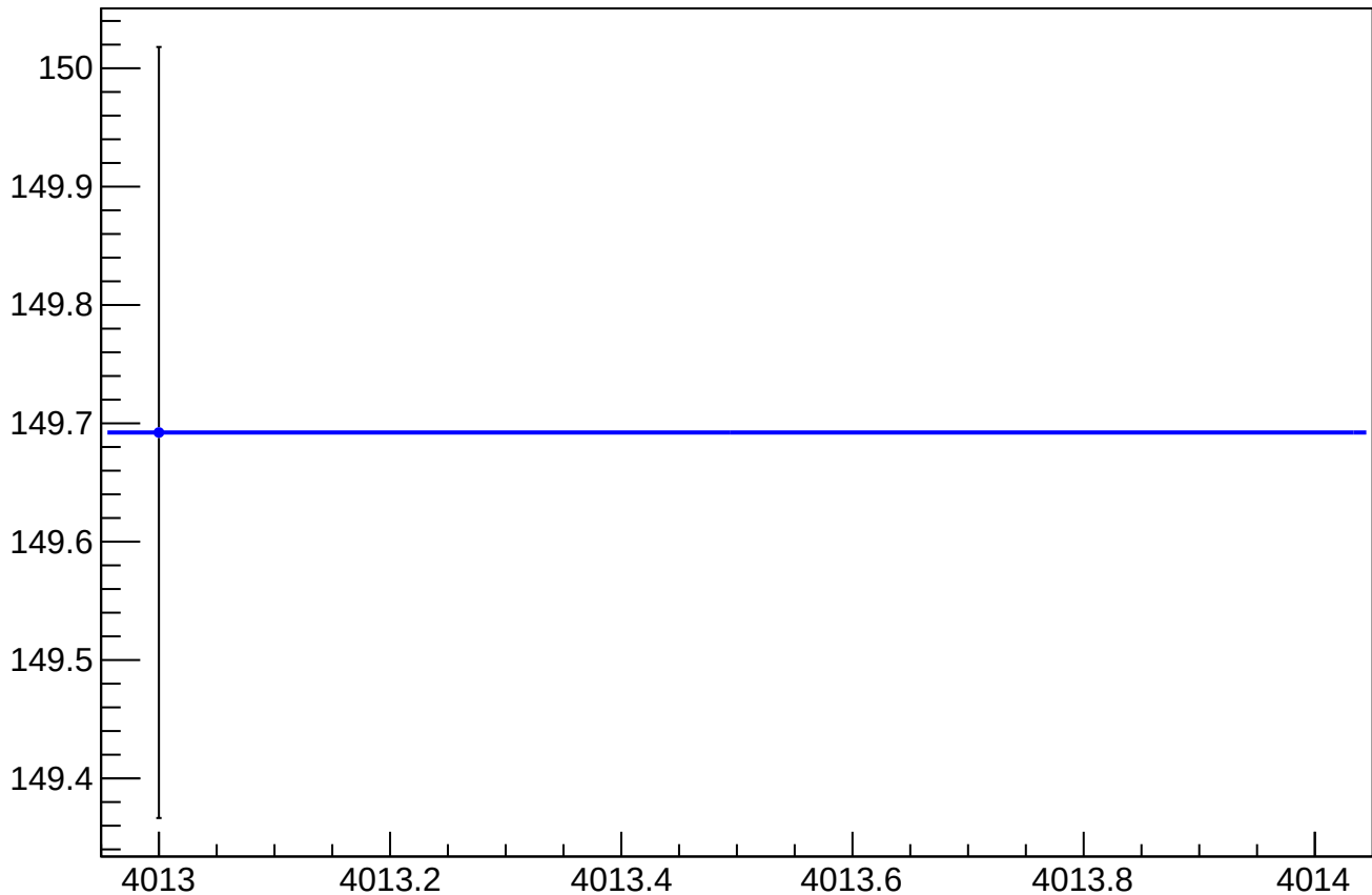
eigen_cor_asym_sam8_rms vs Slug, Sign Corrected
