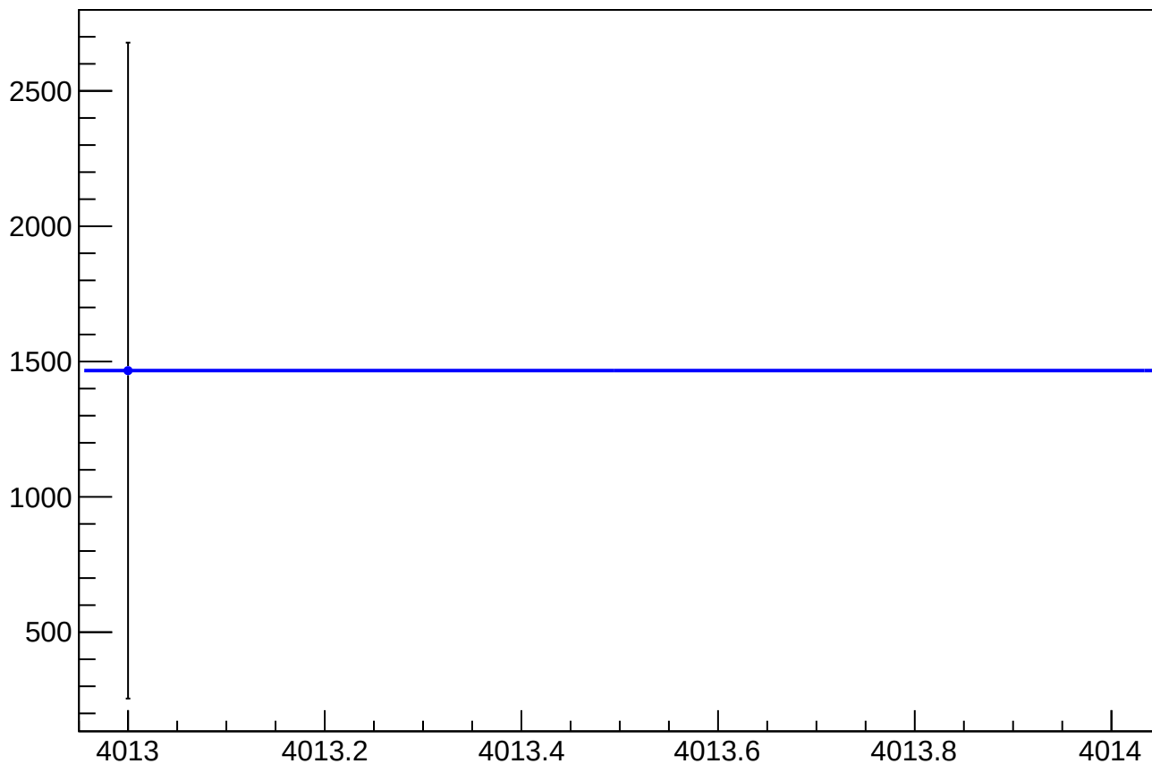
asym_sam_15_37_dd_eigen_dit_correction_mean vs Slug, Sign Corrected
