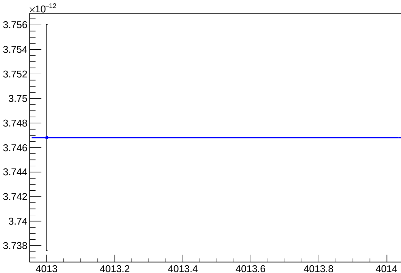
asym_sam_37_26_dd_eigen_cor_vs_cor_diff_rms vs Slug, Sign Corrected
