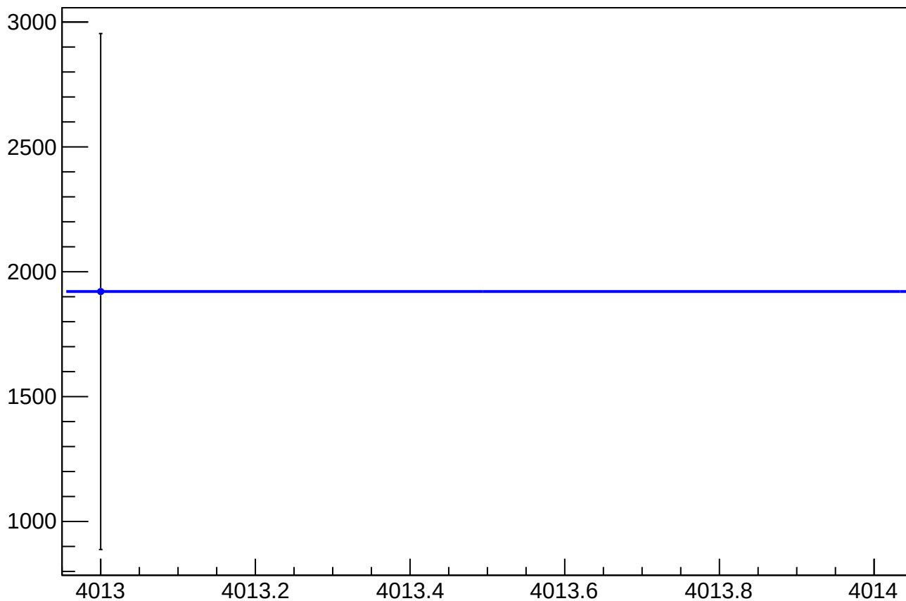
cor_asym_sam_26_dd_mean vs Slug, Sign Corrected
