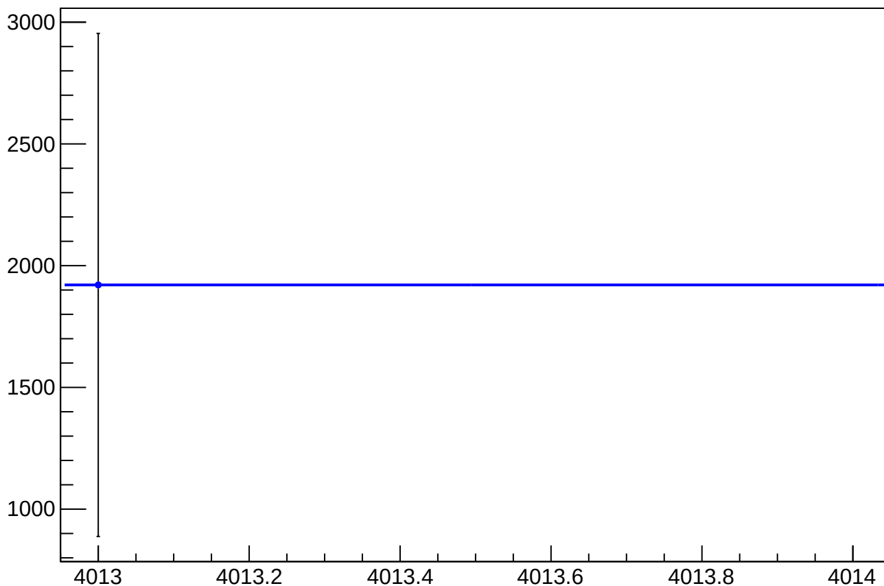
eigen_cor_asym_sam_26_dd_mean vs Slug, Sign Corrected
