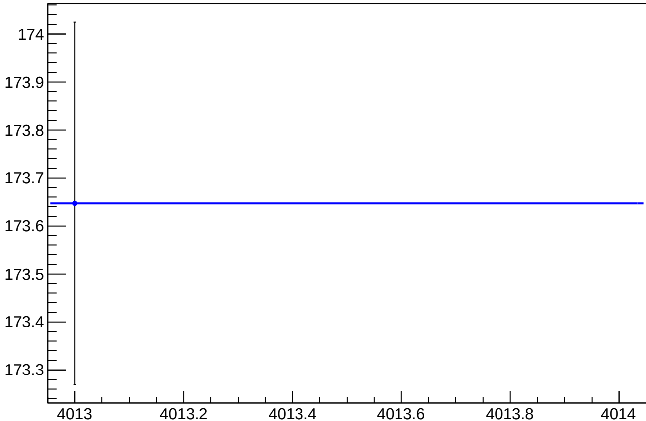
cor_asym_sam_26_48_dd_rms vs Slug, Sign Corrected
