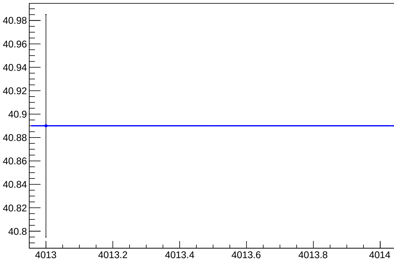
asym_sam_48_dd_dit_vs_slug, Sign Corrected
