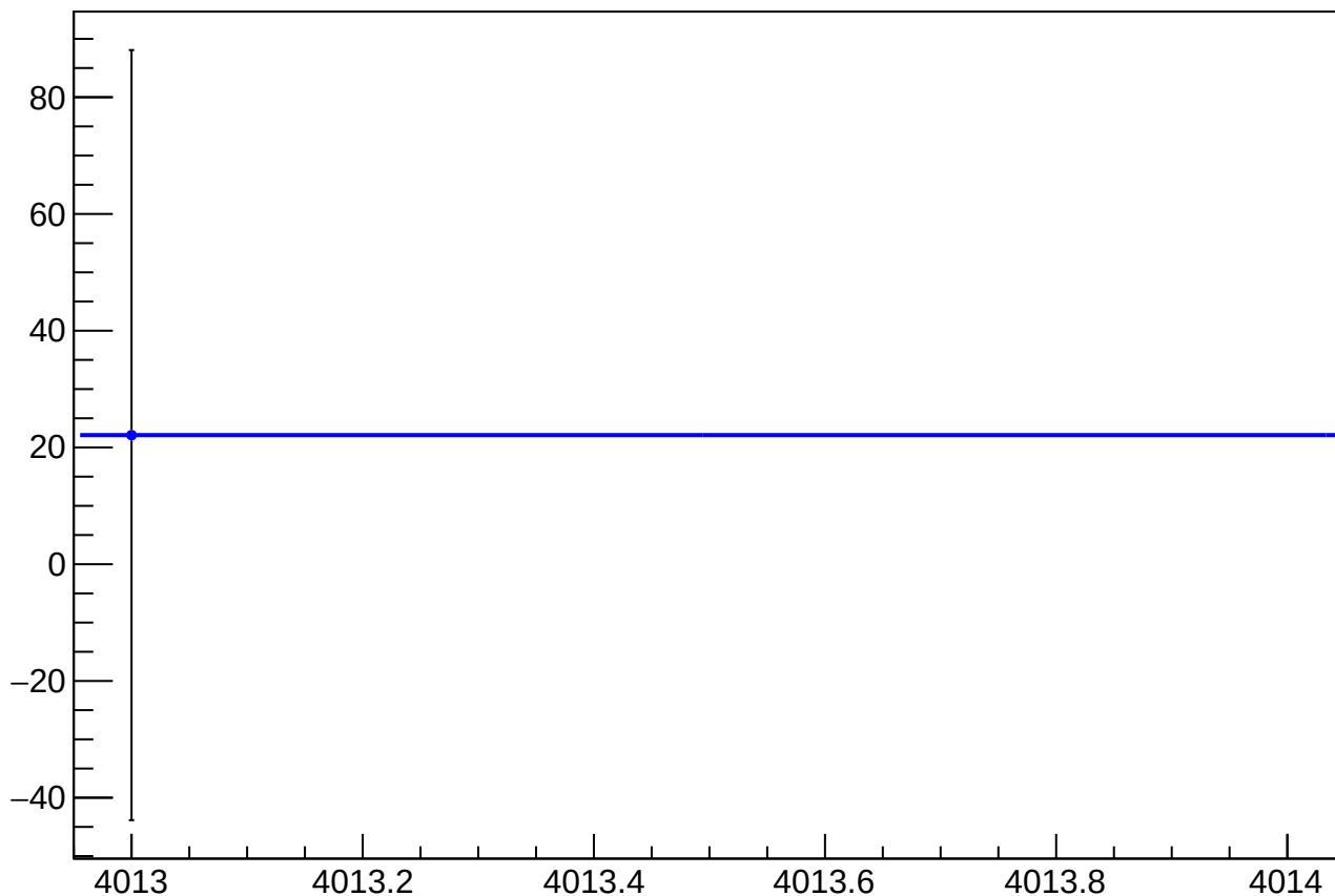
asym_bcm_an_avg_bcm_dg_us_agg_dd_mean vs Slug, Sign Corrected
