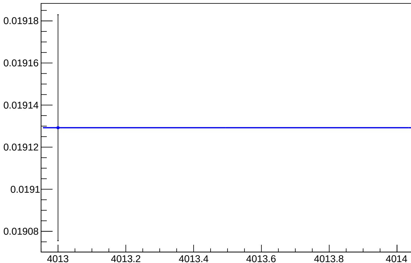
asym_sam_24_68_dd_reg_vs_cor_diff_rms vs Slug, Sign Corrected
