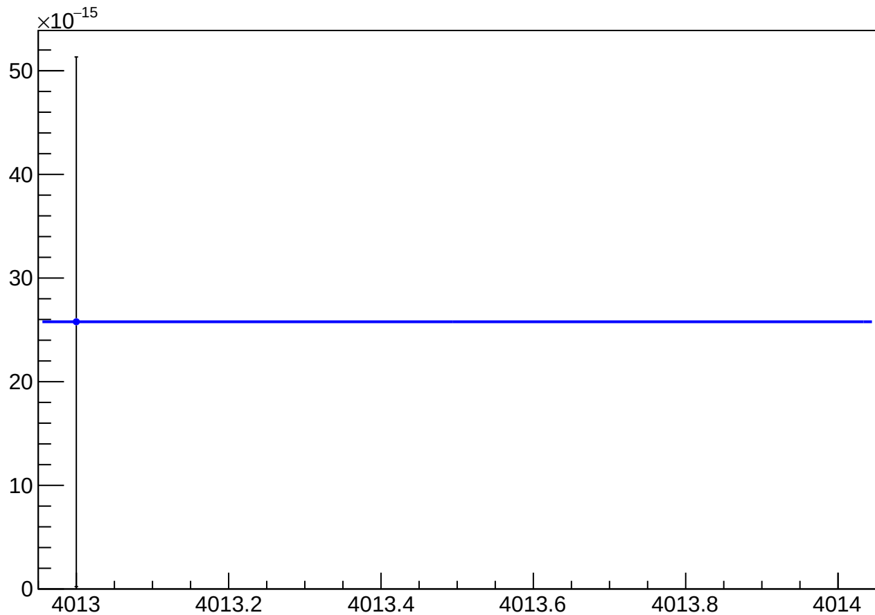
asym_sam7_eigen_cor_vs_cor_diff_mean vs Slug, Sign Corrected
