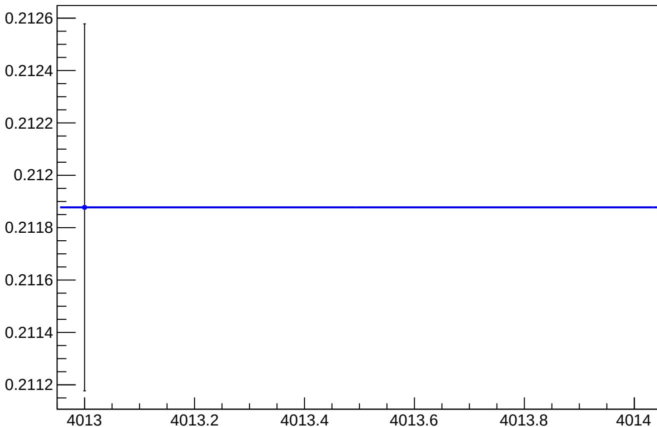
asym_atl1_reg_vs_cor_diff_rms vs Slug, Sign Corrected
