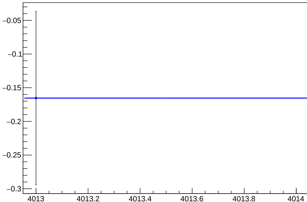
reg_asym_bcm_2an_us_an_ds_dd_diff_bpm4eY_slope vs Slug, Sign Corrected
