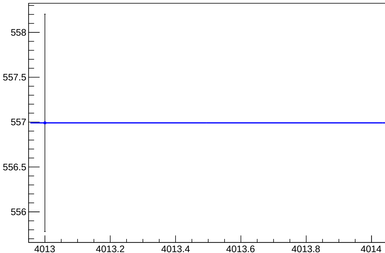
eigen_cor_asym_us_dd_rms vs Slug, Sign Corrected
