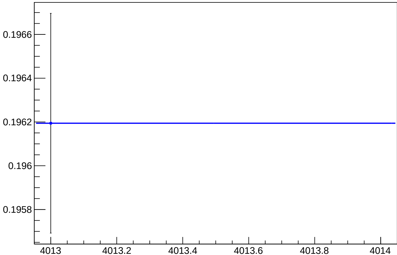
asym_usr_atr2_avg_reg_vs_cor_diff_rms vs Slug, Sign Corrected
