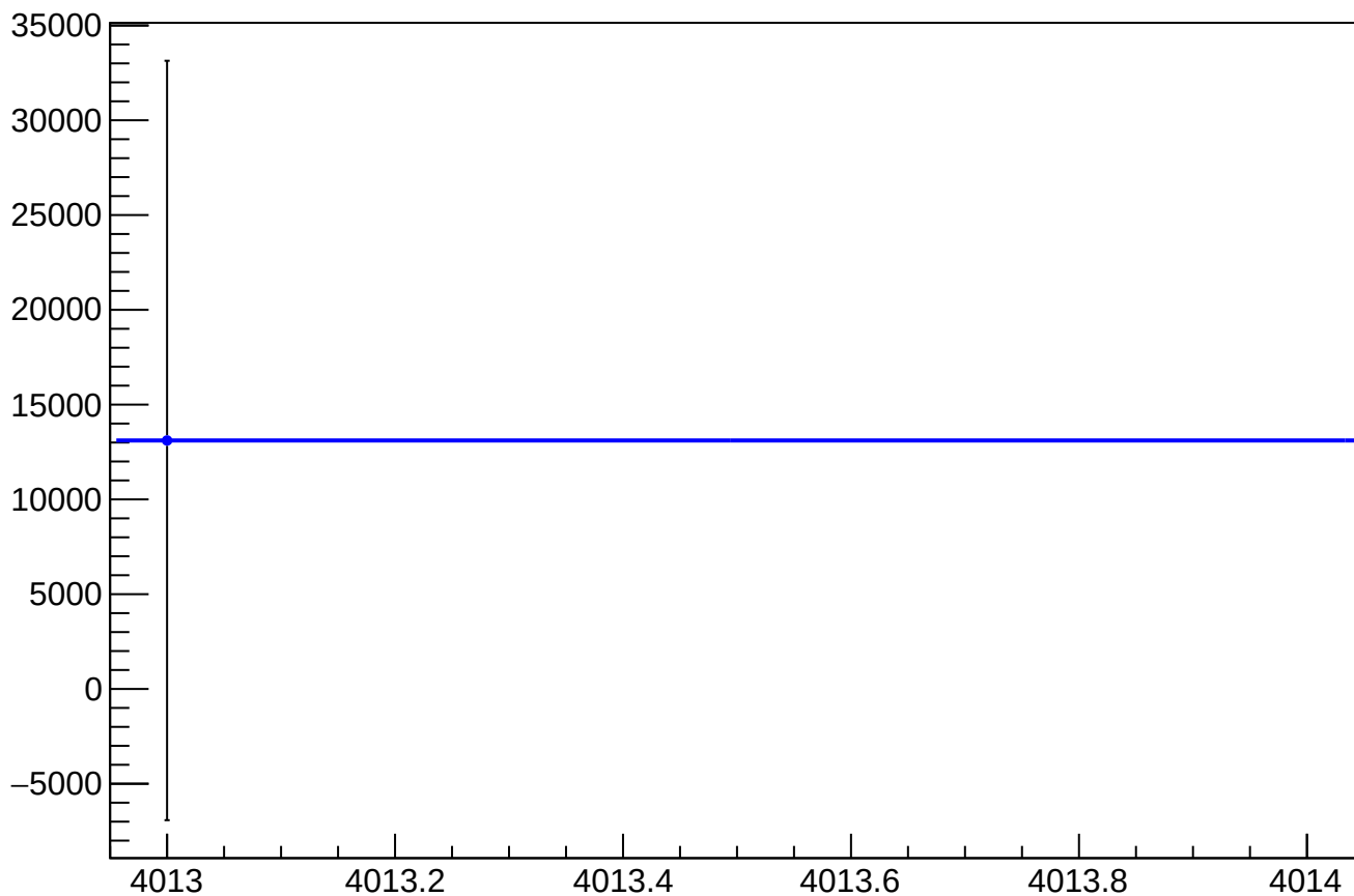
asym_atl_avg_dit_correction_mean vs Slug, Sign Corrected
