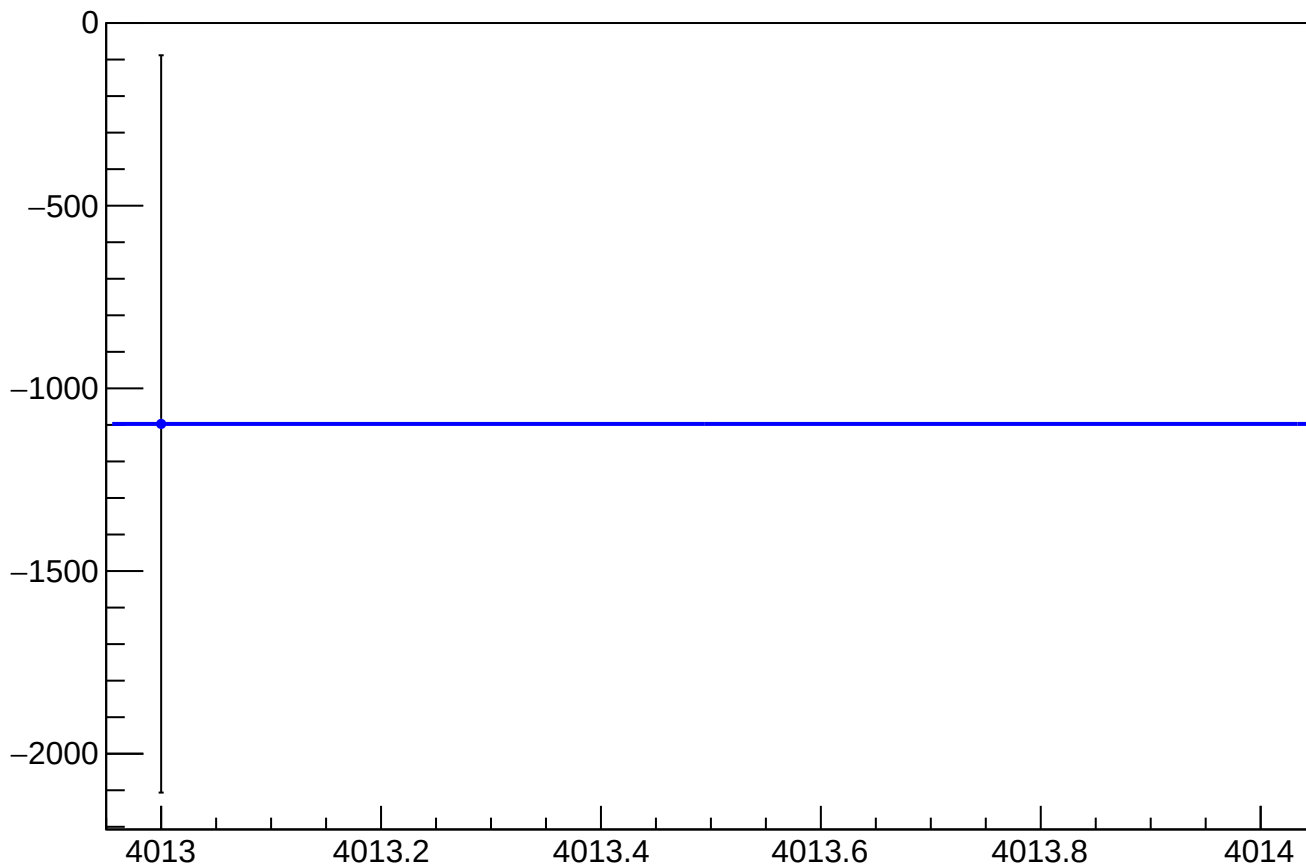
asym_us_dd_atlr_dd_dd_dit_correction_mean vs Slug, Sign Corrected
