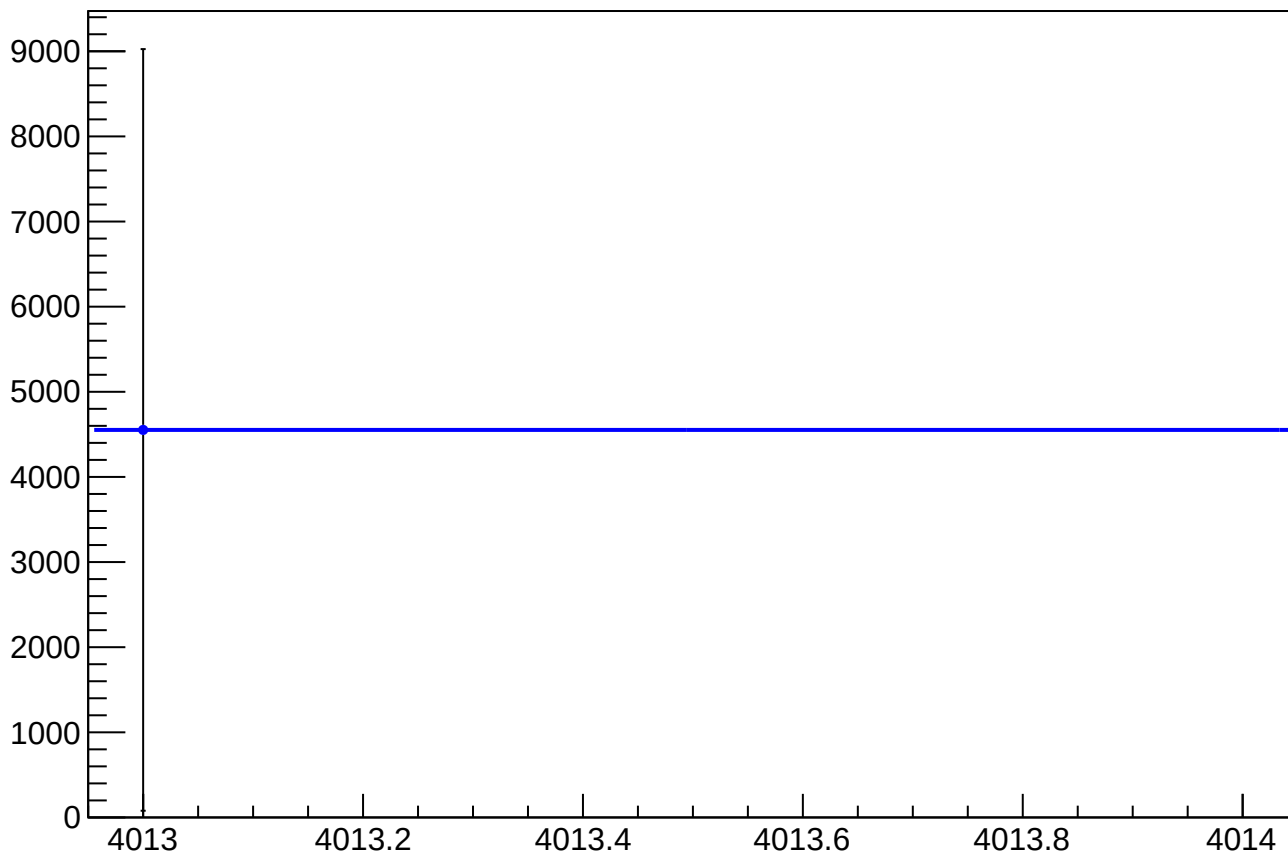
eigen_cor_asym_at2_dd_mean vs Slug, Sign Corrected
