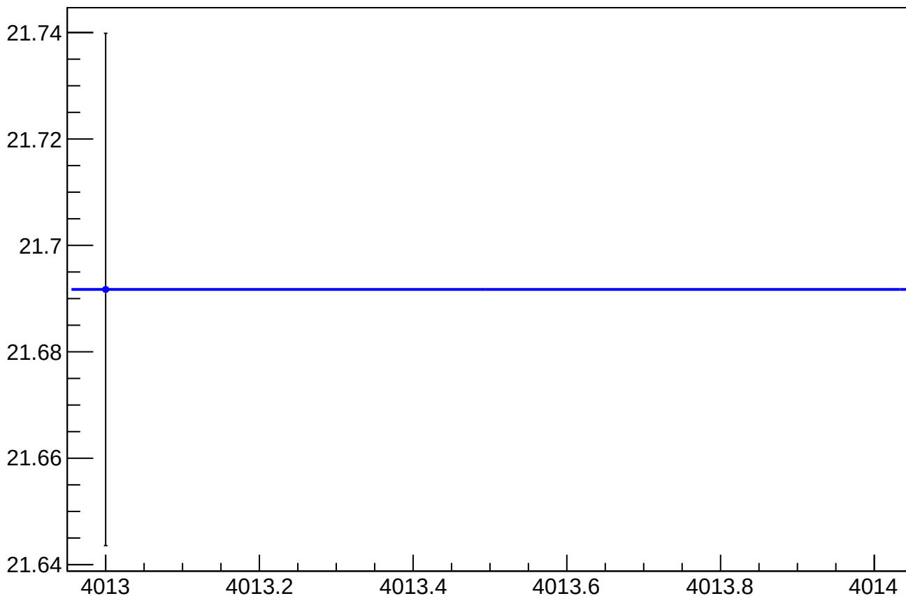
asym_sam_15_avg_dit_vs_eigen_cor_diff_rms vs Slug, Sign Corrected
