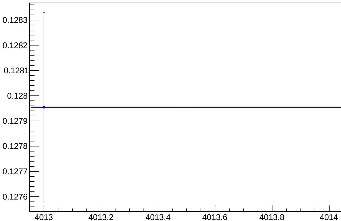
asym_usl_atl2_dd_reg_vs_cor_diff_rms vs Slug, Sign Corrected
