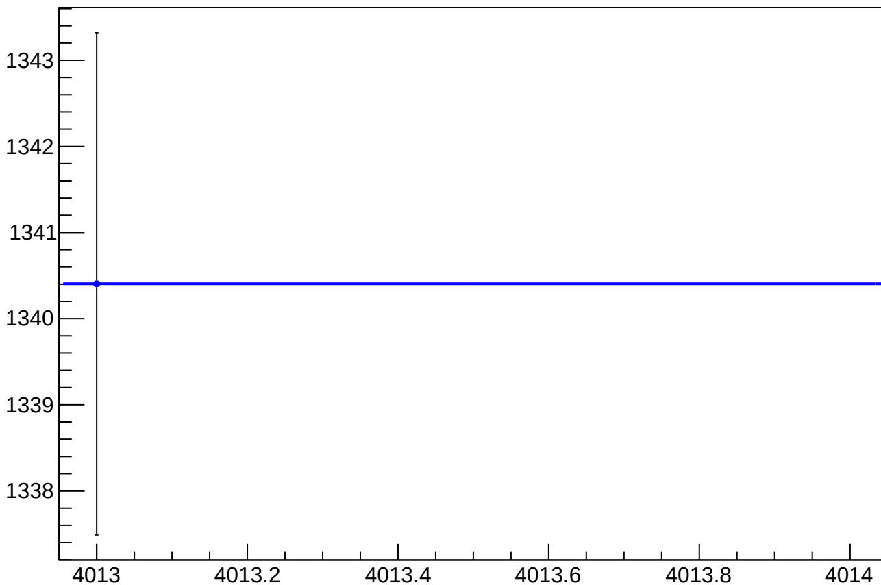
dit_asym_us_dd_at1lr_dd_dd_rms vs Slug, Sign Corrected
