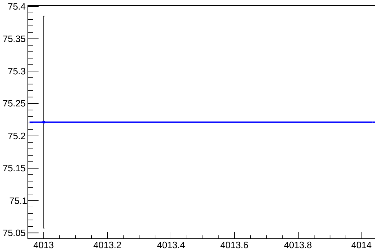
asym_sam_26_dd_dit_vs_slug, Sign Corrected
