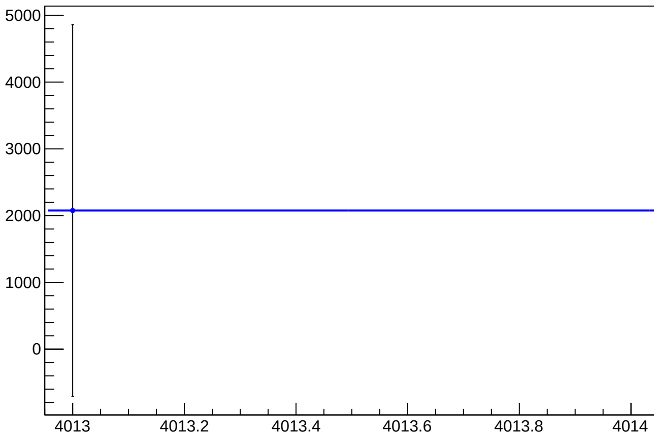
asym_usl_atl1_avg_cor_correction_mean vs Slug, Sign Corrected
