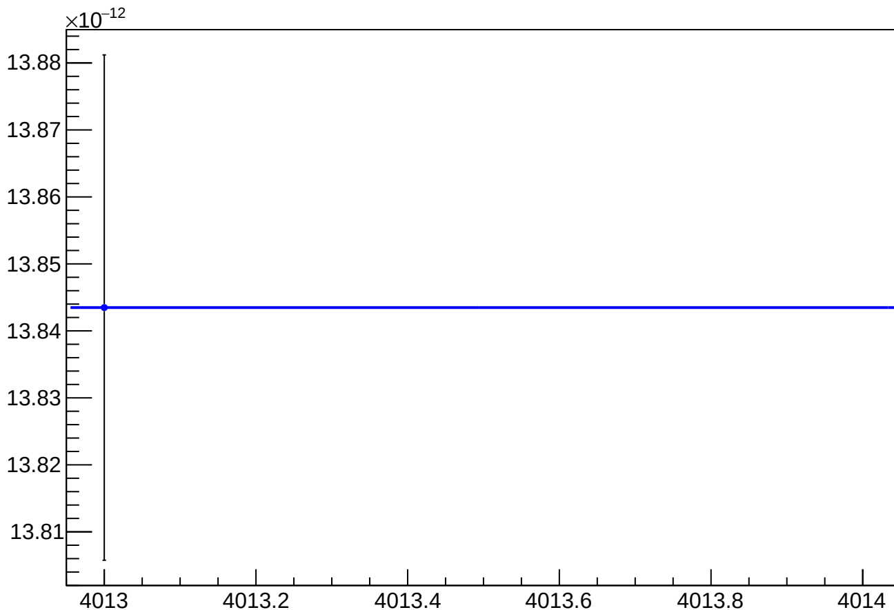
asym_atl_dd_atr_dd_dd_eigen_cor_vs_cor_diff_rms vs Slug, Sign Corrected
