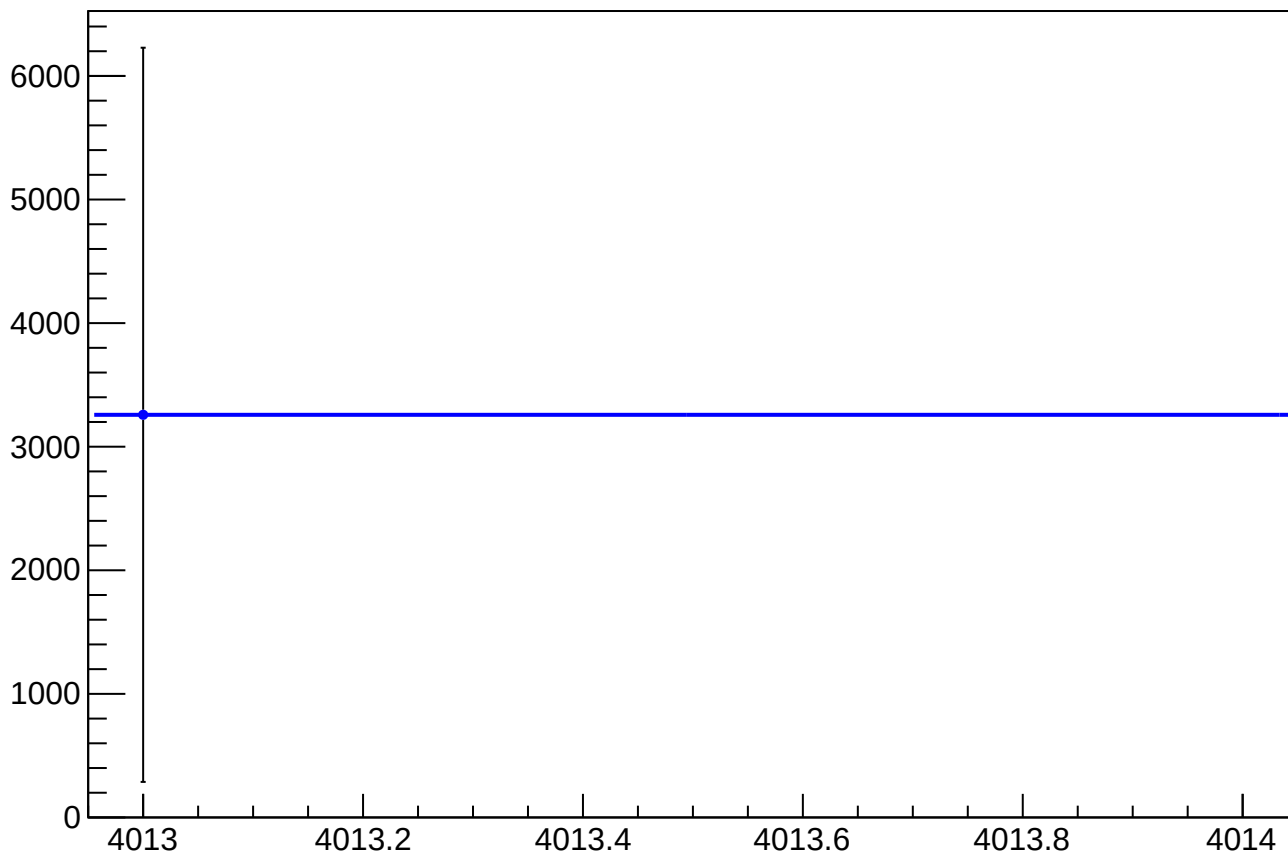
asym_sam6_cor_correction_mean vs Slug, Sign Corrected
