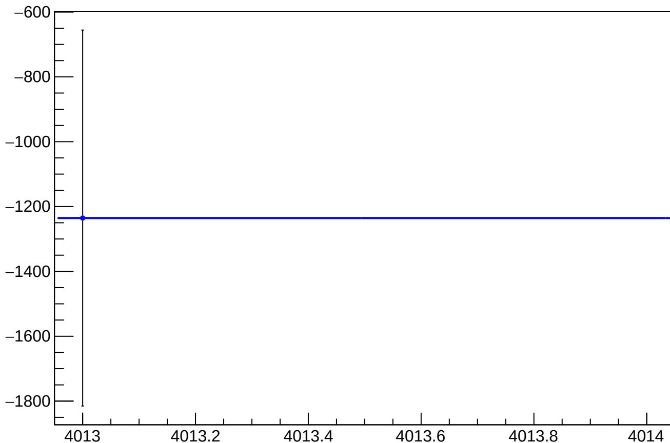
asym_bpm0l06WS_mean vs Slug, Sign Corrected
