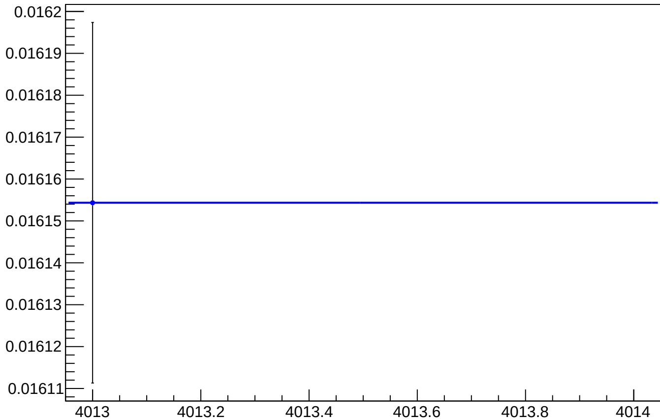
asym_sam_37_48_dd_reg_vs_cor_diff_rms vs Slug, Sign Corrected
