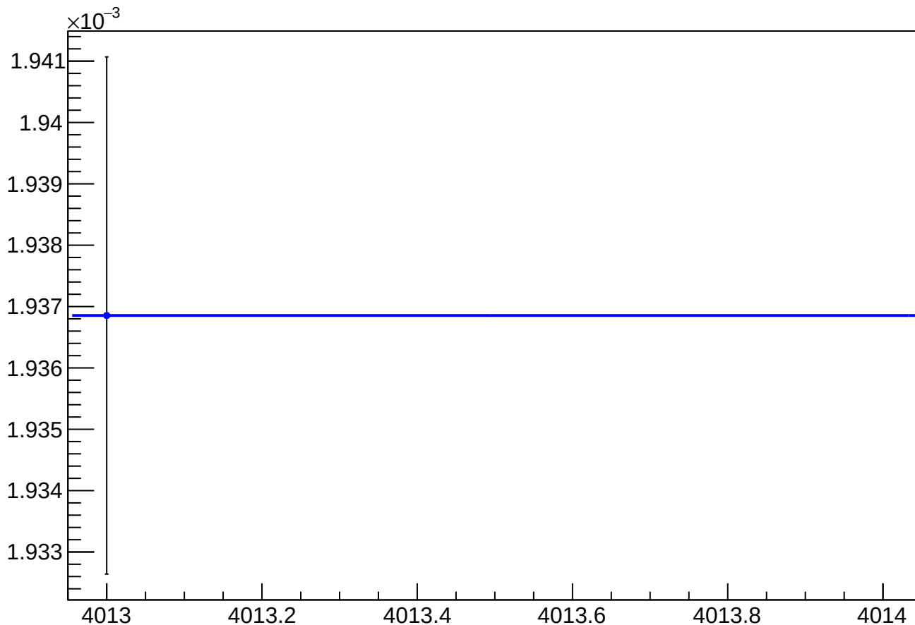
asym_sam_1357_avg_eigen_dit_vs_dit_diff_rms vs Slug, Sign Corrected
