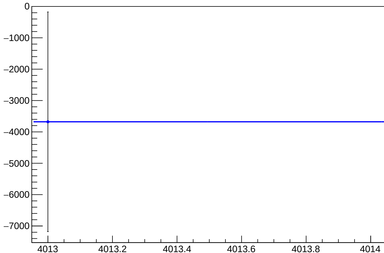
eigen_cor_asym_usl_atl1_avg_mean vs Slug, Sign Corrected
