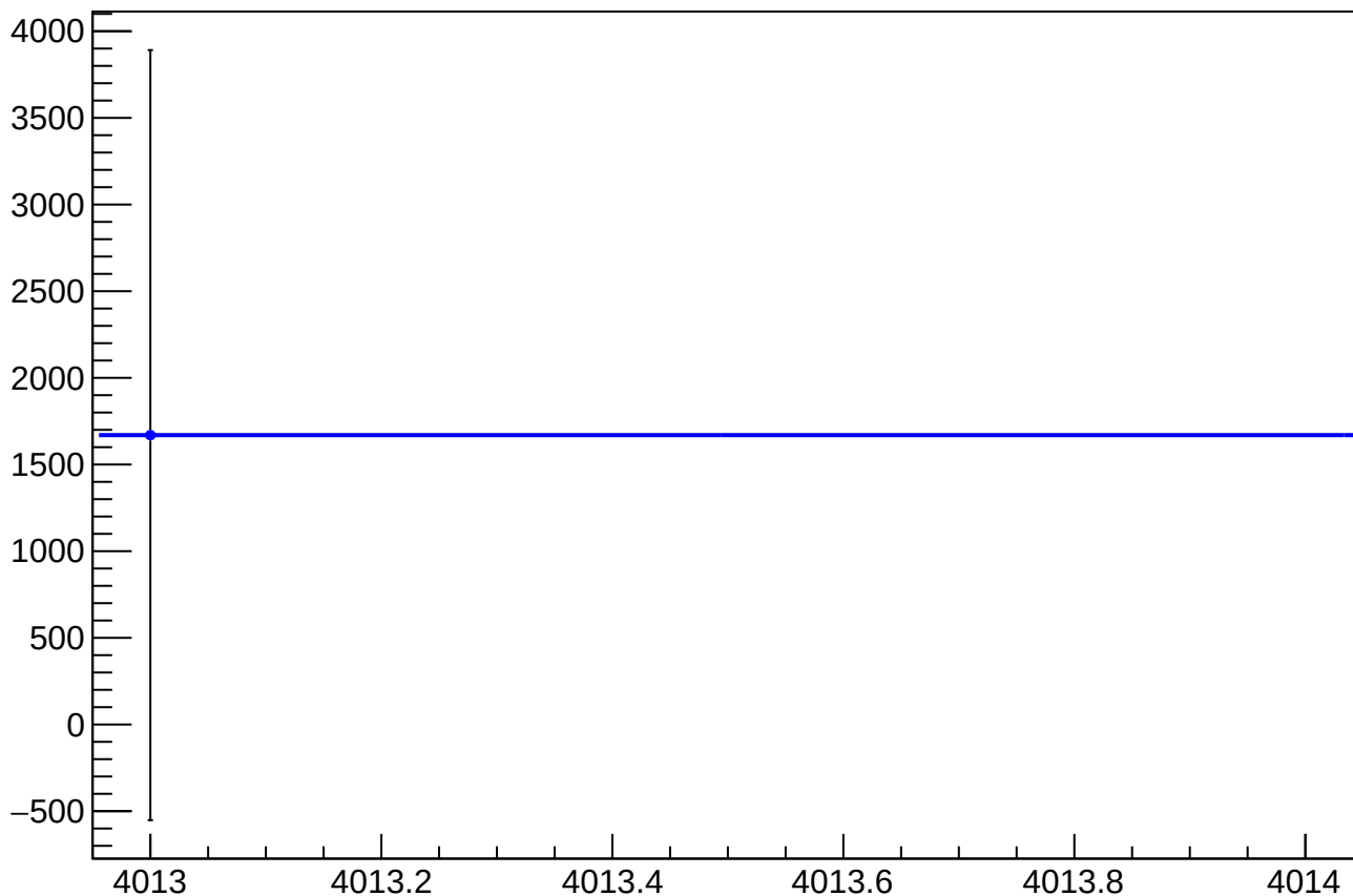
asym_at1_dd_eigen_dit_correction_mean vs Slug, Sign Corrected
