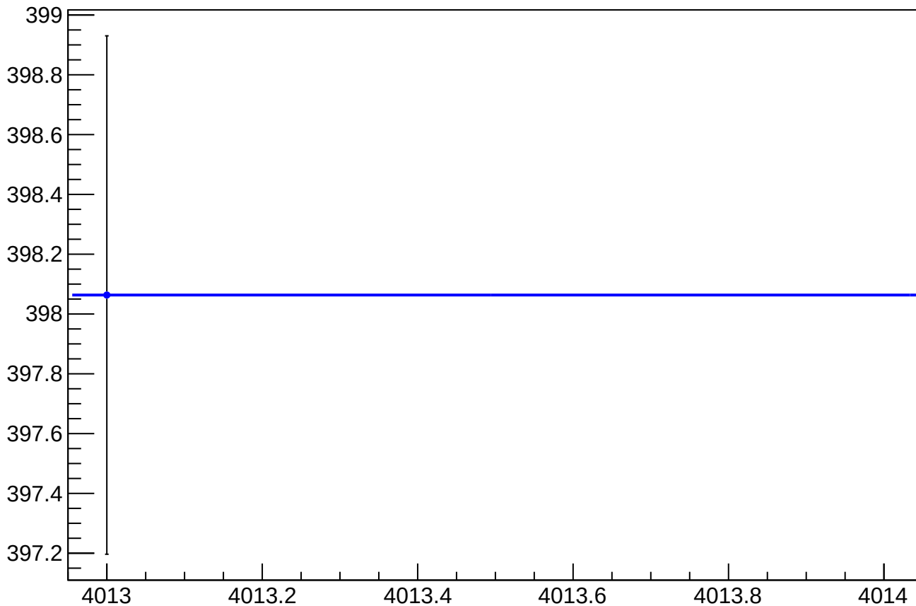
asym_sam_37_dd_dit_correction_rms vs Slug, Sign Corrected
