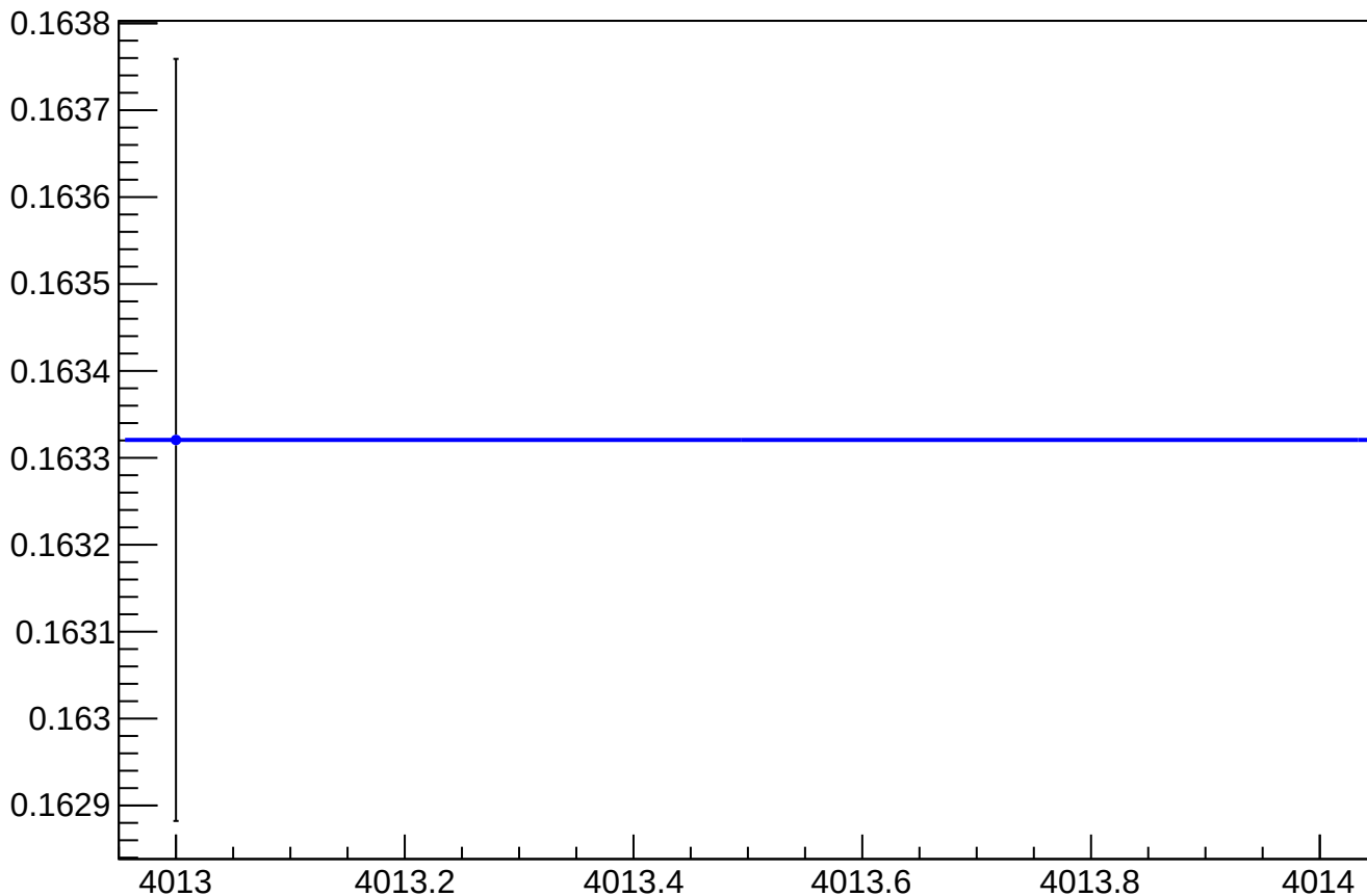
asym_atl_avg_atr_avg_avg_reg_vs_cor_diff_rms vs Slug, Sign Corrected
