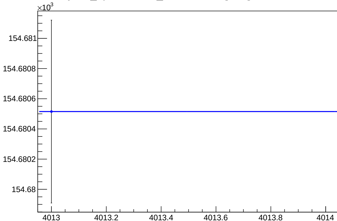
yield_bpm0i01WS_mean vs Slug, Sign Corrected
