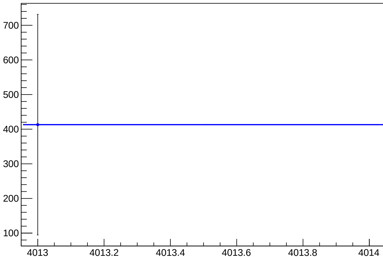
eigen_dit_asym_sam_37_48_dd_mean vs Slug, Sign Corrected
