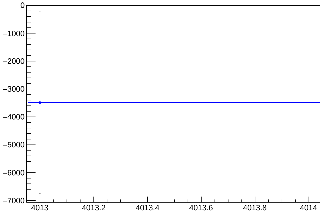
asym_sam_24_68_dd_eigen_cor_correction_mean vs Slug, Sign Corrected
