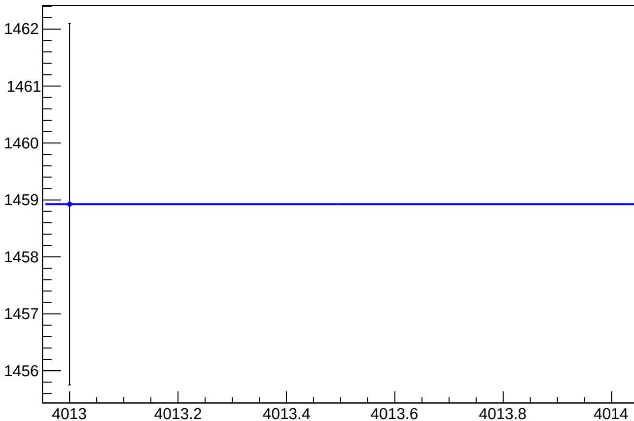
cor_asym_us_avg_at2lr_avg_dd_rms vs Slug, Sign Corrected
