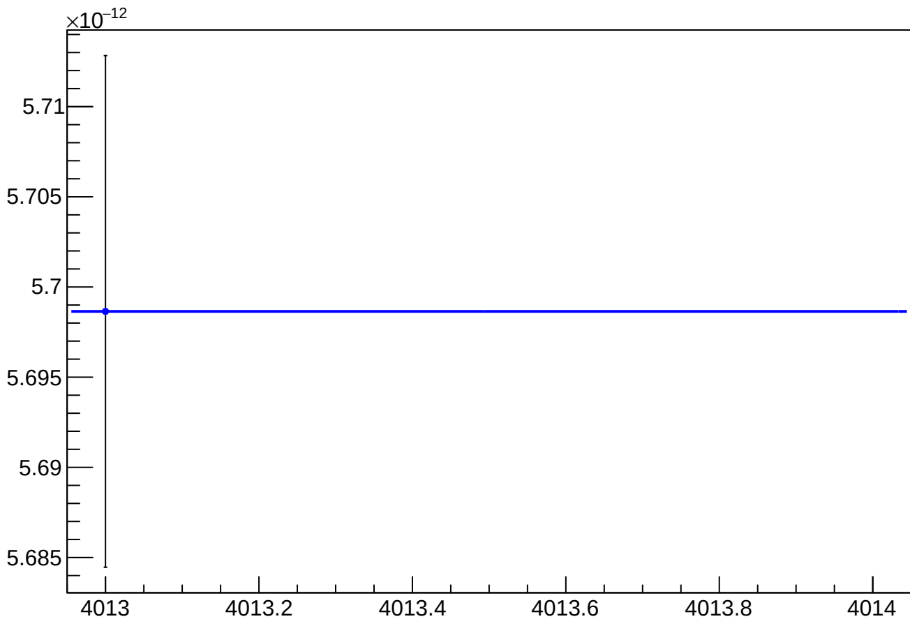
asym_sam_15_dd_eigen_cor_vs_cor_diff_rms vs Slug, Sign Corrected
