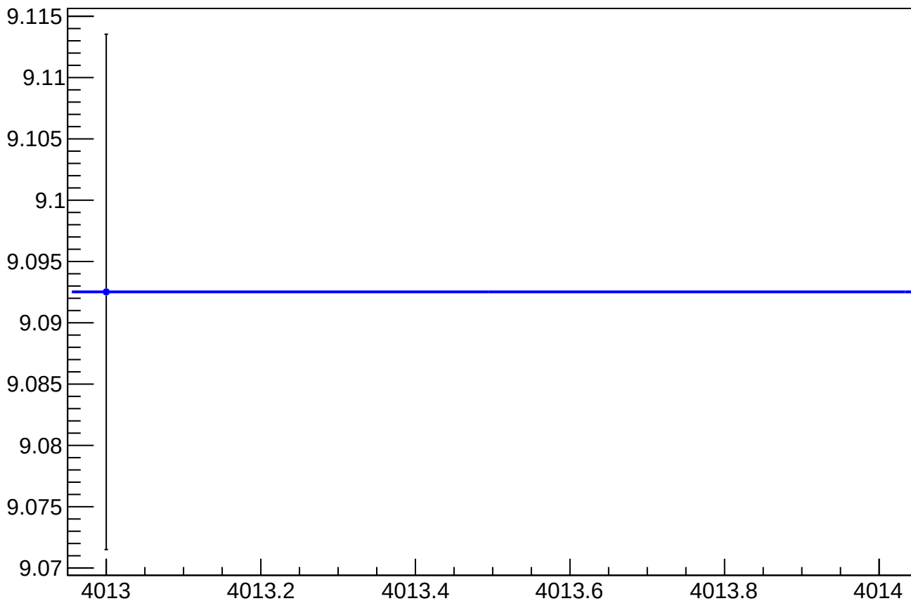
asym_sam1_dit_vs_cor_diff_rms vs Slug, Sign Corrected
