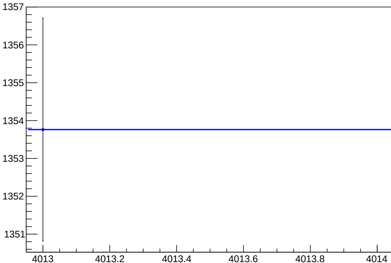
reg_asym_us_dd_at2lr_dd_dd_rms vs Slug, Sign Corrected
