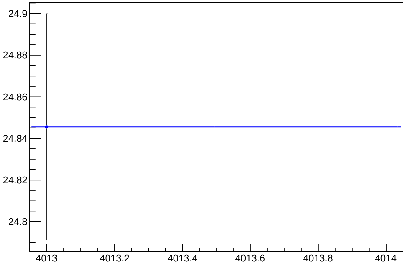
asym_sam_15_37_dd_eigen_dit_vs_cor_diff_rms vs Slug, Sign Corrected
