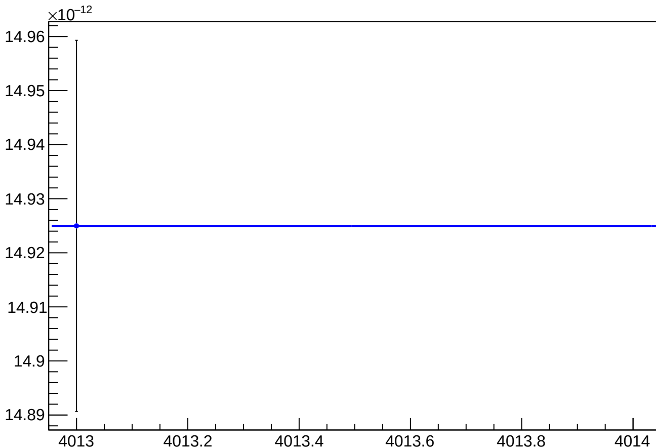
asym_sam8_eigen_cor_vs_cor_diff_rms vs Slug, Sign Corrected
