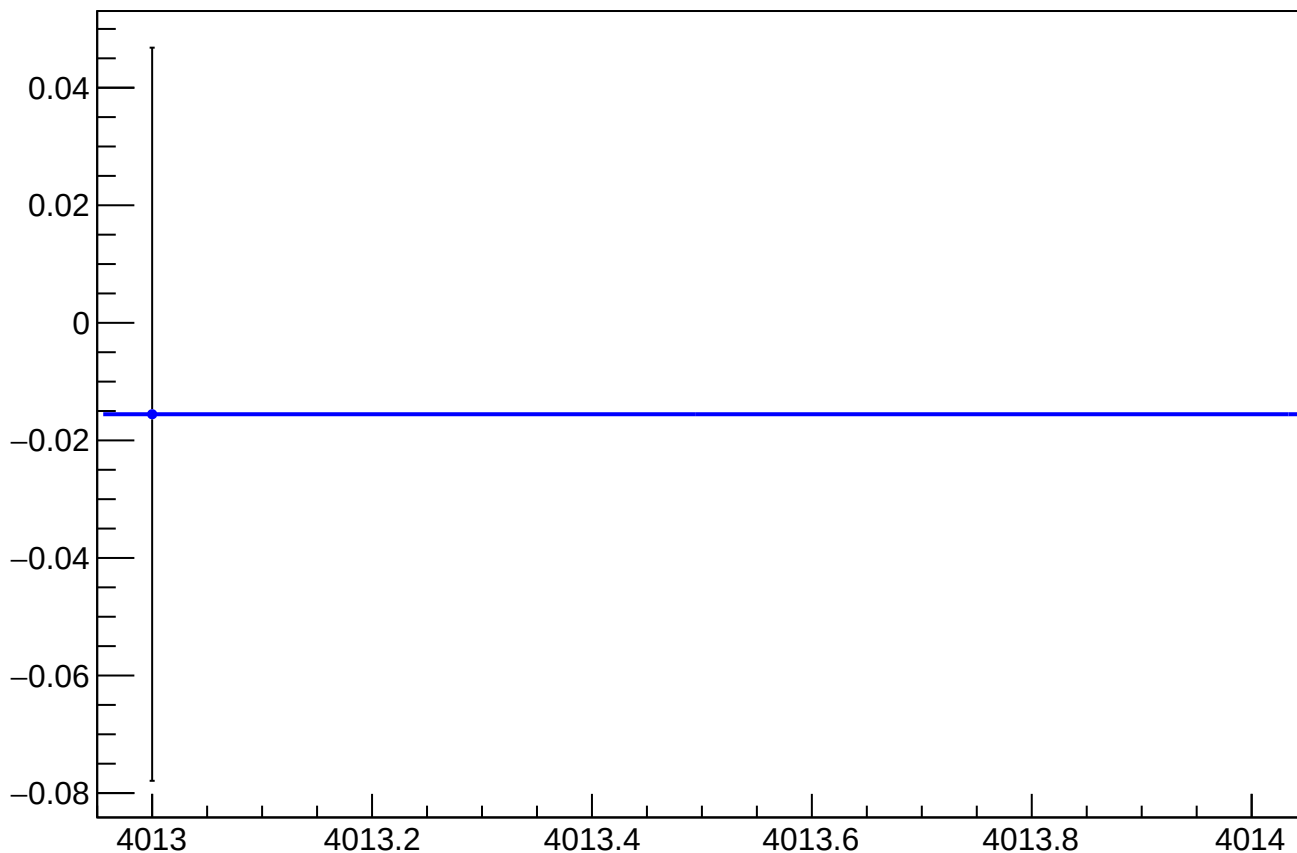
asym_atl1r2_dd_atl2r1_dd_avg_dit_vs_eigen_cor_diff_mean vs Slug, Sign Corrected
