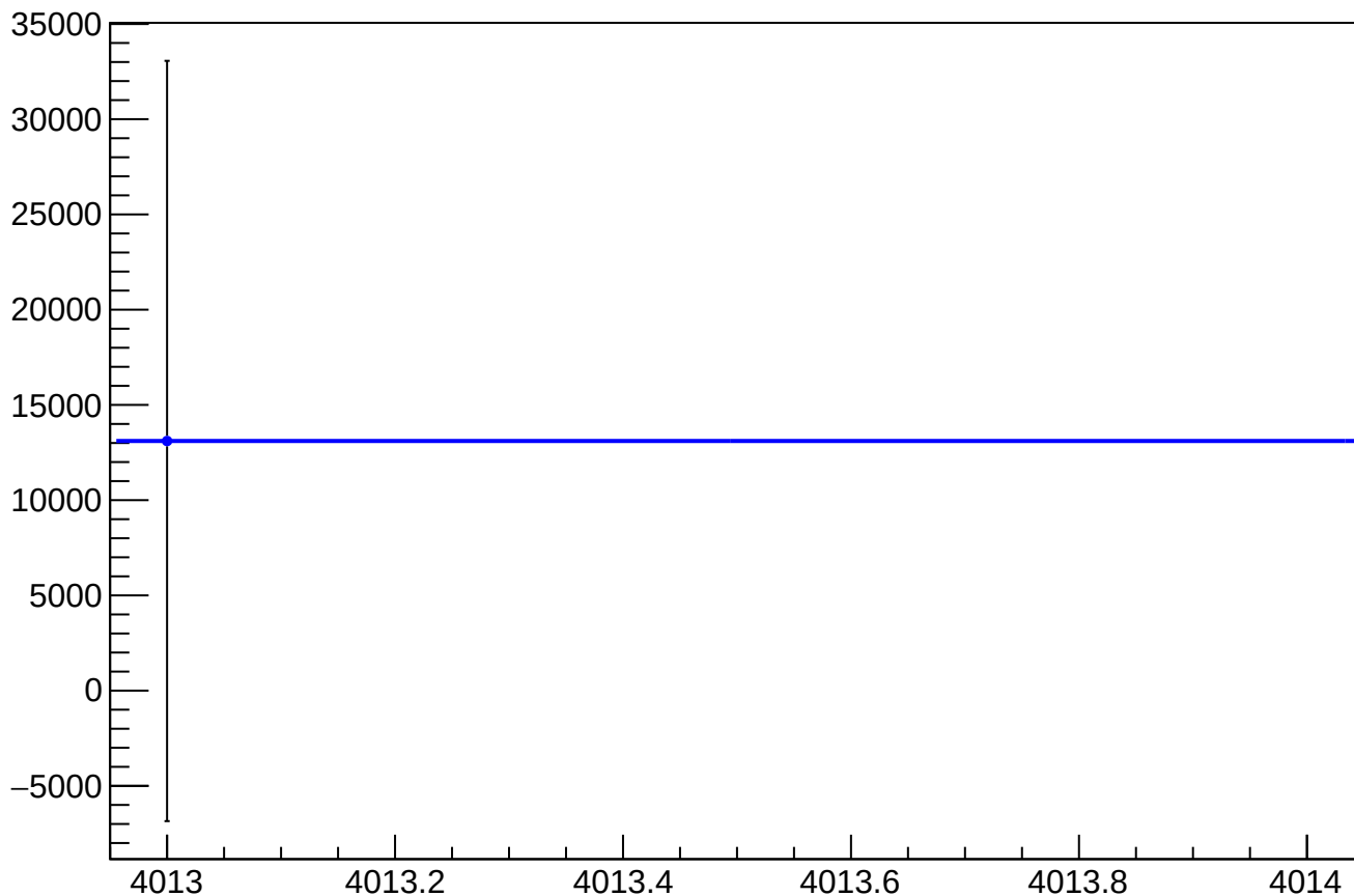
asym_atl_avg_atr_avg_avg_dit_correction_mean vs Slug, Sign Corrected
