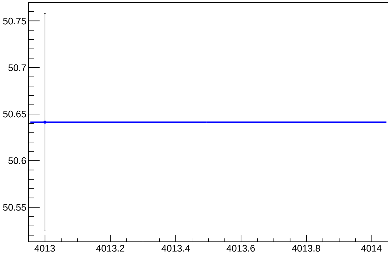
asym_sam_3748_avg_eigen_dit_vs_cor_diff_rms vs Slug, Sign Corrected
