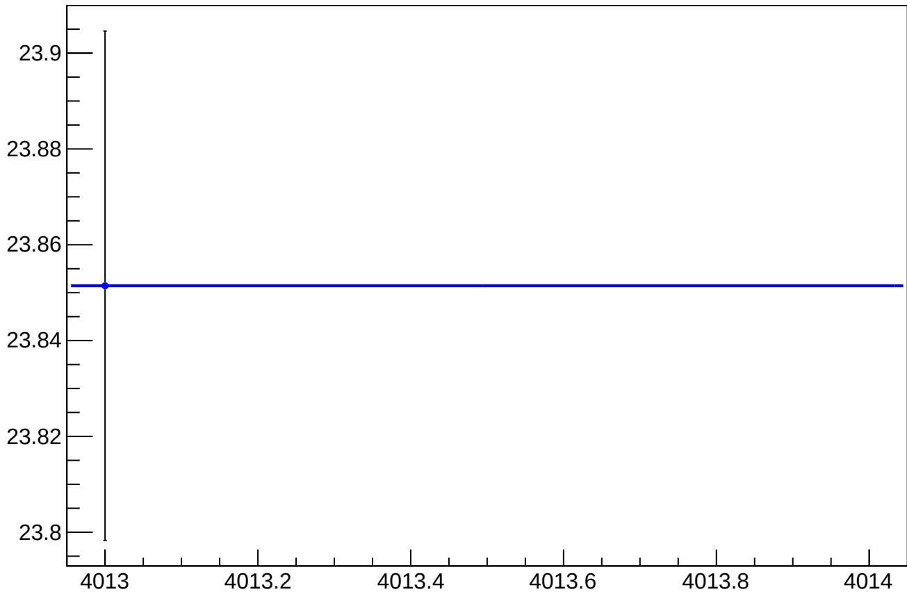
asym_sam_37_48_dd_eigen_dit_vs_cor_diff_rms vs Slug, Sign Corrected
