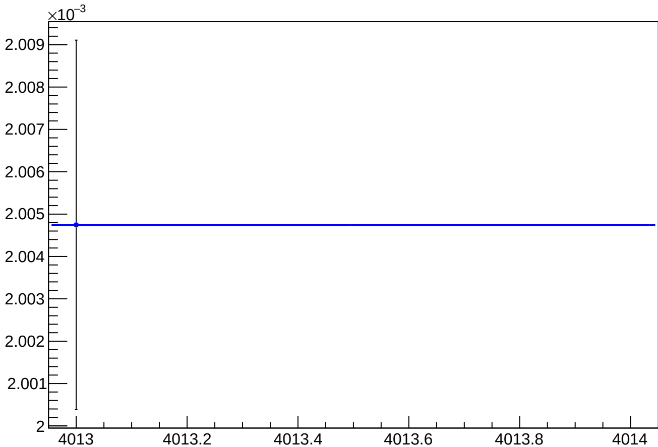
asym_sam_13_57_dd_eigen_dit_vs_dit_diff_rms vs Slug, Sign Corrected
