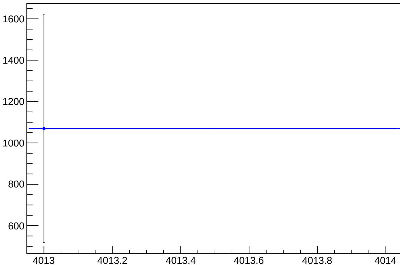
eigen_dit_asym_sam_26_48_dd_mean vs Slug, Sign Corrected
