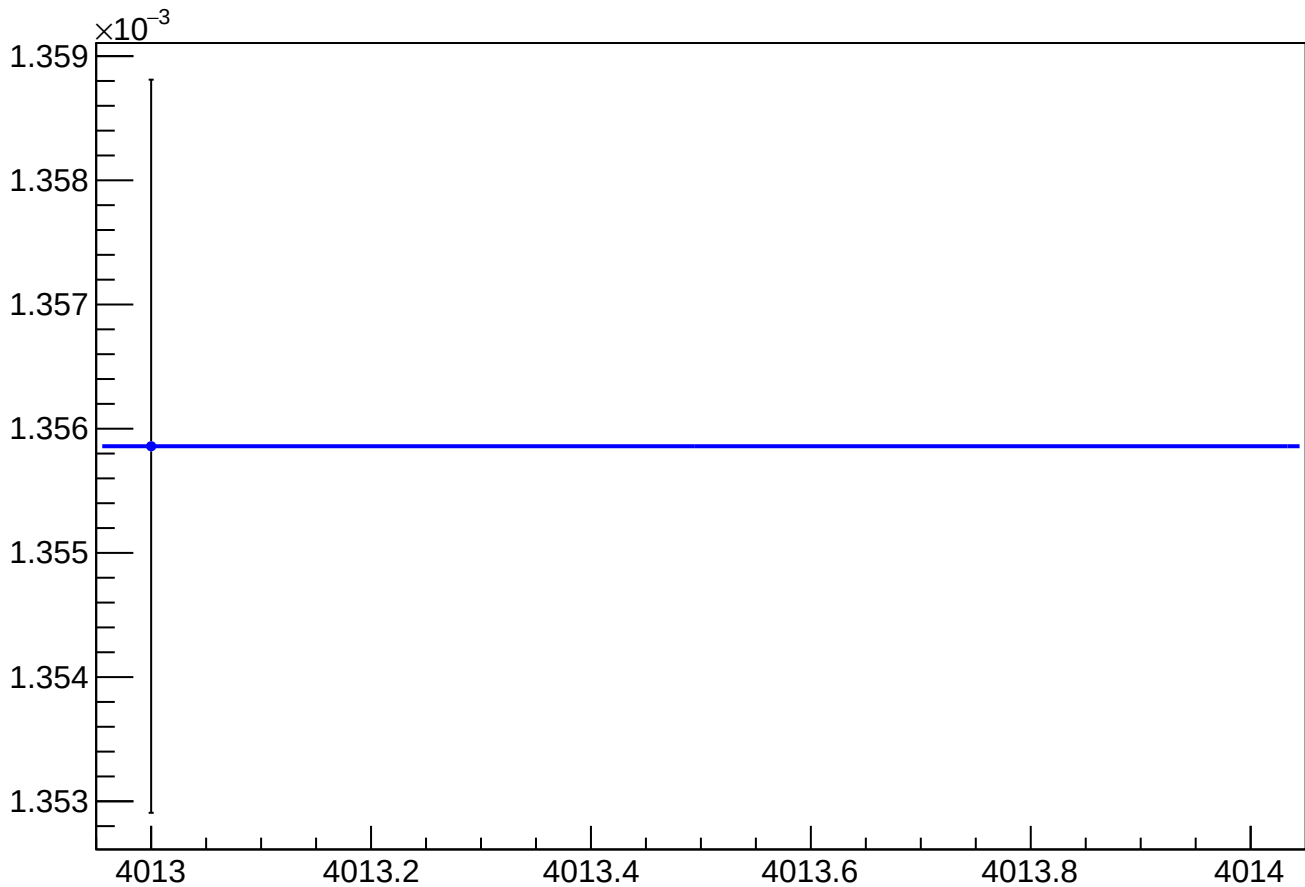
asym_sam_37_48_dd_eigen_dit_vs_dit_diff_rms vs Slug, Sign Corrected
