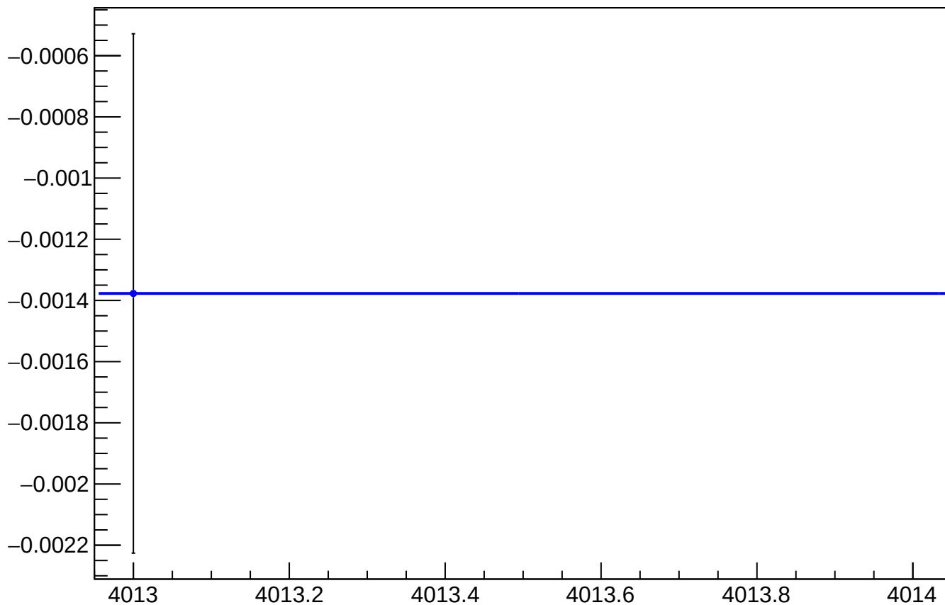
asym_us_dd_atlr_dd_avg_reg_vs_cor_diff_mean vs Slug, Sign Corrected
