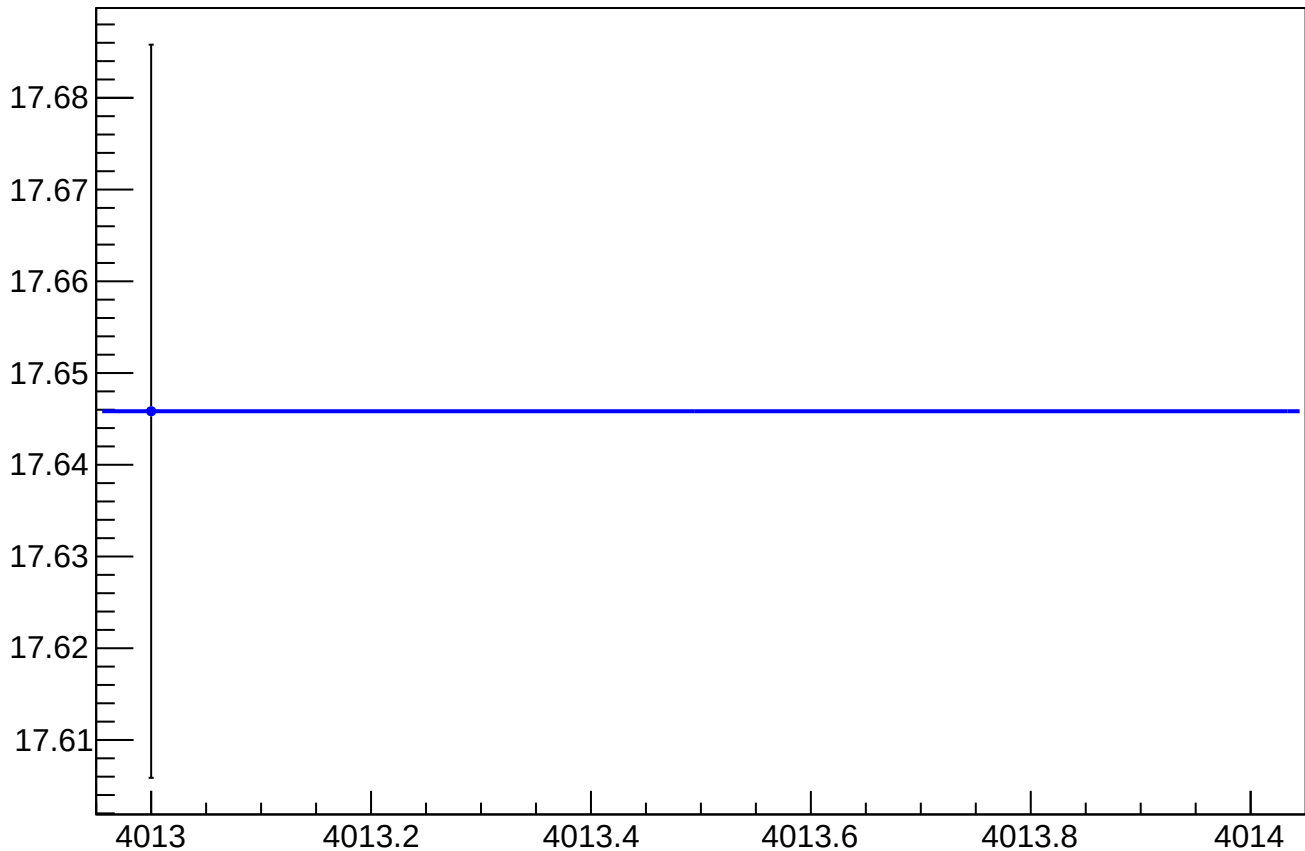
asym_sam_37_dd_dit_vs_eigen_cor_diff_rms vs Slug, Sign Corrected
