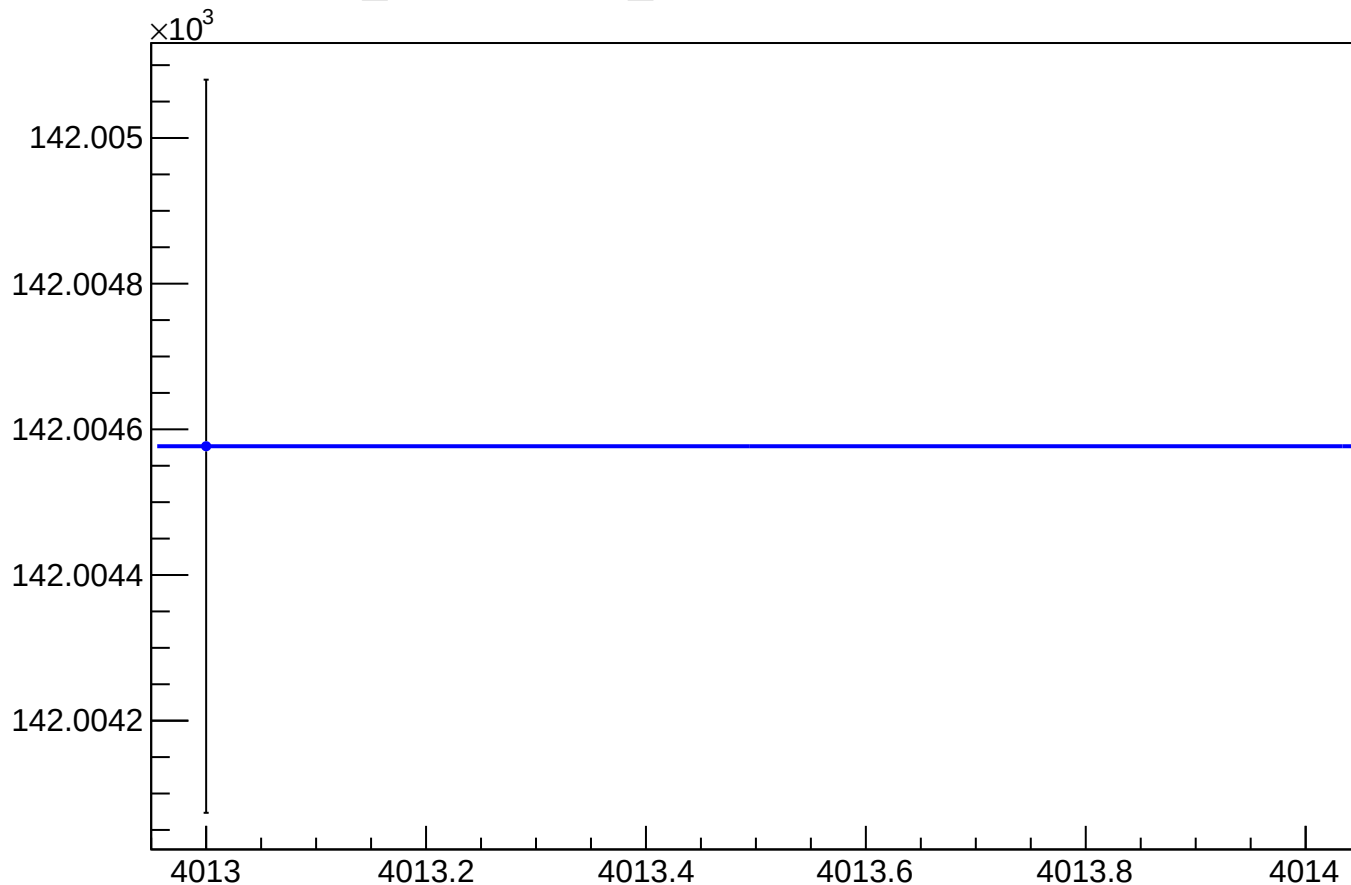
yield_bpm0i05WS_mean vs Slug, Sign Corrected
