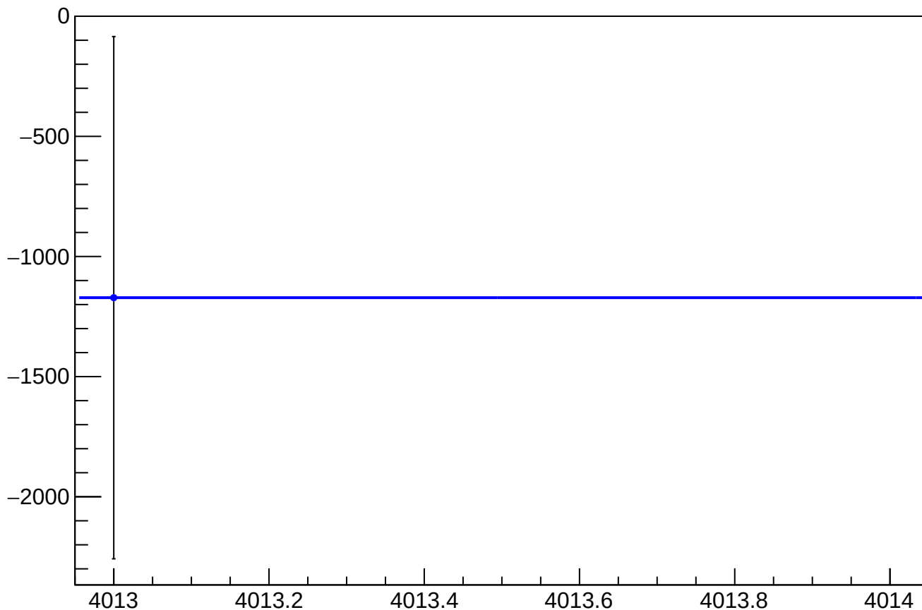
asym_us_dd_eigen_cor_correction_mean vs Slug, Sign Corrected
