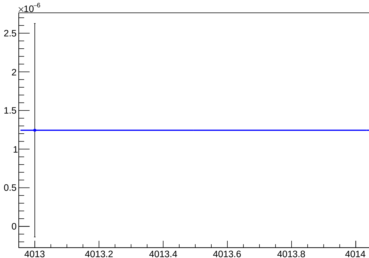
asym_sam_37_dd_eigen_dit_vs_dit_diff_mean vs Slug, Sign Corrected
