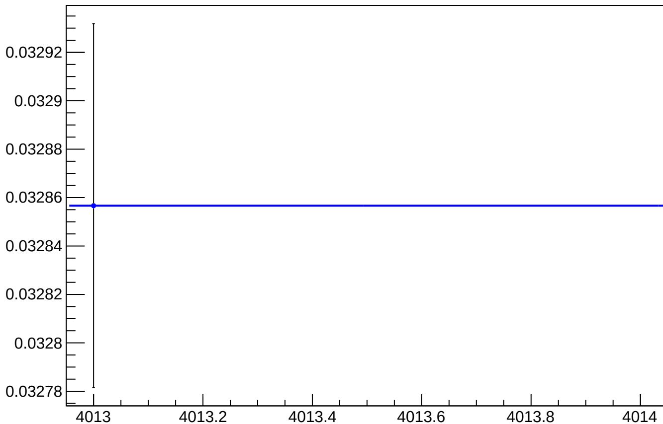
asym_sam_3748_avg_reg_vs_cor_diff_rms vs Slug, Sign Corrected
