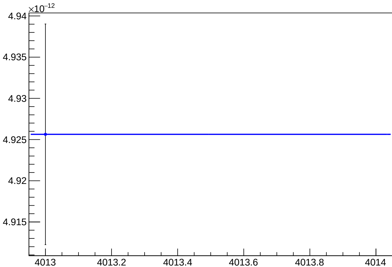
asym_us_dd_atlr_dd_dd_eigen_cor_vs_cor_diff_rms vs Slug, Sign Corrected
