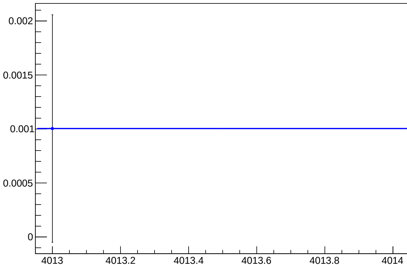
asym_us_avg_at2lr_avg_dd_reg_vs_cor_diff_mean vs Slug, Sign Corrected
