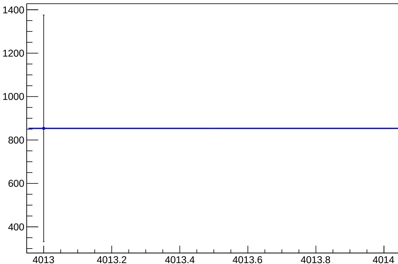
eigen_cor_asym_sam_3726_avg_mean vs Slug, Sign Corrected
