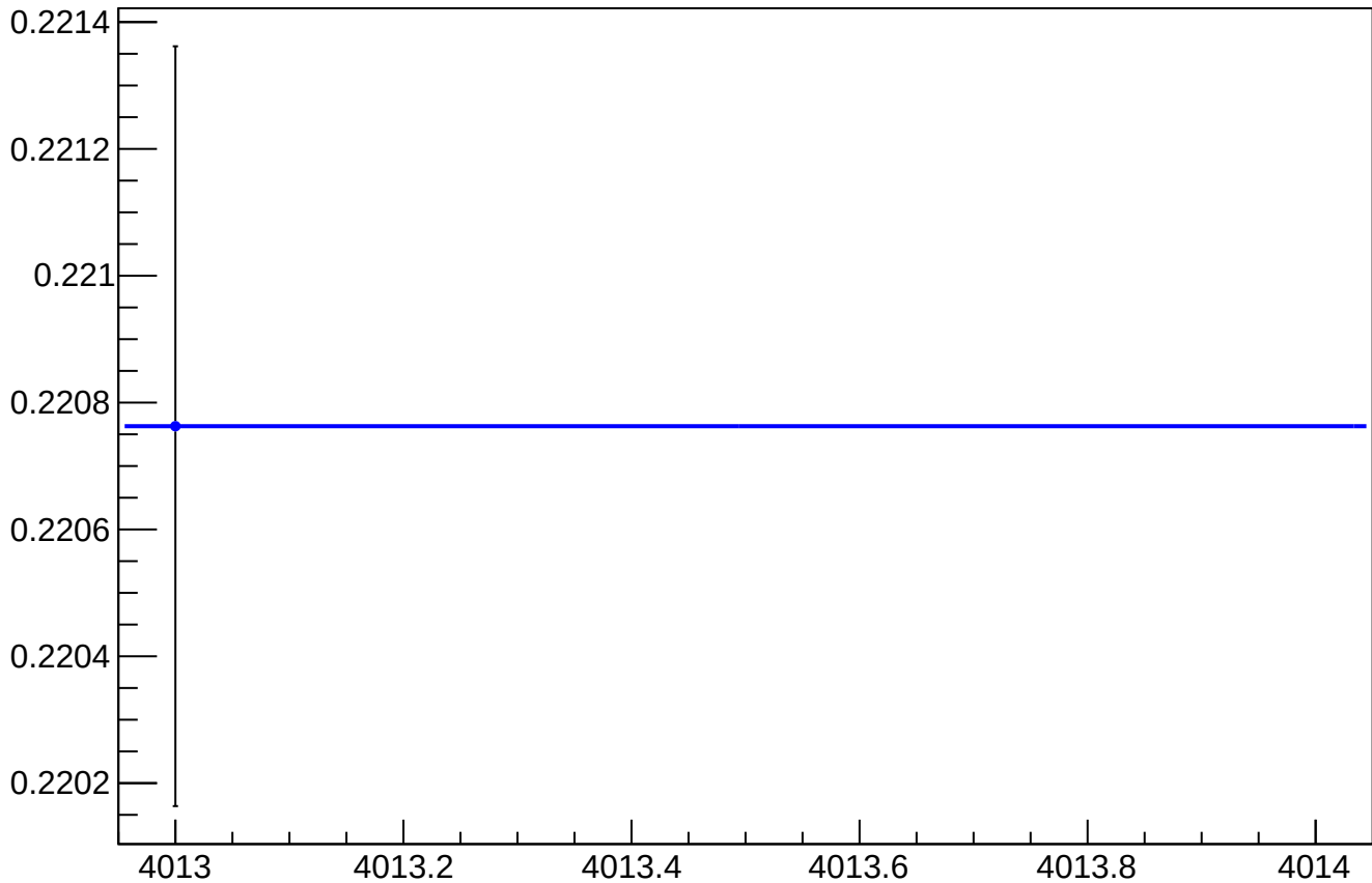
asym_at2_avg_reg_vs_cor_diff_rms vs Slug, Sign Corrected
