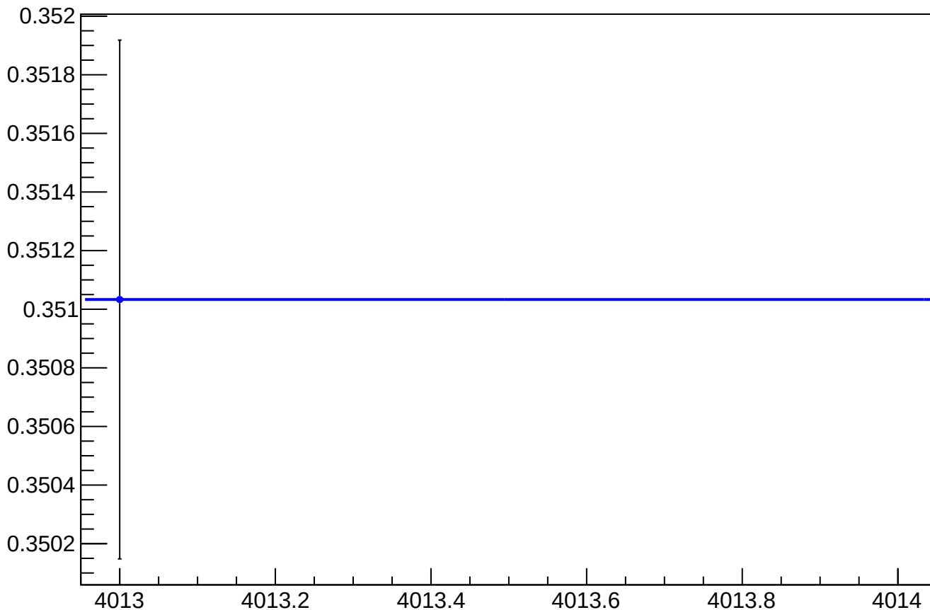
asym_atl_avg_reg_vs_cor_diff_rms vs Slug, Sign Corrected
