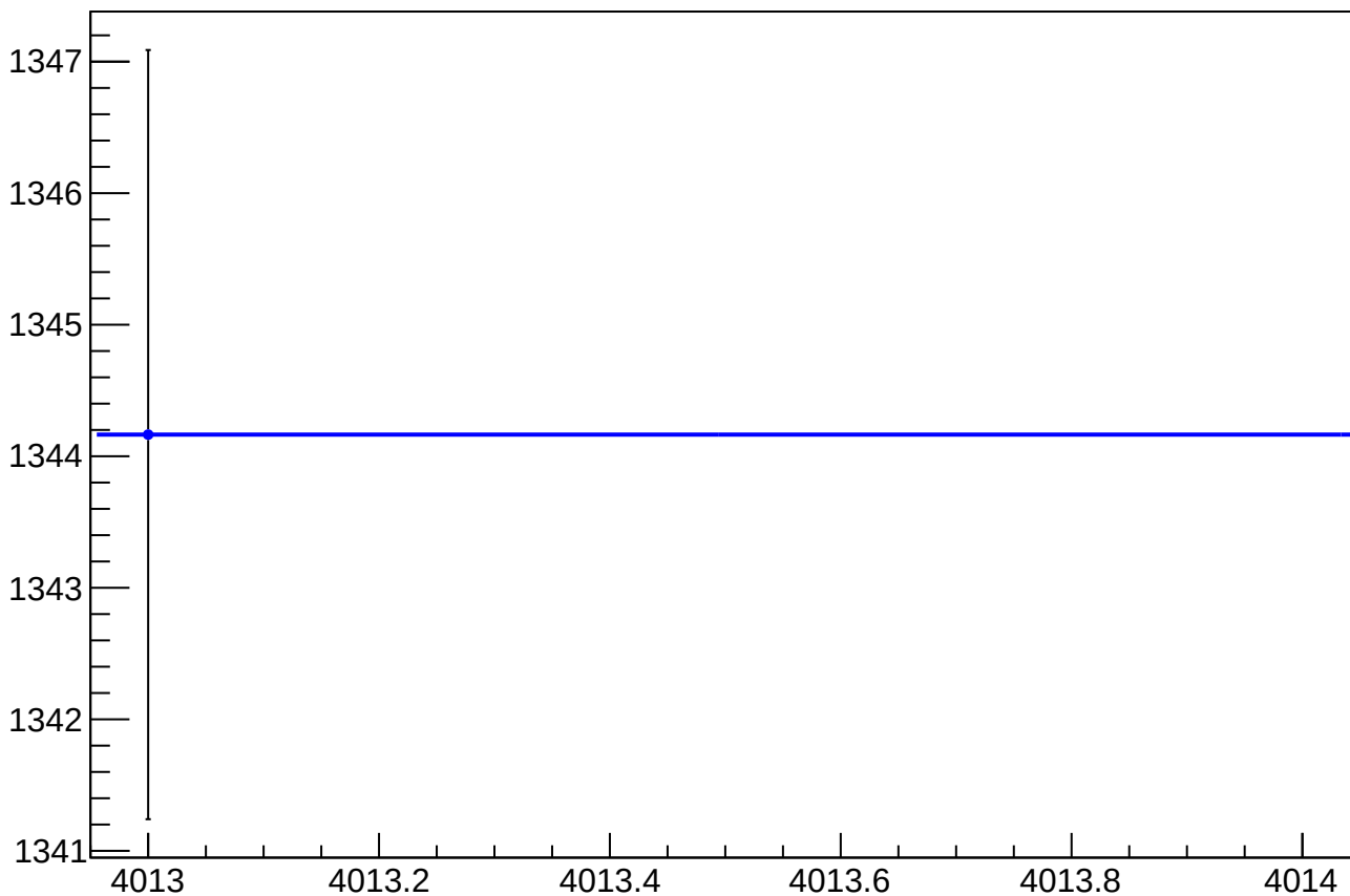
cor_asym_us_avg_at1lr_avg_dd_rms vs Slug, Sign Corrected
