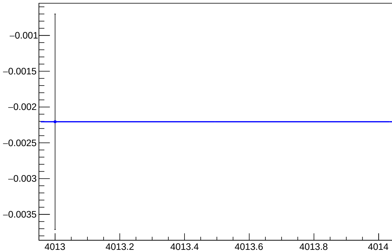
asym_atl2_reg_vs_cor_diff_mean vs Slug, Sign Corrected
