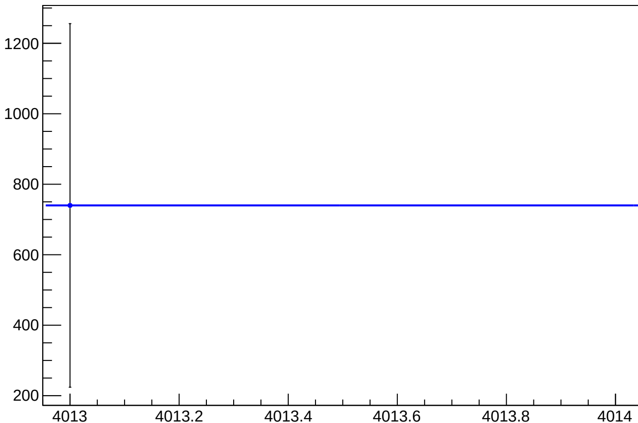
cor_asym_sam_1526_avg_mean vs Slug, Sign Corrected
