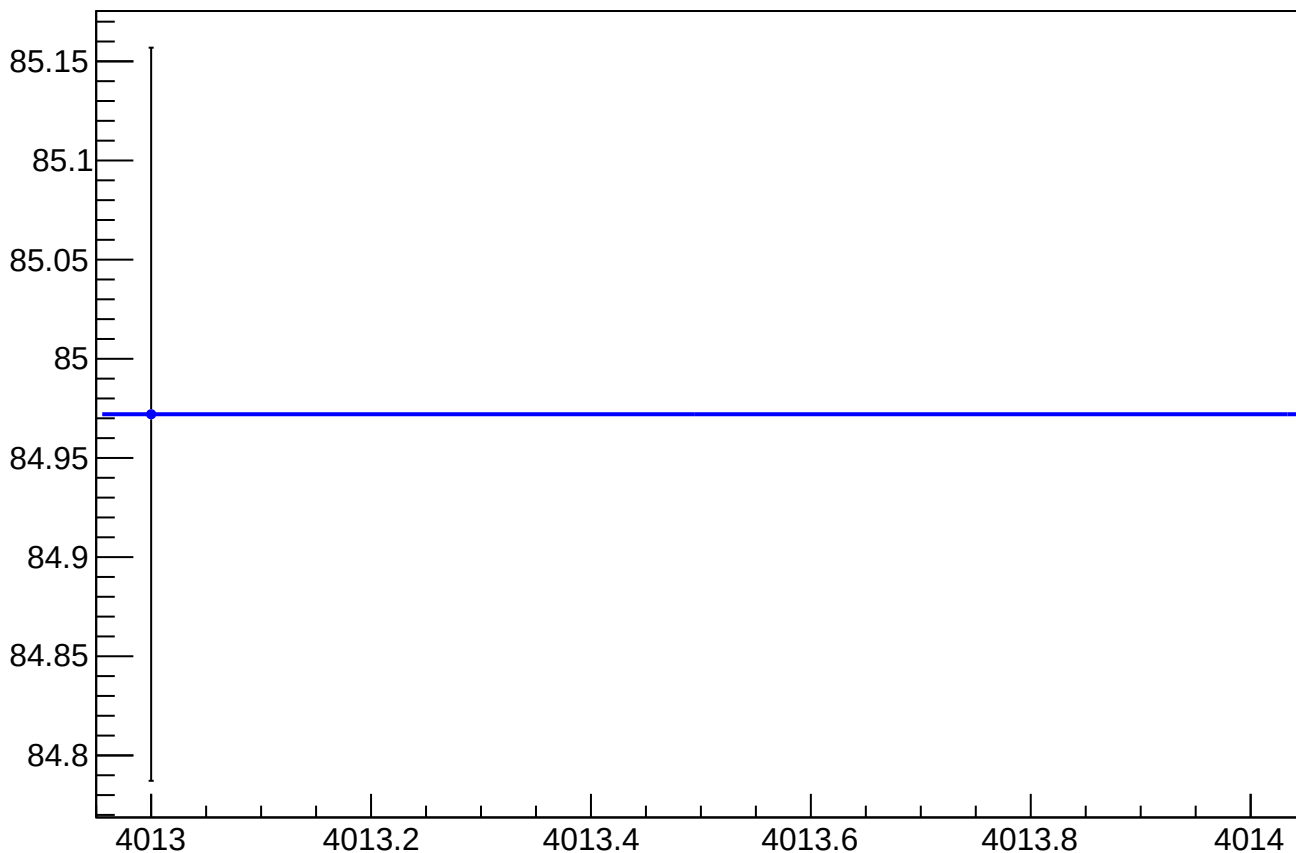
eigen_cor_asym_sam_1357_2468_dd_rms vs Slug, Sign Corrected
