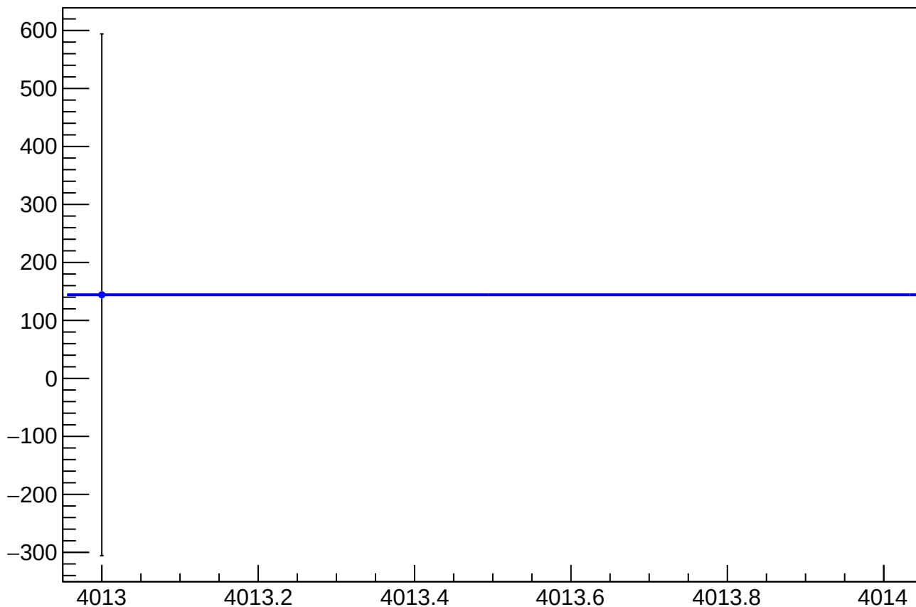
eigen_dit_asym_sam_37_avg_mean vs Slug, Sign Corrected
