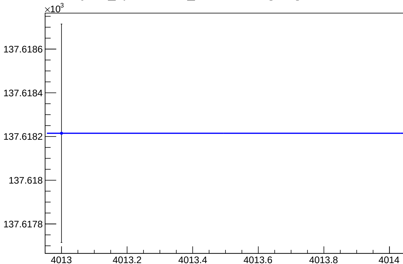
yield_bpm0i02WS_mean vs Slug, Sign Corrected
