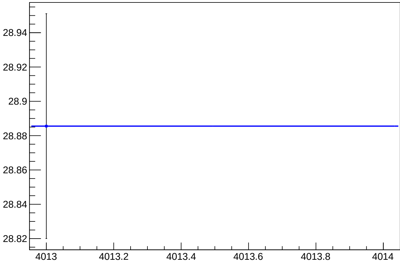
asym_us_dd_at2lr_dd_dd_dit_vs_cor_diff_rms vs Slug, Sign Corrected
