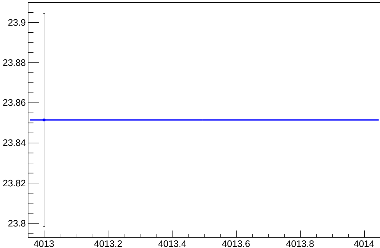
asym_sam_37_48_dd_eigen_dit_vs_eigen_cor_diff_rms vs Slug, Sign Corrected
