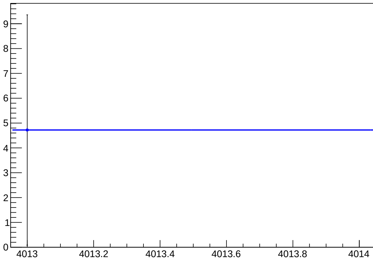
reg_asym_us_dd_at2lr_dd_avg_diff_bpm4eY_slope vs Slug, Sign Corrected
