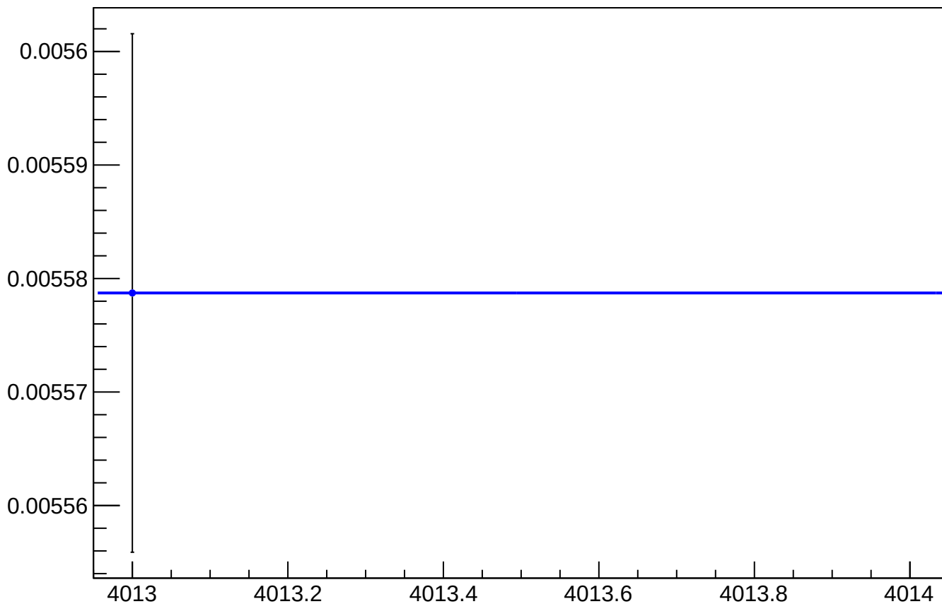
asym_sam1_reg_vs_cor_diff_rms vs Slug, Sign Corrected
