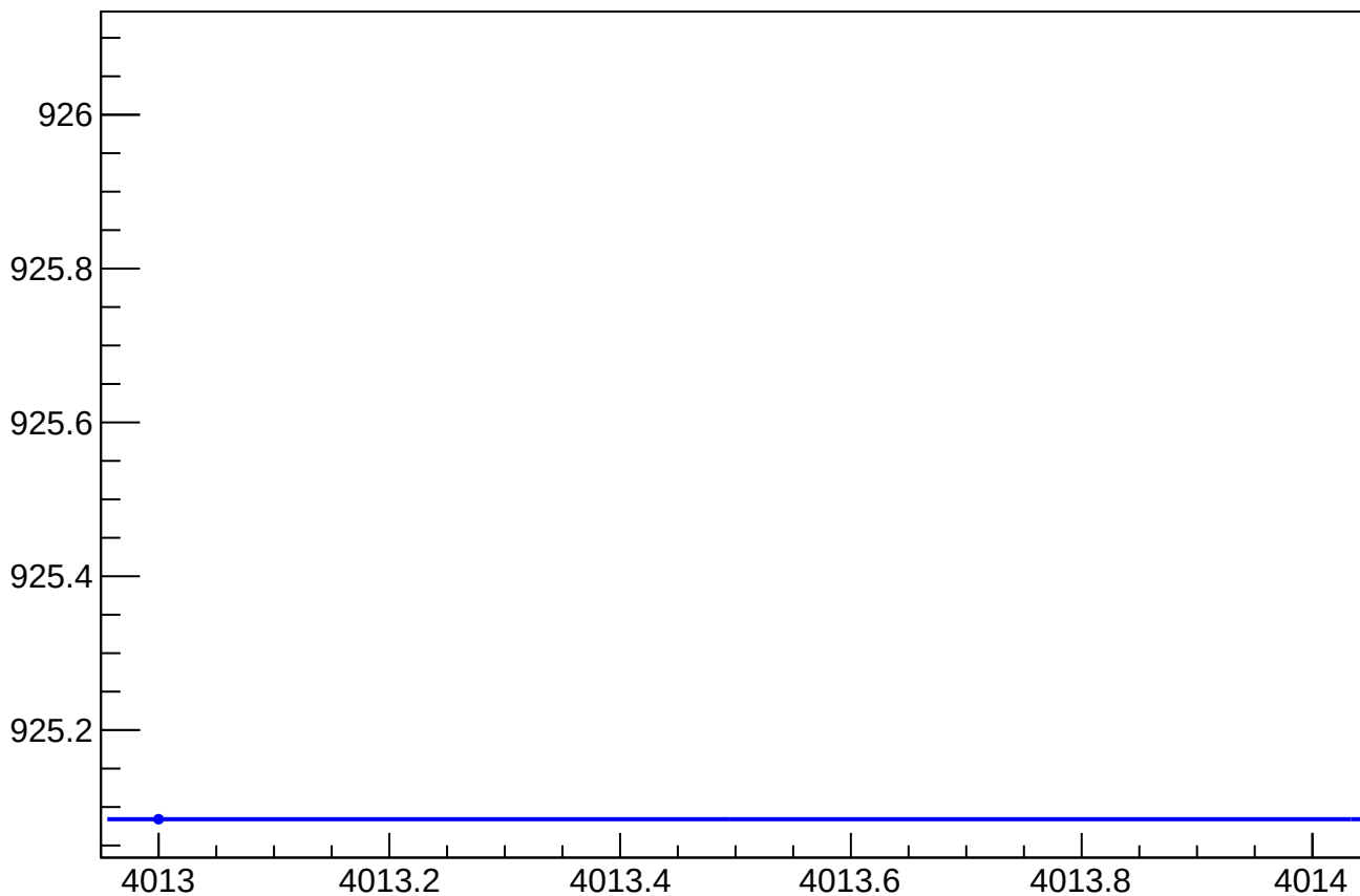
HacR_Q2_HP3458A_IOUT_mean vs Slug, Sign Corrected
