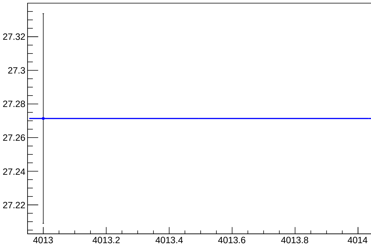
asym_sam8_eigen_dit_vs_cor_diff_rms vs Slug, Sign Corrected
