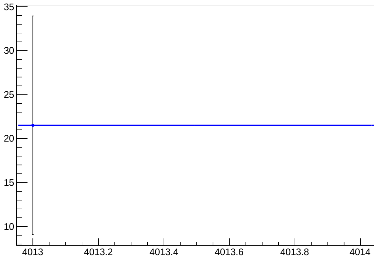
reg_asym_usl_atl2_dd_diff_bpm4aY_slope vs Slug, Sign Corrected
