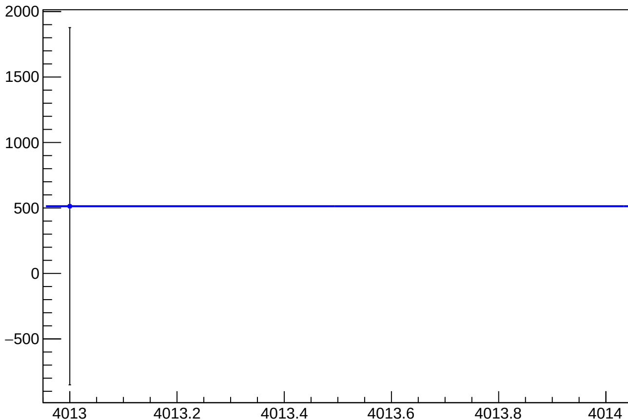
asym_us_dd_at1lr_dd_avg_dit_correction_mean vs Slug, Sign Corrected
