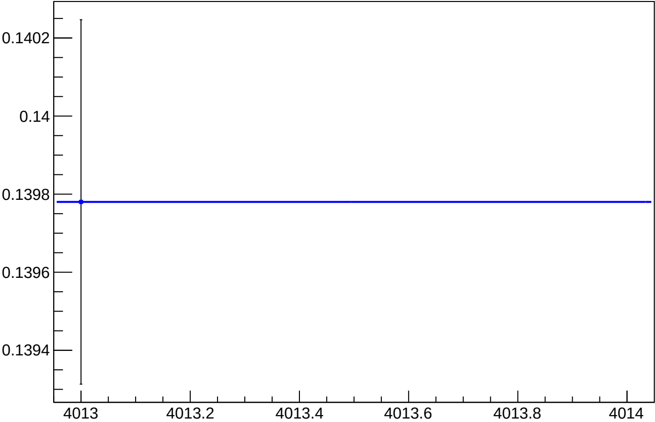
asym_us_dd_at1lr_dd_avg_reg_vs_cor_diff_rms vs Slug, Sign Corrected
