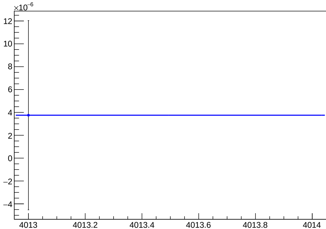
asym_sam3_eigen_dit_vs_dit_diff_mean vs Slug, Sign Corrected
