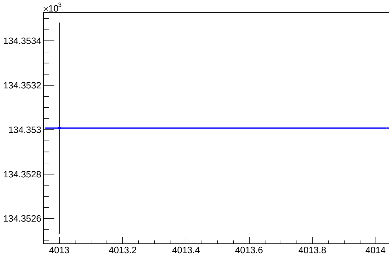
yield_bpm0l06WS_mean vs Slug, Sign Corrected
