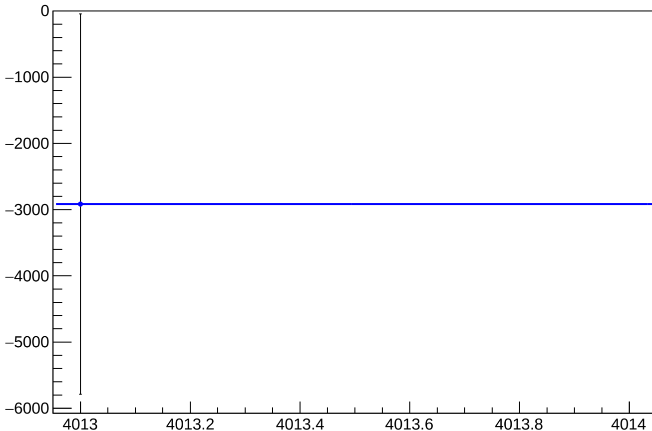
cor_asym_us_avg_atlr_avg_dd_mean vs Slug, Sign Corrected
