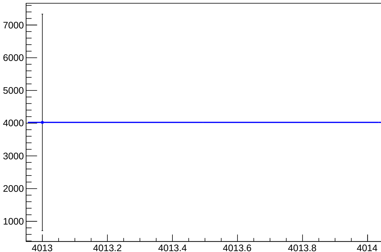
dit_asym_at1_avg_at2_avg_dd_mean vs Slug, Sign Corrected
