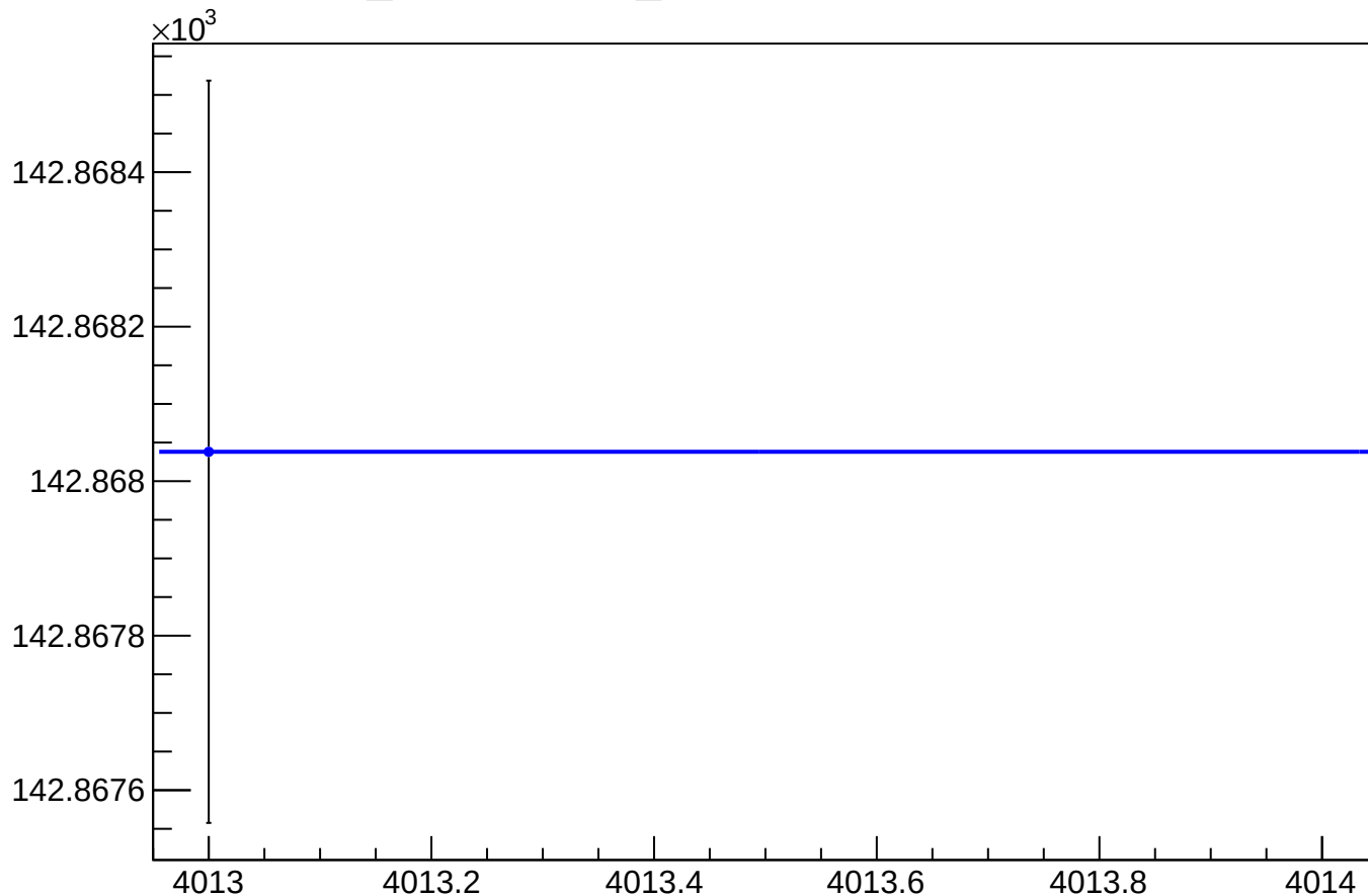
yield_bpm0l07WS_mean vs Slug, Sign Corrected
