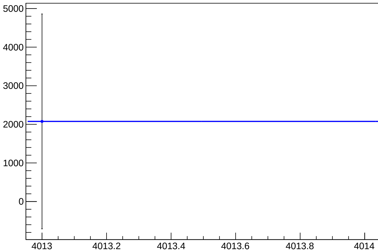
asym_usl_atl1_avg_eigen_cor_correction_mean vs Slug, Sign Corrected
