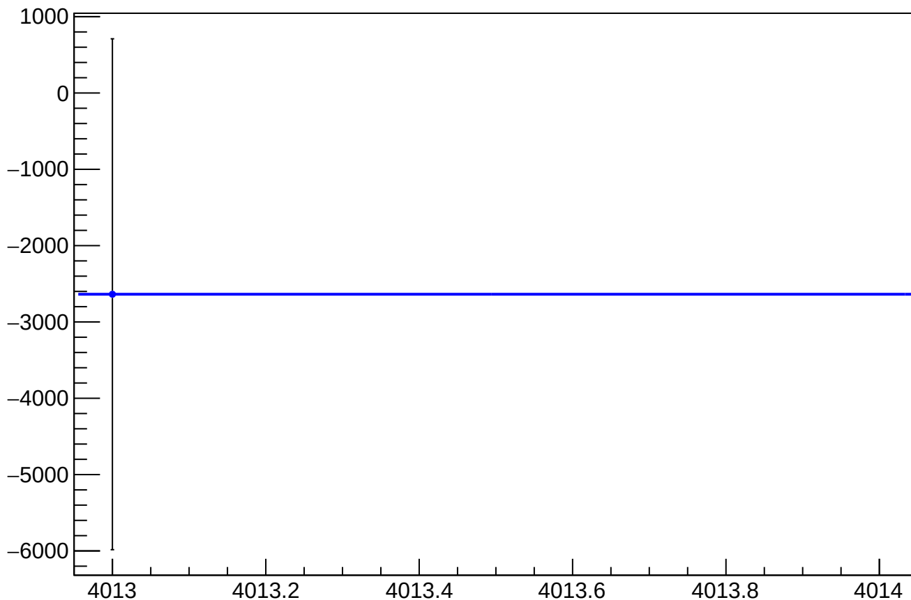
asym_sam3_eigen_dit_correction_mean vs Slug, Sign Corrected
