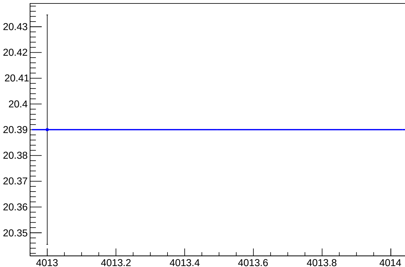
asym_sam_15_dd_dit_vs_cor_diff_rms vs Slug, Sign Corrected
