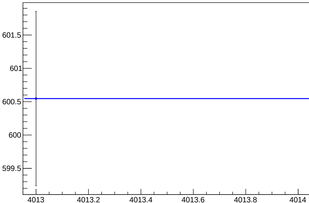
asym_sam_15_48_dd_cor_correction_rms vs Slug, Sign Corrected
