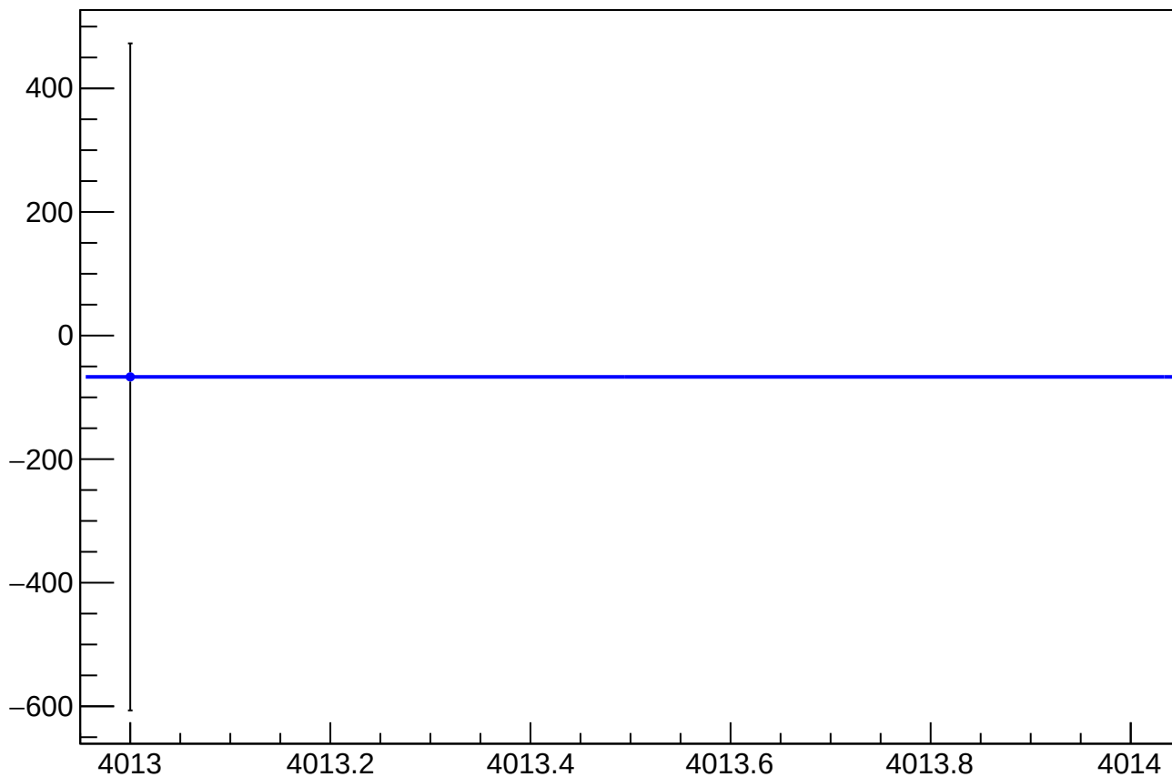
asym_sam1_reg_correction_mean vs Slug, Sign Corrected
