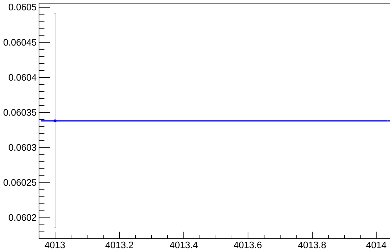
asym_sam_26_dd_reg_vs_cor_diff_rms vs Slug, Sign Corrected
