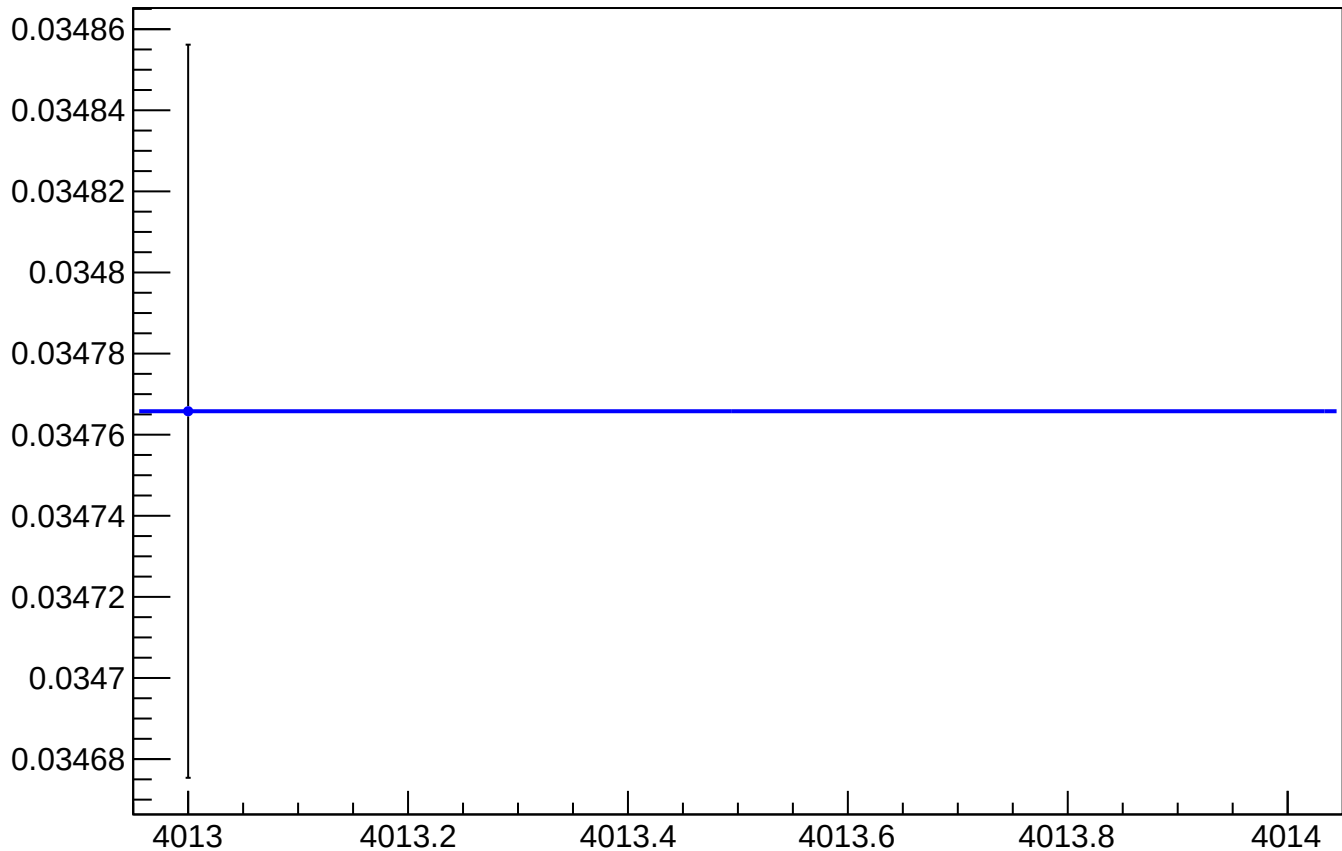
asym_sam7_reg_vs_cor_diff_rms vs Slug, Sign Corrected
