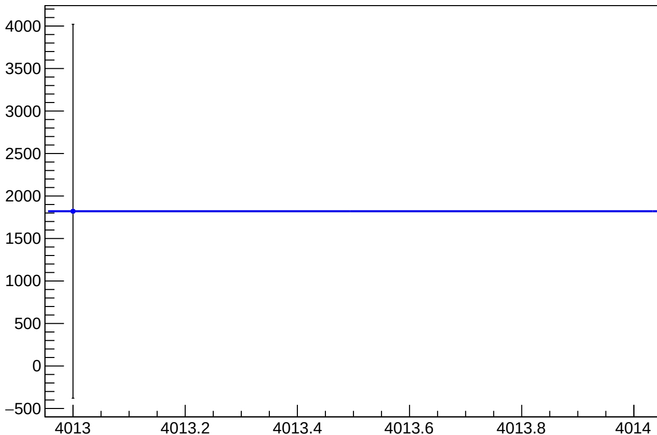
asym_at1_dd_reg_correction_mean vs Slug, Sign Corrected
