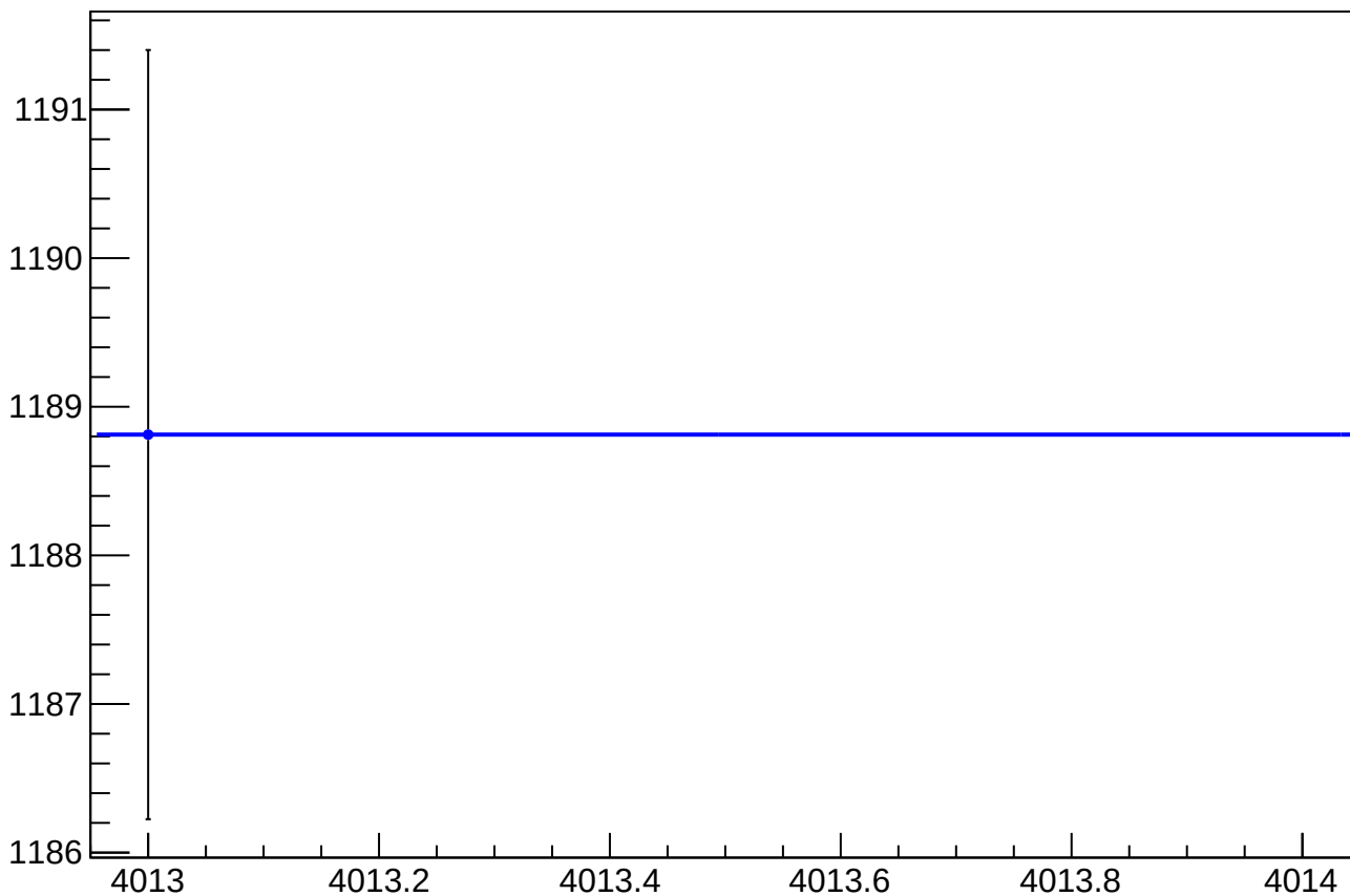
asym_usr_atr1_avg_cor_correction_rms vs Slug, Sign Corrected
