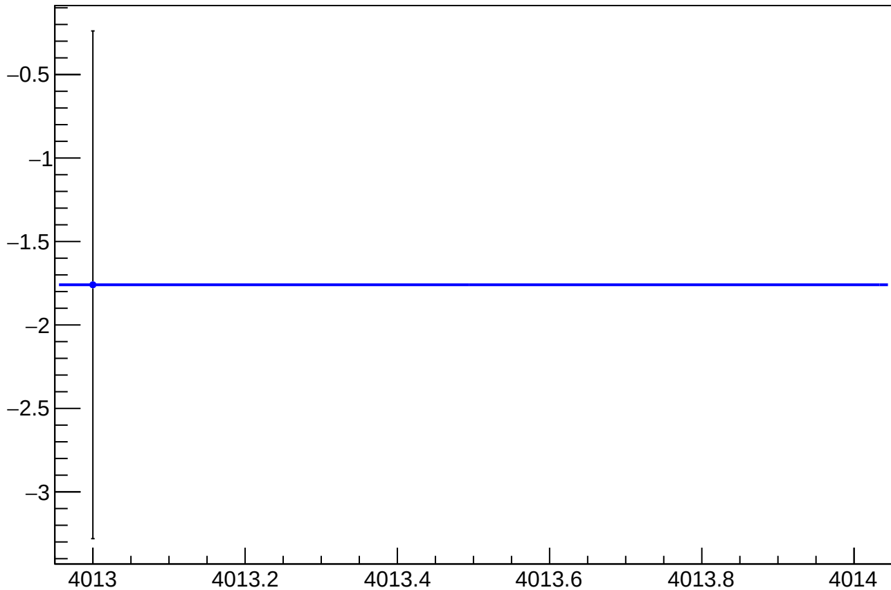
asym_atr2_eigen_dit_vs_eigen_cor_diff_mean vs Slug, Sign Corrected
