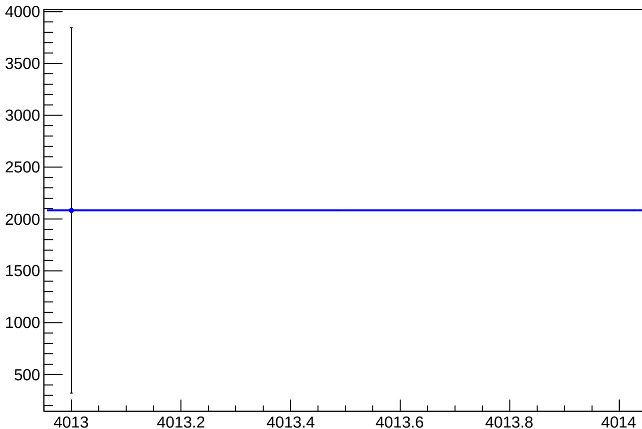
asym_usr_atr1_dd_eigen_cor_correction_mean vs Slug, Sign Corrected
