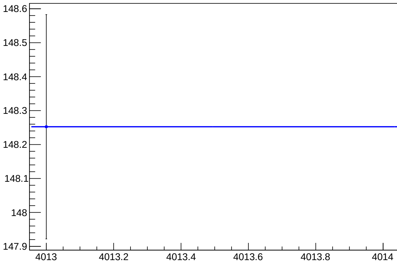
asym_atr1_eigen_dit_vs_eigen_cor_diff_rms vs Slug, Sign Corrected
