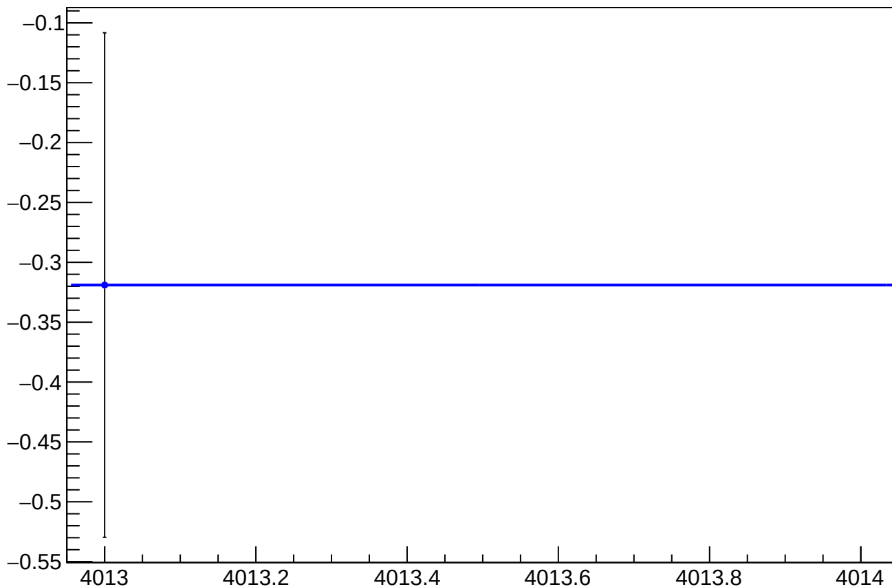
asym_us_avg_at1lr_avg_dd_dit_vs_eigen_cor_diff_mean vs Slug, Sign Corrected
