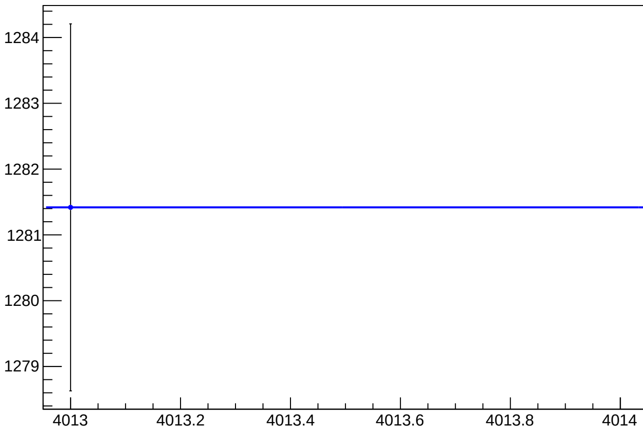
asym_usr_reg_correction_rms vs Slug, Sign Corrected
