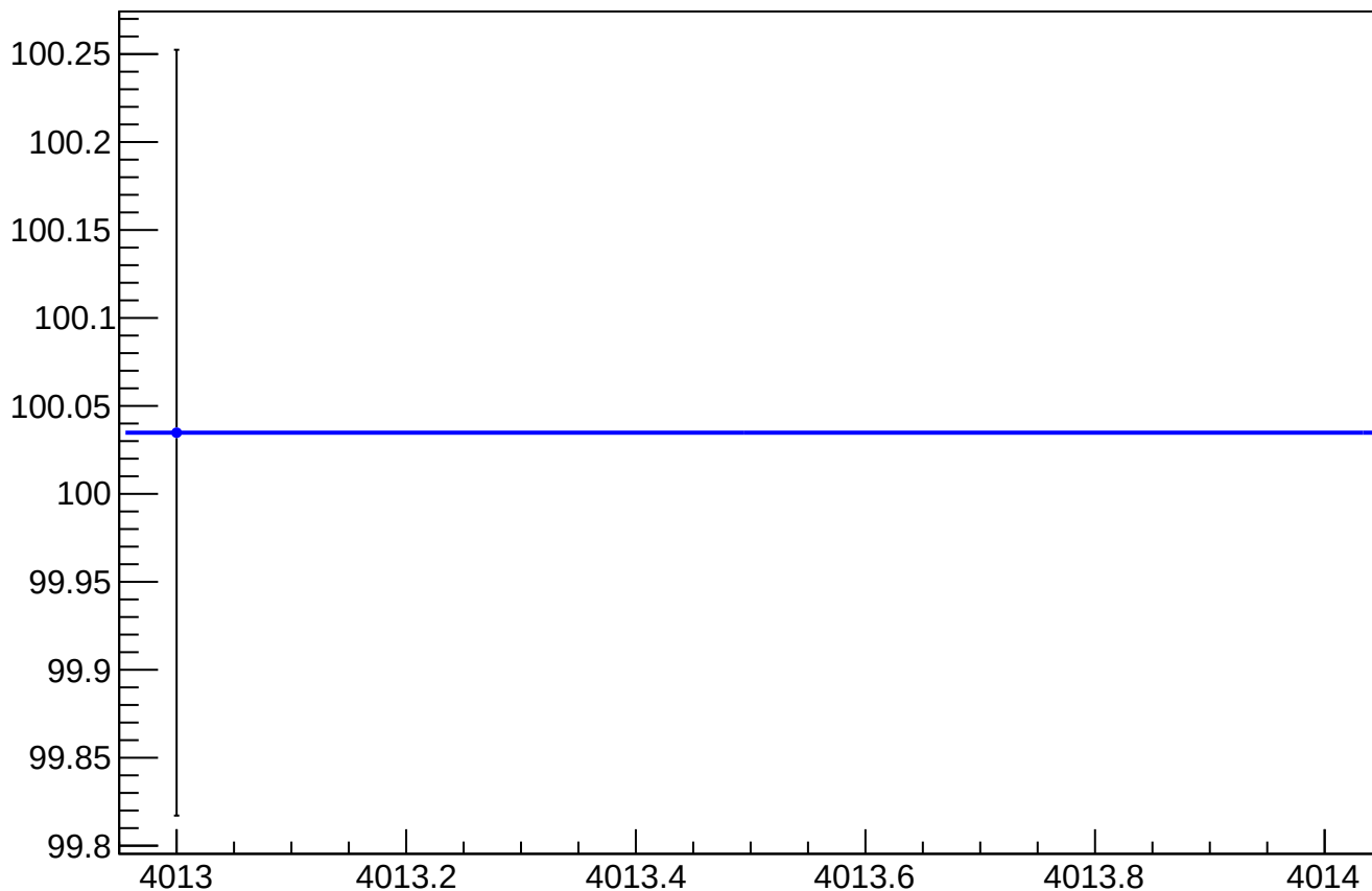
eigen_cor_asym_sam_37_48_dd_rms vs Slug, Sign Corrected
