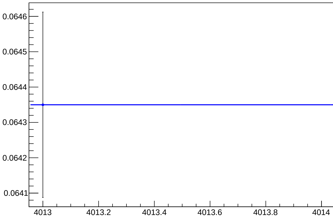
asym_atr_avg_reg_vs_cor_diff_rms vs Slug, Sign Corrected
