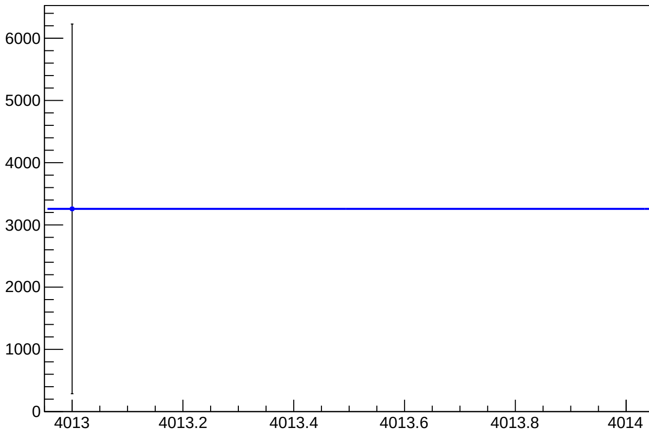
asym_sam6_reg_correction_mean vs Slug, Sign Corrected
