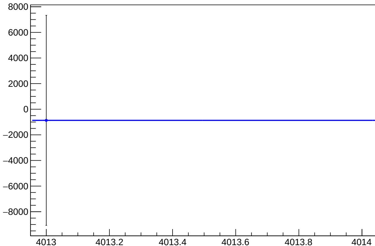
asym_sam4_eigen_dit_correction_mean vs Slug, Sign Corrected
