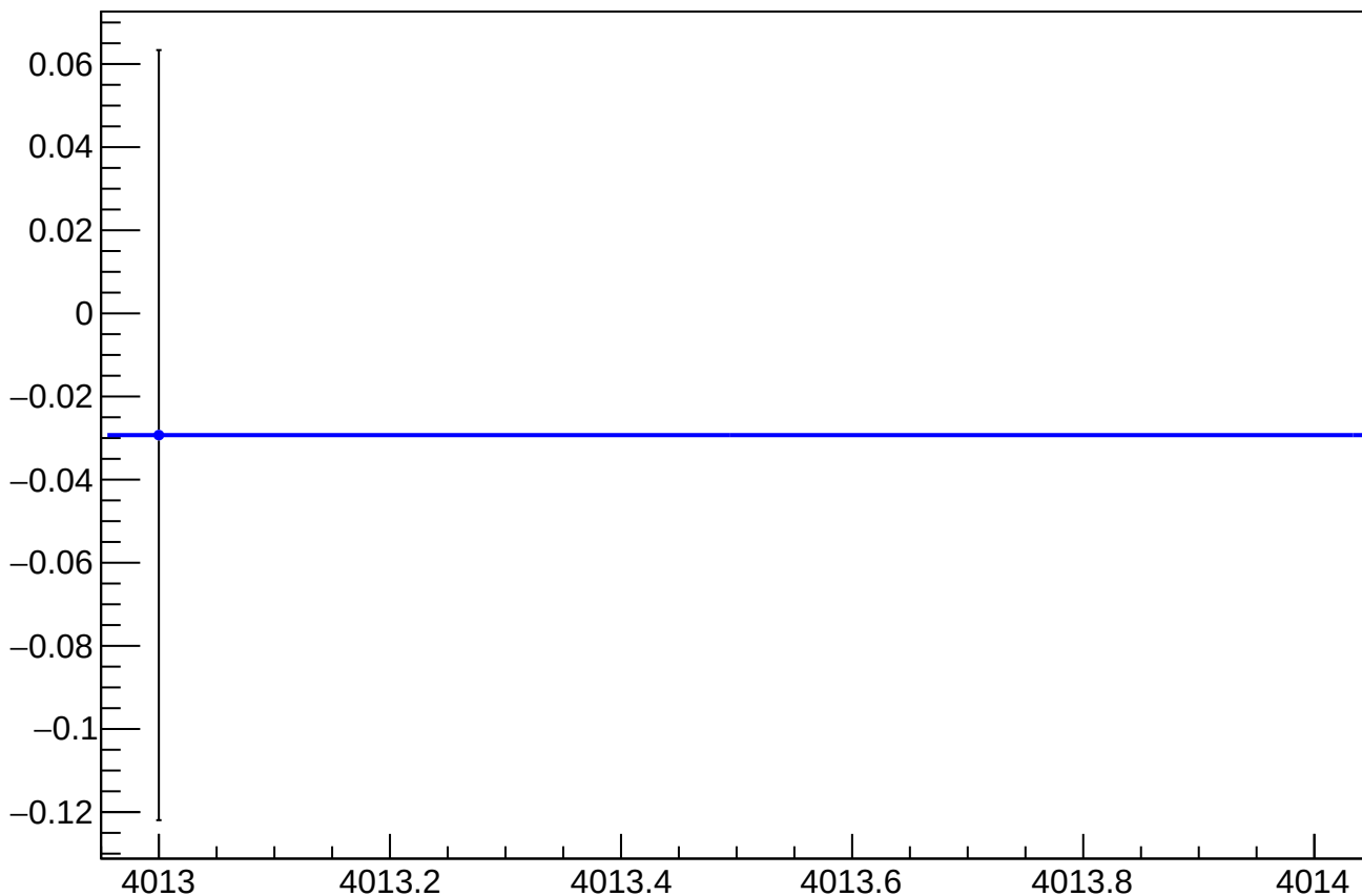
asym_us_dd_at2lr_dd_dd_eigen_dit_vs_eigen_cor_diff_mean vs Slug, Sign Corrected
