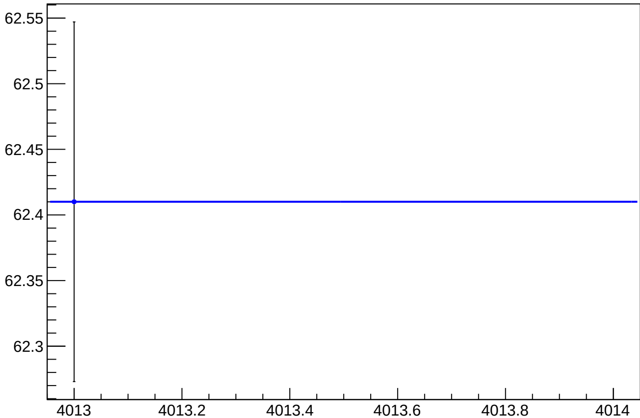
asym_usr_overload_cor_vs_eigen_cor_diff_rms vs Slug, Sign Corrected
