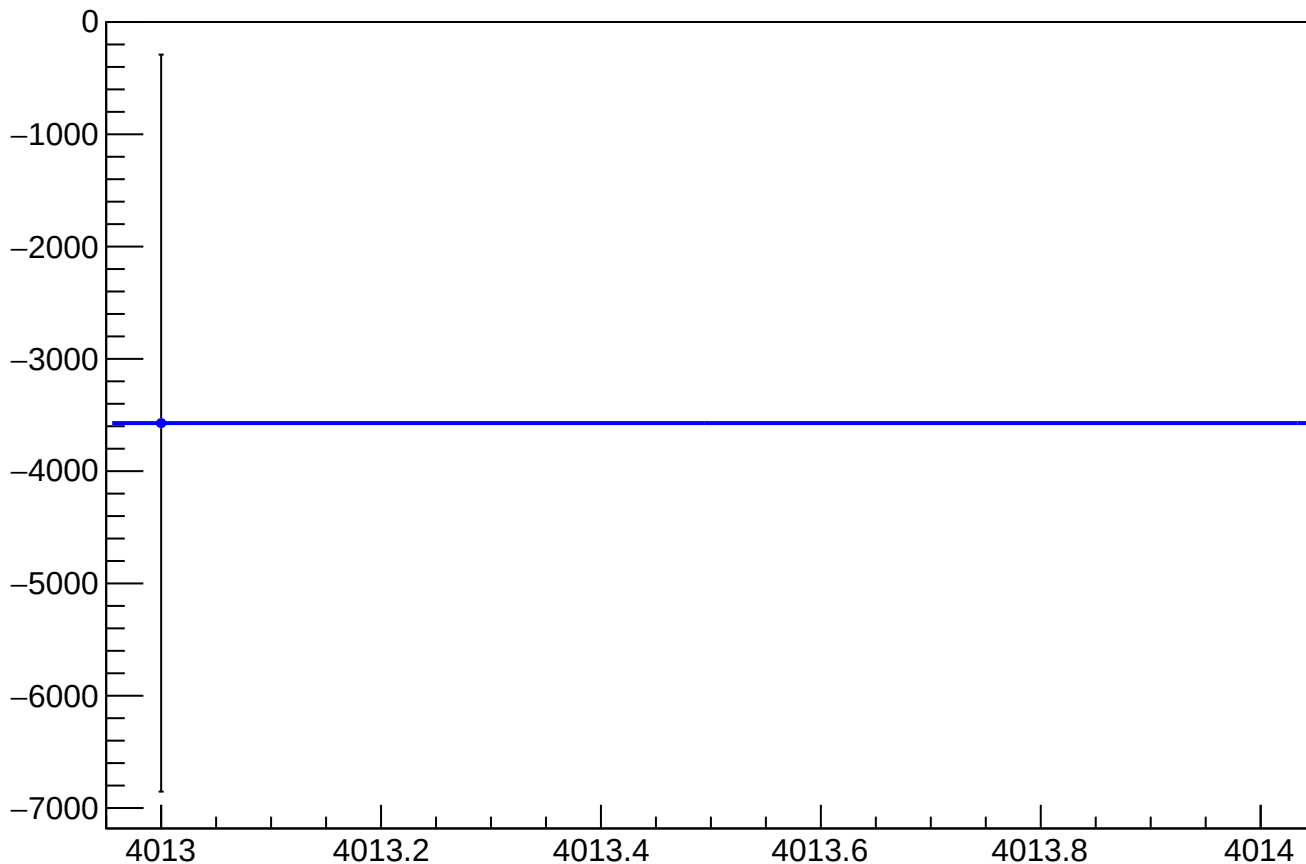
asym_sam_24_68_dd_eigen_dit_correction_mean vs Slug, Sign Corrected
