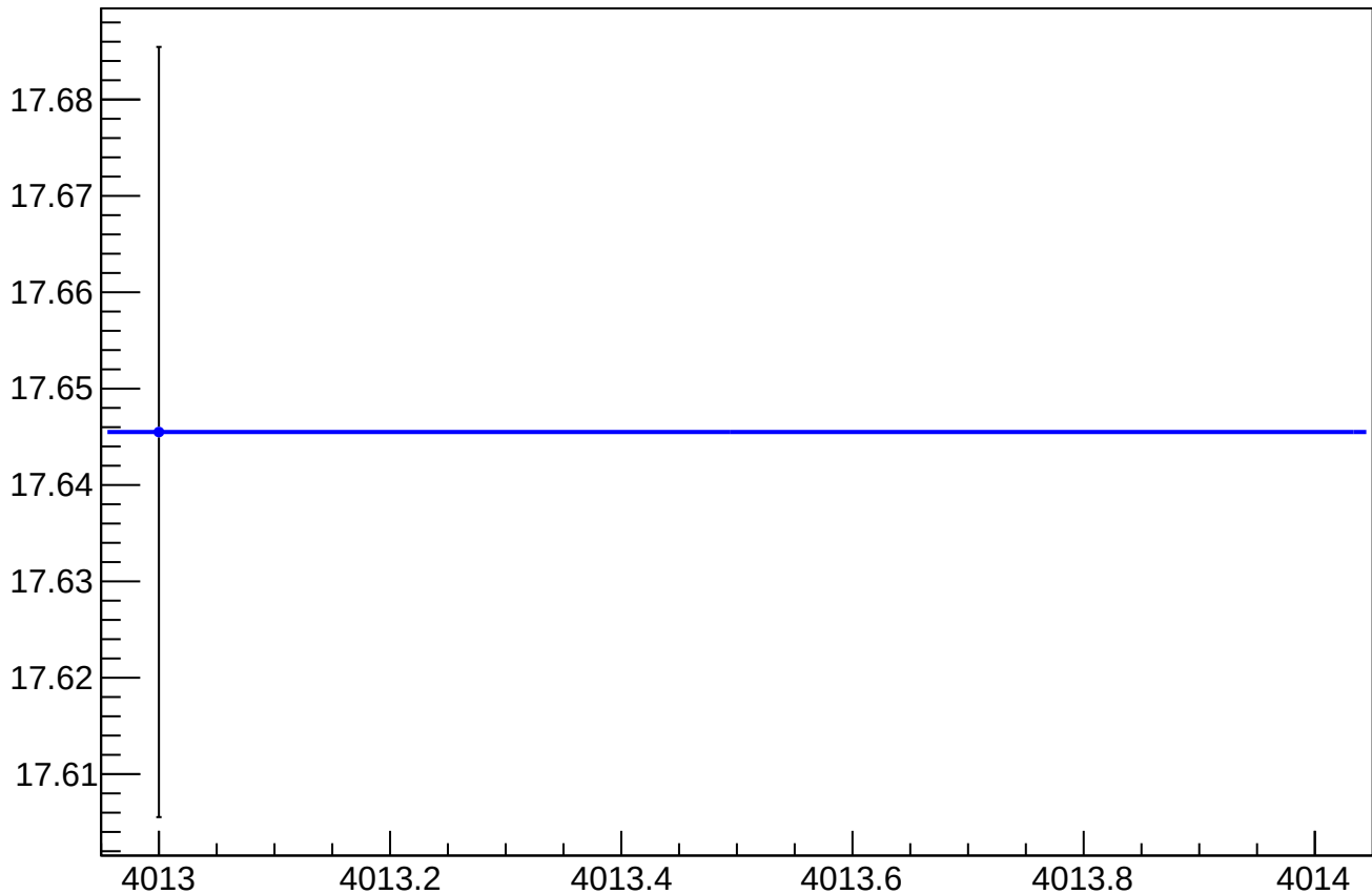
asym_sam_37_dd_eigen_dit_vs_cor_diff_rms vs Slug, Sign Corrected
