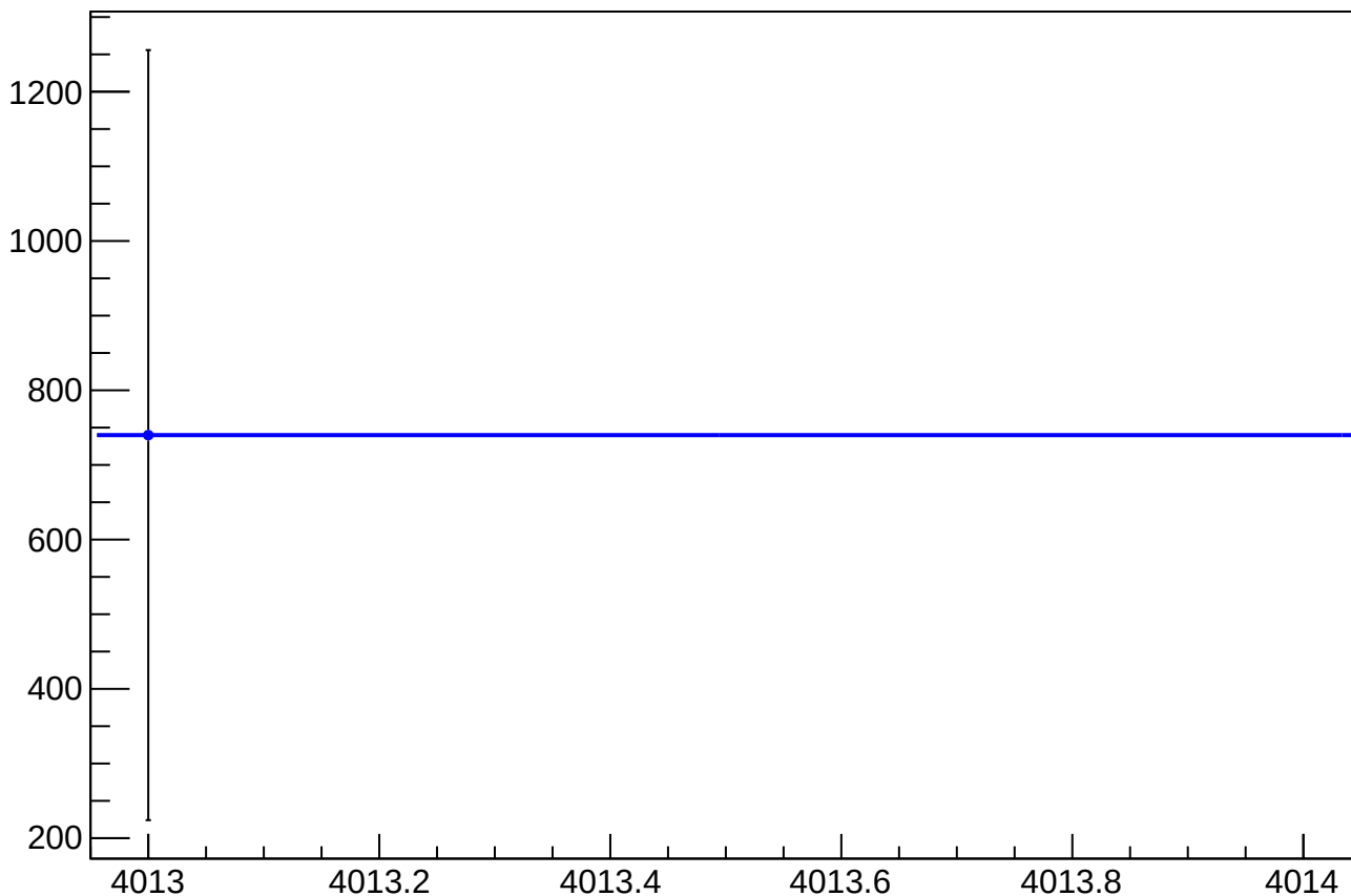
reg_asym_sam_1526_avg_mean vs Slug, Sign Corrected
