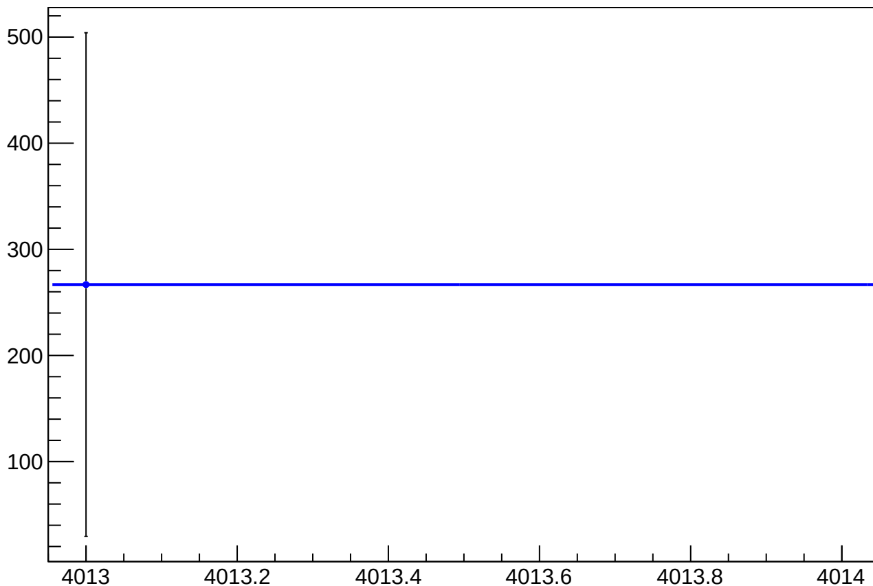
eigen_dit_asym_sam_15_48_dd_mean vs Slug, Sign Corrected
