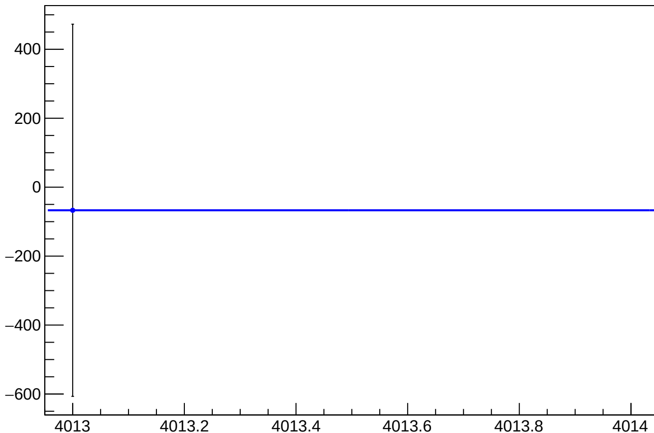
asym_sam1_cor_correction_mean vs Slug, Sign Corrected
