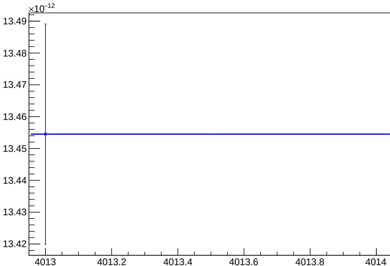
asym_sam6_eigen_cor_vs_cor_diff_rms vs Slug, Sign Corrected
