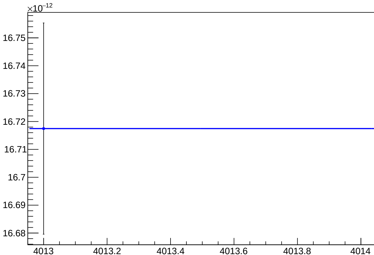
asym_sam_37_48_dd_eigen_cor_vs_cor_diff_rms vs Slug, Sign Corrected
