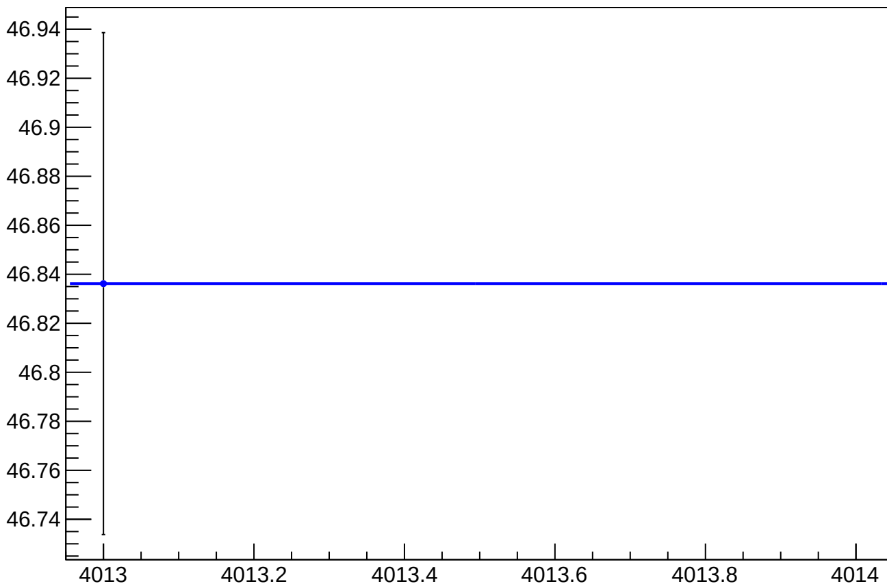
asym_us_avg_overload_cor_vs_cor_diff_rms vs Slug, Sign Corrected
