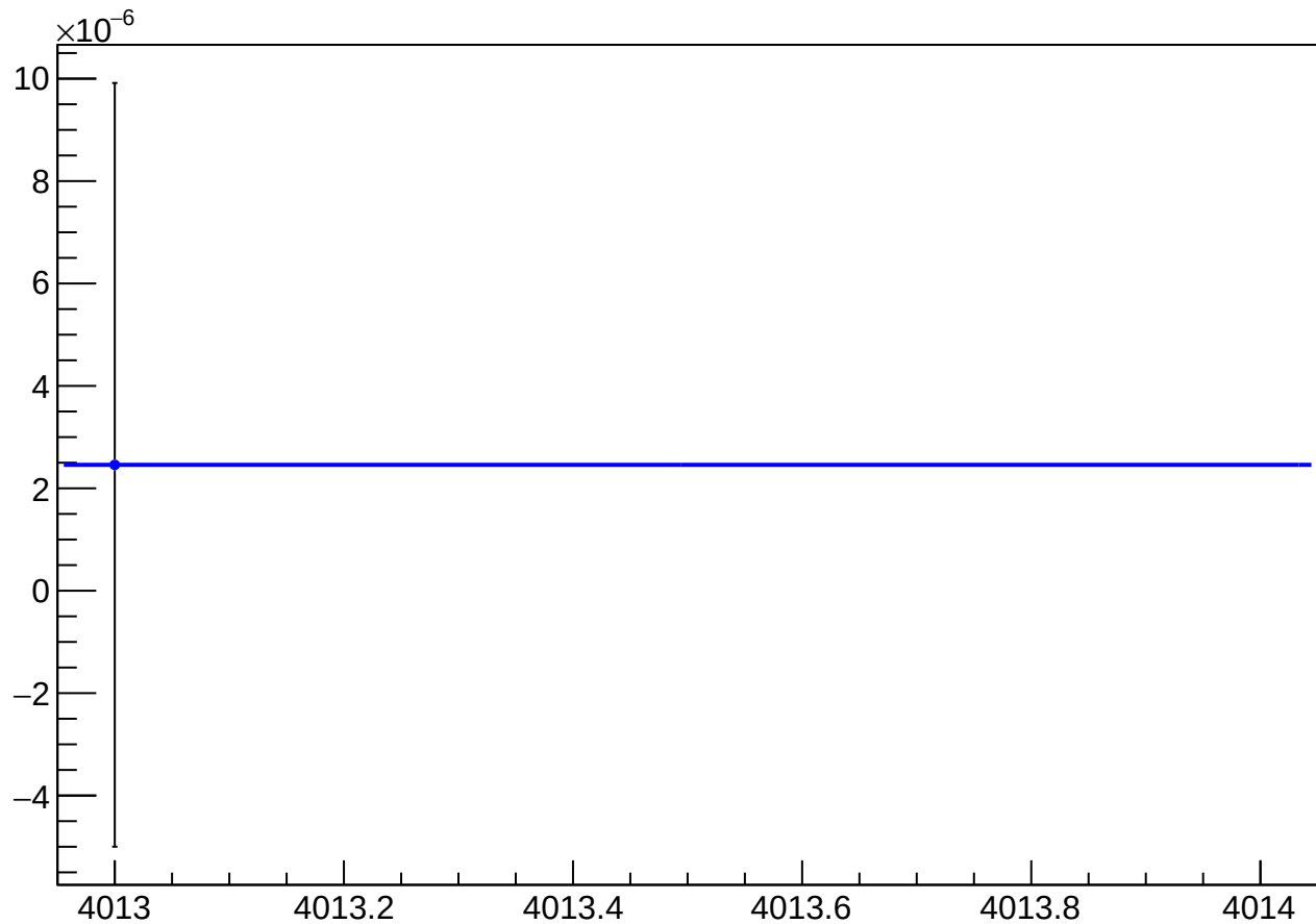
asym_sam_37_avg_eigen_dit_vs_dit_diff_mean vs Slug, Sign Corrected
