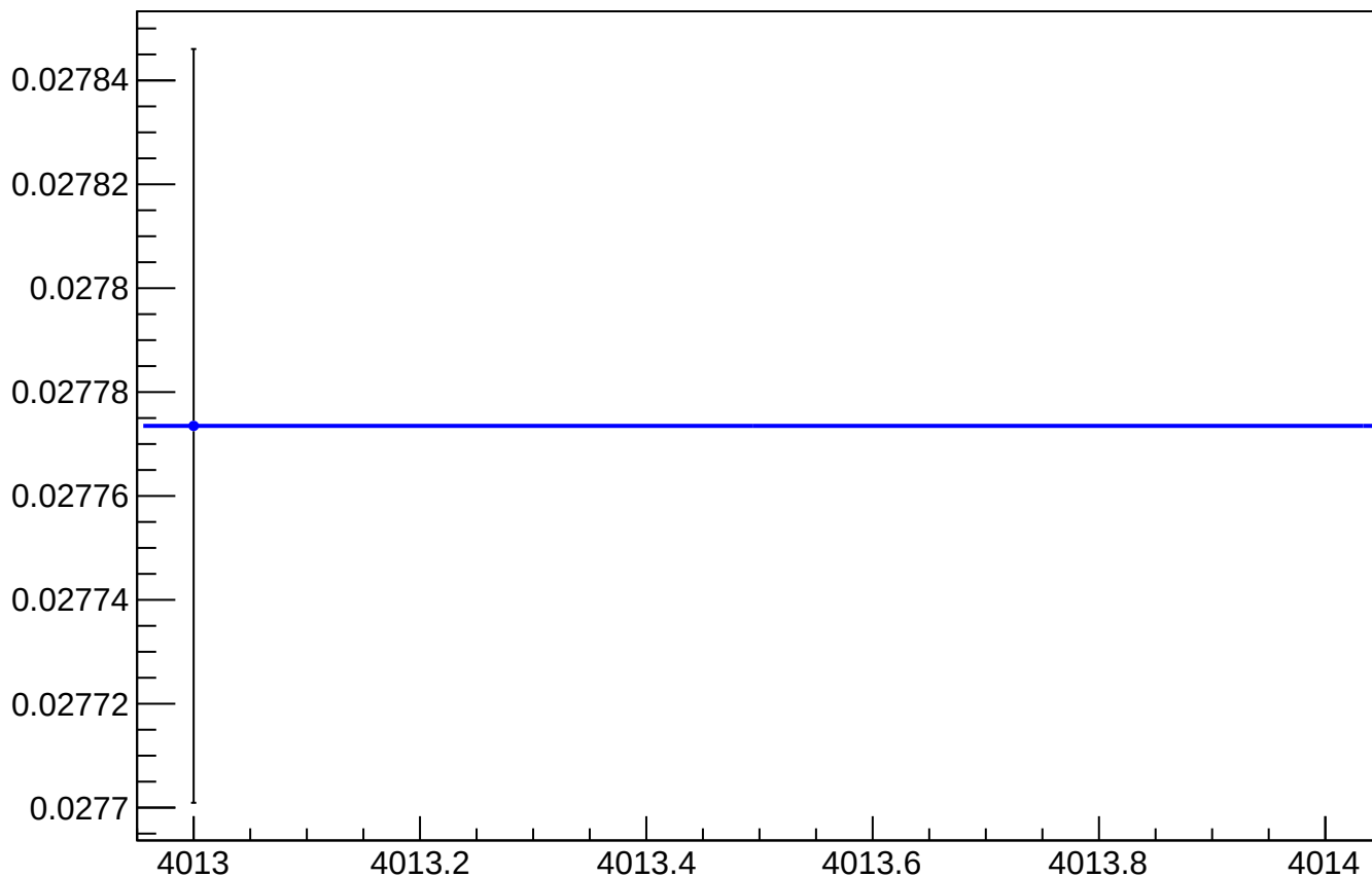
asym_sam_48_avg_reg_vs_cor_diff_rms vs Slug, Sign Corrected
