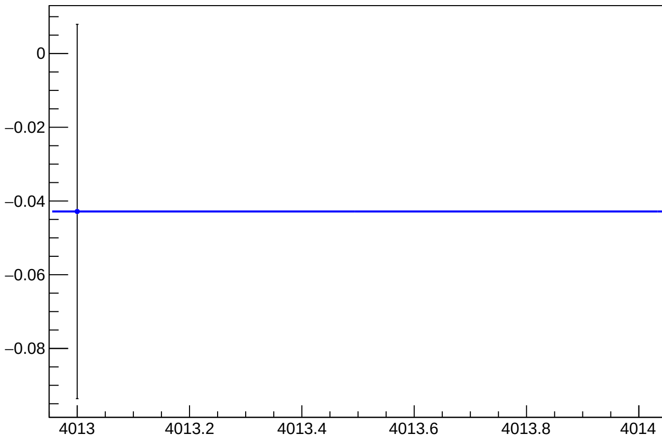
asym_atl_dd_atr_dd_dd_eigen_dit_vs_cor_diff_mean vs Slug, Sign Corrected
