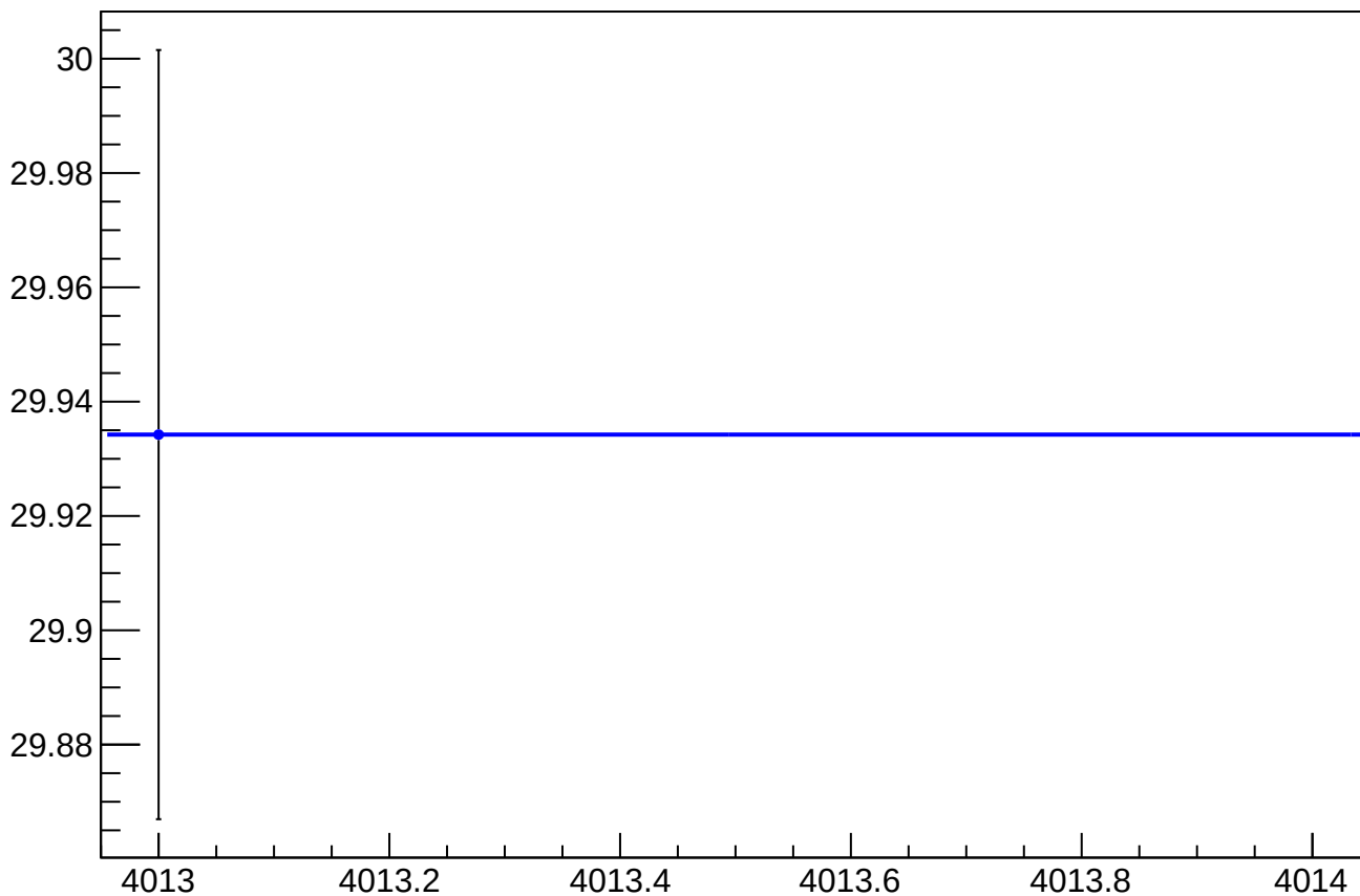
asym_us_dd_dit_vs_overload_cor_diff_rms vs Slug, Sign Corrected
