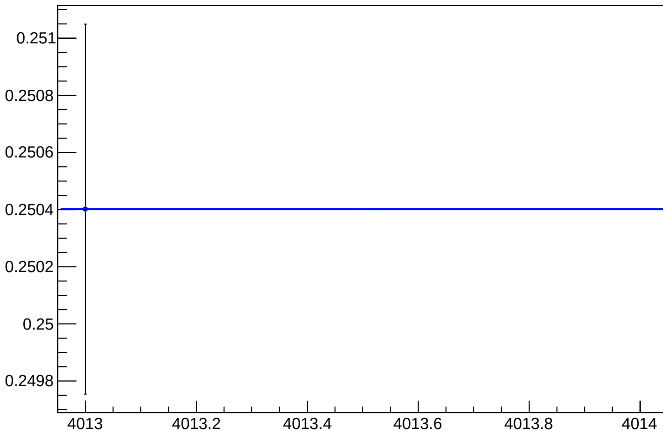
asym_at2_dd_reg_vs_cor_diff_rms vs Slug, Sign Corrected
