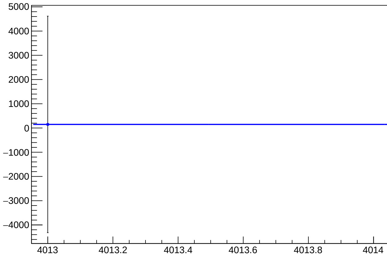
dit_asym_atl1r2_avg_mean vs Slug, Sign Corrected
