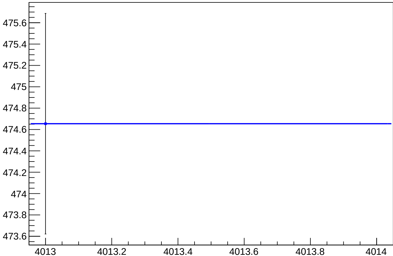
asym_sam_15_avg_eigen_dit_correction_rms vs Slug, Sign Corrected
