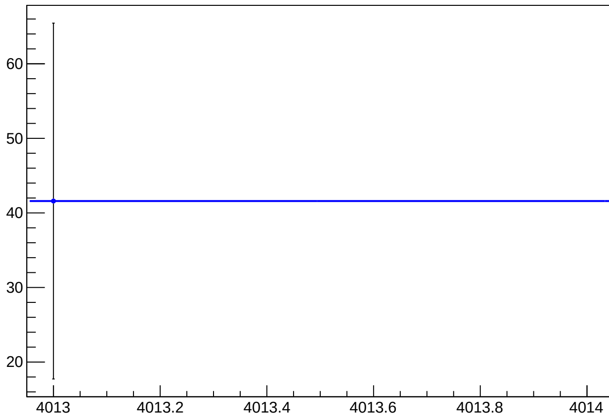
reg_asym_us_avg_at2lr_avg_dd_diff_bpm4aY_slope vs Slug, Sign Corrected
