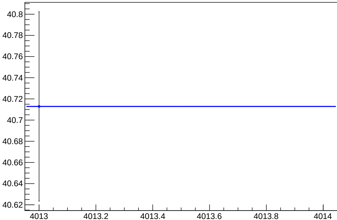
asym_sam_26_48_dd_eigen_dit_vs_eigen_cor_diff_rms vs Slug, Sign Corrected
