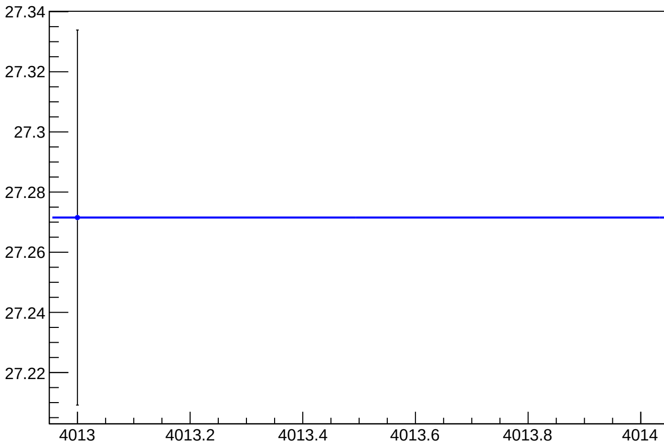
asym_sam8_dit_vs_cor_diff_rms vs Slug, Sign Corrected
