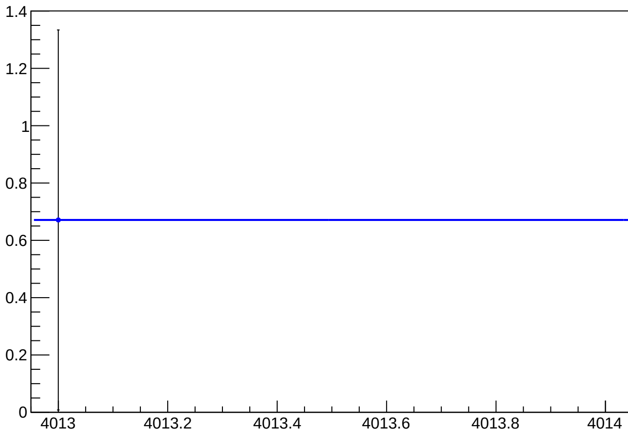
asym_us_avg_atlr_avg_dd_eigen_dit_vs_eigen_cor_diff_mean vs Slug, Sign Corrected
