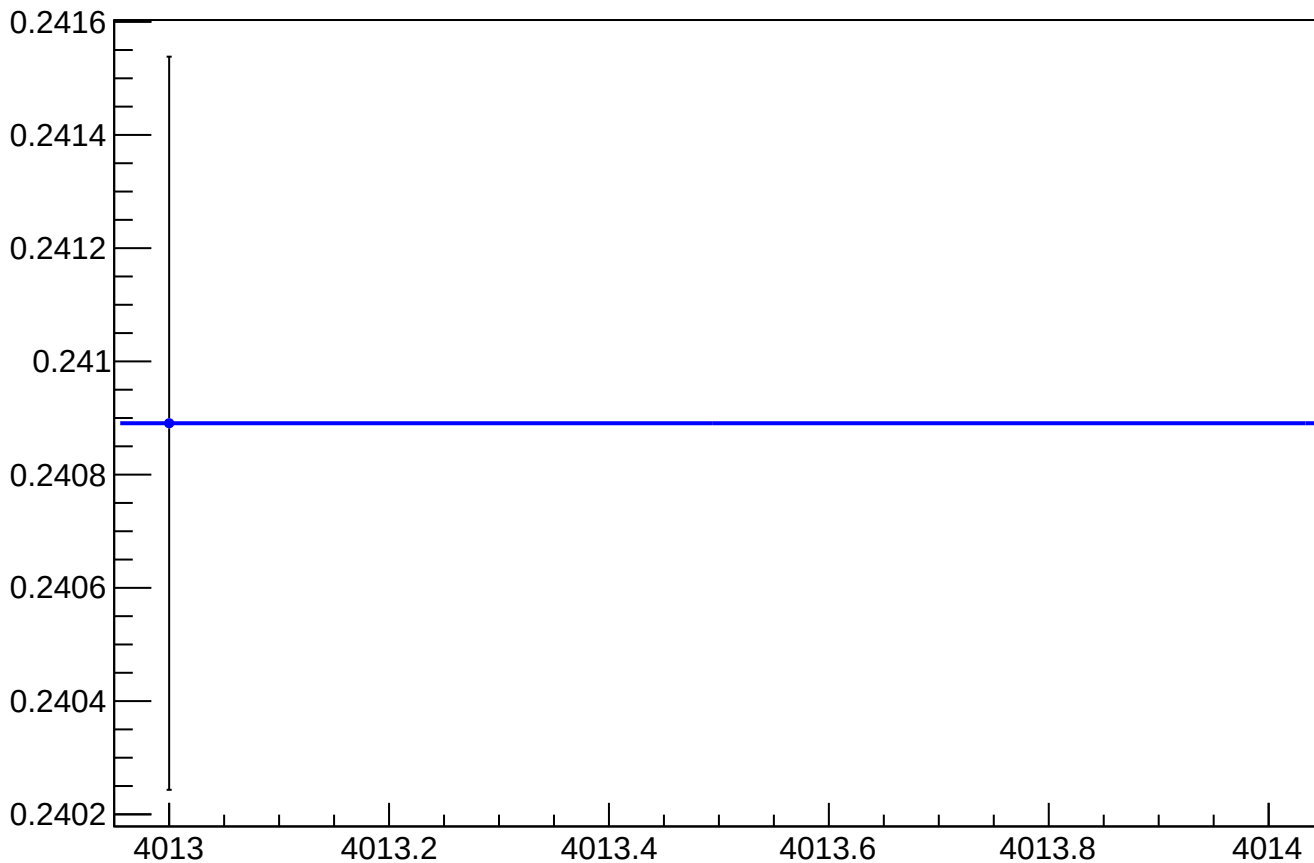
asym_atr1l2_dd_reg_vs_cor_diff_rms vs Slug, Sign Corrected
