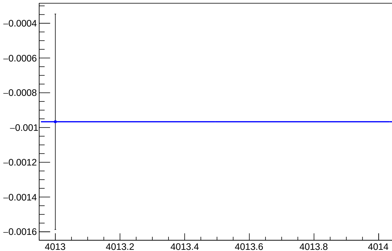
asym_atl_avg_atr_avg_avg_reg_vs_cor_diff_mean vs Slug, Sign Corrected
