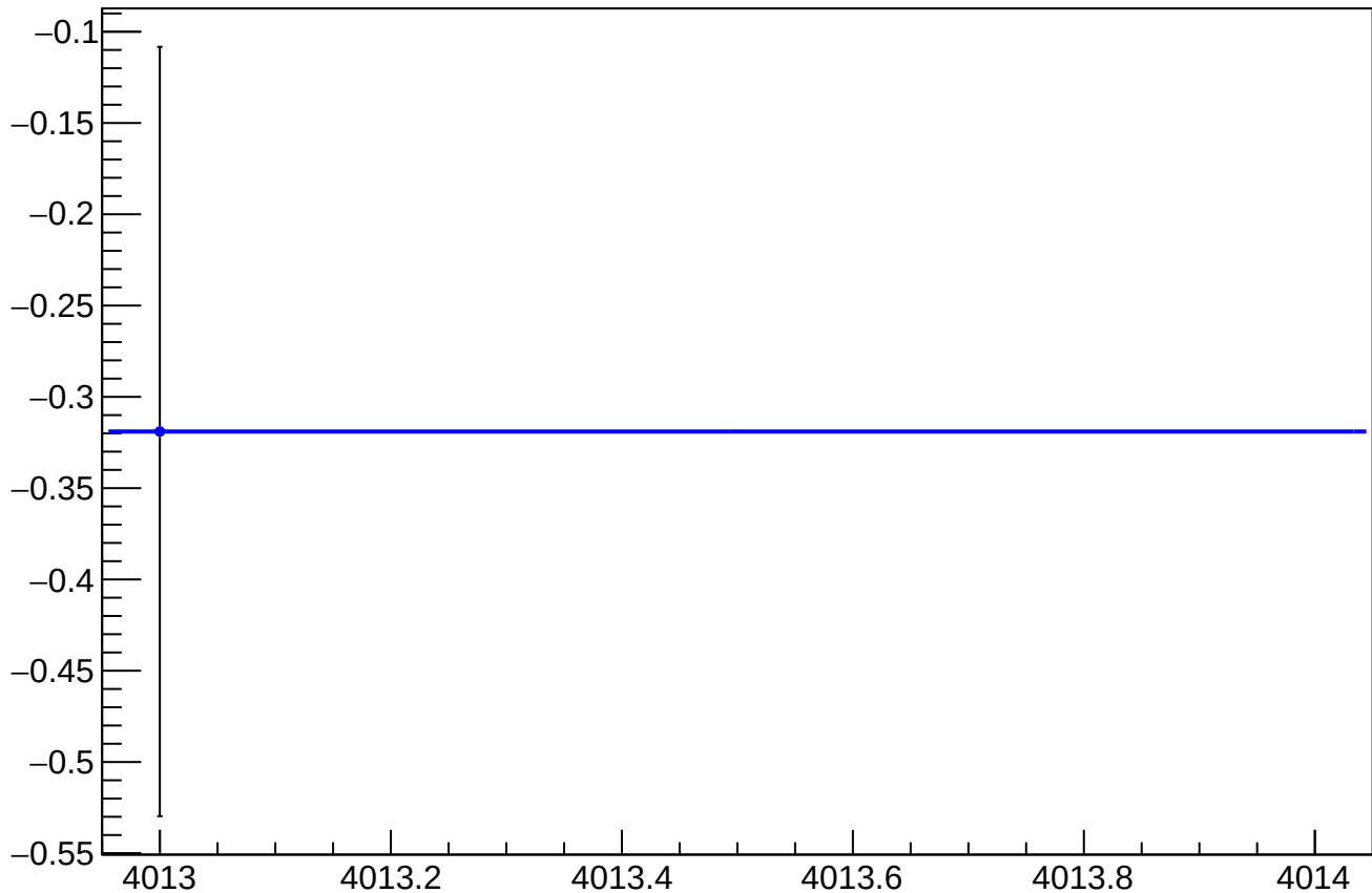
asym_us_avg_at1lr_avg_dd_eigen_dit_vs_eigen_cor_diff_mean vs Slug, Sign Corrected
