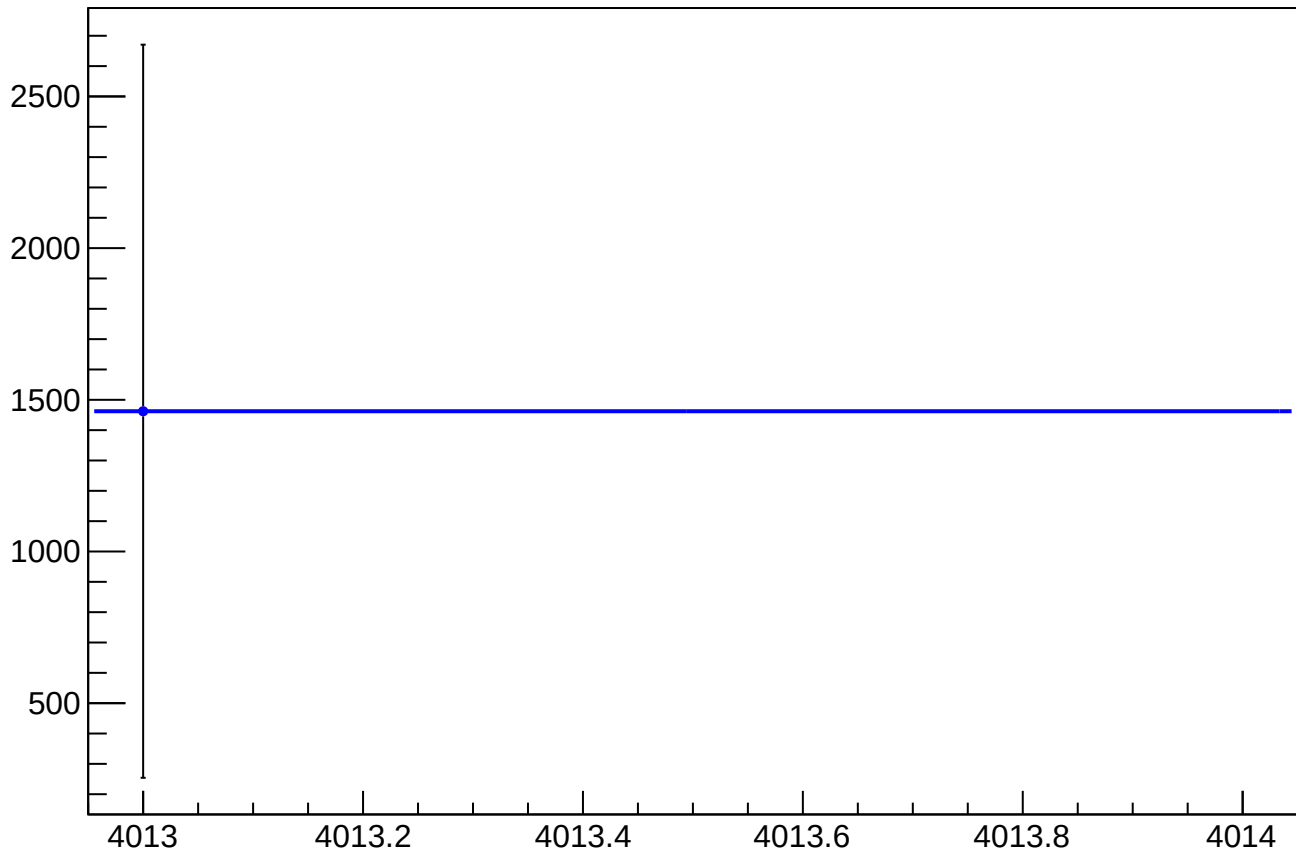
asym_sam_15_37_dd_cor_correction_mean vs Slug, Sign Corrected
