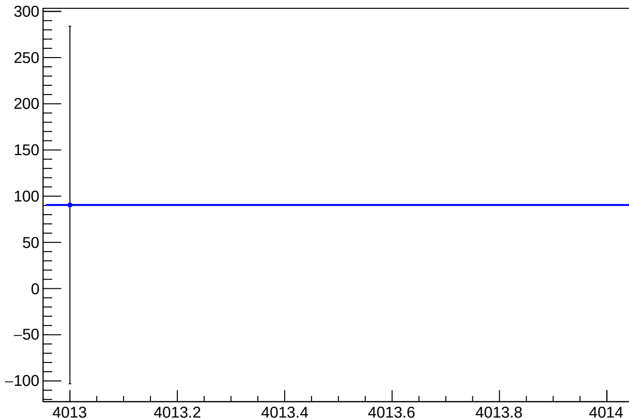
asym_atl1r2_dd_atl2r1_dd_avg_cor_correction_mean vs Slug, Sign Corrected
