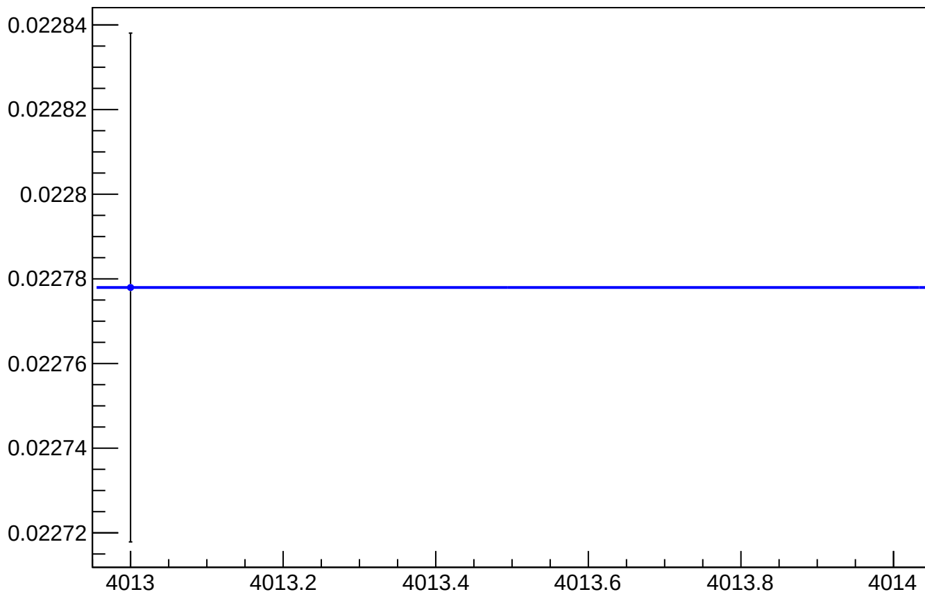
asym_sam_15_26_dd_reg_vs_cor_diff_rms vs Slug, Sign Corrected
