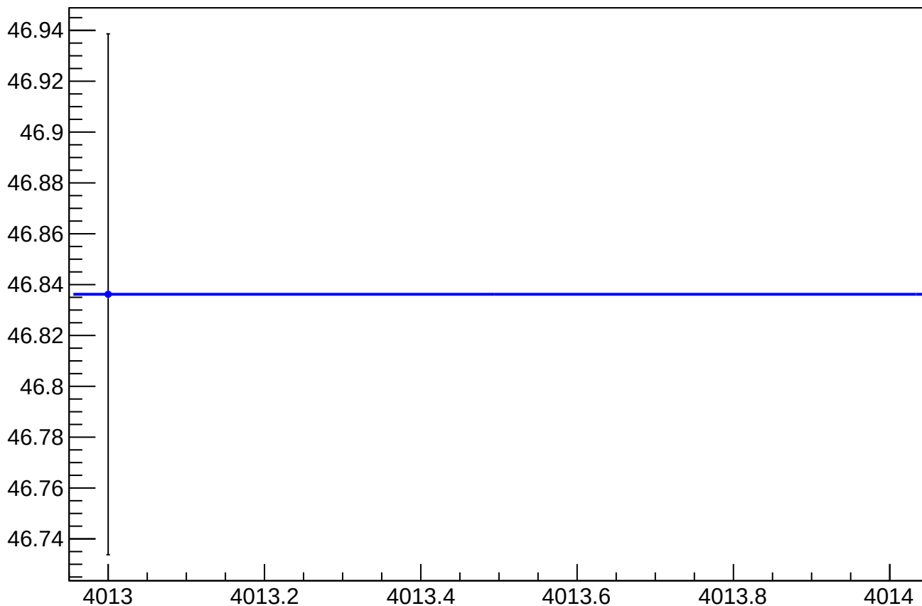
asym_us_avg_overload_cor_vs_eigen_cor_diff_rms vs Slug, Sign Corrected
