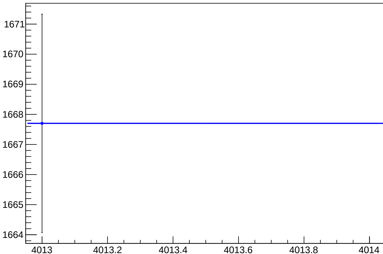
reg_asym_us_dd_at1lr_dd_avg_rms vs Slug, Sign Corrected
