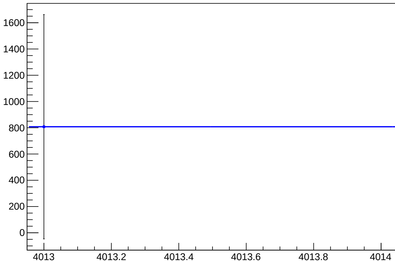
asym_sam_1357_2468_dd_eigen_cor_correction_mean vs Slug, Sign Corrected
