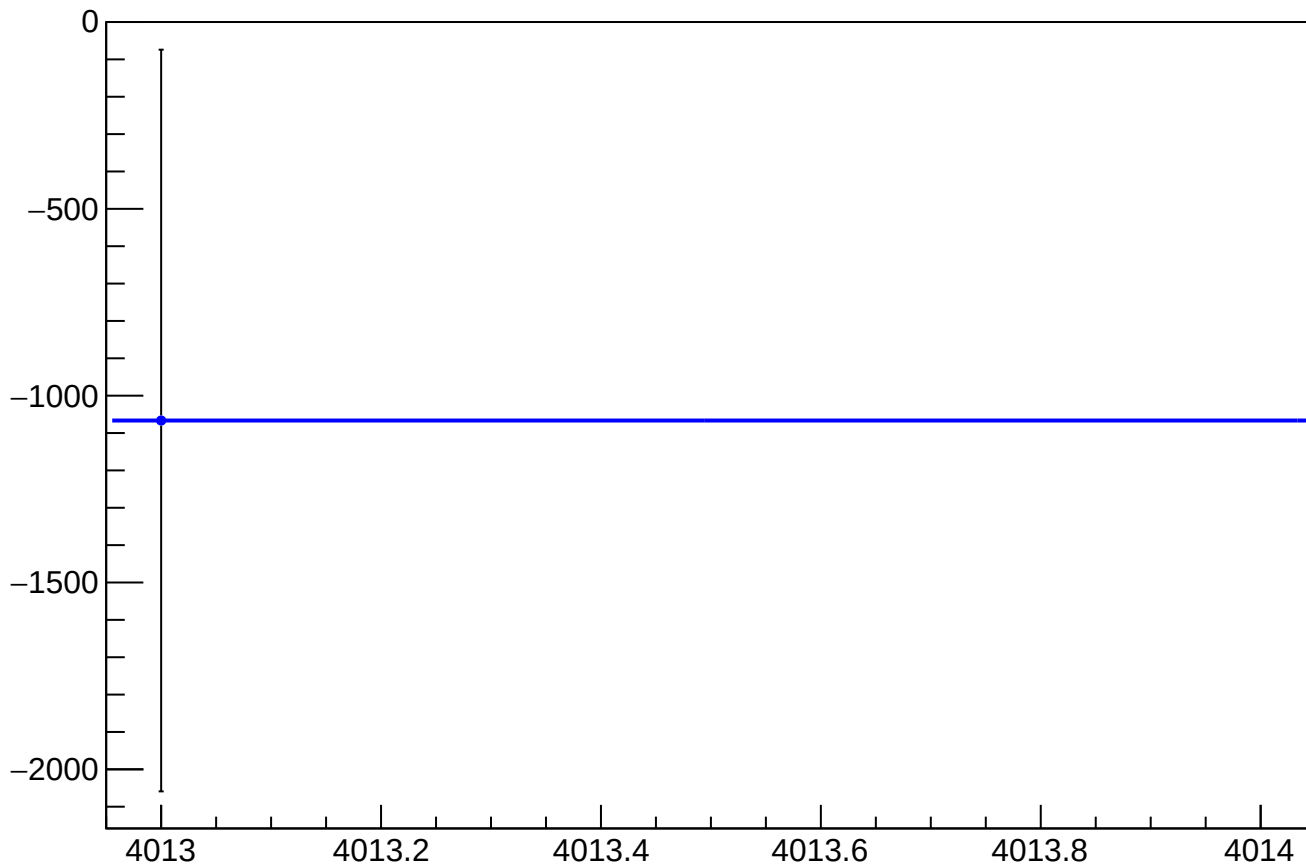
asym_sam7_reg_correction_mean vs Slug, Sign Corrected
