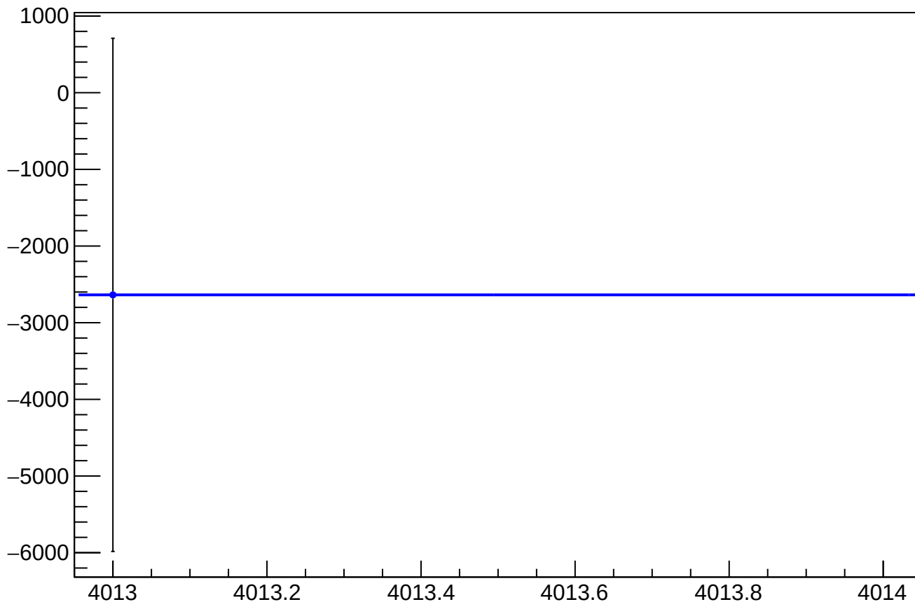
asym_sam3_dit_correction_mean vs Slug, Sign Corrected
