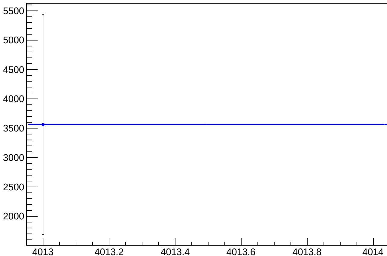
eigen_cor_asym_sam2_mean vs Slug, Sign Corrected
