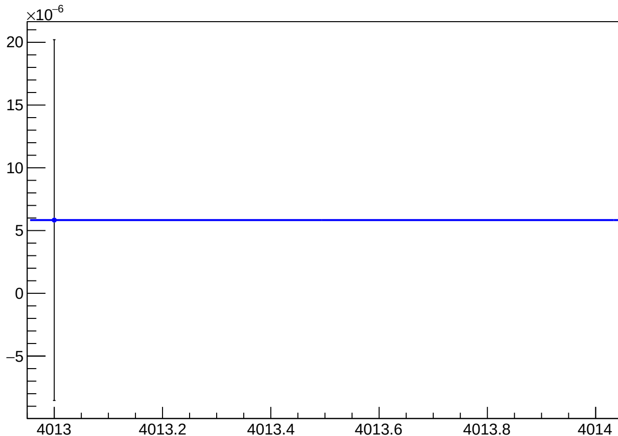
asym_at1_dd_at2_dd_avg_eigen_dit_vs_dit_diff_mean vs Slug, Sign Corrected
