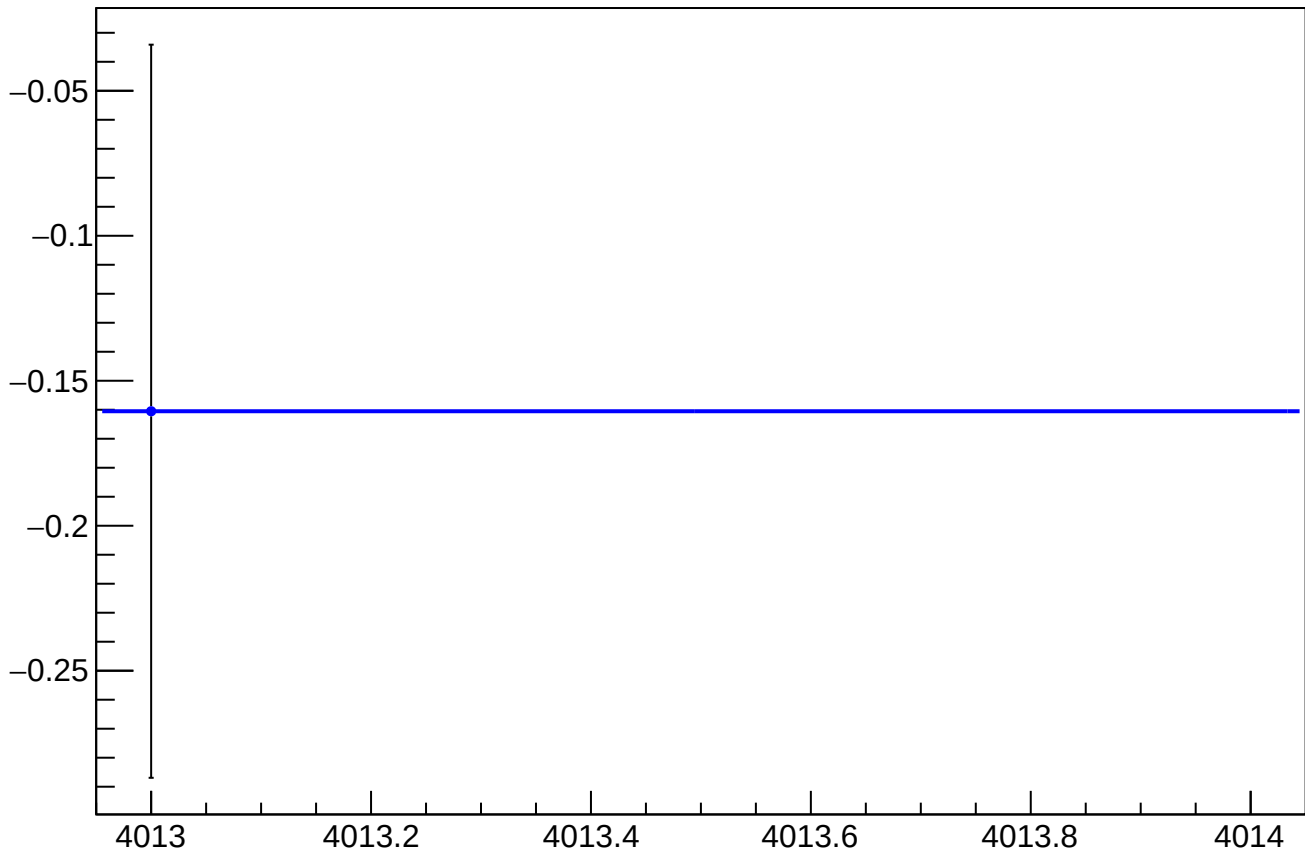
asym_sam_26_48_dd_dit_vs_cor_diff_mean vs Slug, Sign Corrected
