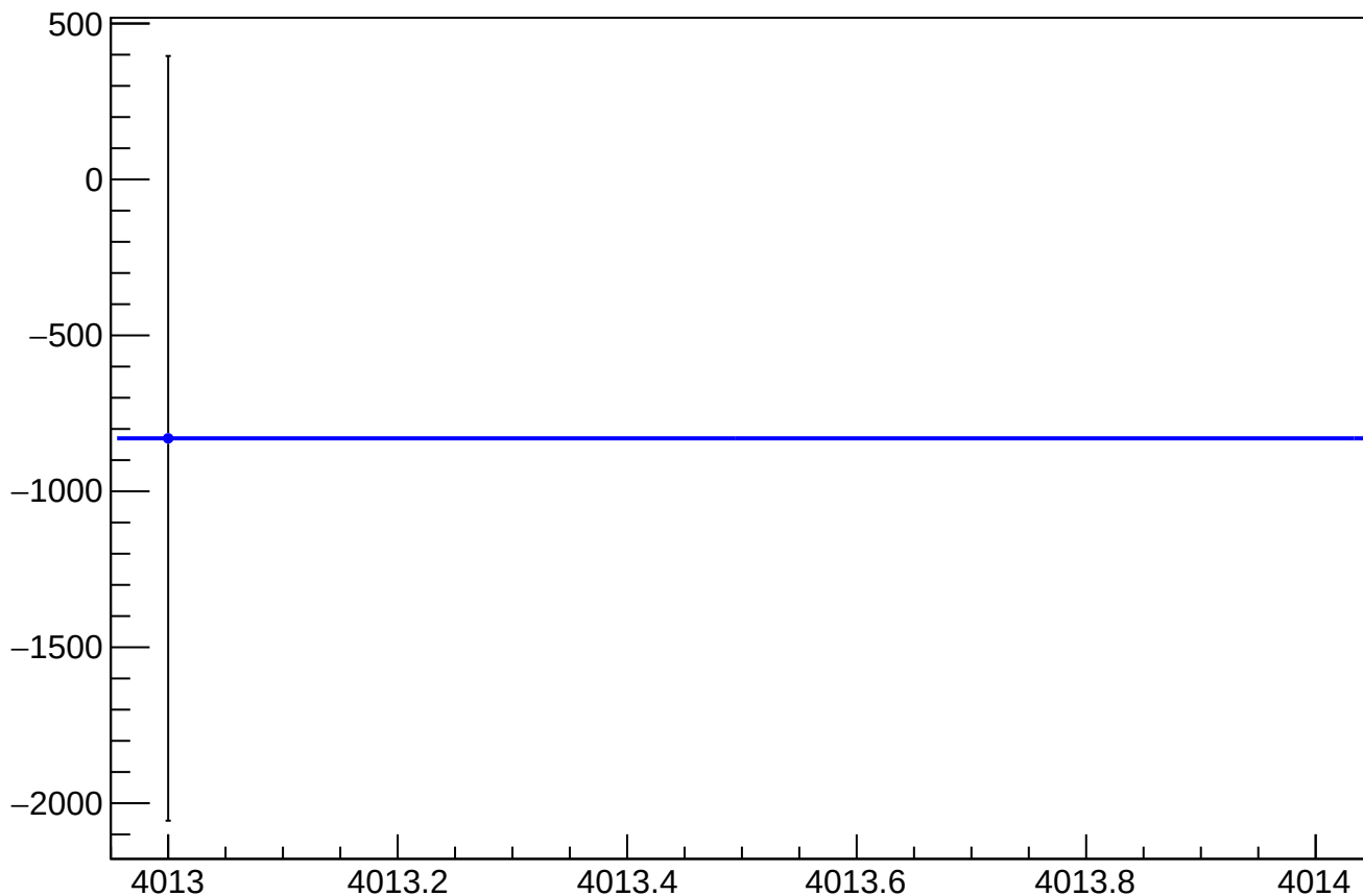
asym_sam_37_dd_eigen_dit_correction_mean vs Slug, Sign Corrected
