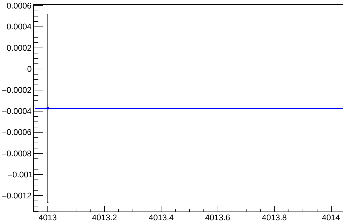
asym_atr1l2_avg_reg_vs_cor_diff_mean vs Slug, Sign Corrected
