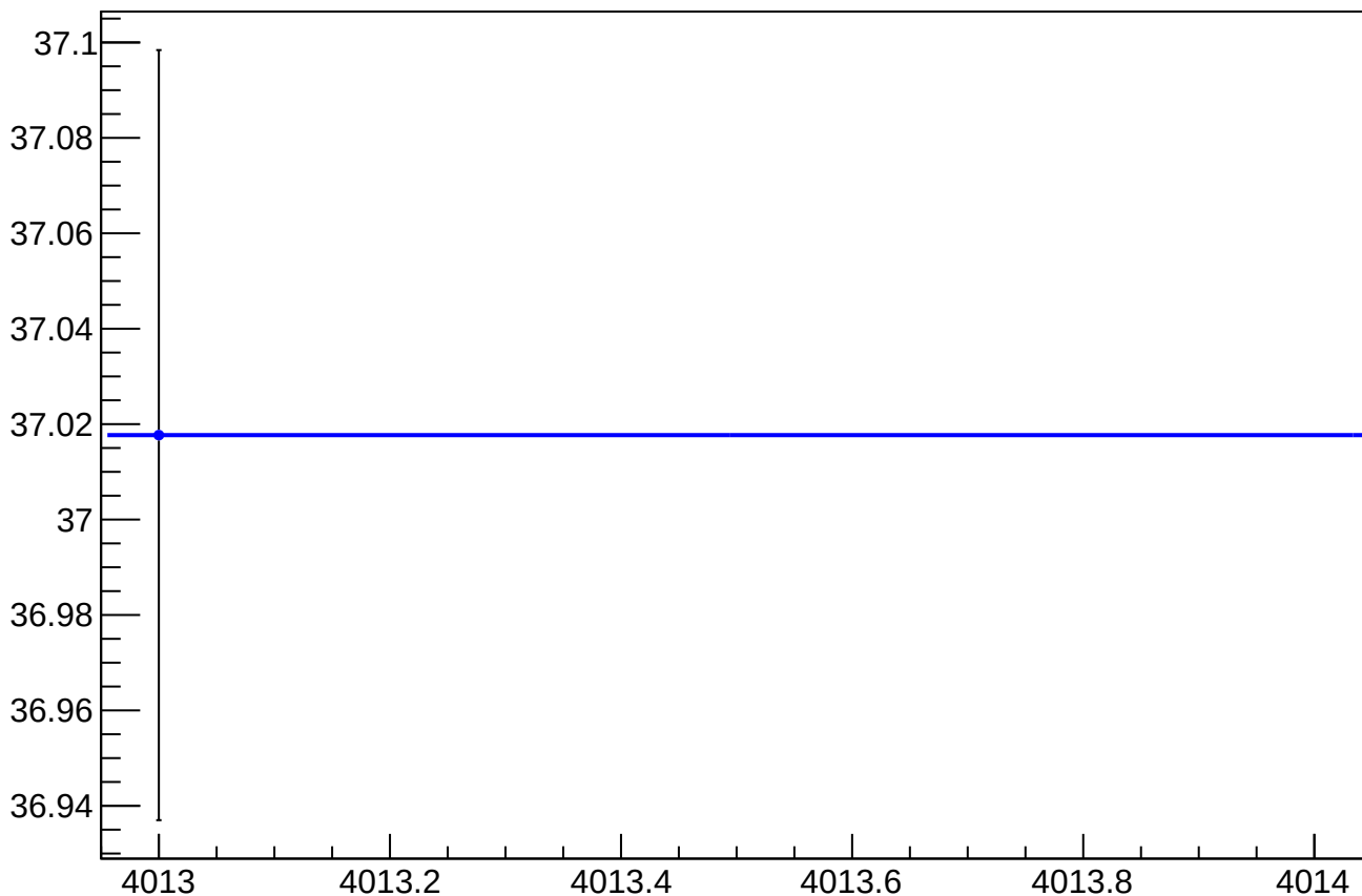
asym_sam_15_26_dd_dit_vs_cor_diff_rms vs Slug, Sign Corrected
