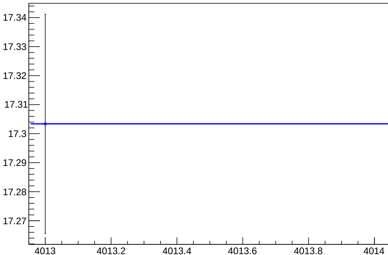
asym_sam_13_57_dd_eigen_dit_vs_cor_diff_rms vs Slug, Sign Corrected
