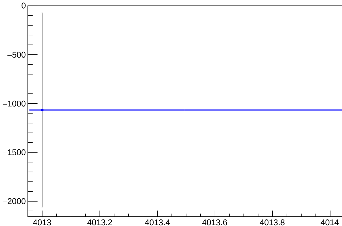
asym_sam7_eigen_cor_correction_mean vs Slug, Sign Corrected
