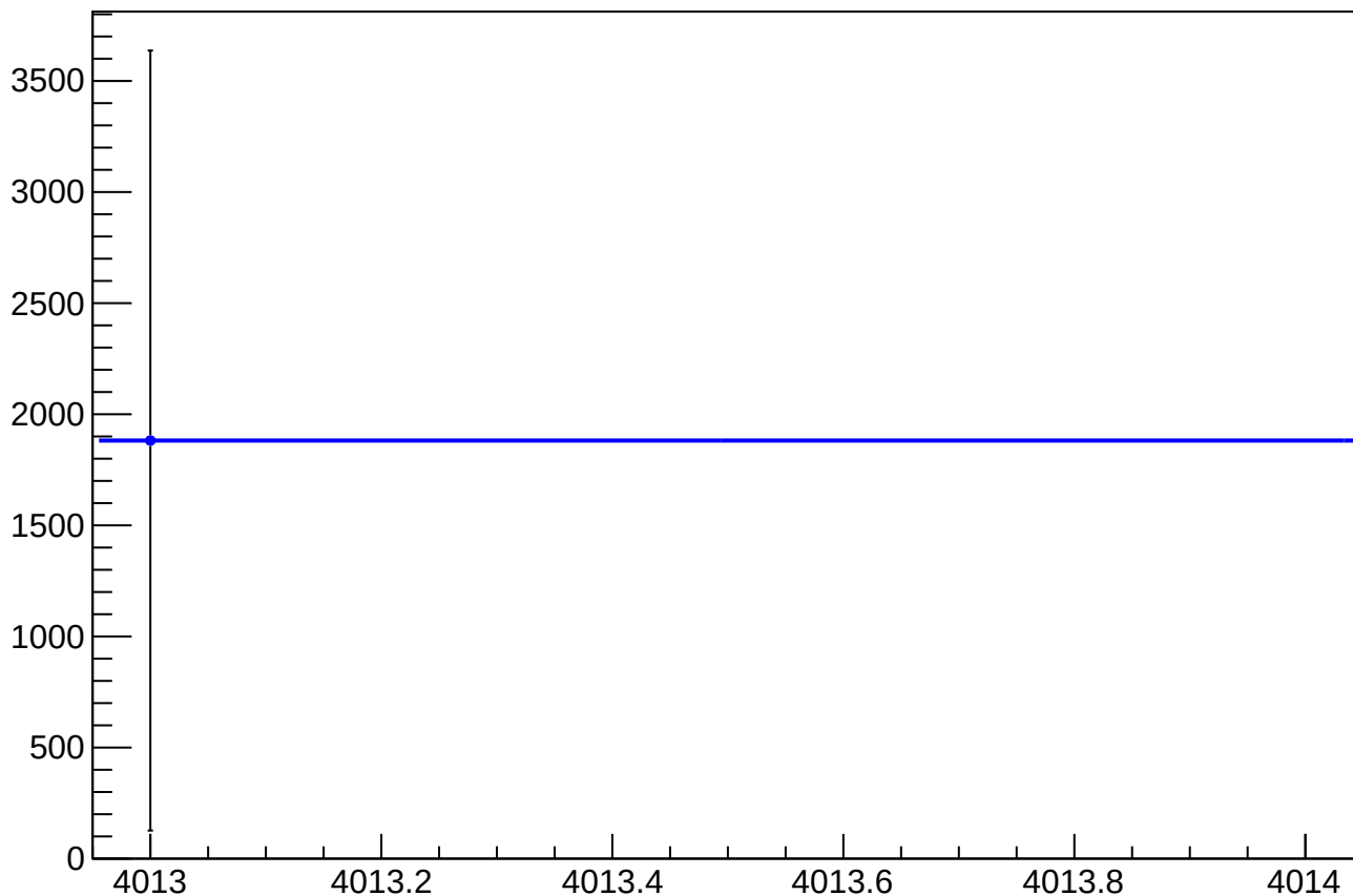
asym_usr_atr1_dd_eigen_dit_correction_mean vs Slug, Sign Corrected
