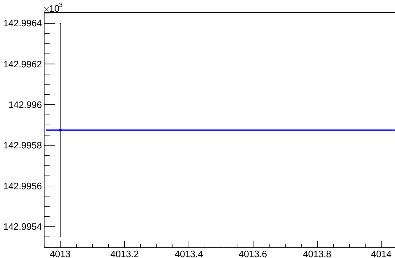
yield_bpm0l10WS_mean vs Slug, Sign Corrected
