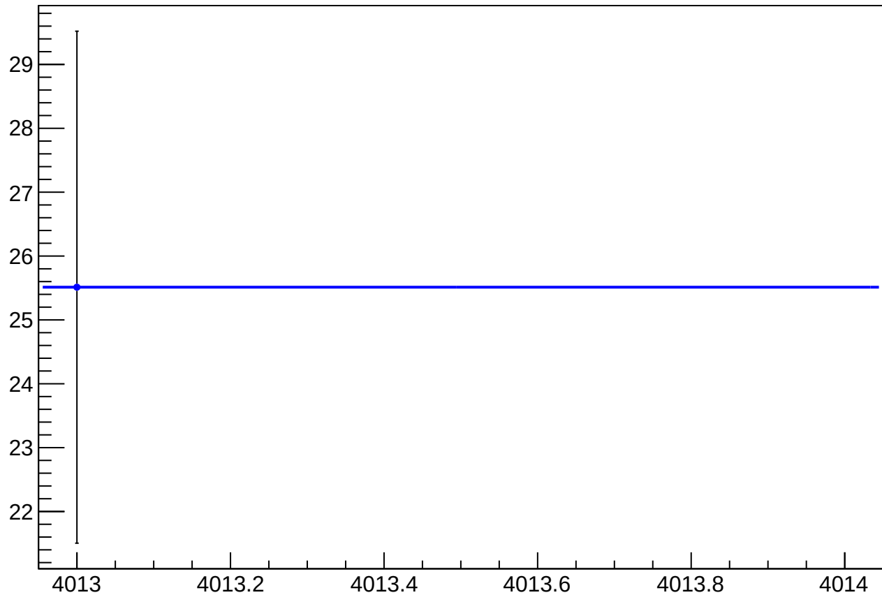
reg_asym_us_dd_at2lr_dd_diff_bpm1X_slope vs Slug, Sign Corrected
