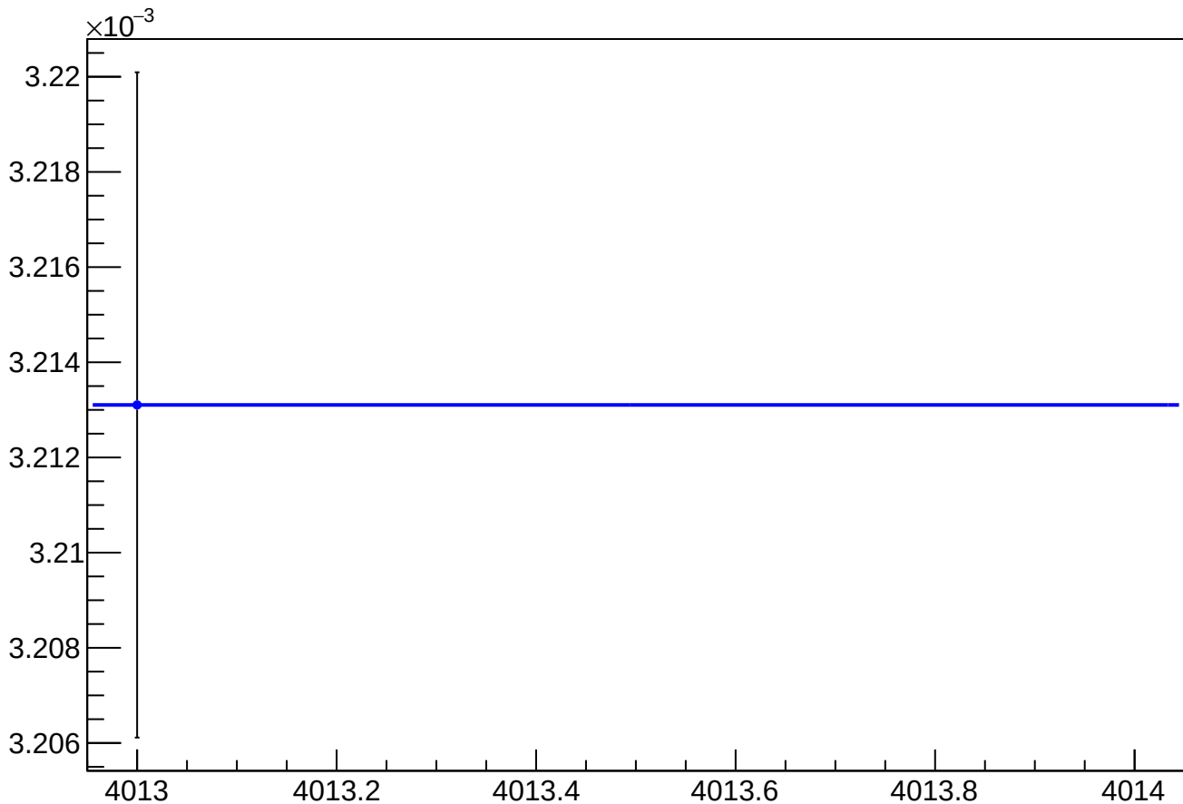
asym_sam_15_48_dd_eigen_dit_vs_dit_diff_rms vs Slug, Sign Corrected
