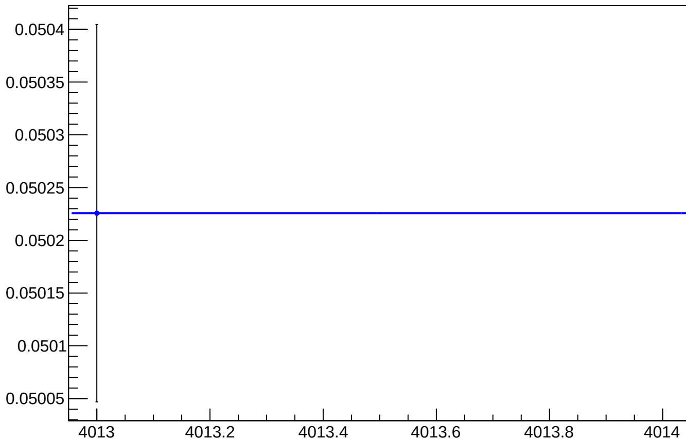
asym_atr_dd_reg_vs_cor_diff_rms vs Slug, Sign Corrected
