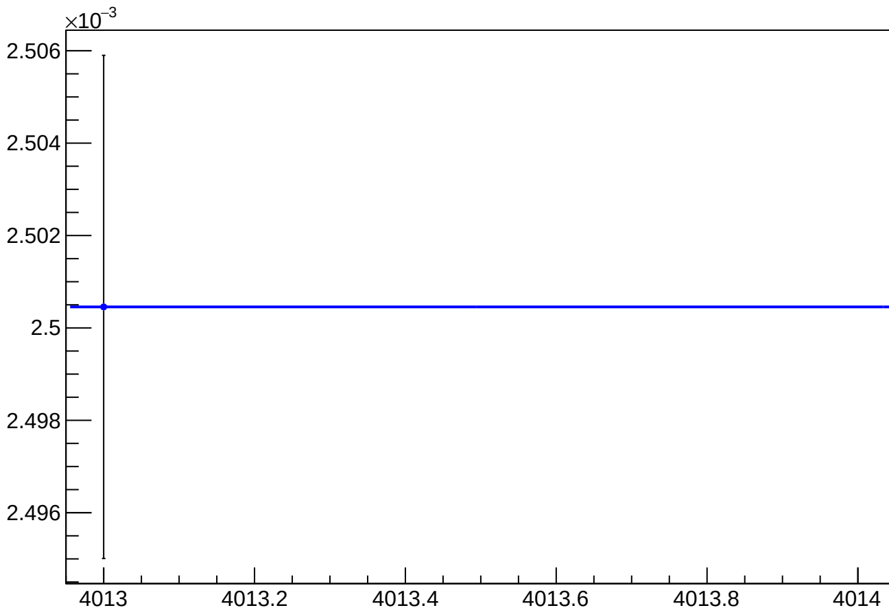
asym_sam_1548_avg_eigen_dit_vs_dit_diff_rms vs Slug, Sign Corrected
