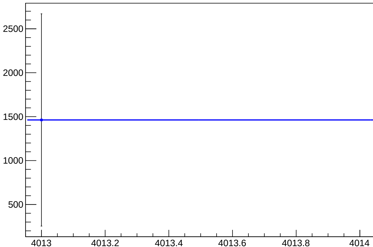
asym_sam_15_37_dd_eigen_cor_correction_mean vs Slug, Sign Corrected
