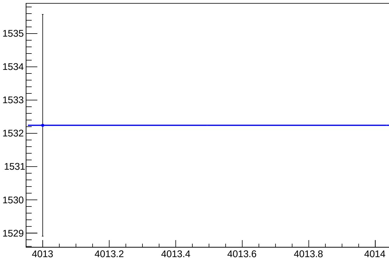
eigen_dit_asym_us_avg_at2lr_avg_dd_rms vs Slug, Sign Corrected
