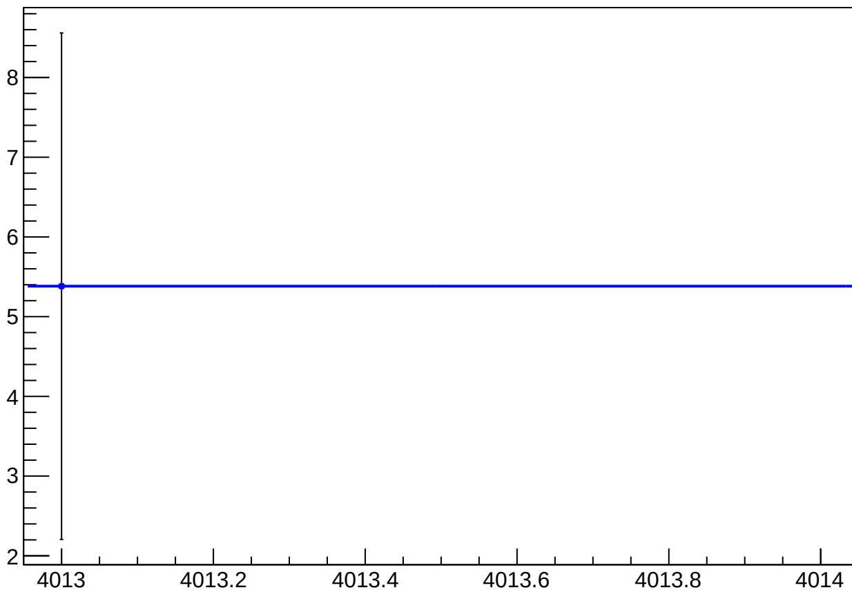
diff_bpmtargetdiffY_mean vs Slug, Sign Corrected
