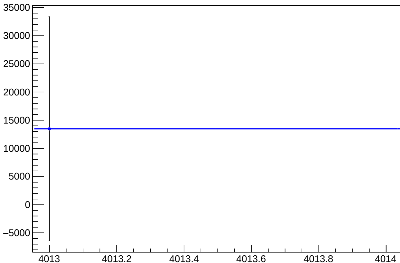
asym_atl_avg_eigen_cor_correction_mean vs Slug, Sign Corrected
