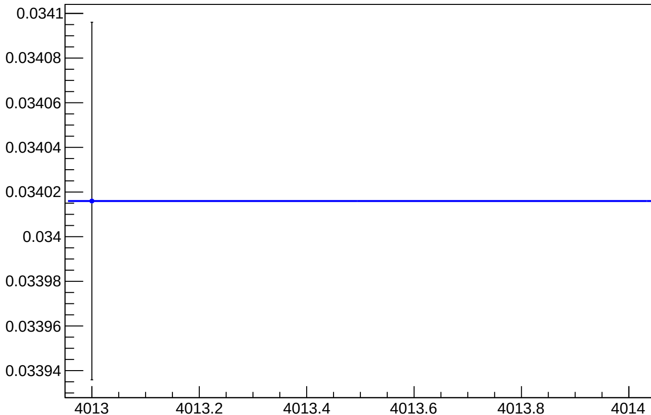
asym_sam_37_avg_reg_vs_cor_diff_rms vs Slug, Sign Corrected
