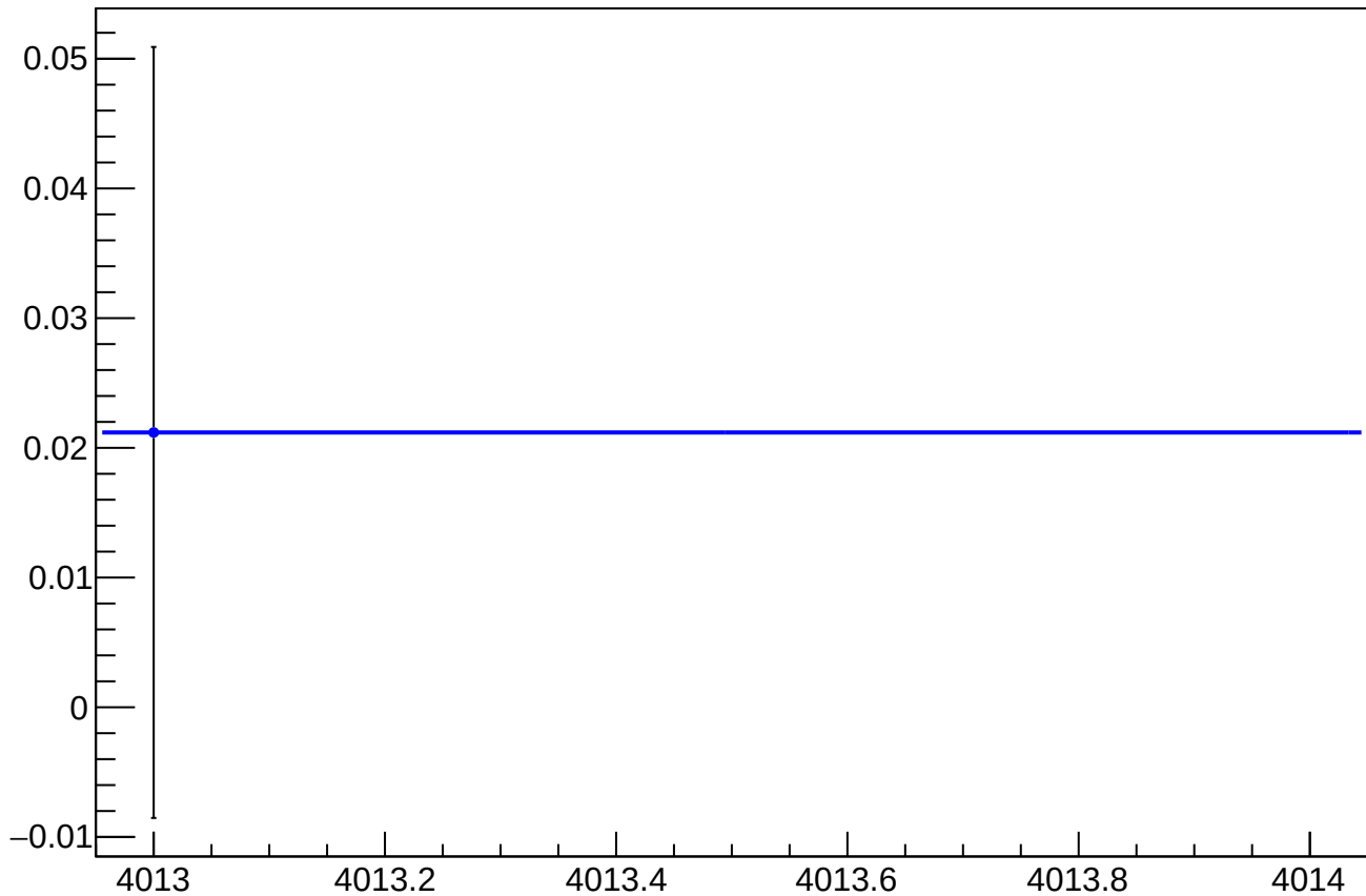
asym_sam1_eigen_dit_vs_eigen_cor_diff_mean vs Slug, Sign Corrected
