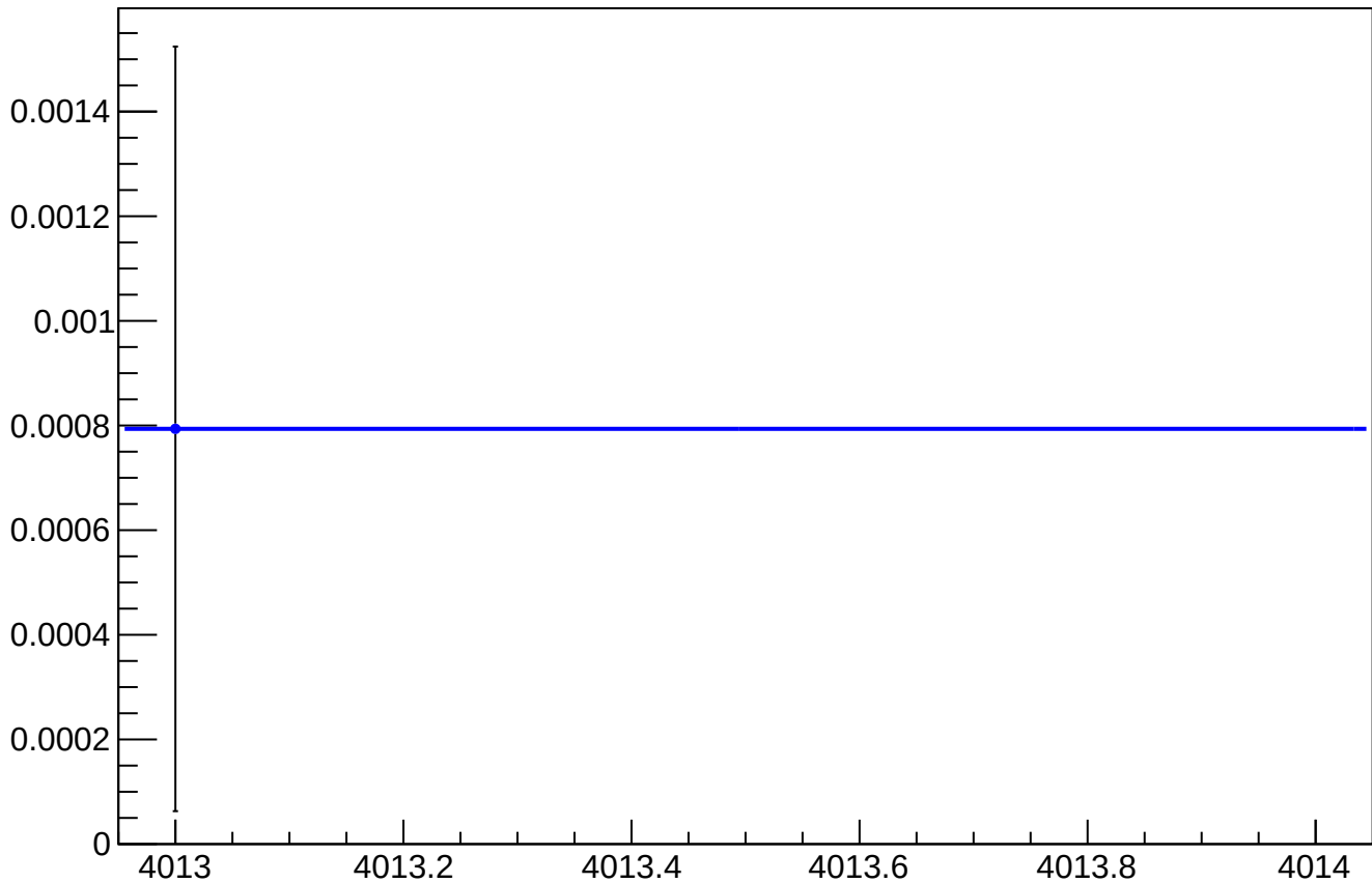
asym_usr_atr1_avg_reg_vs_cor_diff_mean vs Slug, Sign Corrected
