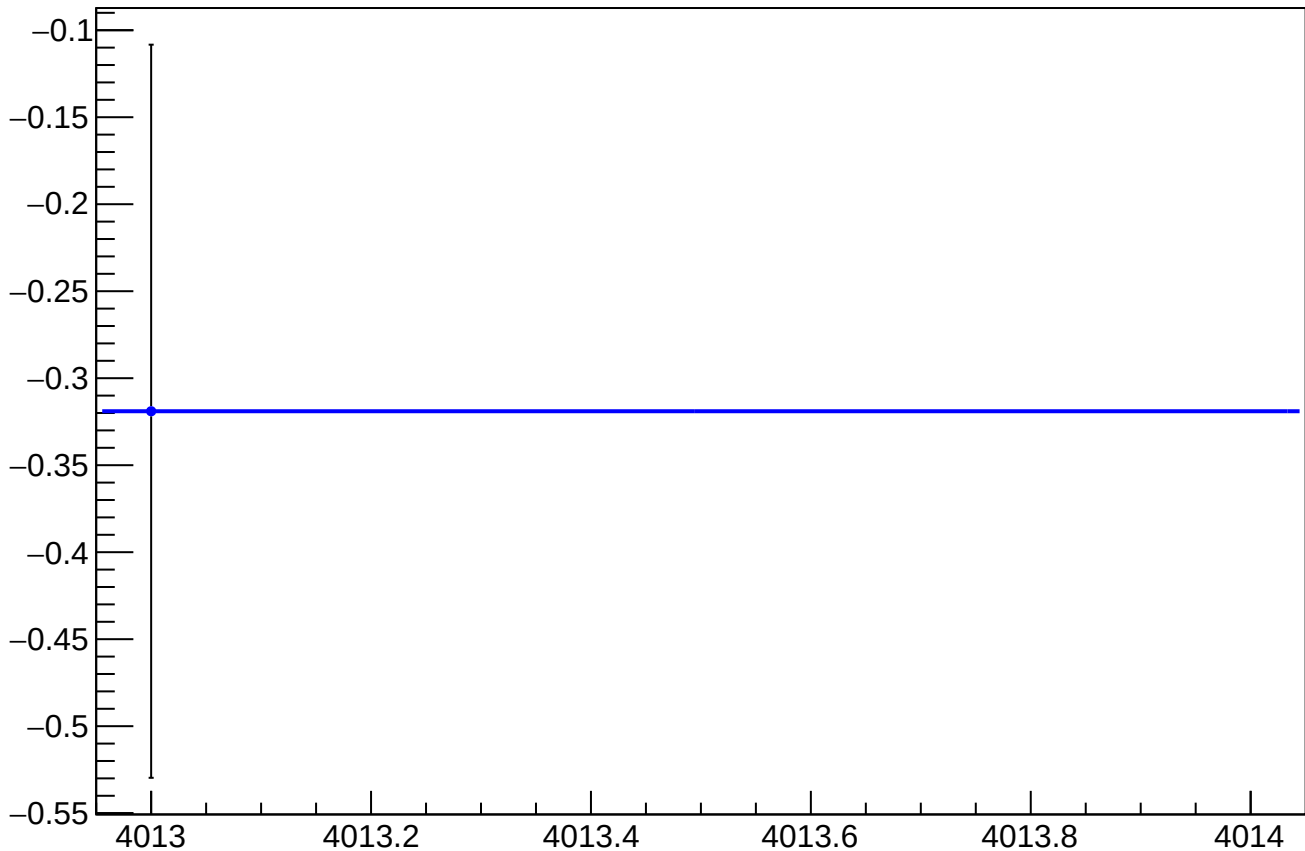
asym_us_avg_at1lr_avg_dd_eigen_dit_vs_cor_diff_mean vs Slug, Sign Corrected
