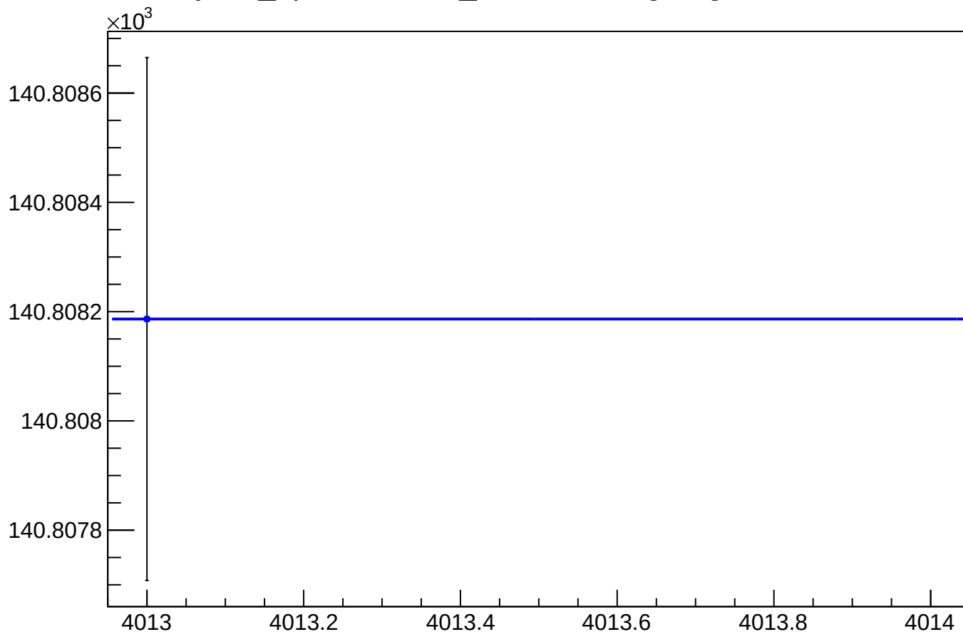
yield_bpm0i02aWS_mean vs Slug, Sign Corrected
