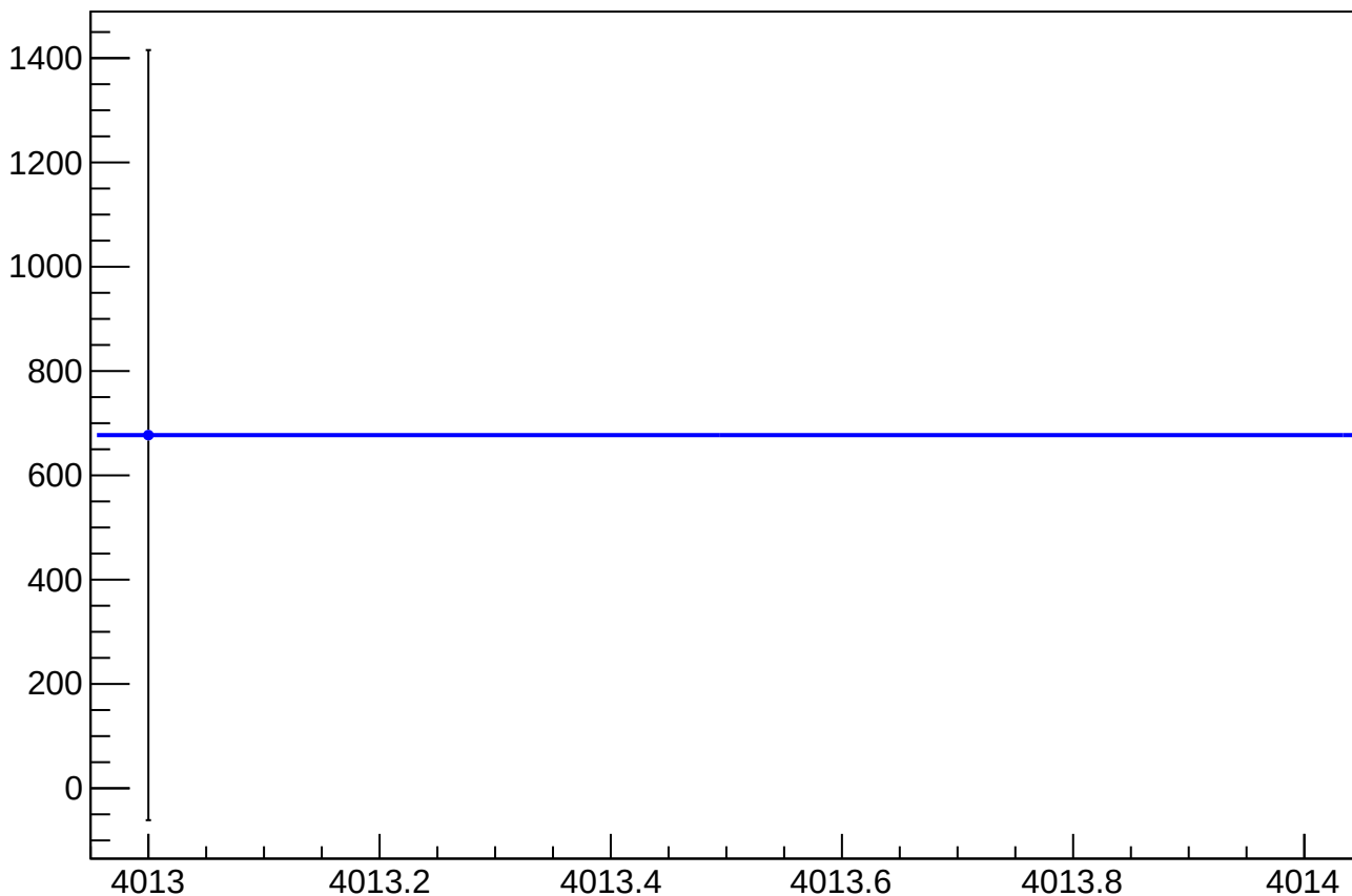
asym_sam_37_26_dd_eigen_cor_correction_mean vs Slug, Sign Corrected
