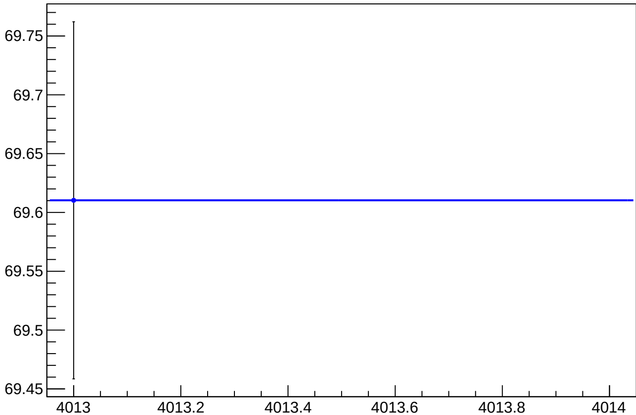
cor_asym_sam_15_48_dd_rms vs Slug, Sign Corrected
