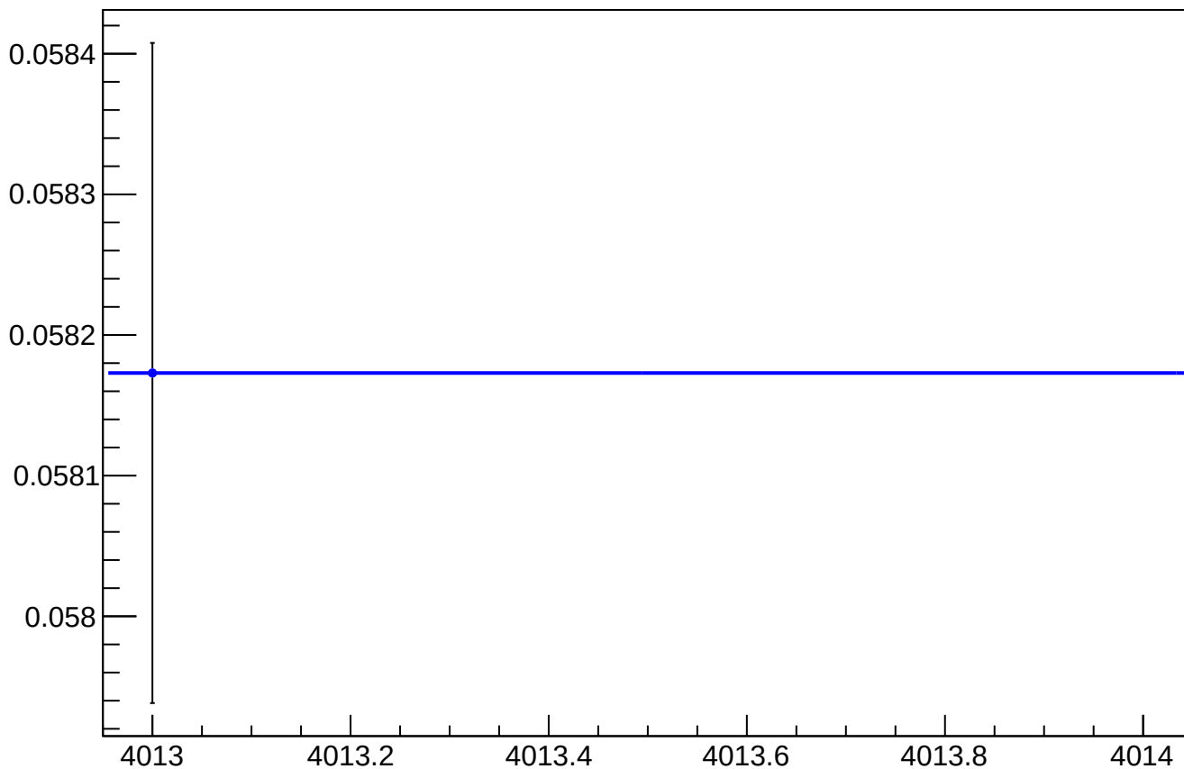
asym_usl_atl1_avg_reg_vs_cor_diff_rms vs Slug, Sign Corrected
