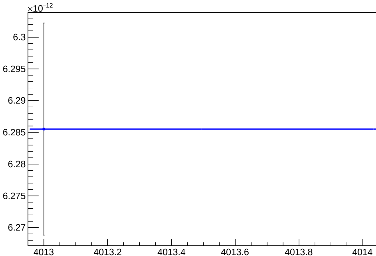
asym_sam_15_37_dd_eigen_cor_vs_cor_diff_rms vs Slug, Sign Corrected
