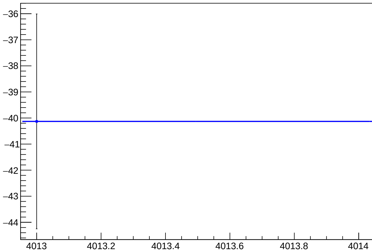
reg_asym_us_dd_atlr_dd_avg_diff_bpm4eX_slope vs Slug, Sign Corrected
