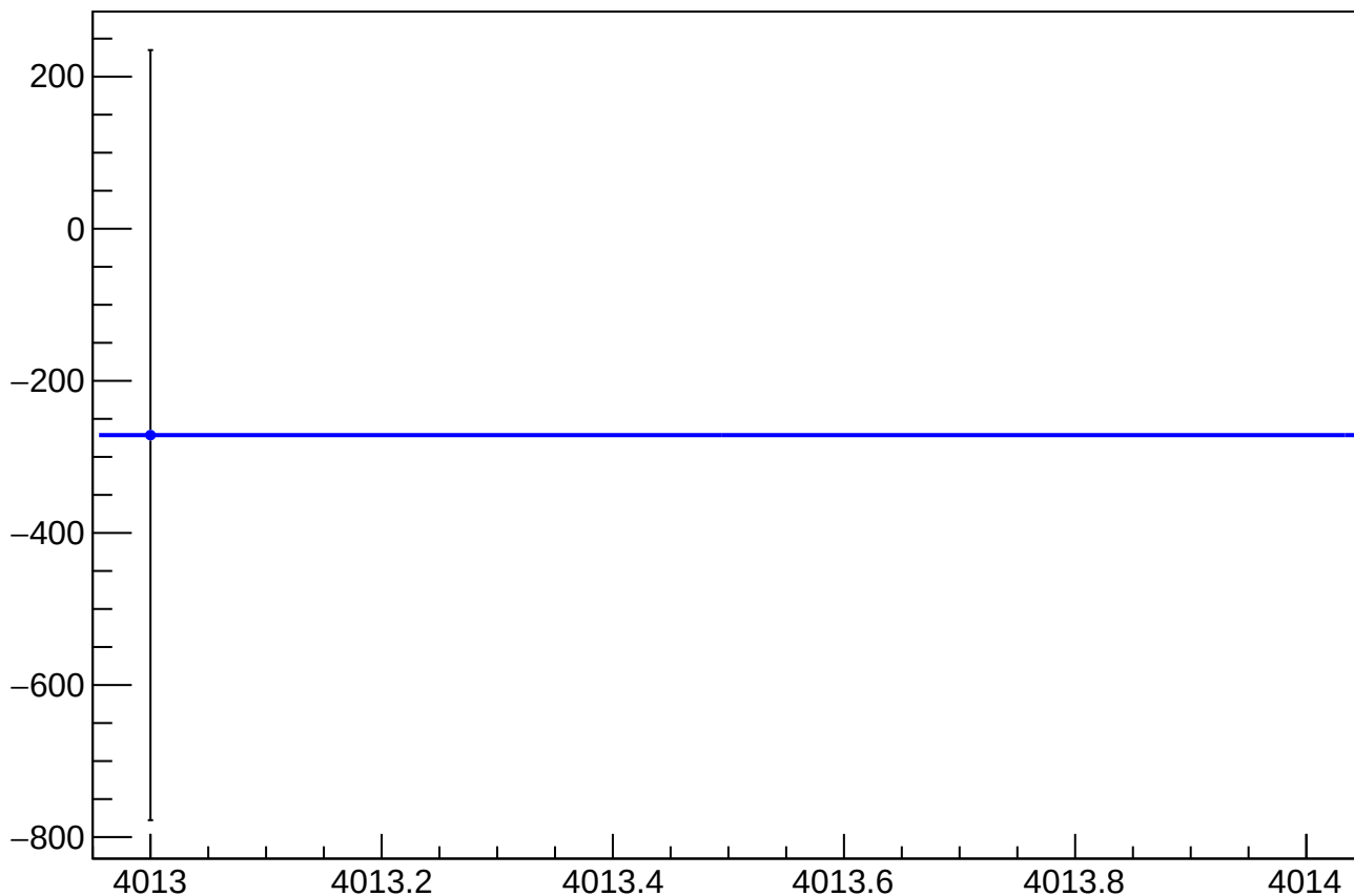
asym_bcm_cav4cQ_an_ds_avg_mean vs Slug, Sign Corrected
