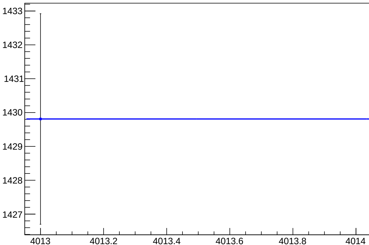
reg_asym_us_avg_atlr_avg_avg_rms vs Slug, Sign Corrected
