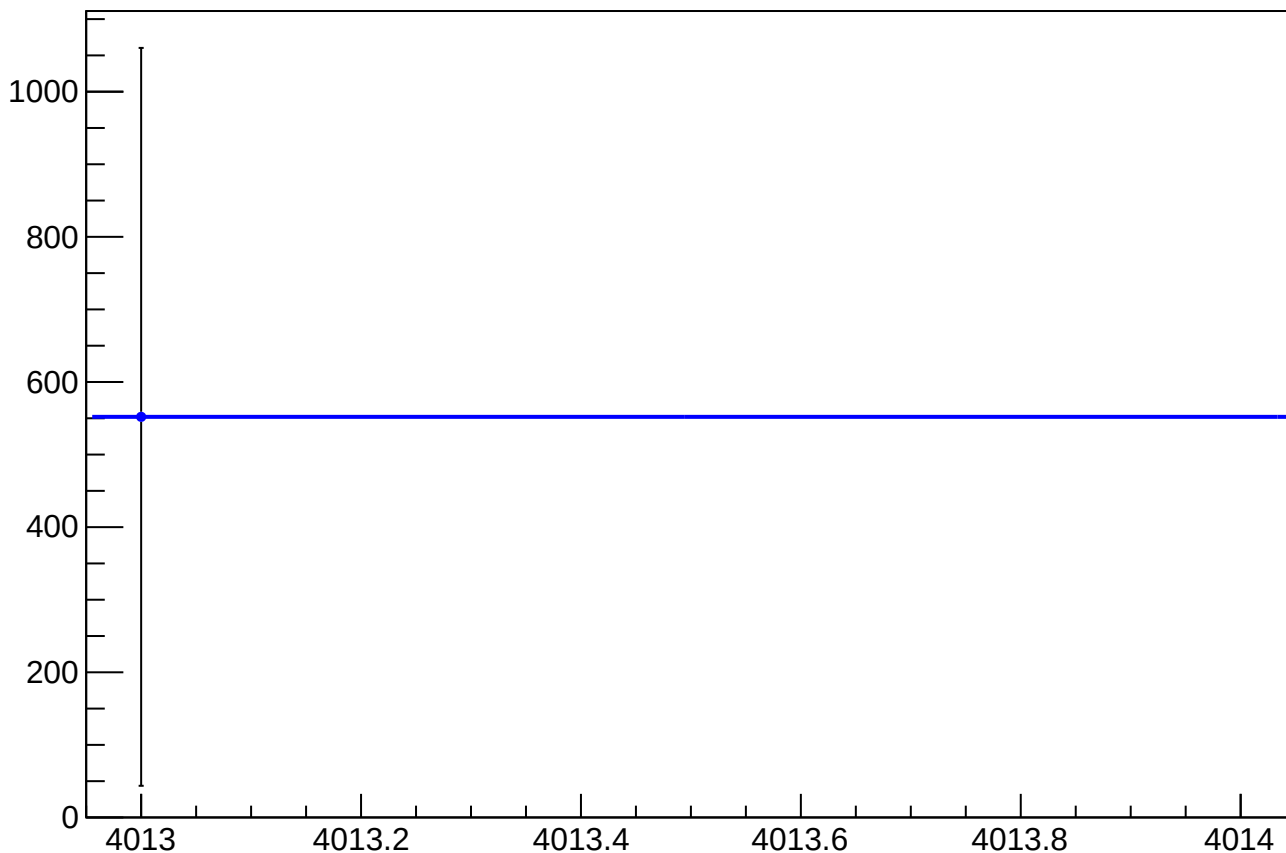
cor_asym_sam_24_68_dd_mean vs Slug, Sign Corrected
