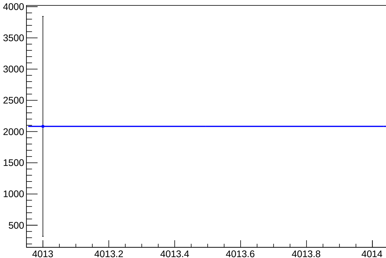
asym_usr_atr1_dd_cor_correction_mean vs Slug, Sign Corrected
