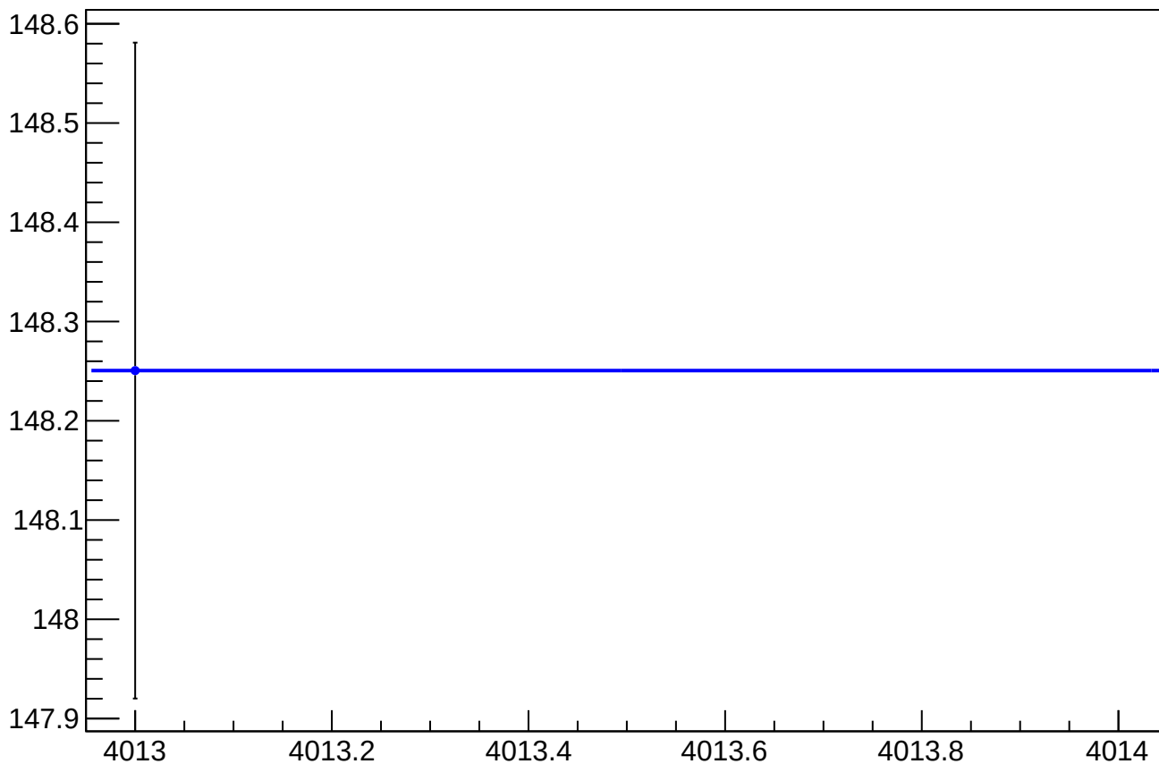
asym_atr1_dit_vs_eigen_cor_diff_rms vs Slug, Sign Corrected
