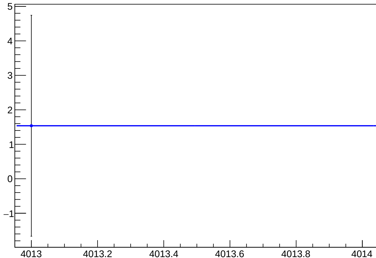
reg_asym_us_dd_at2lr_dd_dd_diff_bpm4aY_slope vs Slug, Sign Corrected
