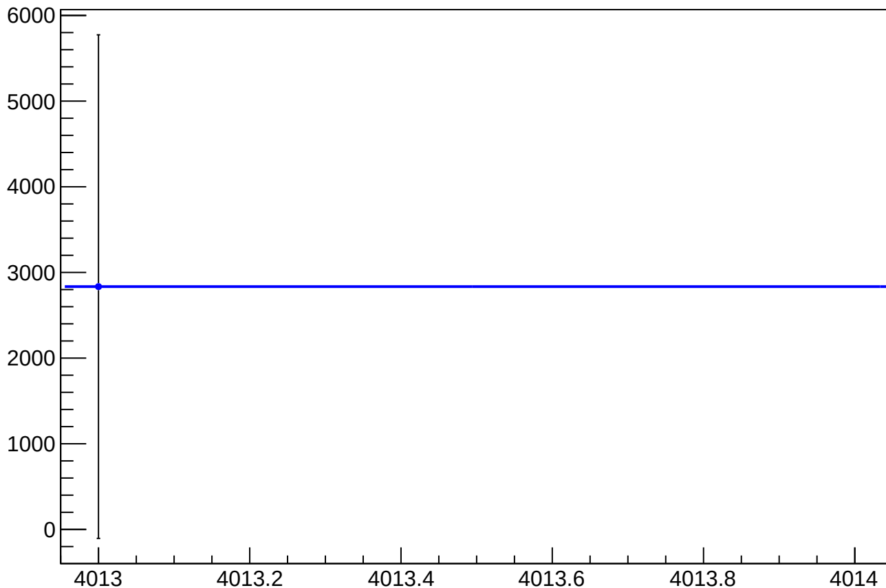
asym_us_dd_atlr_dd_dd_mean vs Slug, Sign Corrected
