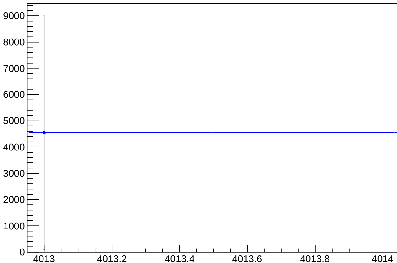
reg_asym_at2_dd_mean vs Slug, Sign Corrected
