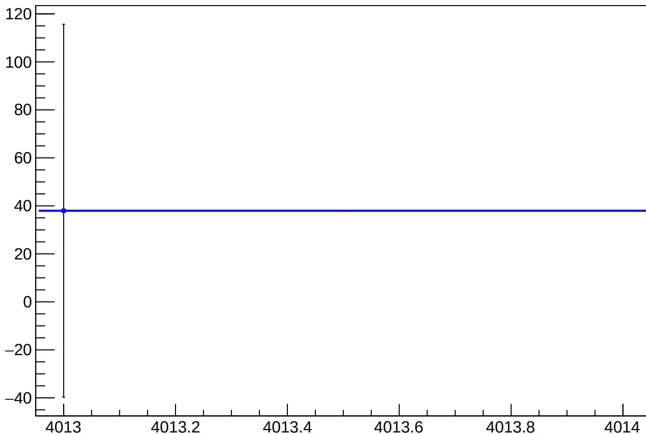
asym_bcm_cav4cQ_an_ds_dd_mean vs Slug, Sign Corrected
