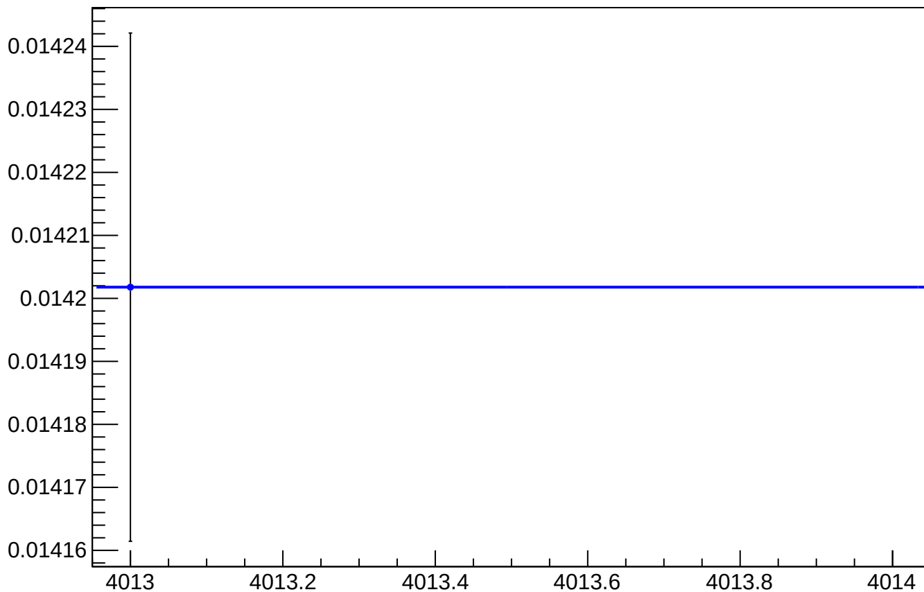
asym_sam3_reg_vs_cor_diff_rms vs Slug, Sign Corrected
