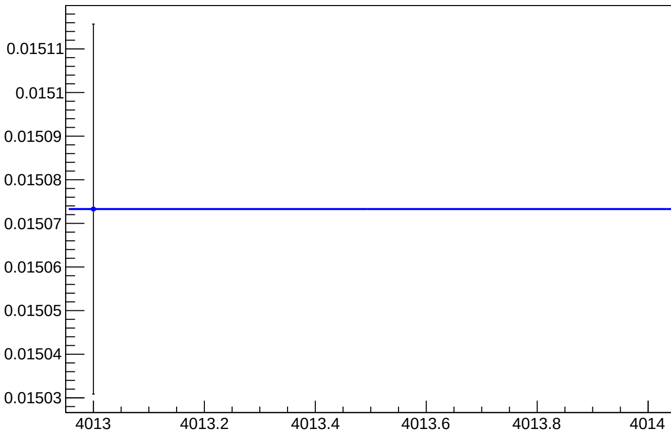
asym_sam_37_dd_reg_vs_cor_diff_rms vs Slug, Sign Corrected
