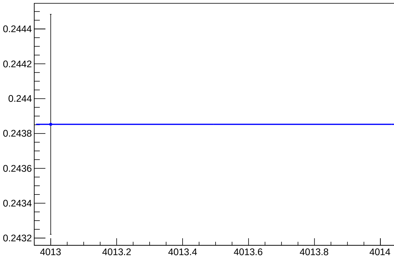
asym_atr1l2_avg_reg_vs_cor_diff_rms vs Slug, Sign Corrected
