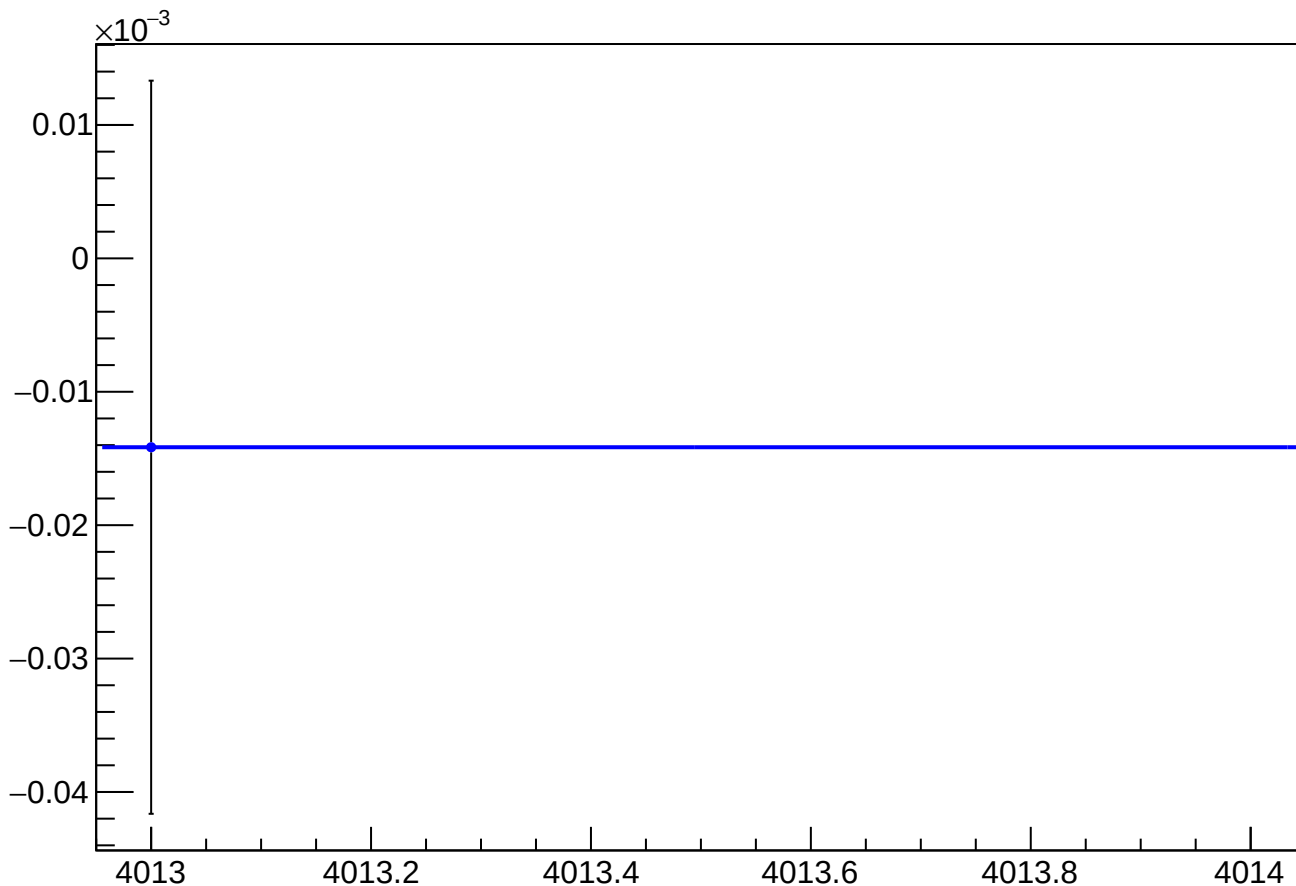
asym_us_avg_atlr_avg_avg_reg_vs_cor_diff_mean vs Slug, Sign Corrected
