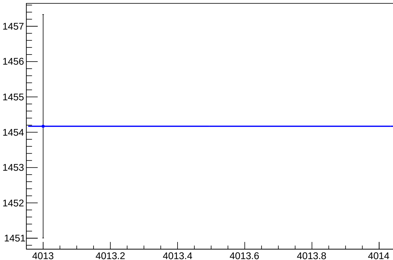
eigen_cor_asym_at2_dd_rms vs Slug, Sign Corrected
