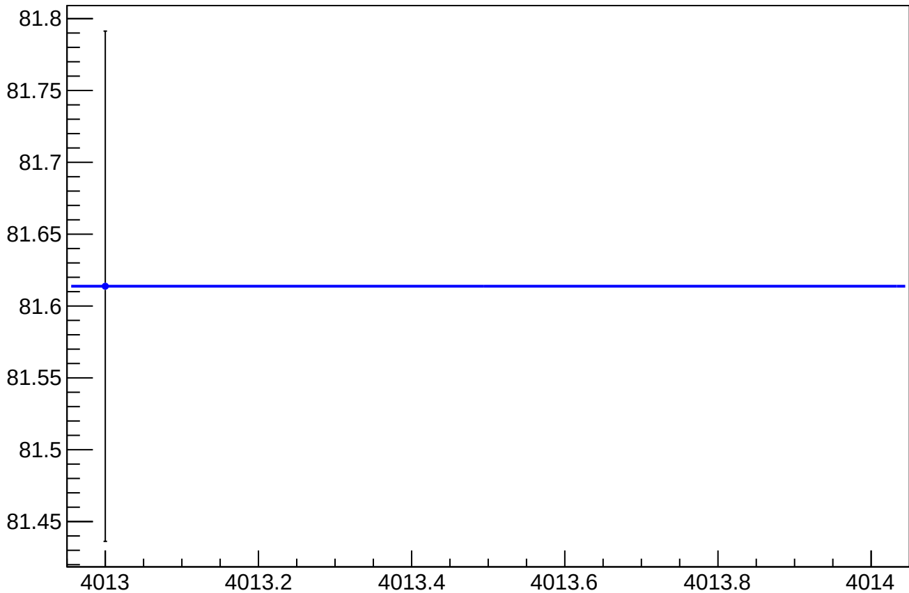
cor_asym_sam_15_37_dd_rms vs Slug, Sign Corrected
