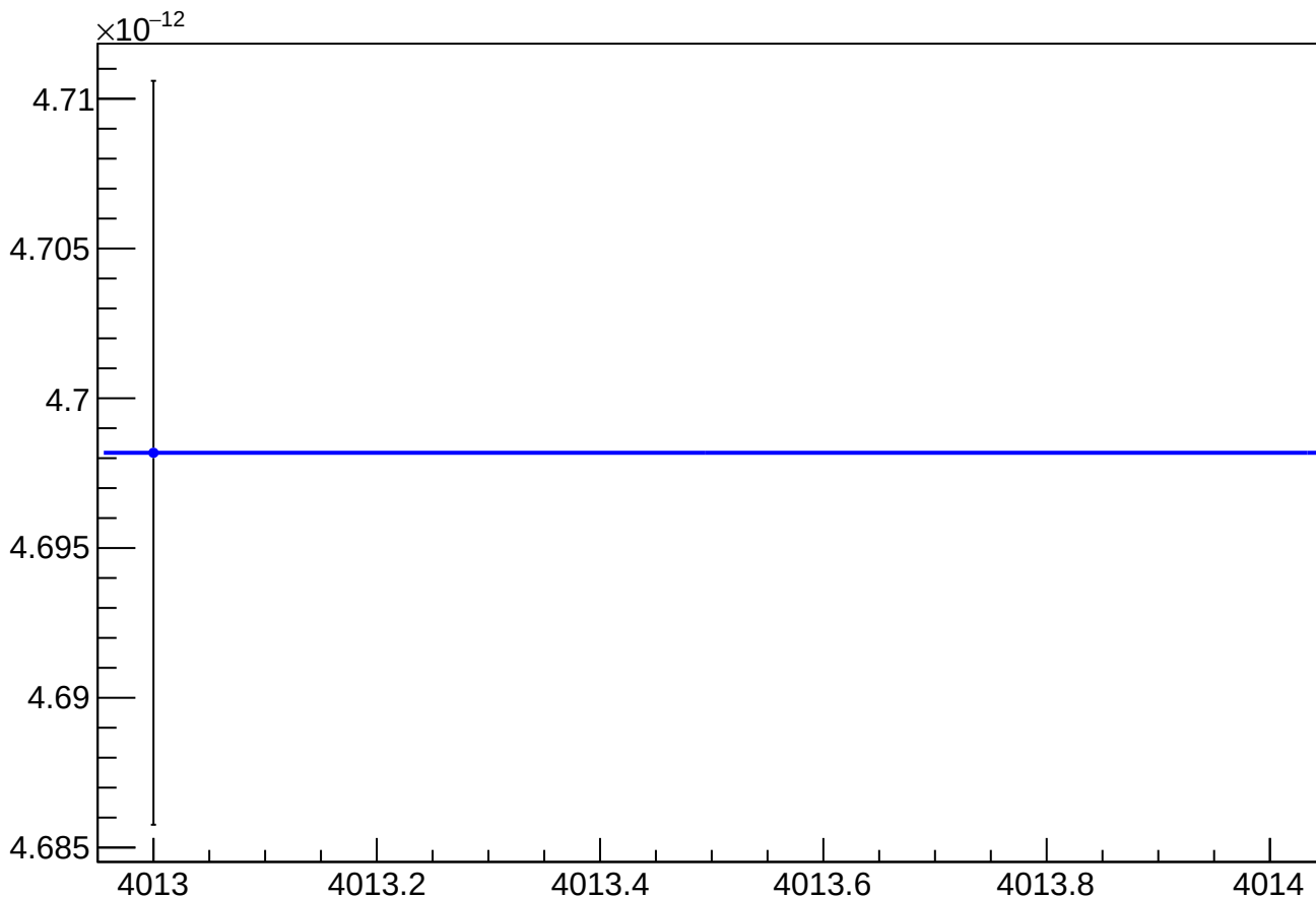
asym_atl_avg_atr_avg_dd_eigen_cor_vs_cor_diff_rms vs Slug, Sign Corrected
