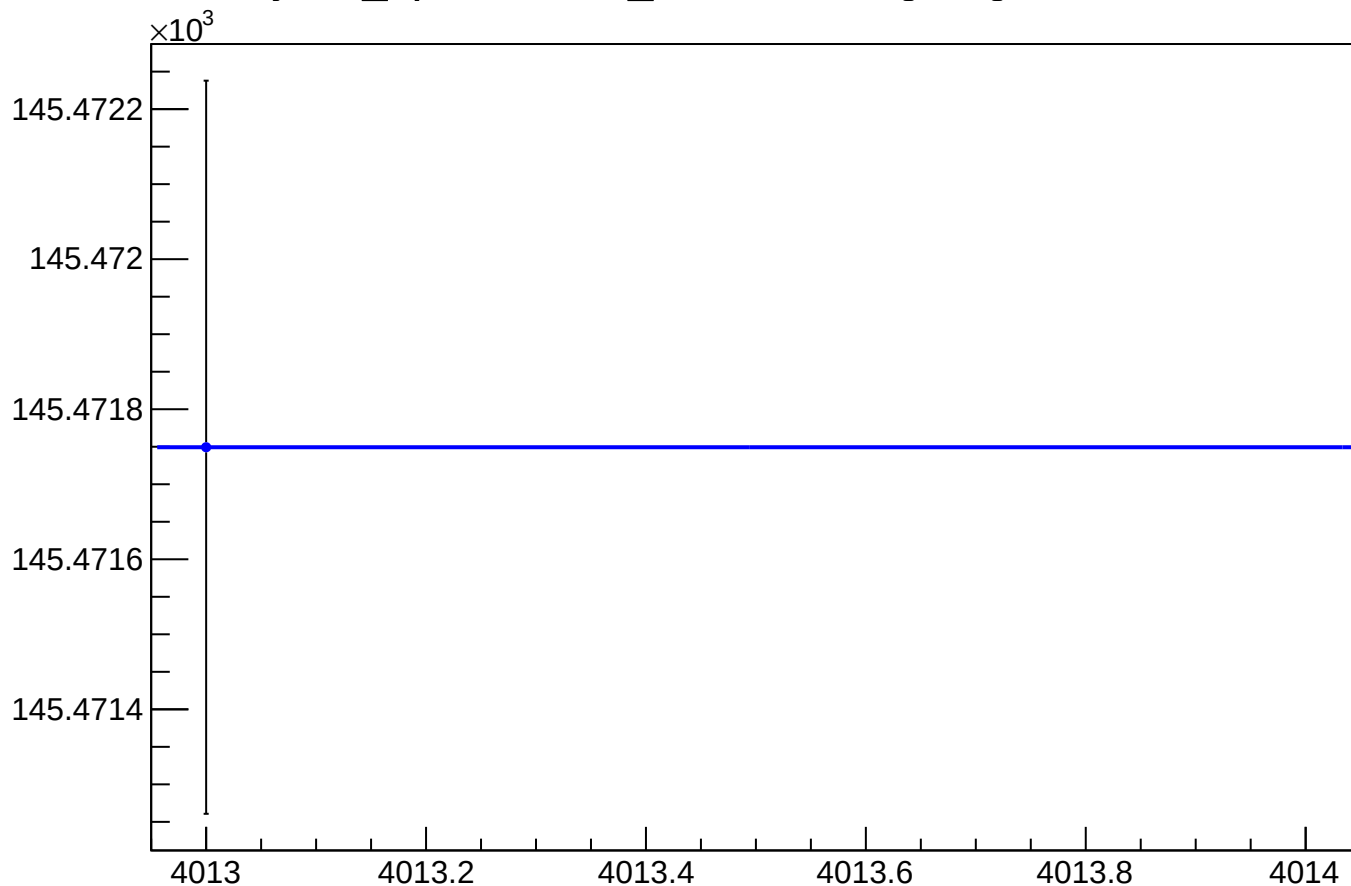
yield_bpm0l08WS_mean vs Slug, Sign Corrected
