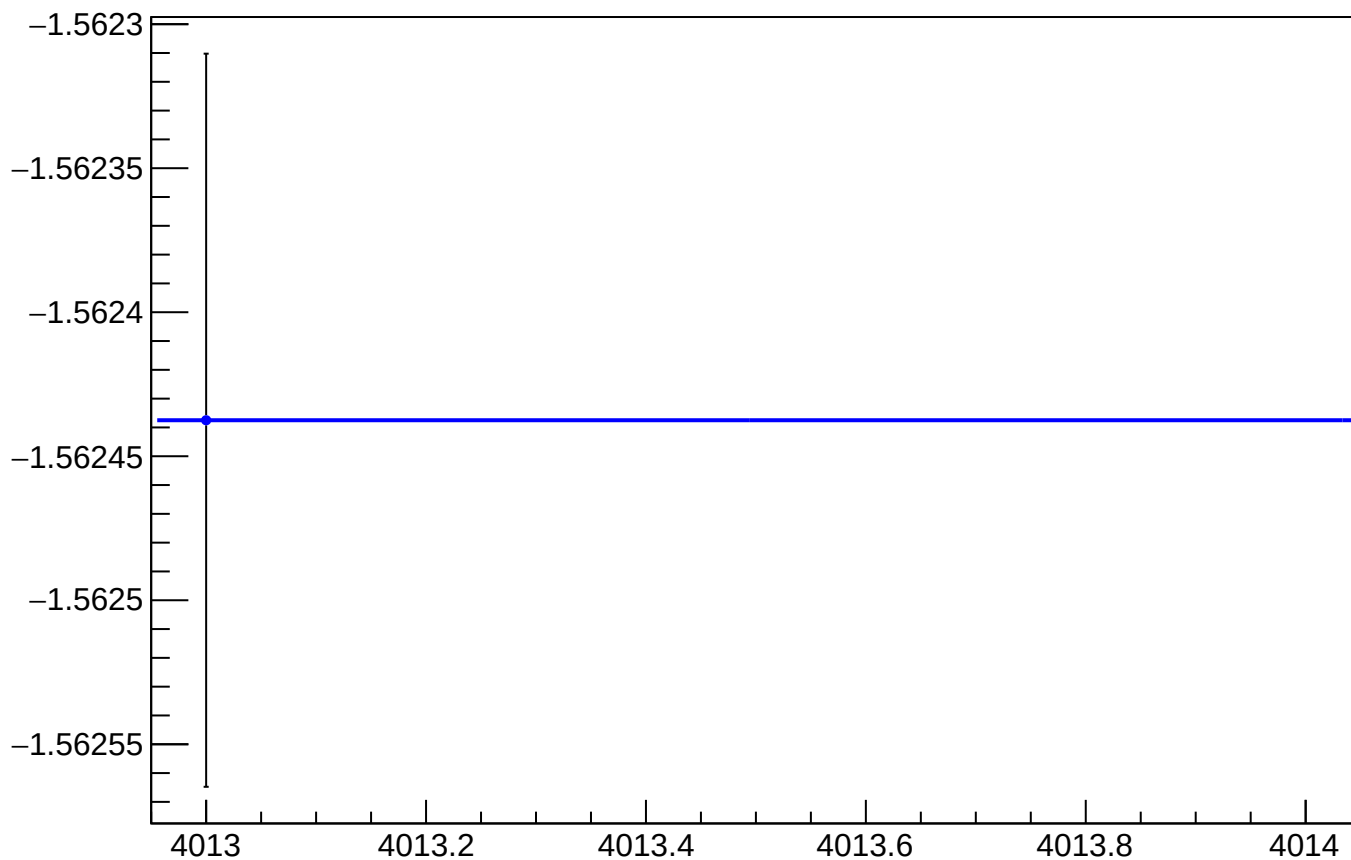
yield_bpm1Y_mean vs Slug, Sign Corrected
