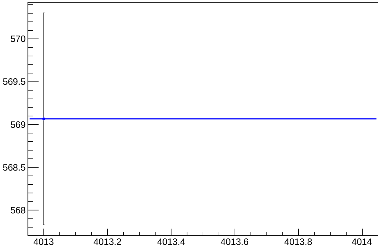
eigen_dit_asym_us_avg_rms vs Slug, Sign Corrected
