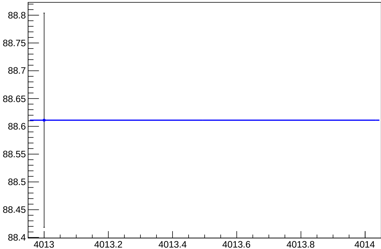
cor_asym_sam_13_57_dd_rms vs Slug, Sign Corrected
