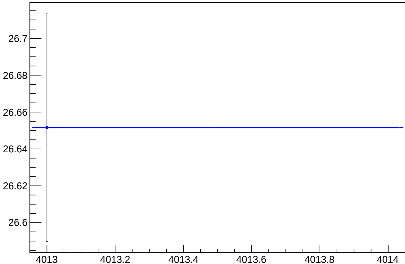
asym_sam_15_48_dd_eigen_dit_vs_cor_diff_rms vs Slug, Sign Corrected
