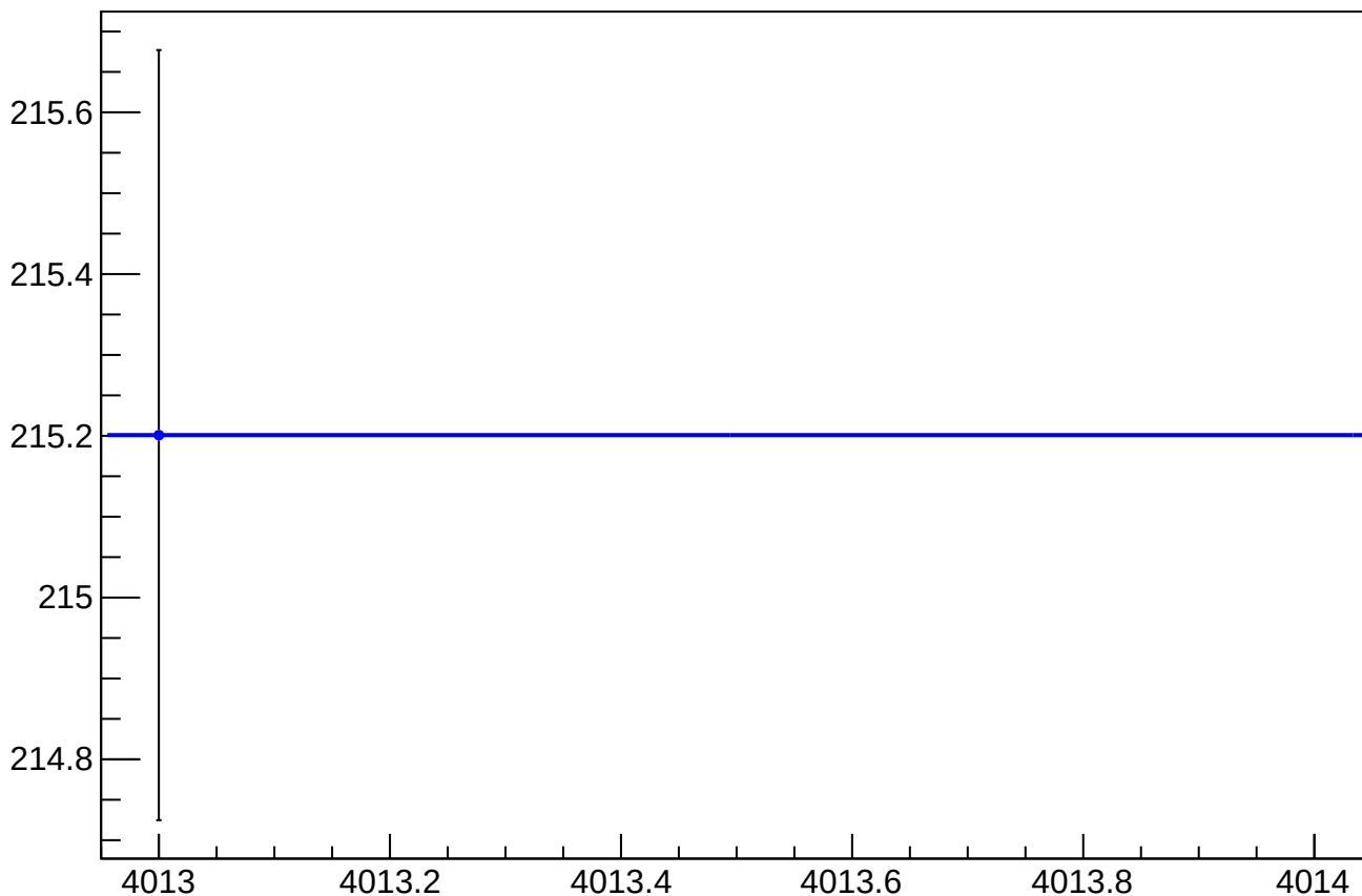
asym_usr_atr2_dd_dit_vs_cor_diff_rms vs Slug, Sign Corrected
