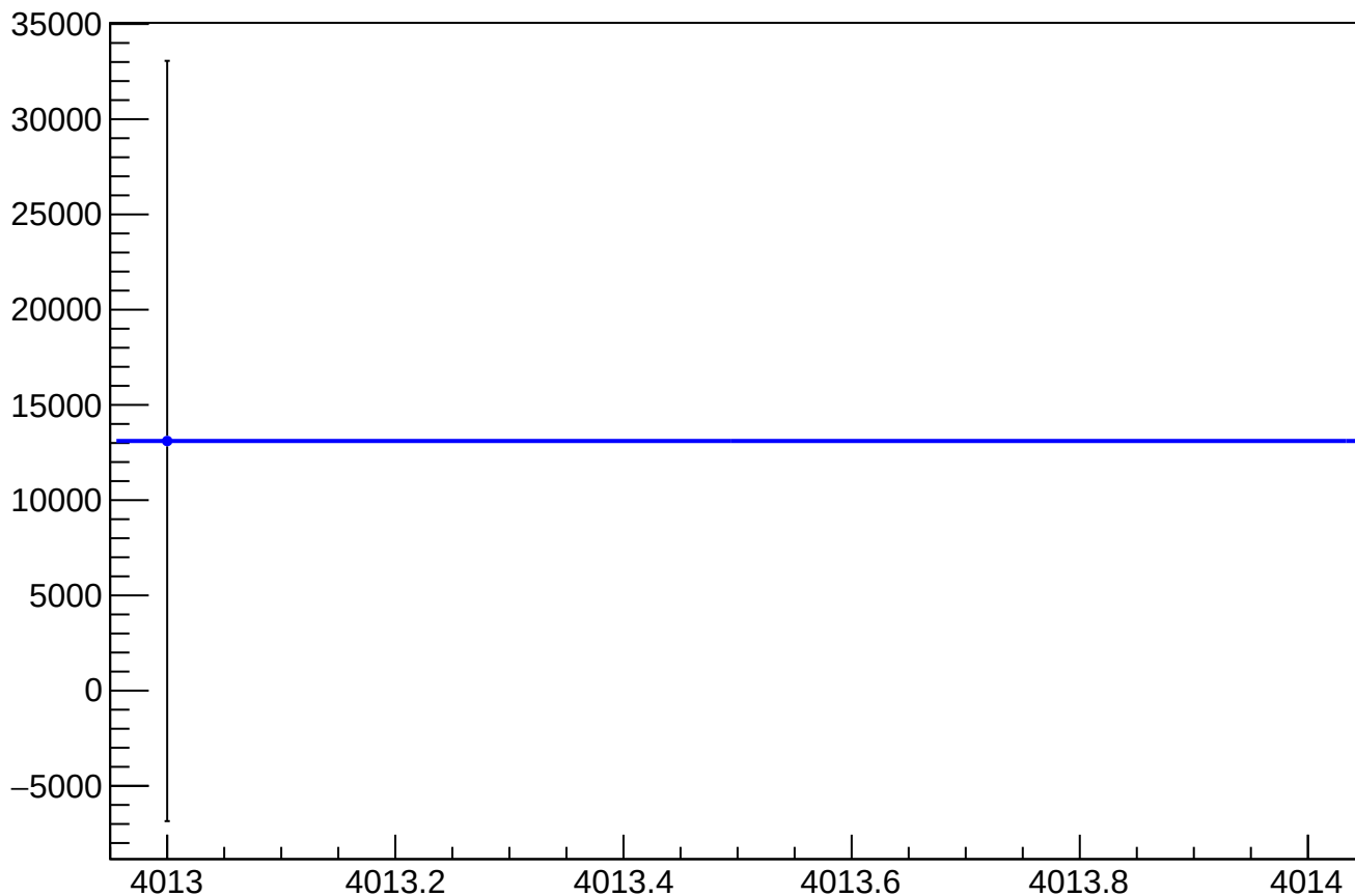
asym_atl_avg_atr_avg_avg_eigen_dit_correction_mean vs Slug, Sign Corrected
