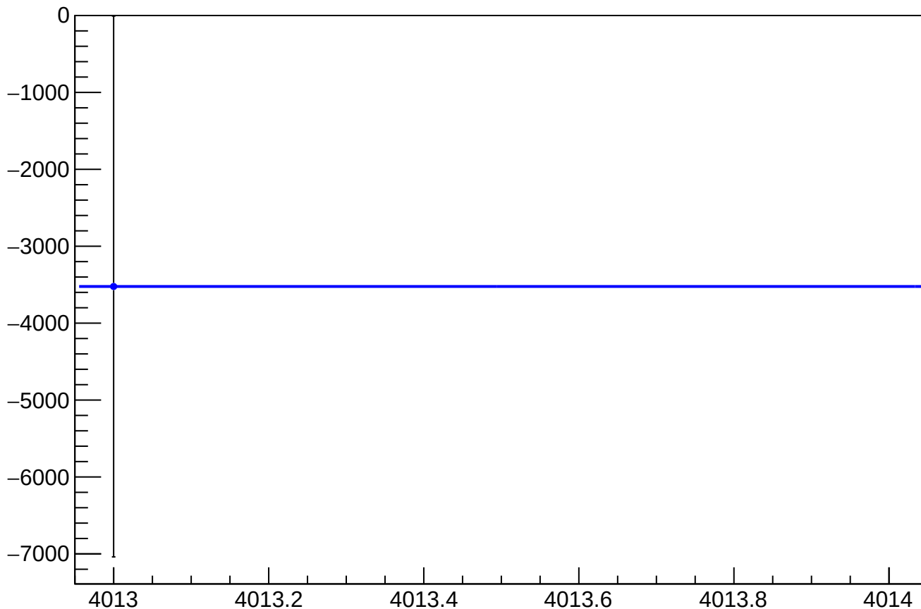
dit_asym_usl_atl1_avg_mean vs Slug, Sign Corrected
