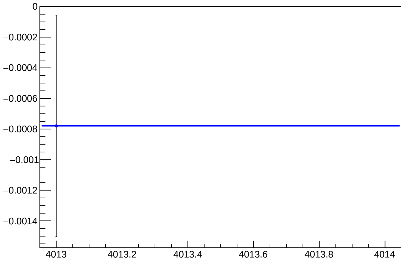
asym_atl_avg_atr_avg_dd_reg_vs_cor_diff_mean vs Slug, Sign Corrected
