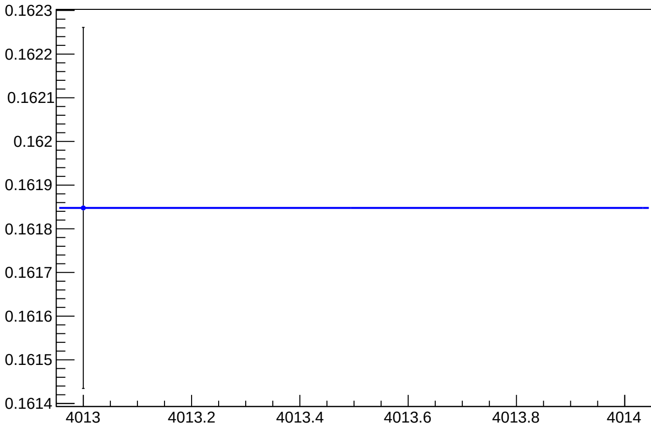
asym_usr_atr1_dd_reg_vs_cor_diff_rms vs Slug, Sign Corrected
