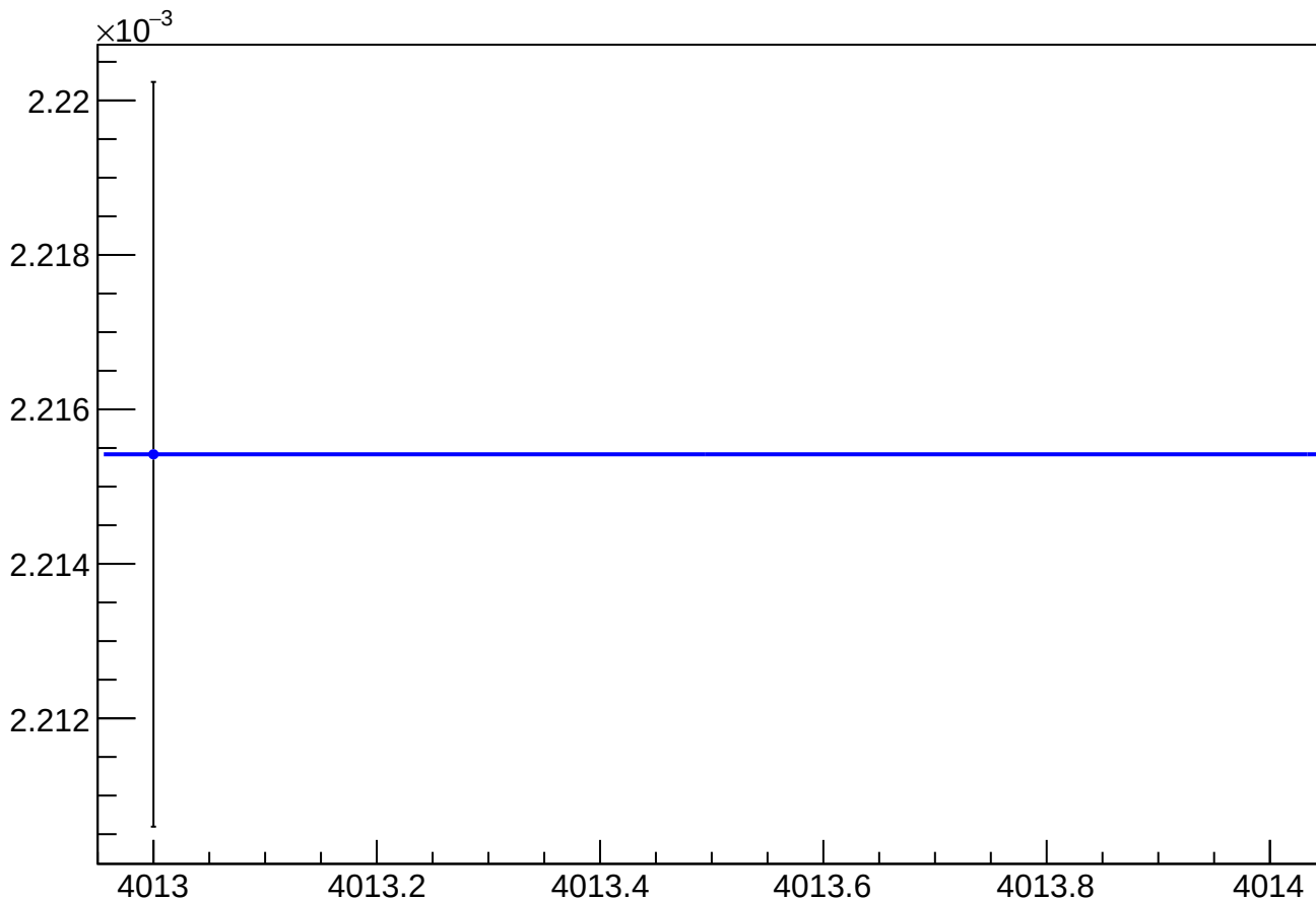
asym_sam7_eigen_dit_vs_dit_diff_rms vs Slug, Sign Corrected
