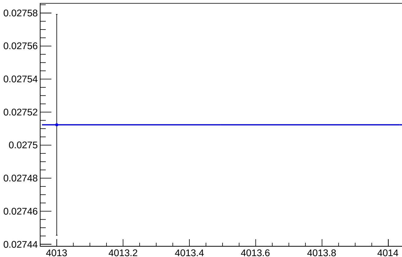
asym_sam_2468_avg_reg_vs_cor_diff_rms vs Slug, Sign Corrected
