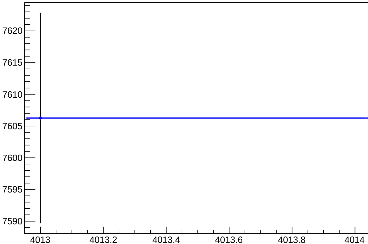
asym_us_avg_atlr_avg_avg_reg_correction_rms vs Slug, Sign Corrected
