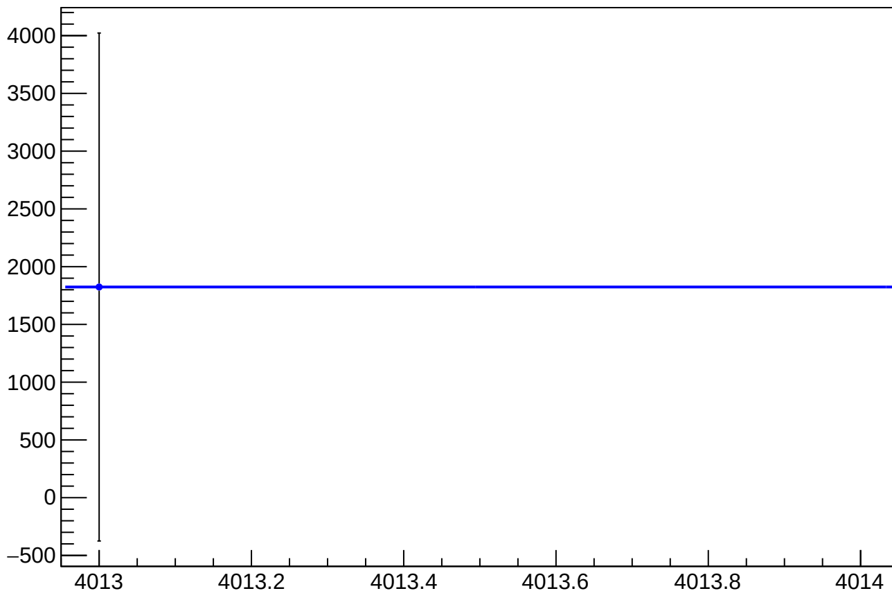
asym_at1_dd_eigen_cor_correction_mean vs Slug, Sign Corrected
