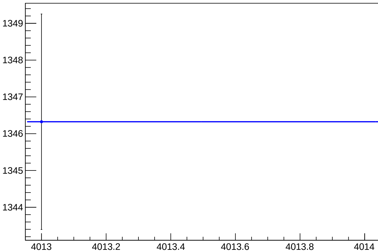
eigen_dit_asym_us_avg_at1lr_avg_dd_rms vs Slug, Sign Corrected
