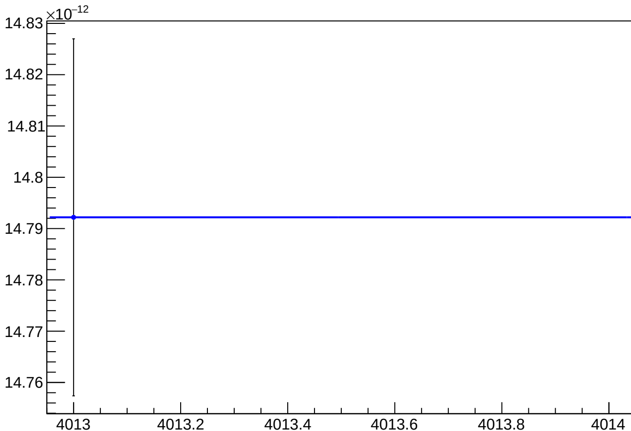
asym_sam_26_48_dd_eigen_cor_vs_cor_diff_rms vs Slug, Sign Corrected
