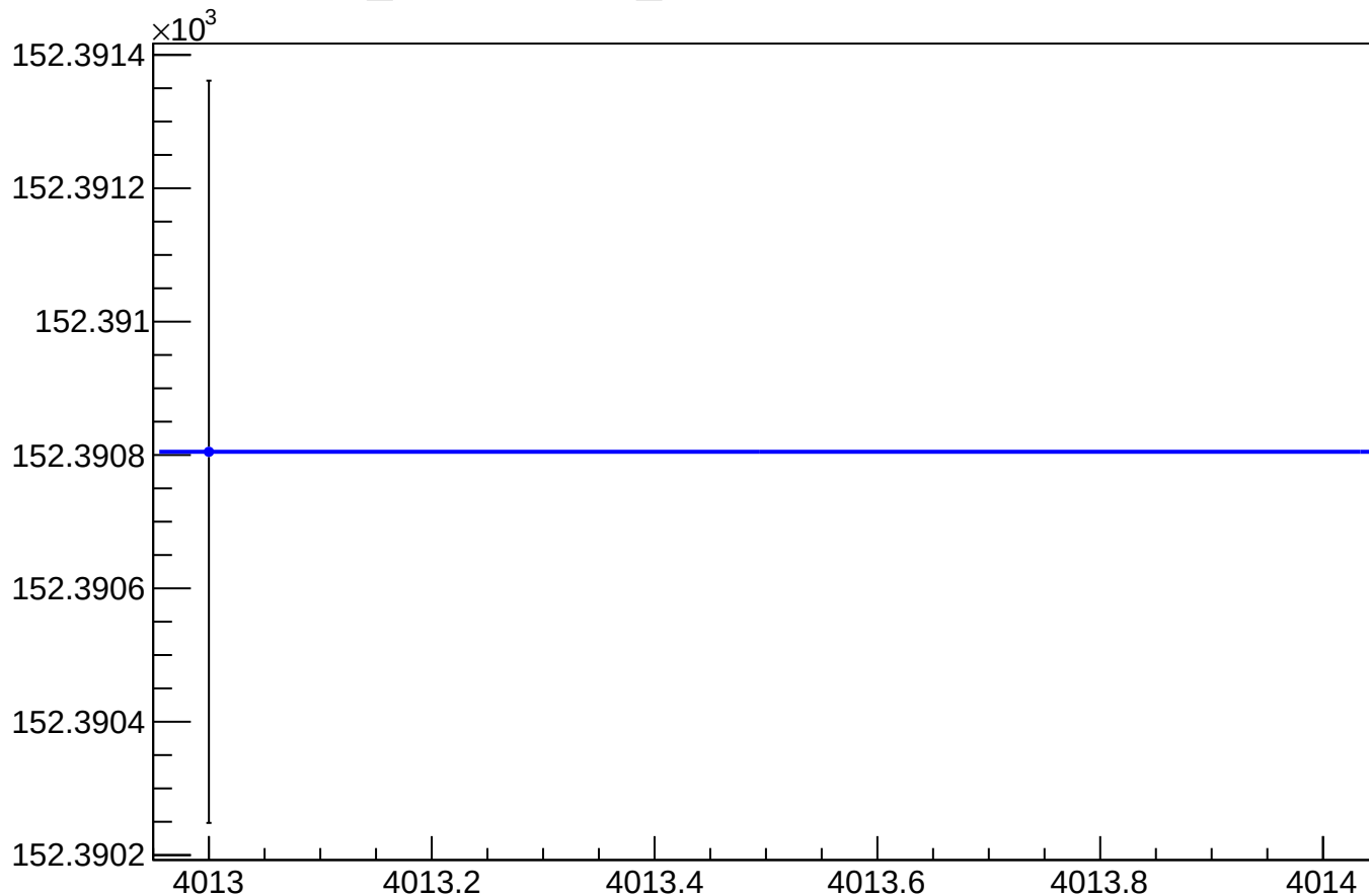
yield_bpm1i02WS_mean vs Slug, Sign Corrected
