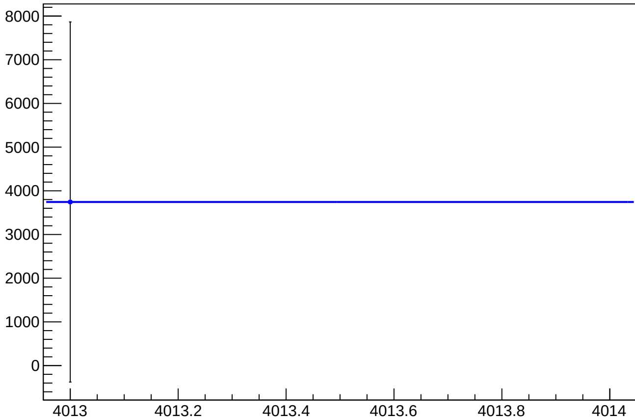
eigen_cor_asym_us_dd_at1lr_dd_dd_mean vs Slug, Sign Corrected
