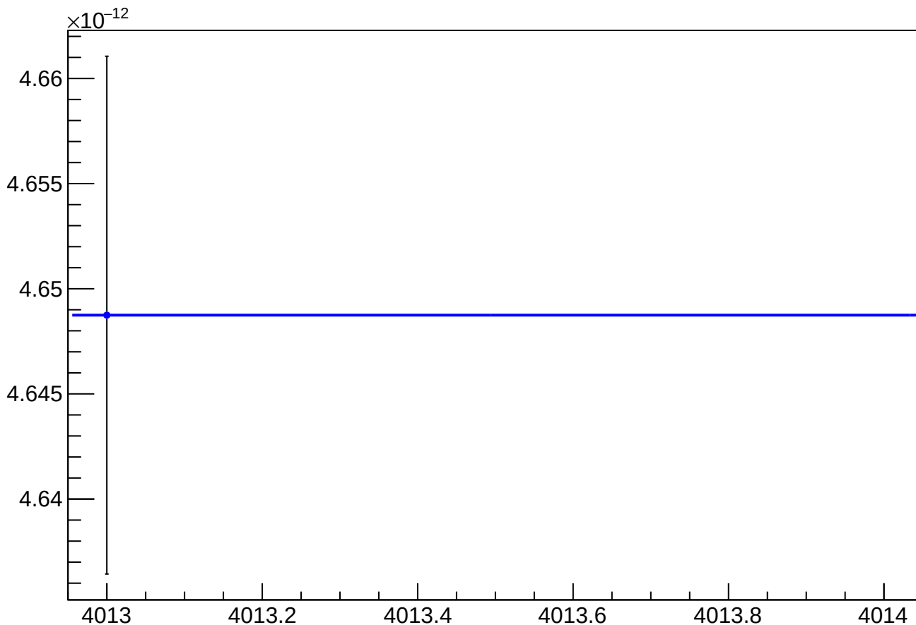
asym_sam_1526_avg_eigen_cor_vs_cor_diff_rms vs Slug, Sign Corrected
