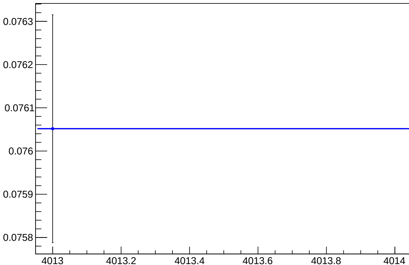
asym_us_avg_at1lr_avg_dd_reg_vs_cor_diff_rms vs Slug, Sign Corrected
