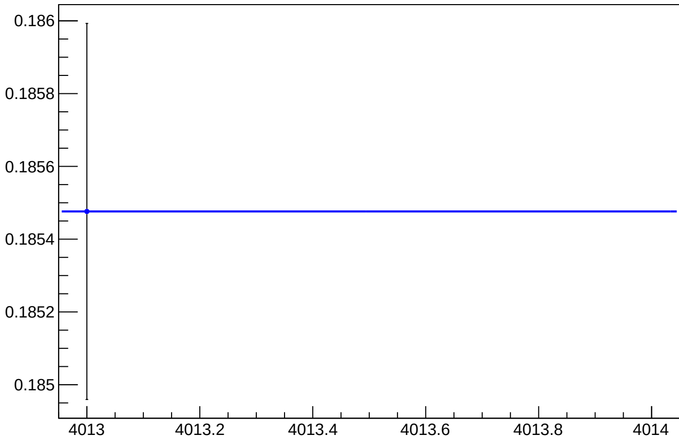
asym_usr_atr1_avg_reg_vs_cor_diff_rms vs Slug, Sign Corrected
