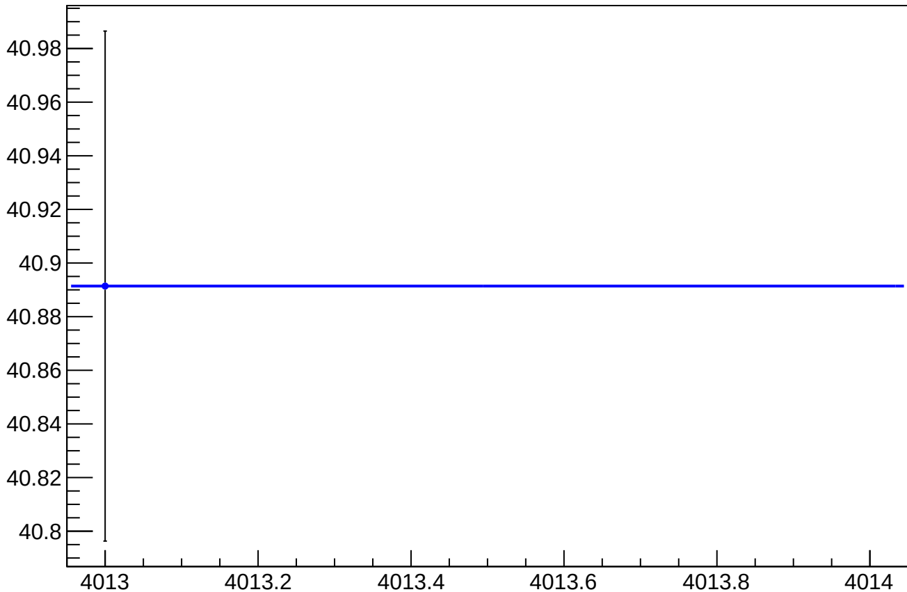
asym_sam_48_dd_eigen_dit_vs_cor_diff_rms vs Slug, Sign Corrected
