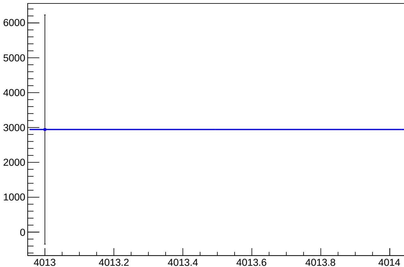
cor_asym_atl_avg_atr_avg_avg_mean vs Slug, Sign Corrected
