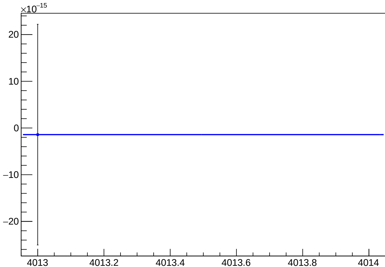
asym_sam_15_37_dd_eigen_cor_vs_cor_diff_mean vs Slug, Sign Corrected
