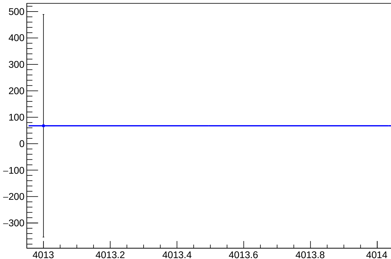
eigen_cor_asym_sam_37_avg_mean vs Slug, Sign Corrected
