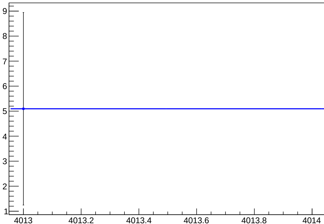
reg_asym_us_dd_at1lr_dd_avg_diff_bpm4eY_slope vs Slug, Sign Corrected
