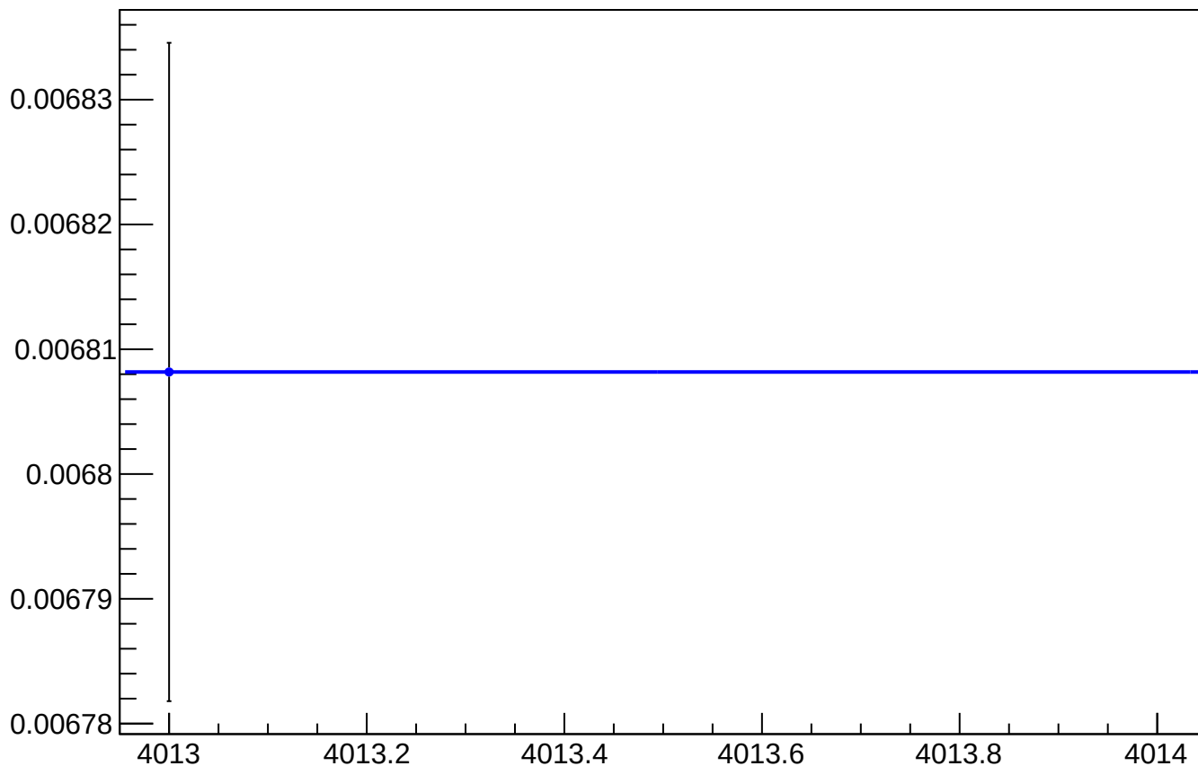
asym_sam5_reg_vs_cor_diff_rms vs Slug, Sign Corrected
