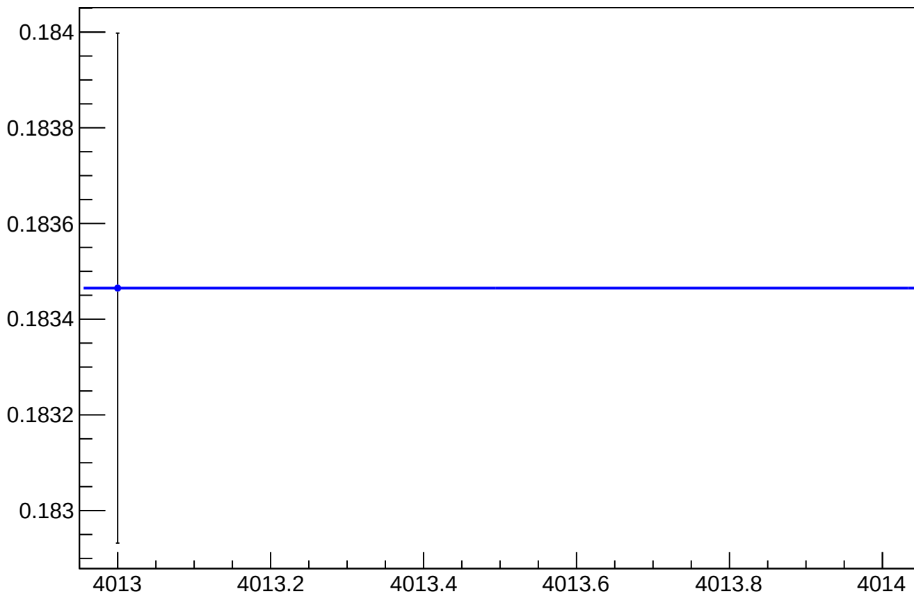
asym_us_avg_at2lr_avg_avg_reg_vs_cor_diff_rms vs Slug, Sign Corrected
