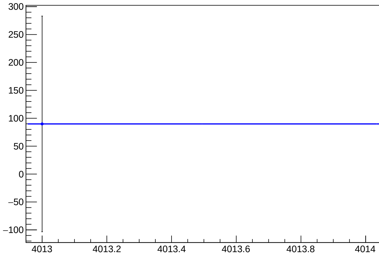
asym_atl1r2_dd_atl2r1_dd_avg_reg_correction_mean vs Slug, Sign Corrected
