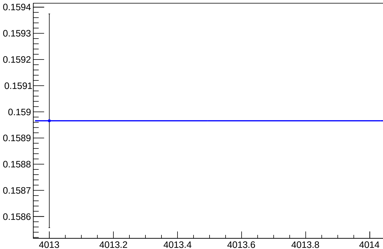
asym_usr_atr2_dd_reg_vs_cor_diff_rms vs Slug, Sign Corrected
