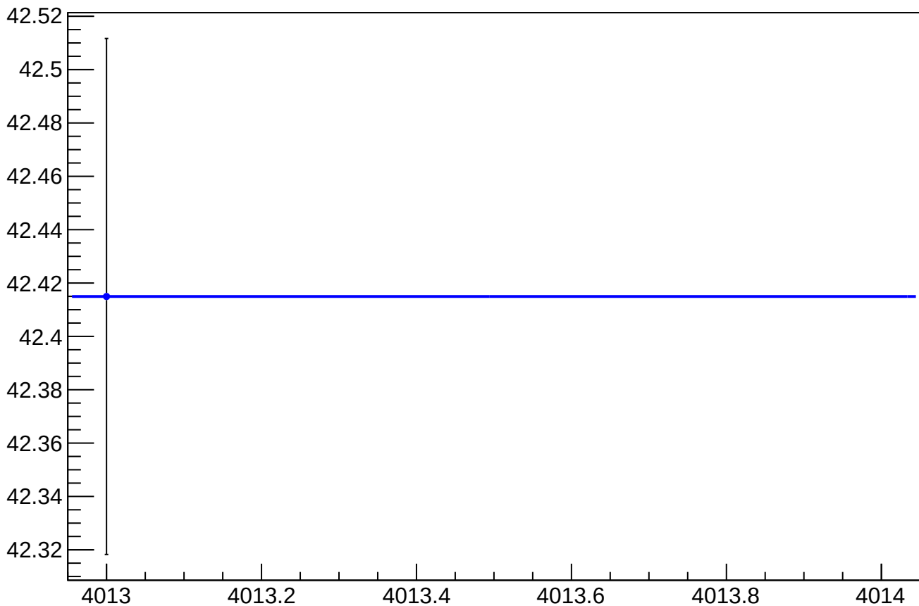
asym_sam_1548_avg_eigen_dit_vs_eigen_cor_diff_rms vs Slug, Sign Corrected
