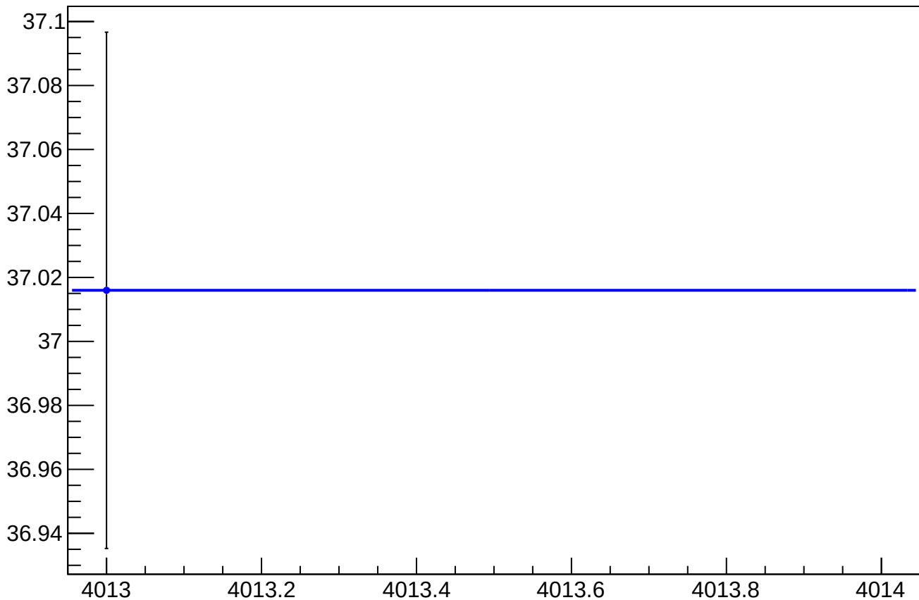
asym_sam_15_26_dd_eigen_dit_vs_eigen_cor_diff_rms vs Slug, Sign Corrected
