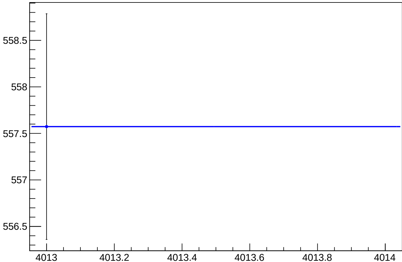
eigen_dit_asym_us_dd_rms vs Slug, Sign Corrected
