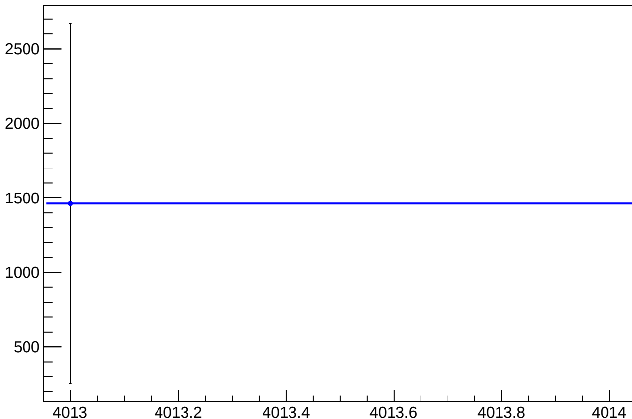
asym_sam_15_37_dd_reg_correction_mean vs Slug, Sign Corrected
