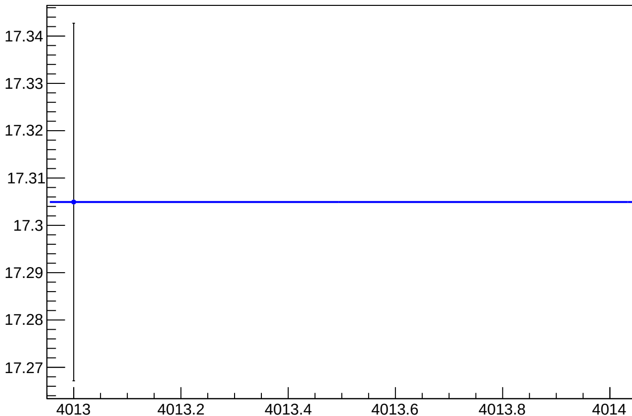
asym_sam_13_57_dd_dit_vs_cor_diff_rms vs Slug, Sign Corrected
