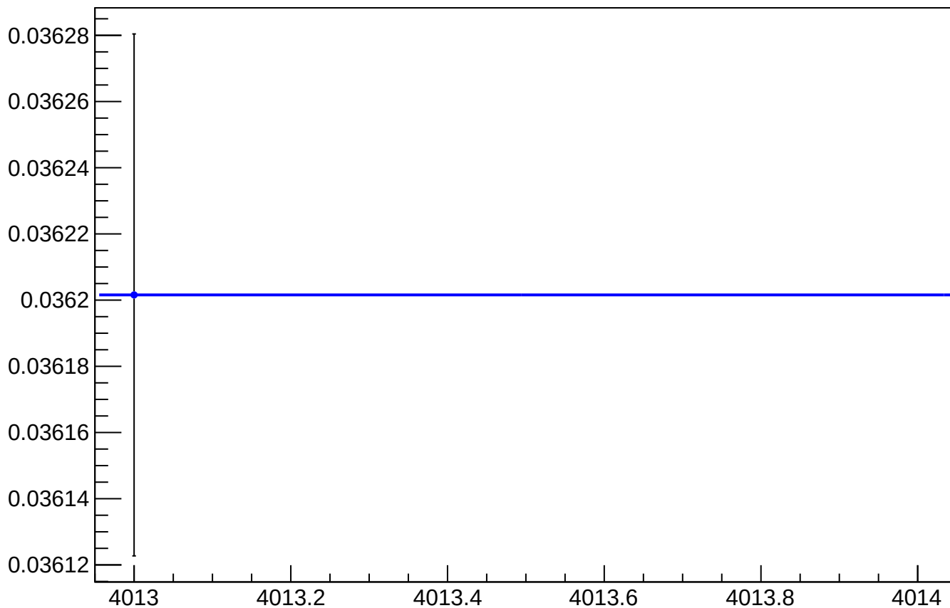
asym_atr2_eigen_dit_vs_dit_diff_rms vs Slug, Sign Corrected
