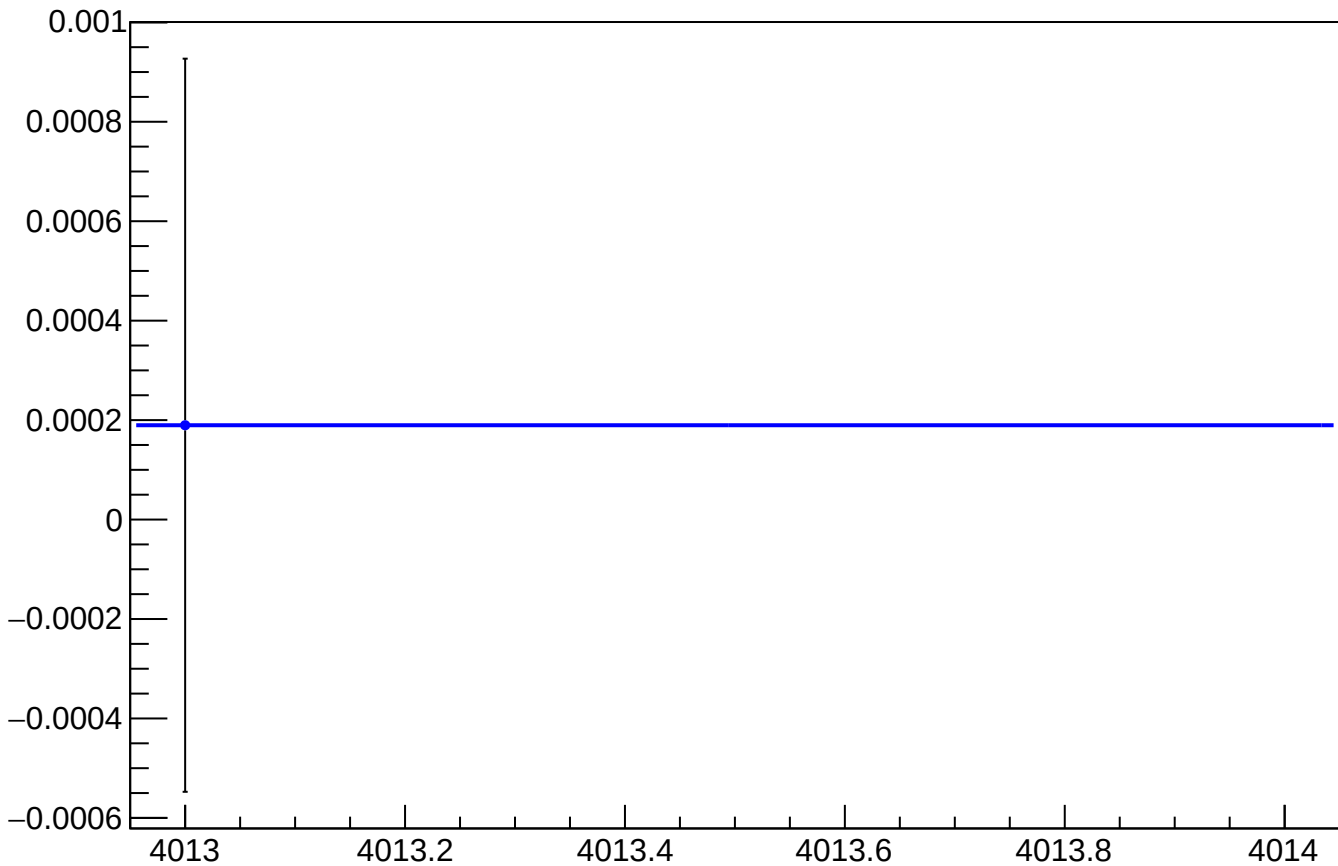
asym_atl_dd_reg_vs_cor_diff_mean vs Slug, Sign Corrected
