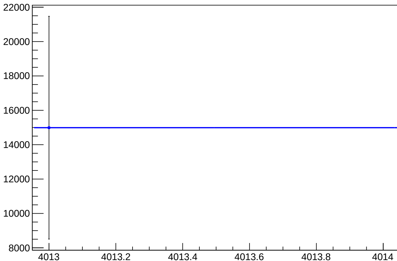
eigen_cor_asym_atr1_mean vs Slug, Sign Corrected
