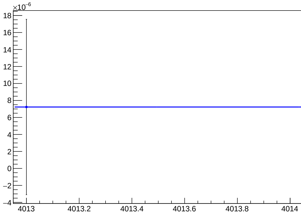
asym_sam_3748_avg_eigen_dit_vs_dit_diff_mean vs Slug, Sign Corrected
