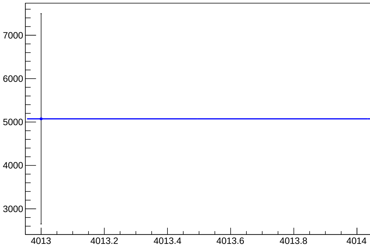
overload_cor_asym_usr_mean vs Slug, Sign Corrected
