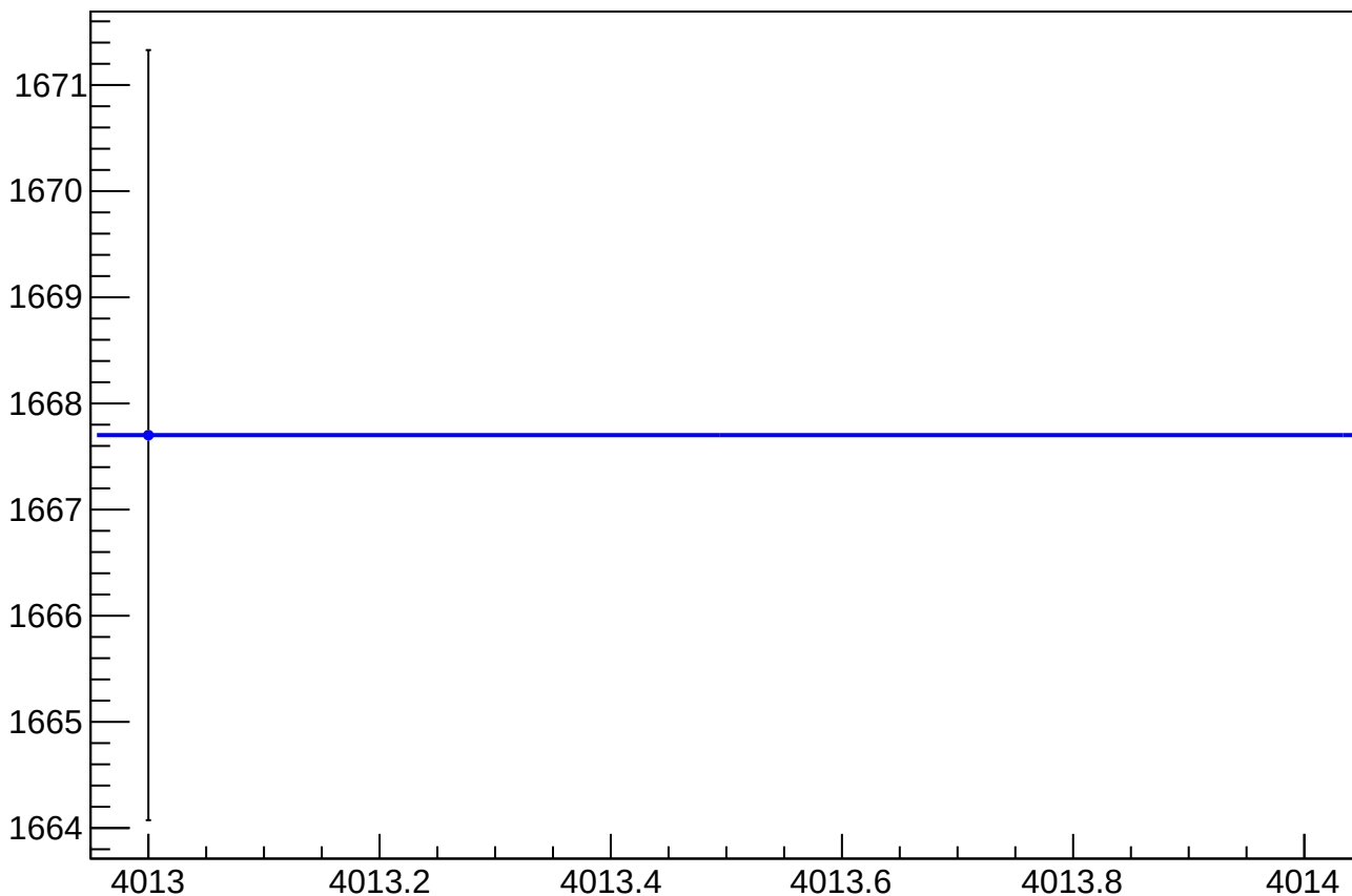
cor_asym_us_dd_at1lr_dd_avg_rms vs Slug, Sign Corrected
