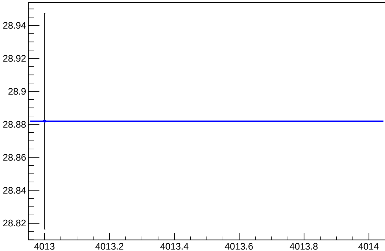
asym_us_dd_at2lr_dd_dd_eigen_dit_vs_eigen_cor_diff_rms vs Slug, Sign Corrected
