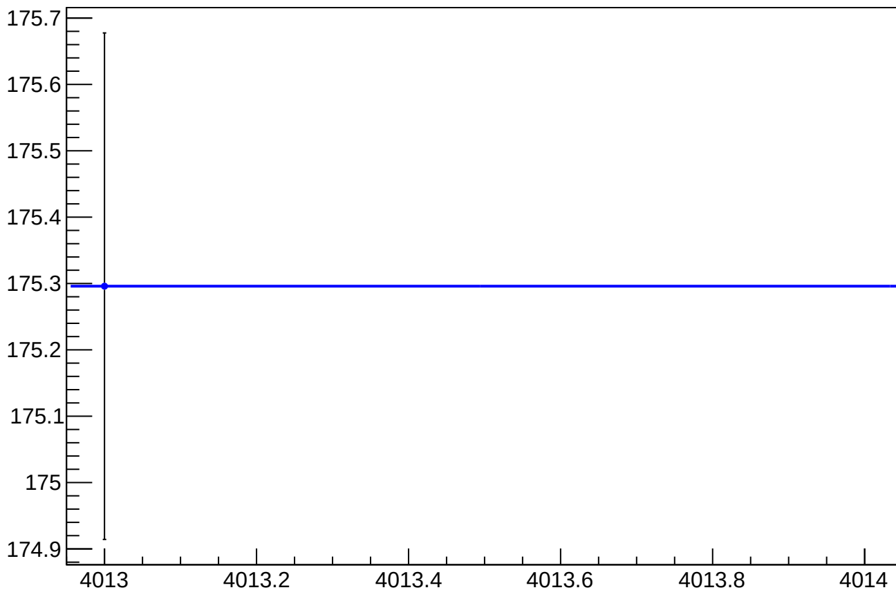
asym_sam1_cor_correction_rms vs Slug, Sign Corrected
