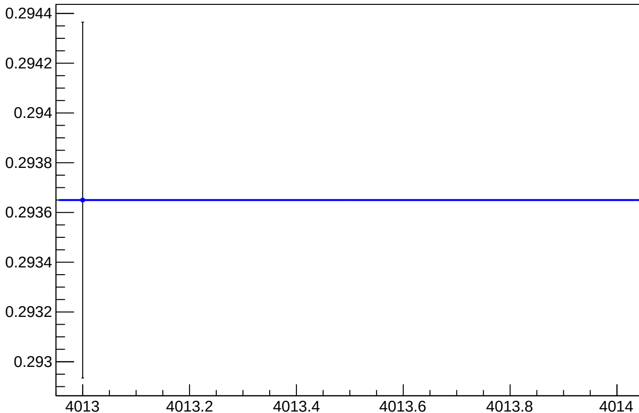
asym_us_dd_at2lr_dd_dd_reg_vs_cor_diff_rms vs Slug, Sign Corrected
