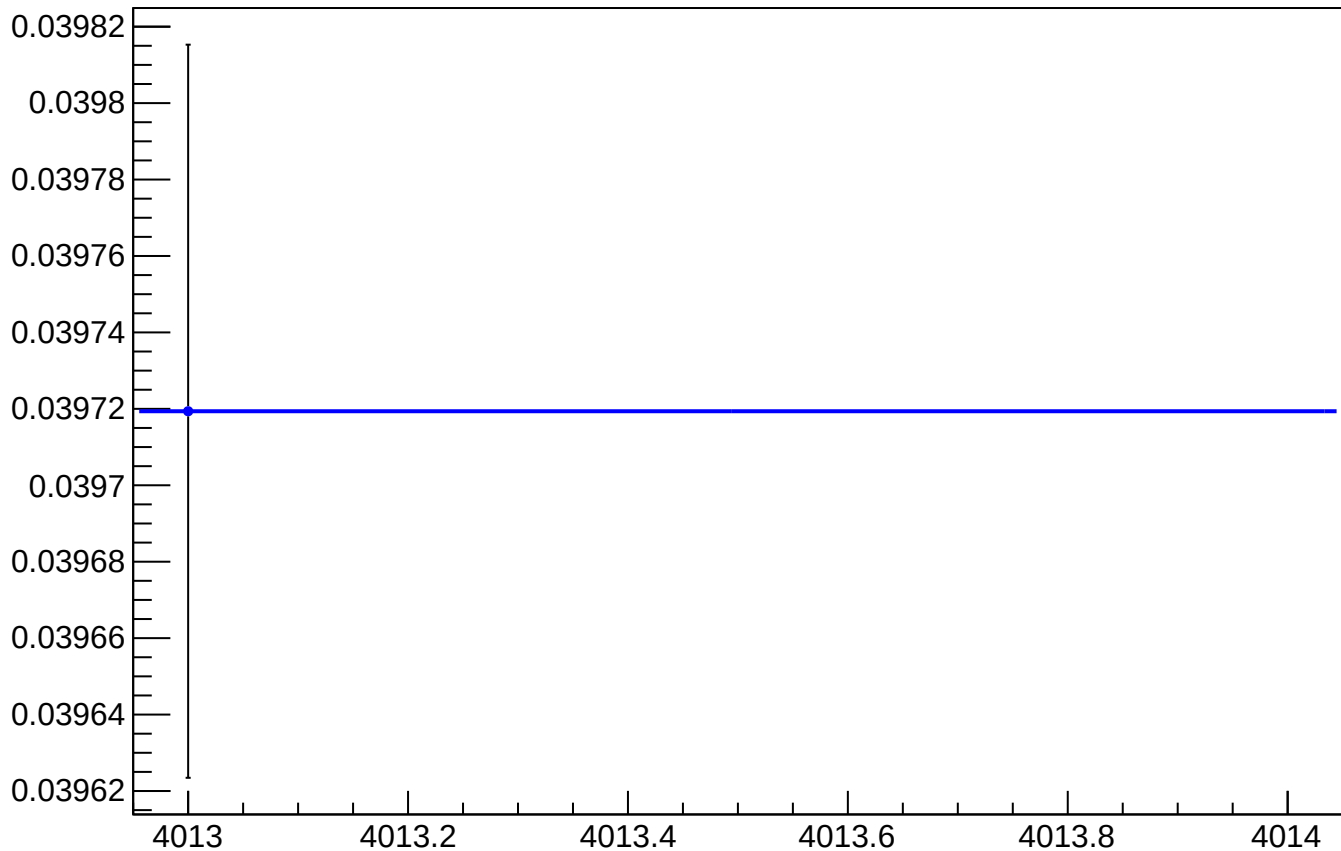
asym_sam_26_48_dd_reg_vs_cor_diff_rms vs Slug, Sign Corrected
