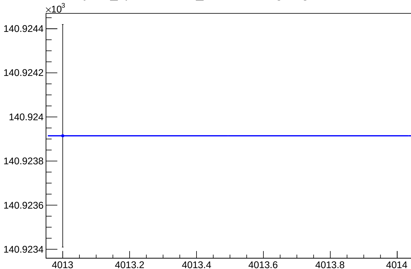
yield_bpm0i01aWS_mean vs Slug, Sign Corrected
