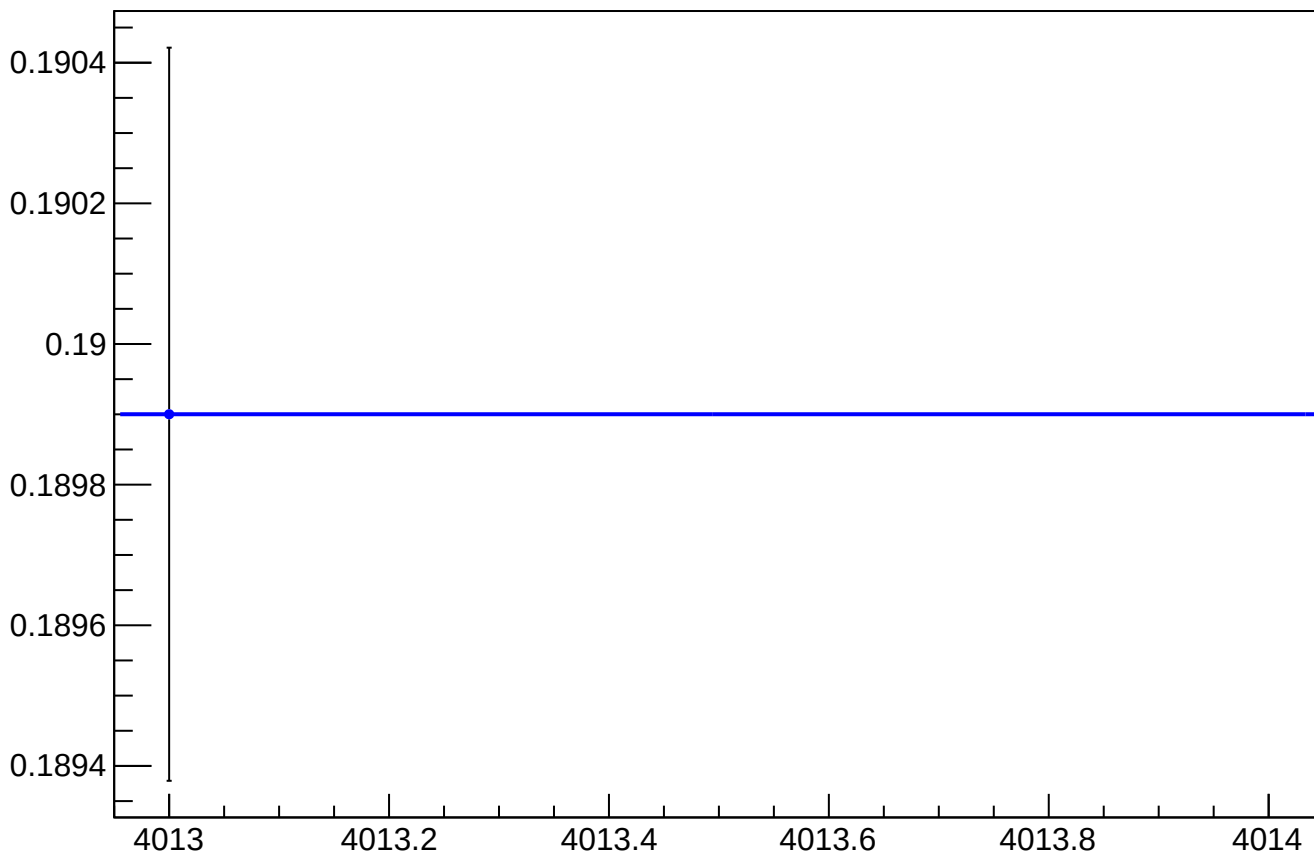
asym_atl_dd_reg_vs_cor_diff_rms vs Slug, Sign Corrected
