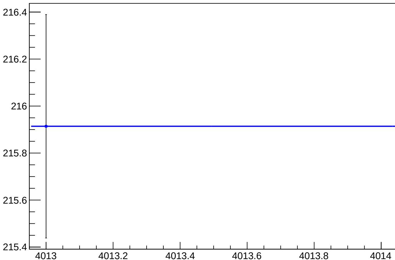
asym_us_avg_at1lr_avg_avg_dit_vs_cor_diff_rms vs Slug, Sign Corrected
