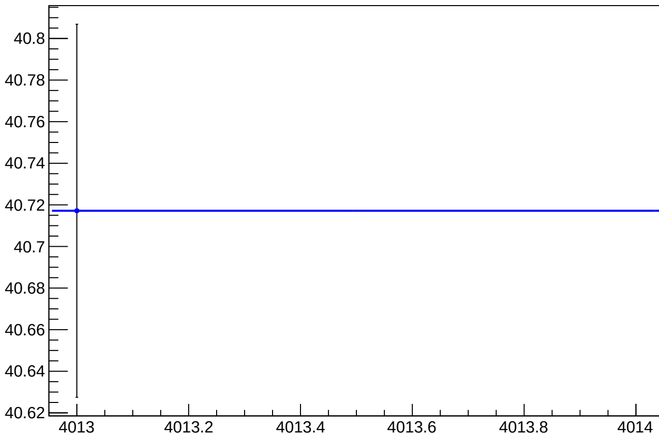
asym_sam5_dit_vs_cor_diff_rms vs Slug, Sign Corrected
