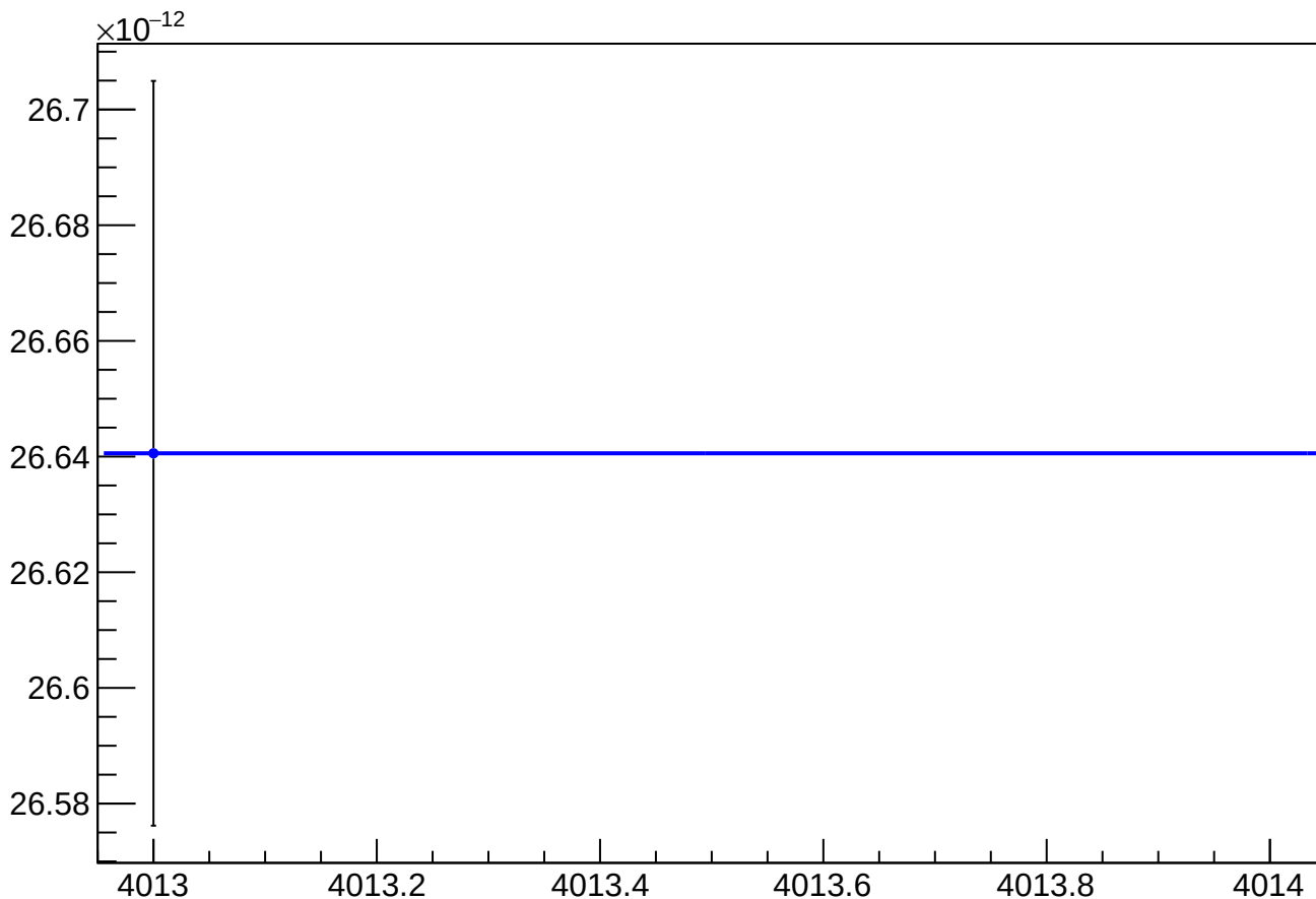
asym_sam_3748_avg_eigen_cor_vs_cor_diff_rms vs Slug, Sign Corrected
