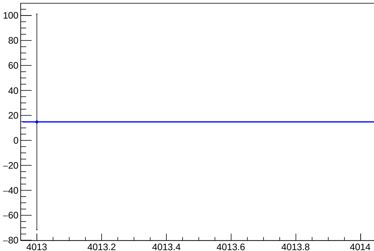
asym_bcm_cav4cQ_dg_ds_dd_mean vs Slug, Sign Corrected
