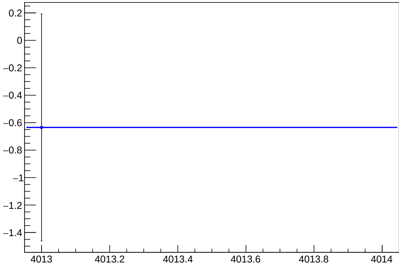
asym_atl_avg_atr_avg_avg_eigen_dit_vs_cor_diff_mean vs Slug, Sign Corrected
