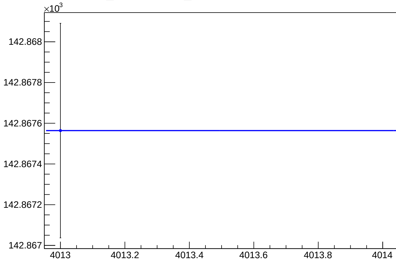
yield_bpm0l09WS_mean vs Slug, Sign Corrected
