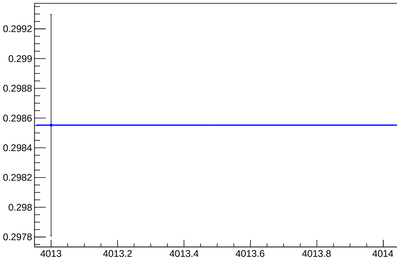
asym_us_avg_at2lr_avg_dd_reg_vs_cor_diff_rms vs Slug, Sign Corrected
