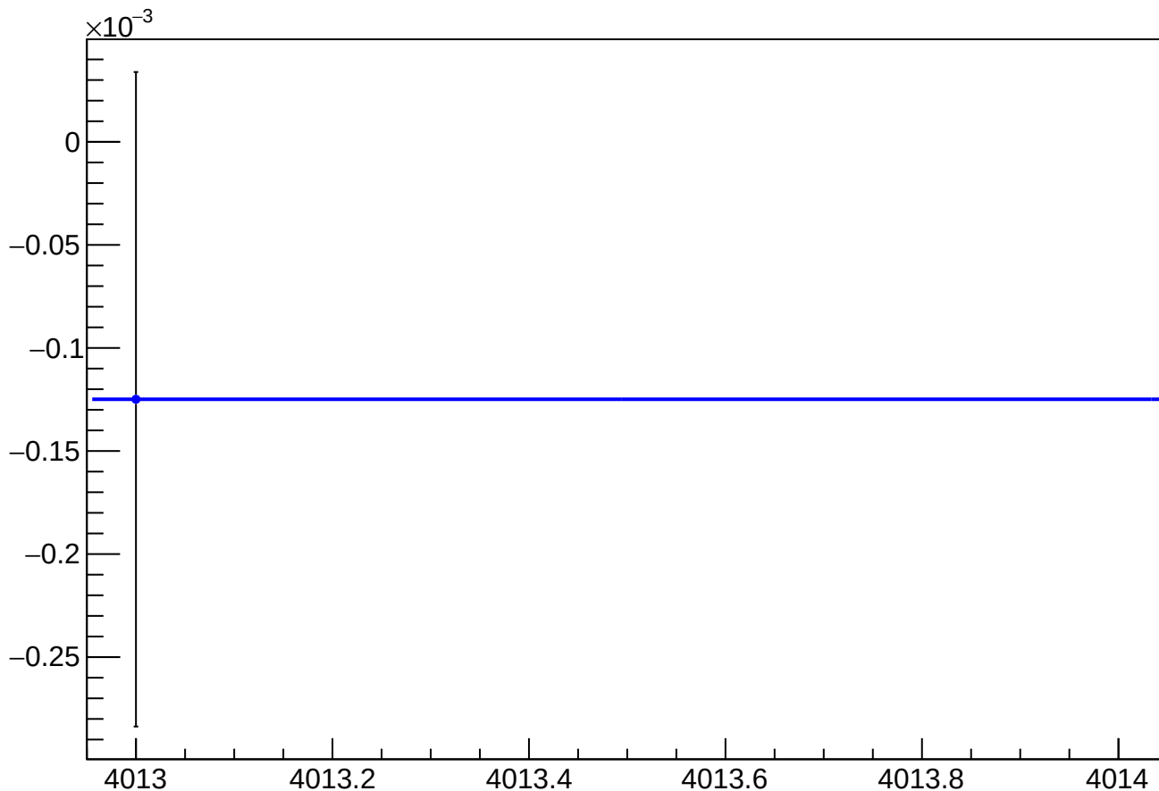
asym_sam4_reg_vs_cor_diff_mean vs Slug, Sign Corrected
