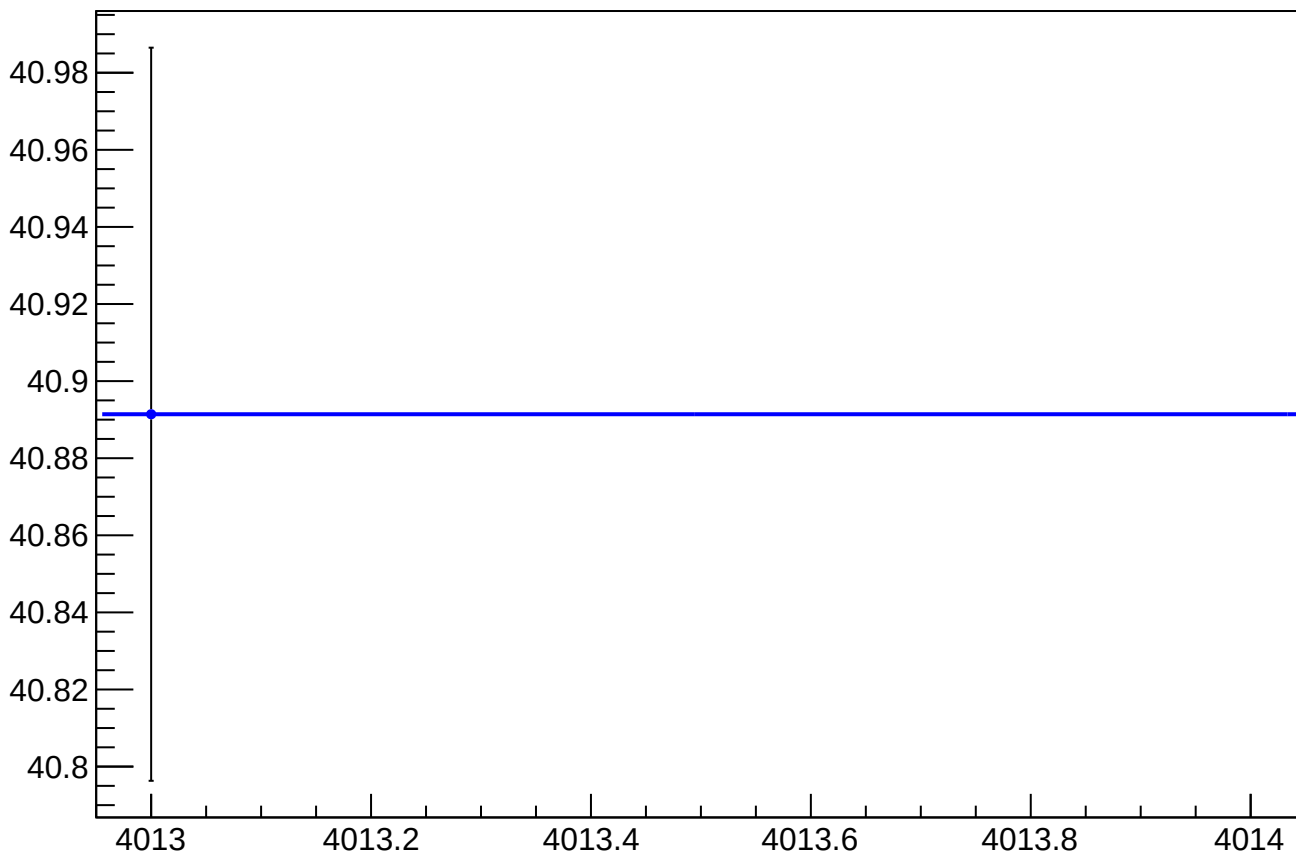
asym_sam_48_dd_eigen_dit_vs_eigen_cor_diff_rms vs Slug, Sign Corrected
