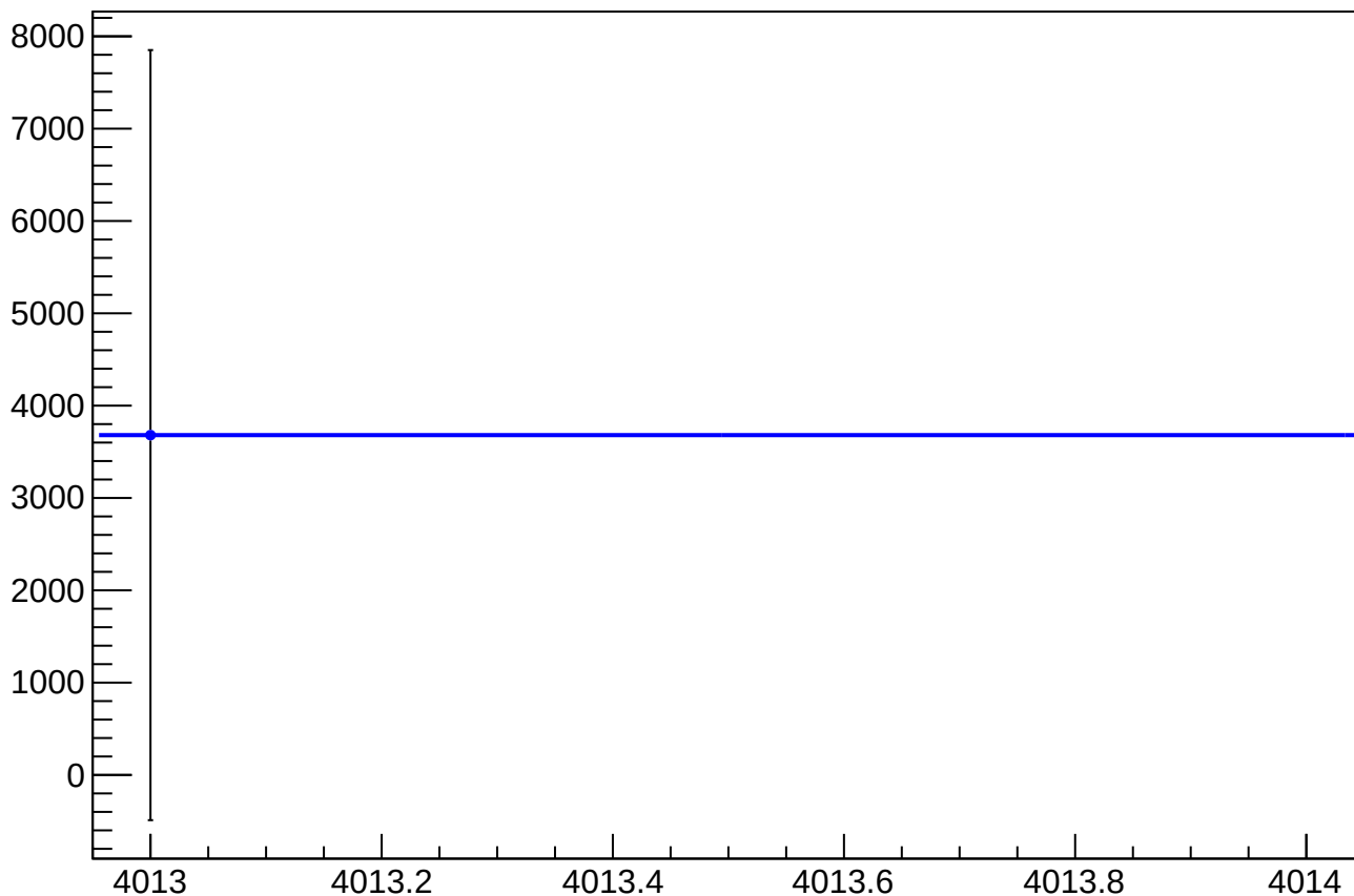
asym_usr_dit_correction_mean vs Slug, Sign Corrected
