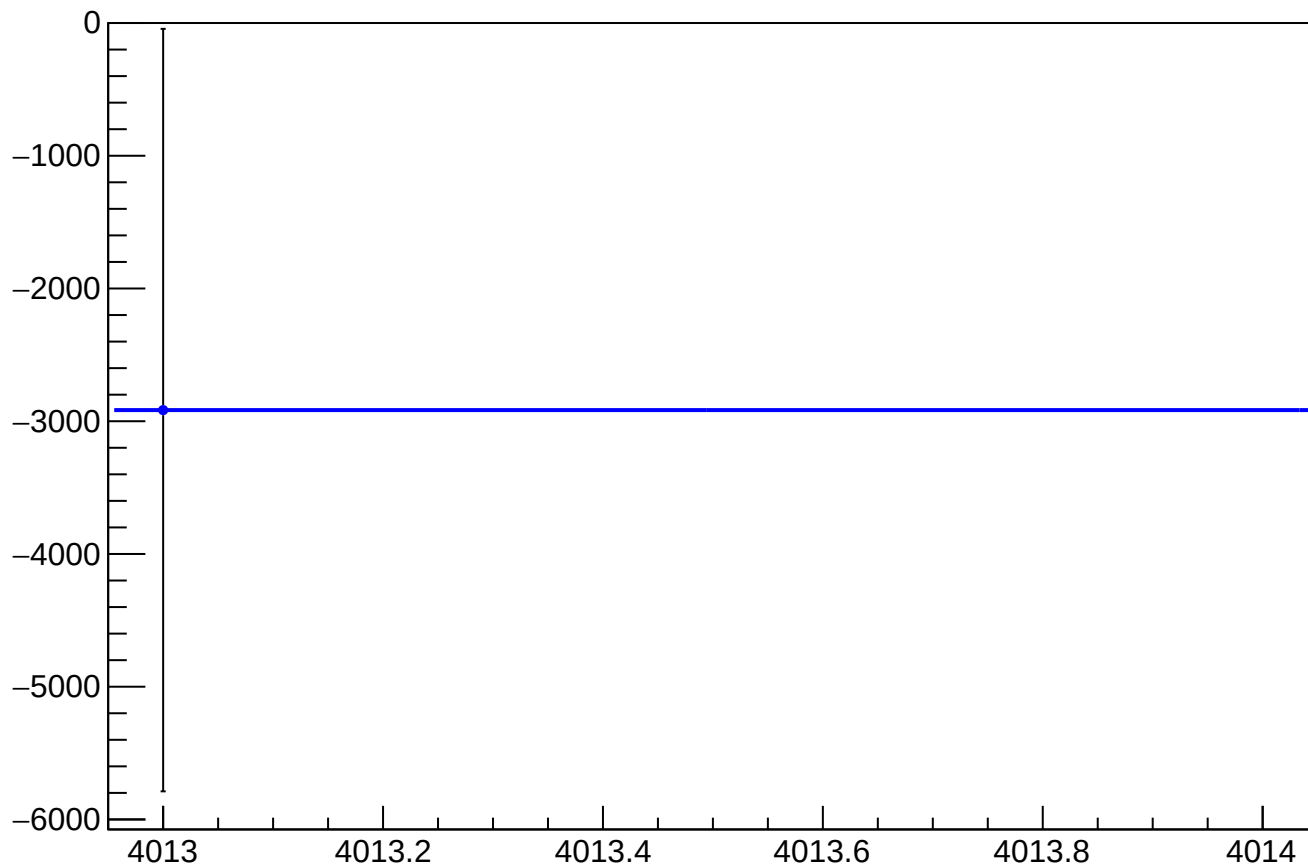
eigen_cor_asym_us_avg_atlr_avg_dd_mean vs Slug, Sign Corrected
