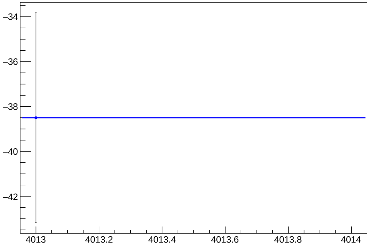
reg_asym_us_dd_at1lr_dd_dd_diff_bpm1X_slope vs Slug, Sign Corrected
