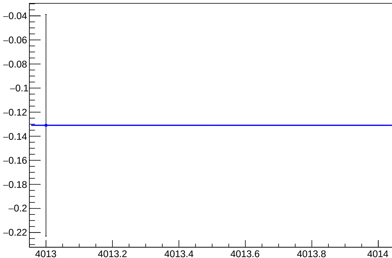
asym_at1_dd_dit_vs_eigen_cor_diff_mean vs Slug, Sign Corrected
