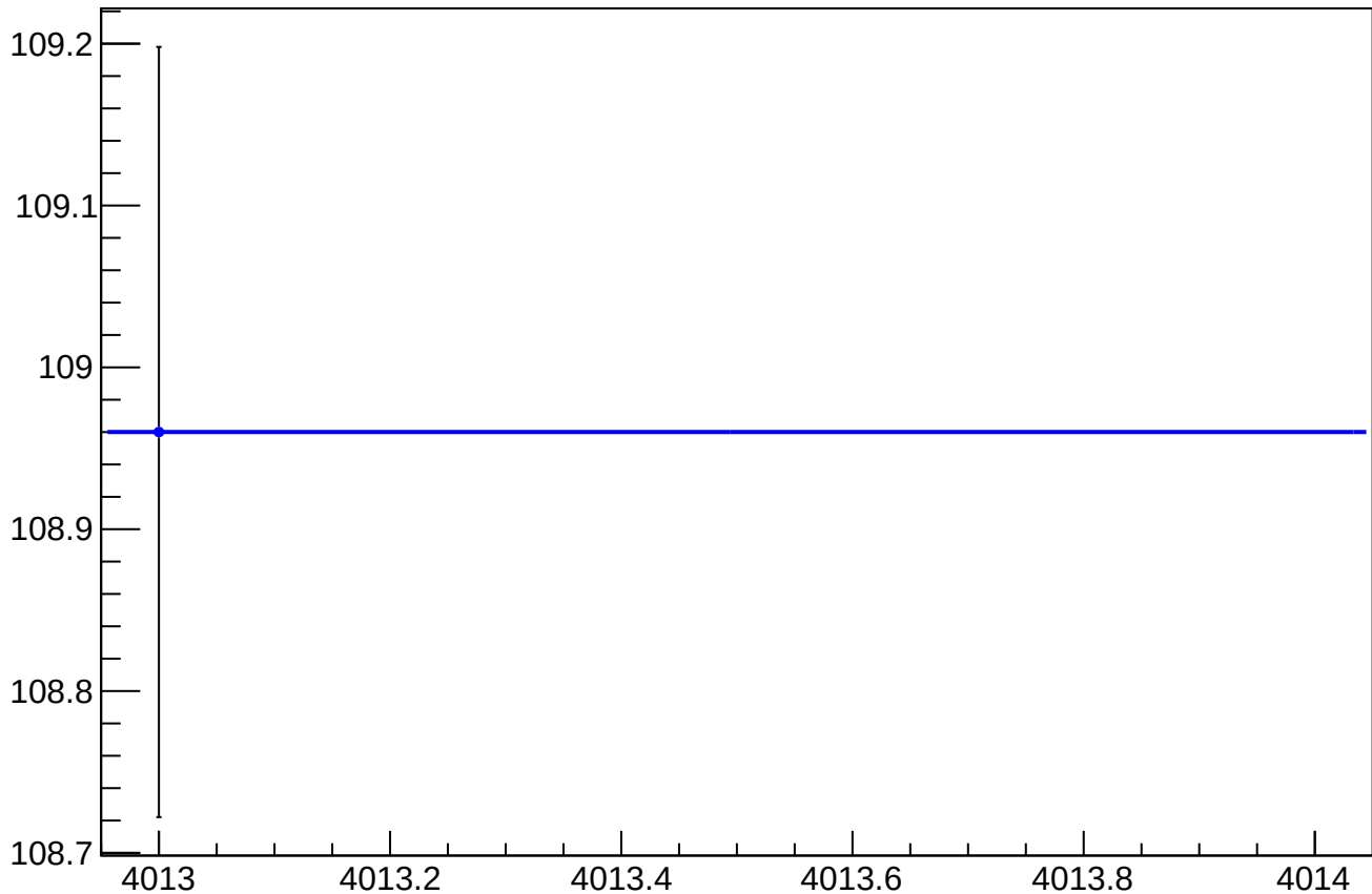
eigen_cor_asym_sam3_rms vs Slug, Sign Corrected
