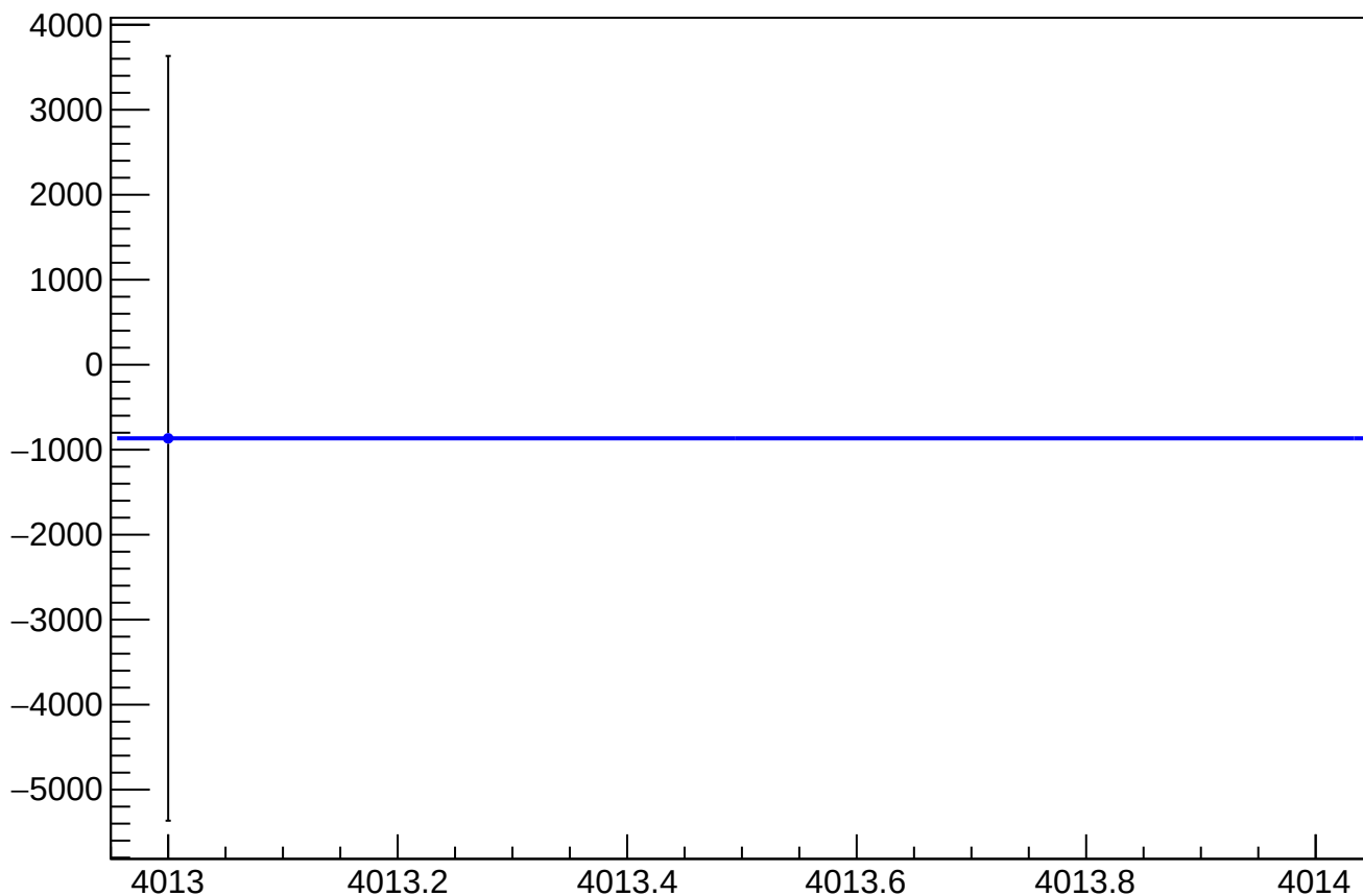
asym_sam_48_avg_reg_correction_mean vs Slug, Sign Corrected
