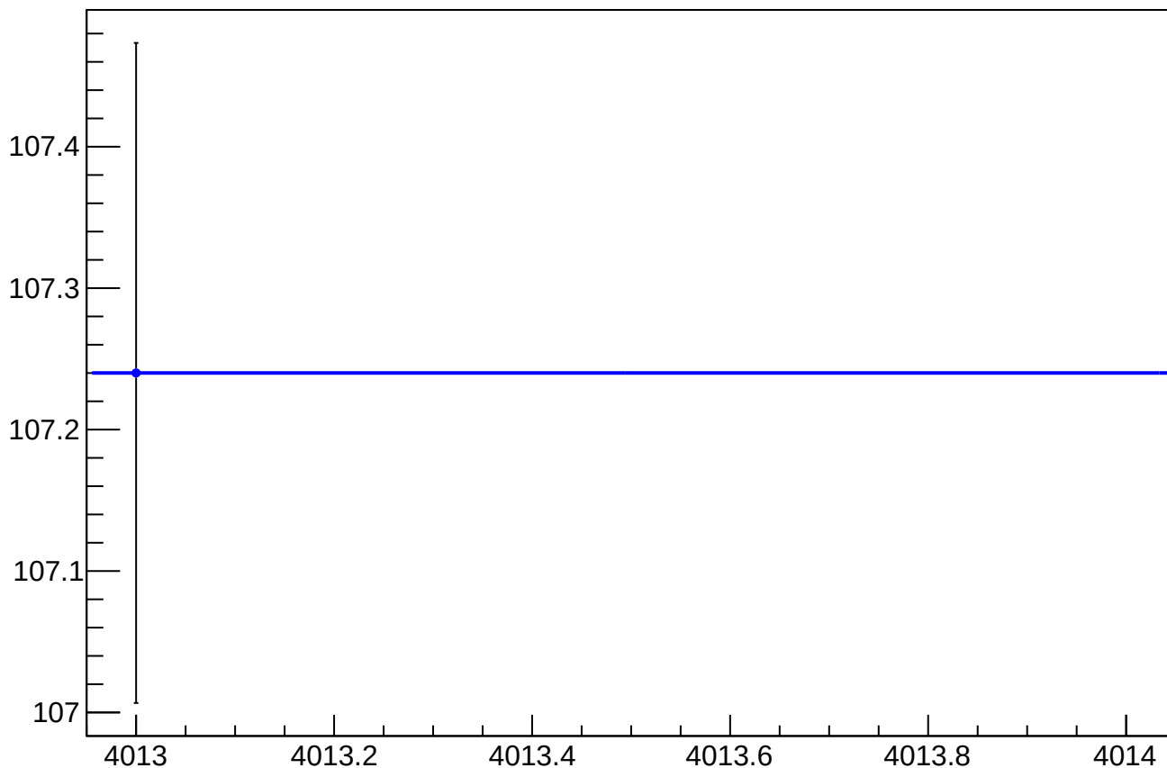
eigen_dit_asym_sam_15_avg_rms vs Slug, Sign Corrected
