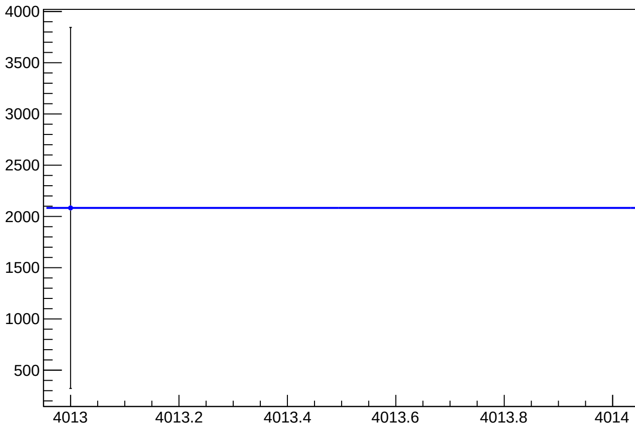
asym_usr_atr1_dd_reg_correction_mean vs Slug, Sign Corrected
