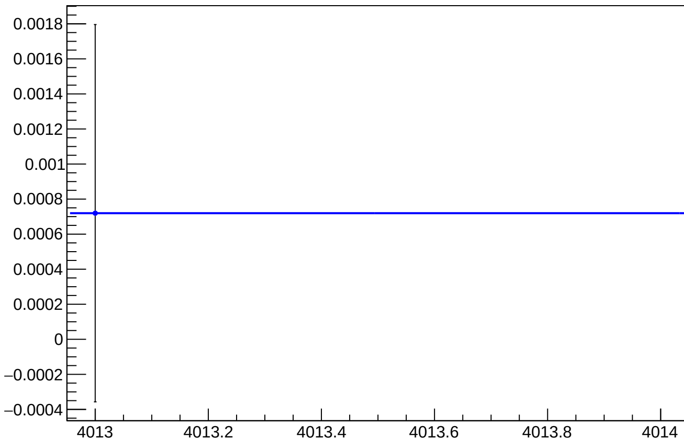
asym_us_dd_at1lr_dd_dd_reg_vs_cor_diff_mean vs Slug, Sign Corrected
