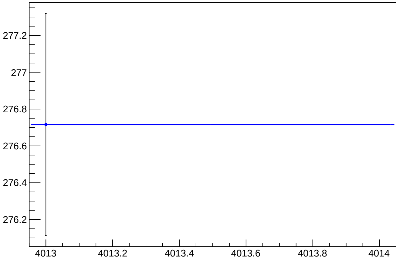
asym_sam_1357_2468_dd_dit_correction_rms vs Slug, Sign Corrected
