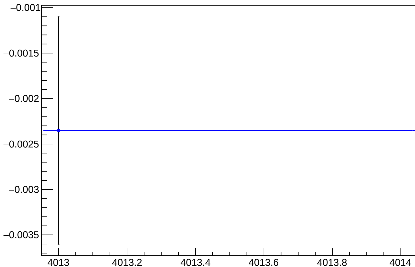
asym_atl_avg_reg_vs_cor_diff_mean vs Slug, Sign Corrected
