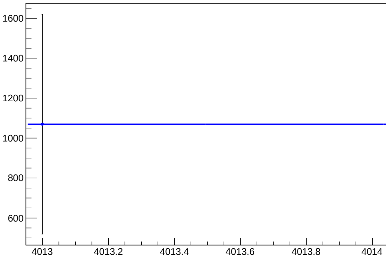
dit_asym_sam_26_48_dd_mean vs Slug, Sign Corrected
