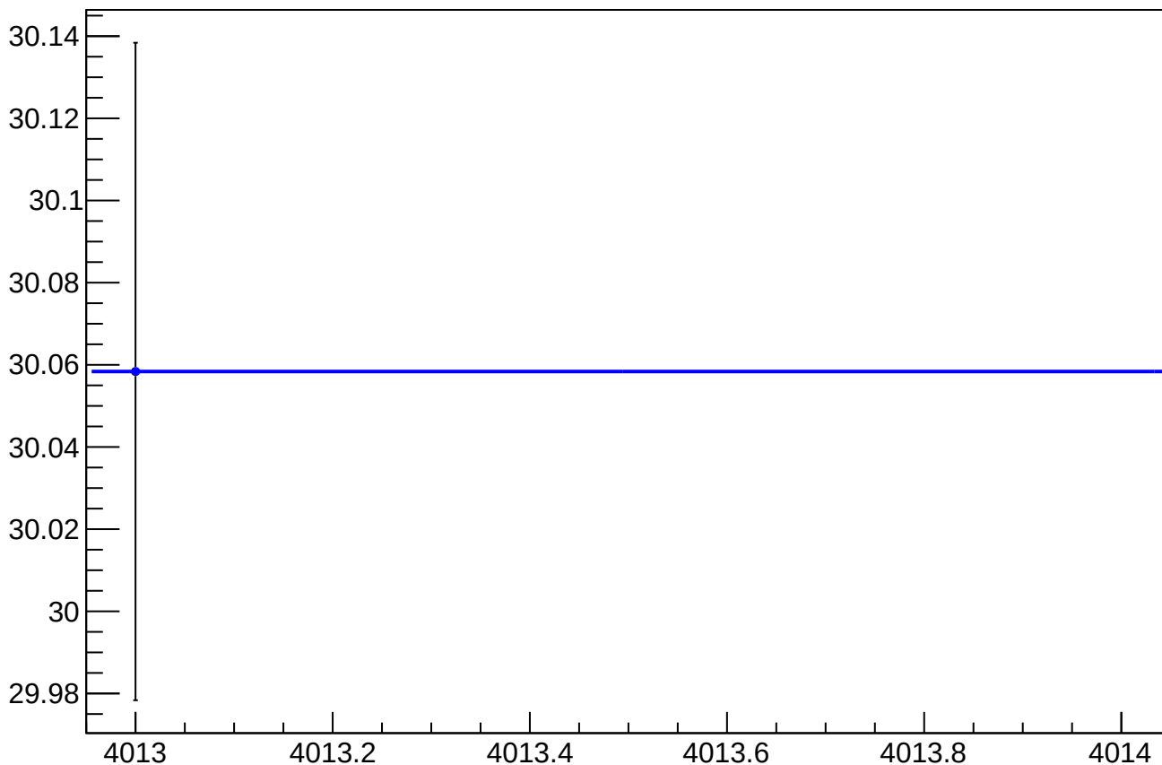
asym_us_dd_at2lr_dd_avg_dit_vs_cor_diff_rms vs Slug, Sign Corrected
