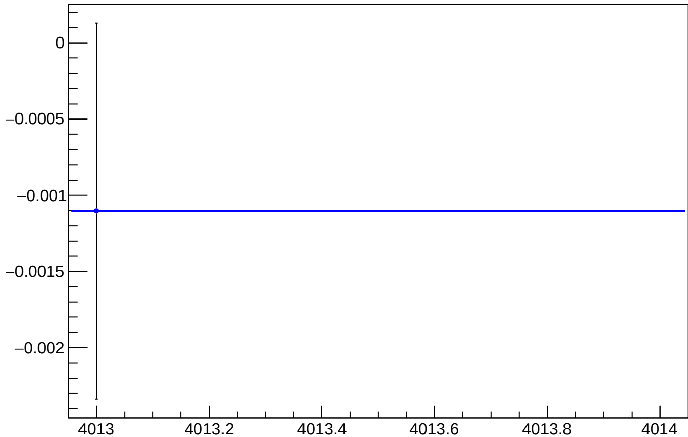
asym_us_dd_at2lr_dd_avg_reg_vs_cor_diff_mean vs Slug, Sign Corrected
