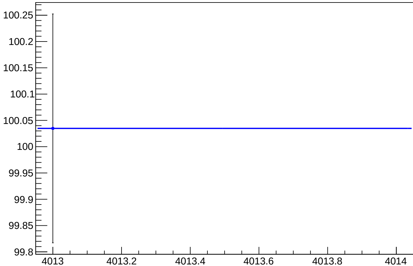
cor_asym_sam_37_48_dd_rms vs Slug, Sign Corrected
