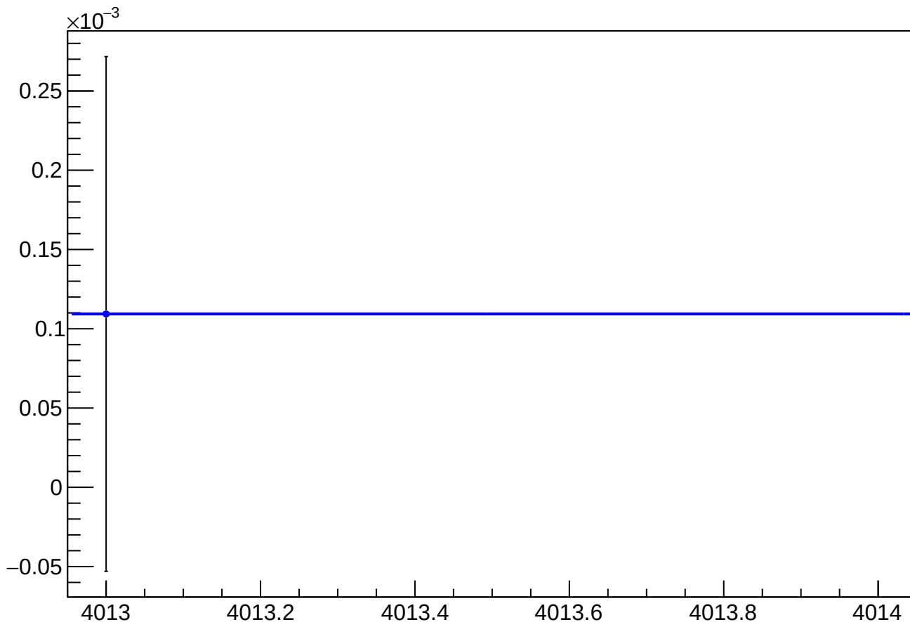
asym_sam_26_avg_reg_vs_cor_diff_mean vs Slug, Sign Corrected
