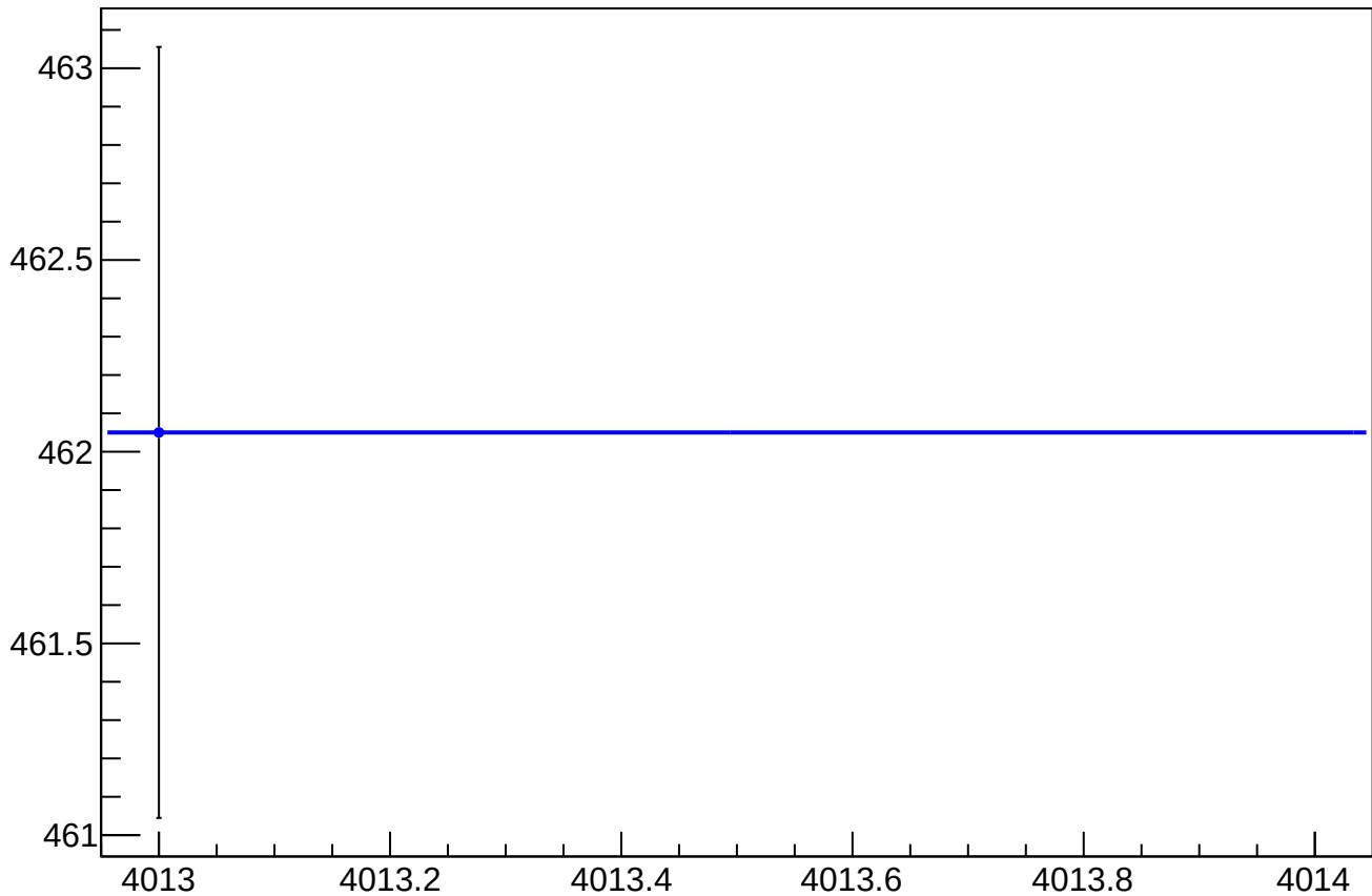
asym_sam_15_avg_eigen_cor_correction_rms vs Slug, Sign Corrected
