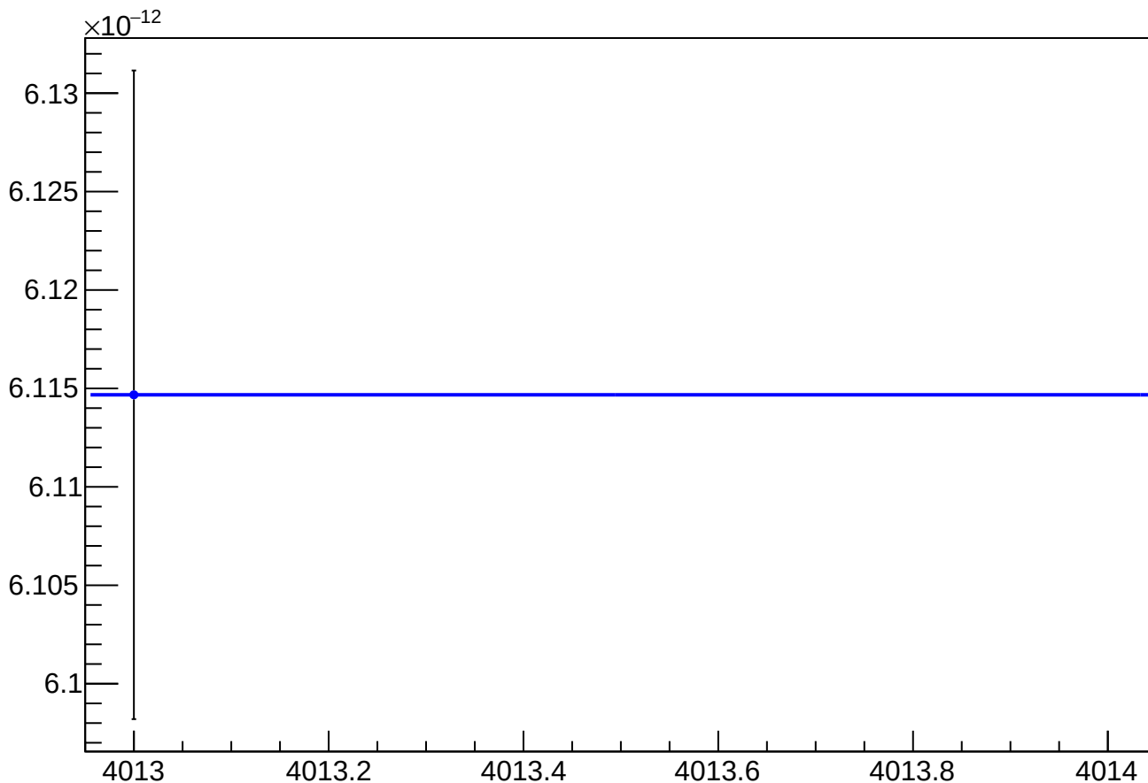
asym_sam_13_57_dd_eigen_cor_vs_cor_diff_rms vs Slug, Sign Corrected
