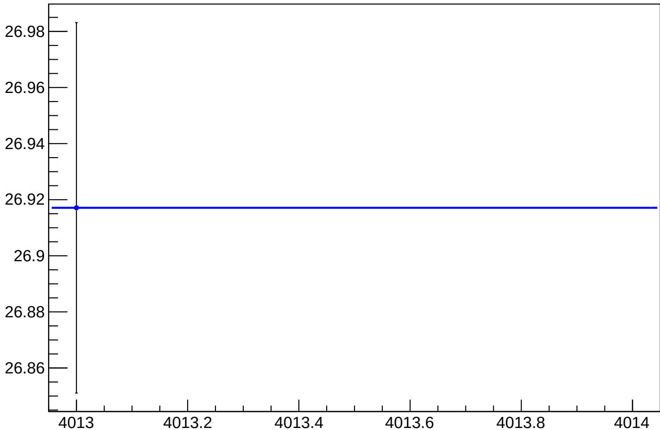
asym_us_dd_at1lr_dd_dd_dit_vs_cor_diff_rms vs Slug, Sign Corrected
