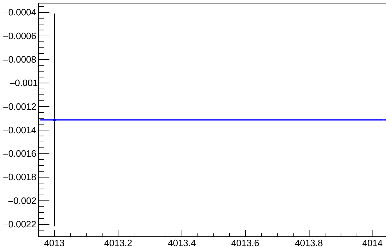
asym_usl_atl2_avg_reg_vs_cor_diff_mean vs Slug, Sign Corrected
