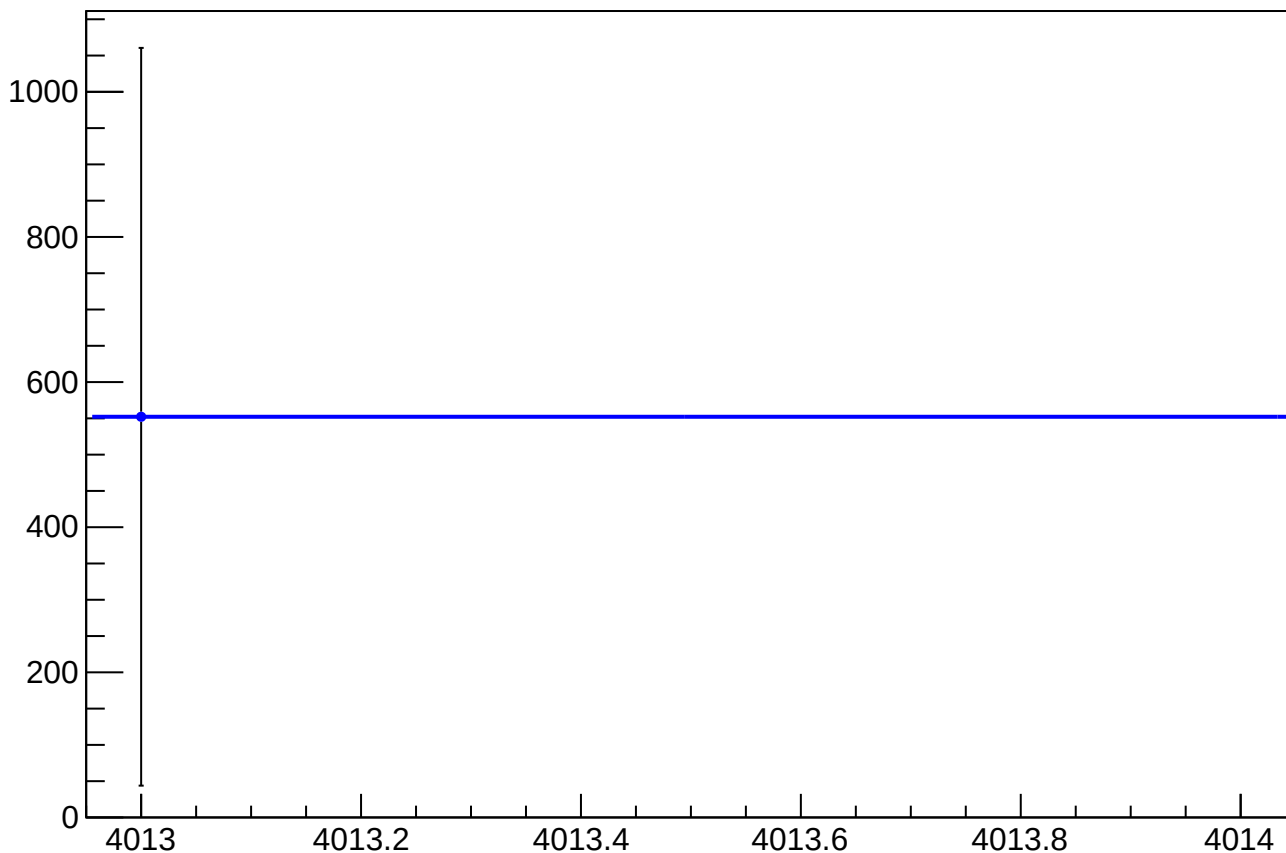
reg_asym_sam_24_68_dd_mean vs Slug, Sign Corrected
