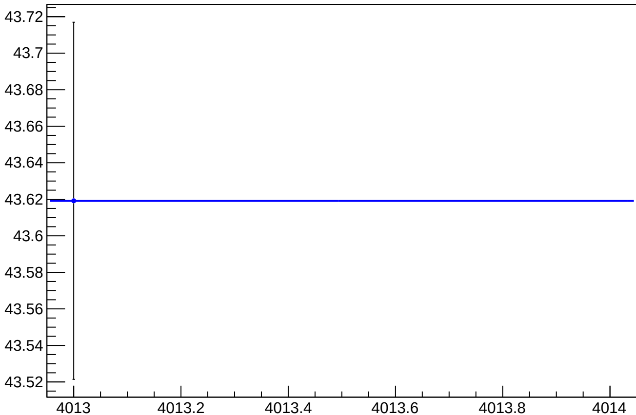
asym_usr_atr1_dd_eigen_dit_vs_eigen_cor_diff_rms vs Slug, Sign Corrected
