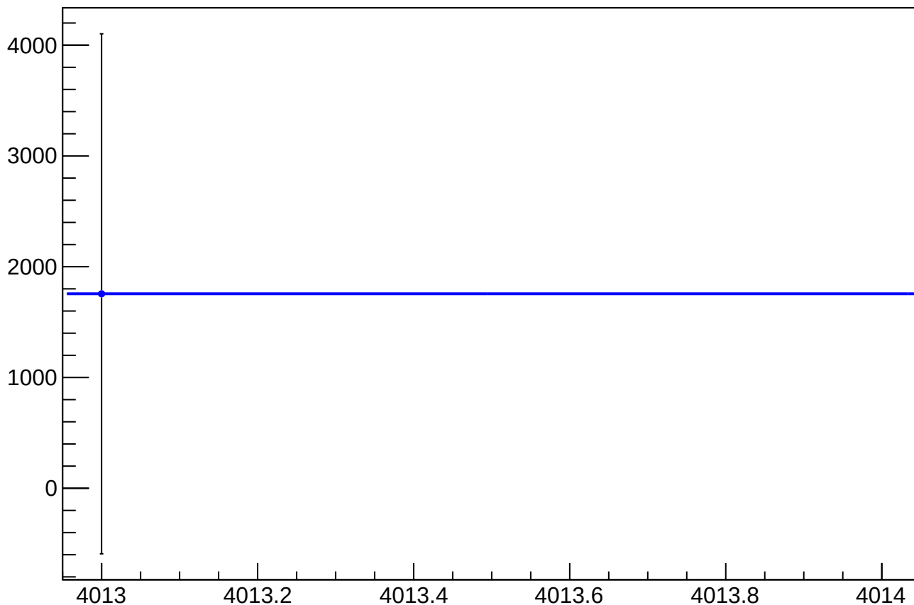
asym_at1_dd_at2_dd_avg_cor_correction_mean vs Slug, Sign Corrected
