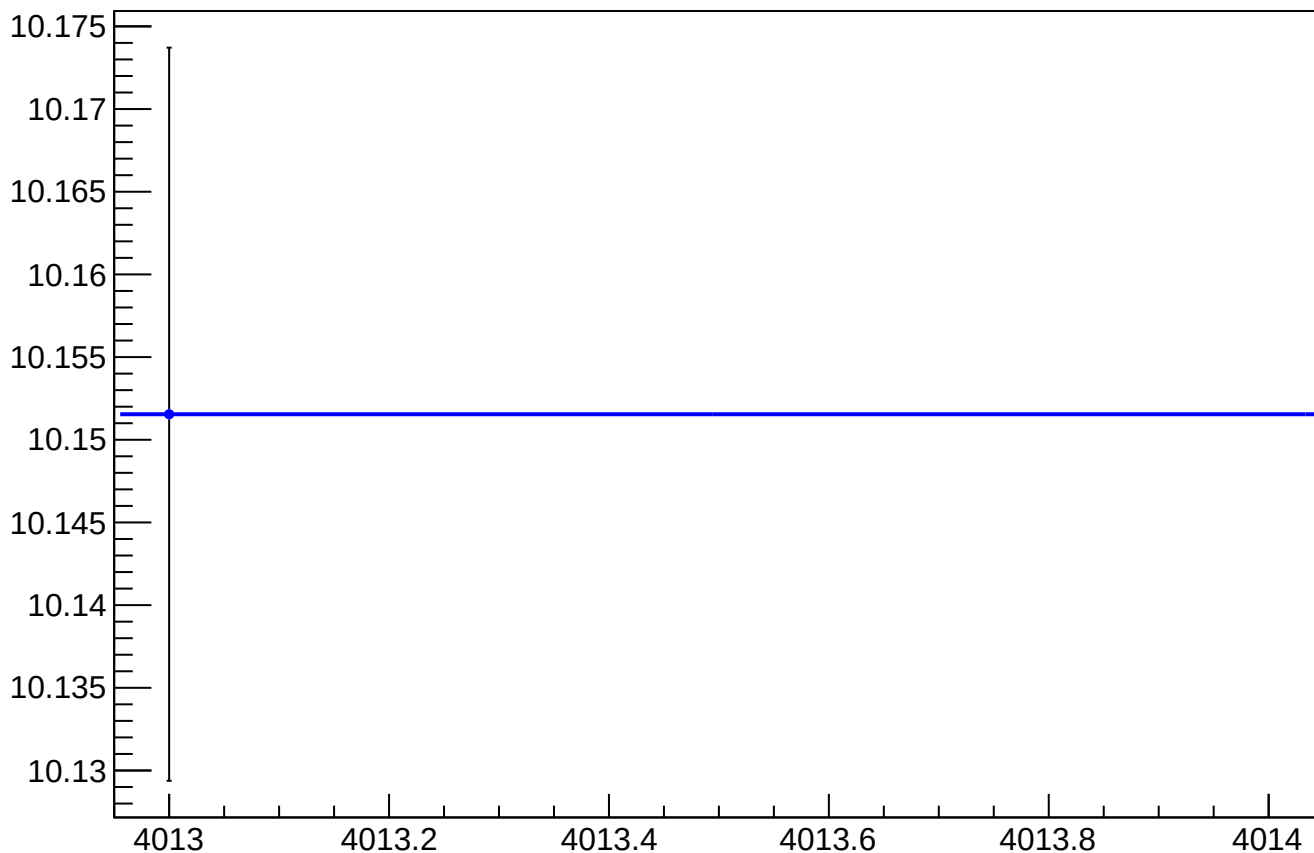
asym_bcm_an_us_an_ds3_dd_rms vs Slug, Sign Corrected
