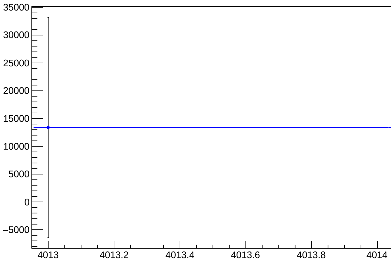
asym_atl_avg_atr_avg_avg_cor_correction_mean vs Slug, Sign Corrected
