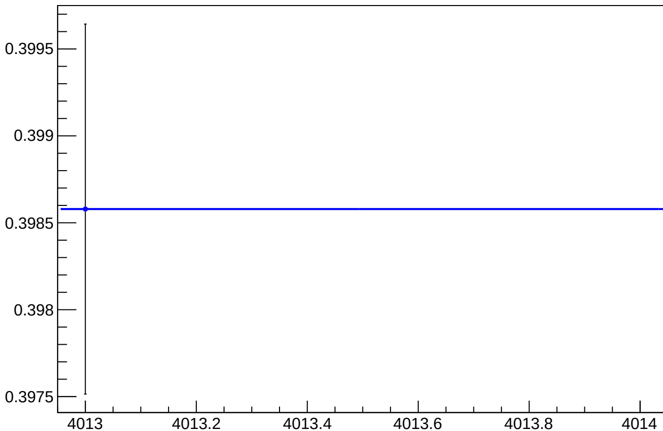
asym_atl2_reg_vs_cor_diff_rms vs Slug, Sign Corrected
