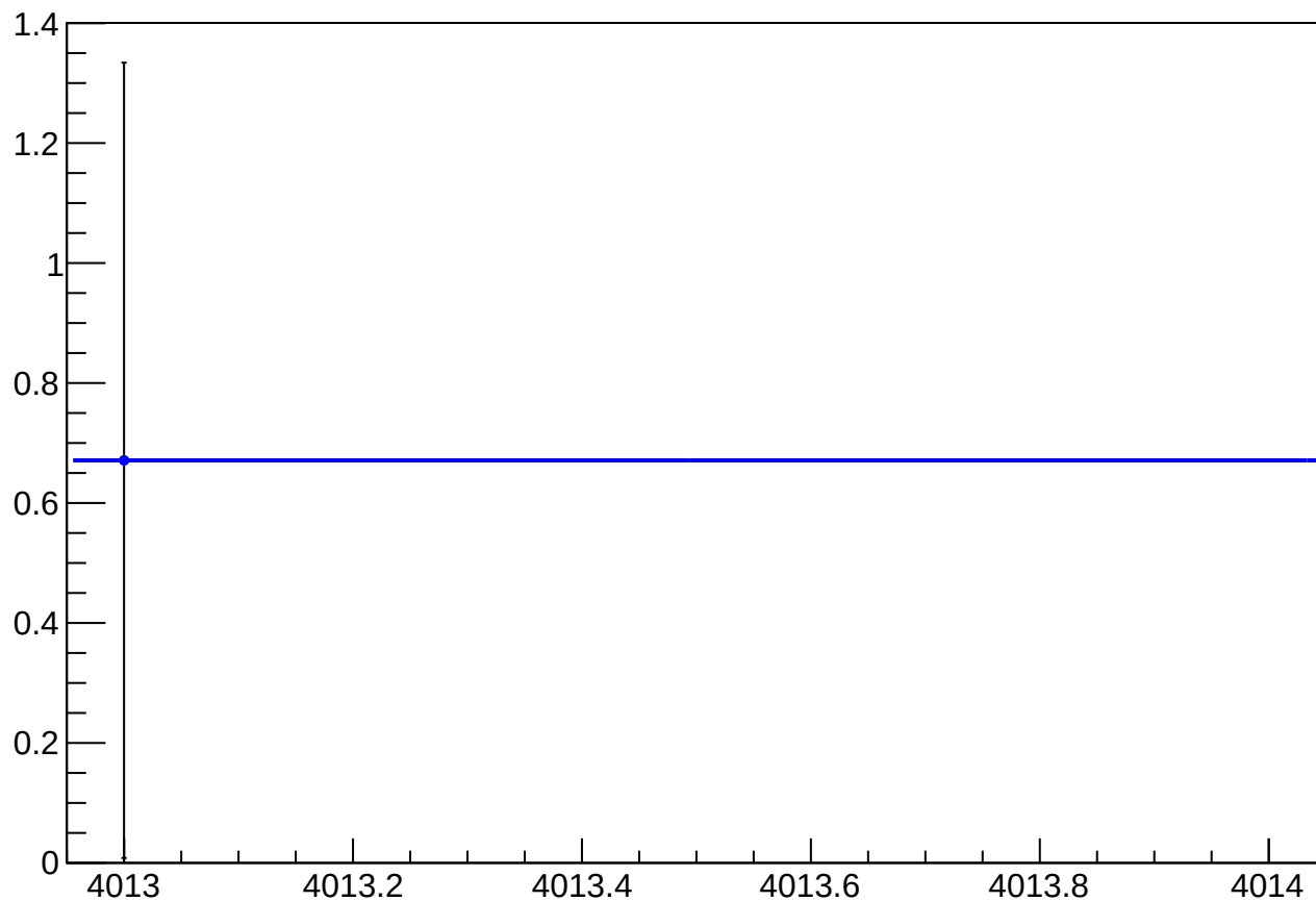
asym_us_avg_atlr_avg_dd_eigen_dit_vs_cor_diff_mean vs Slug, Sign Corrected
