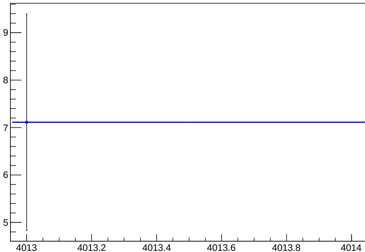
reg_asym_atl1r2_dd_atl2r1_dd_avg_diff_bpm4eY_slope vs Slug, Sign Corrected
