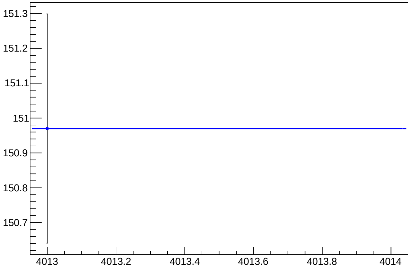
cor_asym_sam_48_dd_rms vs Slug, Sign Corrected
