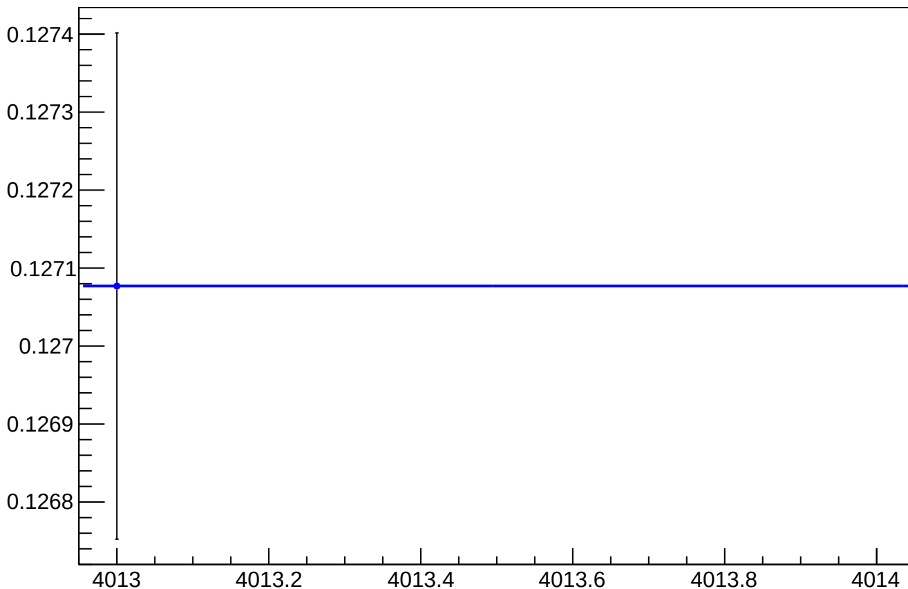
asym_at1_dd_at2_dd_avg_reg_vs_cor_diff_rms vs Slug, Sign Corrected
