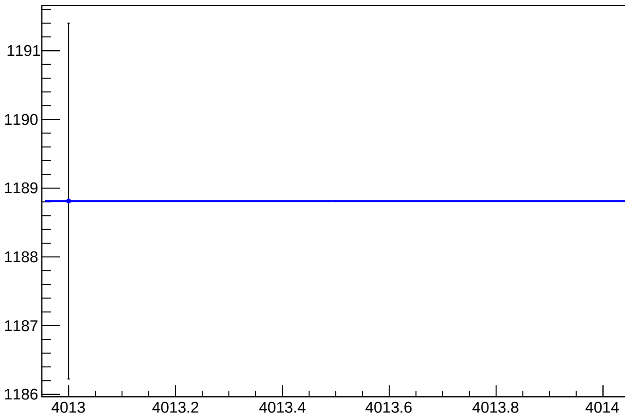
asym_usr_atr1_avg_eigen_cor_correction_rms vs Slug, Sign Corrected
