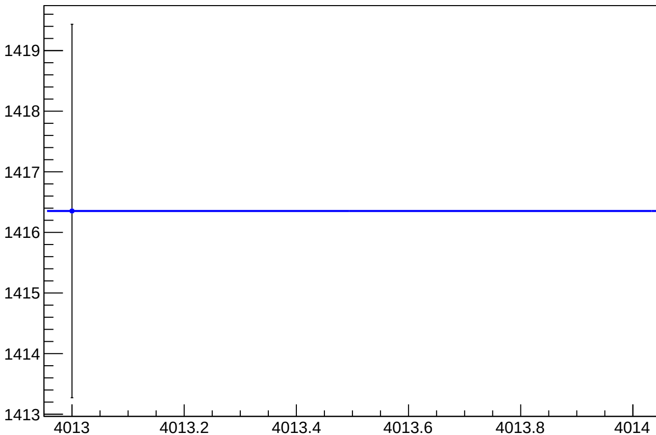
eigen_cor_asym_atl1r2_dd_rms vs Slug, Sign Corrected
