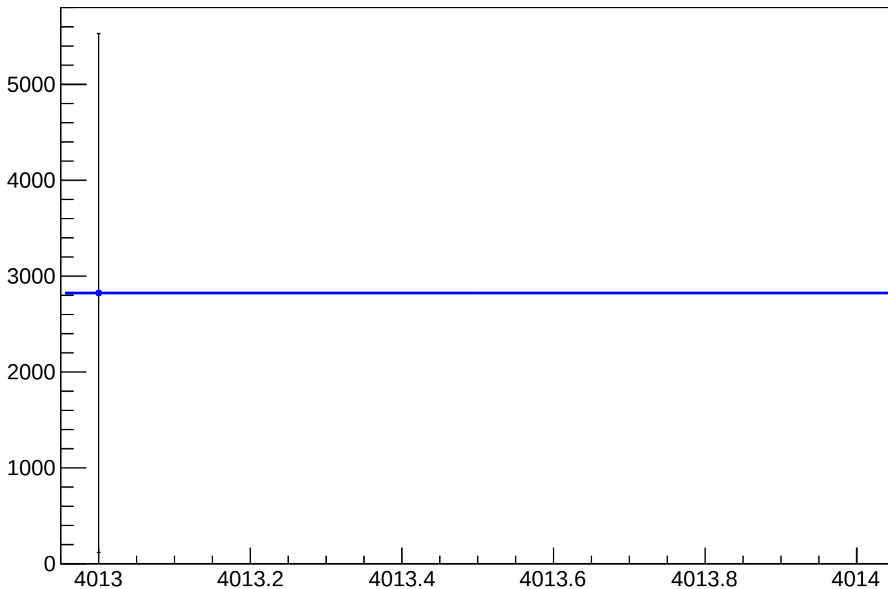
asym_atl1_cor_correction_mean vs Slug, Sign Corrected
