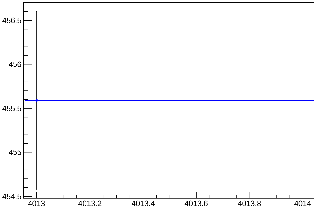
asym_atl2_eigen_dit_vs_eigen_cor_diff_rms vs Slug, Sign Corrected
