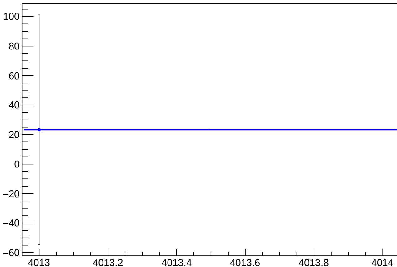
asym_bcm_cav4cQ_bcm_an_us_agg_dd_mean vs Slug, Sign Corrected
