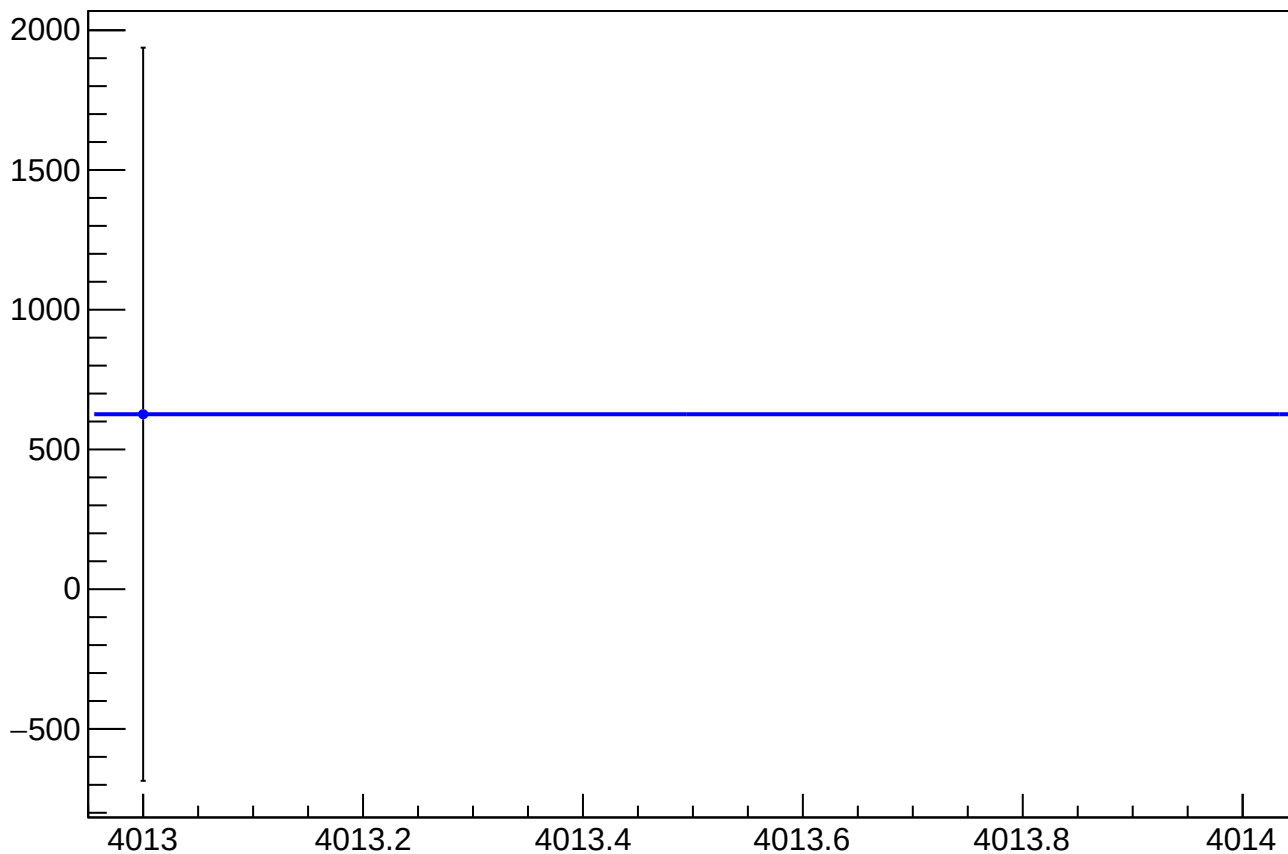
asym_us_dd_at1lr_dd_avg_eigen_cor_correction_mean vs Slug, Sign Corrected
