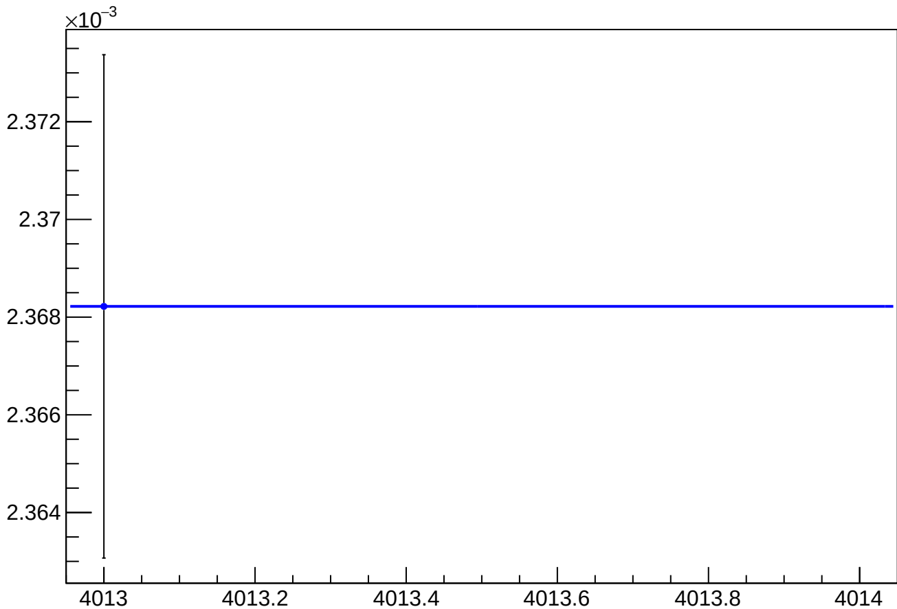
asym_sam_15_37_dd_eigen_dit_vs_dit_diff_rms vs Slug, Sign Corrected
