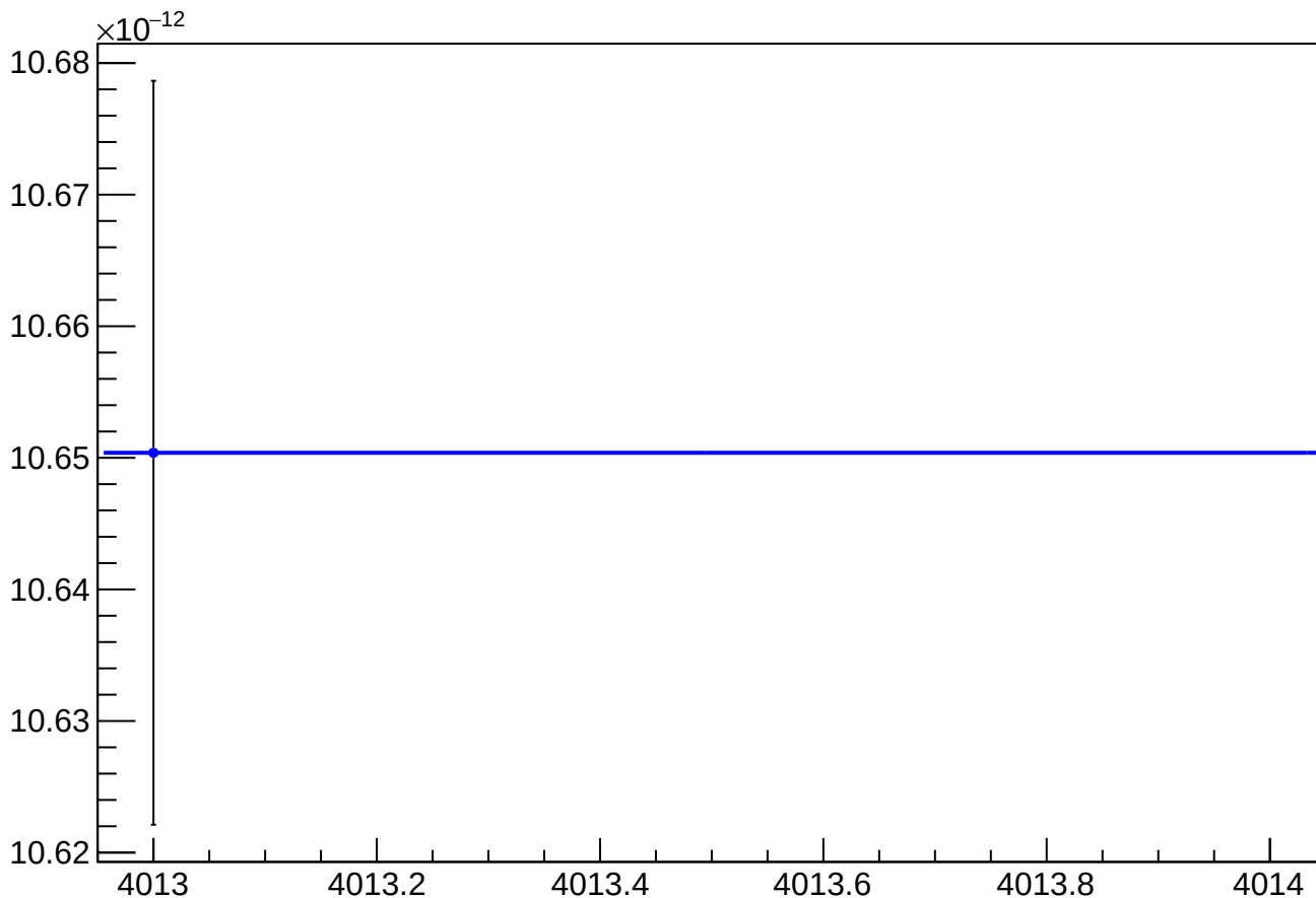
asym_us_dd_eigen_cor_vs_cor_diff_rms vs Slug, Sign Corrected
