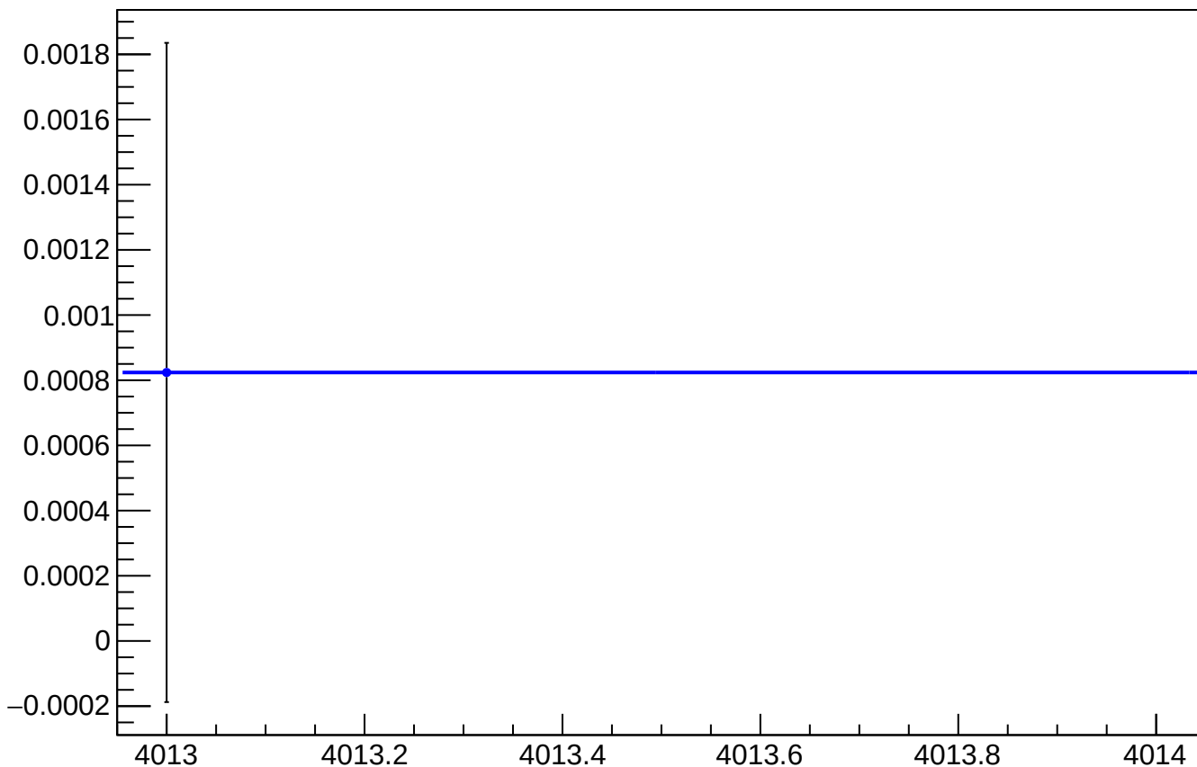
asym_us_dd_at2lr_dd_dd_reg_vs_cor_diff_mean vs Slug, Sign Corrected
