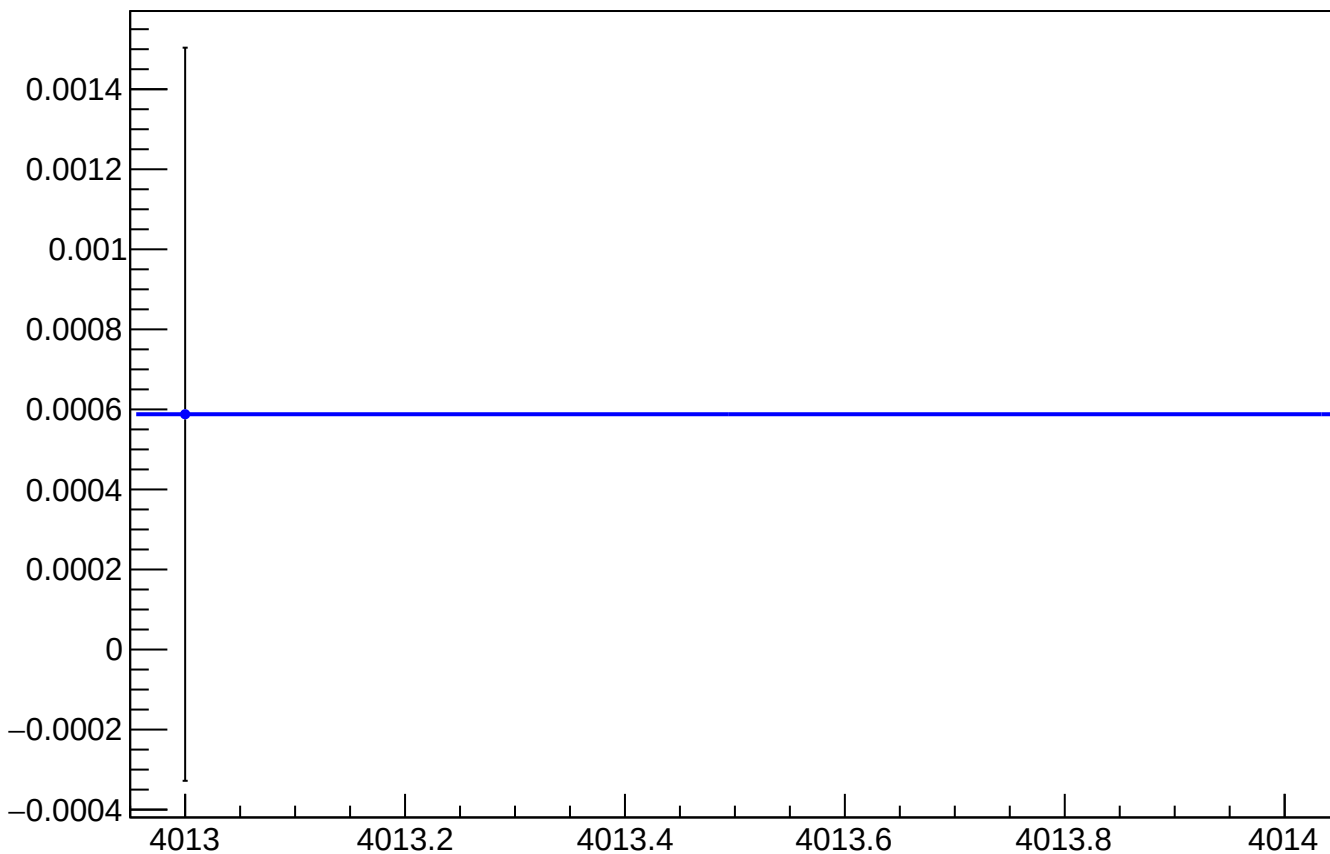
asym_at2_dd_reg_vs_cor_diff_mean vs Slug, Sign Corrected
