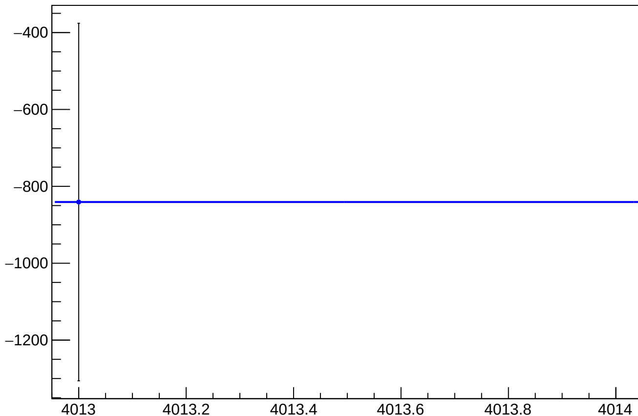
cor_asym_sam_48_dd_mean vs Slug, Sign Corrected
