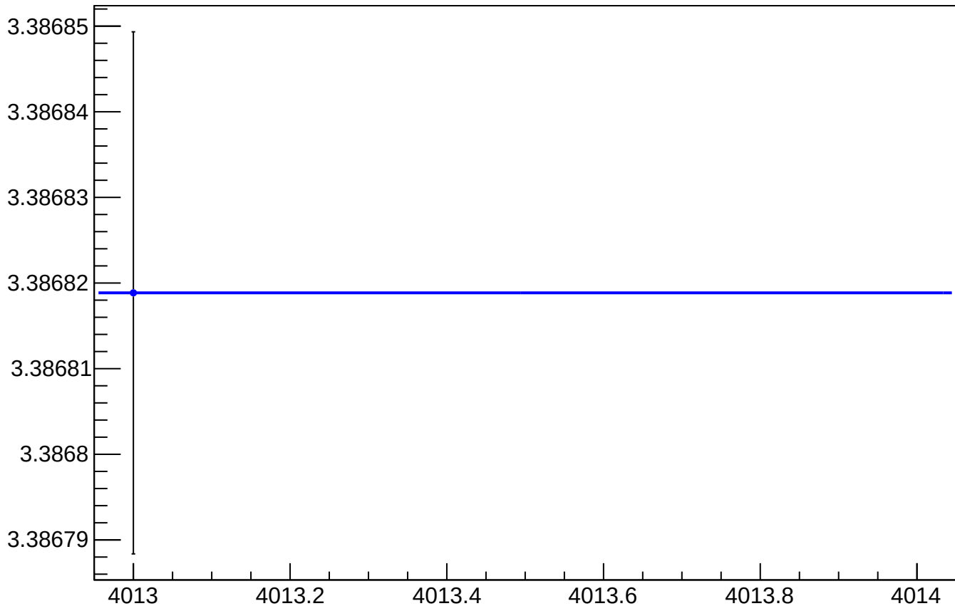
yield_bpm0l05Y_mean vs Slug, Sign Corrected
