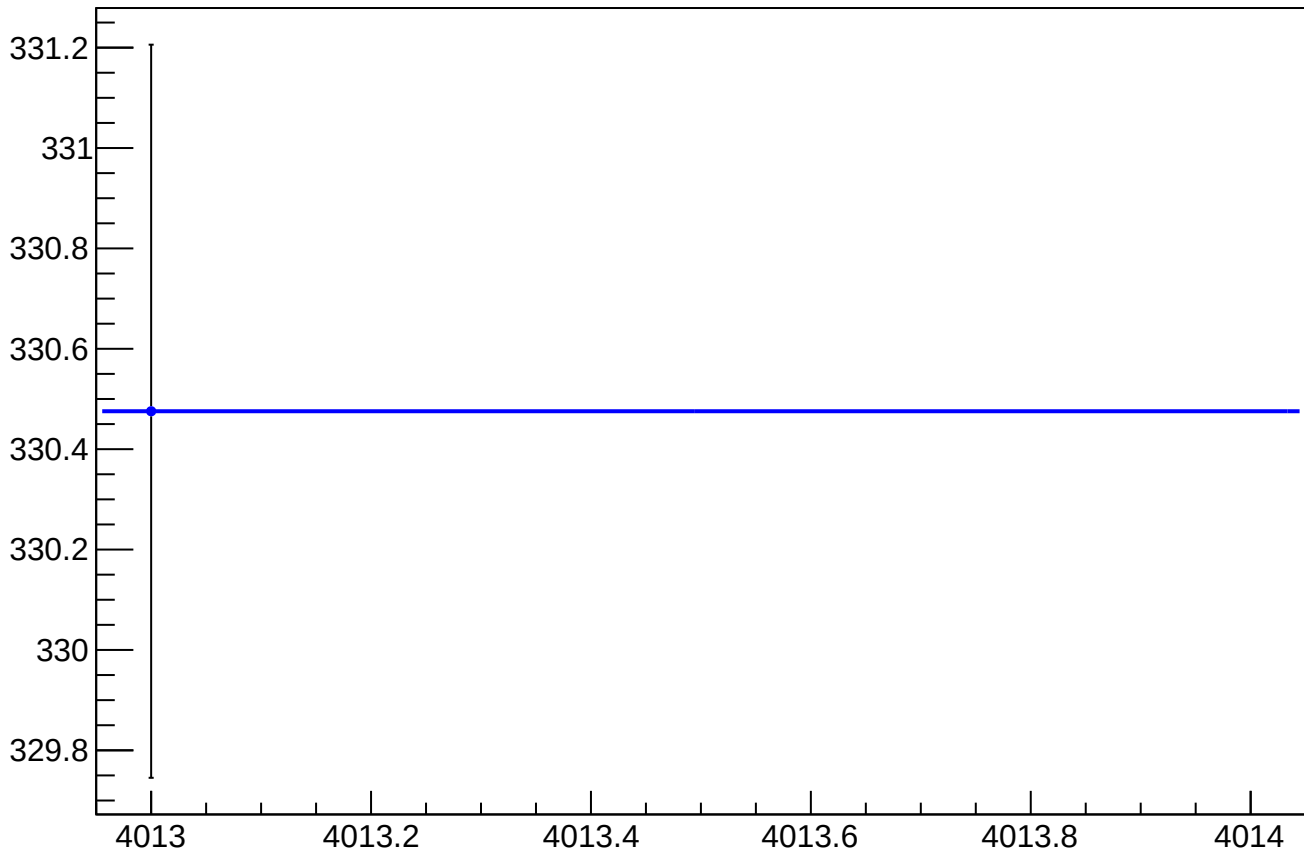
asym_us_avg_atlr_avg_avg_eigen_dit_vs_cor_diff_rms vs Slug, Sign Corrected
