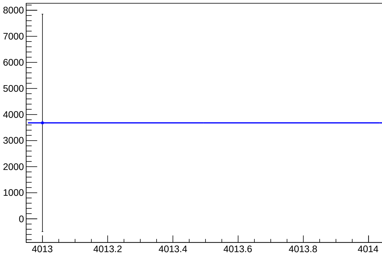
asym_usr_eigen_dit_correction_mean vs Slug, Sign Corrected
