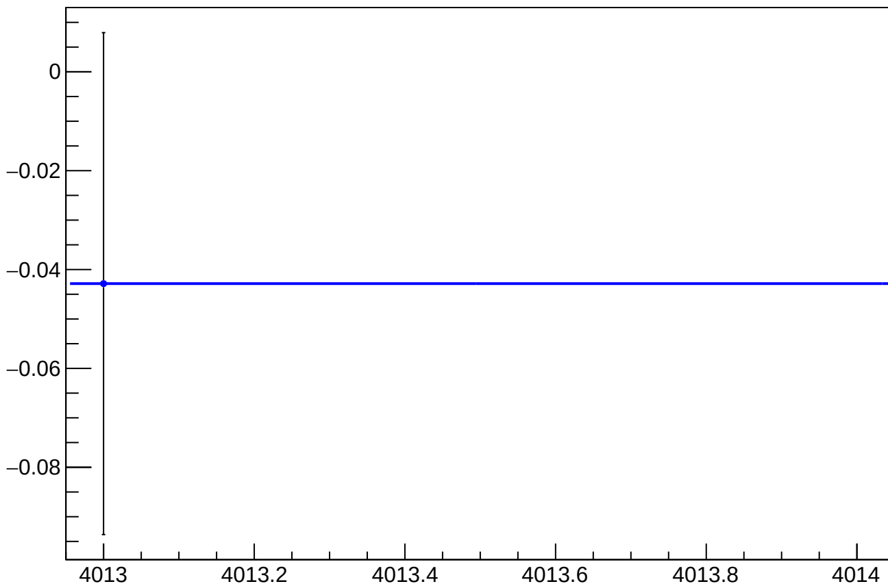
asym_at1_dd_at2_dd_avg_eigen_dit_vs_eigen_cor_diff_mean vs Slug, Sign Corrected
