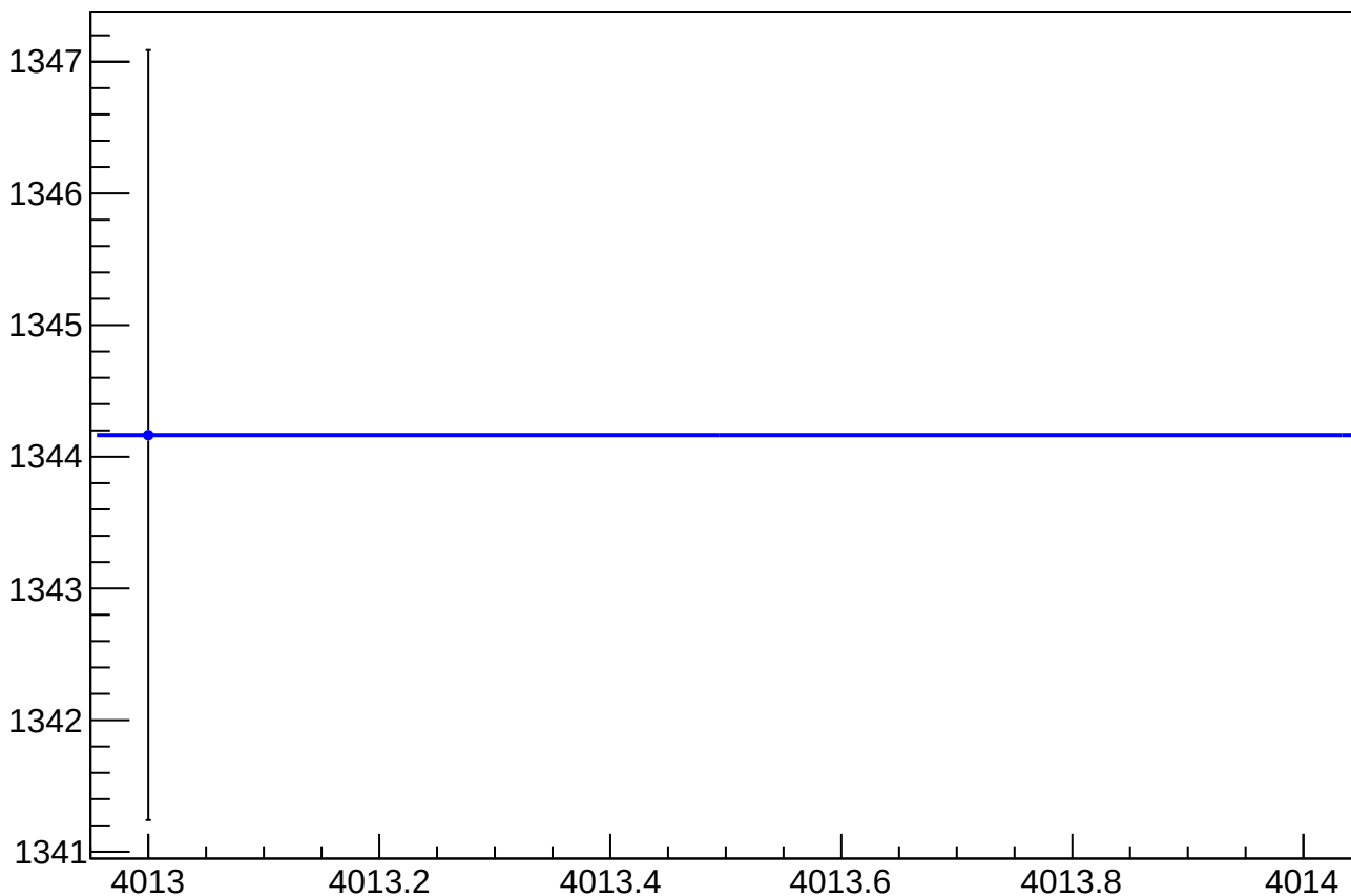
eigen_cor_asym_us_avg_at1lr_avg_dd_rms vs Slug, Sign Corrected
