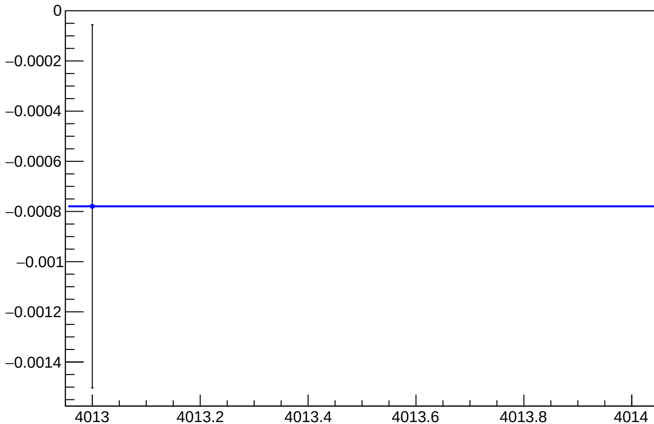
asym_atl1r2_dd_atl2r1_dd_avg_reg_vs_cor_diff_mean vs Slug, Sign Corrected
