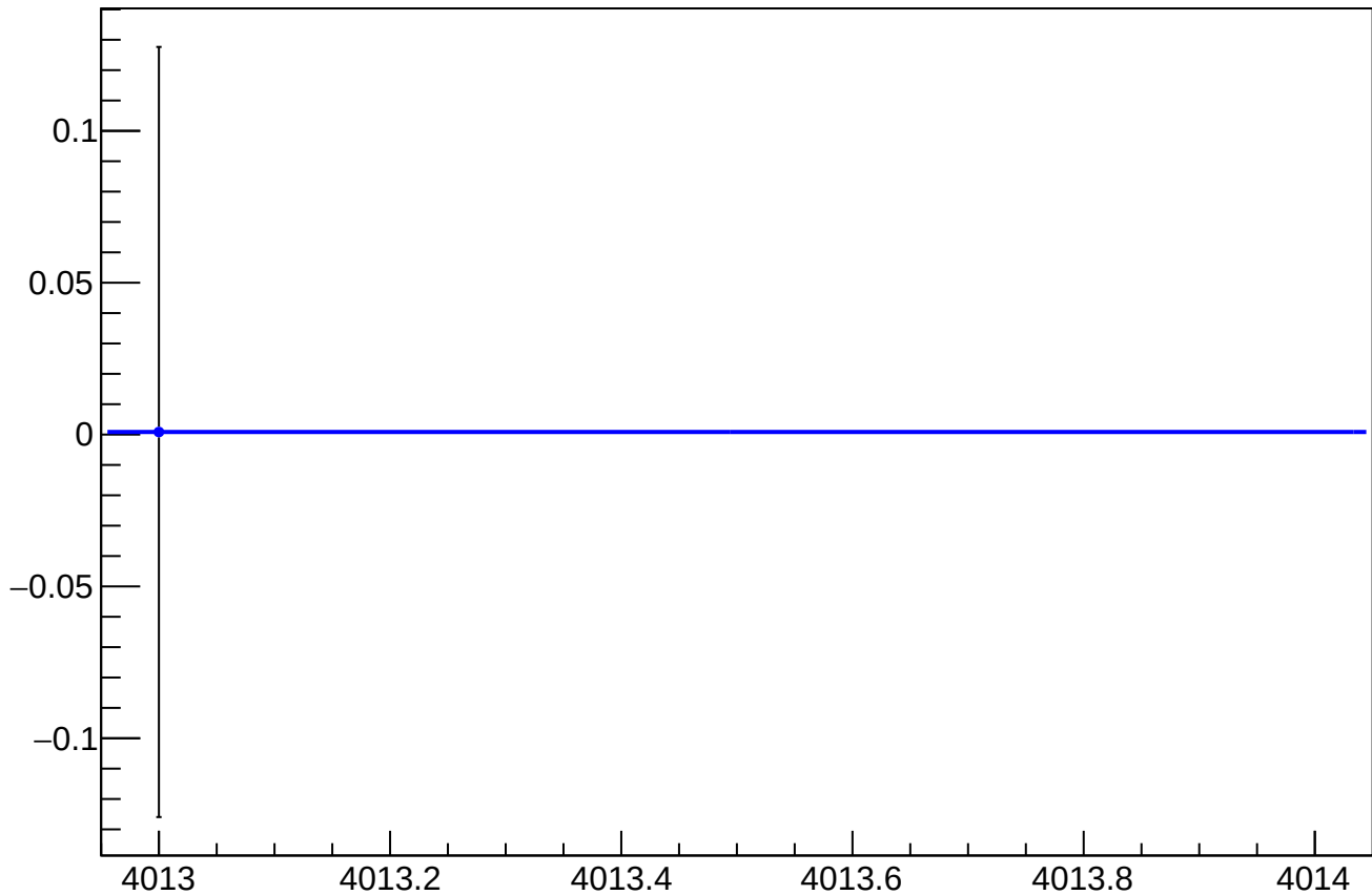
reg_asym_bcm_2an_us_an_ds_dd_diff_bpm4aY_slope vs Slug, Sign Corrected
