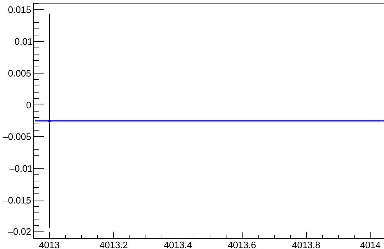
reg_asym_bcm_2an_us_an_ds_avg_diff_bpm12X_slope vs Slug, Sign Corrected
