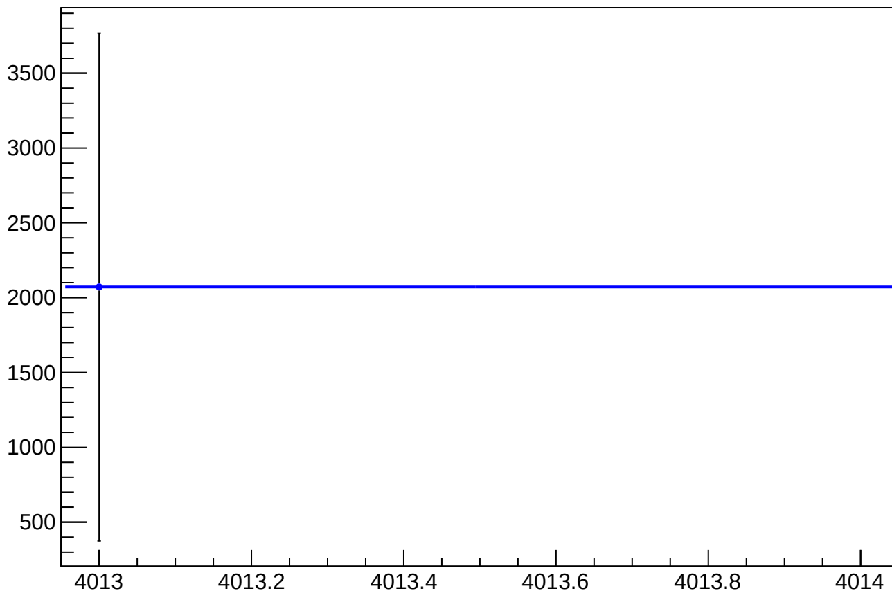
asym_sam_15_26_dd_eigen_cor_correction_mean vs Slug, Sign Corrected
