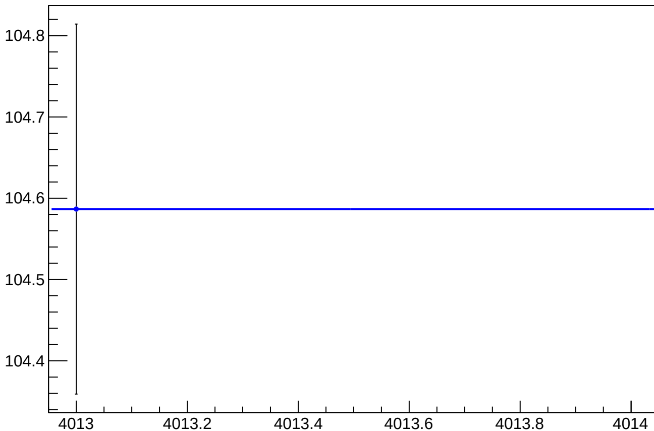
eigen_cor_asym_sam_15_avg_rms vs Slug, Sign Corrected
