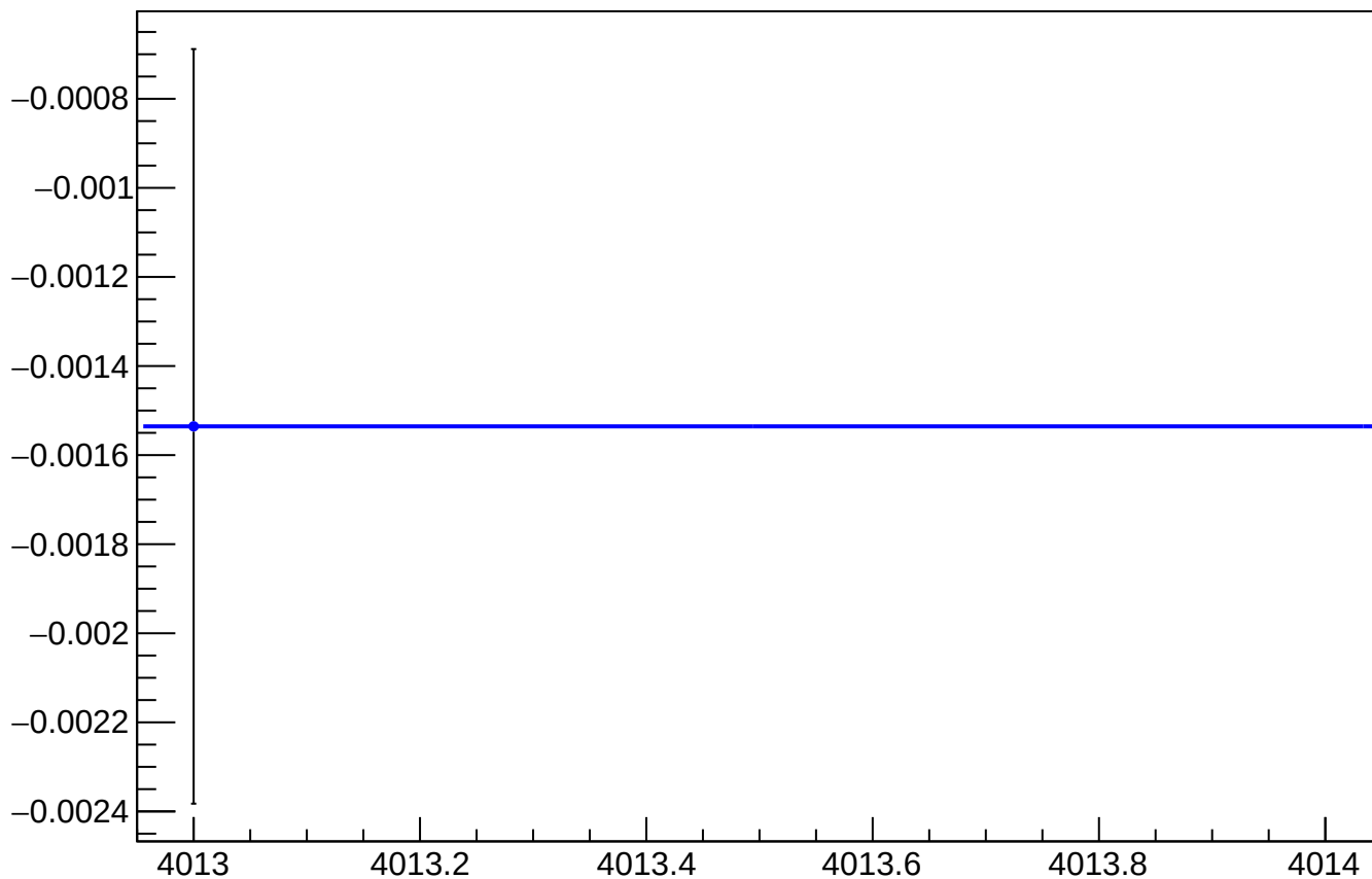
asym_at2_avg_reg_vs_cor_diff_mean vs Slug, Sign Corrected
