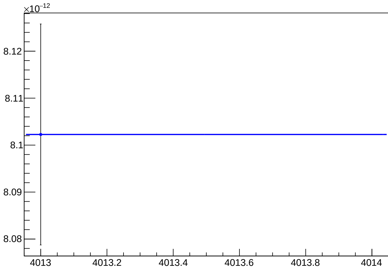
asym_sam_37_dd_eigen_cor_vs_cor_diff_rms vs Slug, Sign Corrected
