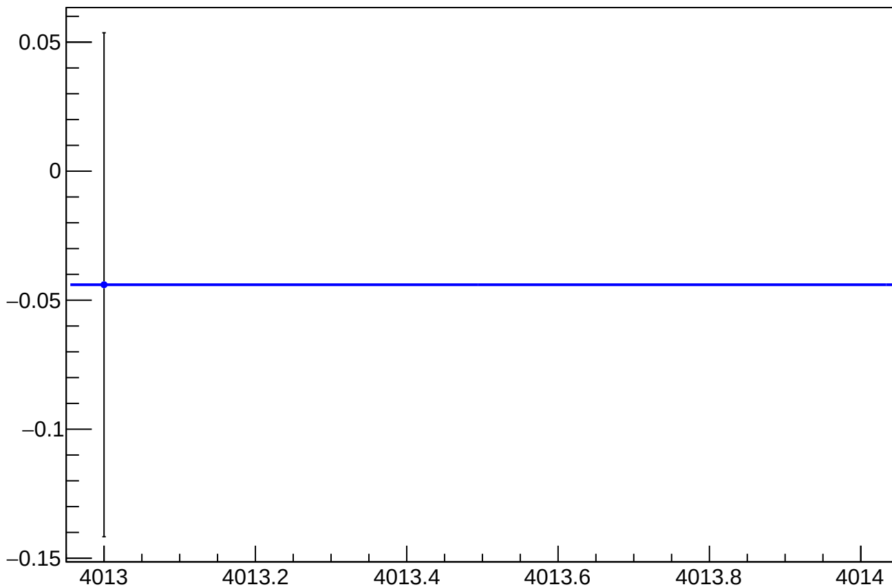
asym usl atl1 dd dit vs cor diff mean vs Slug, Sign Corrected
