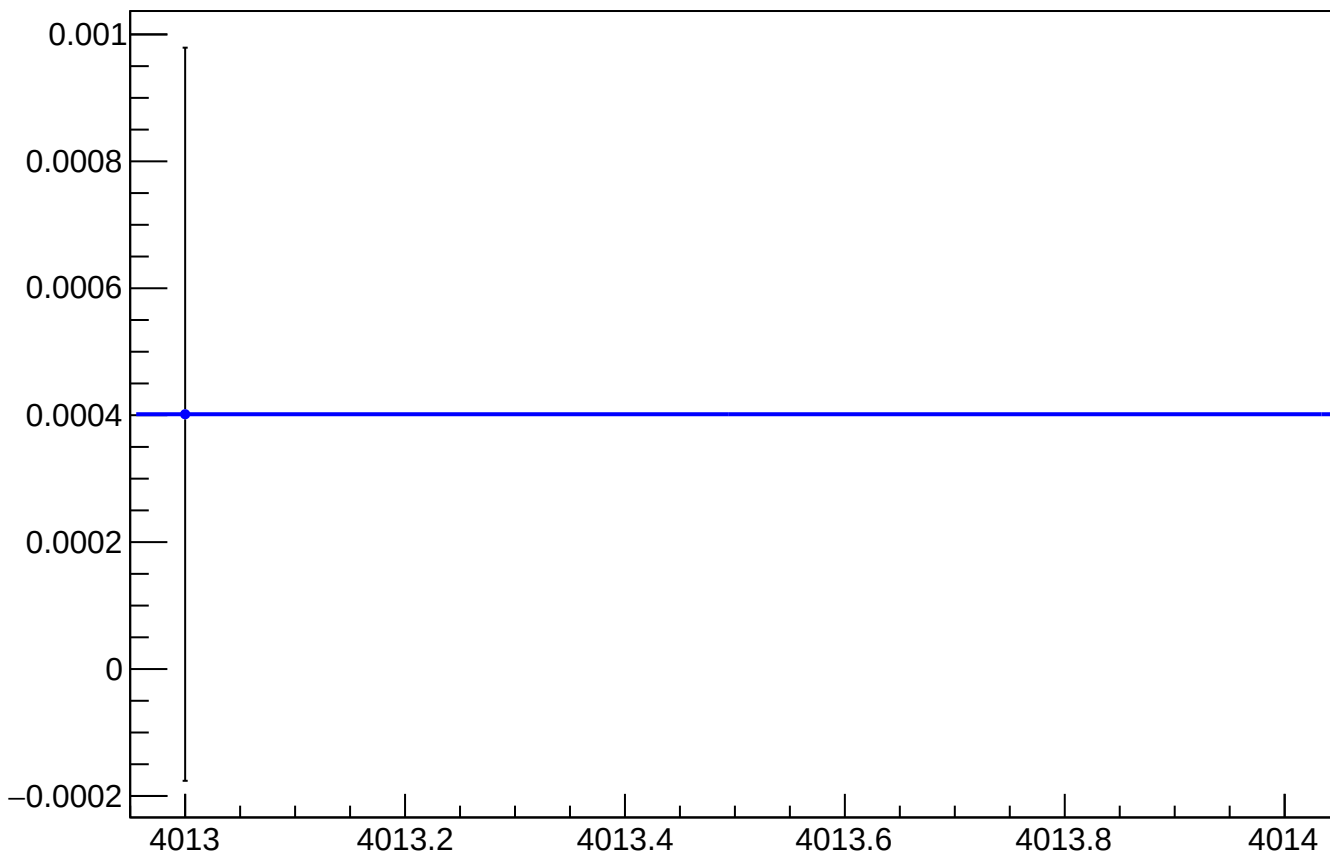
asym_usr_atr2_dd_reg_vs_cor_diff_mean vs Slug, Sign Corrected
