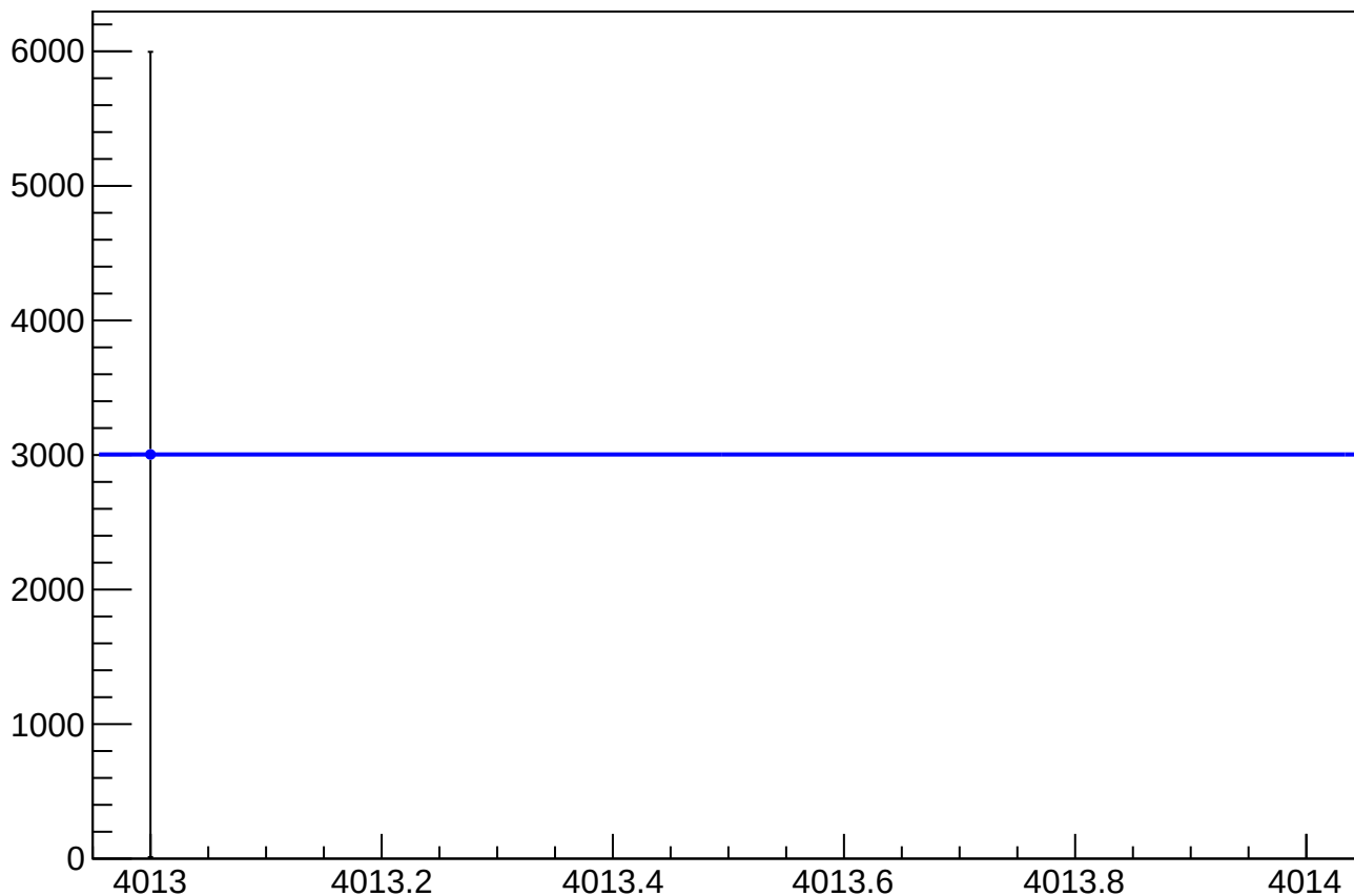
asym_atl1_eigen_dit_correction_mean vs Slug, Sign Corrected
