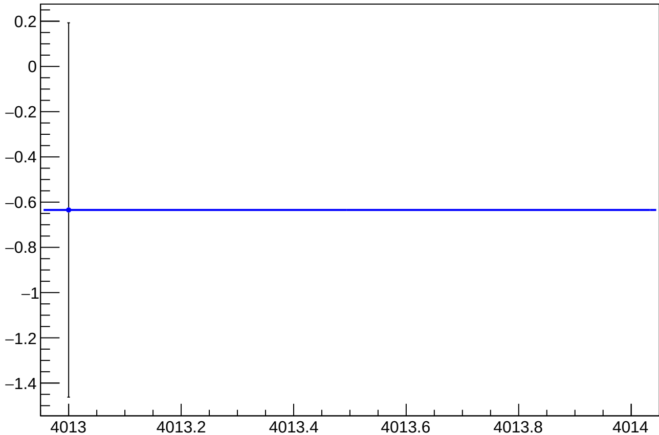
asym_atl_avg_atr_avg_avg_dit_vs_eigen_cor_diff_mean vs Slug, Sign Corrected
