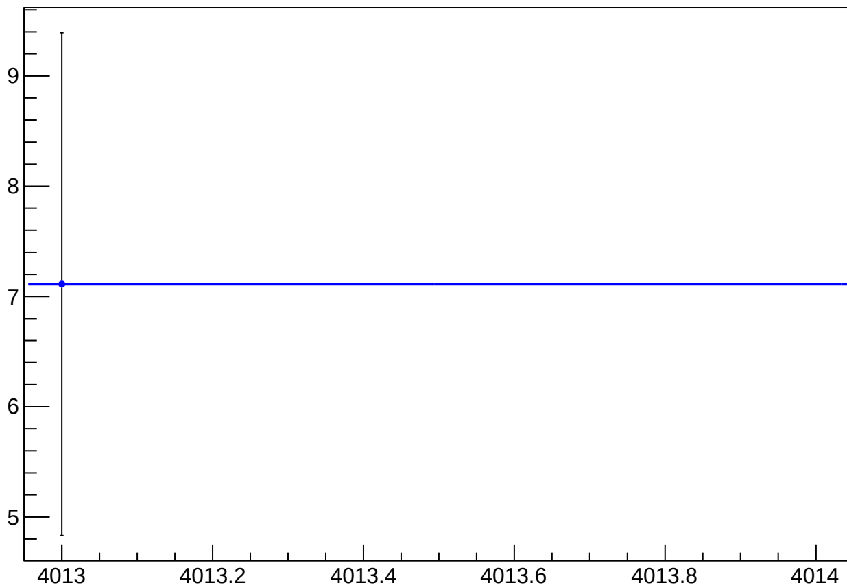
reg_asym_atl_avg_atr_avg_dd_diff_bpm4eY_slope vs Slug, Sign Corrected
