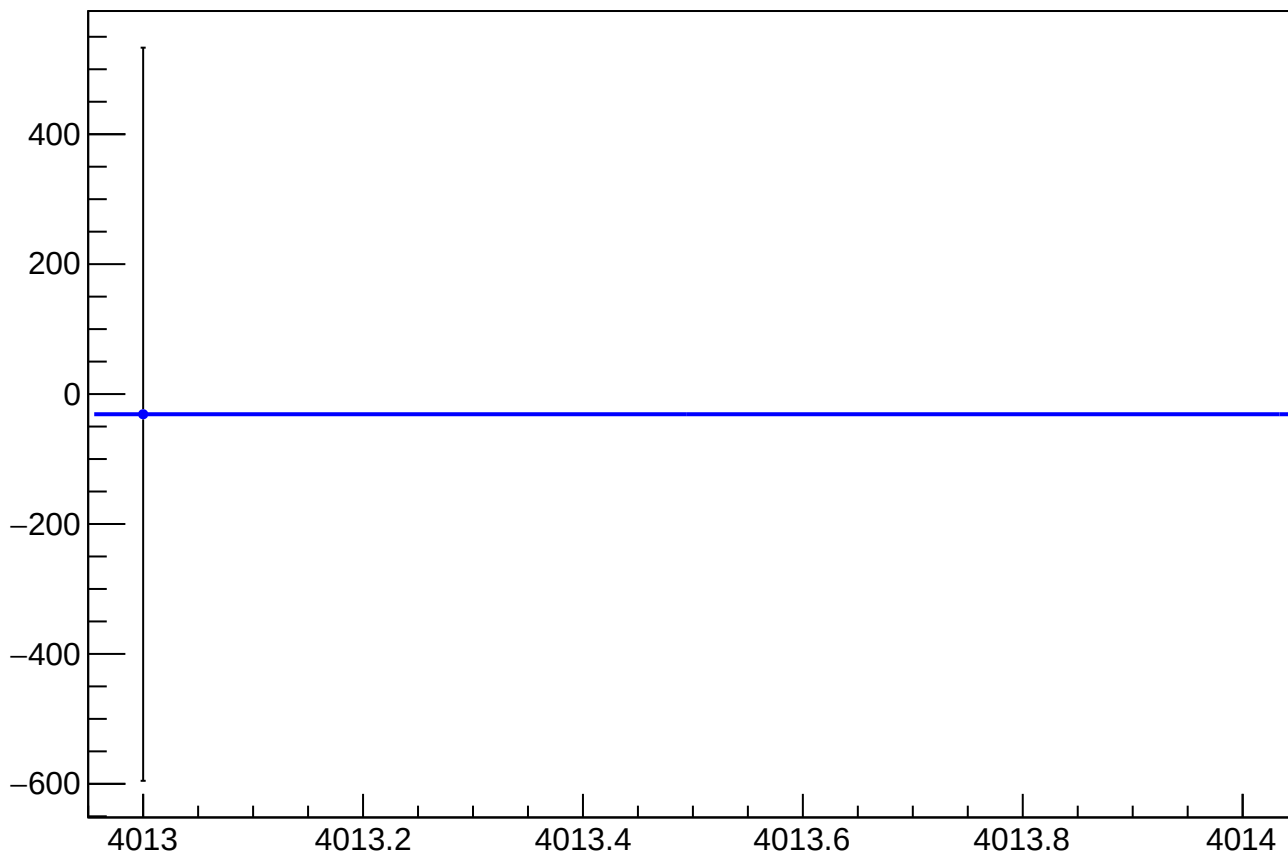
asym_sam1_dit_correction_mean vs Slug, Sign Corrected
