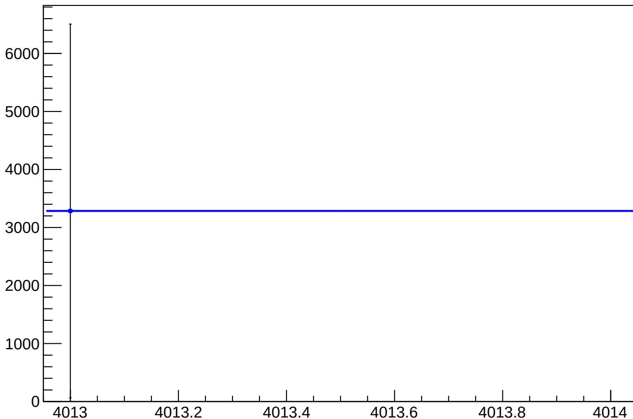
reg_asym_atl_dd_atr_dd_avg_mean vs Slug, Sign Corrected
