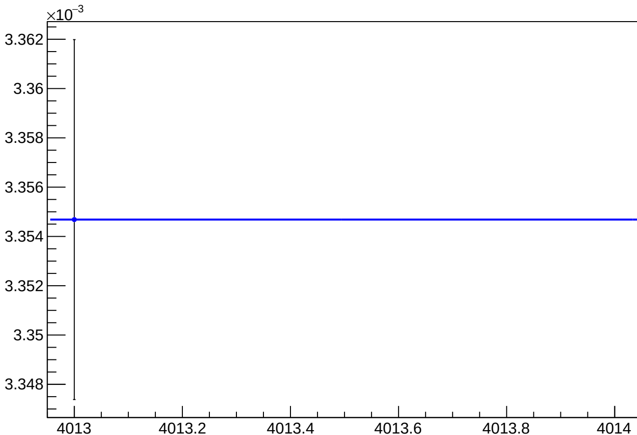
asym_sam_3748_avg_eigen_dit_vs_dit_diff_rms vs Slug, Sign Corrected
