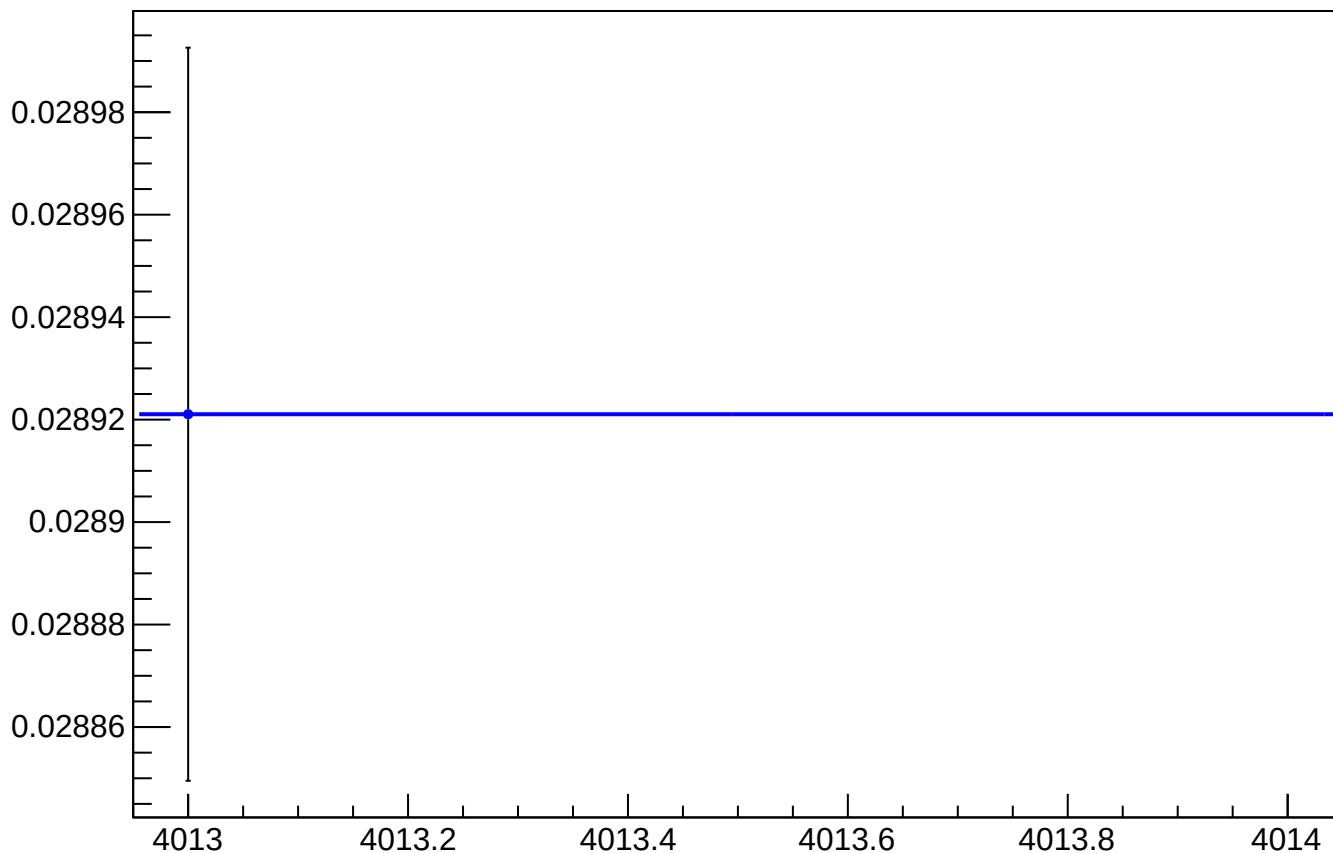
asym_sam6_reg_vs_cor_diff_rms vs Slug, Sign Corrected
