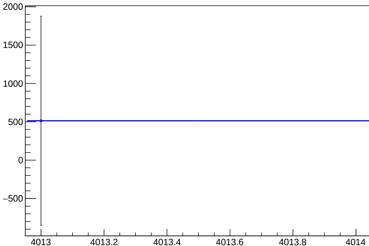
asym_us_dd_at1lr_dd_avg_eigen_dit_correction_mean vs Slug, Sign Corrected
