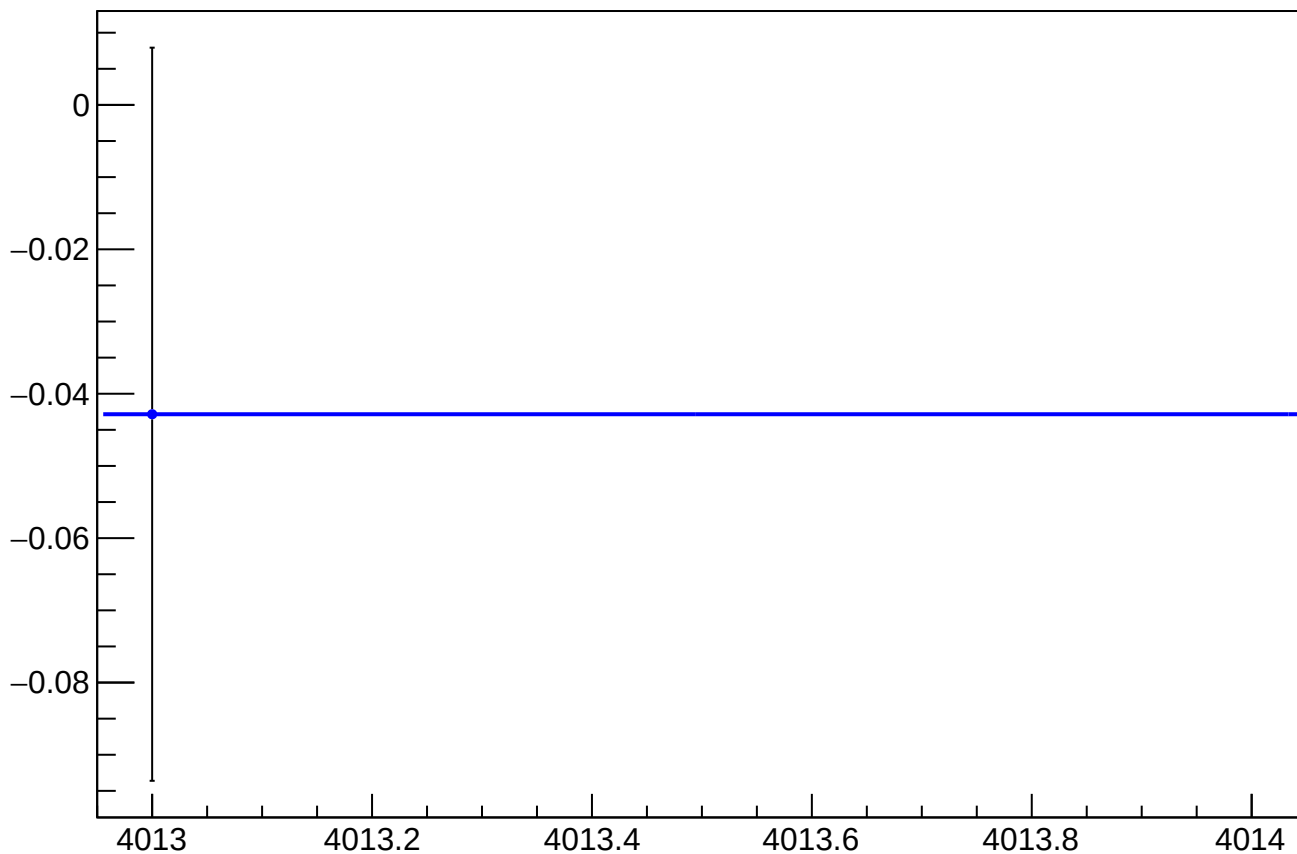
asym_at1_dd_at2_dd_avg_dit_vs_eigen_cor_diff_mean vs Slug, Sign Corrected
