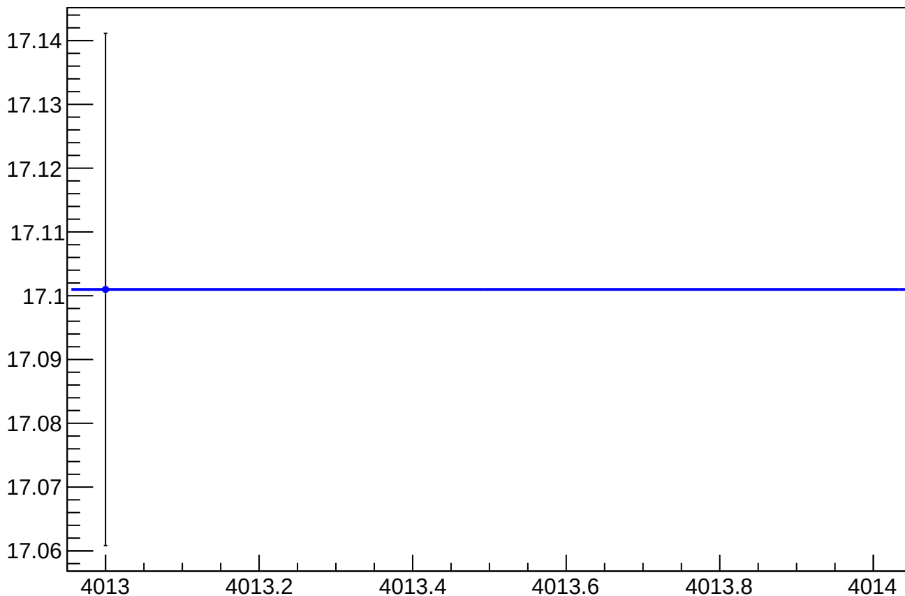
asym_us_dd_eigen_dit_vs_cor_diff_rms vs Slug, Sign Corrected
