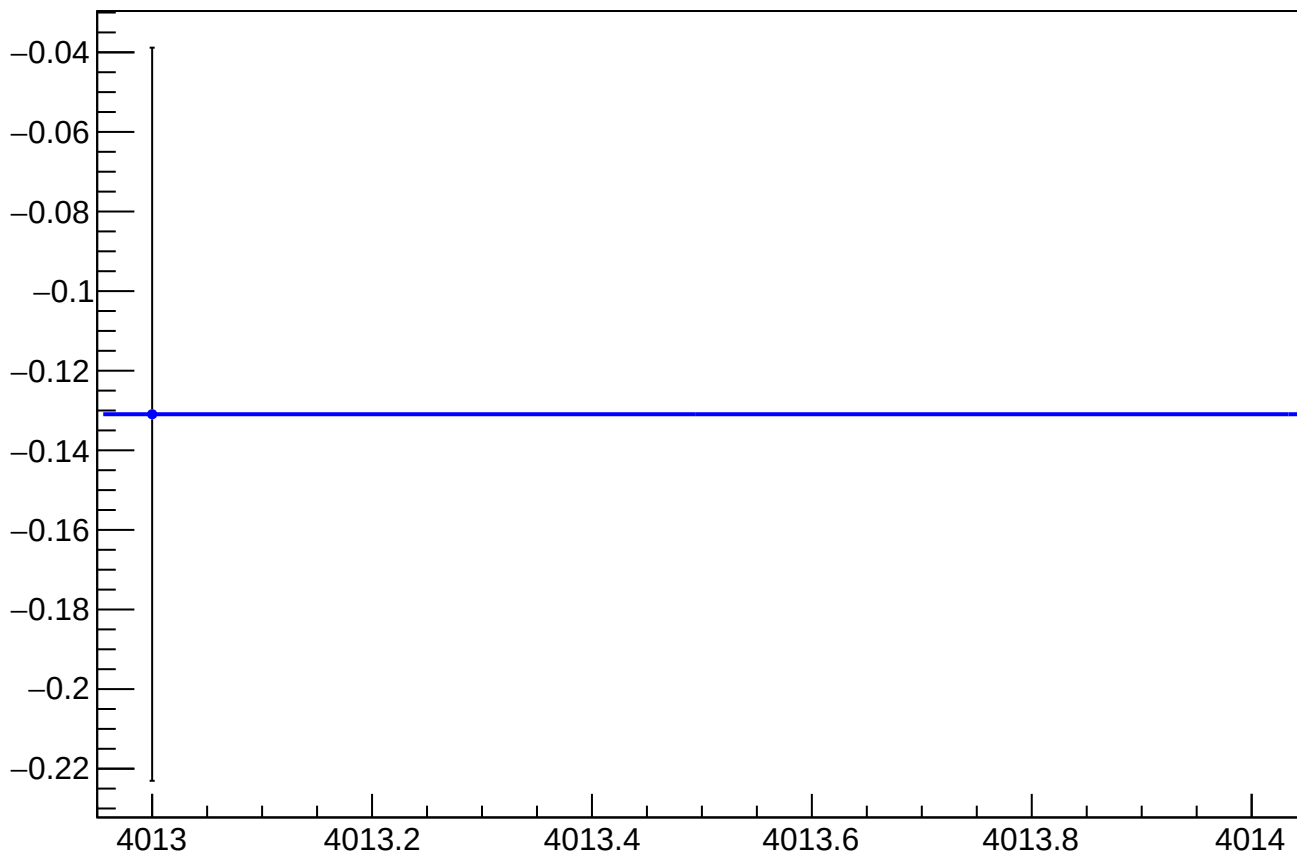
asym_at1_dd_eigen_dit_vs_cor_diff_mean vs Slug, Sign Corrected
