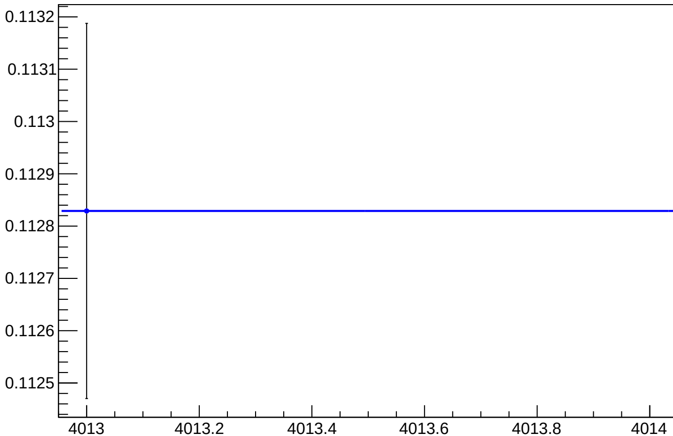
asym_at1_avg_reg_vs_cor_diff_rms vs Slug, Sign Corrected
