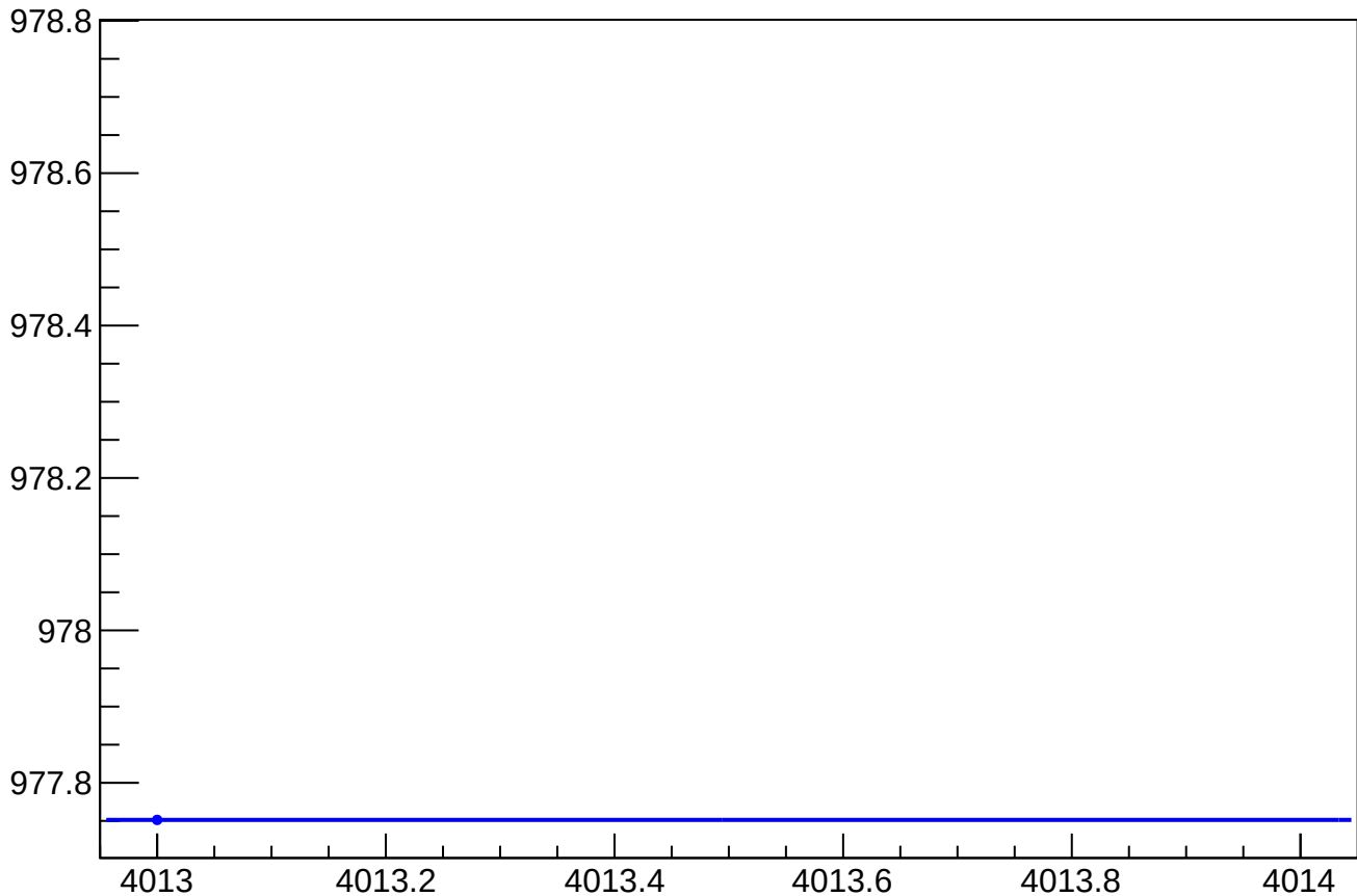
HacR_Q3_HP3458A_IOUT_mean vs Slug, Sign Corrected
