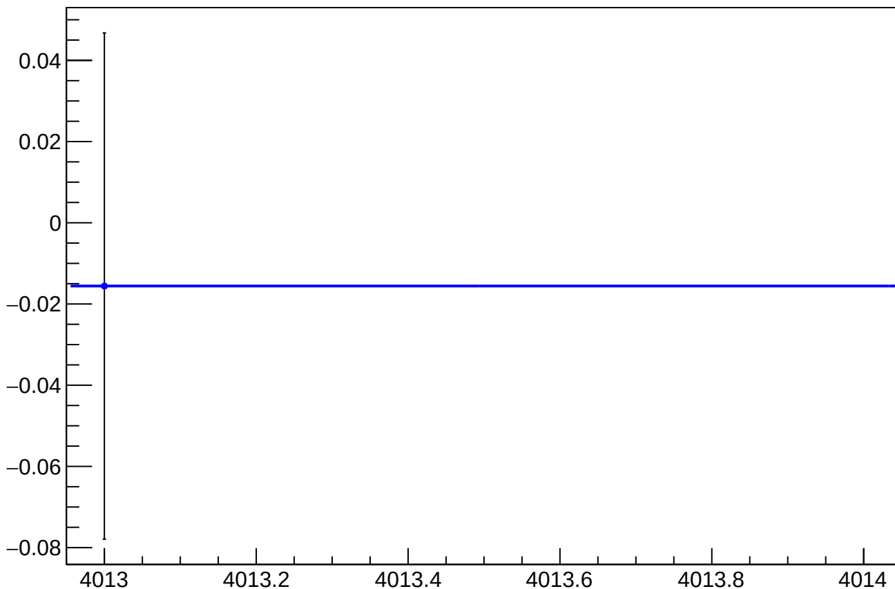
asym_atl_avg_atr_avg_dd_eigen_dit_vs_cor_diff_mean vs Slug, Sign Corrected
