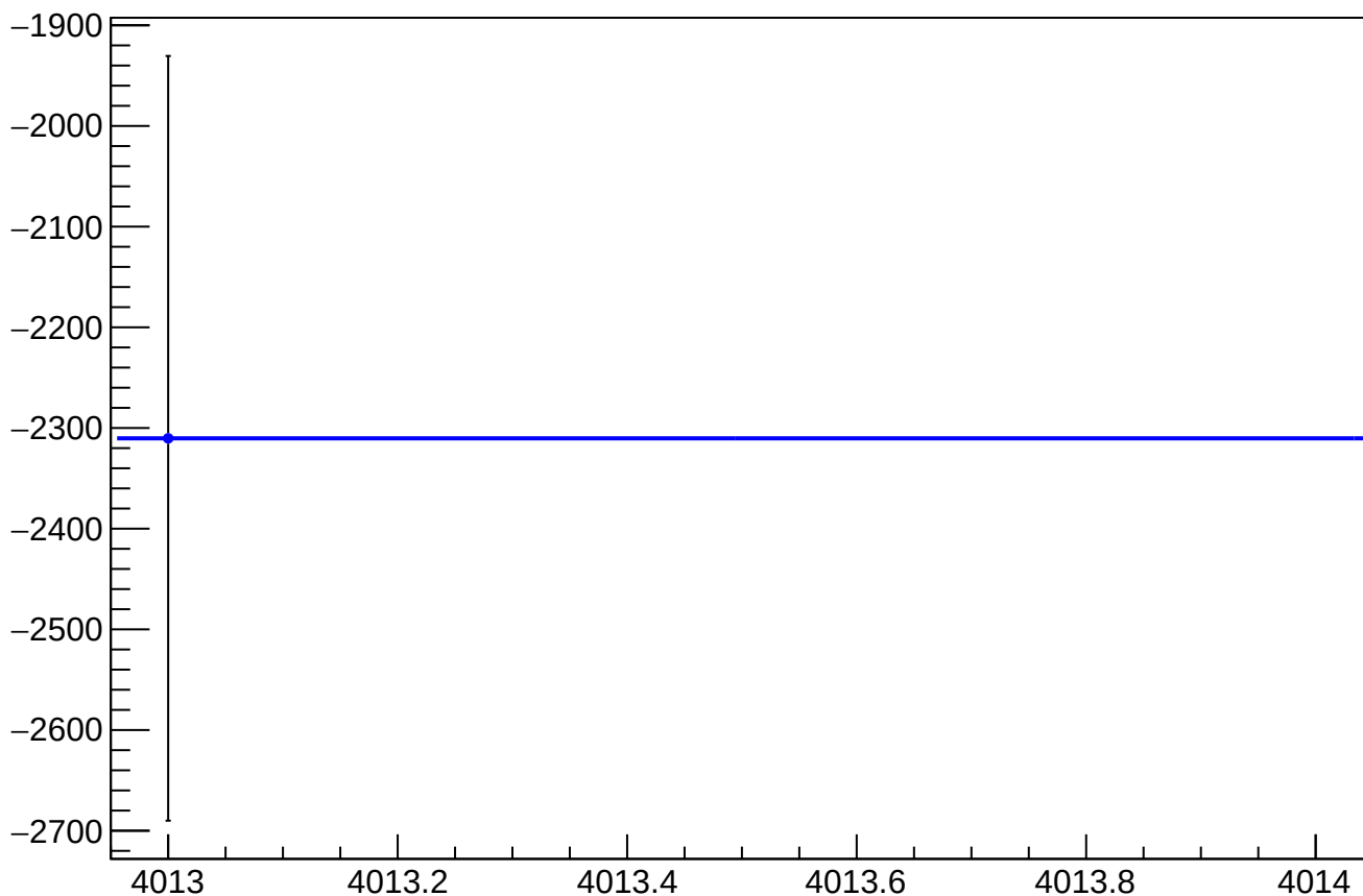
cor_asym_sam_37_dd_mean vs Slug, Sign Corrected
