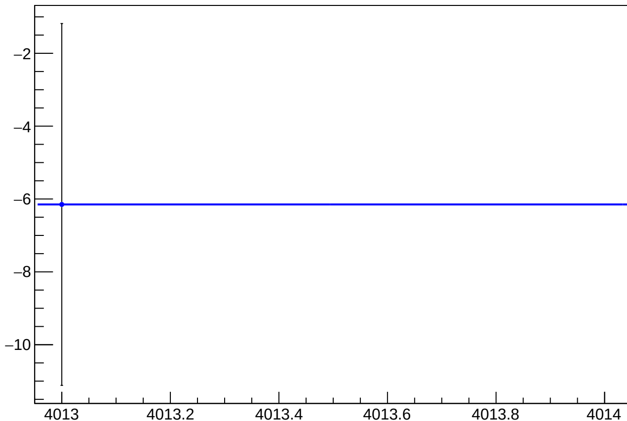
reg_asym_us_dd_at1lr_dd_avg_diff_bpm4eX_slope vs Slug, Sign Corrected
