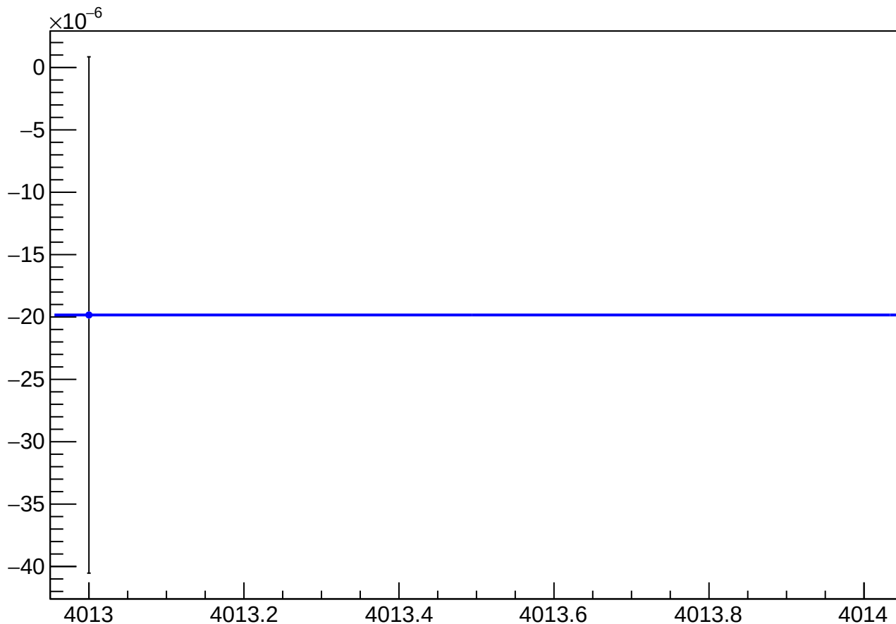
asym_us_dd_atlr_dd_avg_eigen_dit_vs_dit_diff_mean vs Slug, Sign Corrected
