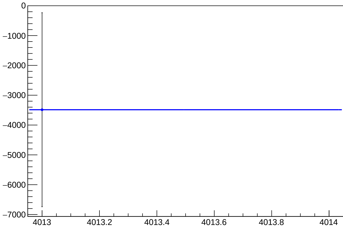
asym_sam_24_68_dd_reg_correction_mean vs Slug, Sign Corrected
