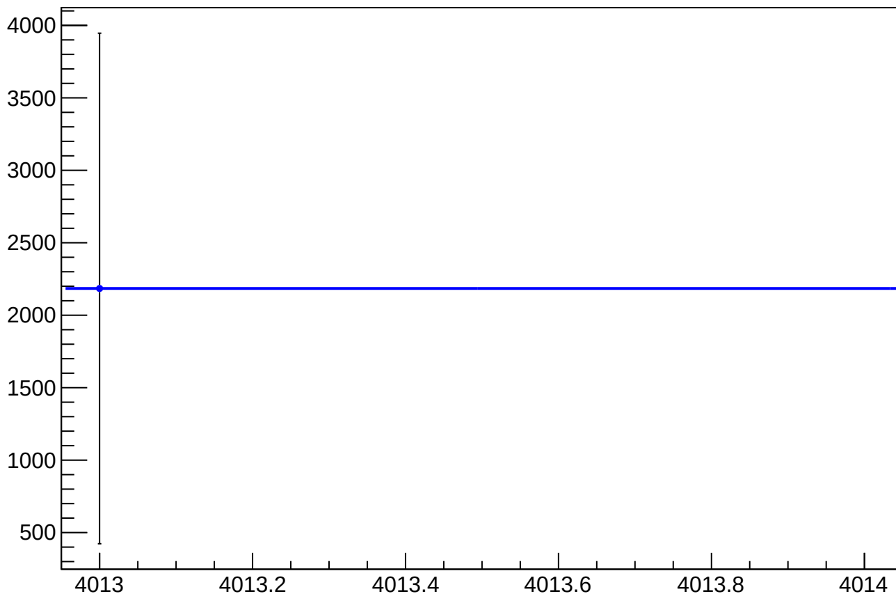
asym_sam_15_26_dd_eigen_dit_correction_mean vs Slug, Sign Corrected
