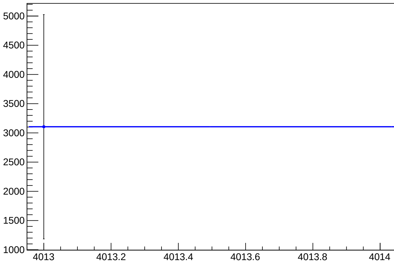
eigen_dit_asym_sam2_mean vs Slug, Sign Corrected
