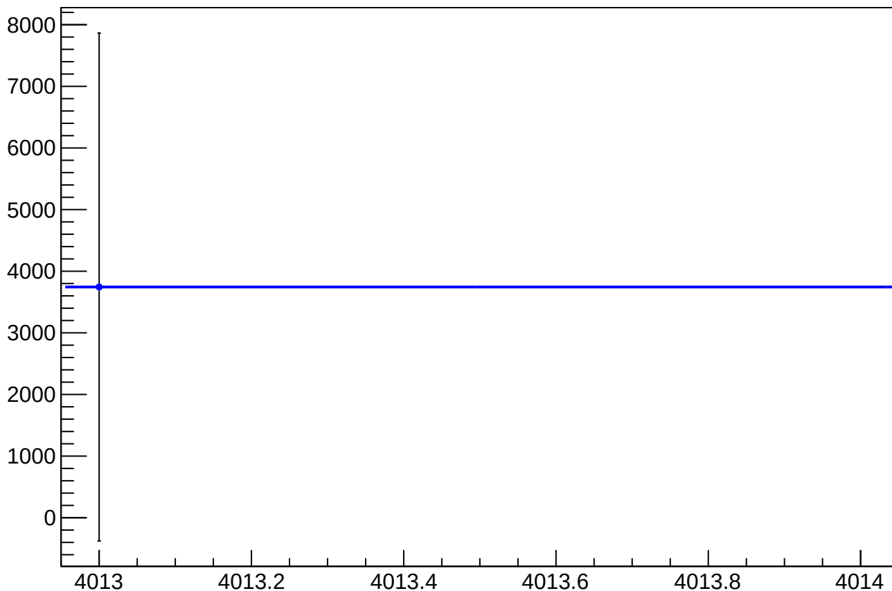
cor_asym_us_dd_at1lr_dd_dd_mean vs Slug, Sign Corrected
