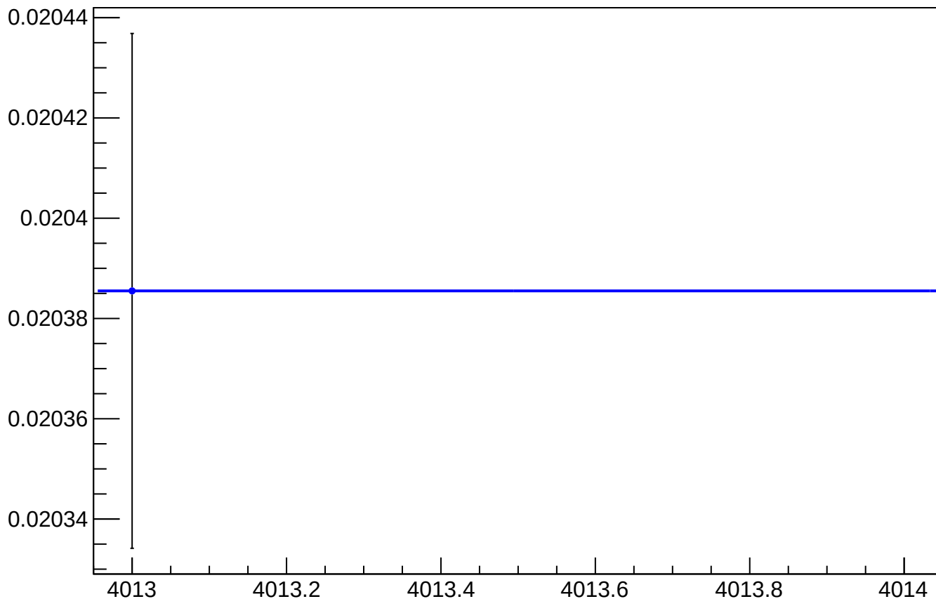
asym_sam_48_dd_reg_vs_cor_diff_rms vs Slug, Sign Corrected
