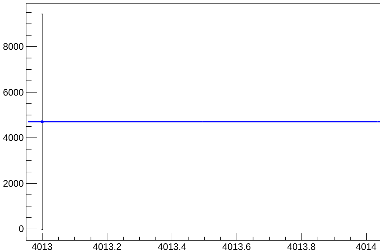
eigen_dit_asym_atr1l2_avg_mean vs Slug, Sign Corrected
