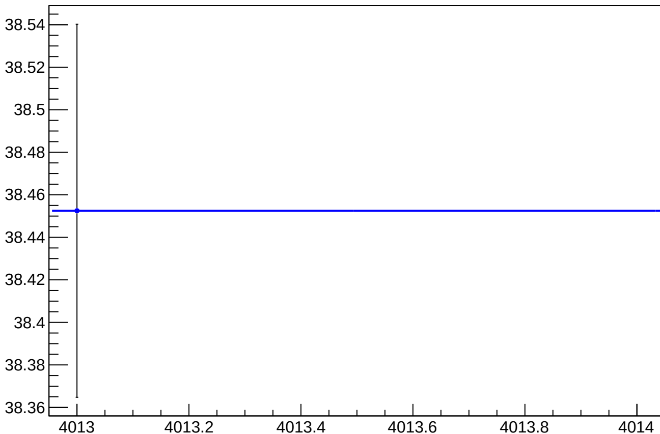
asym_sam_12345678_avg_dit_vs_eigen_cor_diff_rms vs Slug, Sign Corrected
