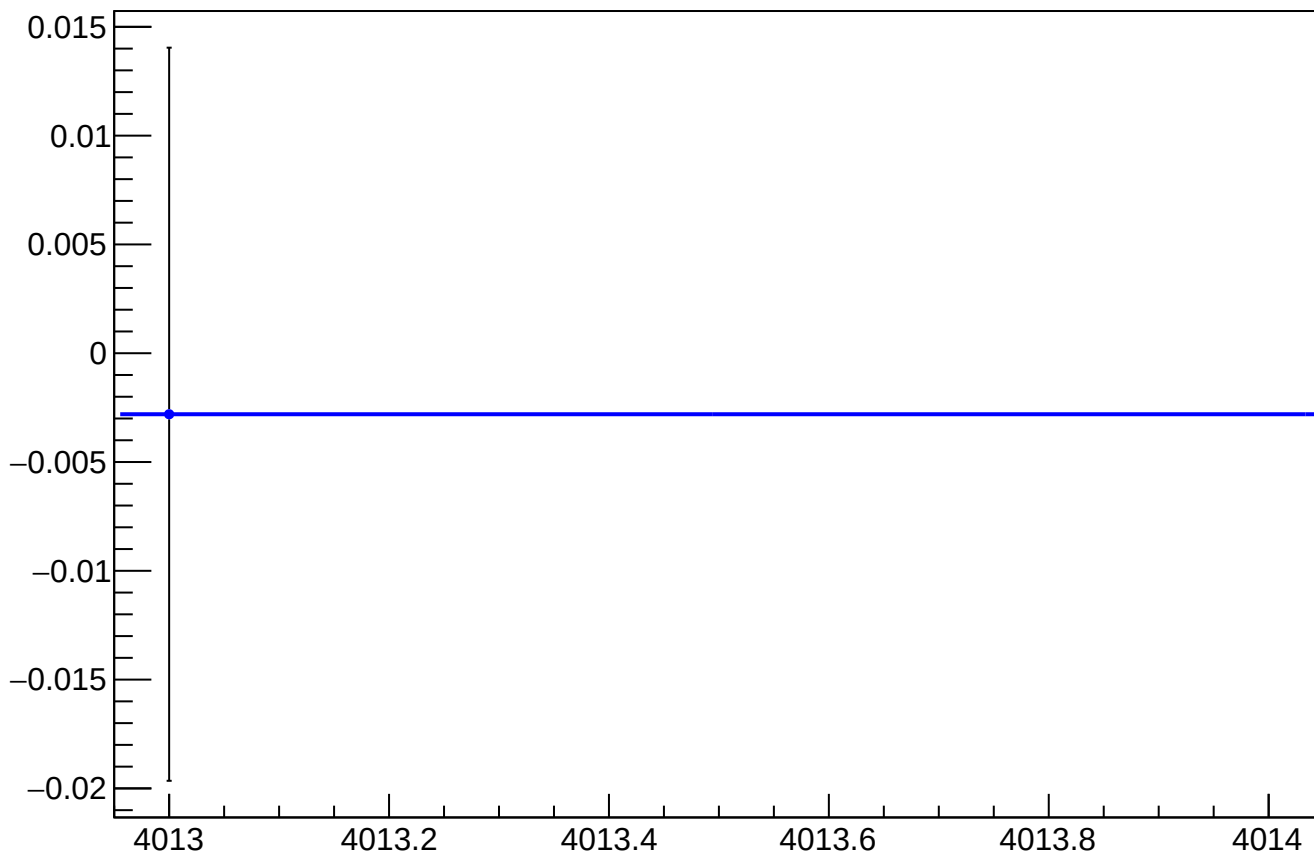
reg_asym_bcm_an_us_an_ds_avg_diff_bpm12X_slope vs Slug, Sign Corrected
