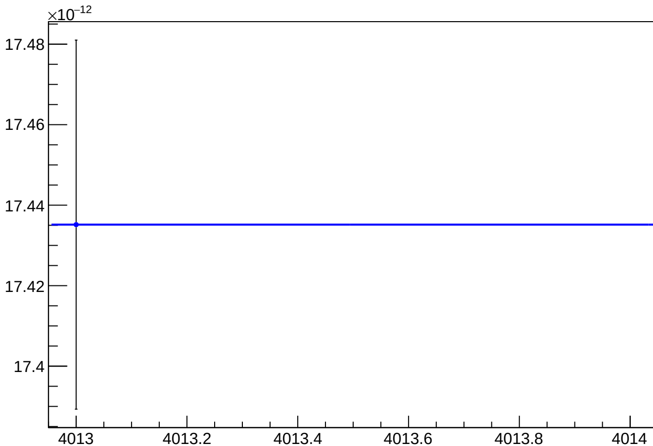
asym_sam_24_68_dd_eigen_cor_vs_cor_diff_rms vs Slug, Sign Corrected
