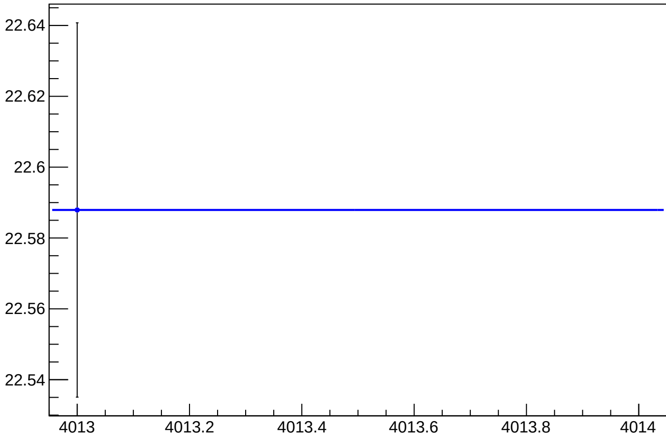
asym_us_dd_atlr_dd_dd_dit_vs_cor_diff_rms vs Slug, Sign Corrected
