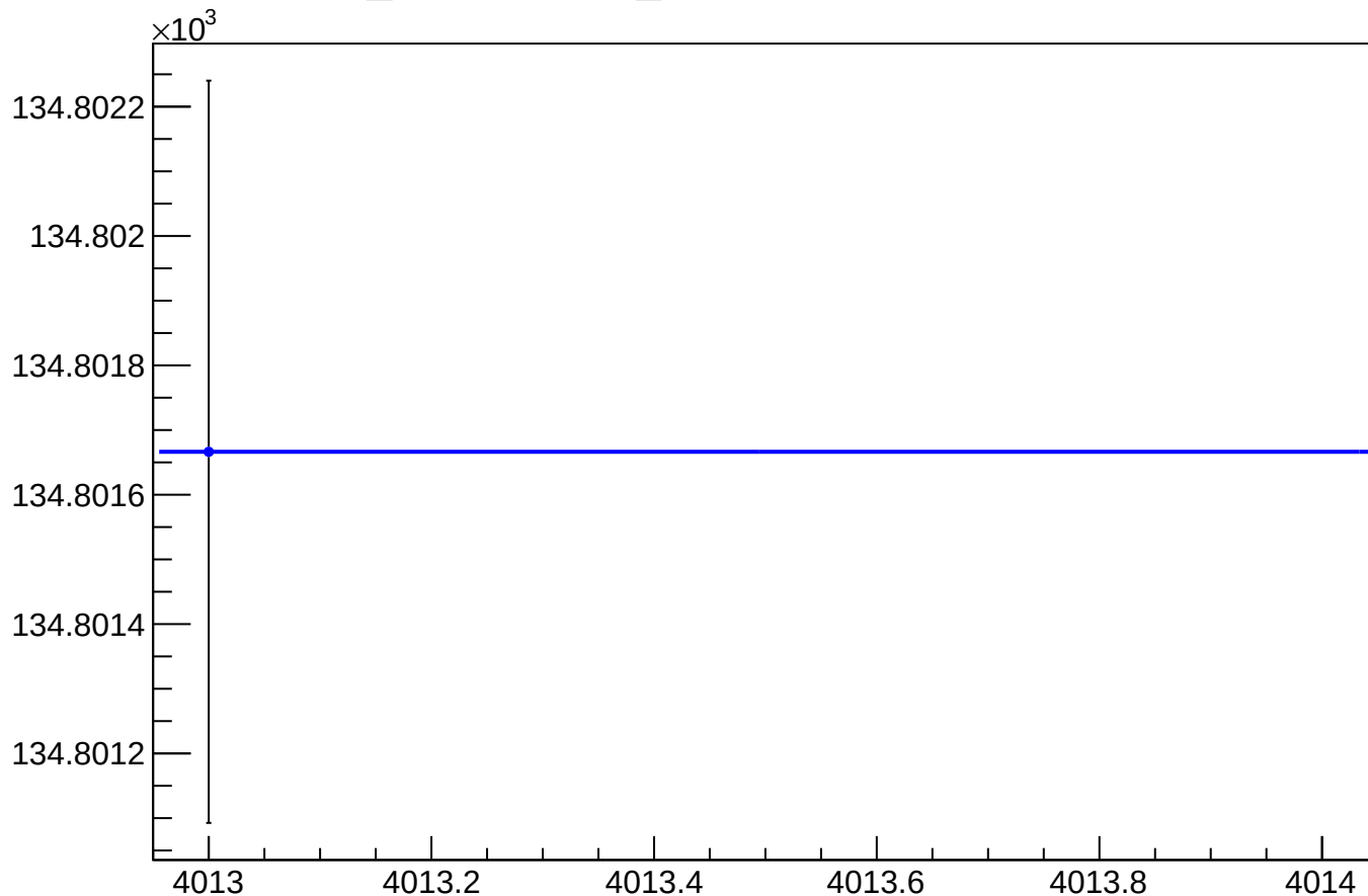
yield_bpm0l04WS_mean vs Slug, Sign Corrected
