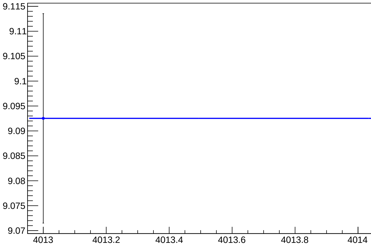
asym_sam1_dit_vs_eigen_cor_diff_rms vs Slug, Sign Corrected
