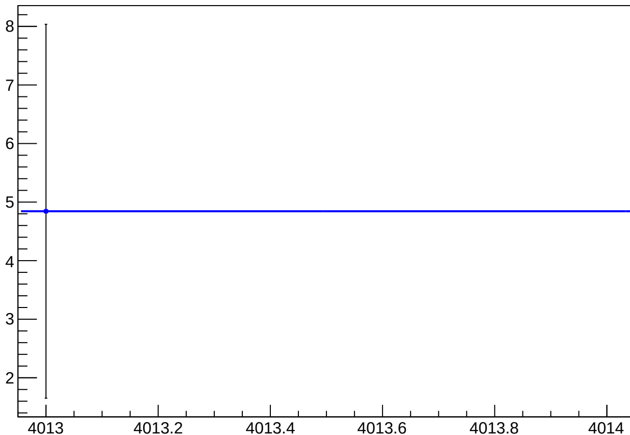
reg_asym_us_dd_atlr_dd_avg_diff_bpm4eY_slope vs Slug, Sign Corrected
