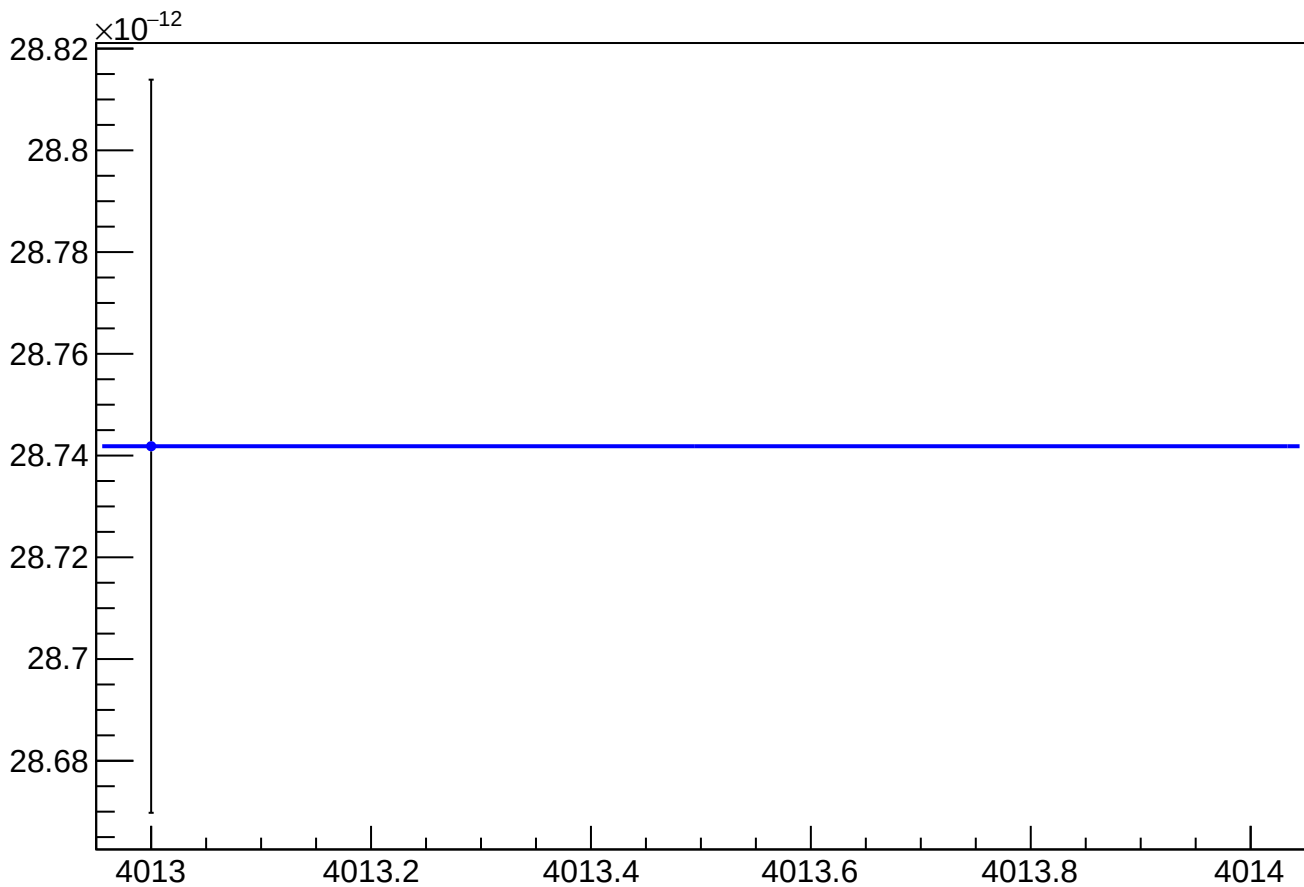
asym_sam_48_dd_eigen_cor_vs_cor_diff_rms vs Slug, Sign Corrected
