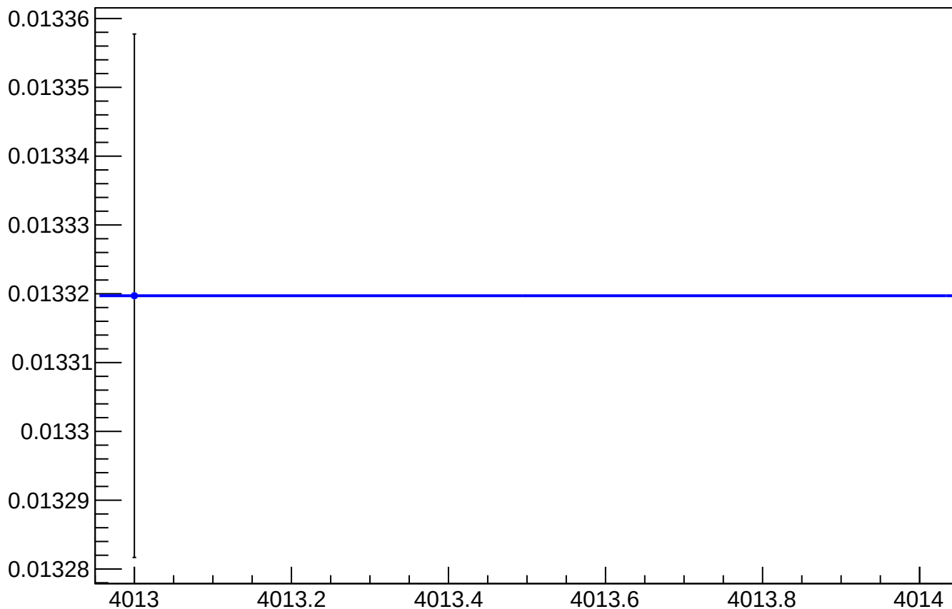
asym_sam_3726_avg_reg_vs_cor_diff_rms vs Slug, Sign Corrected
