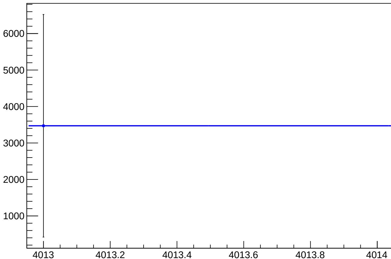
asym_sam6_eigen_dit_correction_mean vs Slug, Sign Corrected
