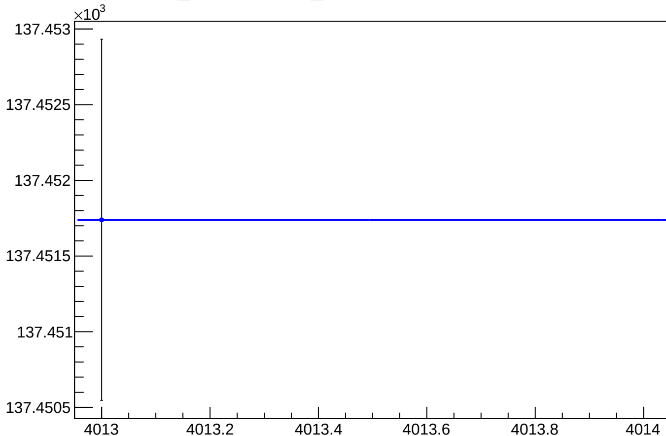
yield_bpm0r05WS_mean vs Slug, Sign Corrected
