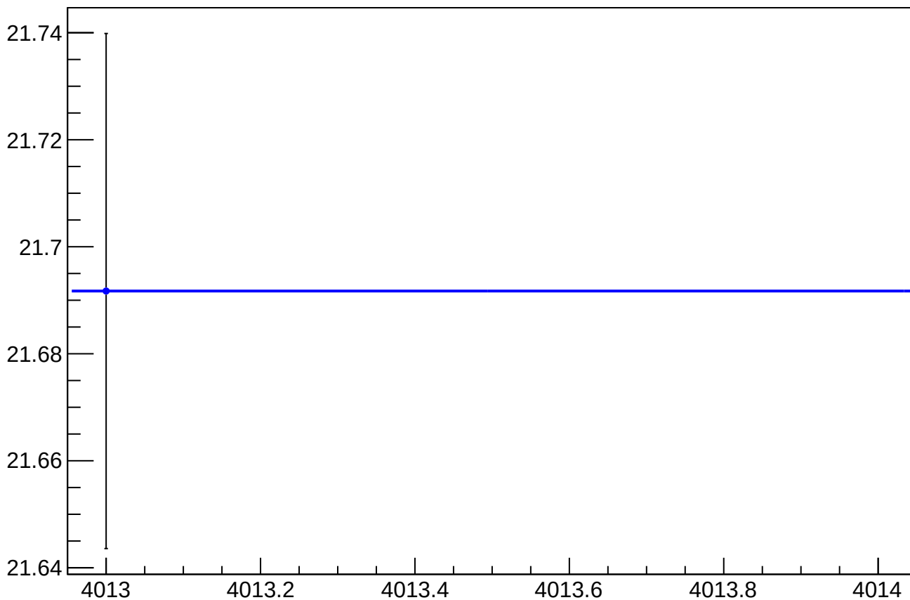
asym_sam_15_avg_dit_vs_cor_diff_rms vs Slug, Sign Corrected
