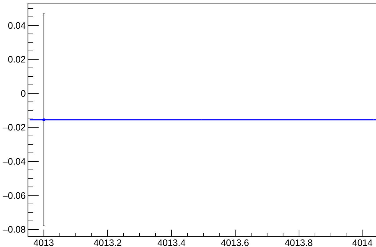
asym_atl1r2_dd_atl2r1_dd_avg_dit_vs_cor_diff_mean vs Slug, Sign Corrected
