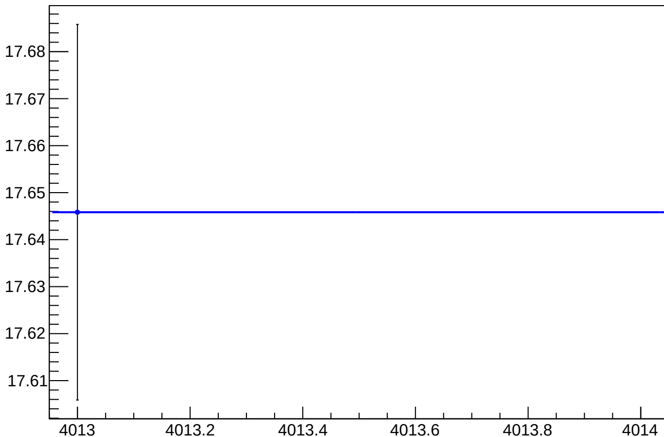
asym_sam_37_dd_dit_vs_cor_diff_rms vs Slug, Sign Corrected
