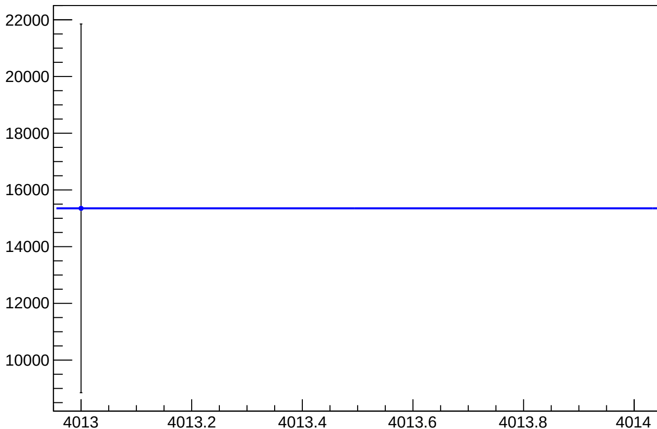
eigen_dit_asym_atr1_mean vs Slug, Sign Corrected
