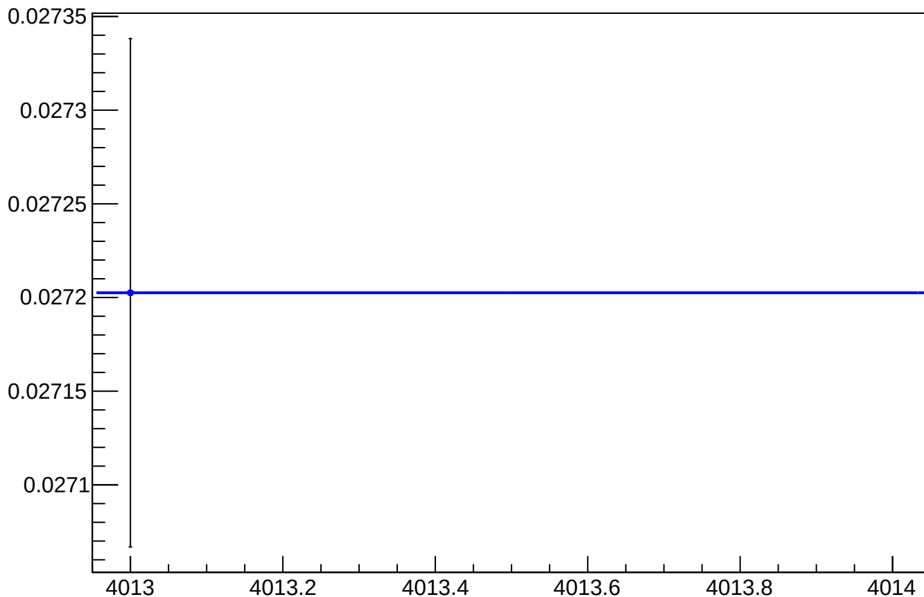
asym_atl1r2_dd_reg_vs_cor_diff_rms vs Slug, Sign Corrected
