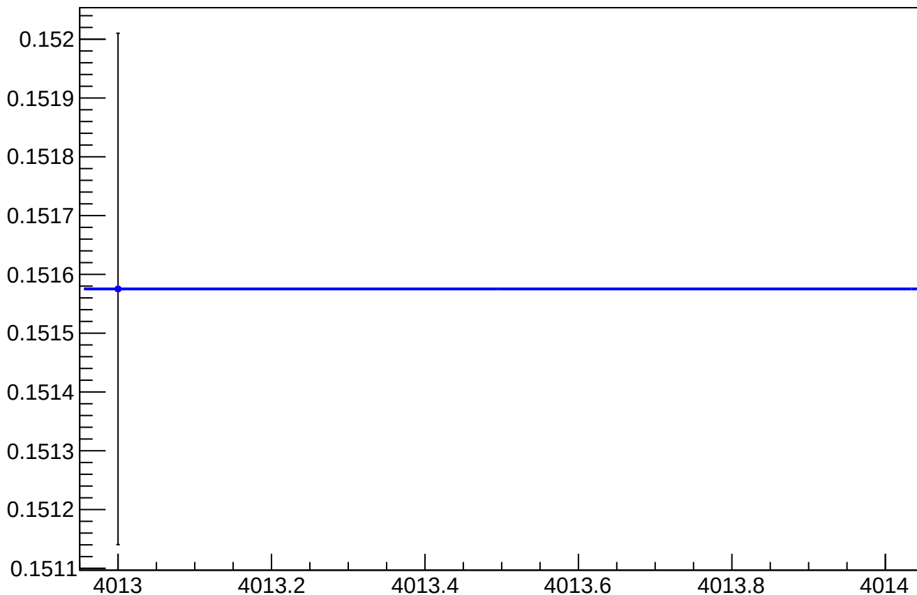
asym_usl_atl1_dd_reg_vs_cor_diff_rms vs Slug, Sign Corrected
