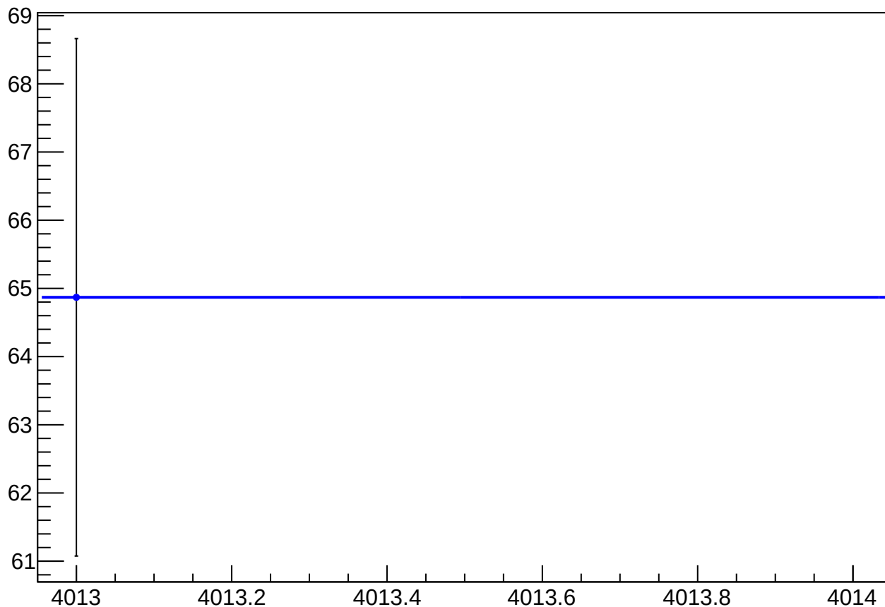
reg_asym_us_avg_diff_bpm4eX_slope vs Slug, Sign Corrected
