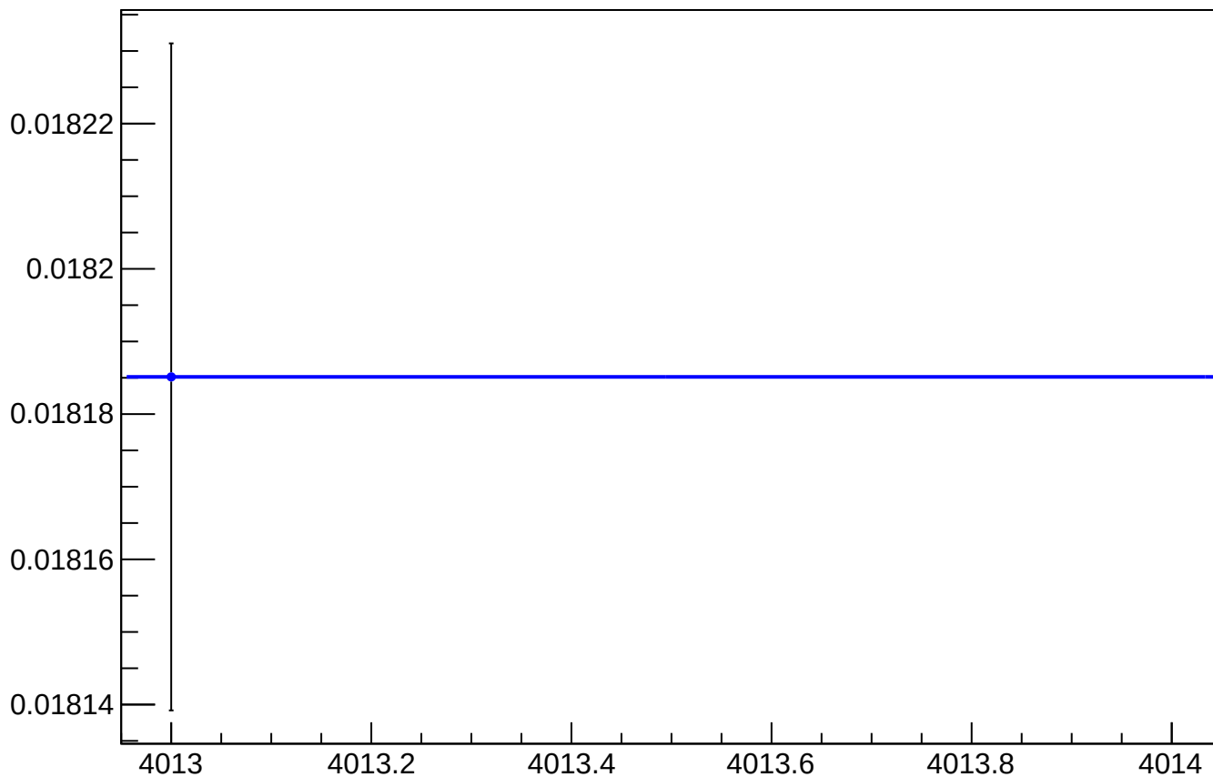
asym_sam_15_37_dd_reg_vs_cor_diff_rms vs Slug, Sign Corrected
