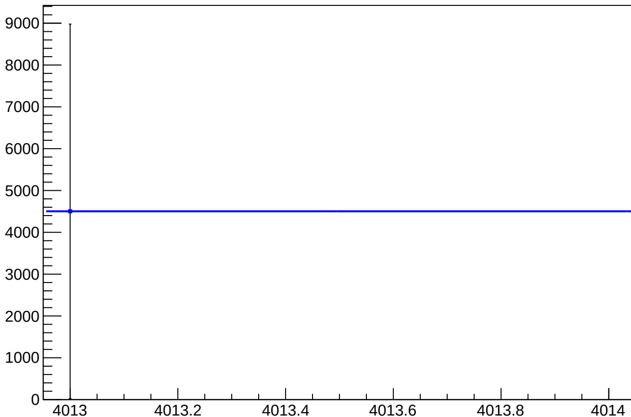
eigen_dit_asym_at2_dd_mean vs Slug, Sign Corrected
