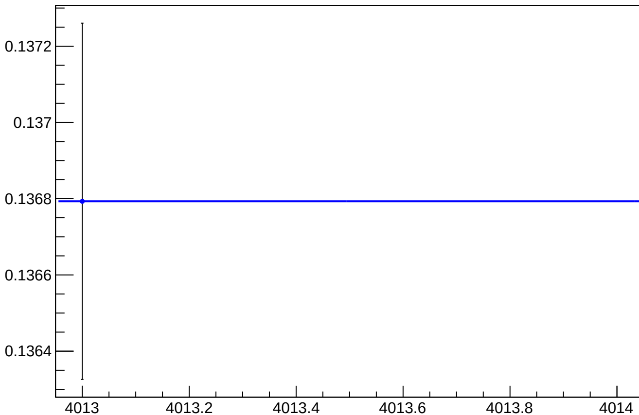
asym_atr2_reg_vs_cor_diff_rms vs Slug, Sign Corrected
