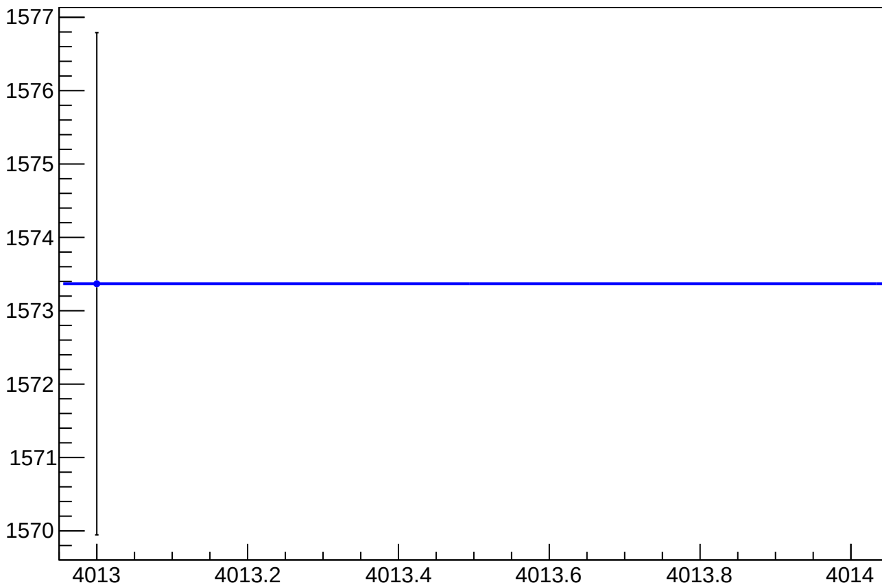
eigen_cor_asym_at2_avg_rms vs Slug, Sign Corrected
