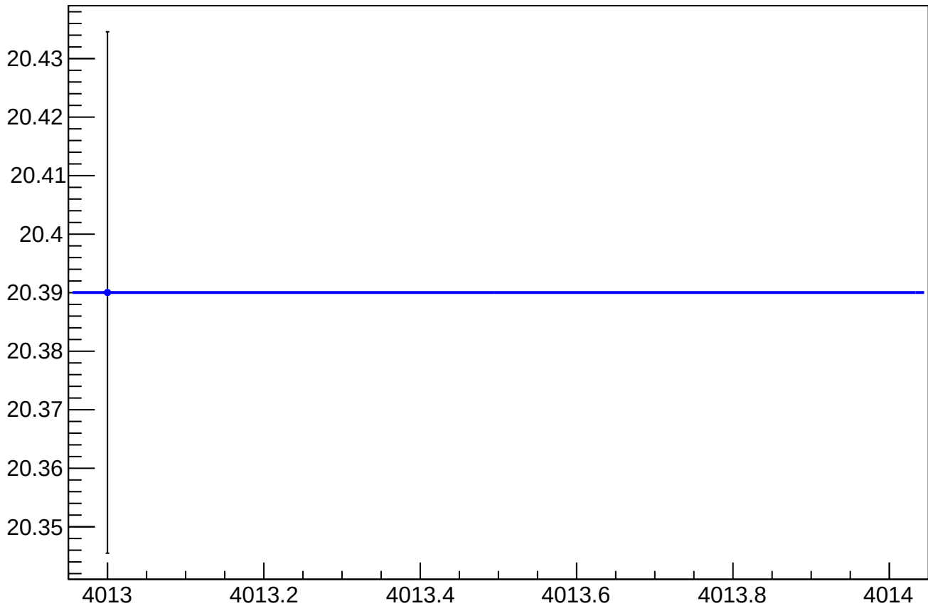
asym_sam_15_dd_dit_vs_eigen_cor_diff_rms vs Slug, Sign Corrected
