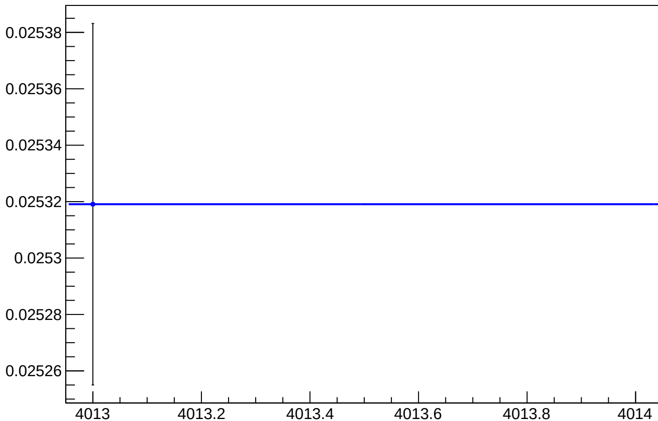
asym_sam_37_26_dd_reg_vs_cor_diff_rms vs Slug, Sign Corrected
