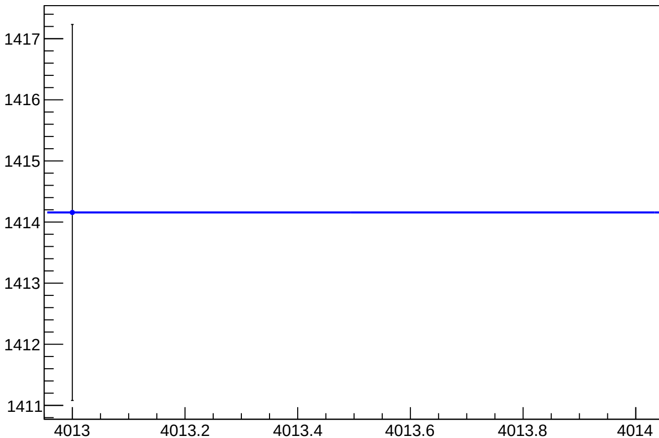
eigen_cor_asym_at1_avg_rms vs Slug, Sign Corrected
