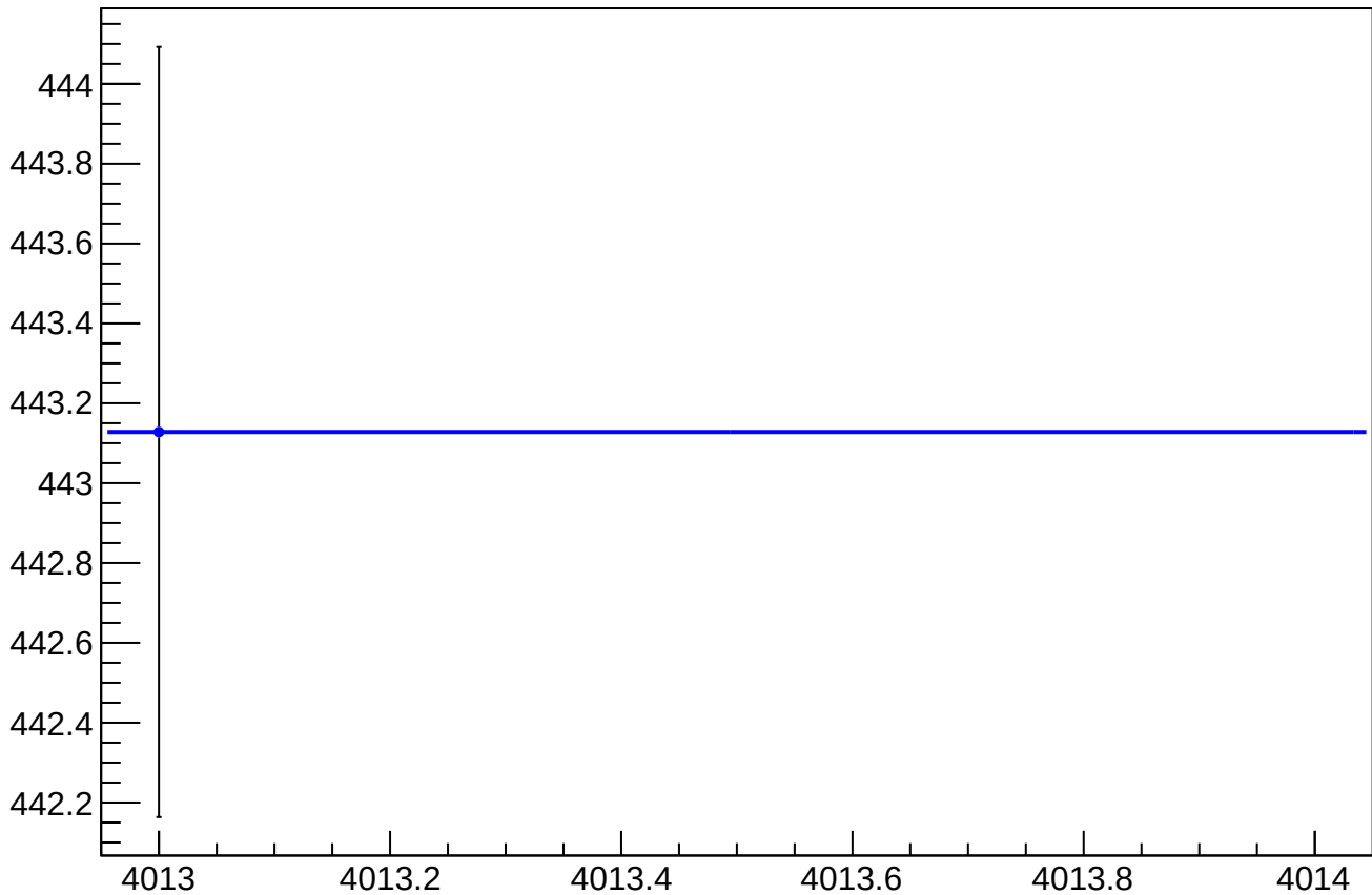
asym_us_dd_at1lr_dd_avg_dit_correction_rms vs Slug, Sign Corrected
