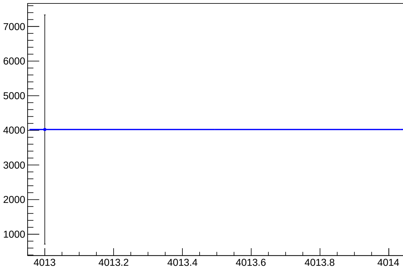
dit_asym_atl1r2_dd_atl2r1_dd_dd_mean vs Slug, Sign Corrected
