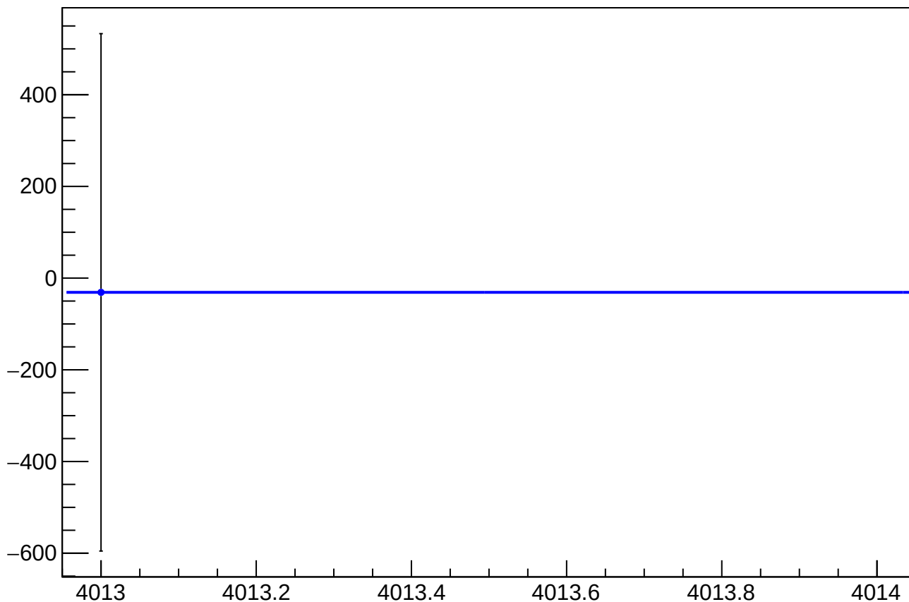
asym_sam1_eigen_dit_correction_mean vs Slug, Sign Corrected
