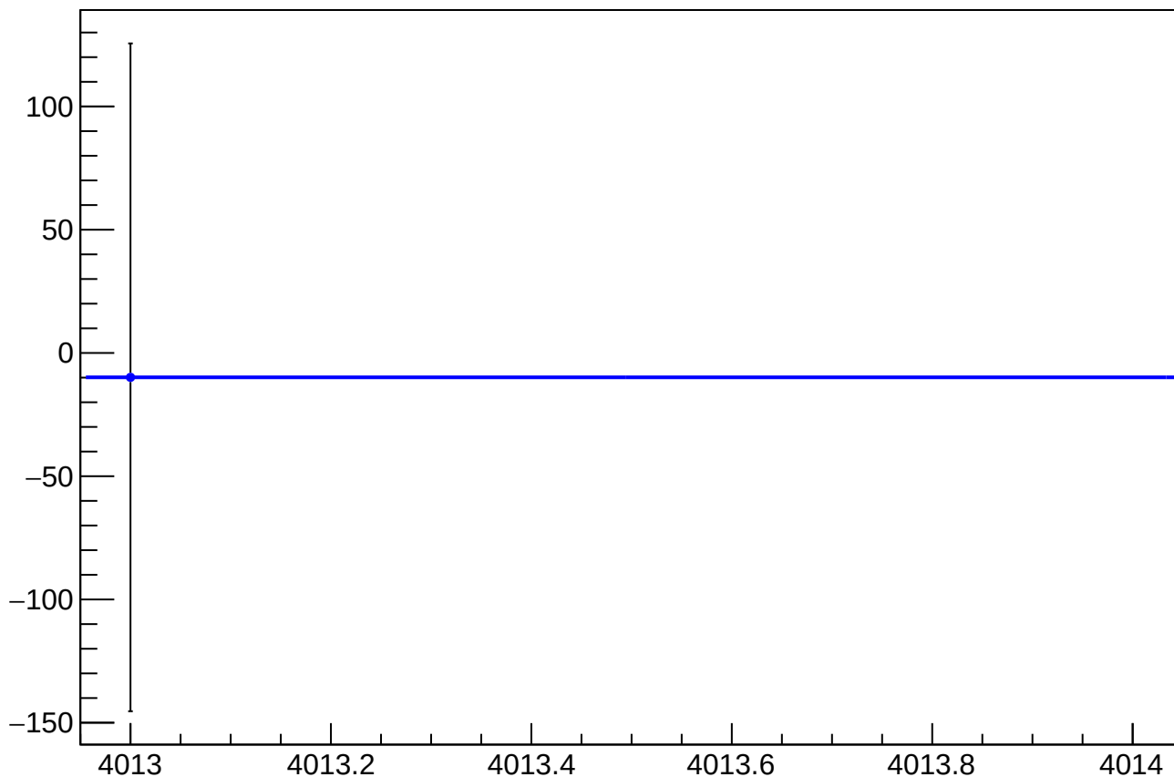
asym_atl_avg_atr_avg_dd_eigen_dit_correction_mean vs Slug, Sign Corrected
