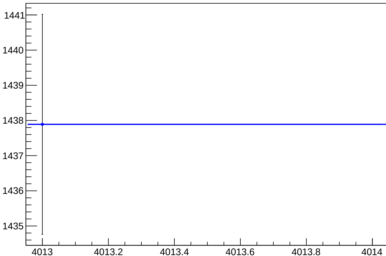
eigen_dit_asym_atl1r2_dd_rms vs Slug, Sign Corrected
