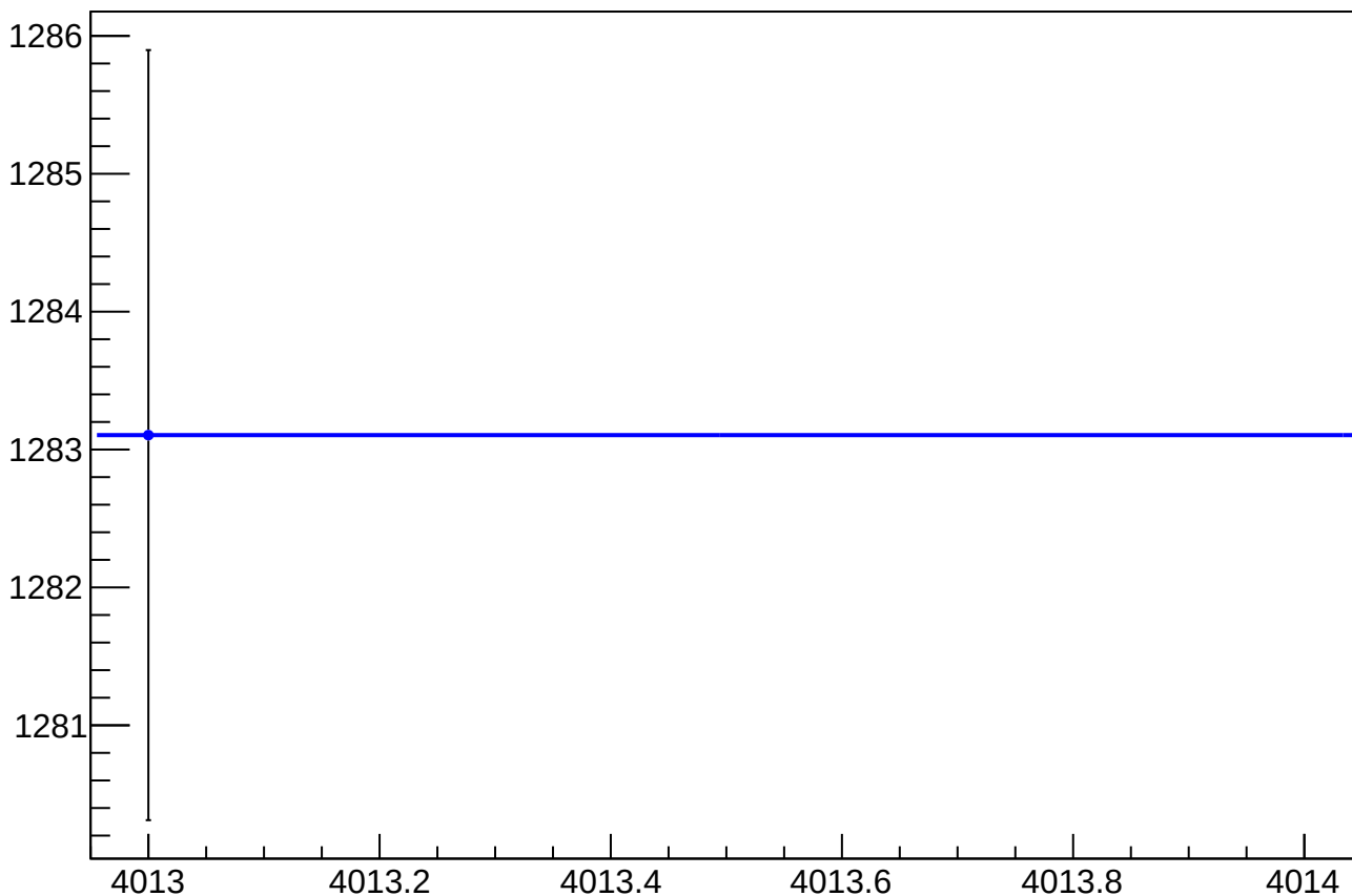
asym_usr_overload_cor_correction_rms vs Slug, Sign Corrected
