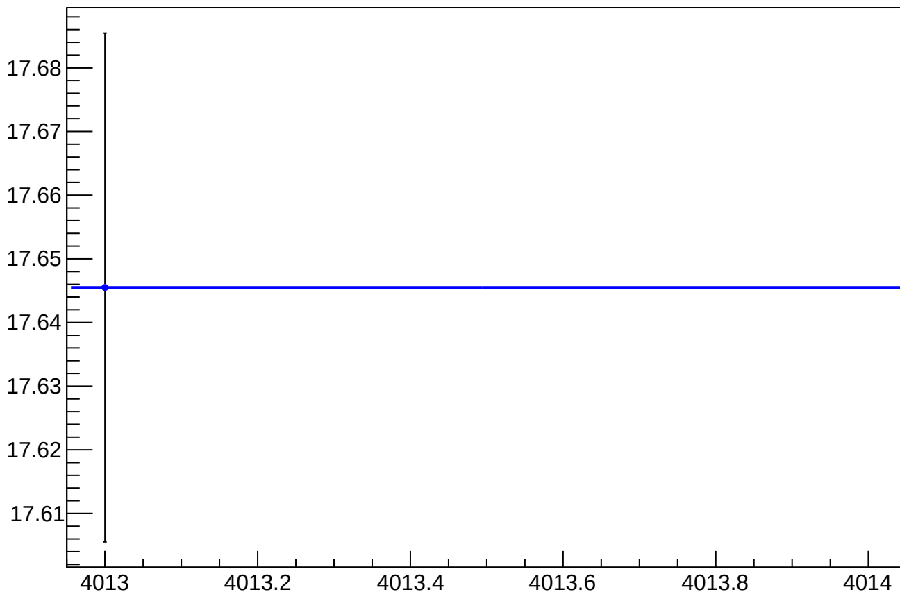
asym_sam_37_dd_eigen_dit_vs_eigen_cor_diff_rms vs Slug, Sign Corrected
