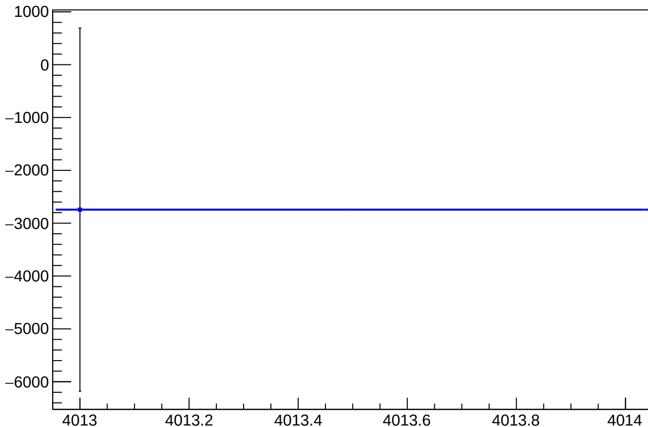
asym_sam3_eigen_cor_correction_mean vs Slug, Sign Corrected
