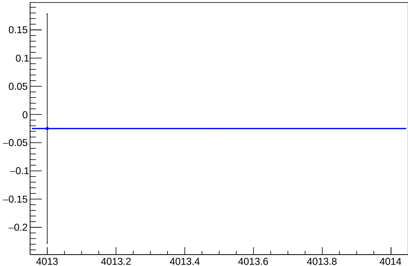
asym_sam_26_avg_eigen_dit_vs_cor_diff_mean vs Slug, Sign Corrected
