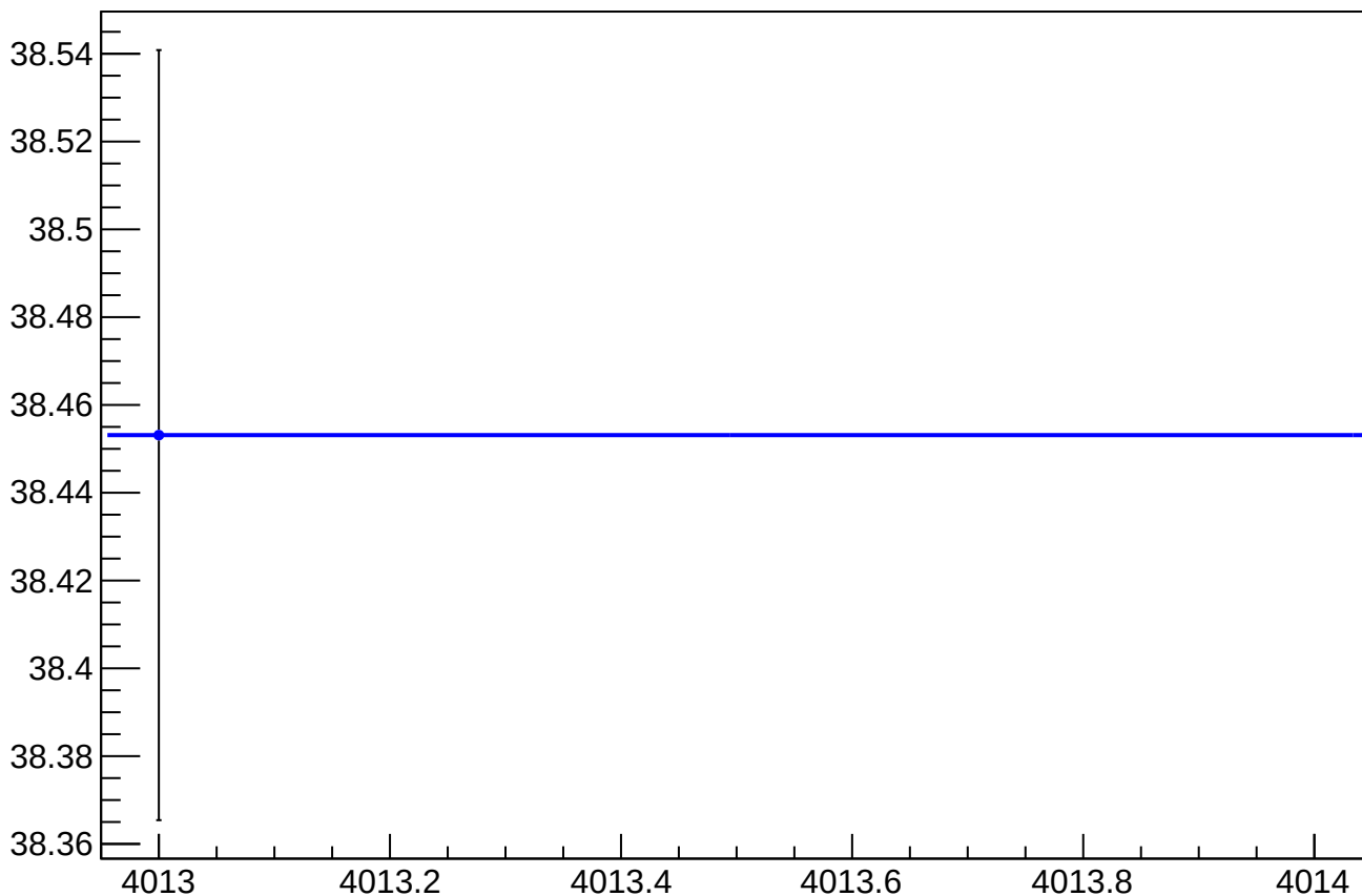
asym_sam_12345678_avg_eigen_dit_vs_eigen_cor_diff_rms vs Slug, Sign Corrected
