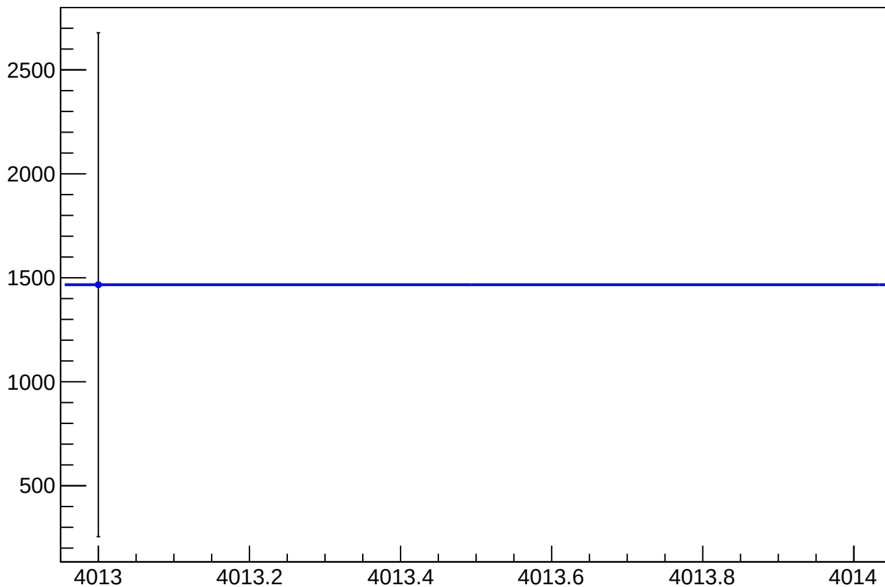
asym_sam_15_37_dd_dit_correction_mean vs Slug, Sign Corrected
