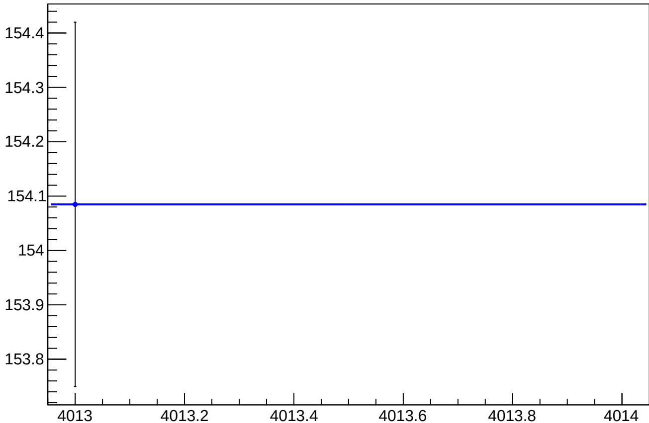
cor_asym_sam_15_26_dd_rms vs Slug, Sign Corrected
