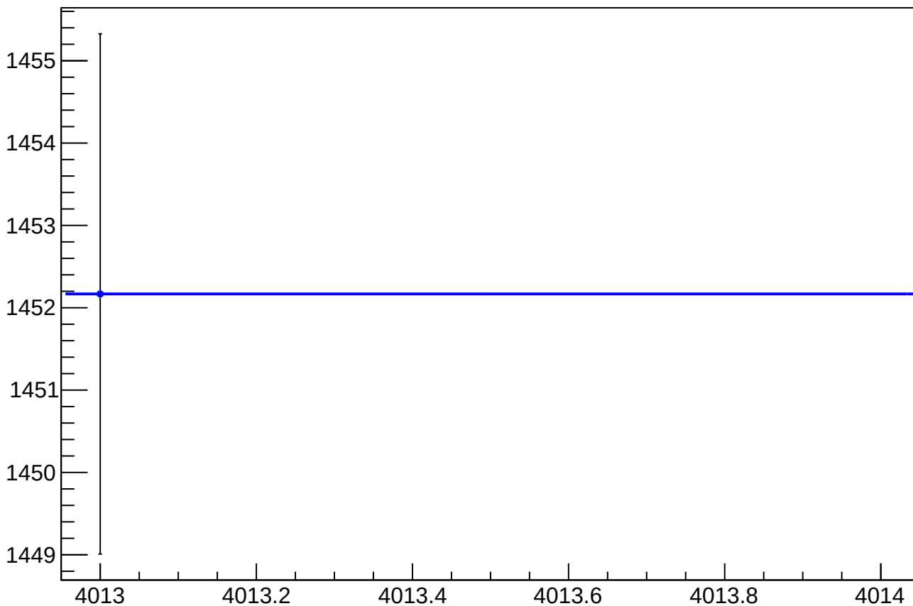
eigen_dit_asym_atl1r2_avg_rms vs Slug, Sign Corrected
