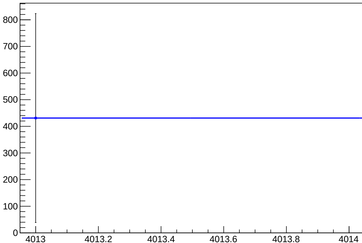
reg_asym_sam_15_dd_mean vs Slug, Sign Corrected
