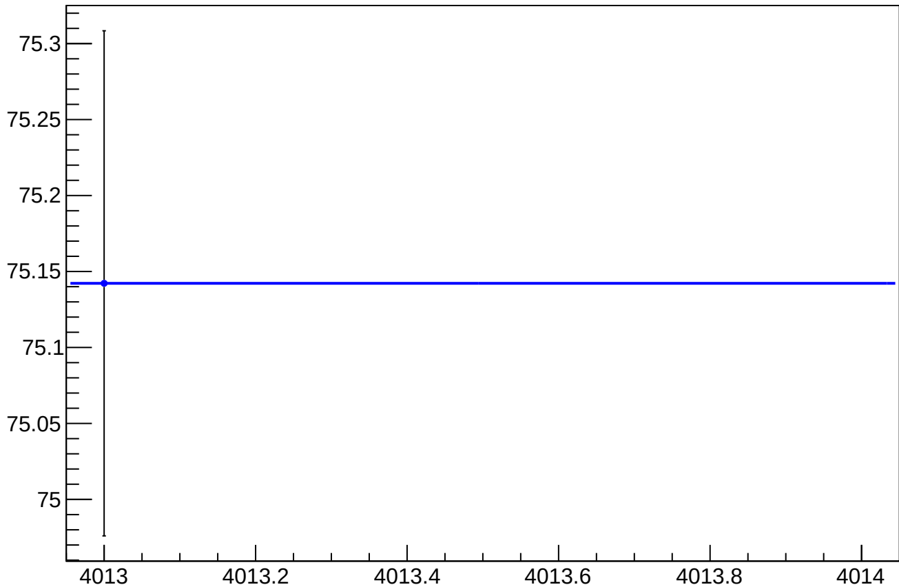
asym_usl_eigen_dit_vs_overload_cor_diff_rms vs Slug, Sign Corrected
