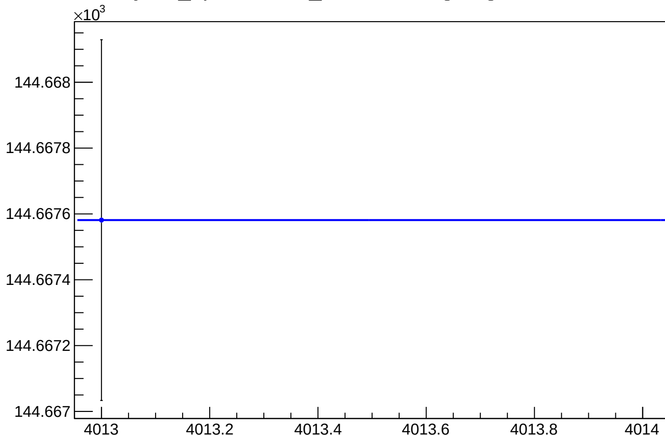
yield_bpm1i06WS_mean vs Slug, Sign Corrected
