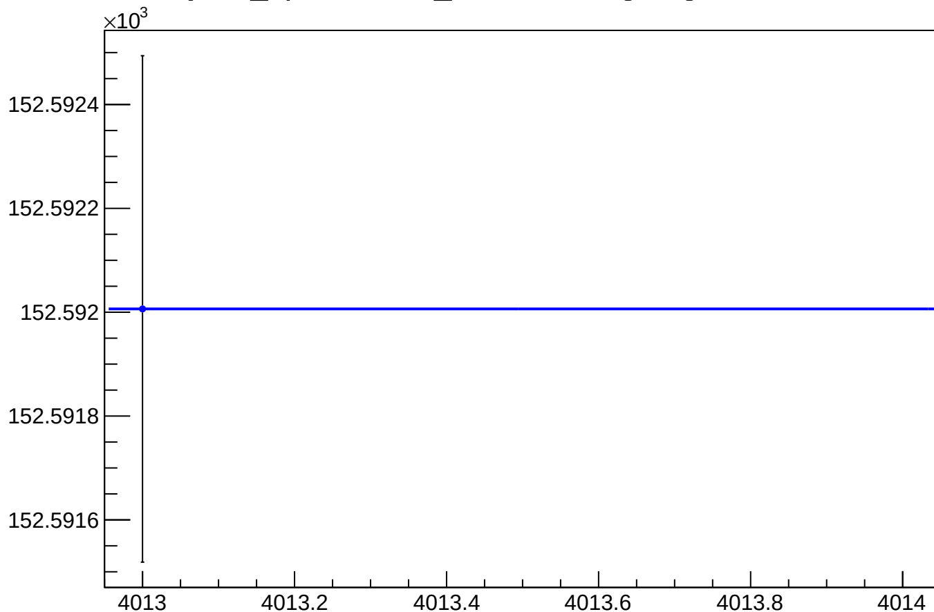
yield_bpm0i07WS_mean vs Slug, Sign Corrected
