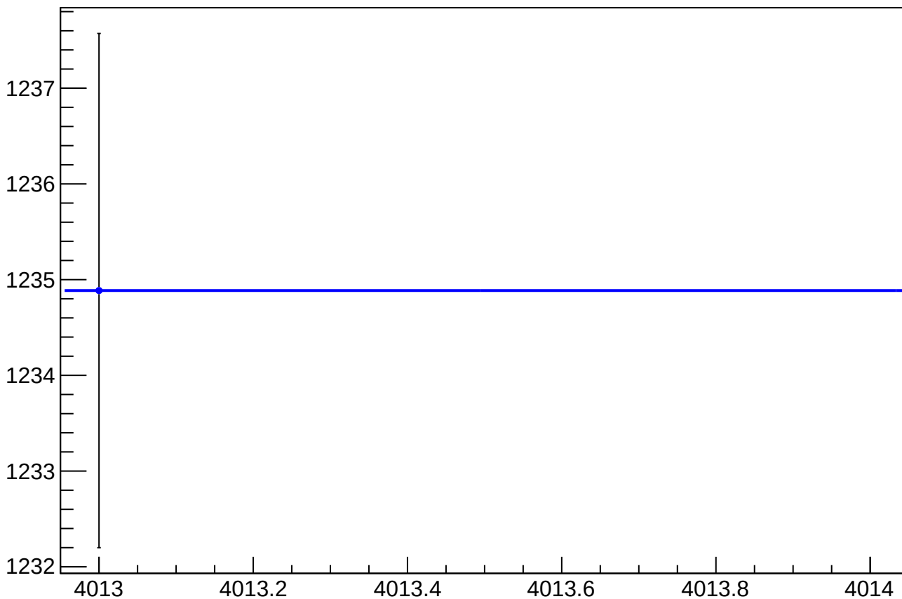
eigen_dit_asym_usr_atr1_avg_rms vs Slug, Sign Corrected
