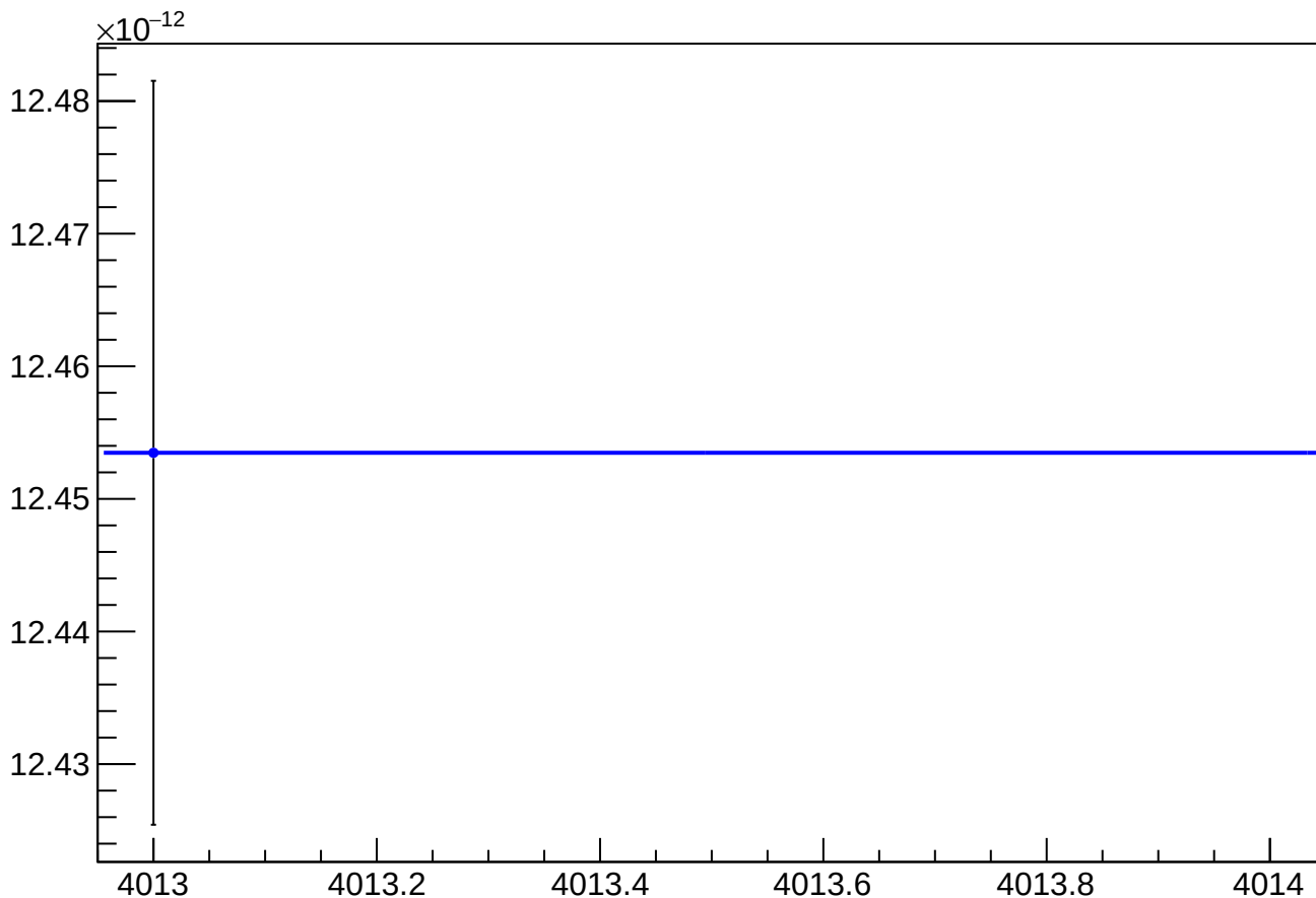
asym_sam_1357_avg_eigen_cor_vs_cor_diff_rms vs Slug, Sign Corrected
