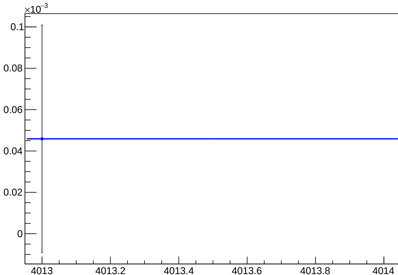
asym_usr_atr2_avg_eigen_dit_vs_dit_diff_mean vs Slug, Sign Corrected
