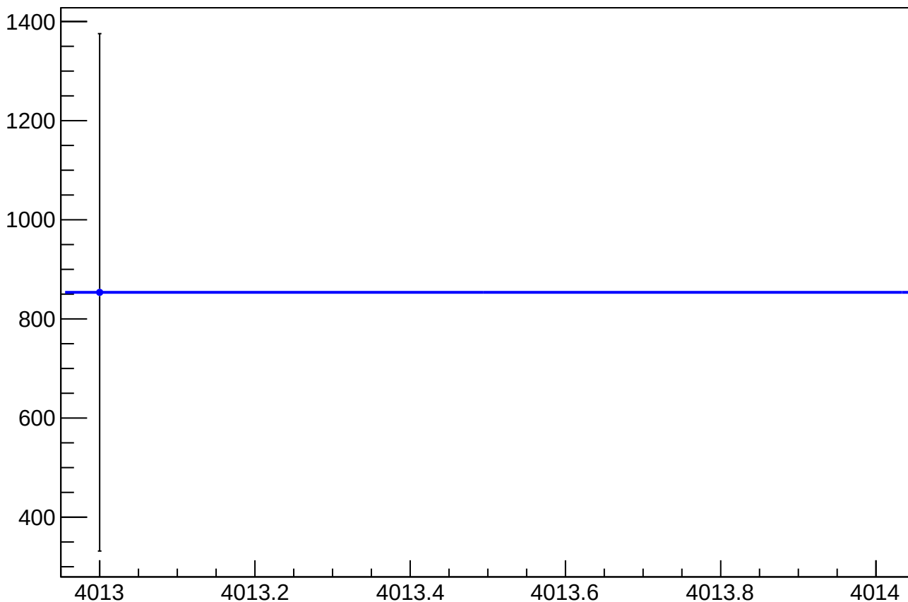
cor_asym_sam_3726_avg_mean vs Slug, Sign Corrected
