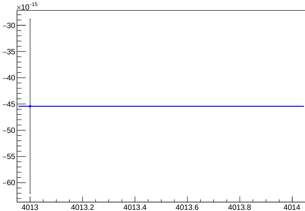
asym_sam_1357_2468_dd_eigen_cor_vs_cor_diff_mean vs Slug, Sign Corrected
