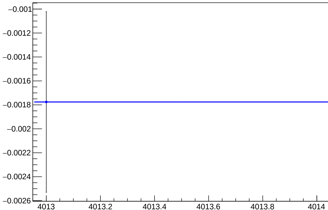
asym_us_avg_at2lr_avg_avg_reg_vs_cor_diff_mean vs Slug, Sign Corrected
