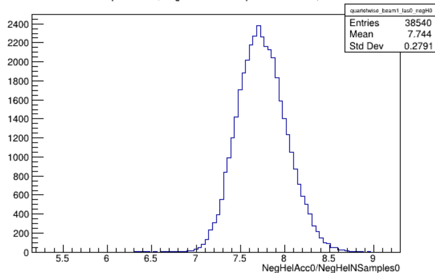
Run 4304 quartetwise, NegHelAcc0/NSamples0: Beam ON, Laser OFF
