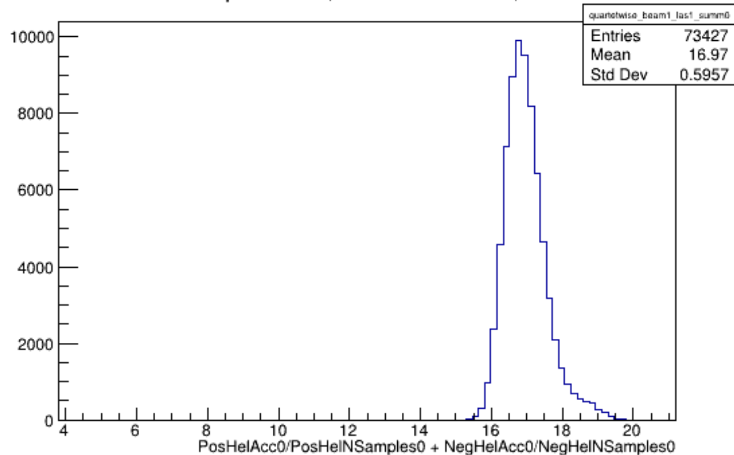
Run 4304 quartetwise, Sums0: Beam ON, Laser ON
