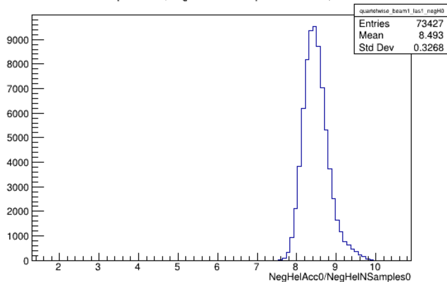
Run 4304 quartetwise, NegHelAcc0/NSamples0: Beam ON, Laser ON
