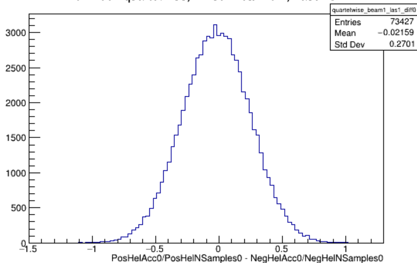
Run 4304 quartetwise, Diffs0: Beam ON, Laser ON
