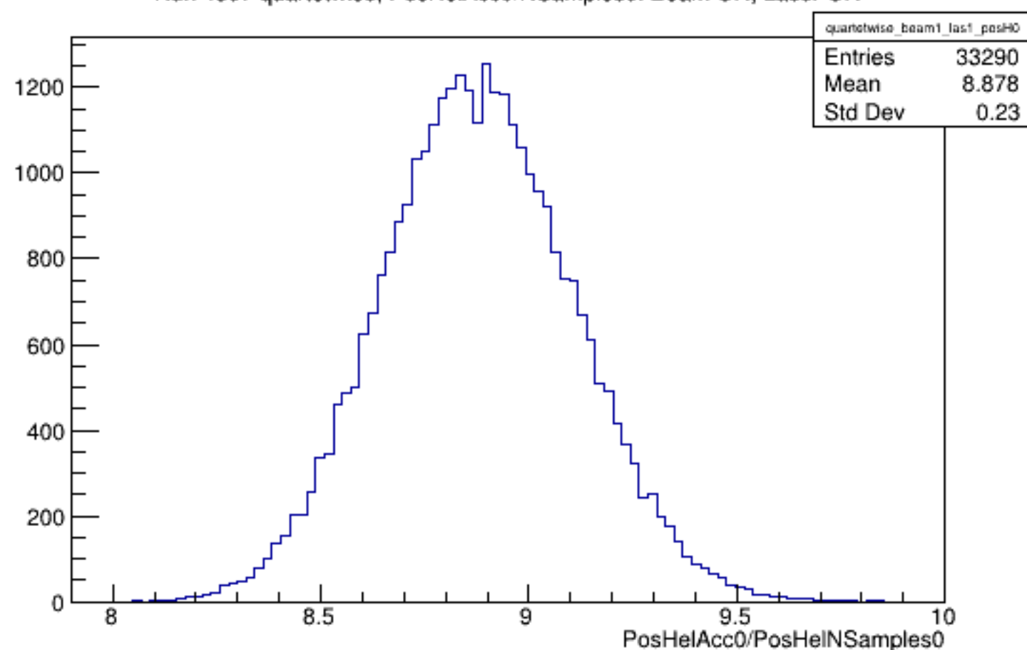
Run 4307 quartetwise, PosHelAcc0/NSamples0: Beam ON, Laser ON
