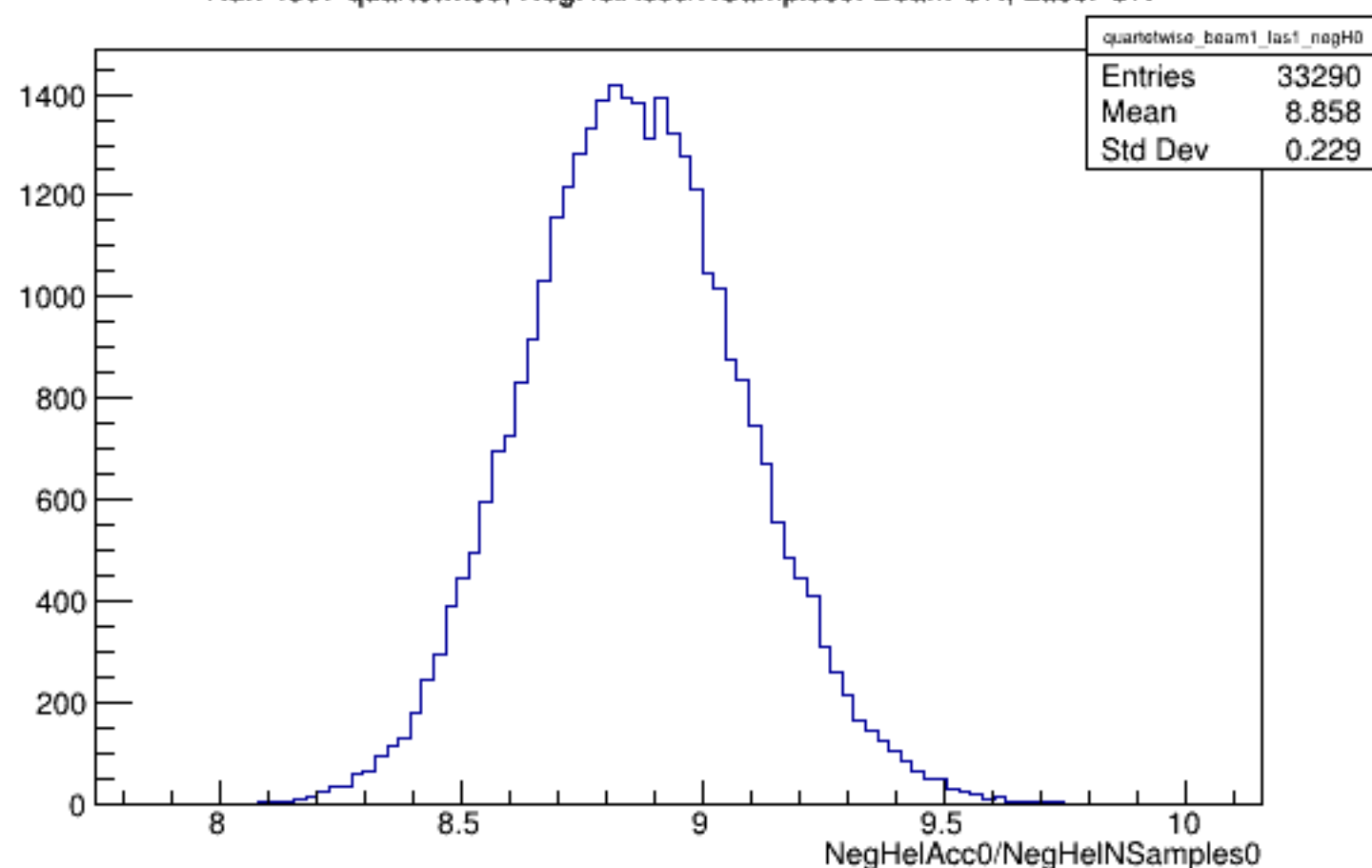
Run 4307 quartetwise, NegHelAcc0/NSamples0: Beam ON, Laser ON
