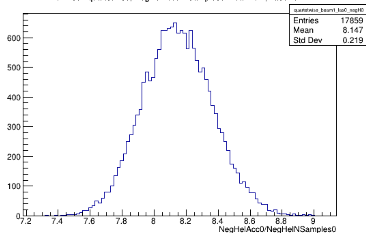
Run 4307 quartetwise, NegHelAcc0/NSamples0: Beam ON, Laser OFF
