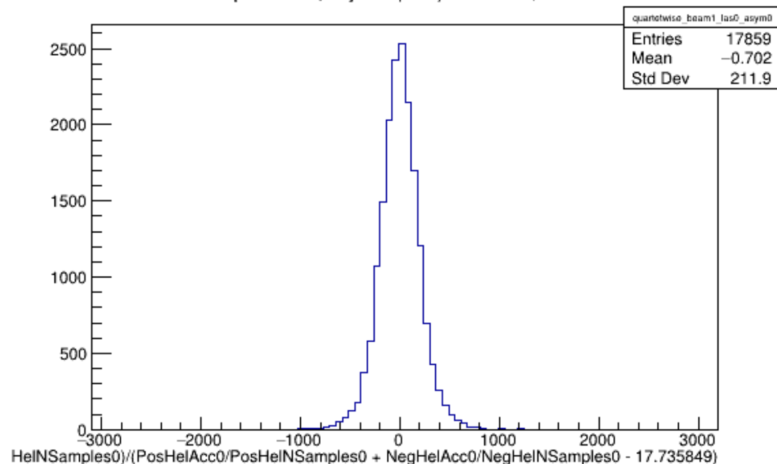
Run 4307 quartetwise, Asyms0 (Raw): Beam ON, Laser OFF
