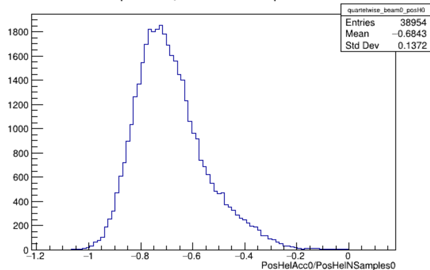
Run 4307 quartetwise, PosHelAcc0/NSamples0: Beam OFF
