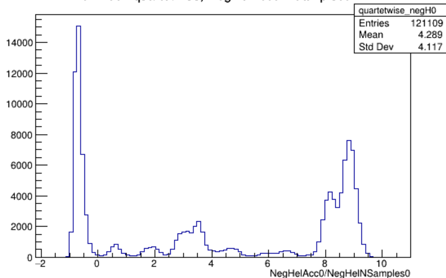
Run 4307 quartetwise, NegHelAcc0/NSamples0: All
