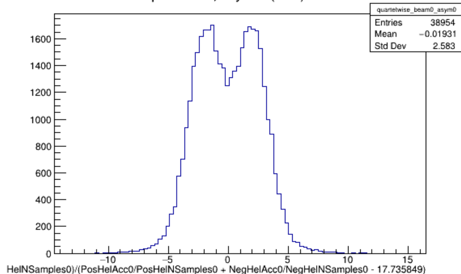
Run 4307 quartetwise, Asyms0 (Raw): Beam OFF
