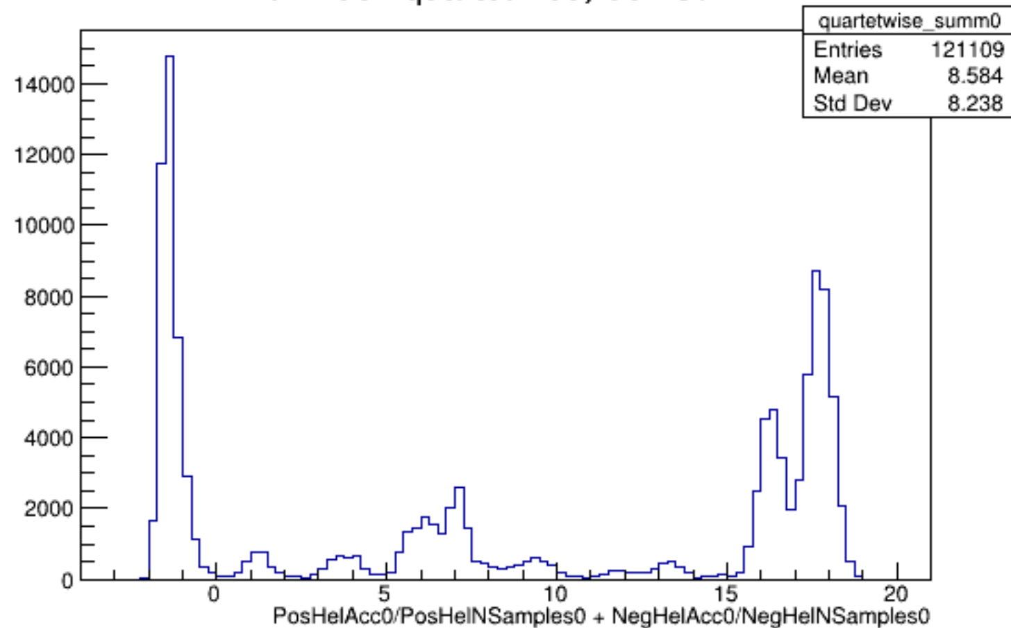
Run 4307 quartetwise, Sums0: All
