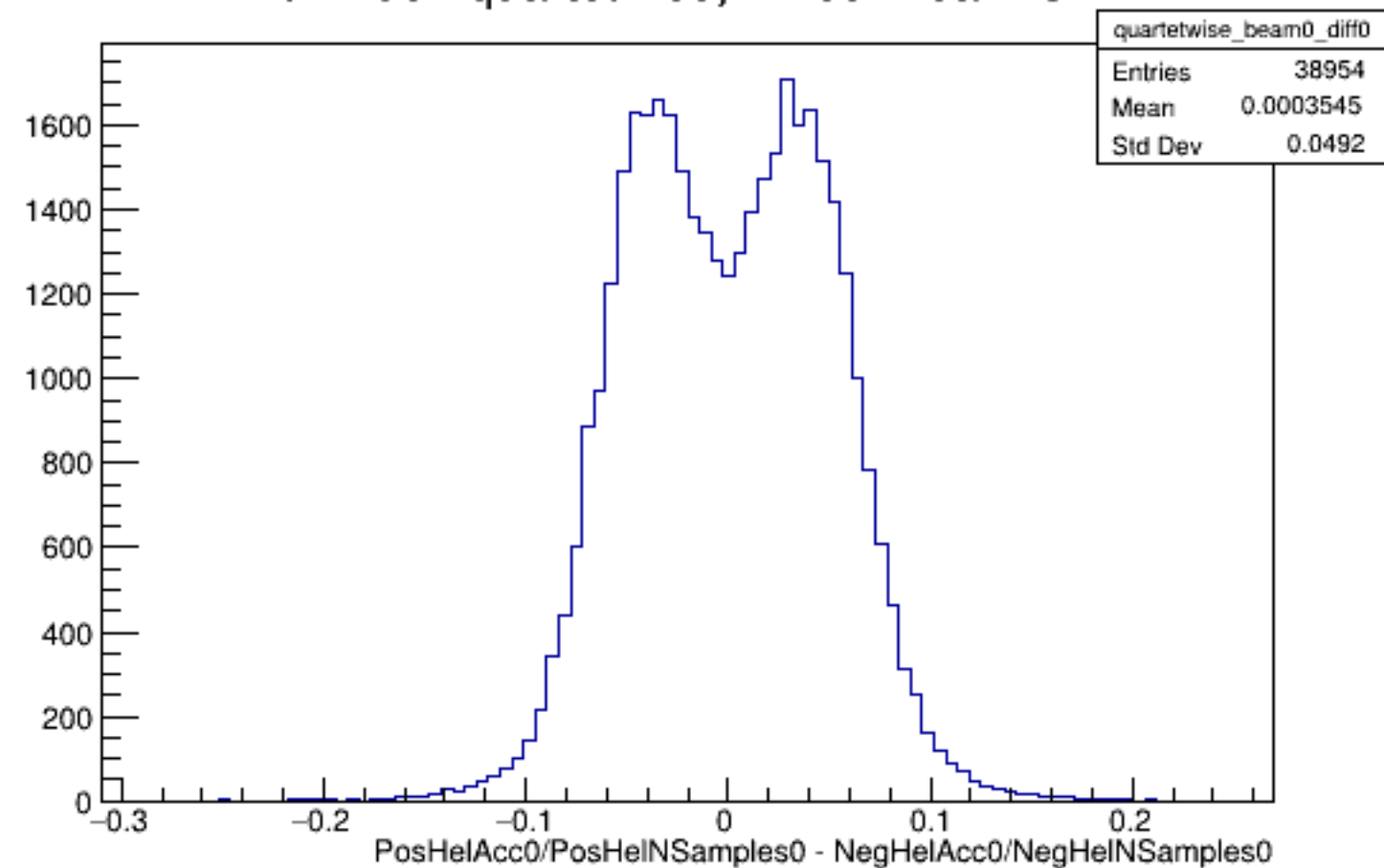
Run 4307 quartetwise, Diffs0: Beam OFF
