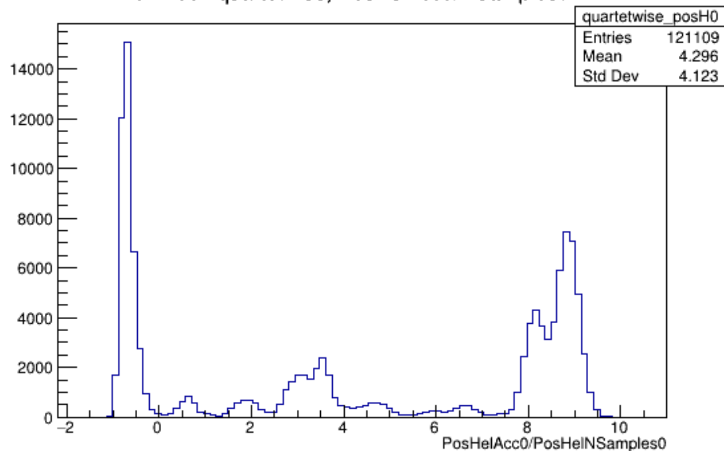
Run 4307 quartetwise, PosHelAcc0/NSamples0: All
