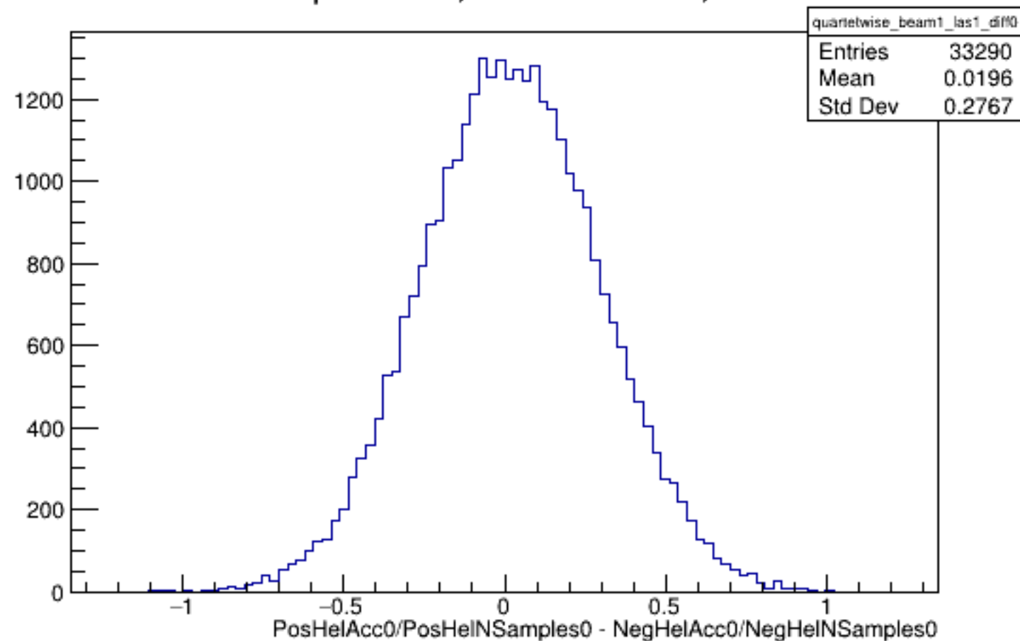
Run 4307 quartetwise, Diffs0: Beam ON, Laser ON
