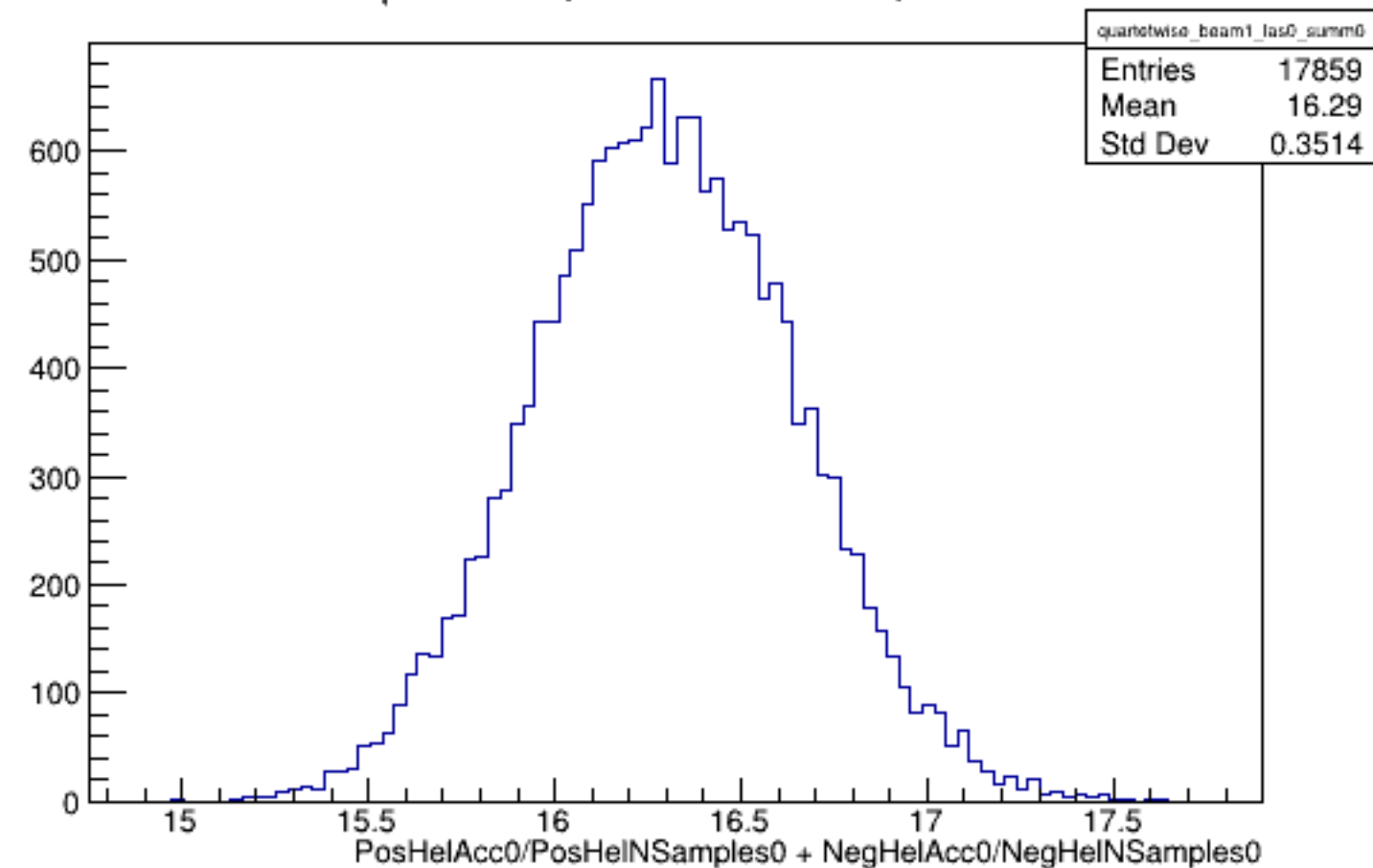
Run 4307 quartetwise, Sums0: Beam ON, Laser OFF
