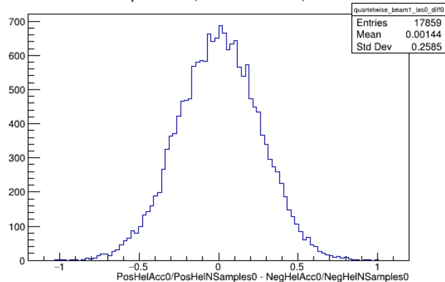
Run 4307 quartetwise, Diffs0: Beam ON, Laser OFF
