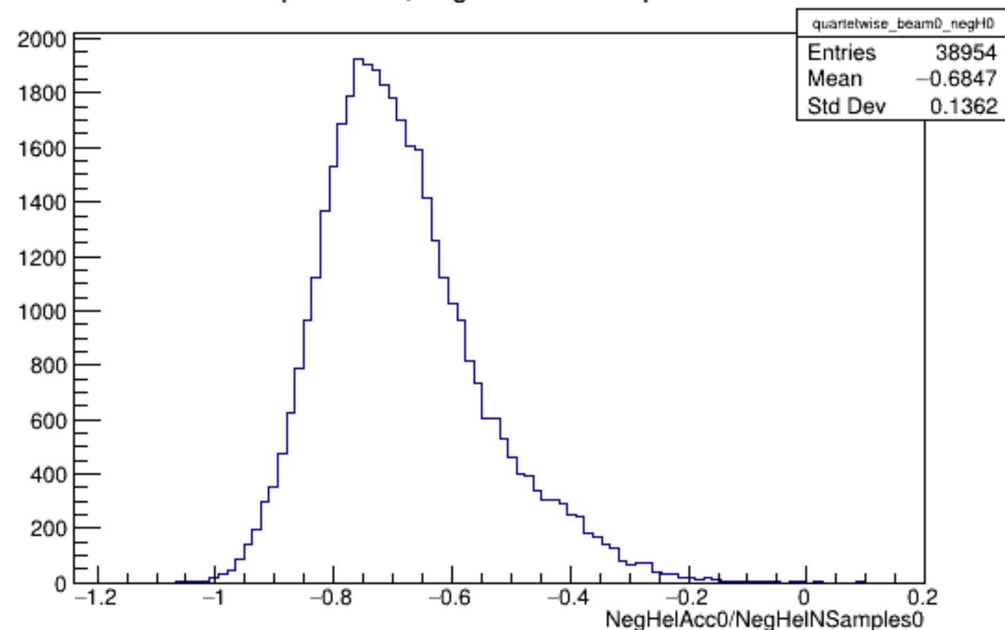
Run 4307 quartetwise, NegHelAcc0/NSamples0: Beam OFF
