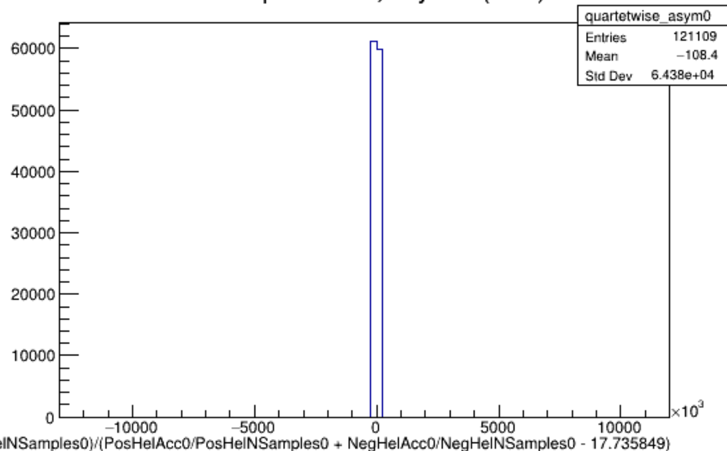
Run 4307 quartetwise, Asyms0 (Raw): All
