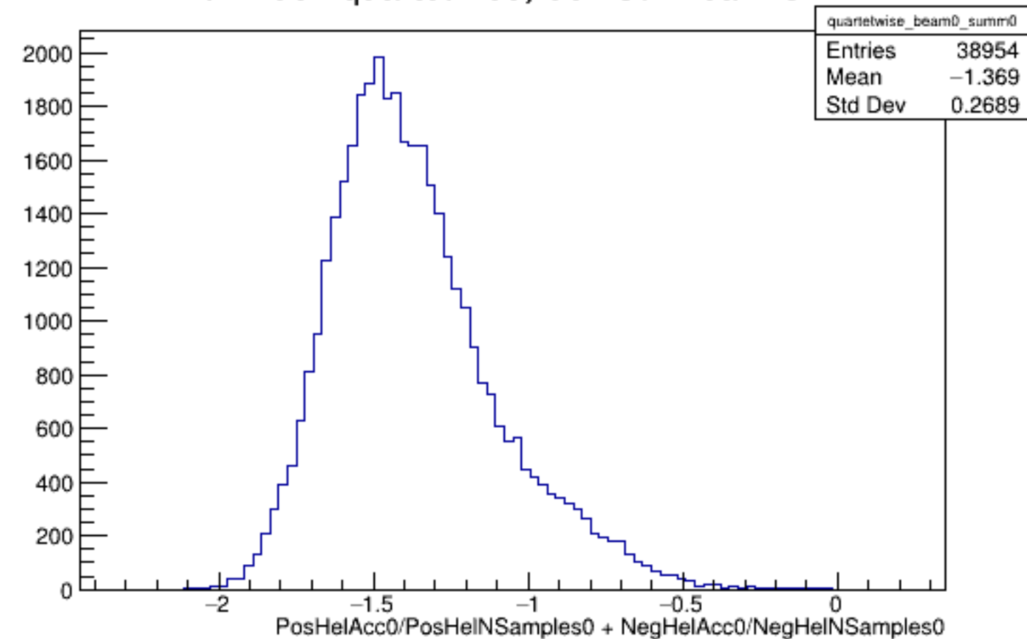
Run 4307 quartetwise, Sums0: Beam OFF
