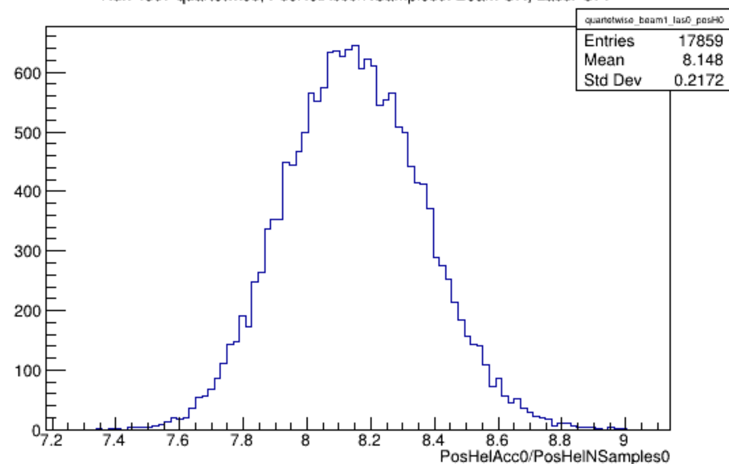
Run 4307 quartetwise, PosHelAcc0/NSamples0: Beam ON, Laser OFF
