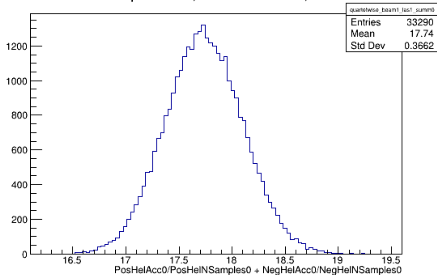
Run 4307 quartetwise, Sums0: Beam ON, Laser ON
