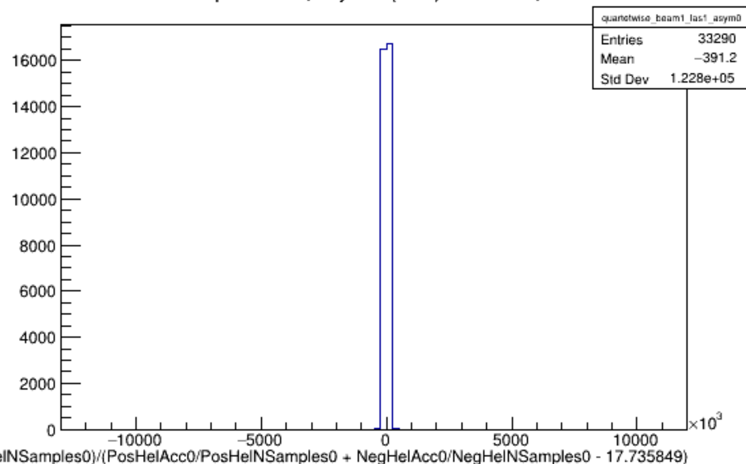
Run 4307 quartetwise, Asyms0 (Raw): Beam ON, Laser ON
