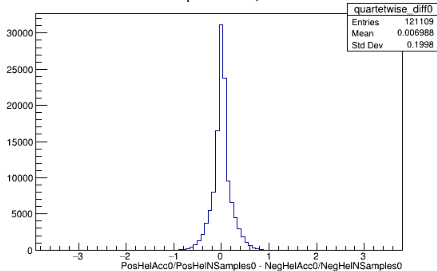
Run 4307 quartetwise, Diffs0: All
