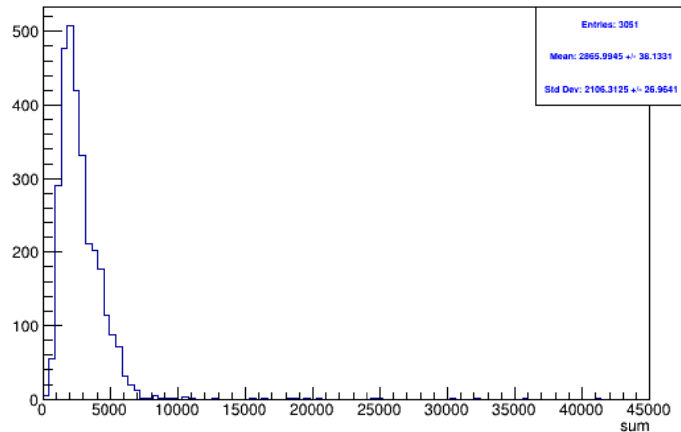
Run 4307 triggerwise, sums: Beam OFF
