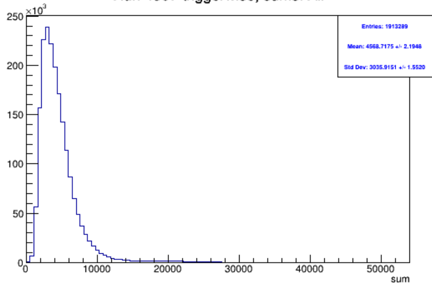
Run 4307 triggerwise, sums: All
