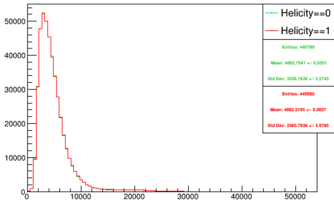
Run 4307 triggerwise, sums: Beam ON, Laser ON
