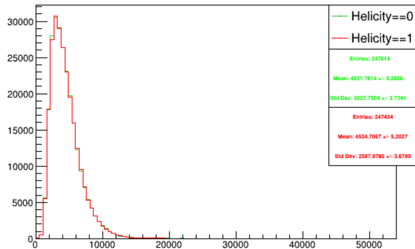
Run 4307 triggerwise, sums: Beam ON, Laser OFF
