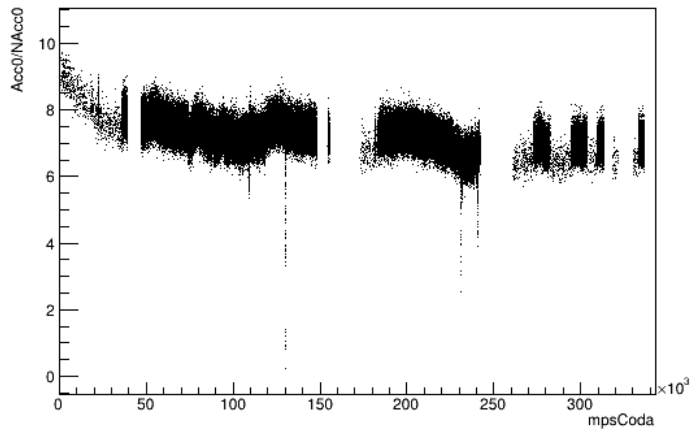
Run 4311 mpwise, Acc0/NAcc0:mpsCoda, beam ON, laser ON
