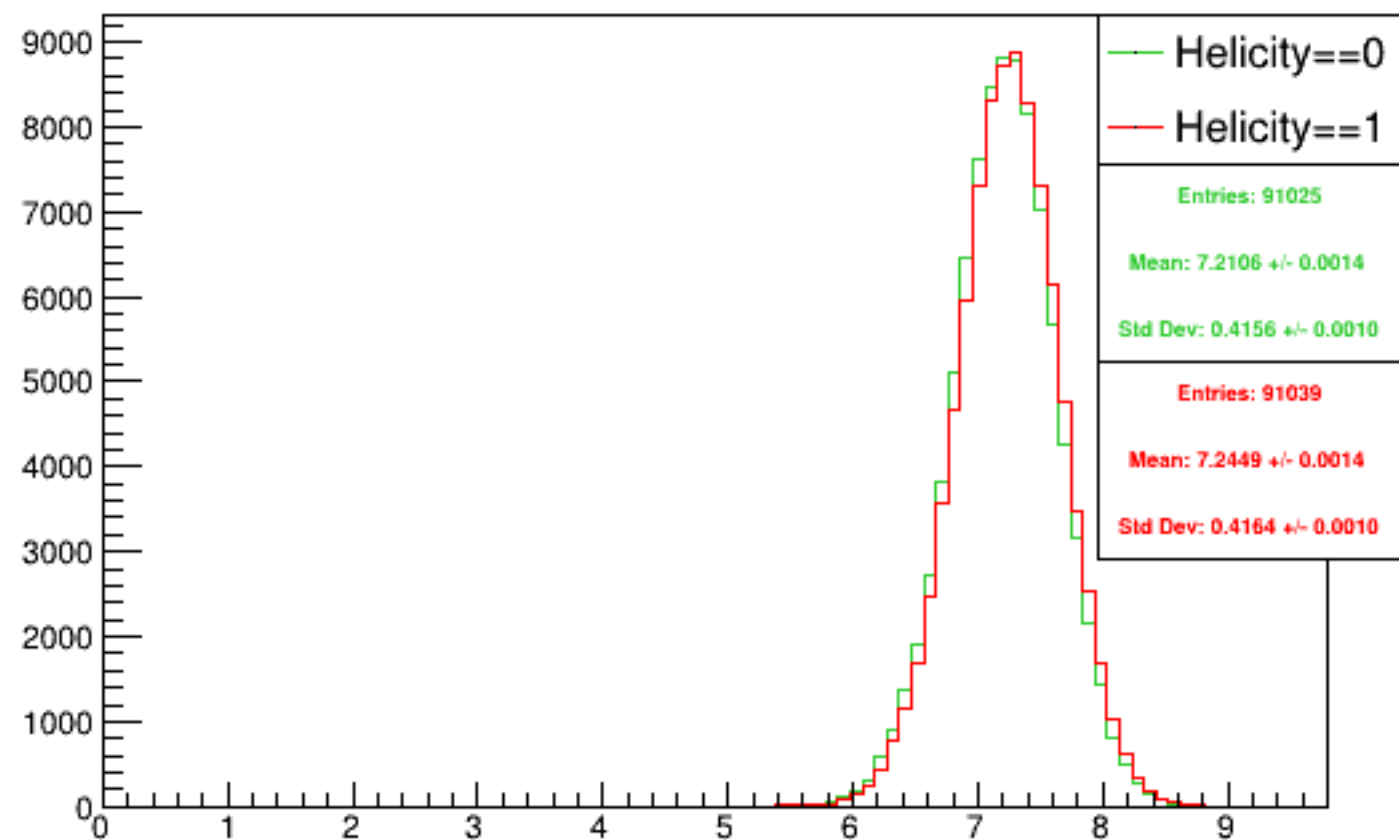
Run 4311 mpwise, acc0: Beam ON, Laser ON
