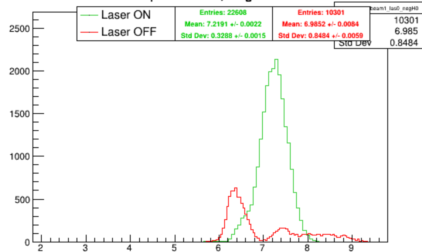
Run 4311 quartetwise, negH0: Beam ON
