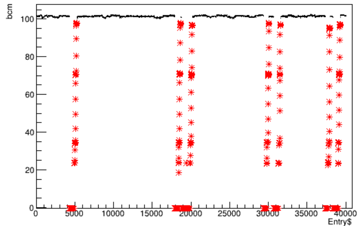
Run 4311 quartetwise, bcm vs time
