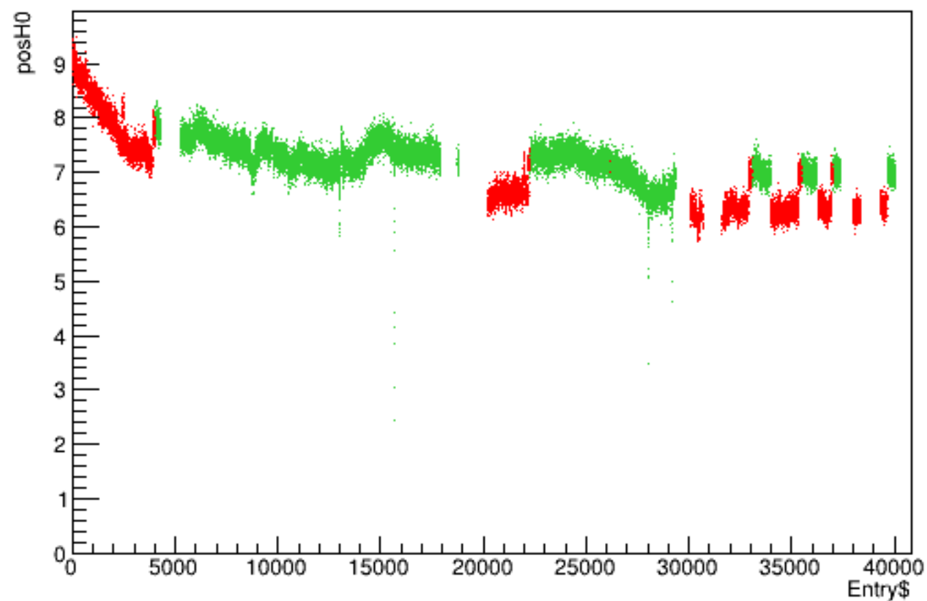
Run 4311 quartetwise, posH0 vs time
