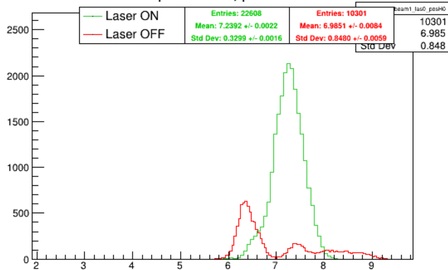
Run 4311 quartetwise, posH0: Beam ON
