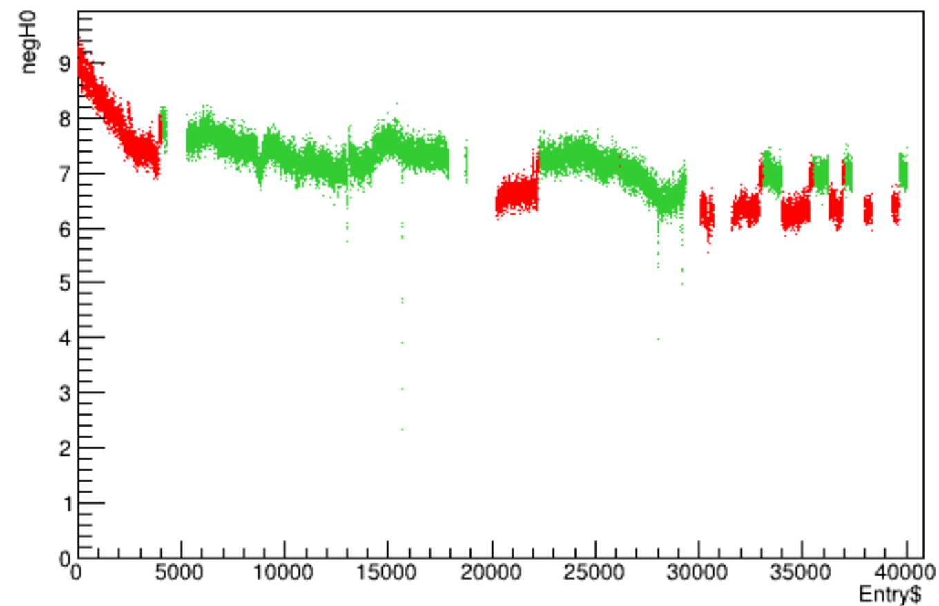
Run 4311 quartetwise, negH0 vs time
