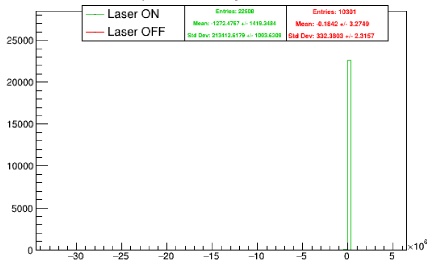
Run 4311 quartetwise, asym0sub: Beam ON
