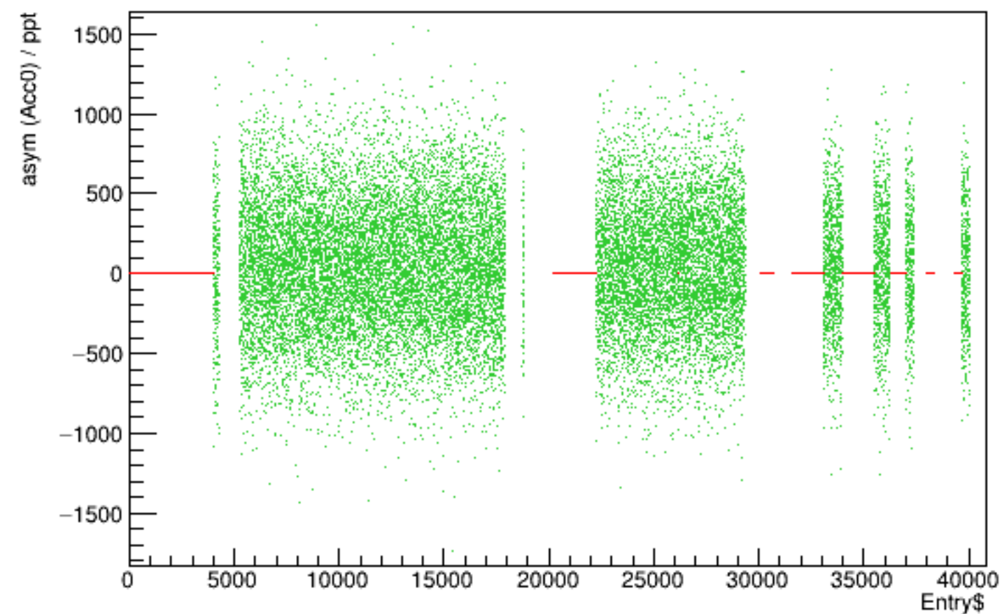
Run 4311 quartetwise, asym (Acc0) / ppt vs time
