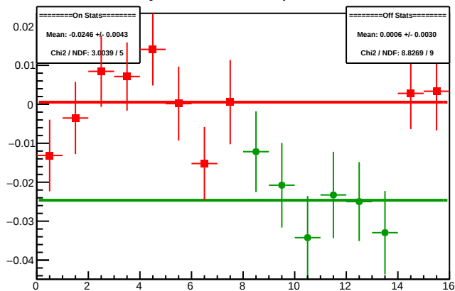
Cycle 4315.3: Multiplet Diffs
