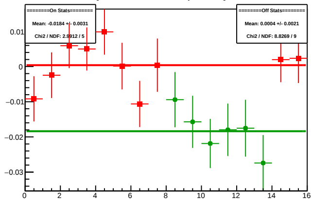
Cycle 4315.3: Multiplet Asyms
