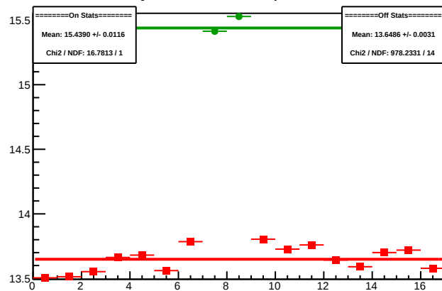
Cycle 4315.2: Multiplet Sums
