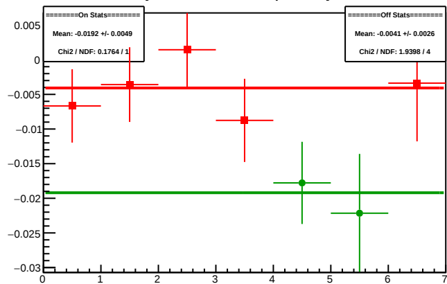
Cycle 4315.5: Multiplet Asyms
