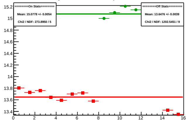
Cycle 4315.3: Multiplet Sums
