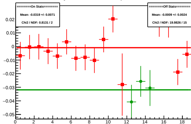
Cycle 4315.1: Multiplet Diffs
