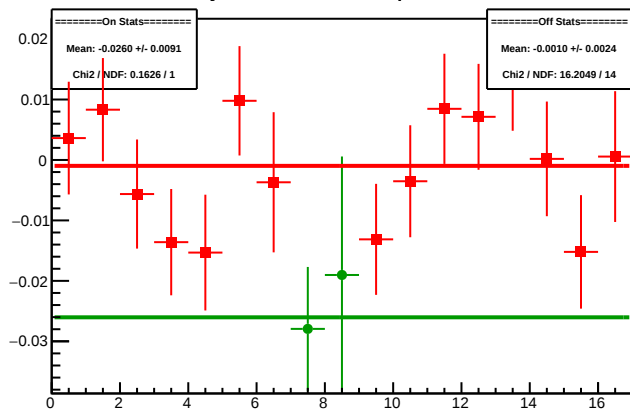
Cycle 4315.2: Multiplet Diffs
