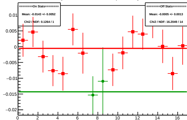
Cycle 4315.2: Multiplet Asyms
