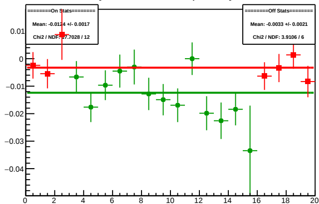
Cycle 4315.4: Multiplet Asyms
