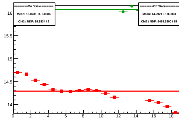
Cycle 4315.1: Multiplet Sums
