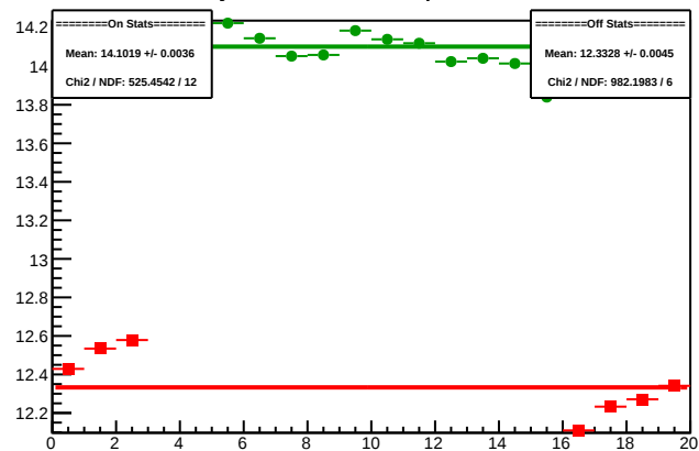
Cycle 4315.4: Multiplet Sums
