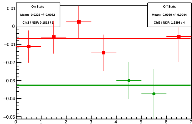
Cycle 4315.5: Multiplet Diffs
