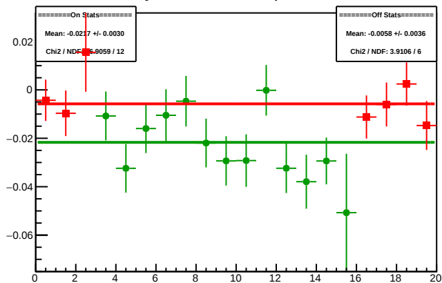
Cycle 4315.4: Multiplet Diffs
