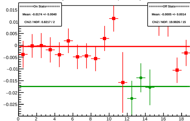
Cycle 4315.1: Multiplet Asyms
