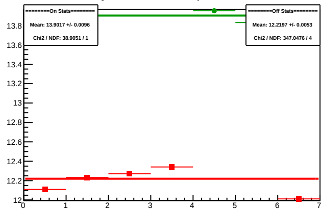
Cycle 4315.5: Multiplet Sums
