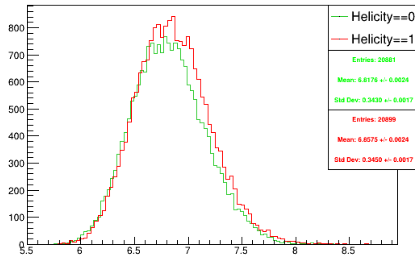
Run 4320 mpwise, acc0: Beam ON, Laser OFF
