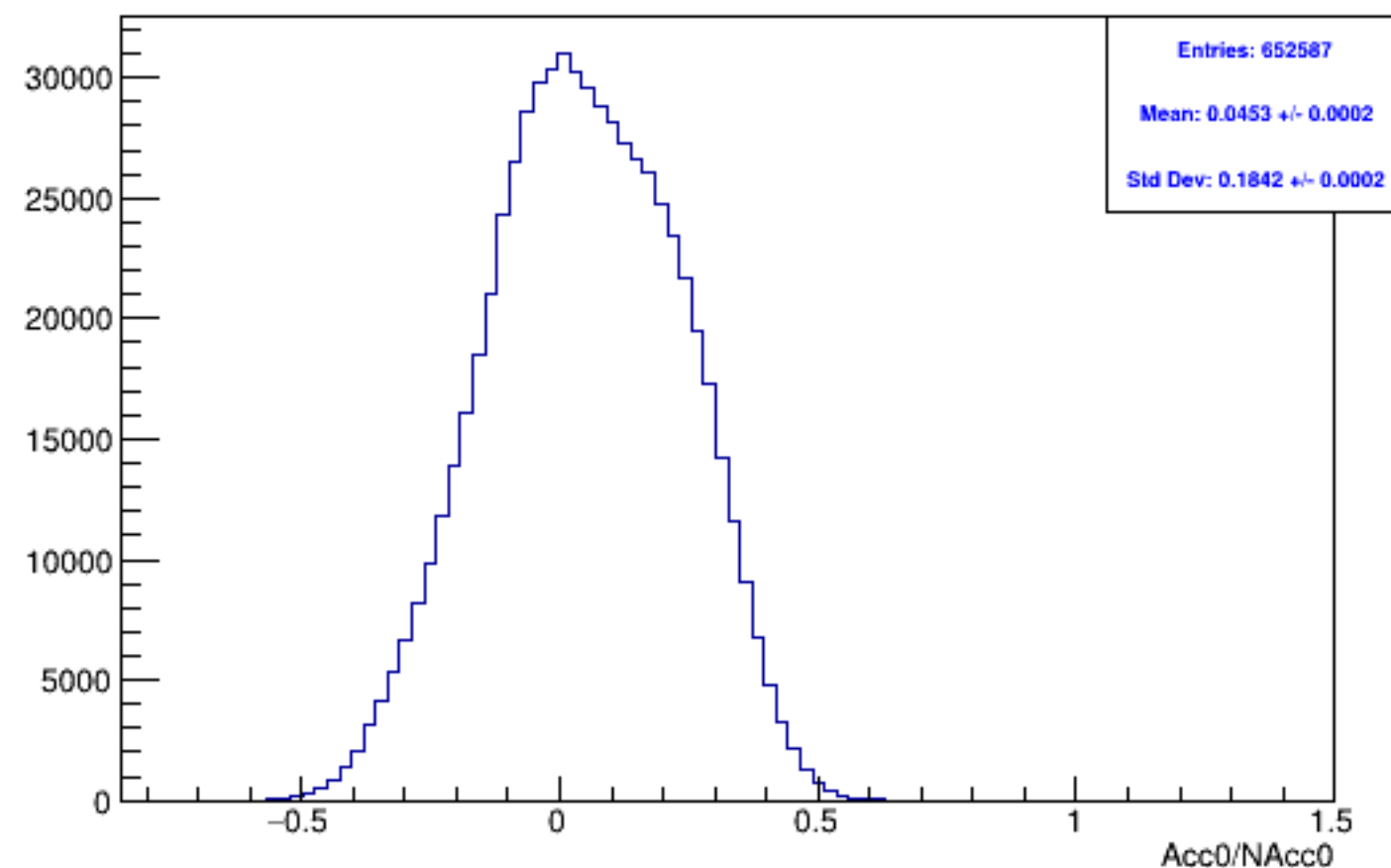
Run 4320 mpwise, acc0: Beam OFF
