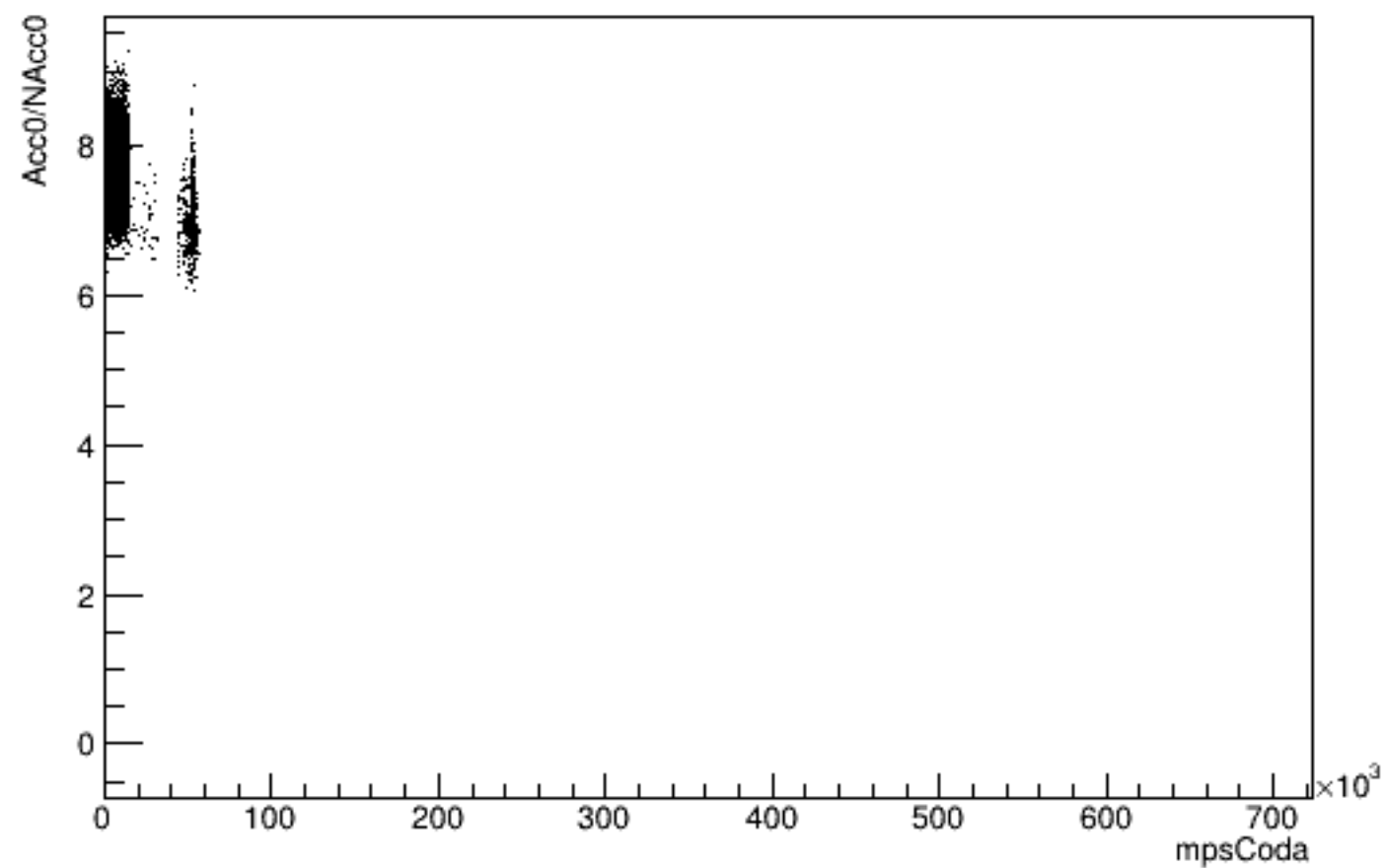
Run 4320 mpwise, Acc0/NAcc0:mpsCoda, beam ON, laser ON
