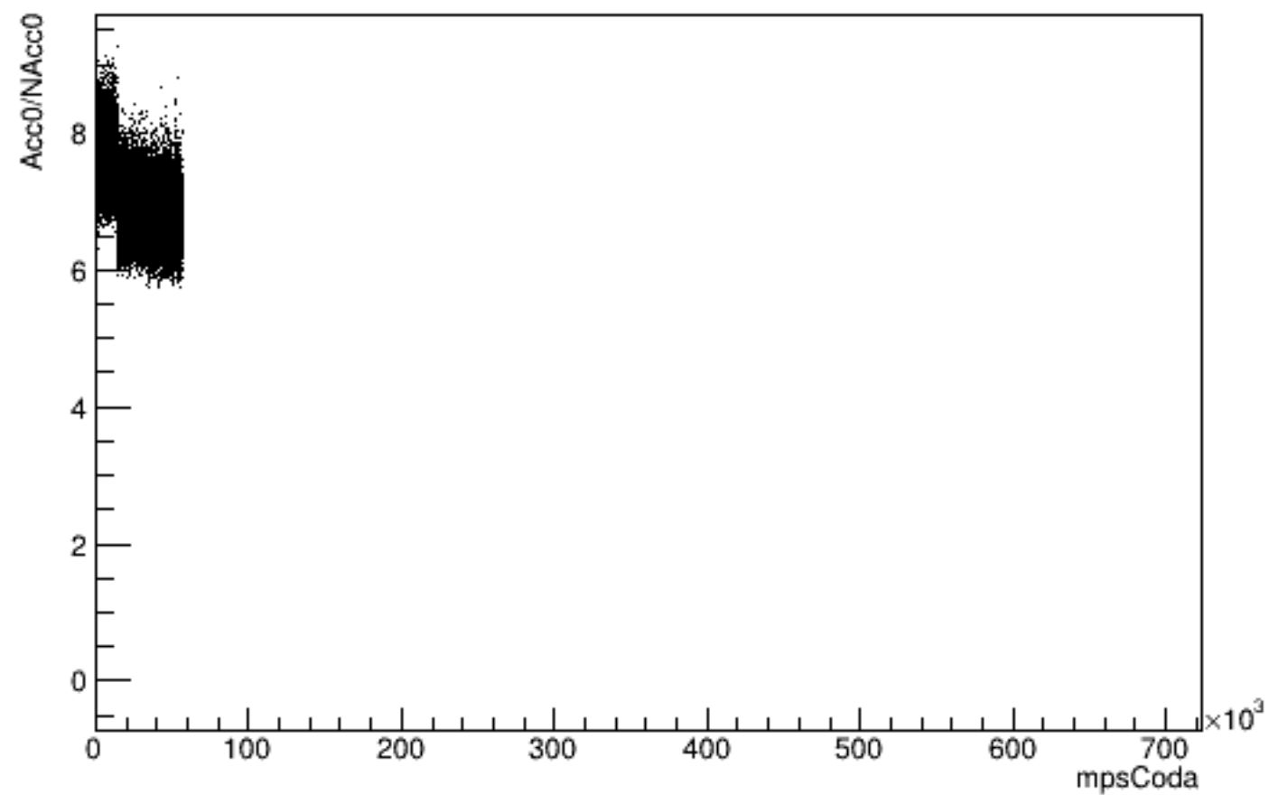
Run 4320 mpwise, Acc0/NAcc0:mpsCoda, beam ON, laser OFF
