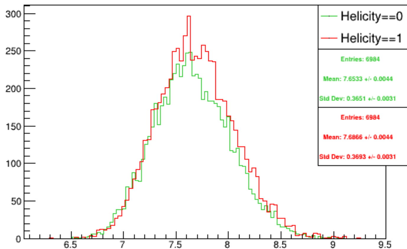
Run 4320 mpwise, acc0: Beam ON, Laser ON
