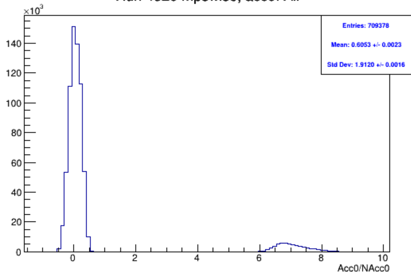
Run 4320 mpwise, acc0: All
