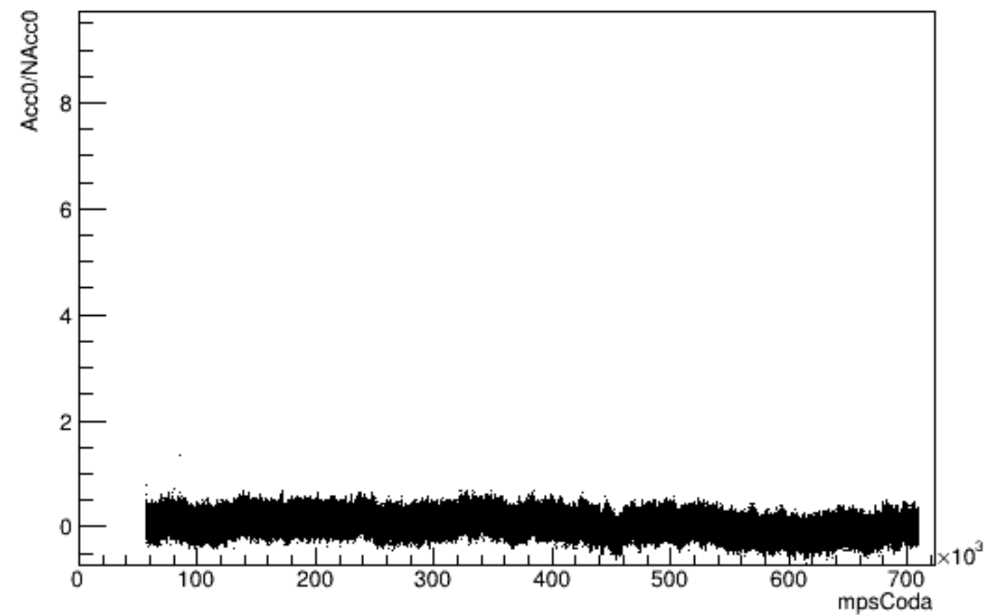
Run 4320 mpwise, Acc0/NAcc0:mpsCoda, beam OFF
