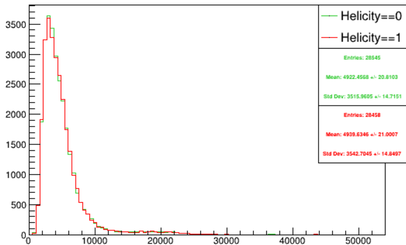
Run 4320 triggerwise, sums: Beam ON, Laser ON
