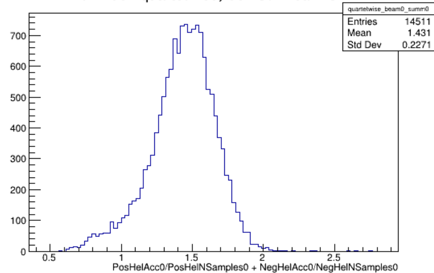
Run 4331 quartetwise, Sums0: Beam OFF
