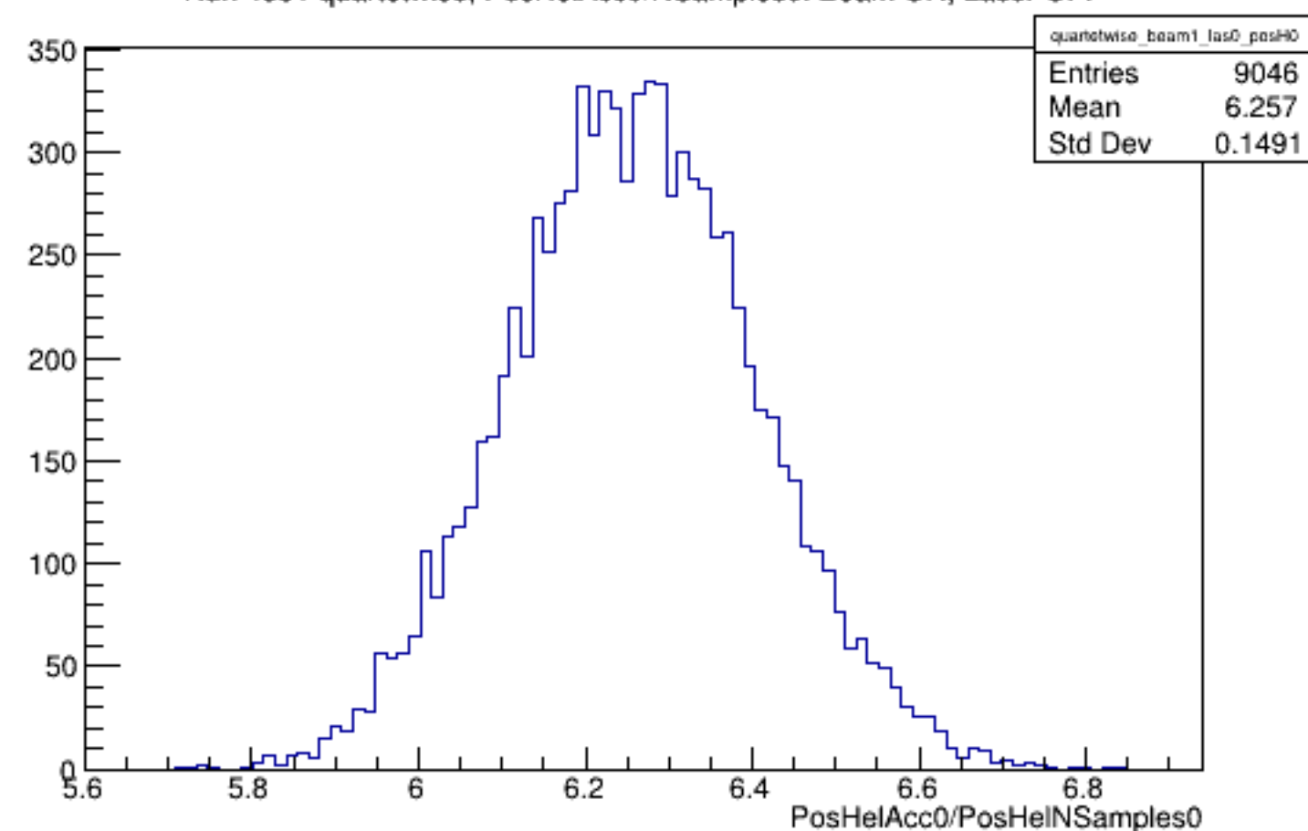
Run 4331 quartetwise, PosHelAcc0/NSamples0: Beam ON, Laser OFF
