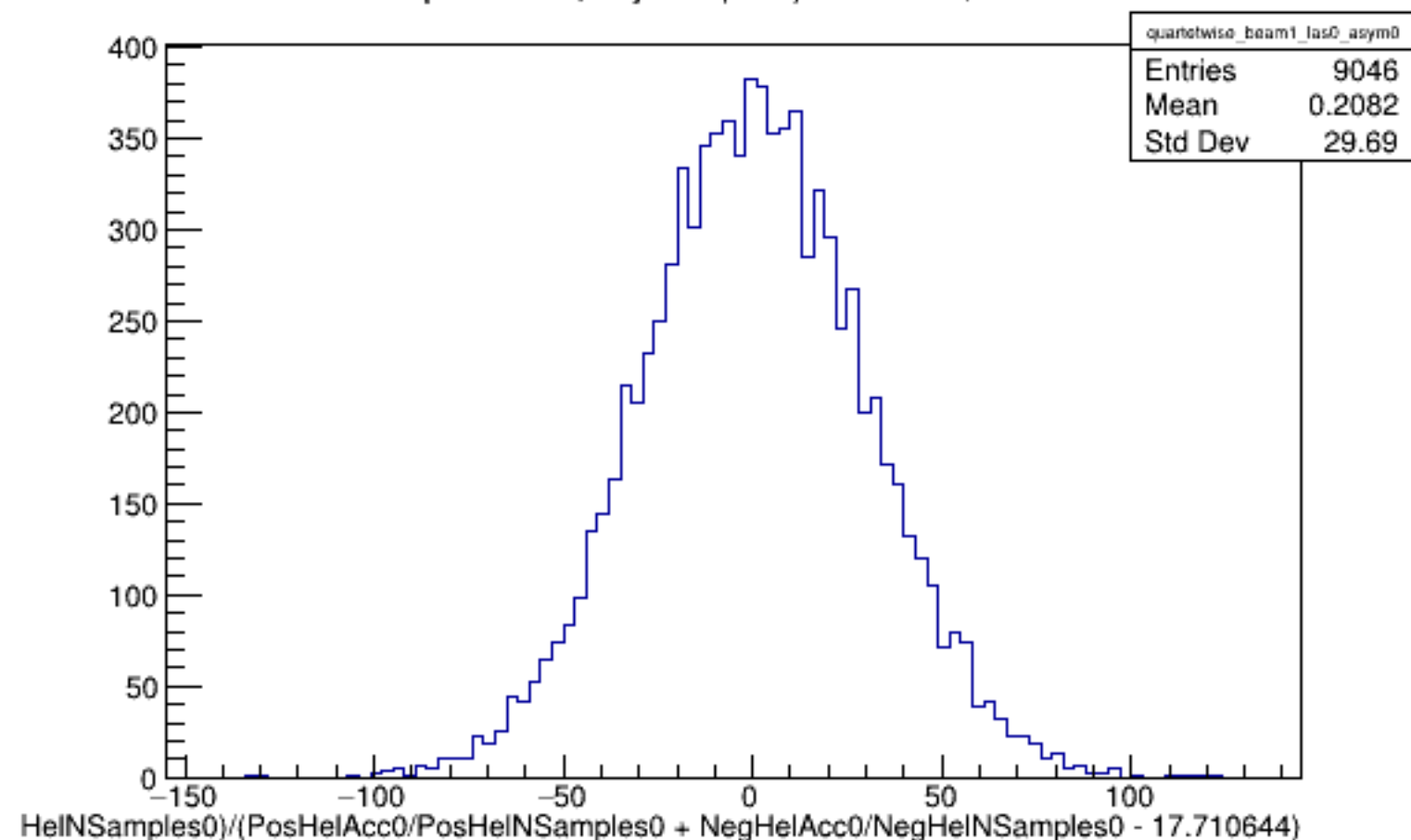
Run 4331 quartetwise, Asyms0 (Raw): Beam ON, Laser OFF
