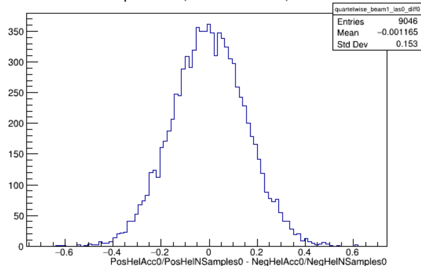
Run 4331 quartetwise, Diffs0: Beam ON, Laser OFF
