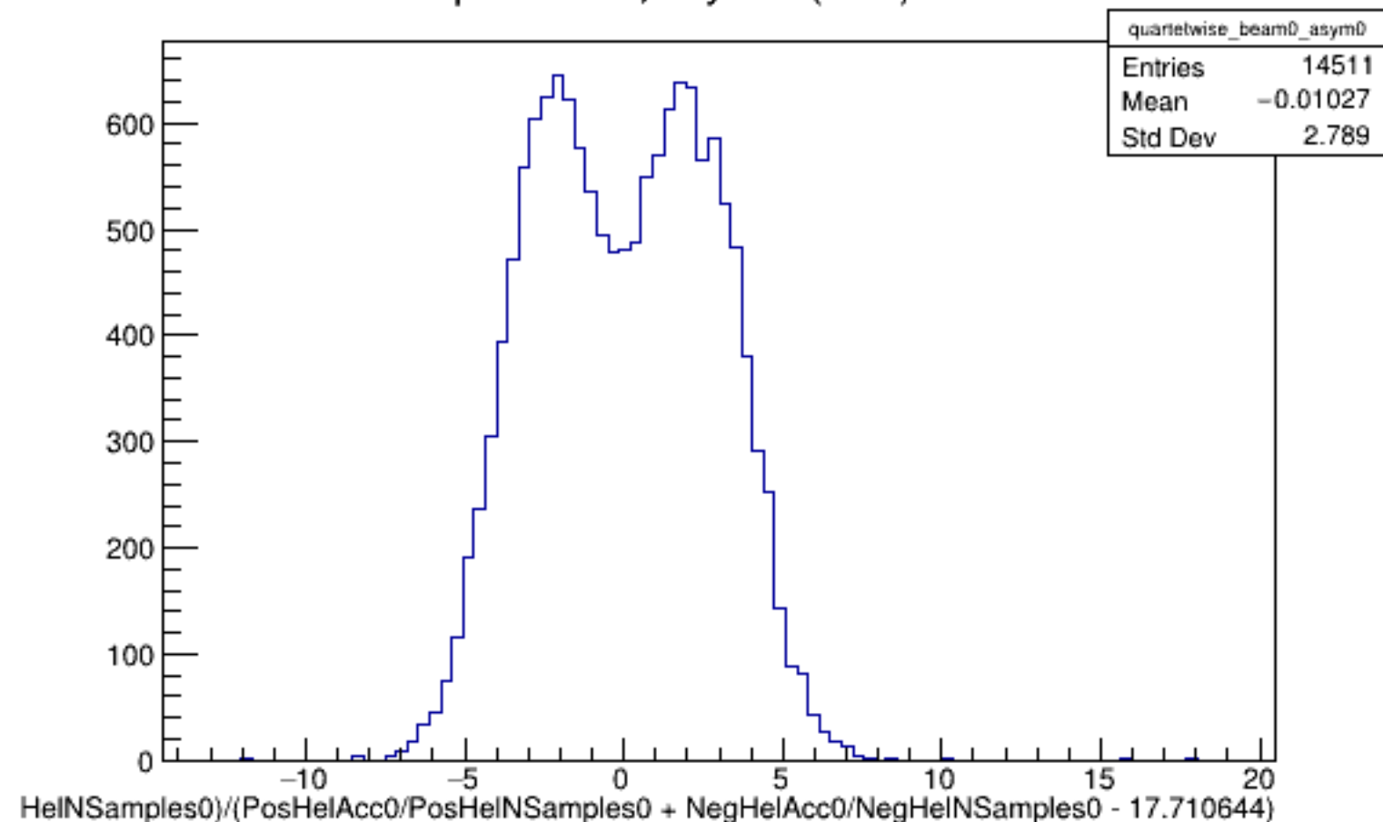
Run 4331 quartetwise, Asyms0 (Raw): Beam OFF
