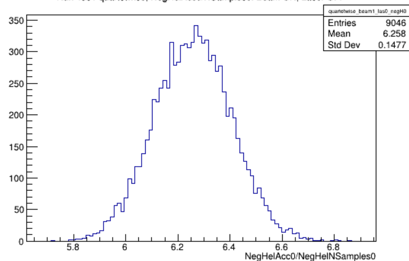
Run 4331 quartetwise, NegHelAcc0/NSamples0: Beam ON, Laser OFF
