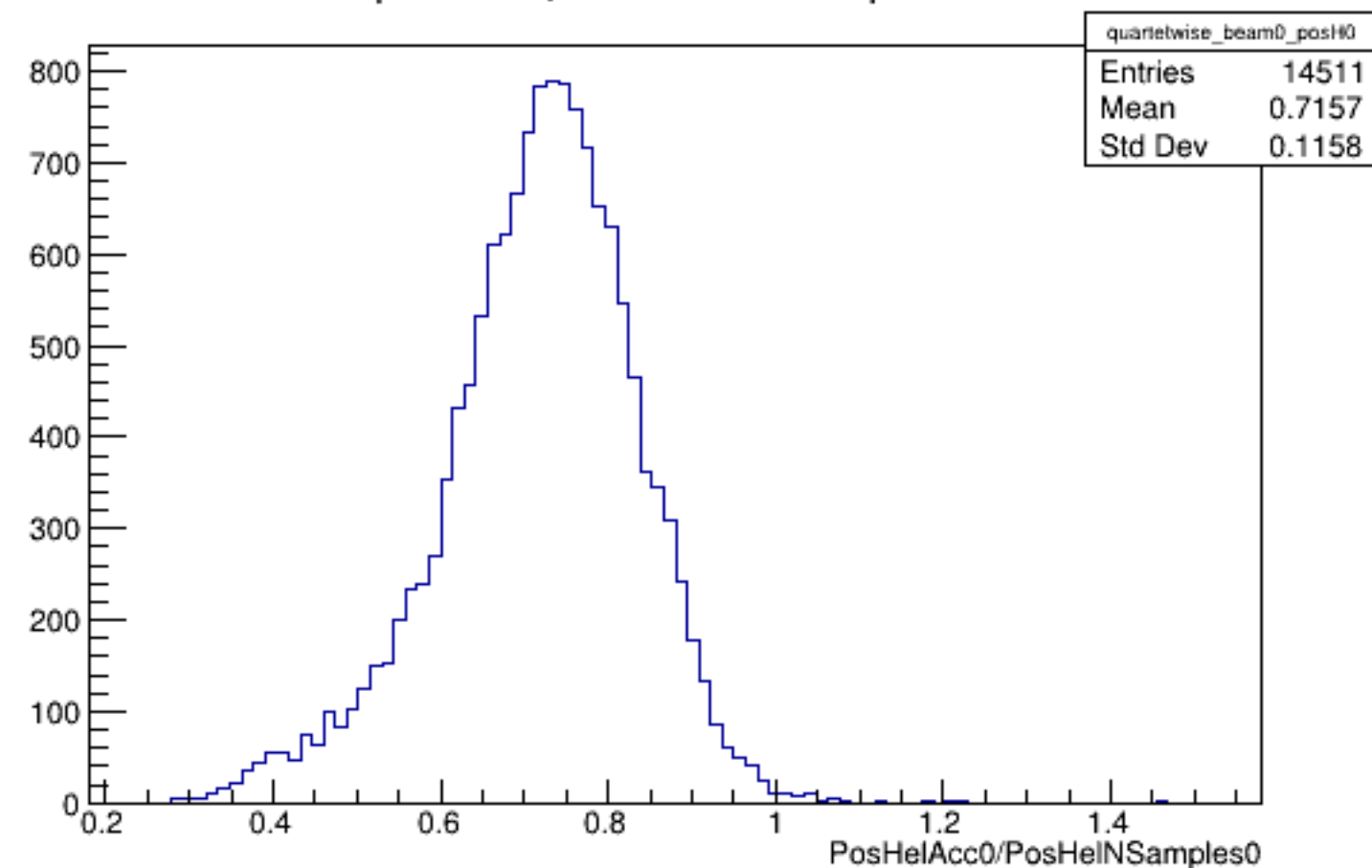
Run 4331 quartetwise, PosHelAcc0/NSamples0: Beam OFF
