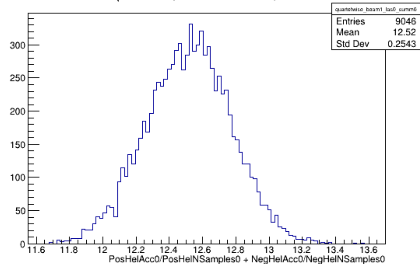
Run 4331 quartetwise, Sums0: Beam ON, Laser OFF
