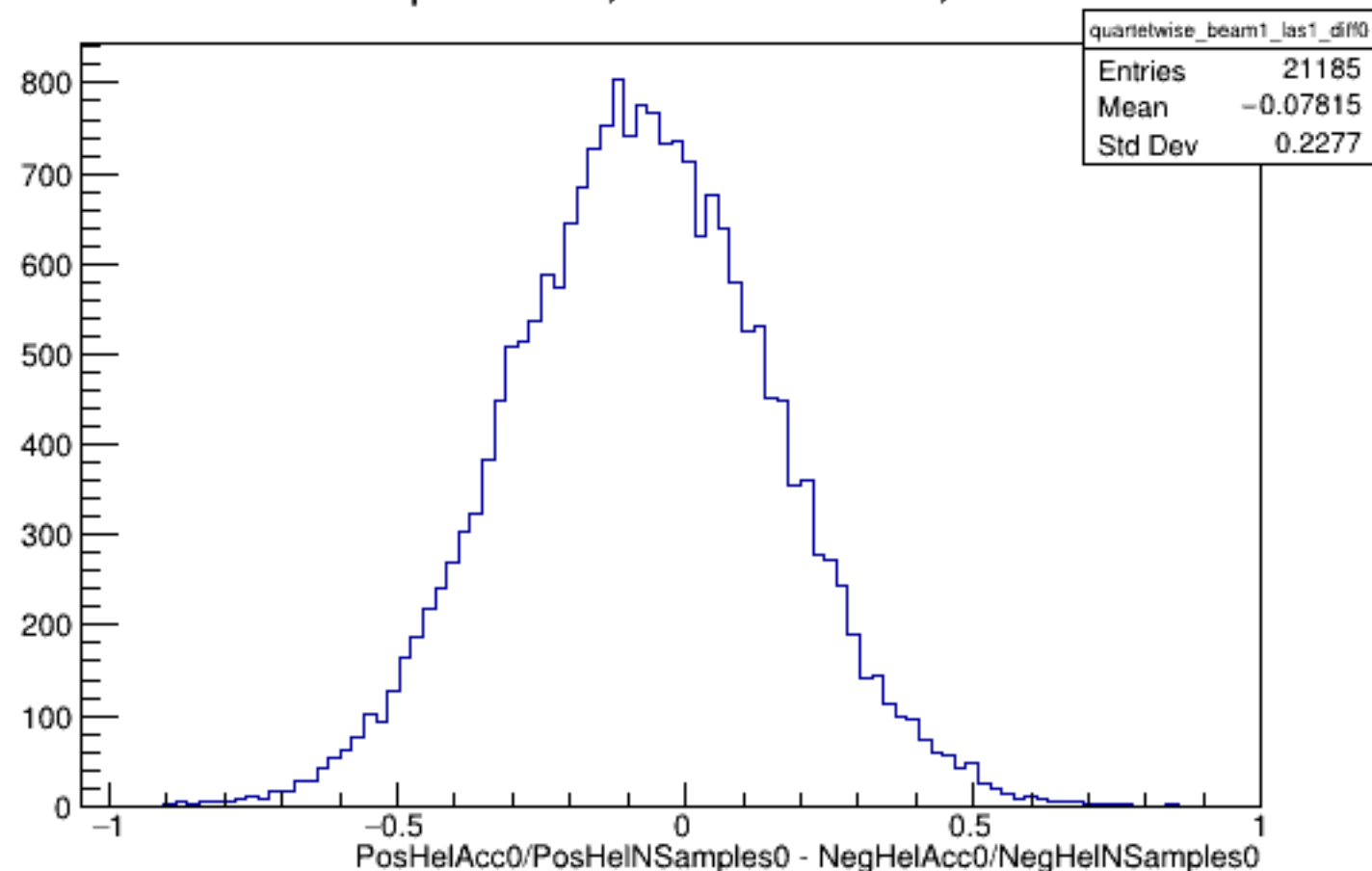
Run 4331 quartetwise, Diffs0: Beam ON, Laser ON
