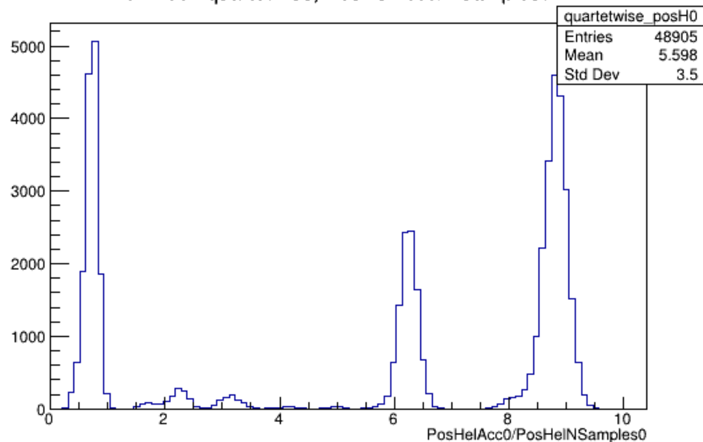
Run 4331 quartetwise, PosHelAcc0/NSamples0: All
