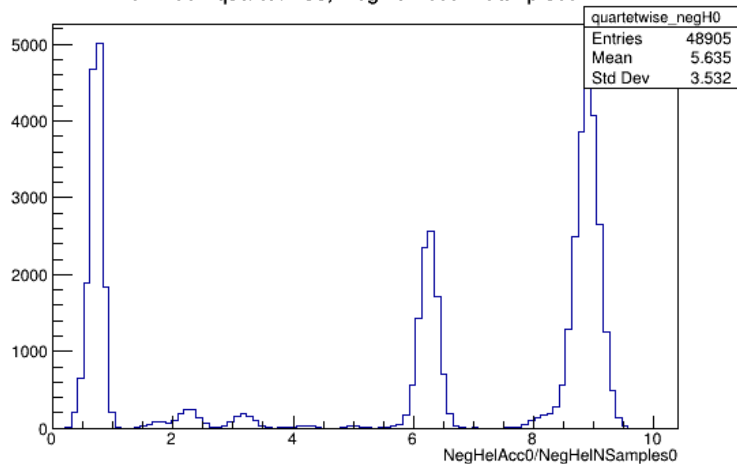
Run 4331 quartetwise, NegHelAcc0/NSamples0: All
