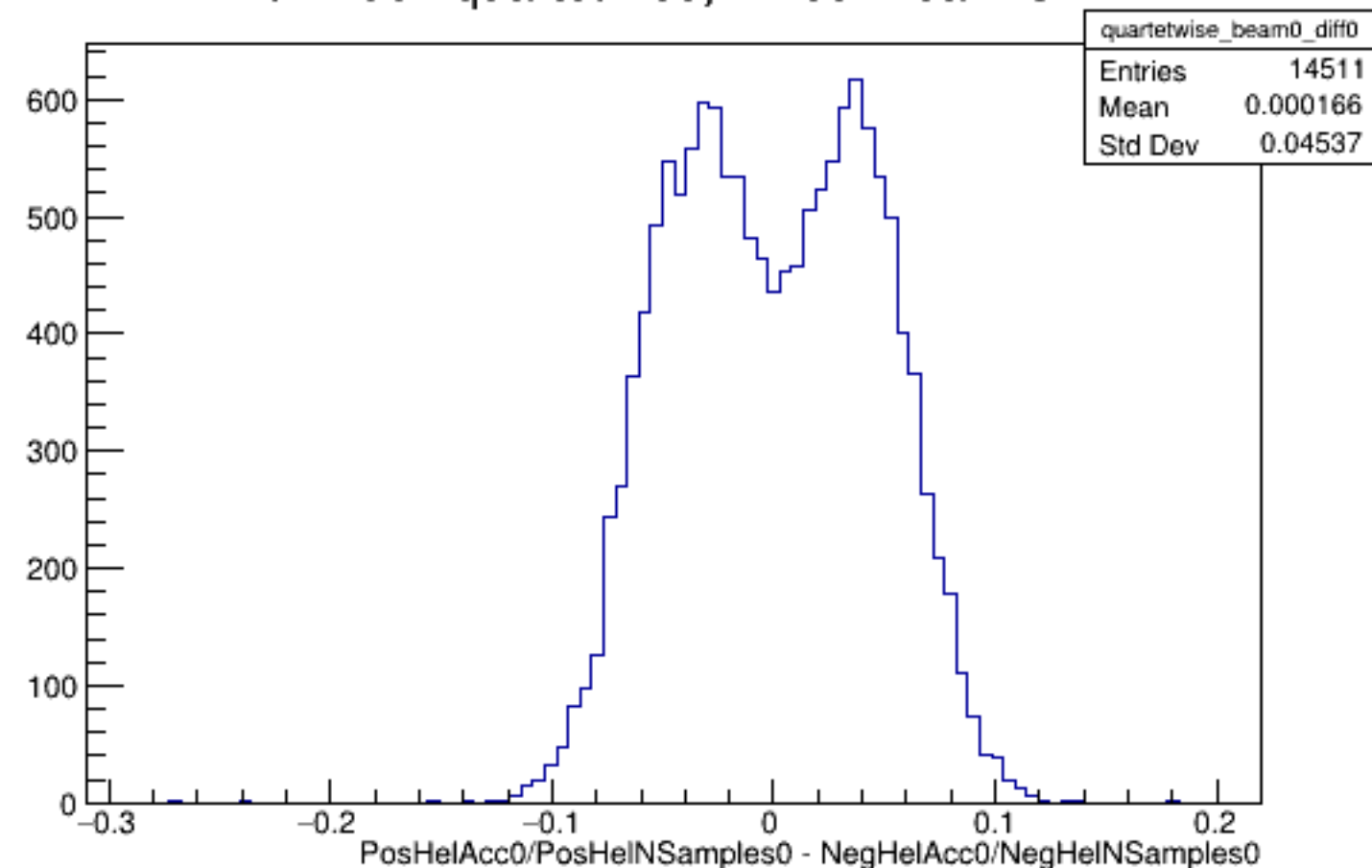
Run 4331 quartetwise, Diffs0: Beam OFF
