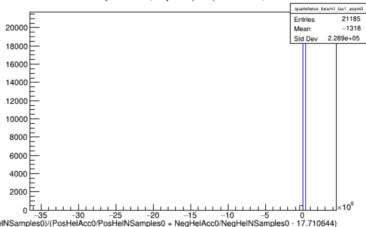
Run 4331 quartetwise, Asyms0 (Raw): Beam ON, Laser ON
