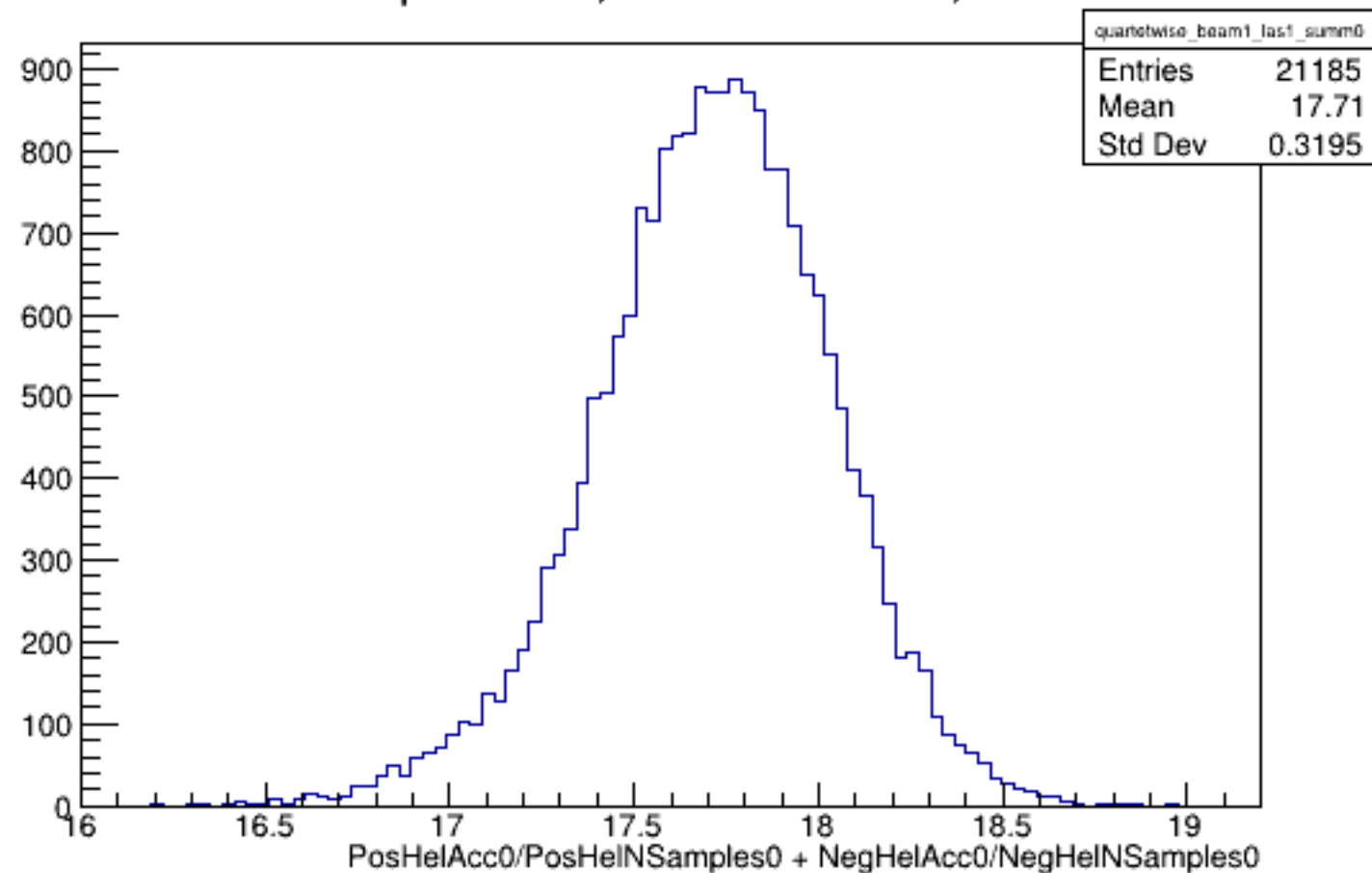
Run 4331 quartetwise, Sums0: Beam ON, Laser ON
