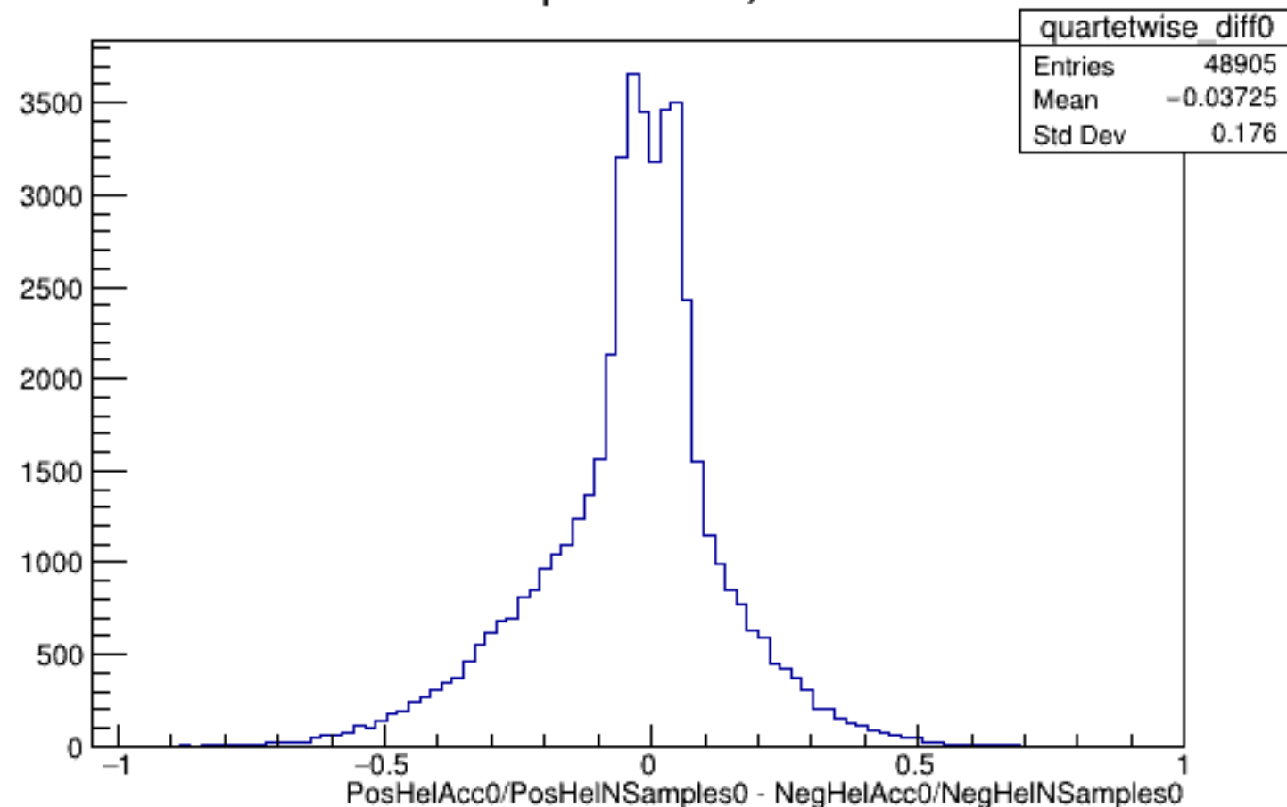
Run 4331 quartetwise, Diffs0: All
