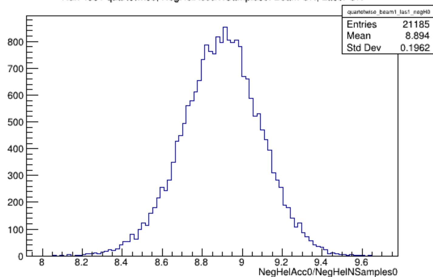
Run 4331 quartetwise, NegHelAcc0/NSamples0: Beam ON, Laser ON
