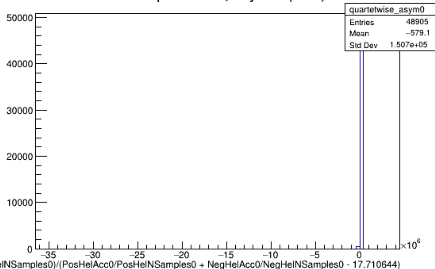
Run 4331 quartetwise, Asyms0 (Raw): All
