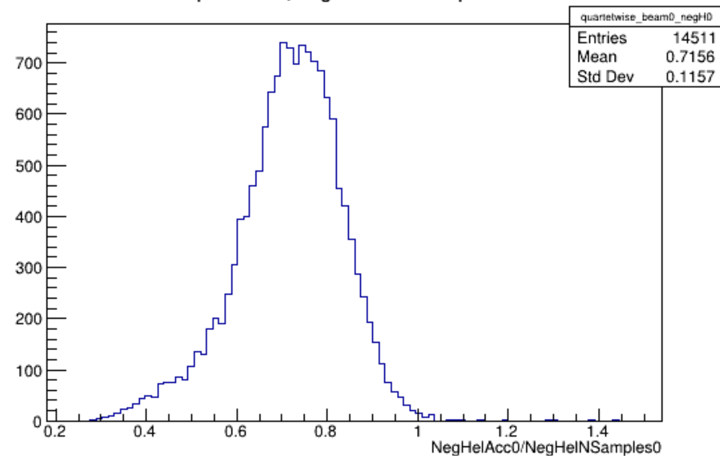
Run 4331 quartetwise, NegHelAcc0/NSamples0: Beam OFF
