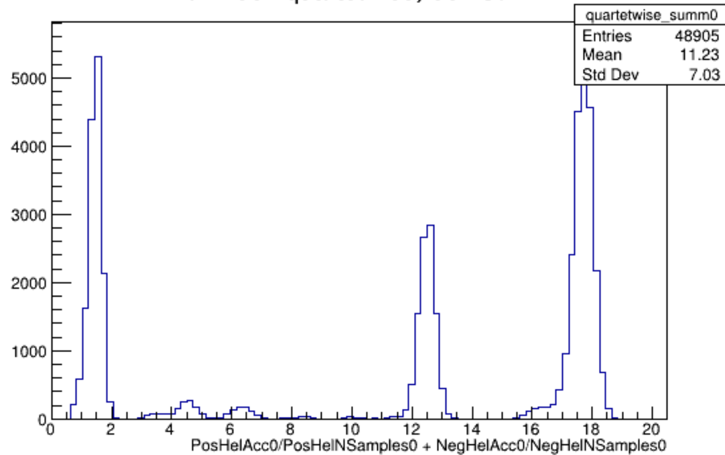
Run 4331 quartetwise, Sums0: All
