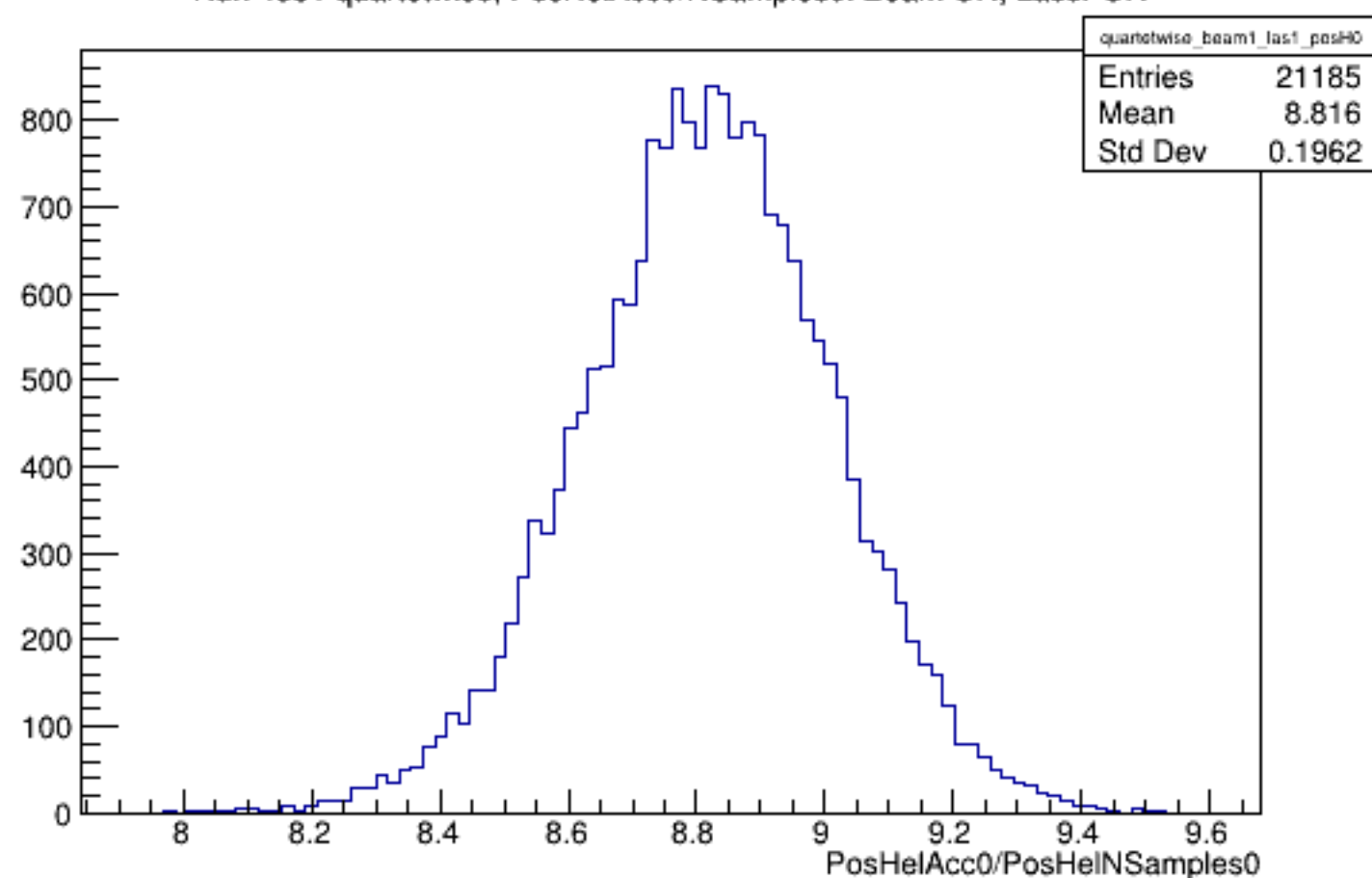
Run 4331 quartetwise, PosHelAcc0/NSamples0: Beam ON, Laser ON
