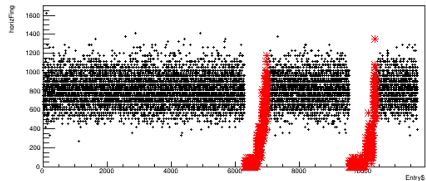
Run 4334, quartetwise: horizFing vs time
