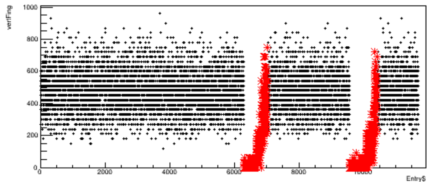
Run 4334, quartetwise: vertFing vs time
