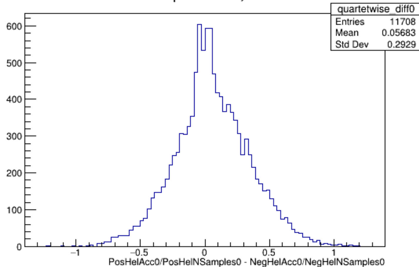
Run 4334 quartetwise, Diffs0: All
