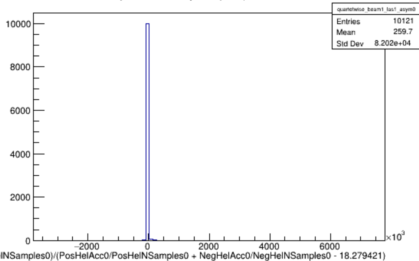
Run 4334 quartetwise, Asyms0 (Raw): Beam ON, Laser ON
