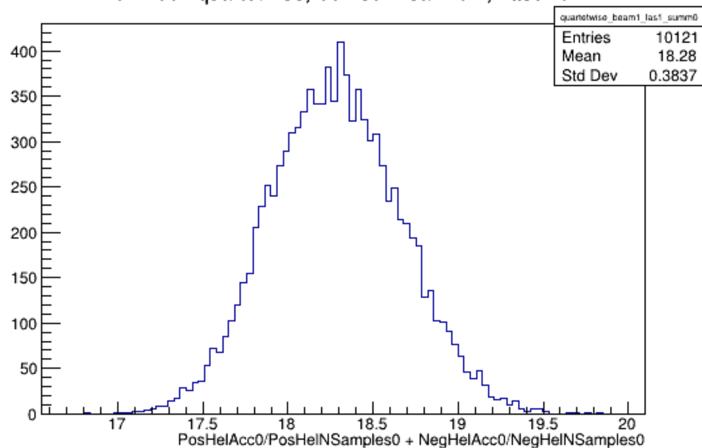
Run 4334 quartetwise, Sums0: Beam ON, Laser ON
