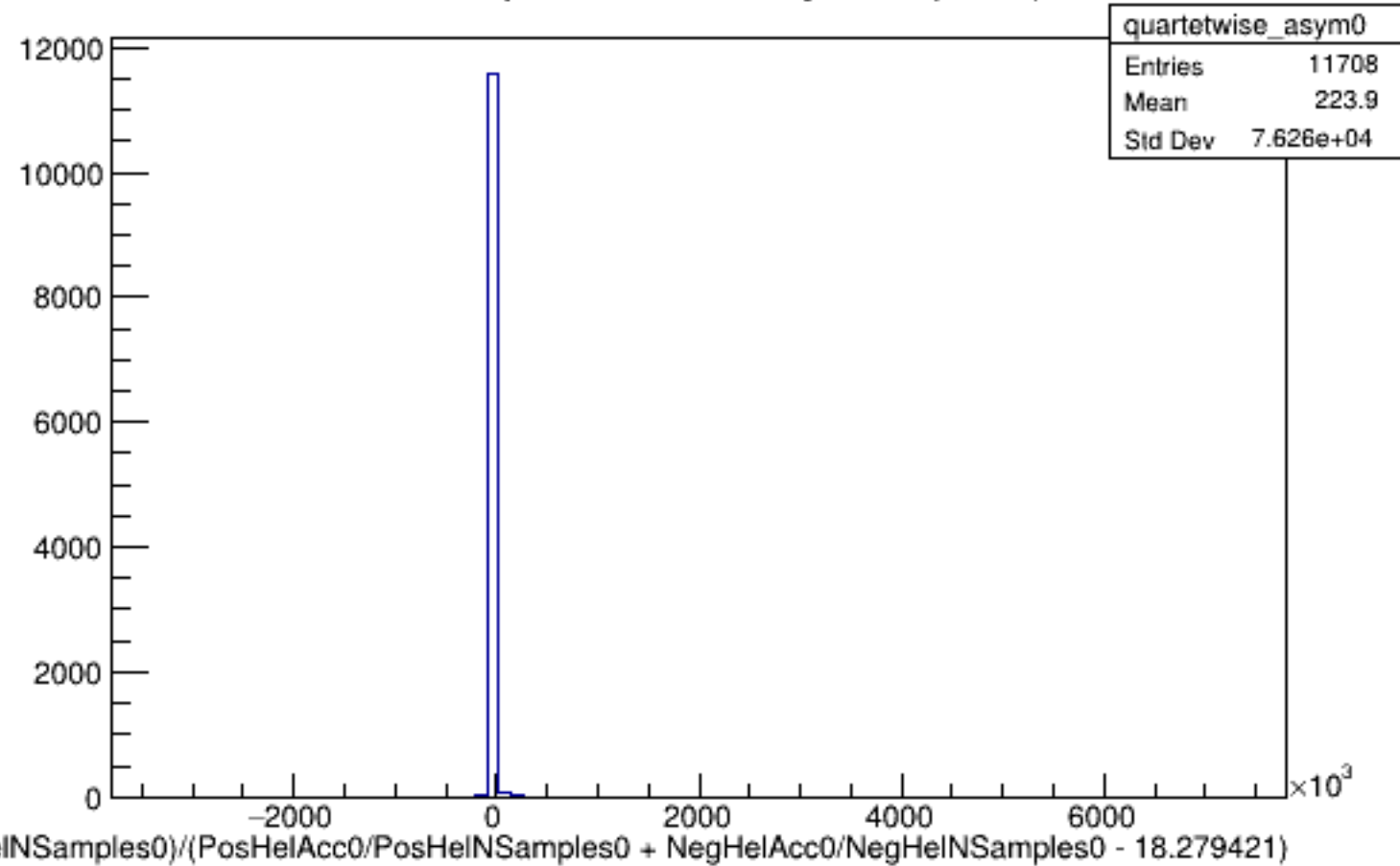
Run 4334 quartetwise, Asyms0 (Raw): All
