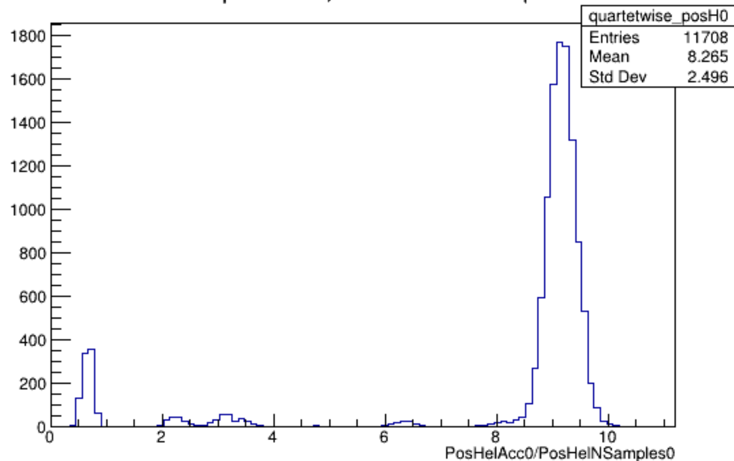
Run 4334 quartetwise, PosHelAcc0/NSamples0: All
