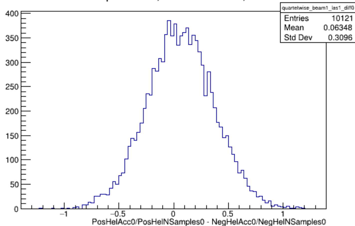
Run 4334 quartetwise, Diffs0: Beam ON, Laser ON
