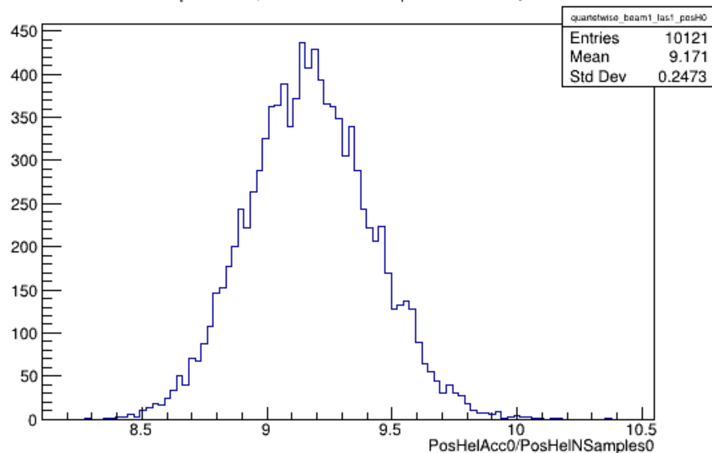
Run 4334 quartetwise, PosHelAcc0/NSamples0: Beam ON, Laser ON
