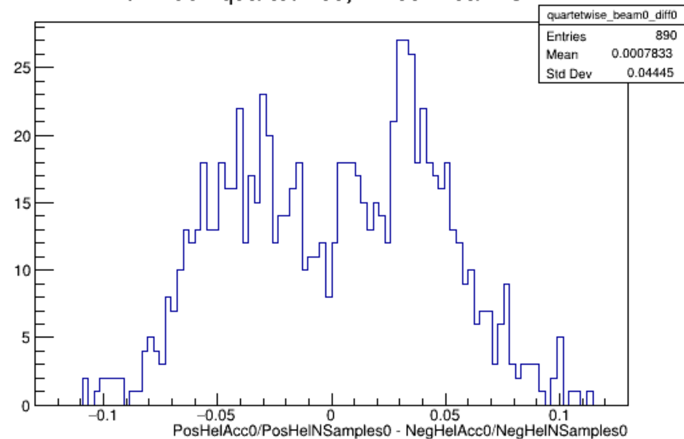
Run 4334 quartetwise, Diffs0: Beam OFF
