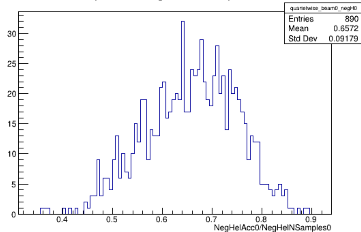
Run 4334 quartetwise, NegHelAcc0/NSamples0: Beam OFF
