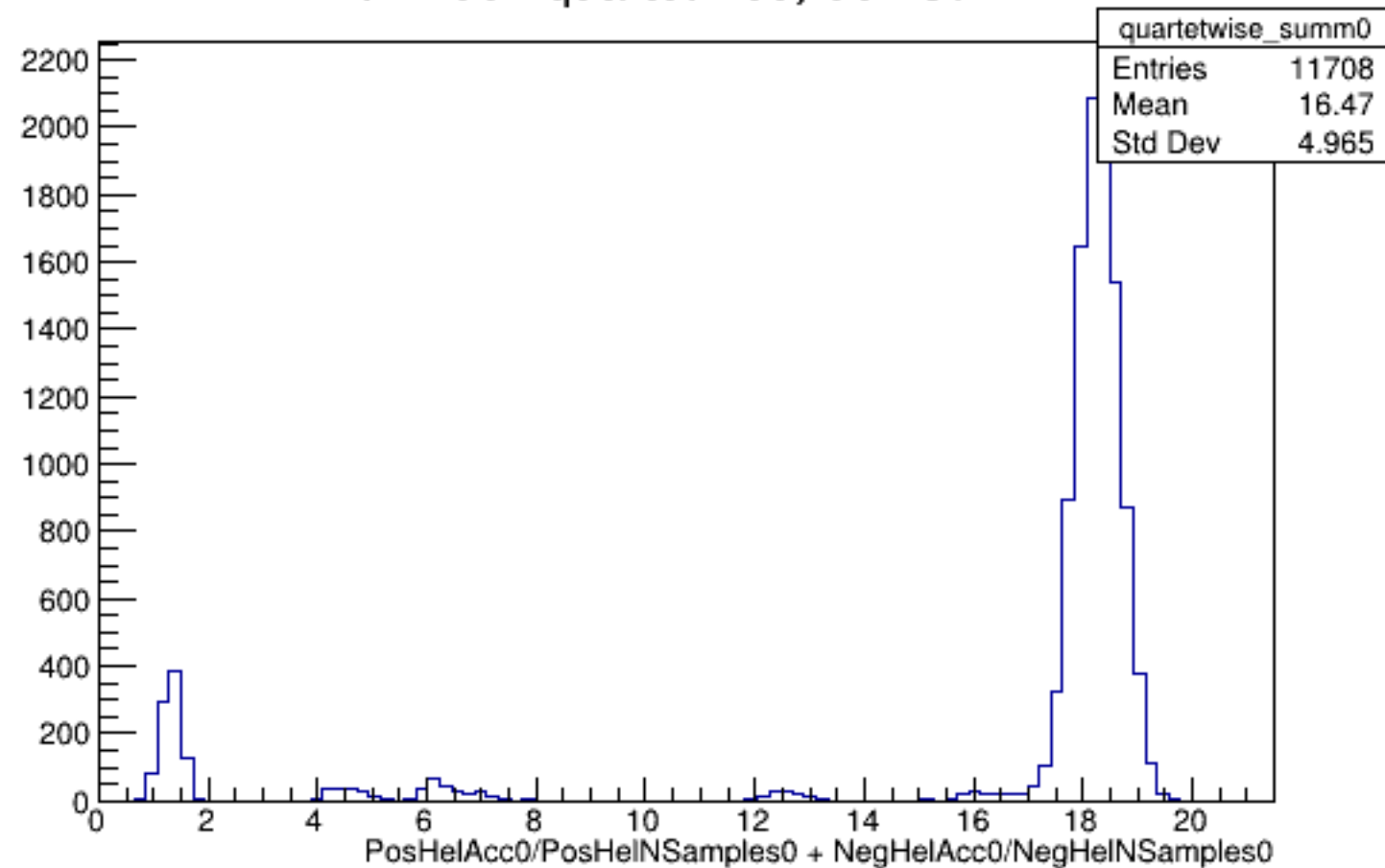
Run 4334 quartetwise, Sums0: All
