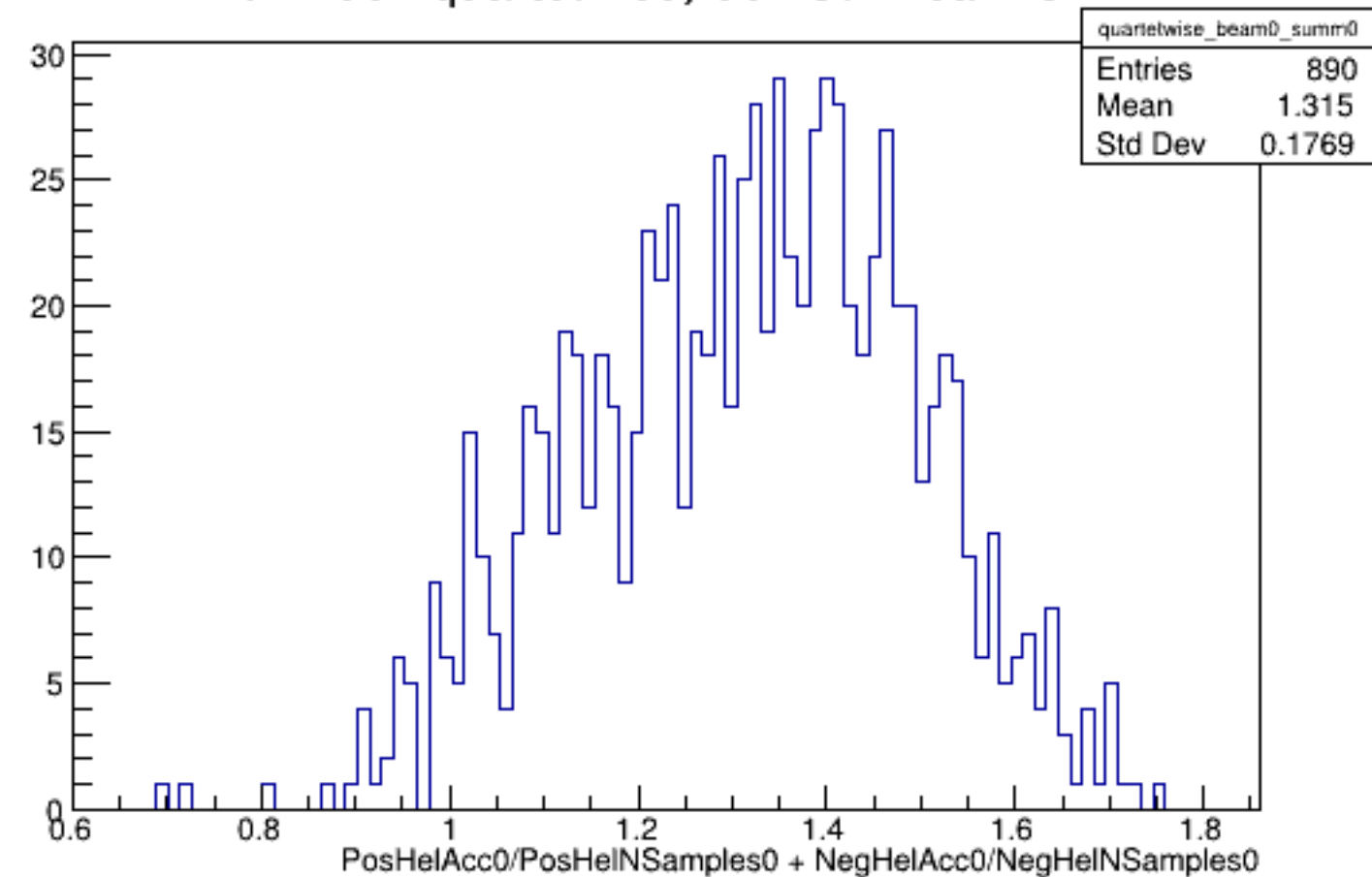
Run 4334 quartetwise, Sums0: Beam OFF
