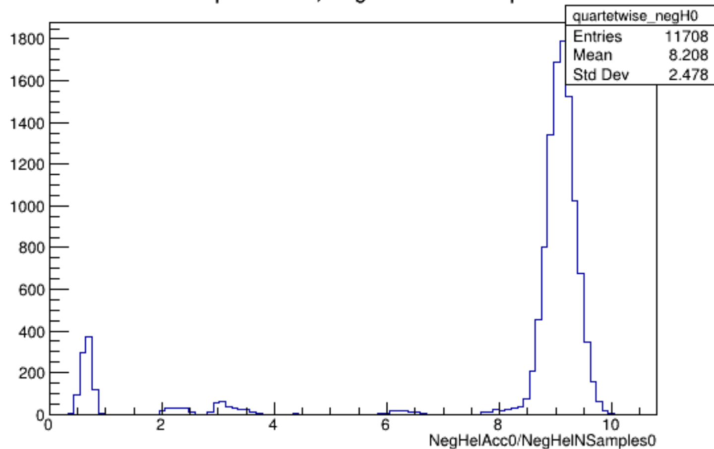
Run 4334 quartetwise, NegHelAcc0/NSamples0: All
