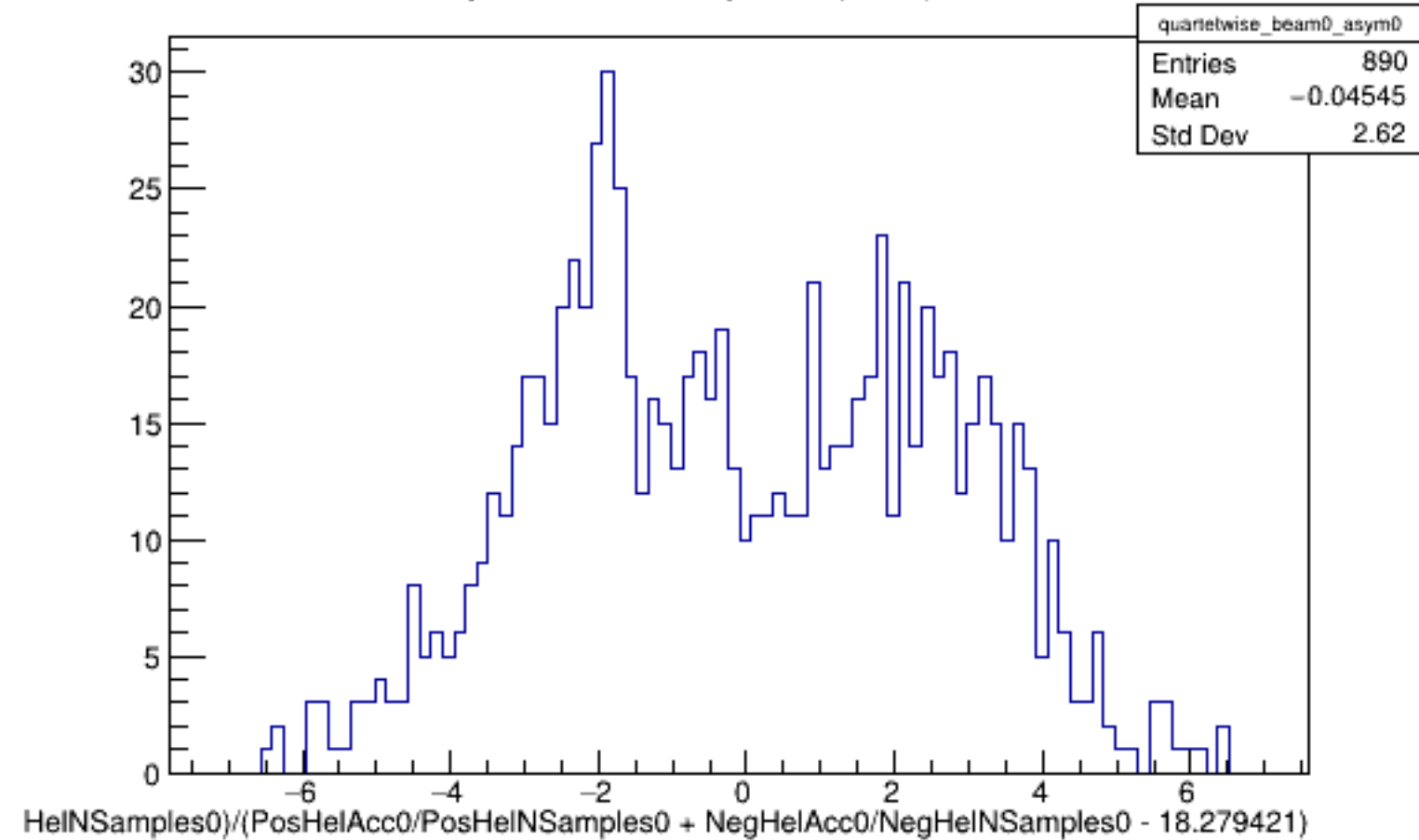
Run 4334 quartetwise, Asyms0 (Raw): Beam OFF
