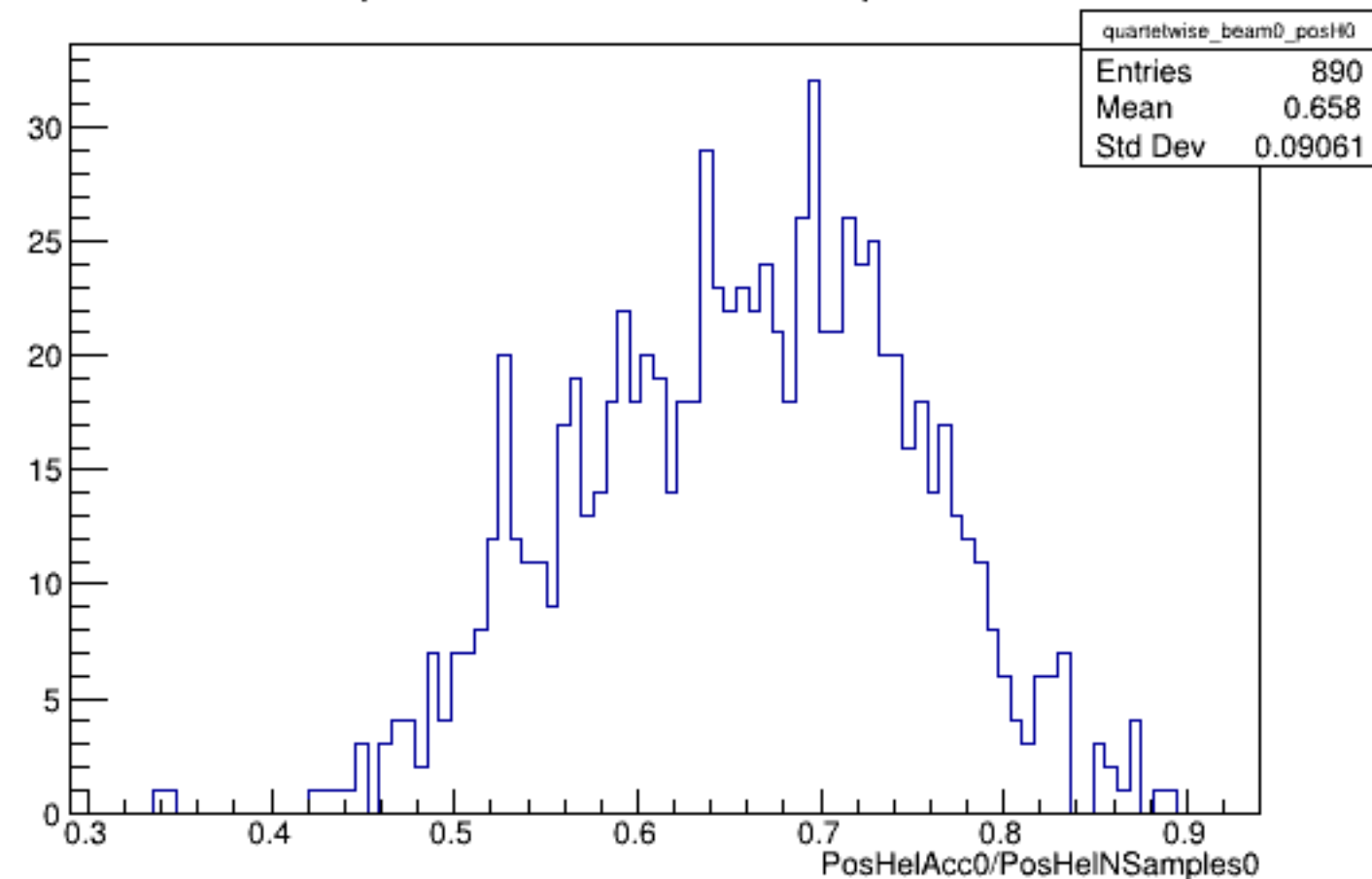
Run 4334 quartetwise, PosHelAcc0/NSamples0: Beam OFF
