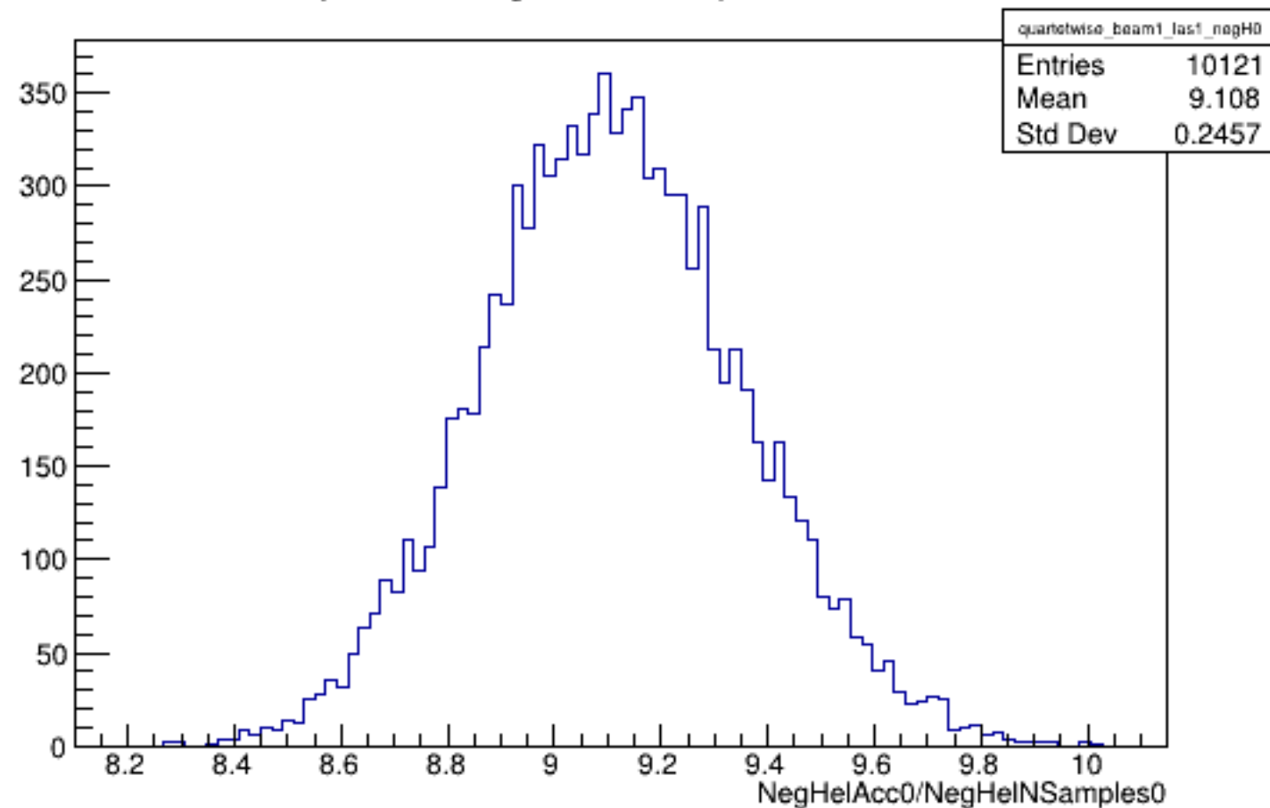
Run 4334 quartetwise, NegHelAcc0/NSamples0: Beam ON, Laser ON
