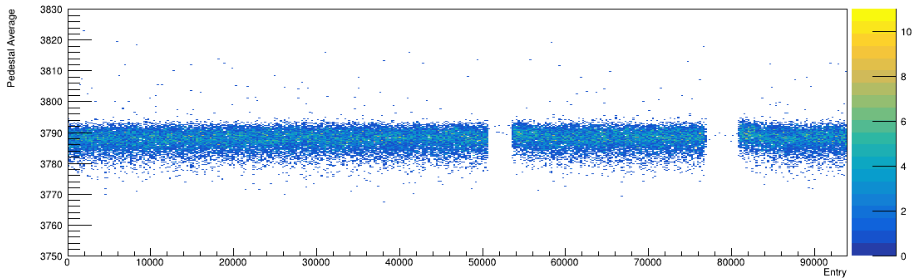
Run 4334, snapshots: Pedestal vs. Time
