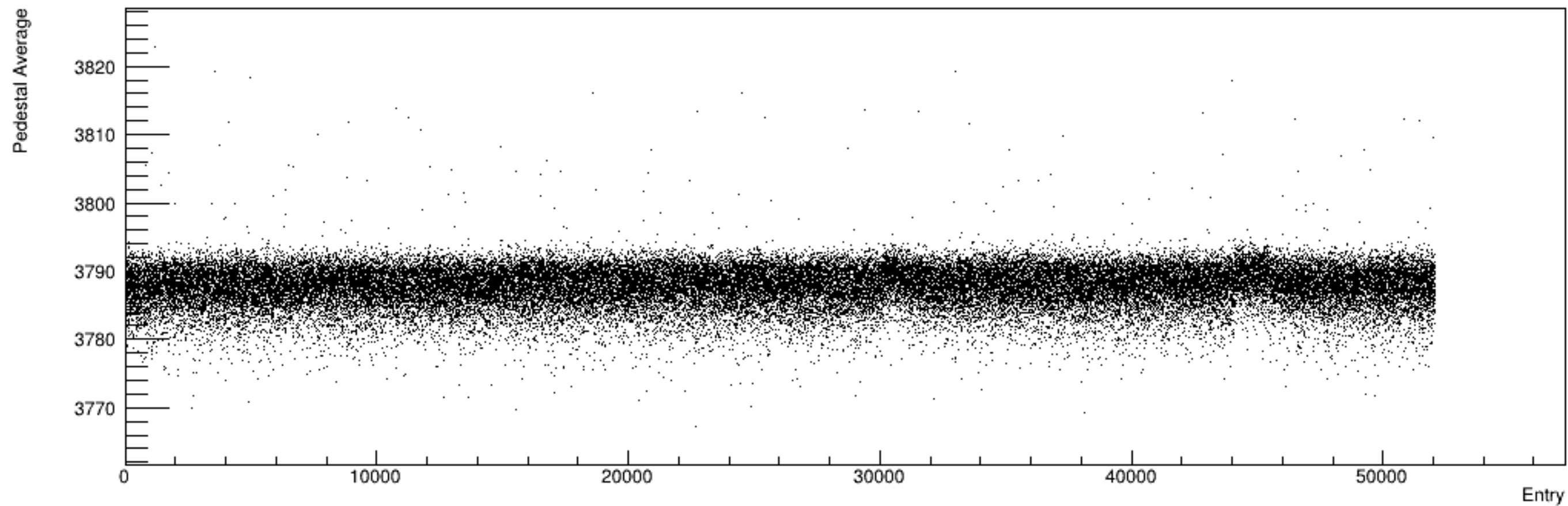
Run 4334, snapshots: Pedestal vs. Time
