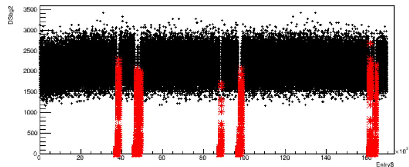
Run 4343, quartetwise: DSbg2 vs time
