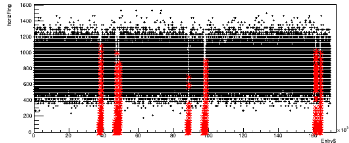
Run 4343, quartetwise: horizFing vs time
