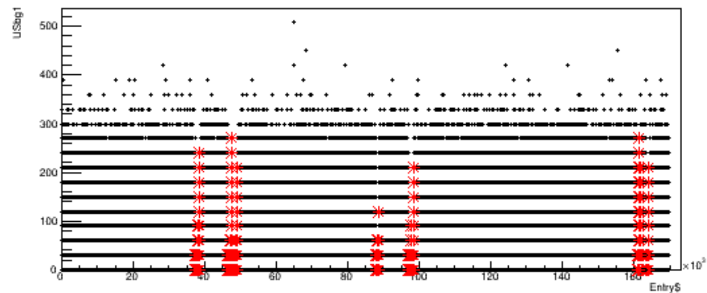
Run 4343, quartetwise: USbg1 vs time
