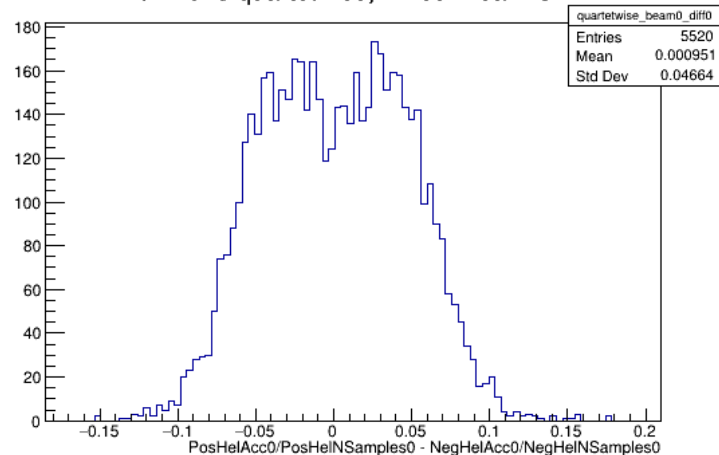
Run 4343 quartetwise, Diffs0: Beam OFF
