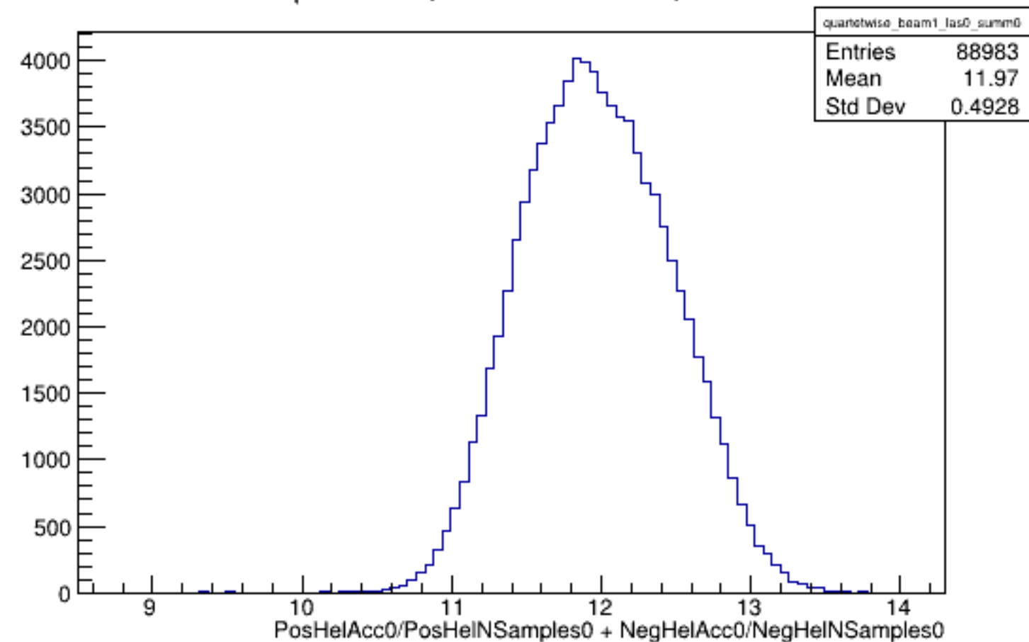
Run 4343 quartetwise, Sums0: Beam ON, Laser OFF
