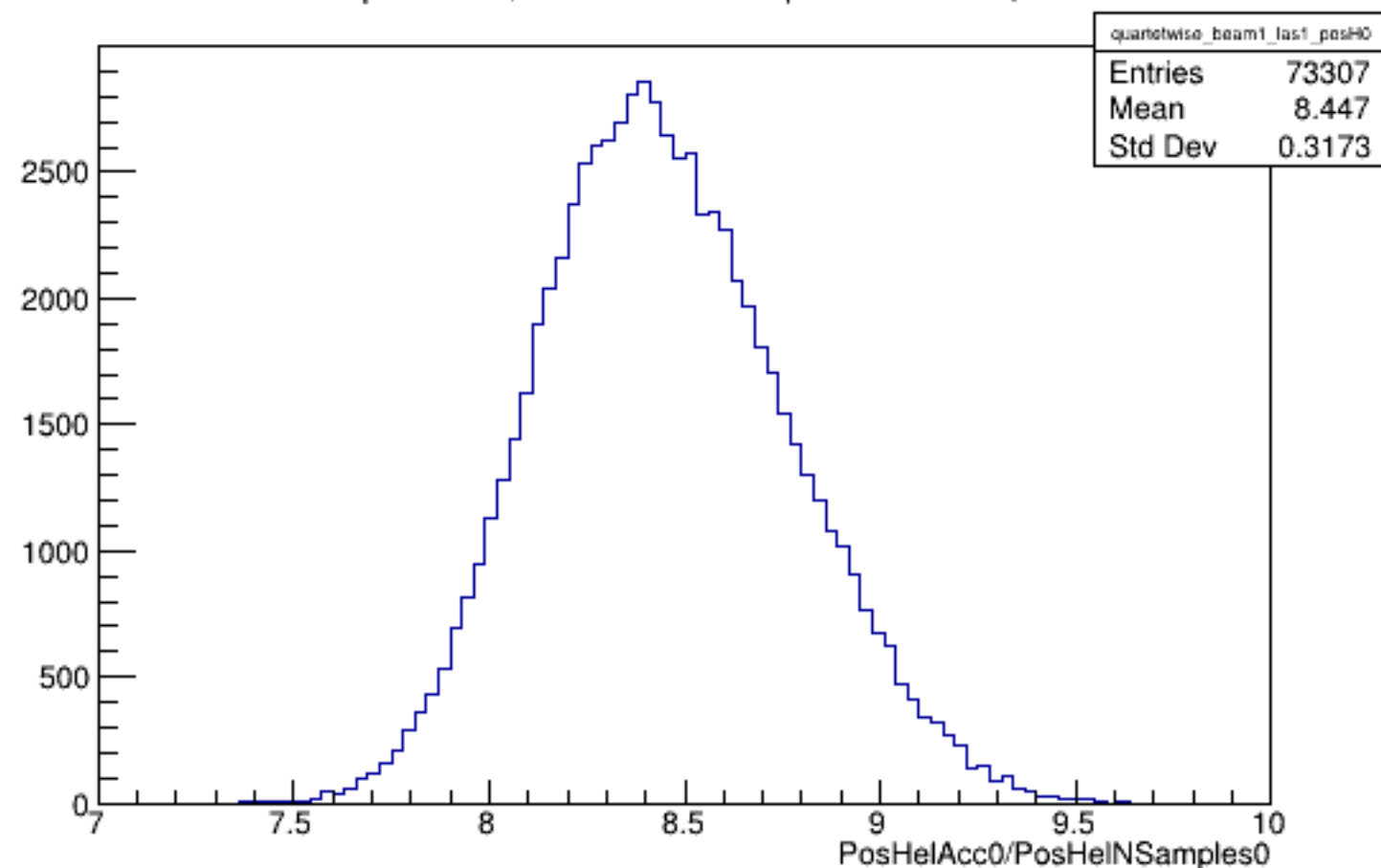
Run 4343 quartetwise, PosHelAcc0/NSamples0: Beam ON, Laser ON
