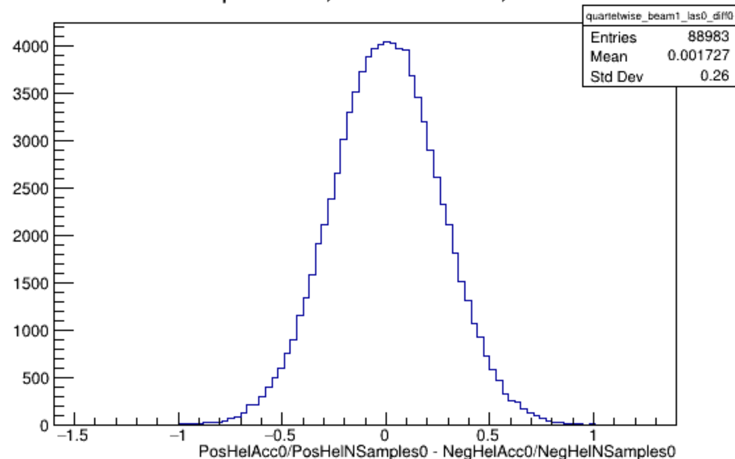
Run 4343 quartetwise, Diffs0: Beam ON, Laser OFF
