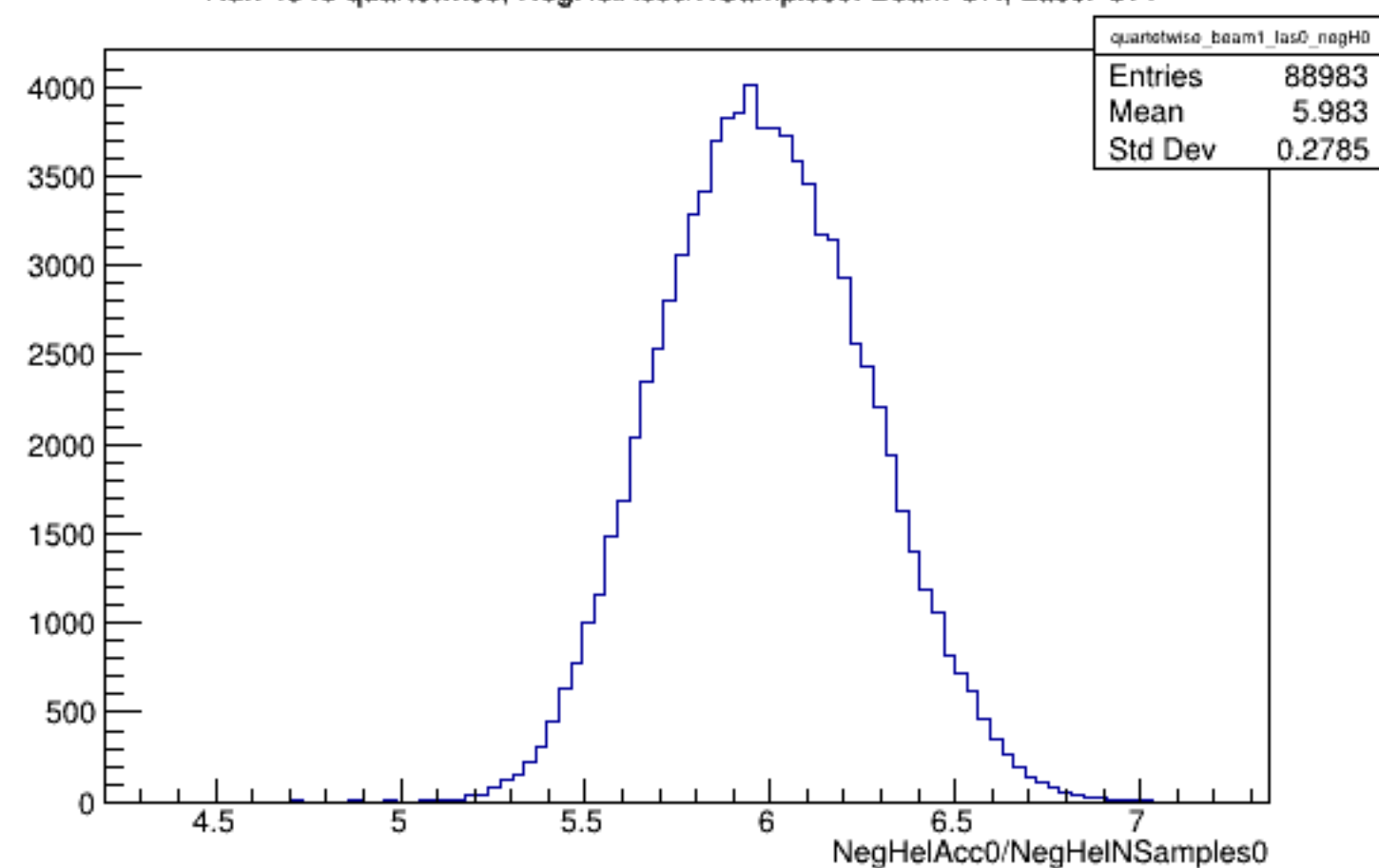
Run 4343 quartetwise, NegHelAcc0/NSamples0: Beam ON, Laser OFF
