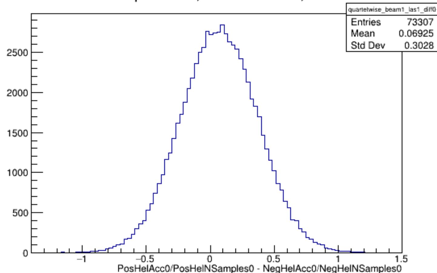
Run 4343 quartetwise, Diffs0: Beam ON, Laser ON
