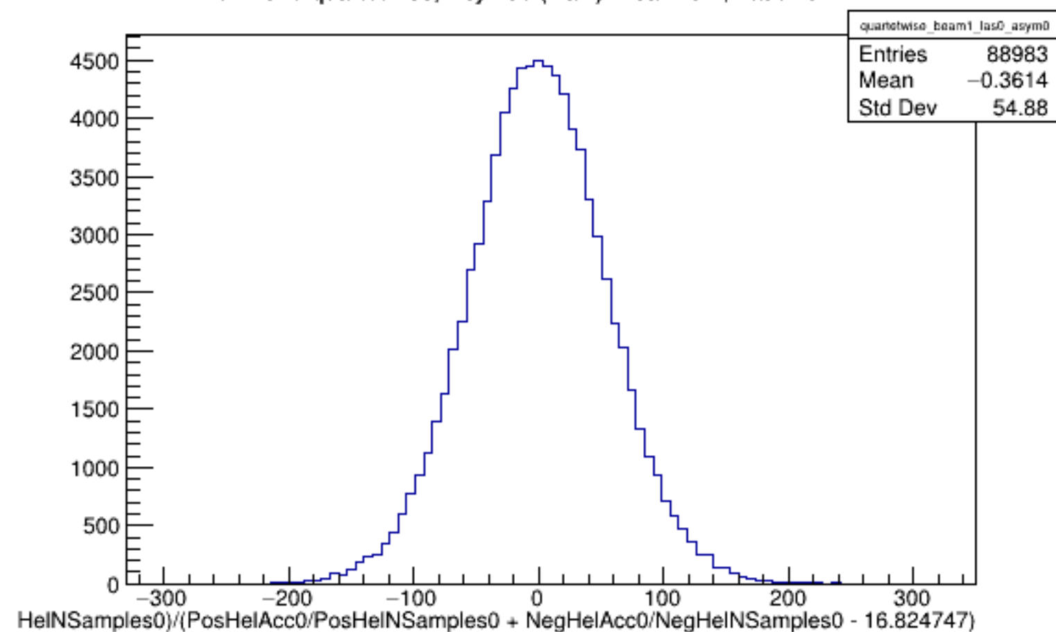
Run 4343 quartetwise, Asyms0 (Raw): Beam ON, Laser OFF
