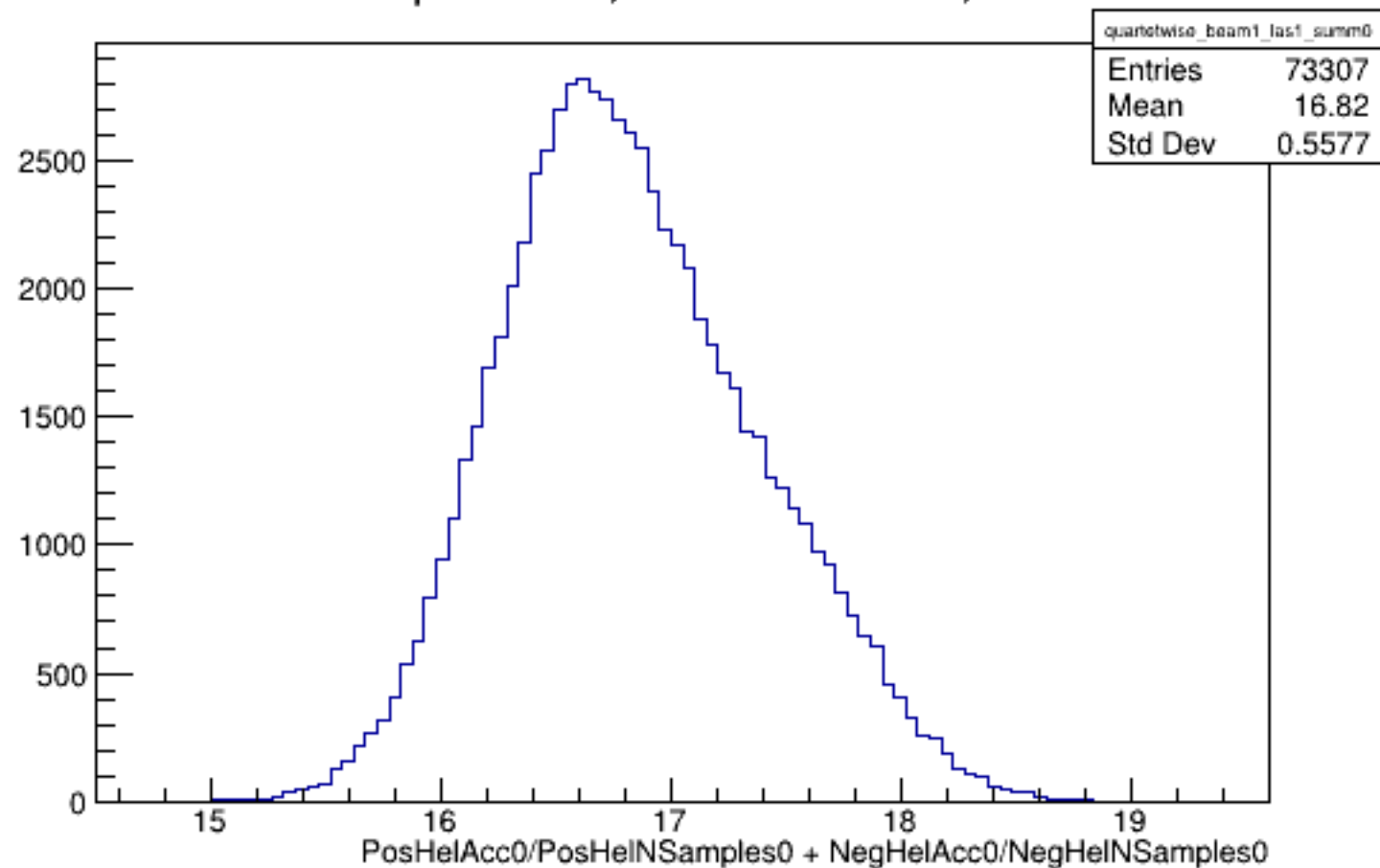
Run 4343 quartetwise, Sums0: Beam ON, Laser ON
