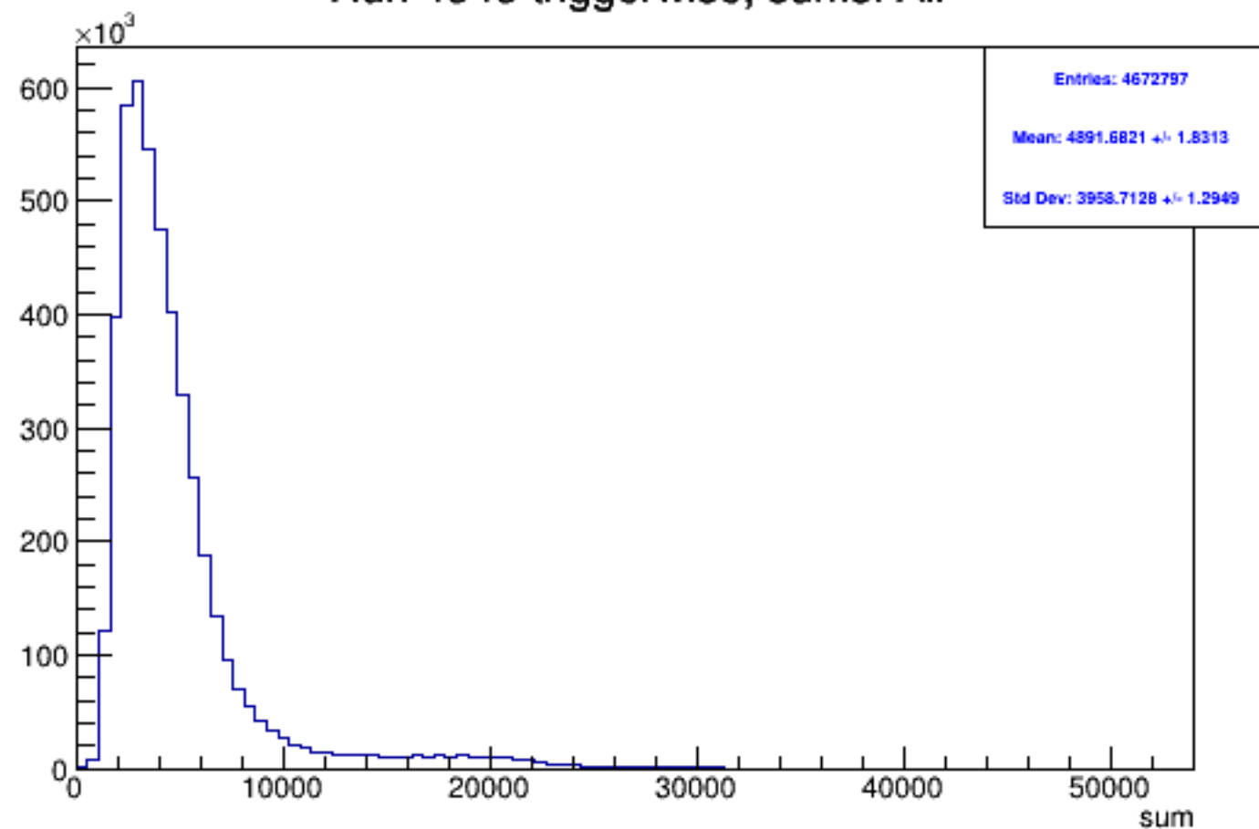
Run 4343 triggerwise, sums: All
