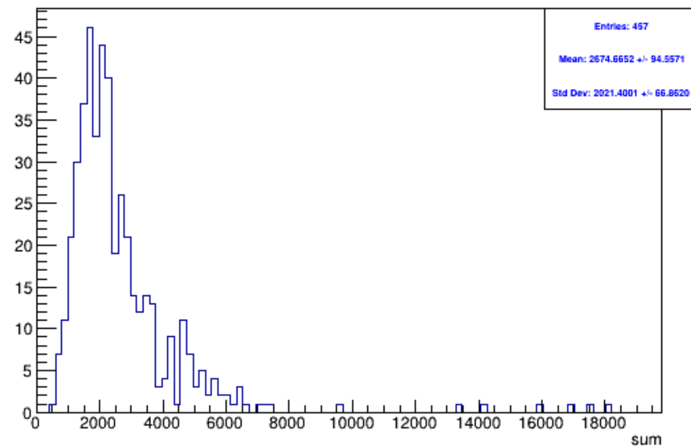
Run 4343 triggerwise, sums: Beam OFF
