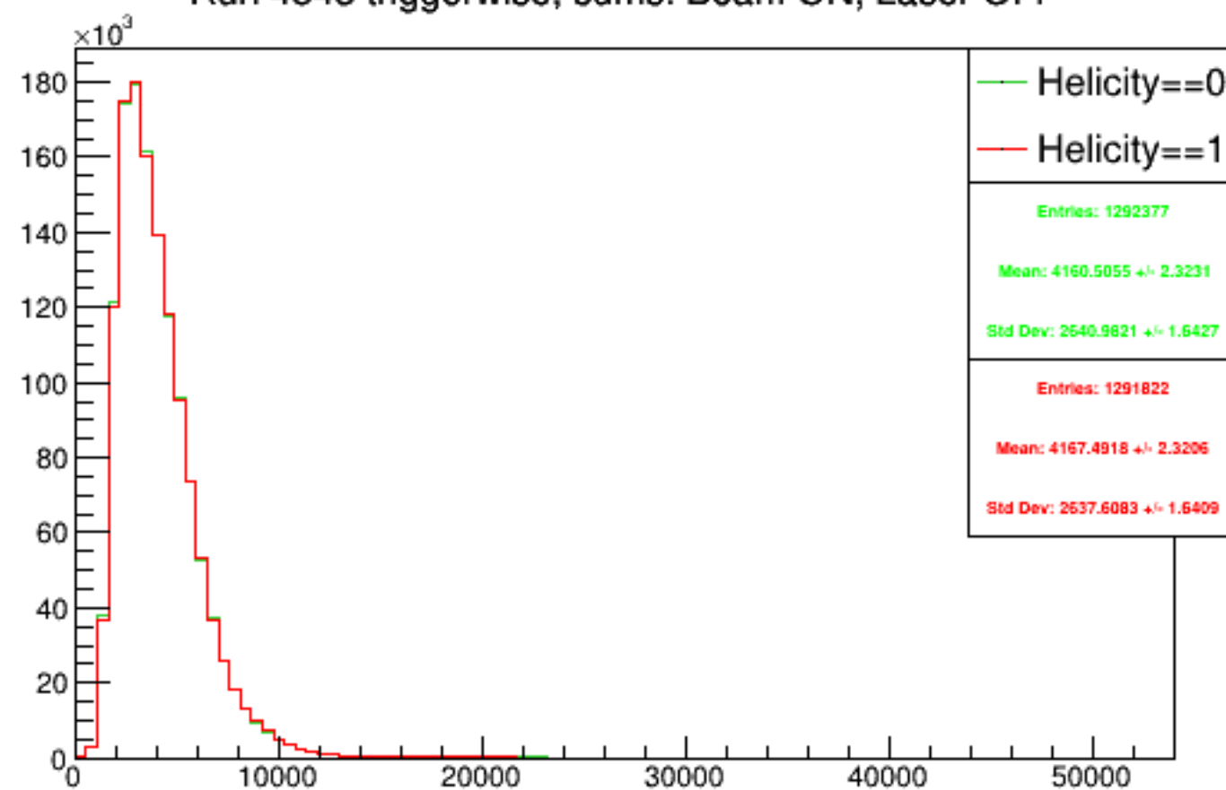
Run 4343 triggerwise, sums: Beam ON, Laser OFF
