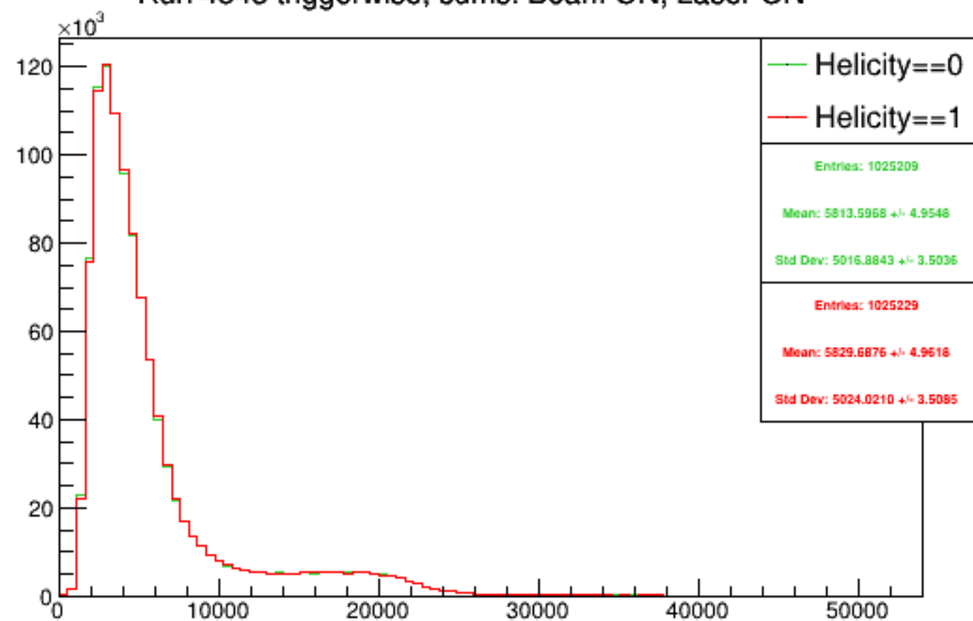
Run 4343 triggerwise, sums: Beam ON, Laser ON
