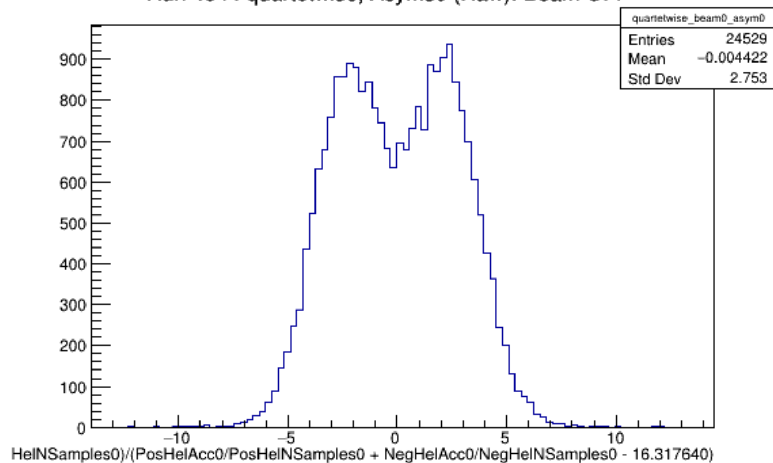
Run 4344 quartetwise, Asyms0 (Raw): Beam OFF
