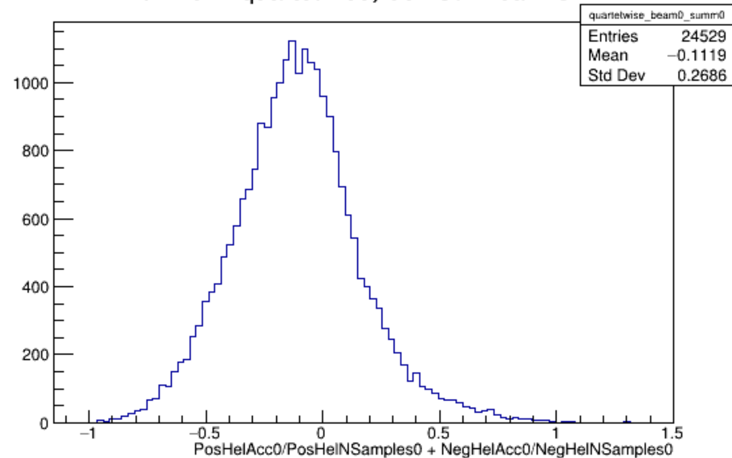
Run 4344 quartetwise, Sums0: Beam OFF
