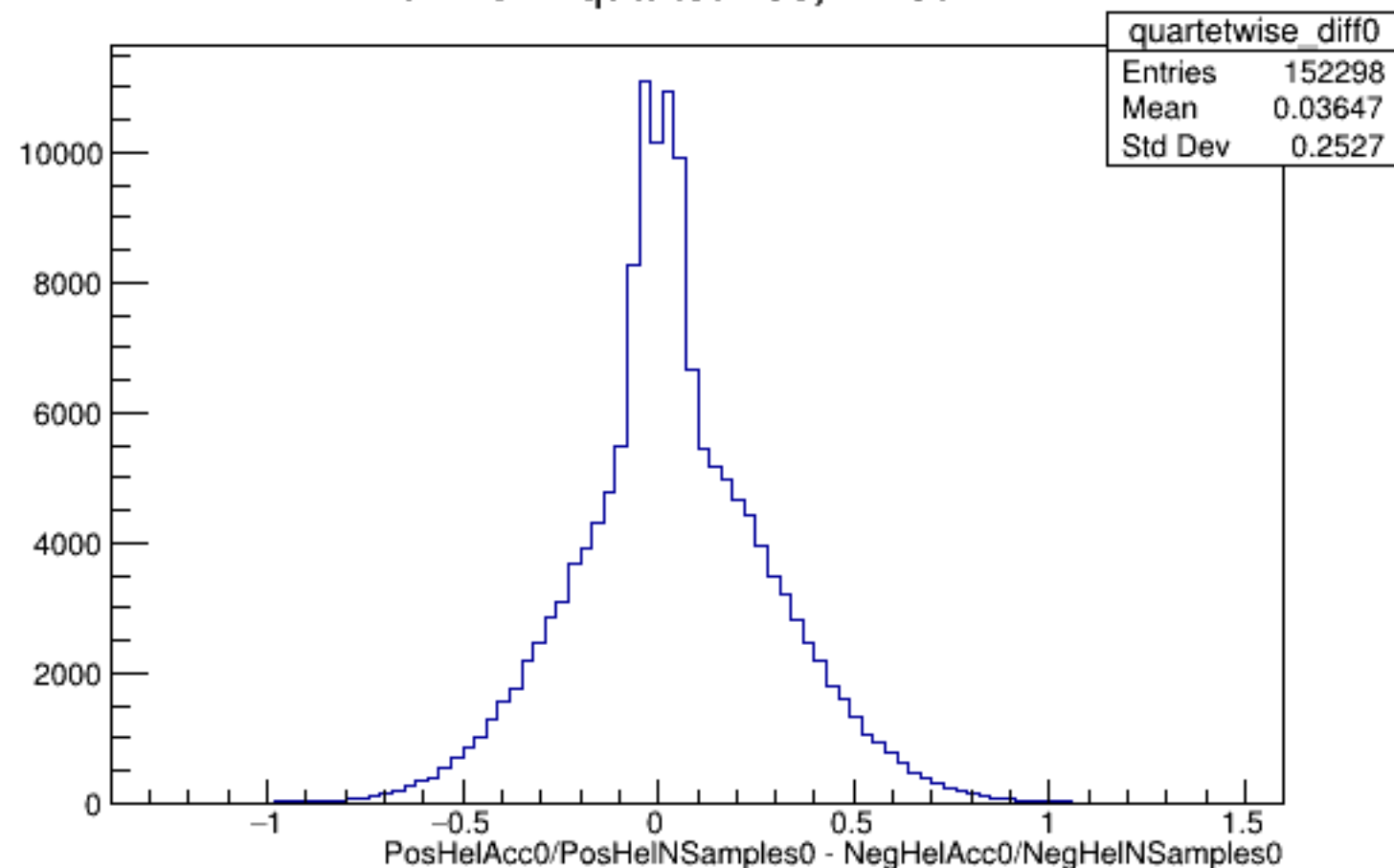
Run 4344 quartetwise, Diffs0: All
