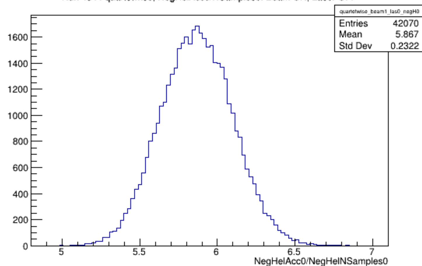
Run 4344 quartetwise, NegHelAcc0/NSamples0: Beam ON, Laser OFF
