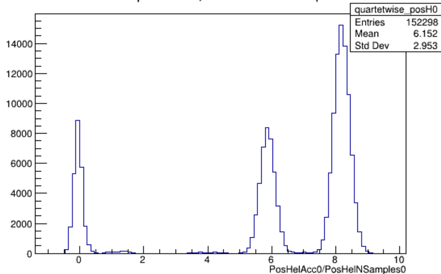
Run 4344 quartetwise, PosHelAcc0/NSamples0: All
