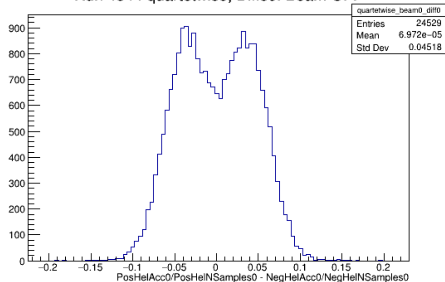
Run 4344 quartetwise, Diffs0: Beam OFF
