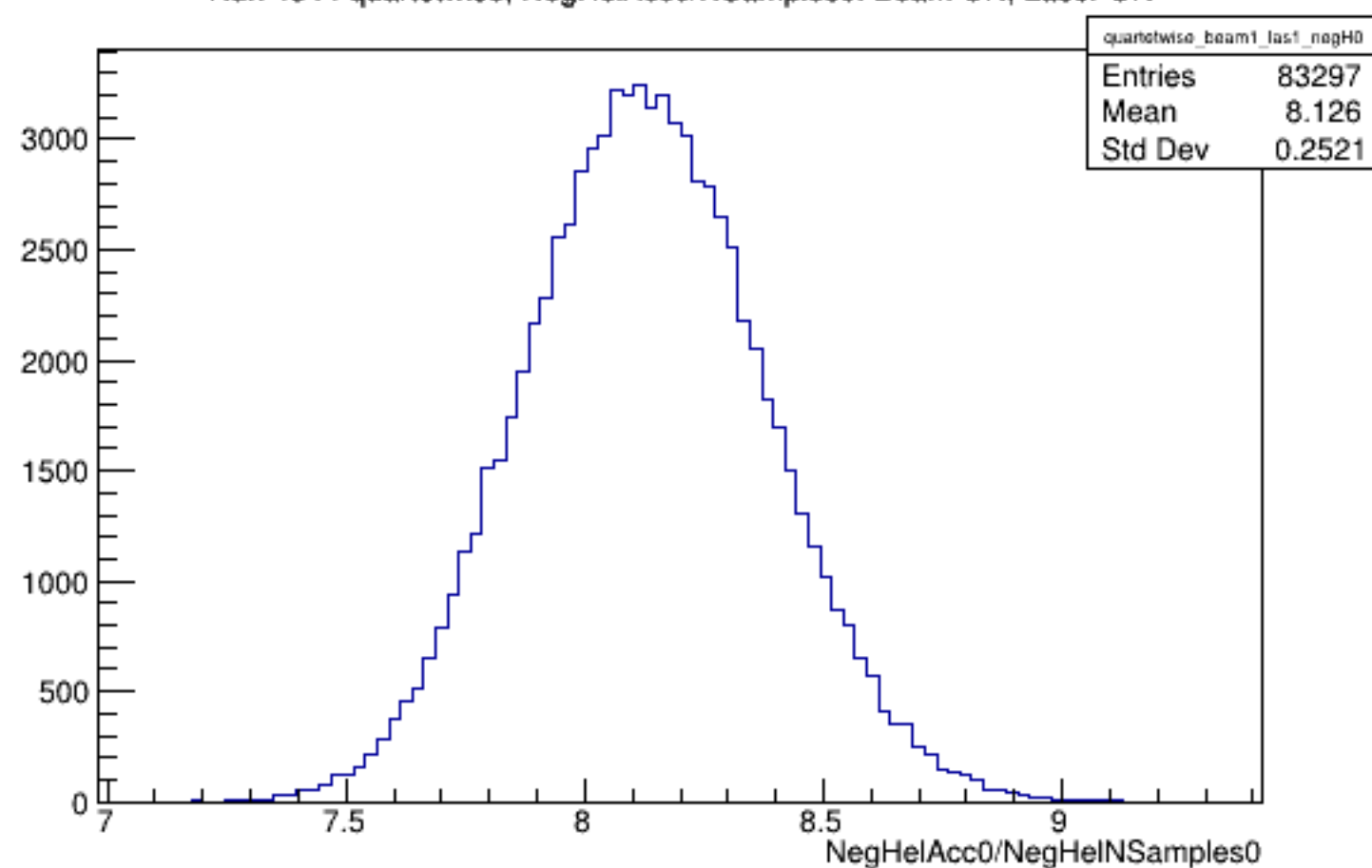
Run 4344 quartetwise, NegHelAcc0/NSamples0: Beam ON, Laser ON
