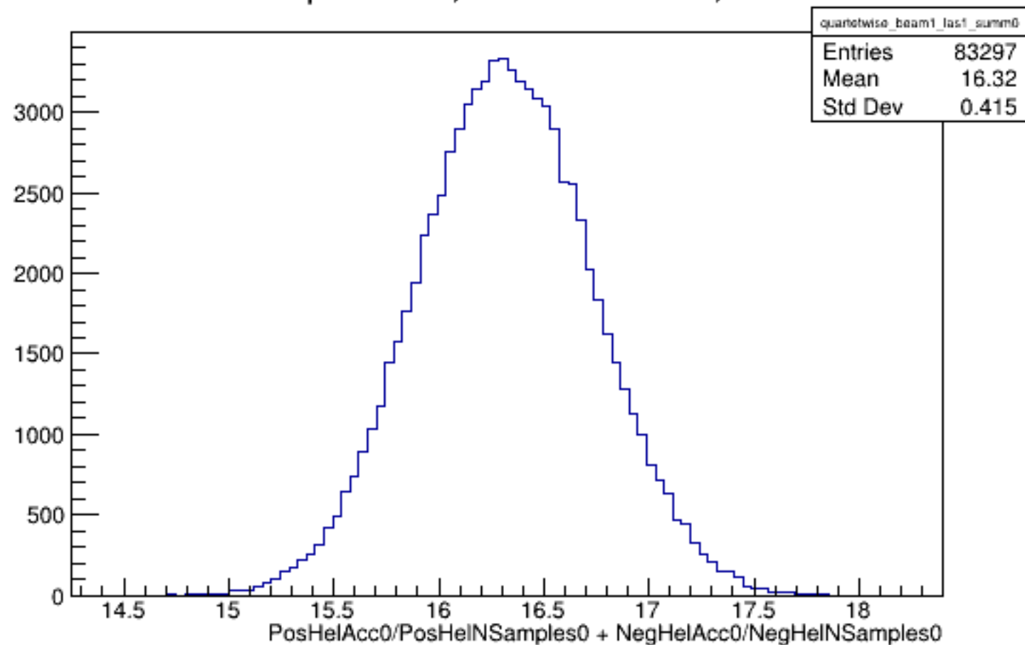
Run 4344 quartetwise, Sums0: Beam ON, Laser ON
