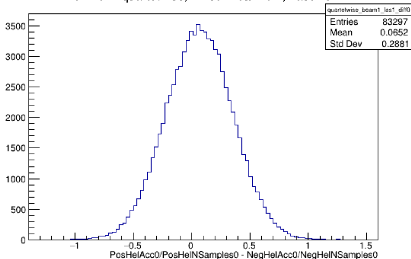
Run 4344 quartetwise, Diffs0: Beam ON, Laser ON
