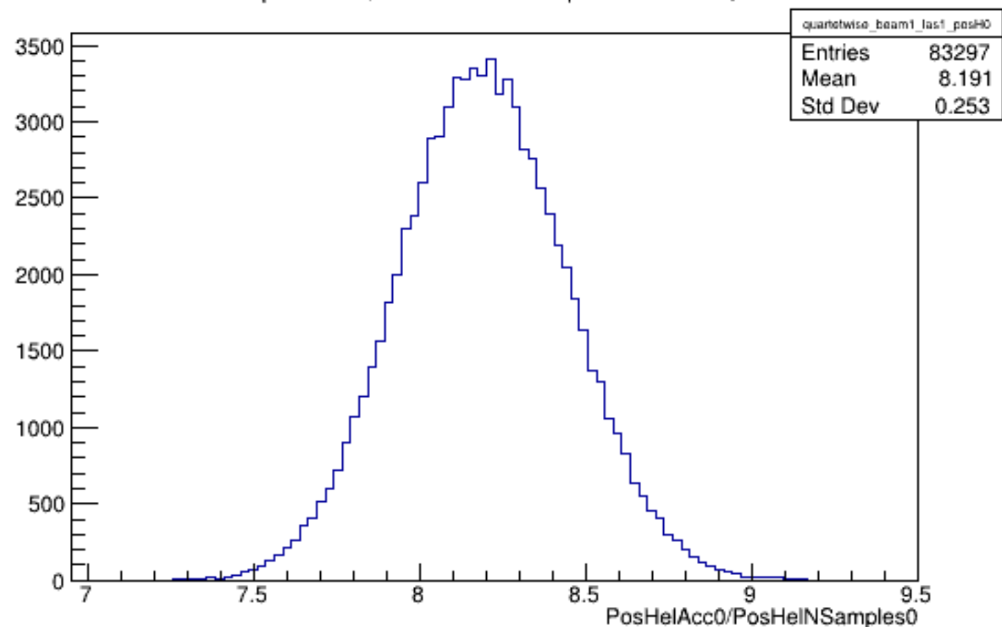
Run 4344 quartetwise, PosHelAcc0/NSamples0: Beam ON, Laser ON
