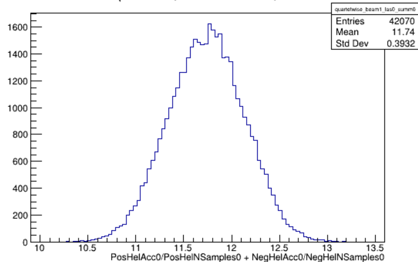
Run 4344 quartetwise, Sums0: Beam ON, Laser OFF
