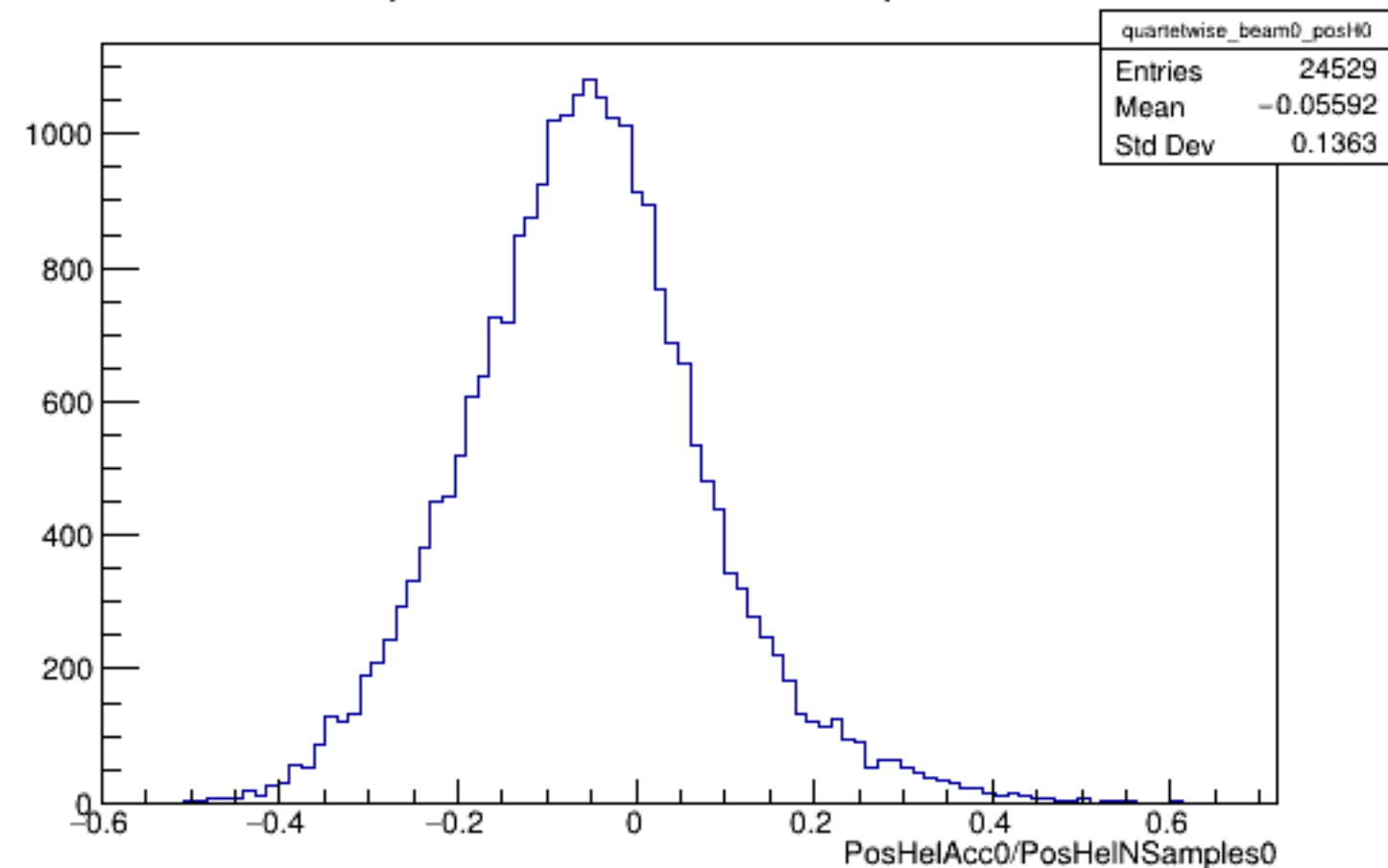
Run 4344 quartetwise, PosHelAcc0/NSamples0: Beam OFF
