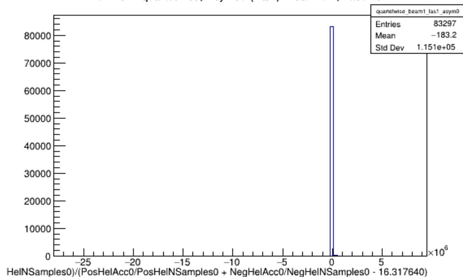
Run 4344 quartetwise, Asyms0 (Raw): Beam ON, Laser ON
