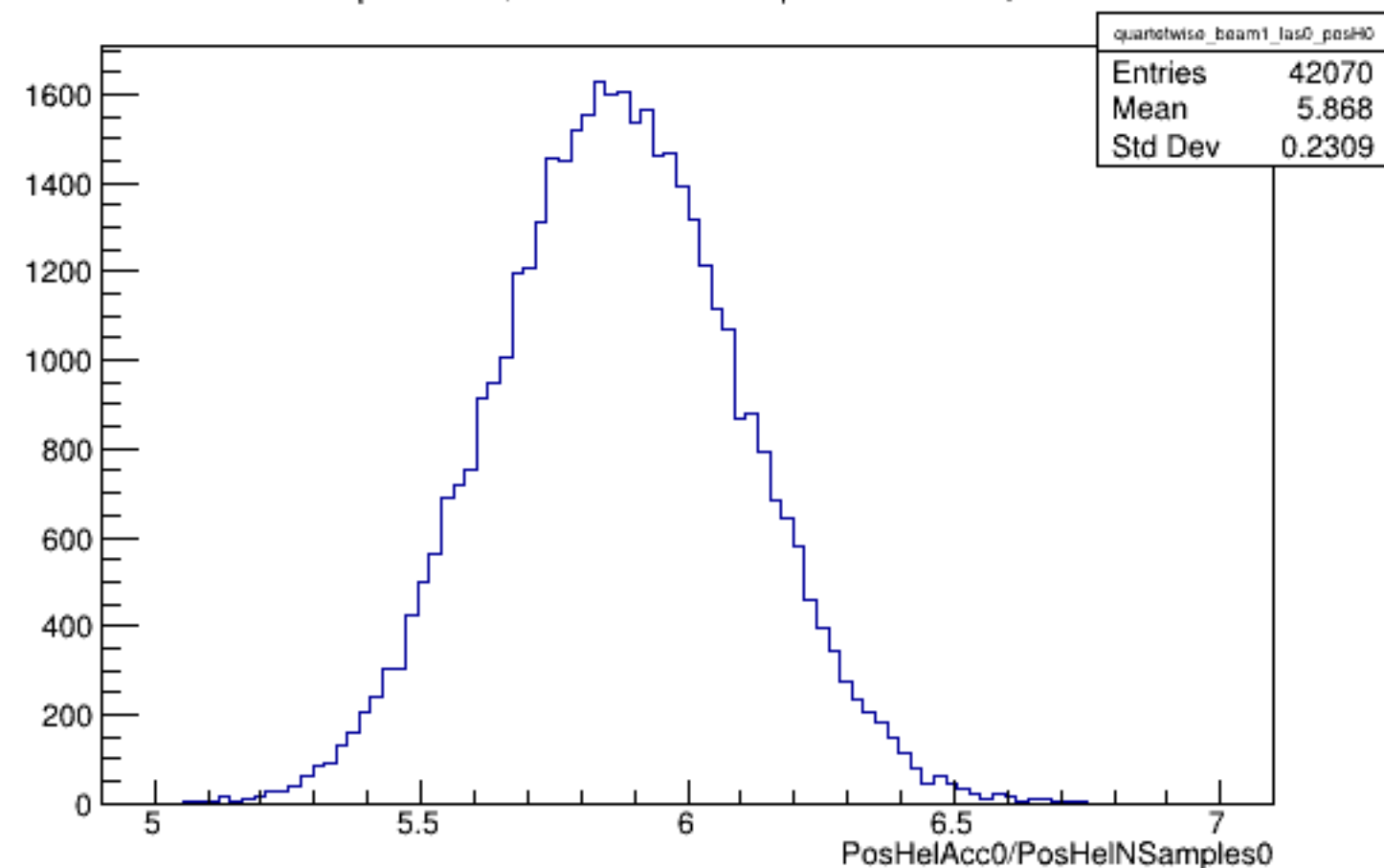
Run 4344 quartetwise, PosHelAcc0/NSamples0: Beam ON, Laser OFF
