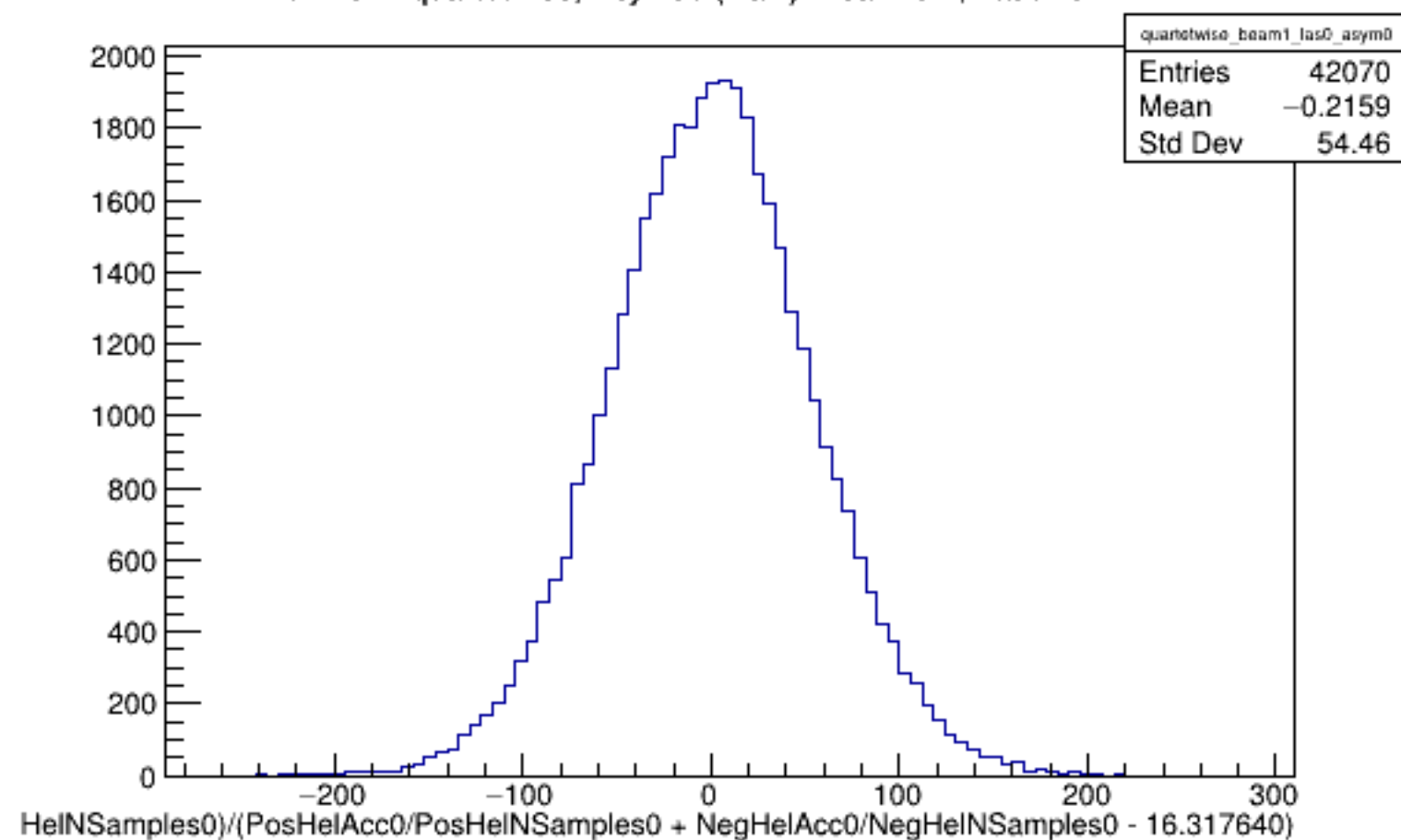
Run 4344 quartetwise, Asyms0 (Raw): Beam ON, Laser OFF
