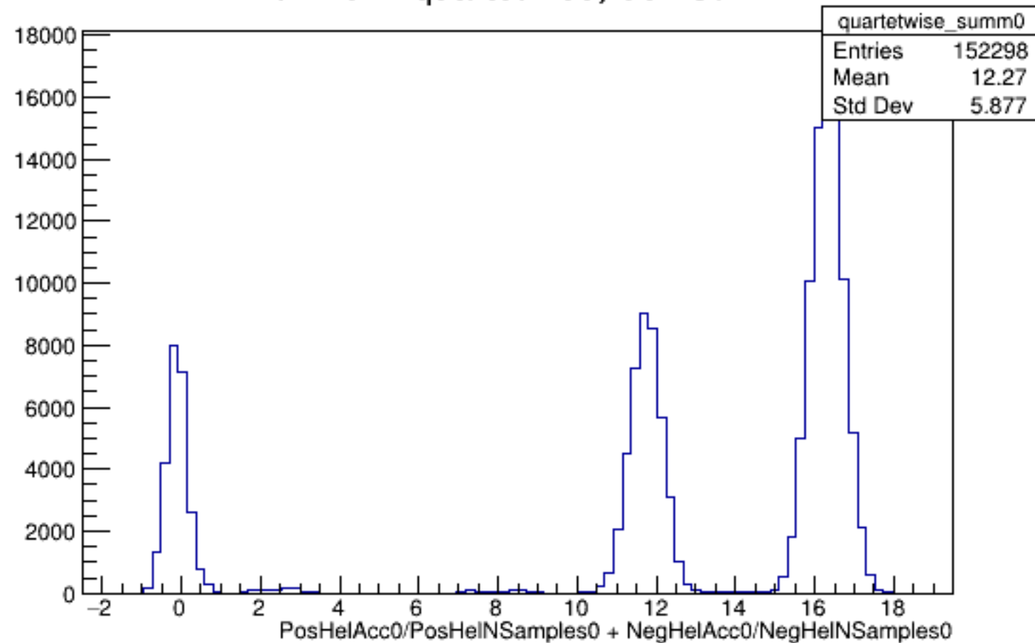
Run 4344 quartetwise, Sums0: All
