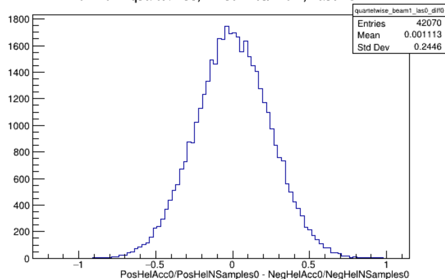
Run 4344 quartetwise, Diffs0: Beam ON, Laser OFF
