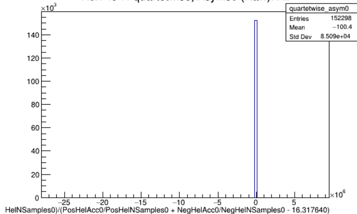
Run 4344 quartetwise, Asyms0 (Raw): All
