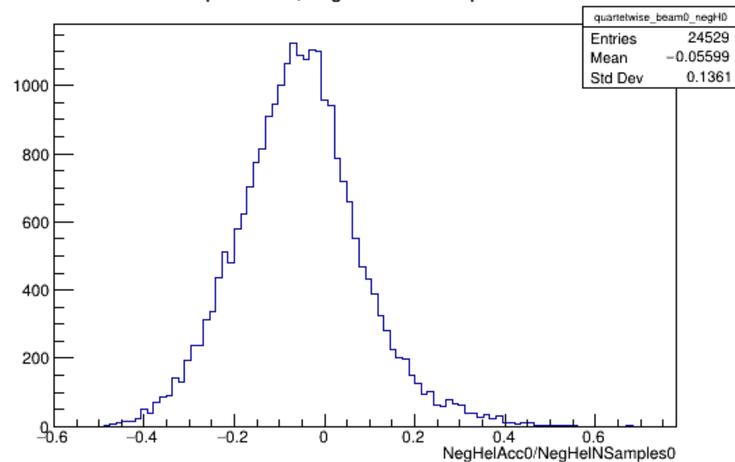
Run 4344 quartetwise, NegHelAcc0/NSamples0: Beam OFF
