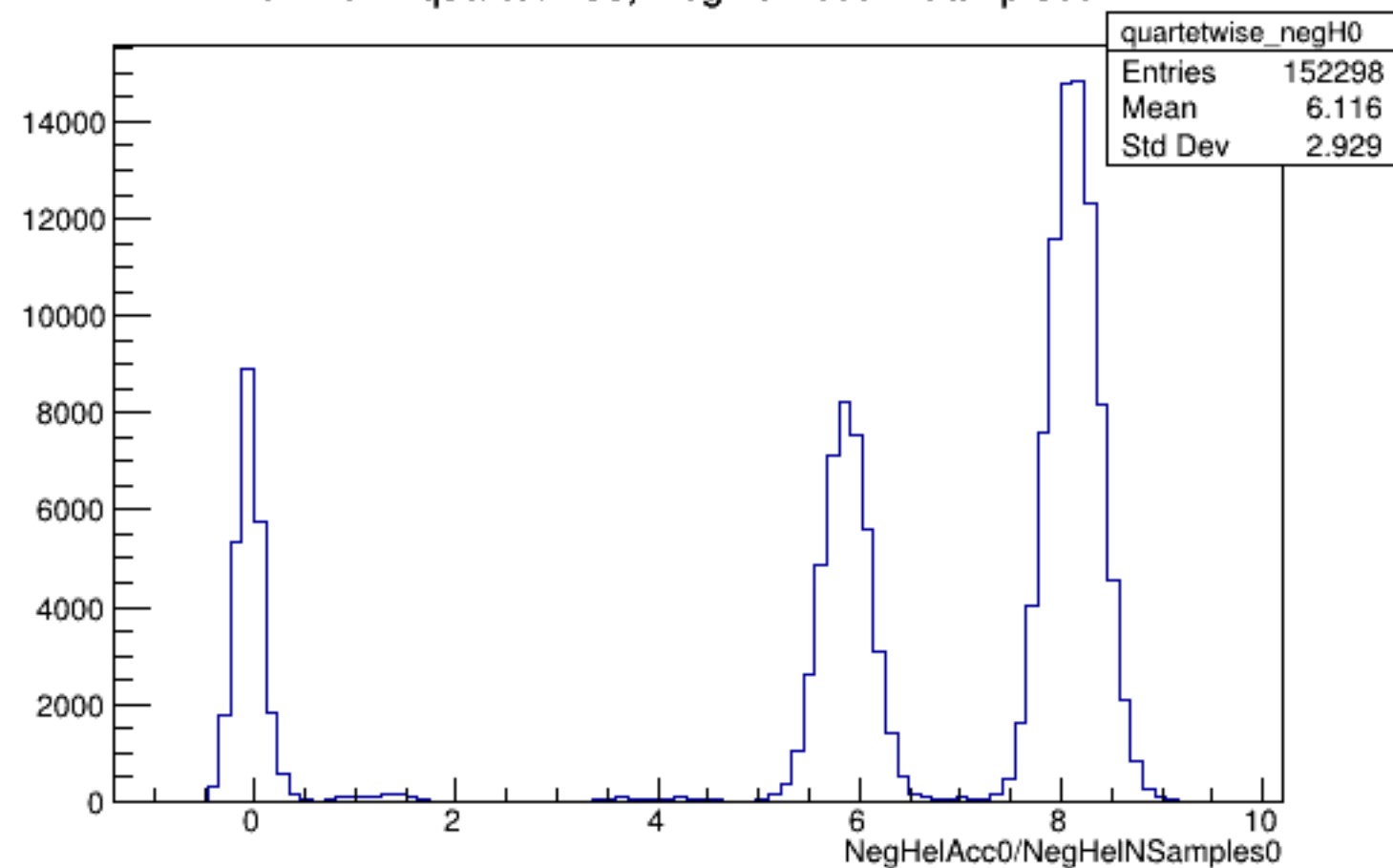
Run 4344 quartetwise, NegHelAcc0/NSamples0: All
