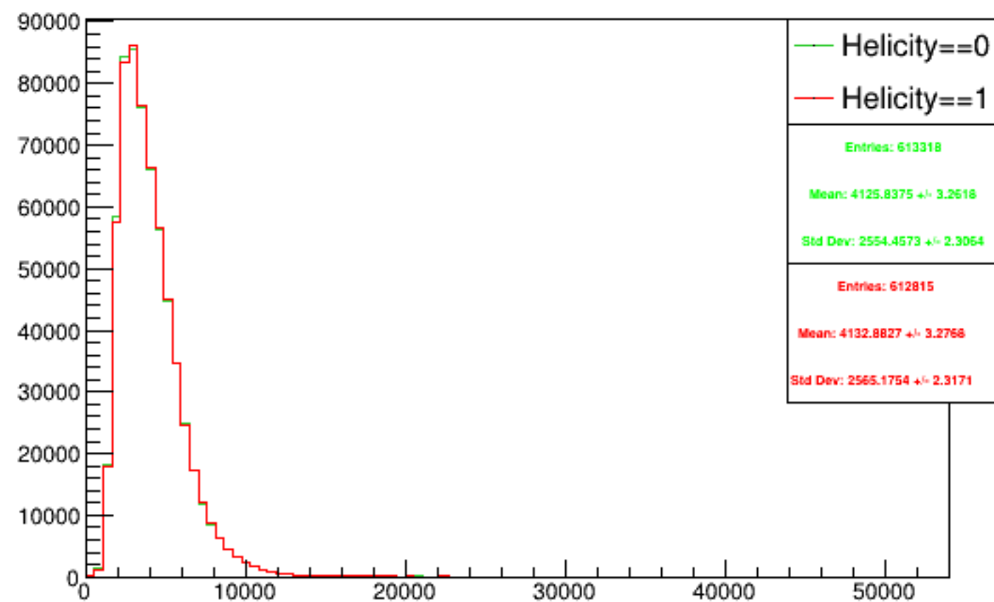
Run 4344 triggerwise, sums: Beam ON, Laser OFF
