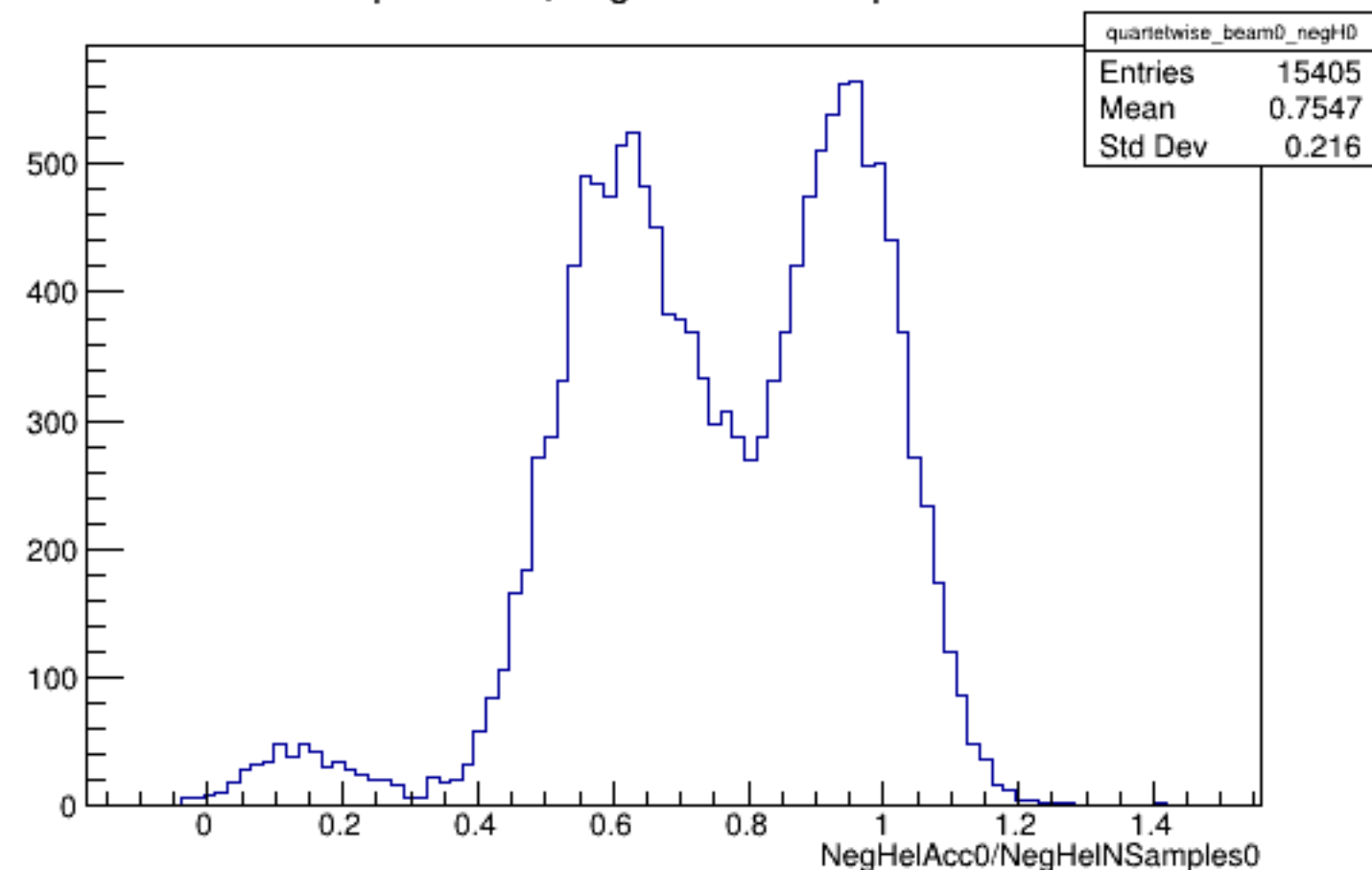
Run 4352 quartetwise, NegHelAcc0/NSamples0: Beam OFF
