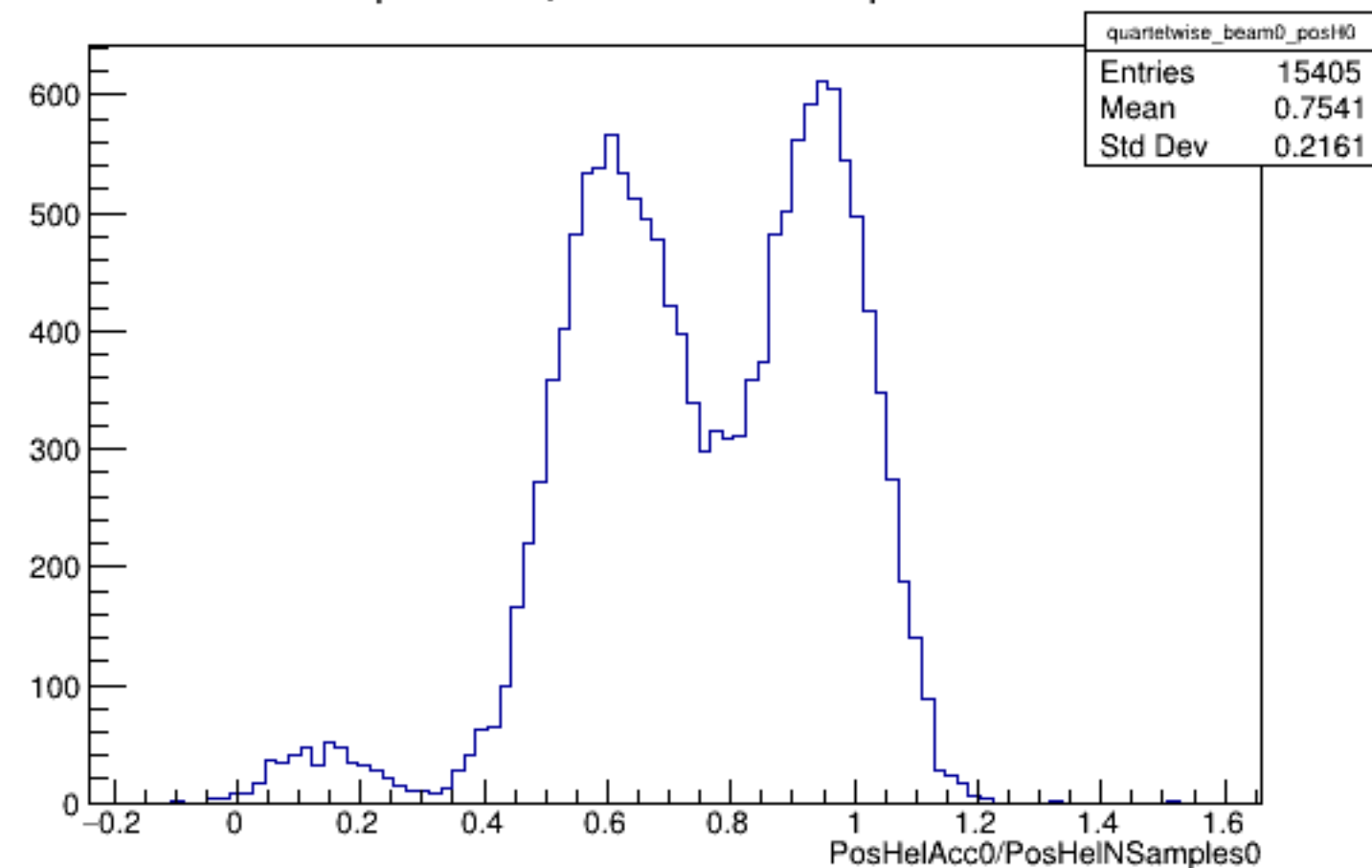
Run 4352 quartetwise, PosHelAcc0/NSamples0: Beam OFF
