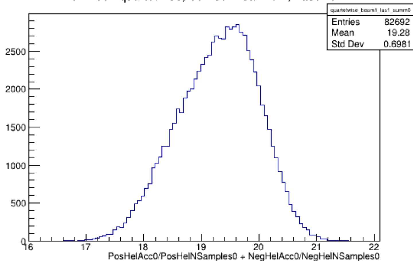
Run 4352 quartetwise, Sums0: Beam ON, Laser ON
