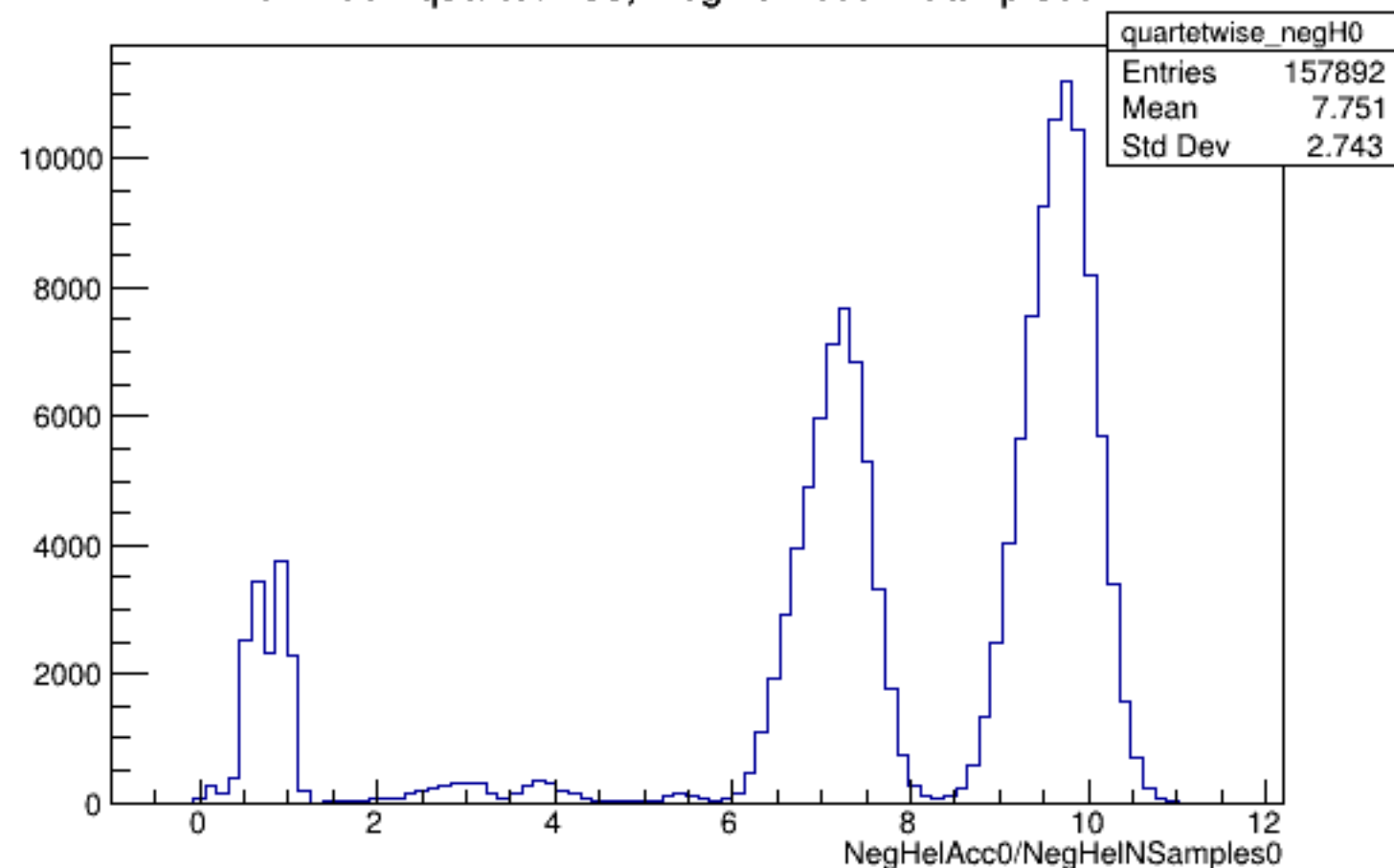
Run 4352 quartetwise, NegHelAcc0/NSamples0: All
