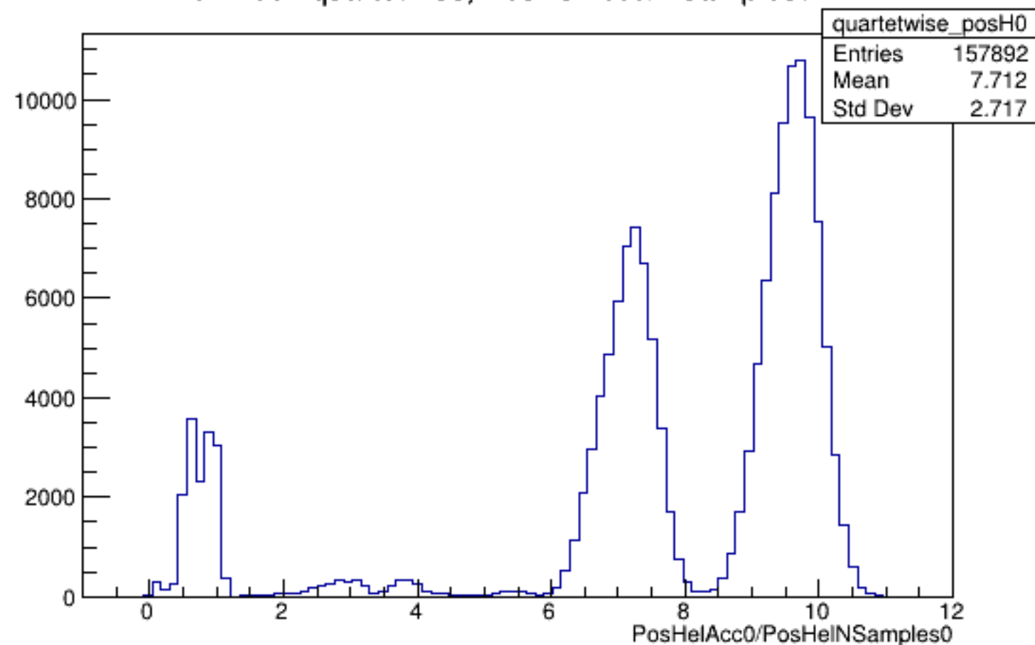
Run 4352 quartetwise, PosHelAcc0/NSamples0: All
