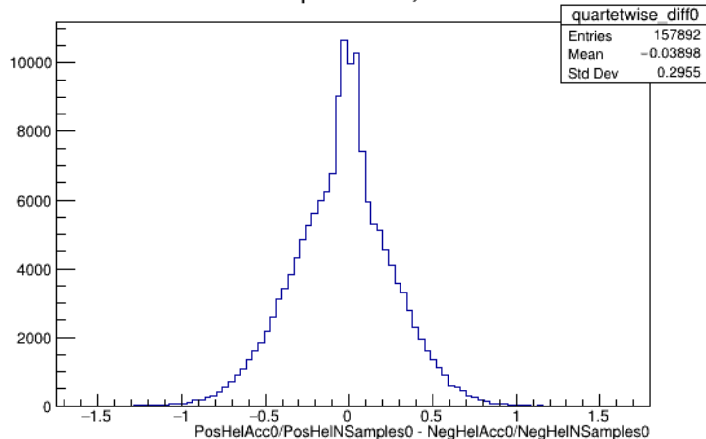
Run 4352 quartetwise, Diffs0: All
