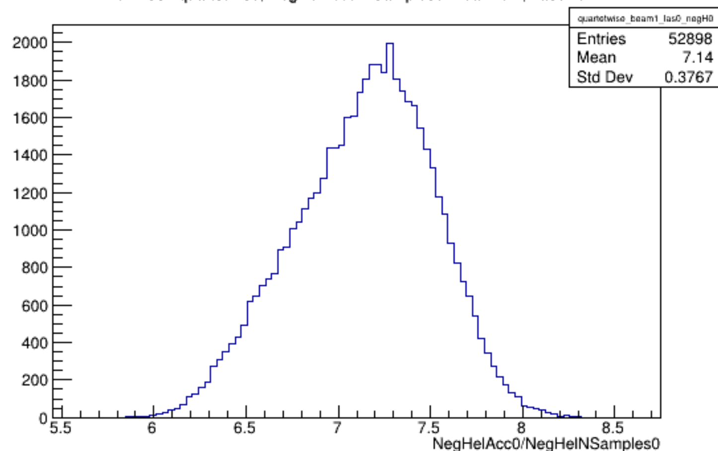
Run 4352 quartetwise, NegHelAcc0/NSamples0: Beam ON, Laser OFF
