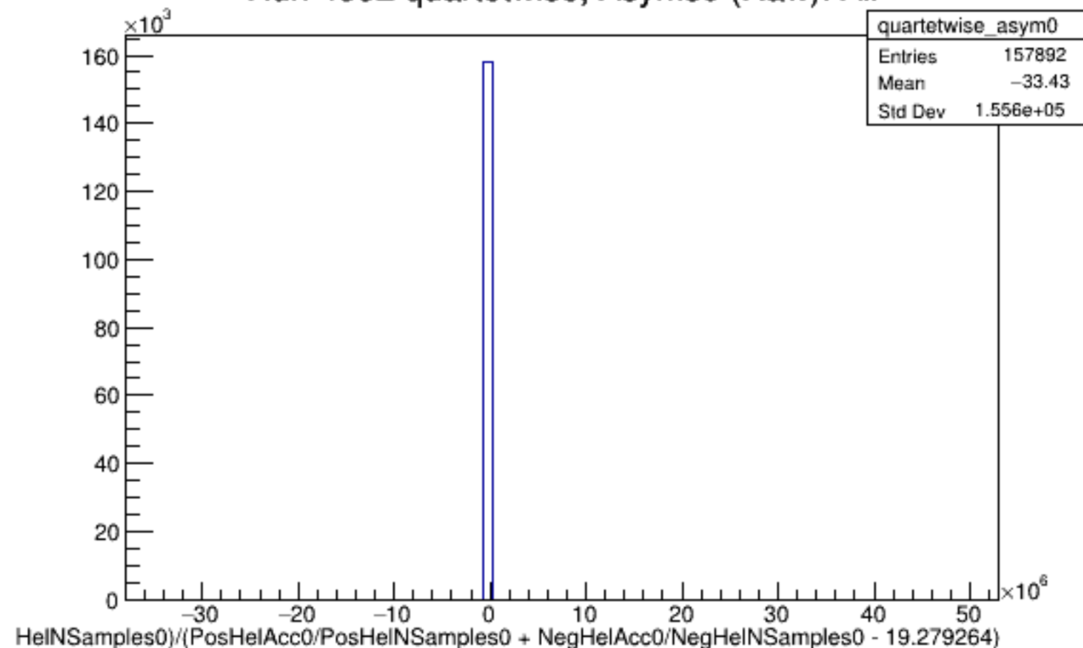
Run 4352 quartetwise, Asyms0 (Raw): All
