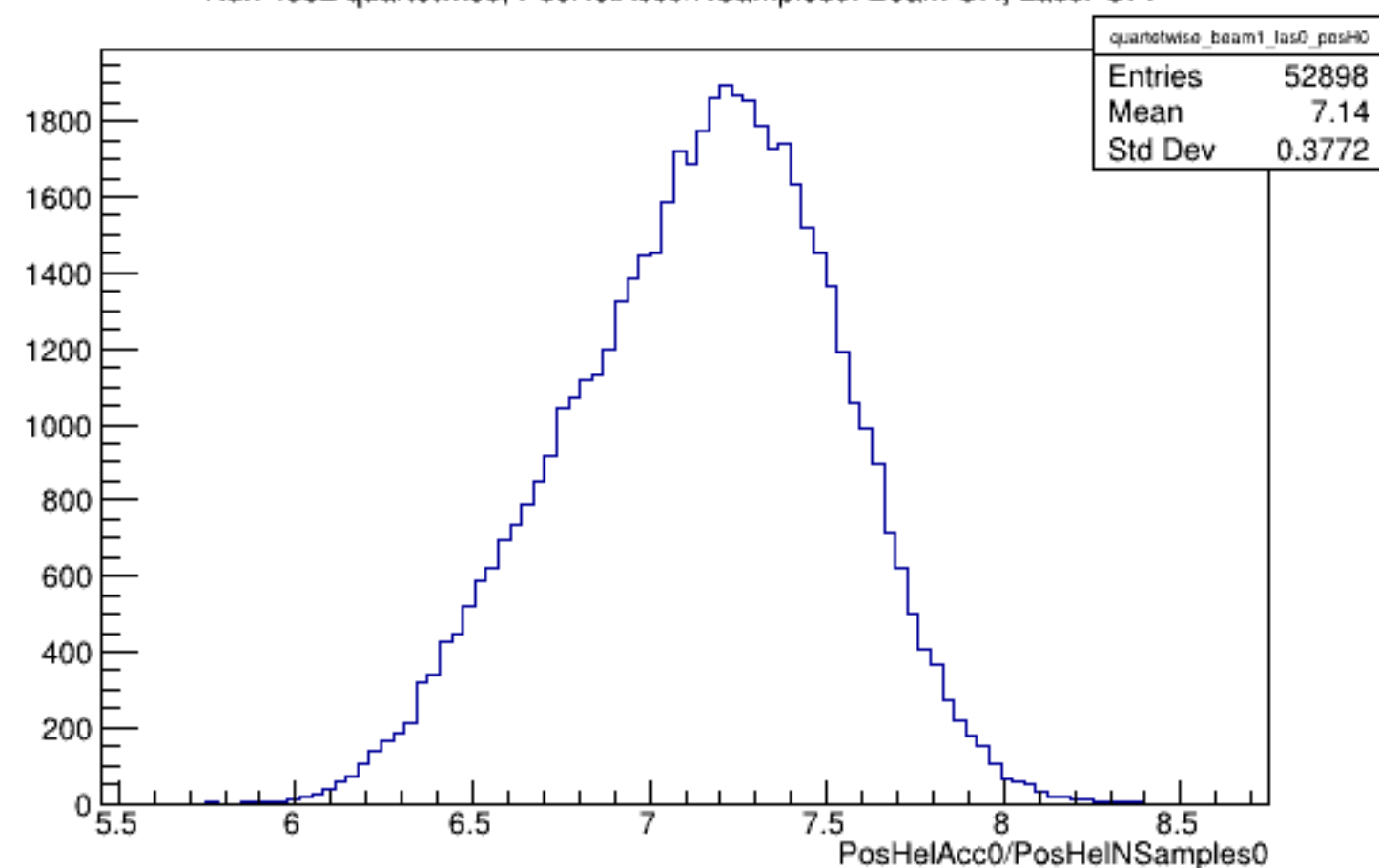
Run 4352 quartetwise, PosHelAcc0/NSamples0: Beam ON, Laser OFF
