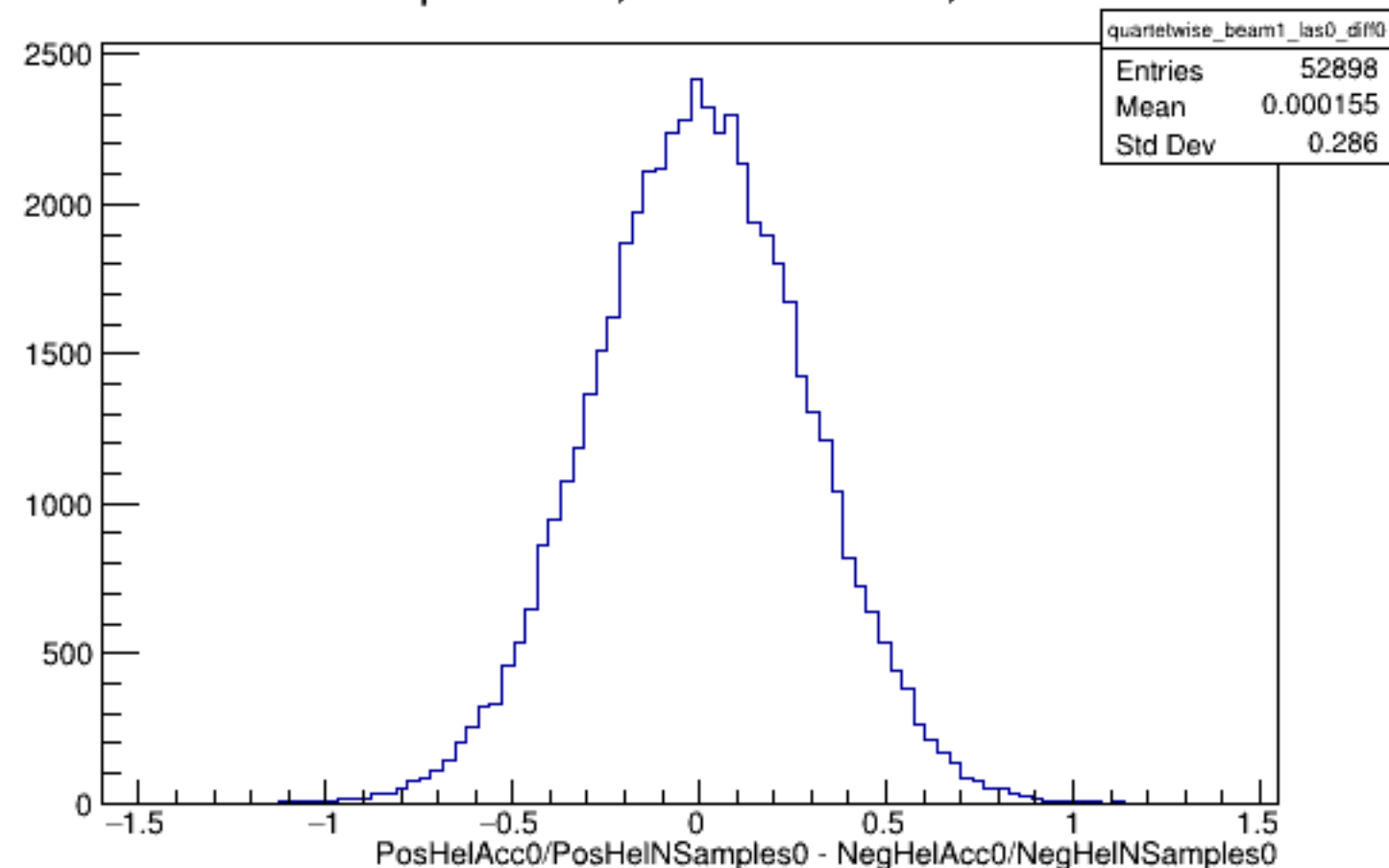
Run 4352 quartetwise, Diffs0: Beam ON, Laser OFF
