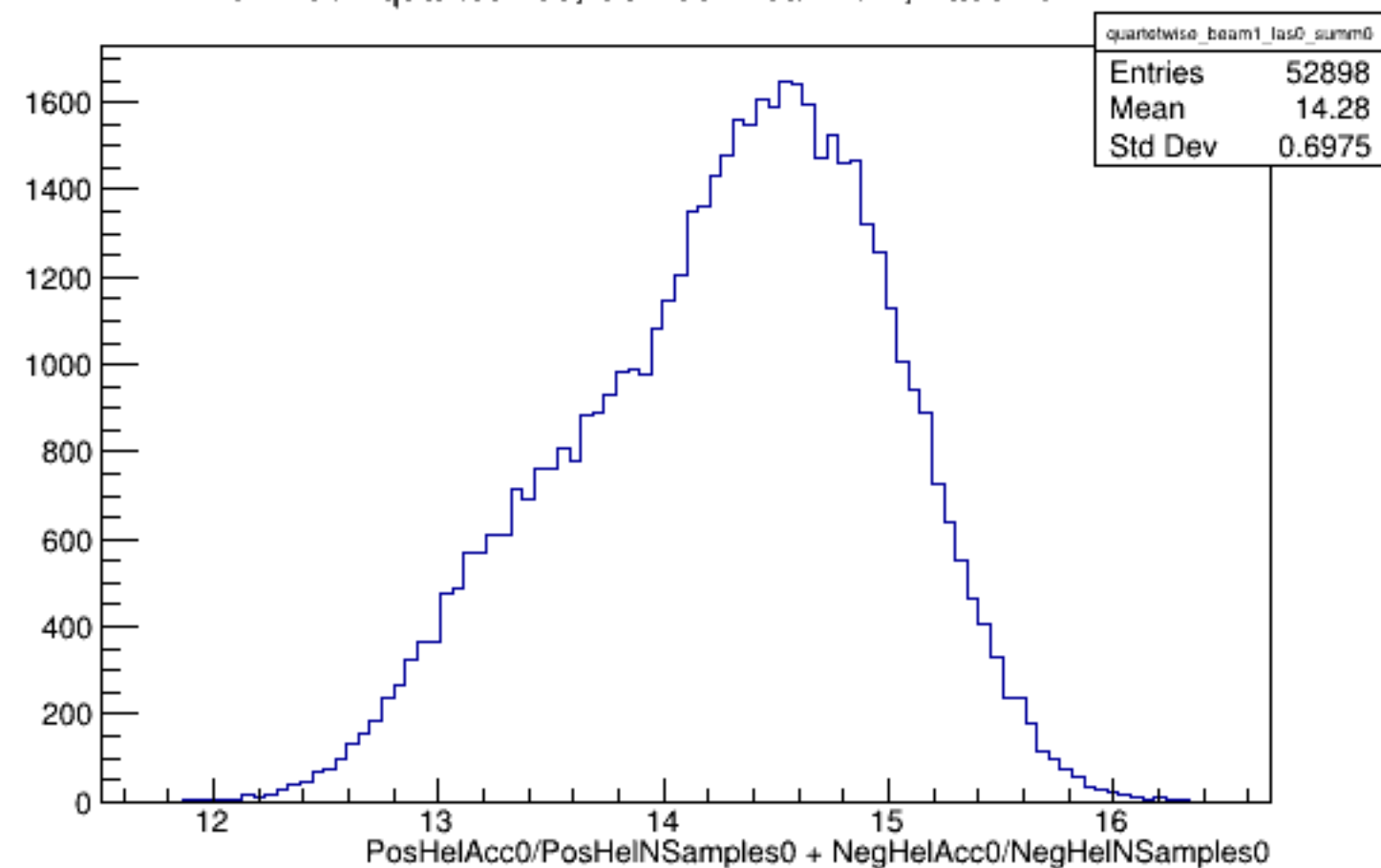
Run 4352 quartetwise, Sums0: Beam ON, Laser OFF
