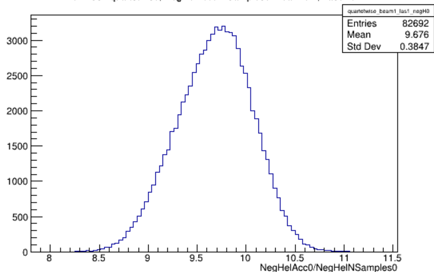
Run 4352 quartetwise, NegHelAcc0/NSamples0: Beam ON, Laser ON
