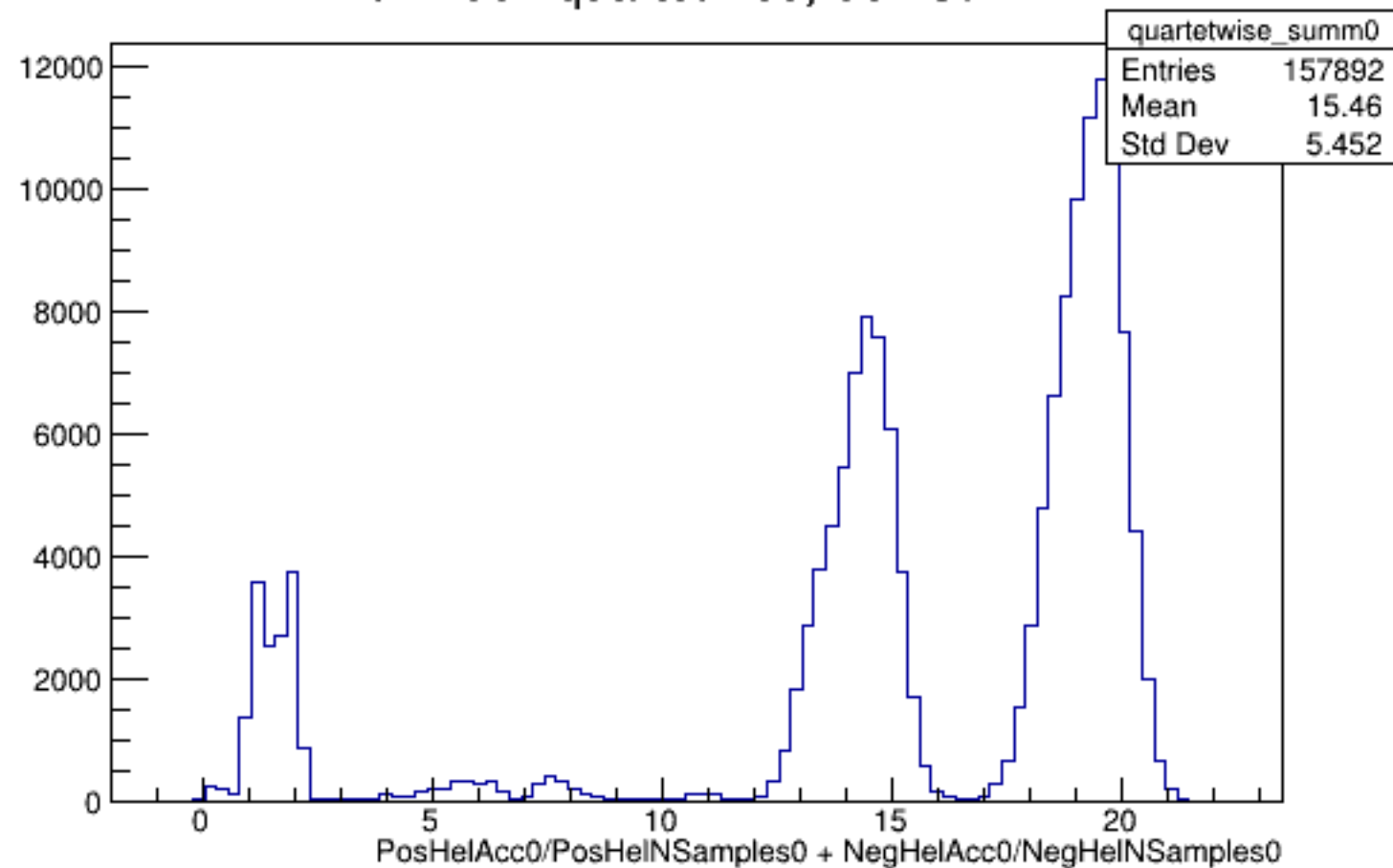
Run 4352 quartetwise, Sums0: All
