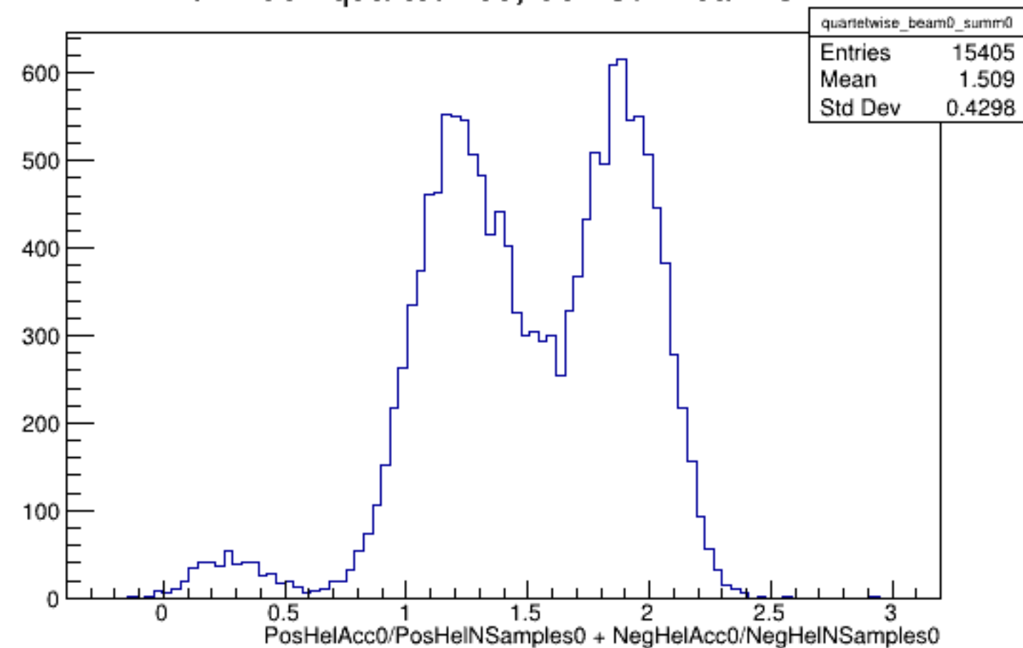
Run 4352 quartetwise, Sums0: Beam OFF
