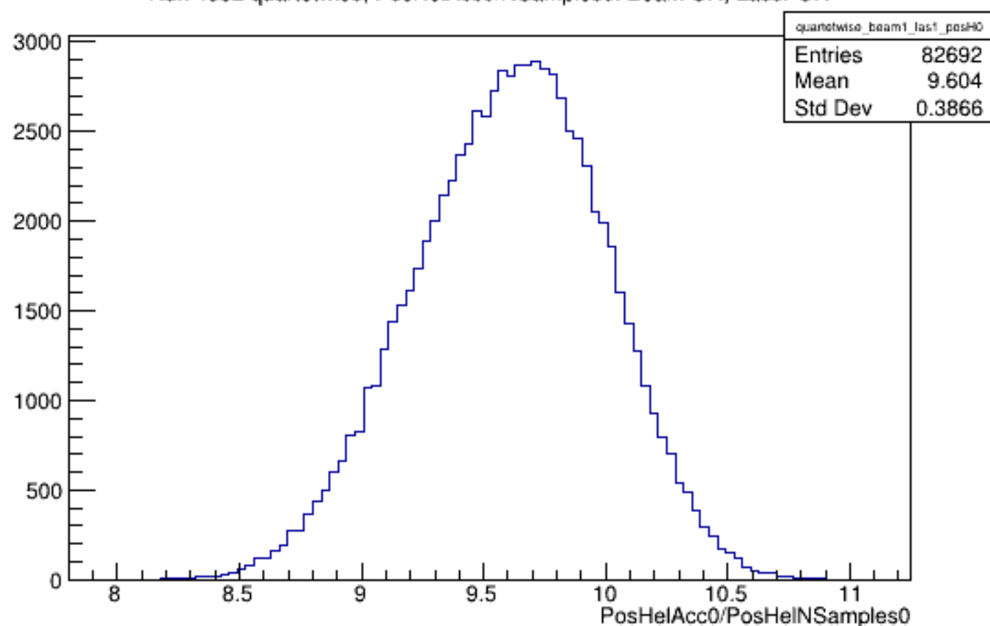
Run 4352 quartetwise, PosHelAcc0/NSamples0: Beam ON, Laser ON
