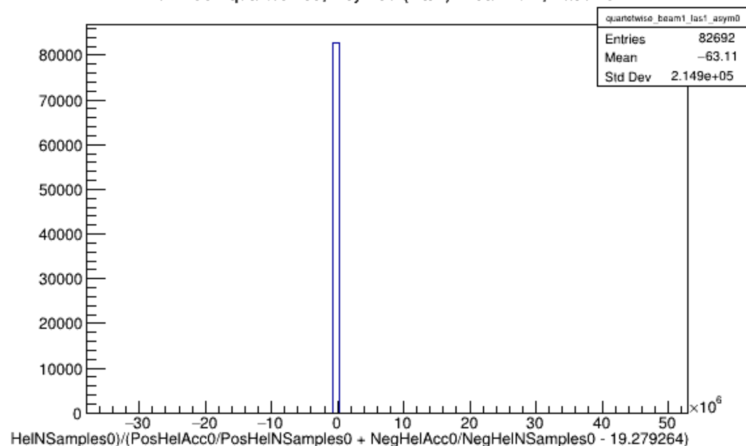
Run 4352 quartetwise, Asyms0 (Raw): Beam ON, Laser ON
