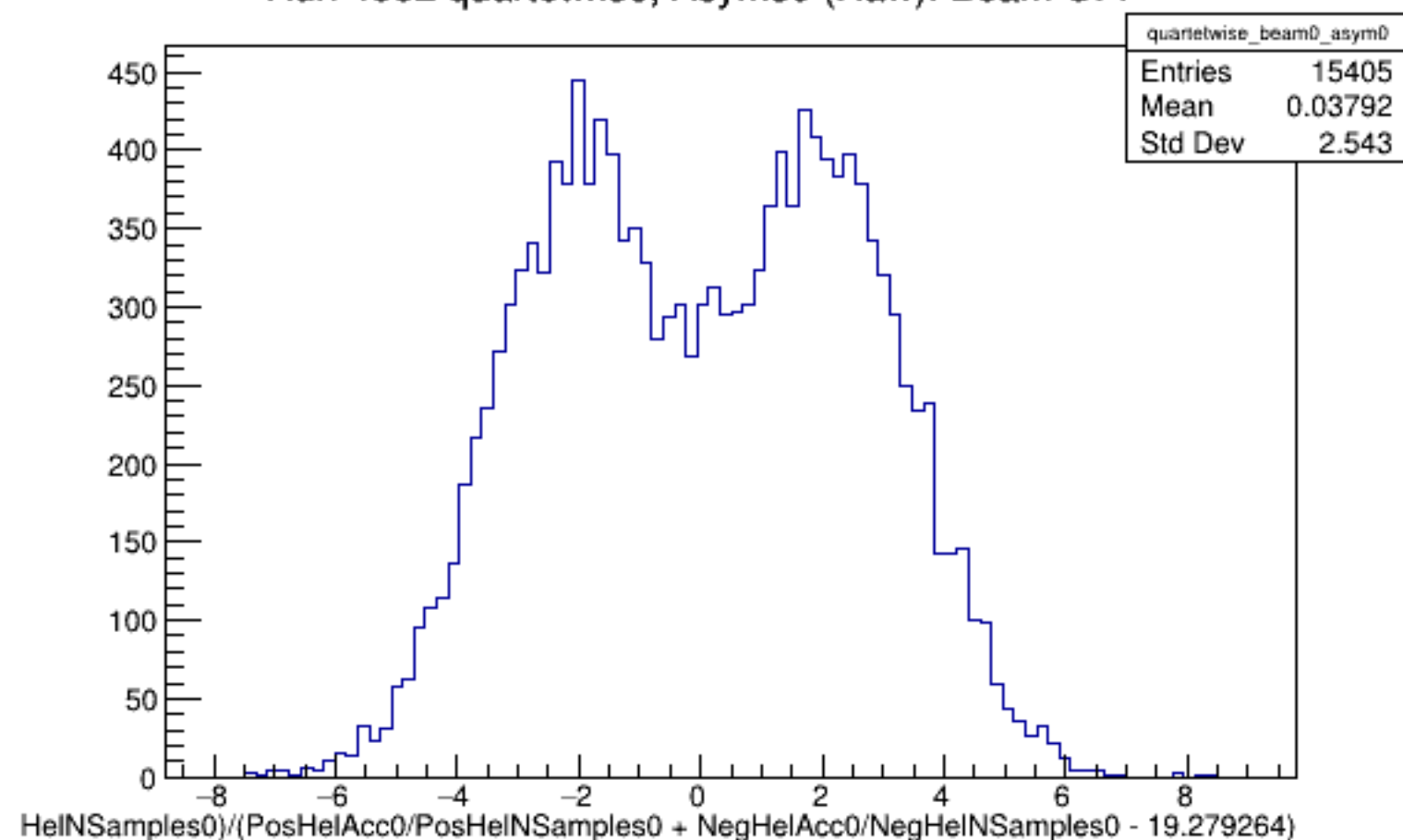
Run 4352 quartetwise, Asyms0 (Raw): Beam OFF
