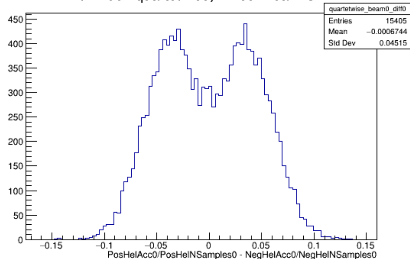
Run 4352 quartetwise, Diffs0: Beam OFF
