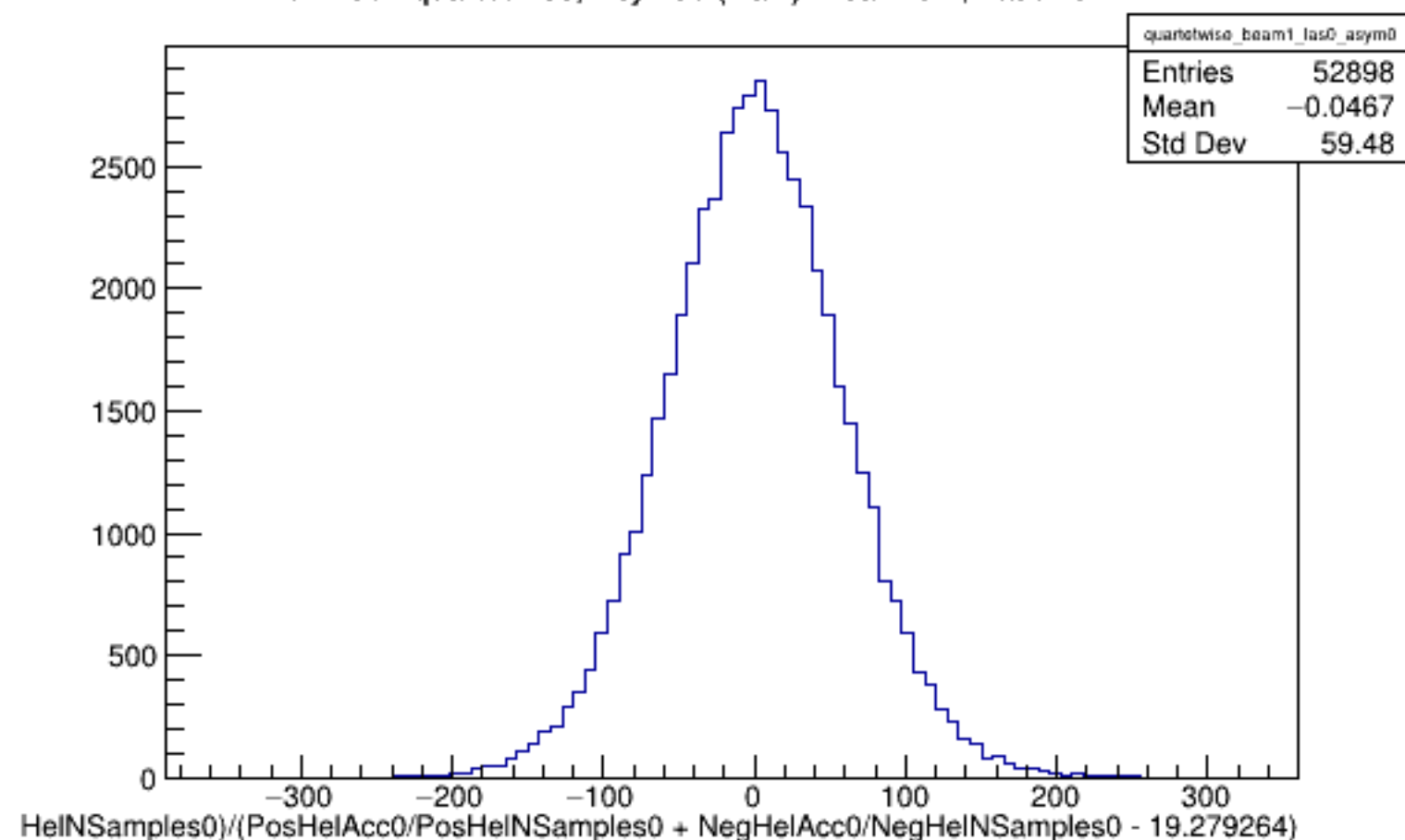
Run 4352 quartetwise, Asyms0 (Raw): Beam ON, Laser OFF
