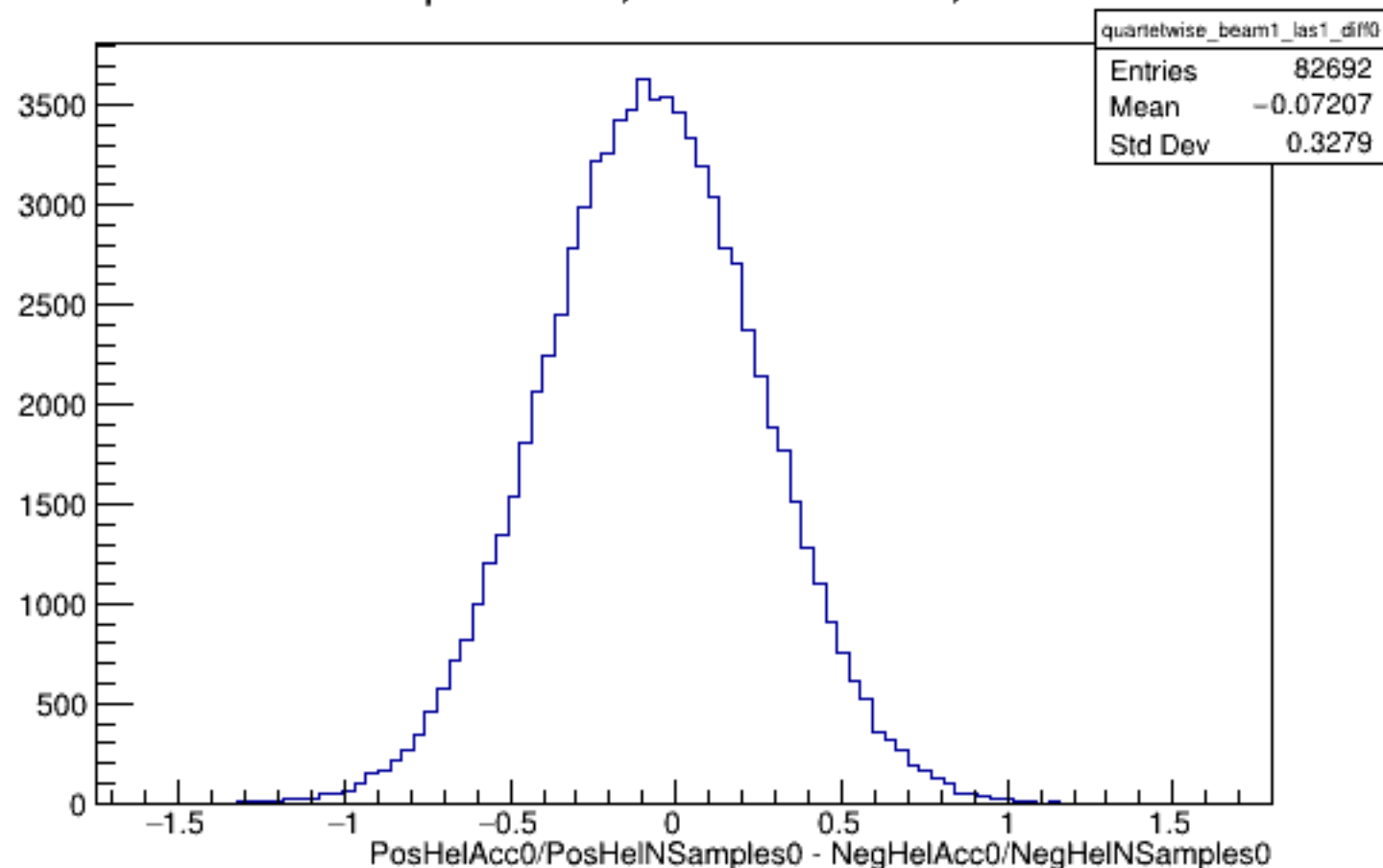
Run 4352 quartetwise, Diffs0: Beam ON, Laser ON
