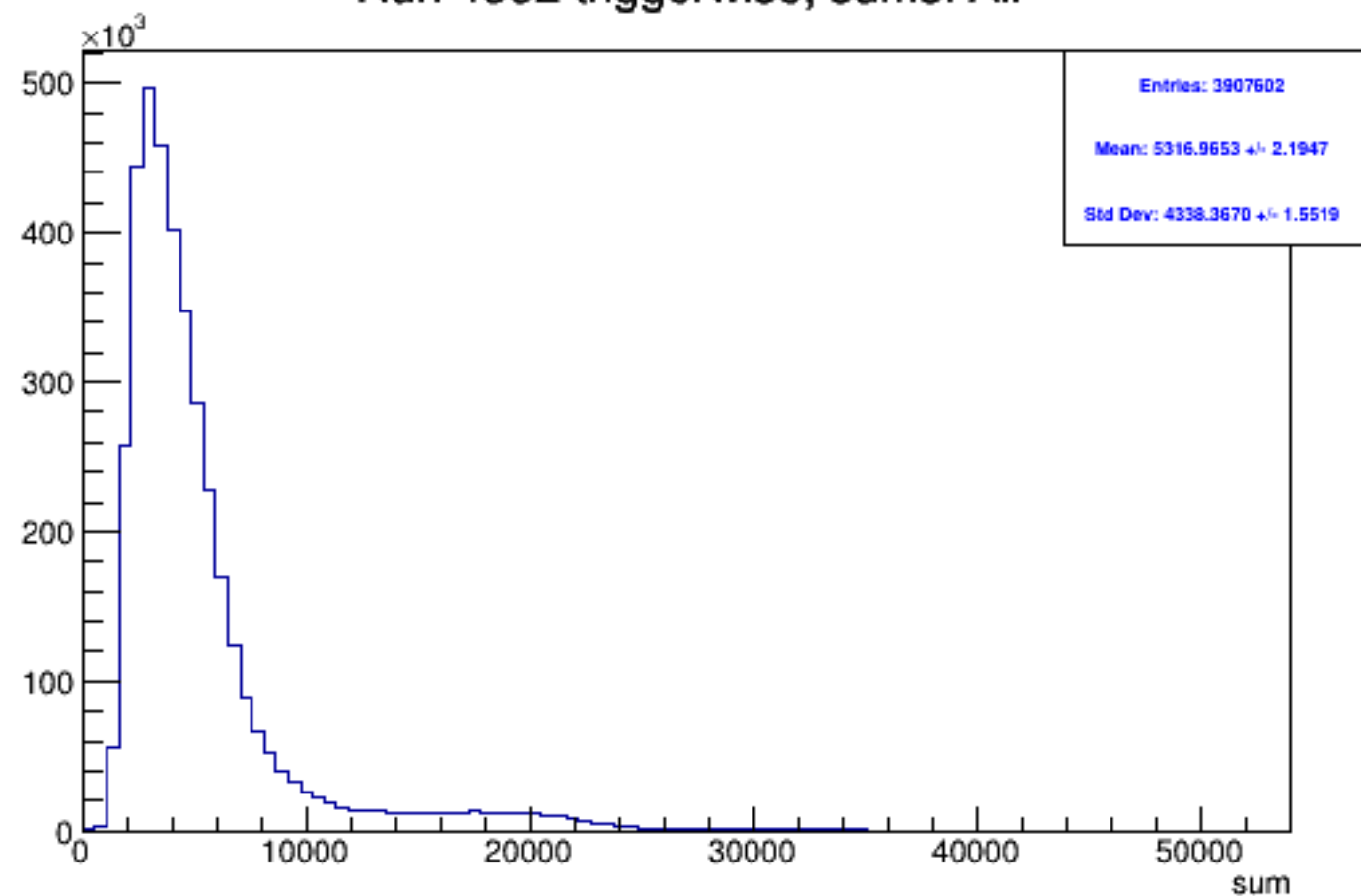
Run 4352 triggerwise, sums: All
