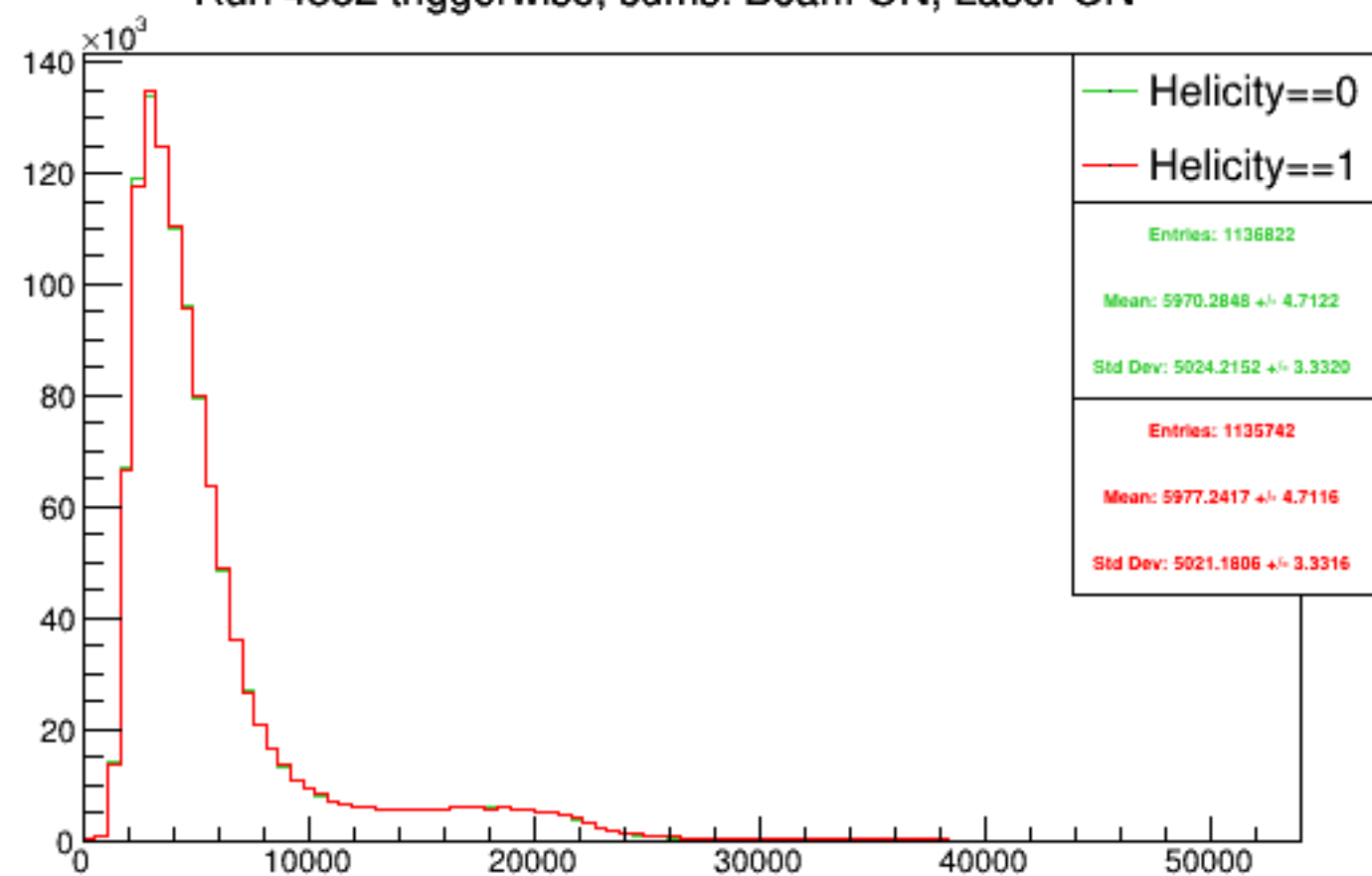
Run 4352 triggerwise, sums: Beam ON, Laser ON
