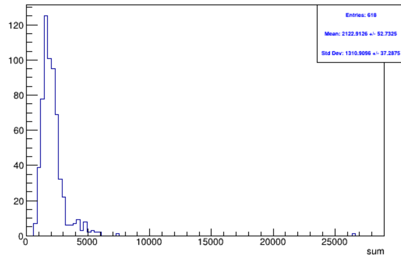
Run 4352 triggerwise, sums: Beam OFF
