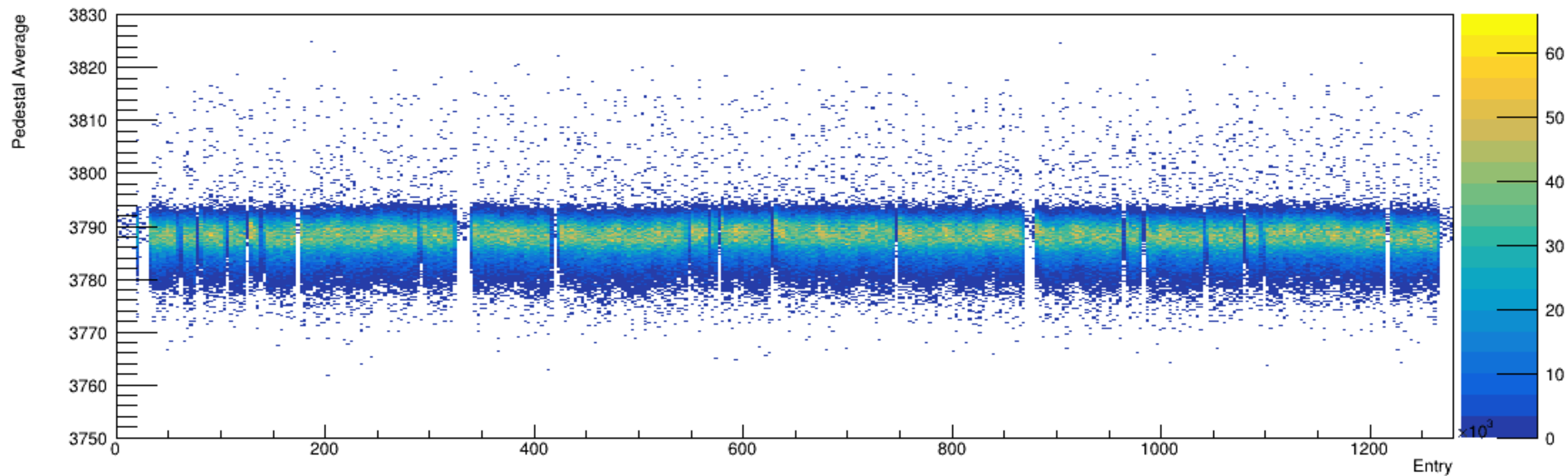
Run 4353, snapshots: Pedestal vs. Time
