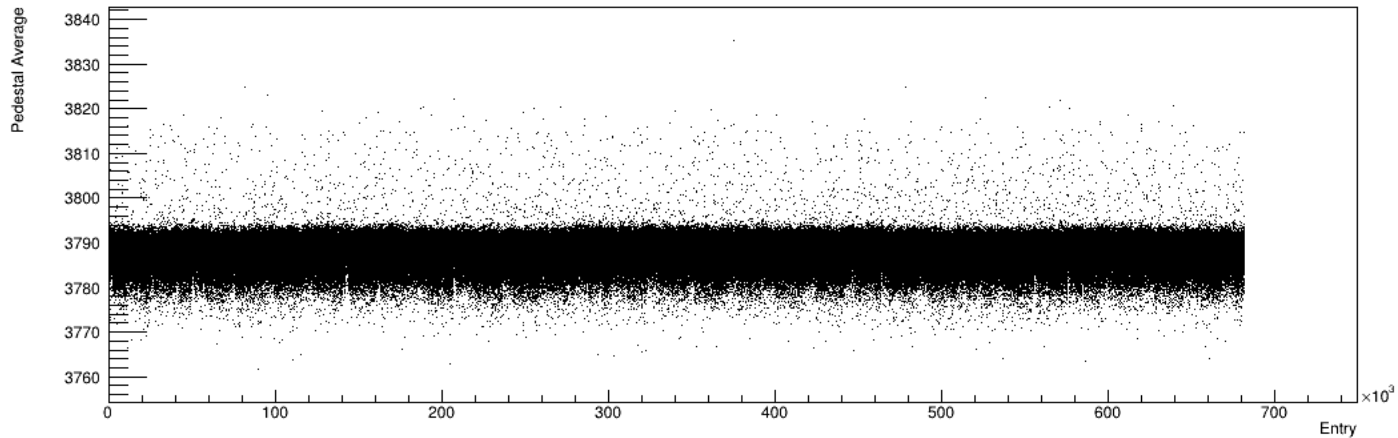
Run 4353, snapshots: Pedestal vs. Time
