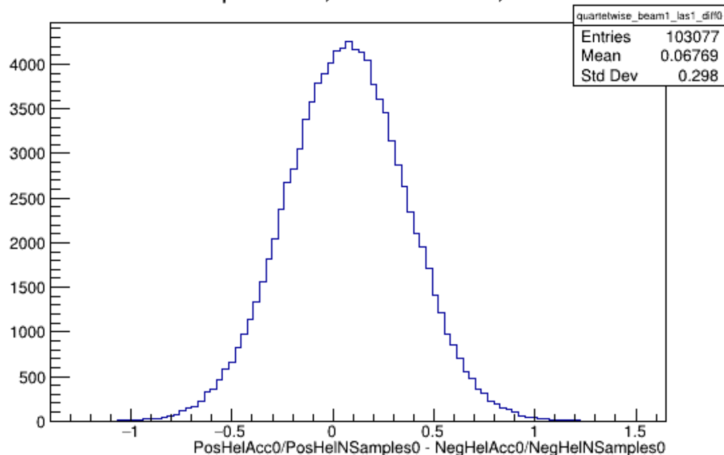
Run 4356 quartetwise, Diffs0: Beam ON, Laser ON
