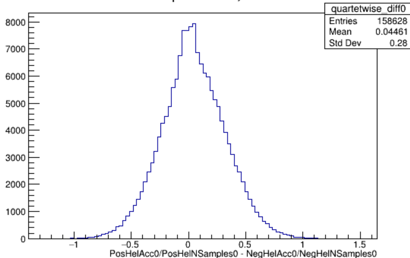
Run 4356 quartetwise, Diffs0: All
