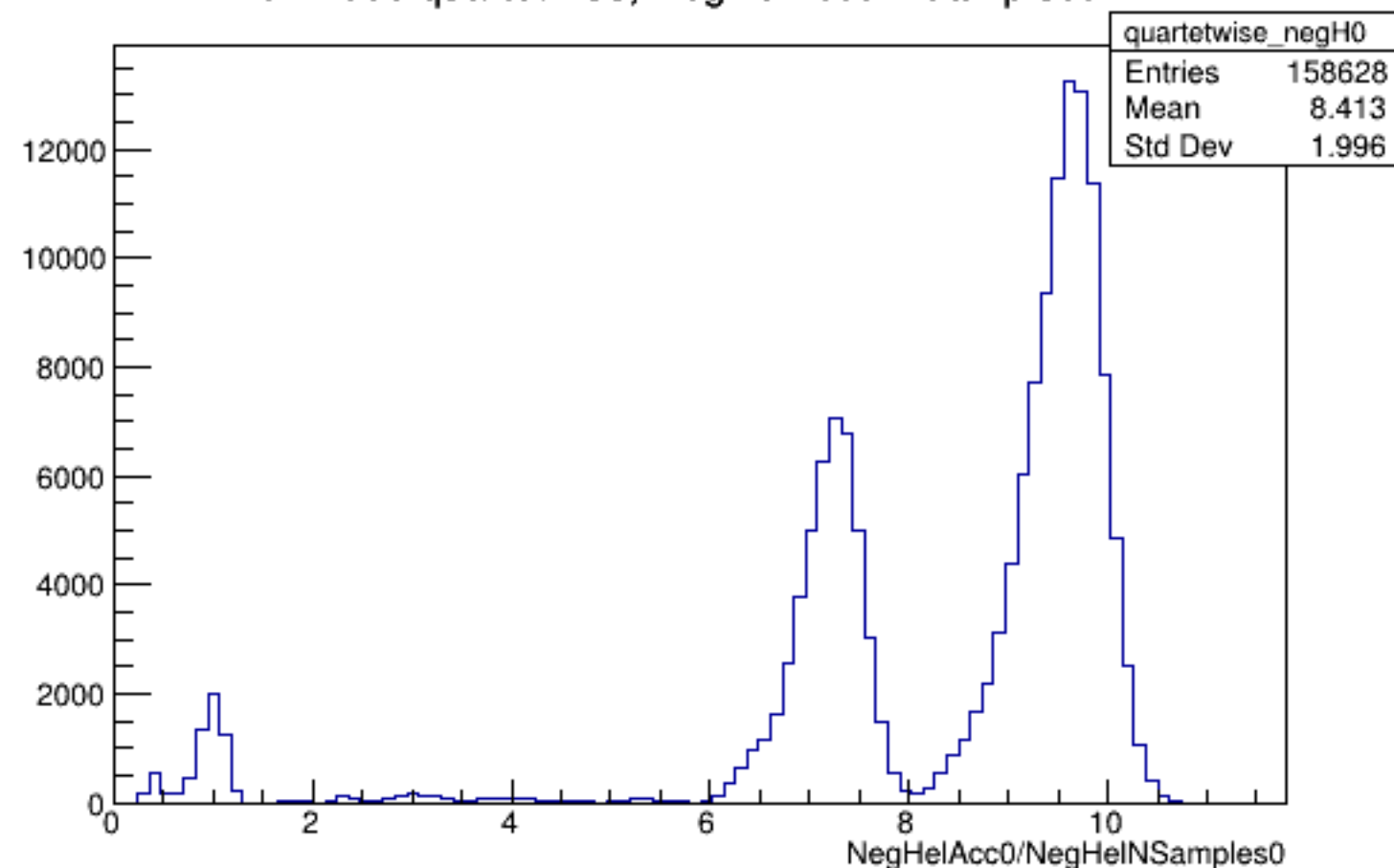
Run 4356 quartetwise, NegHelAcc0/NSamples0: All
