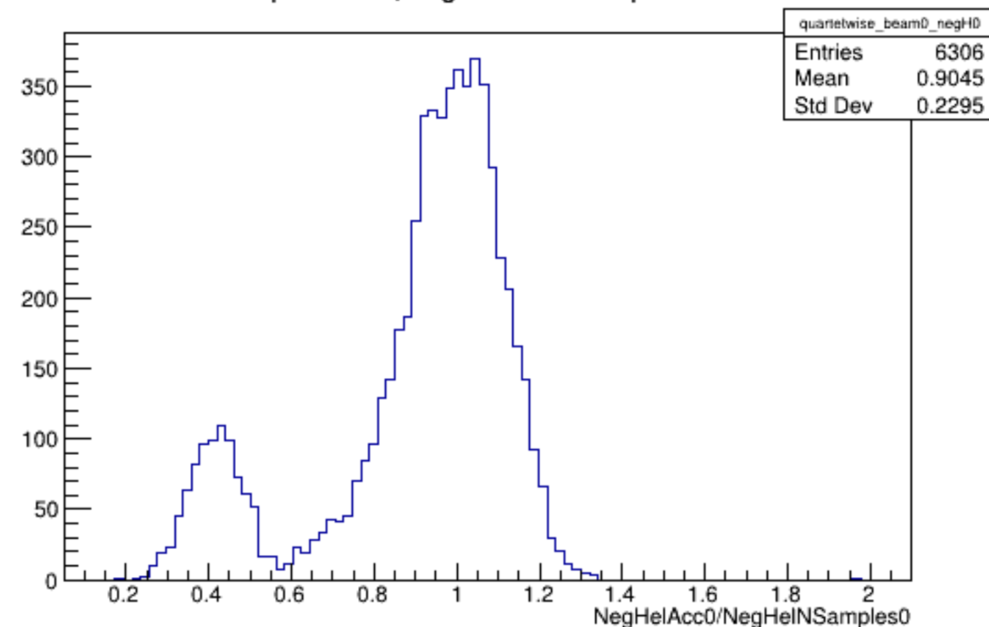
Run 4356 quartetwise, NegHelAcc0/NSamples0: Beam OFF
