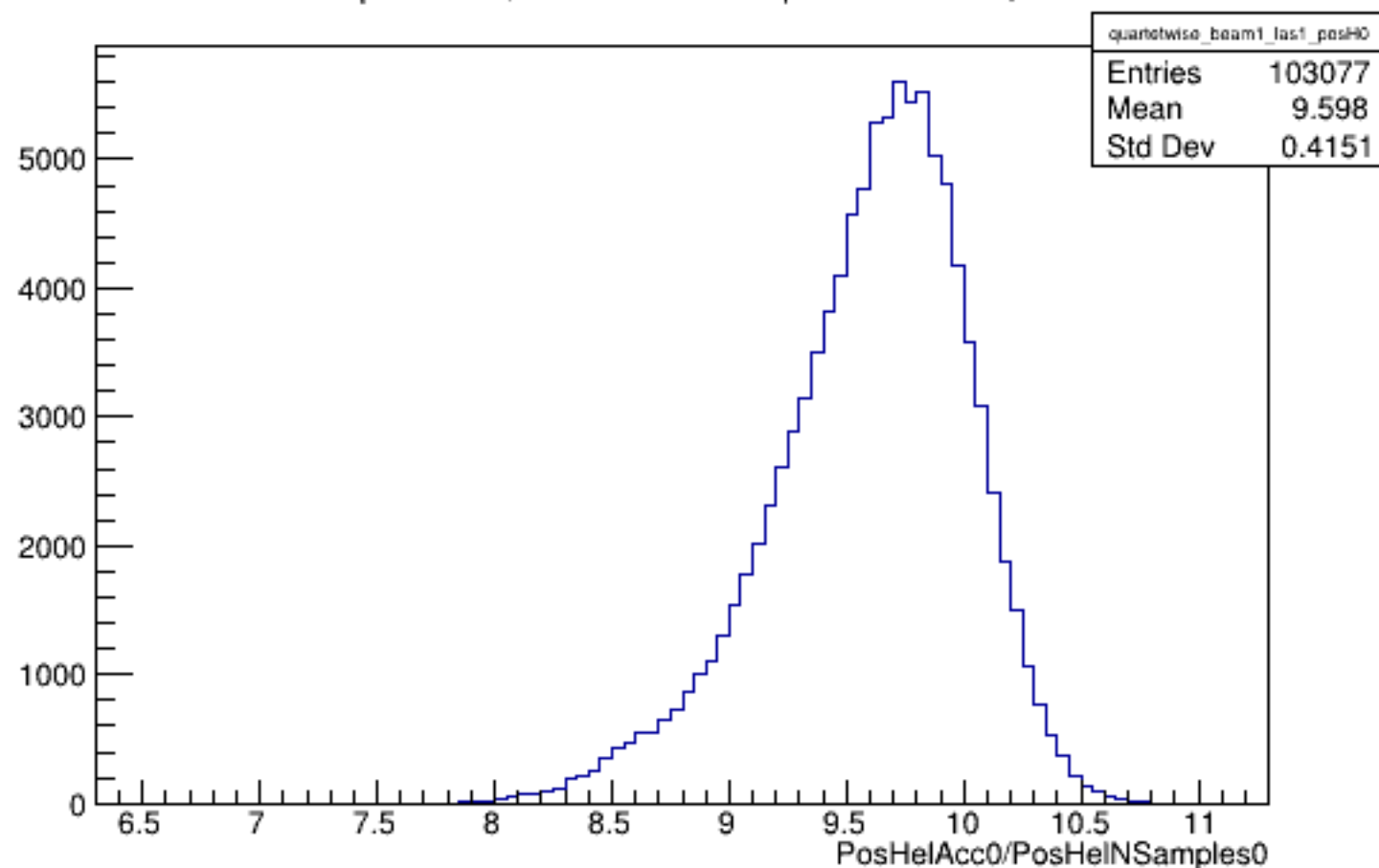
Run 4356 quartetwise, PosHelAcc0/NSamples0: Beam ON, Laser ON
