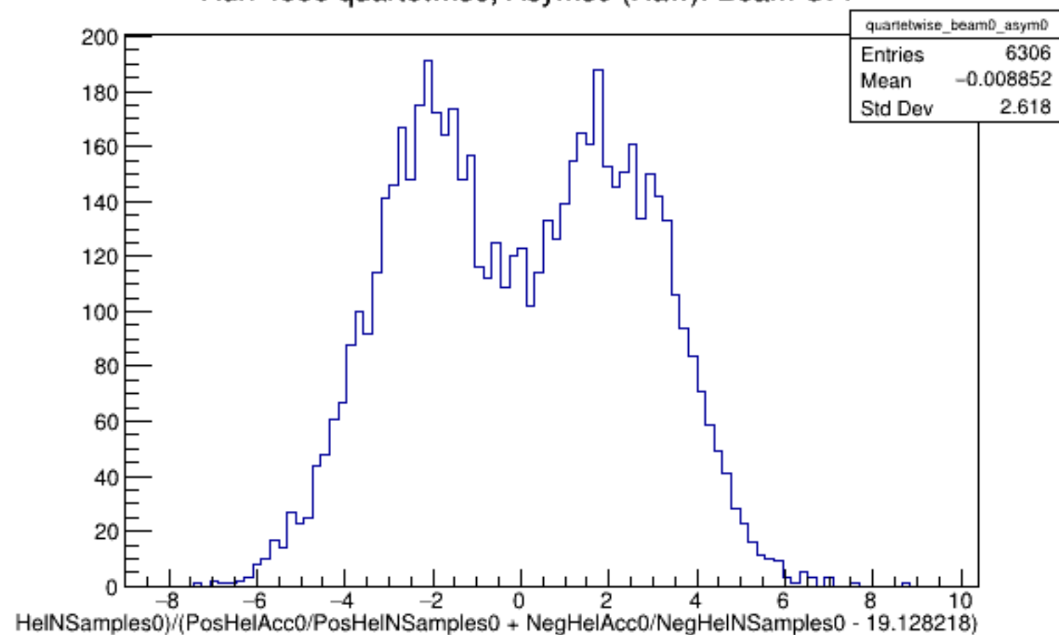
Run 4356 quartetwise, Asyms0 (Raw): Beam OFF
