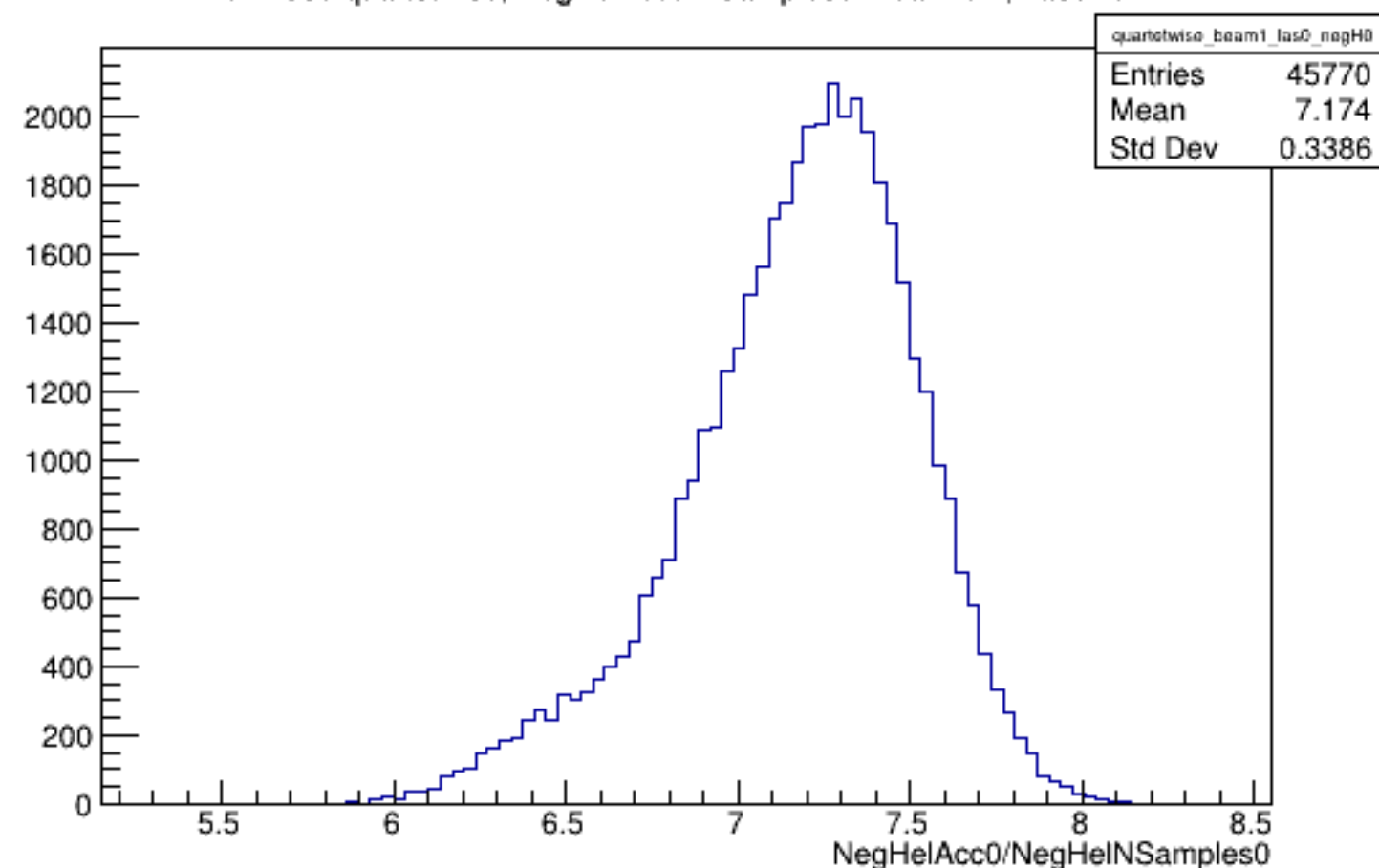
Run 4356 quartetwise, NegHelAcc0/NSamples0: Beam ON, Laser OFF
