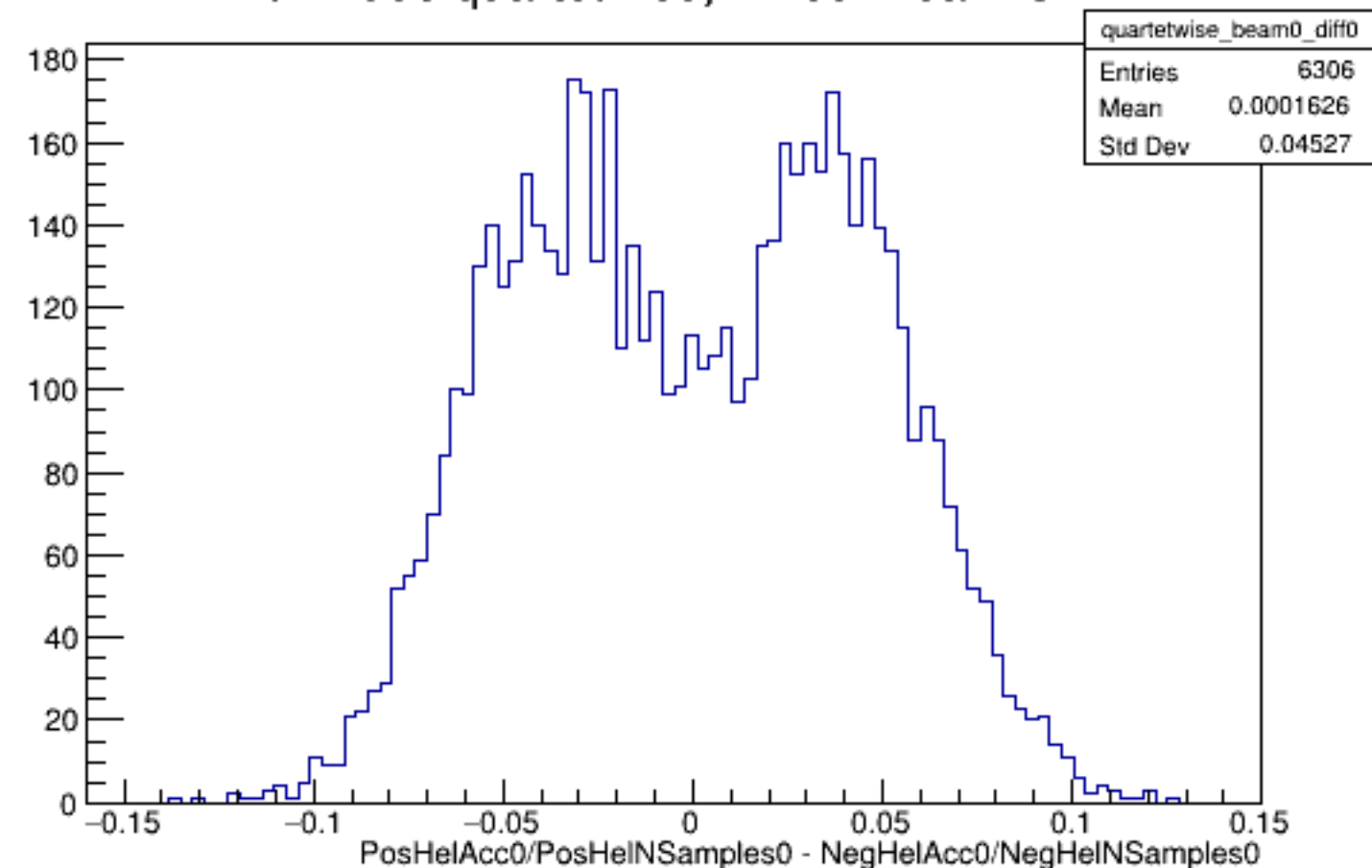
Run 4356 quartetwise, Diffs0: Beam OFF
