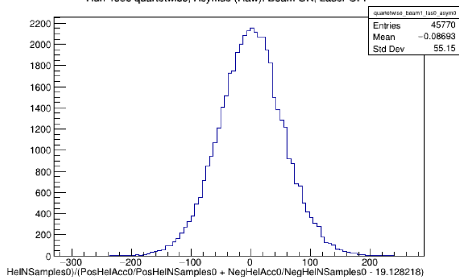
Run 4356 quartetwise, Asyms0 (Raw): Beam ON, Laser OFF
