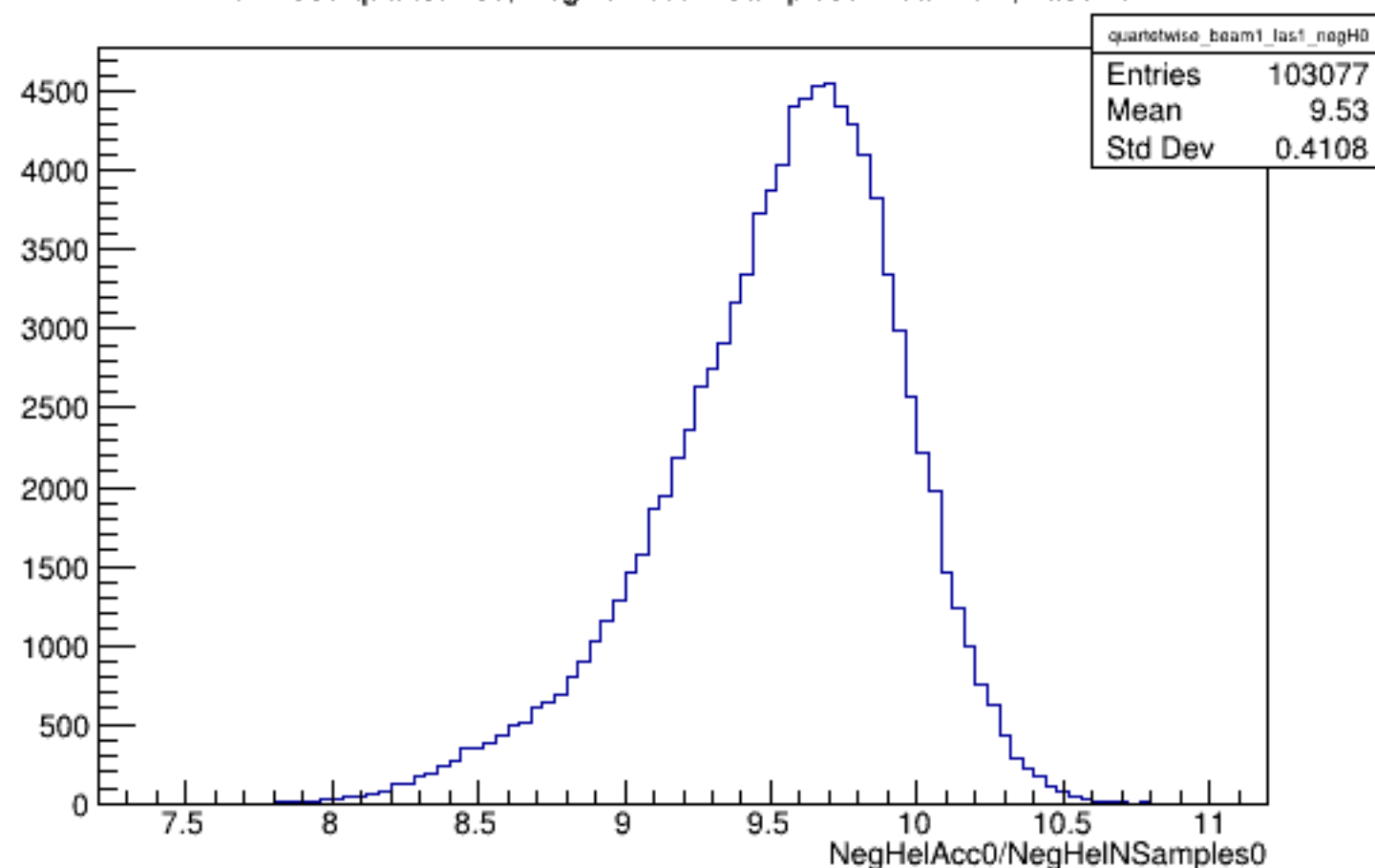
Run 4356 quartetwise, NegHelAcc0/NSamples0: Beam ON, Laser ON
