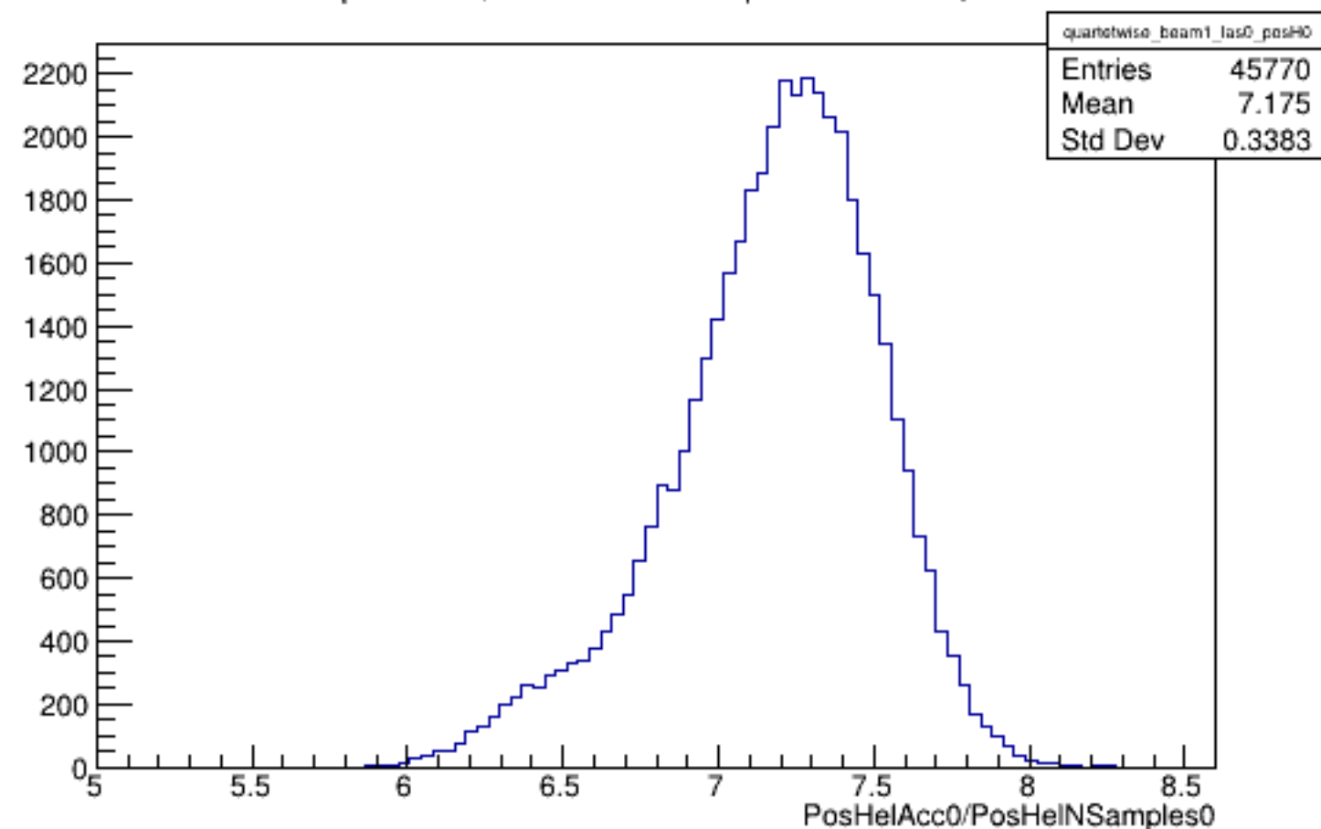
Run 4356 quartetwise, PosHelAcc0/NSamples0: Beam ON, Laser OFF
