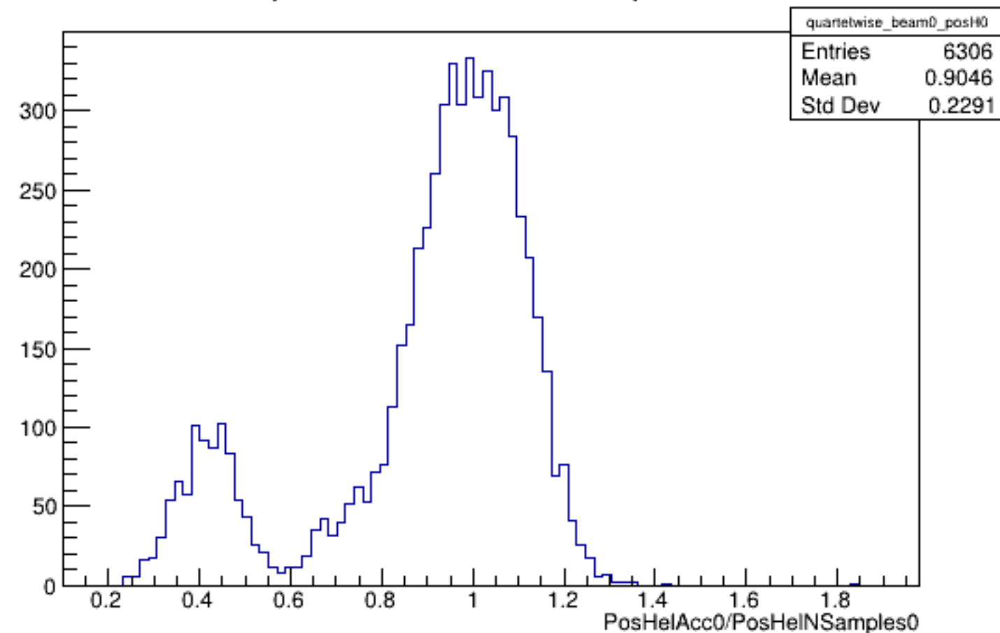
Run 4356 quartetwise, PosHelAcc0/NSamples0: Beam OFF
