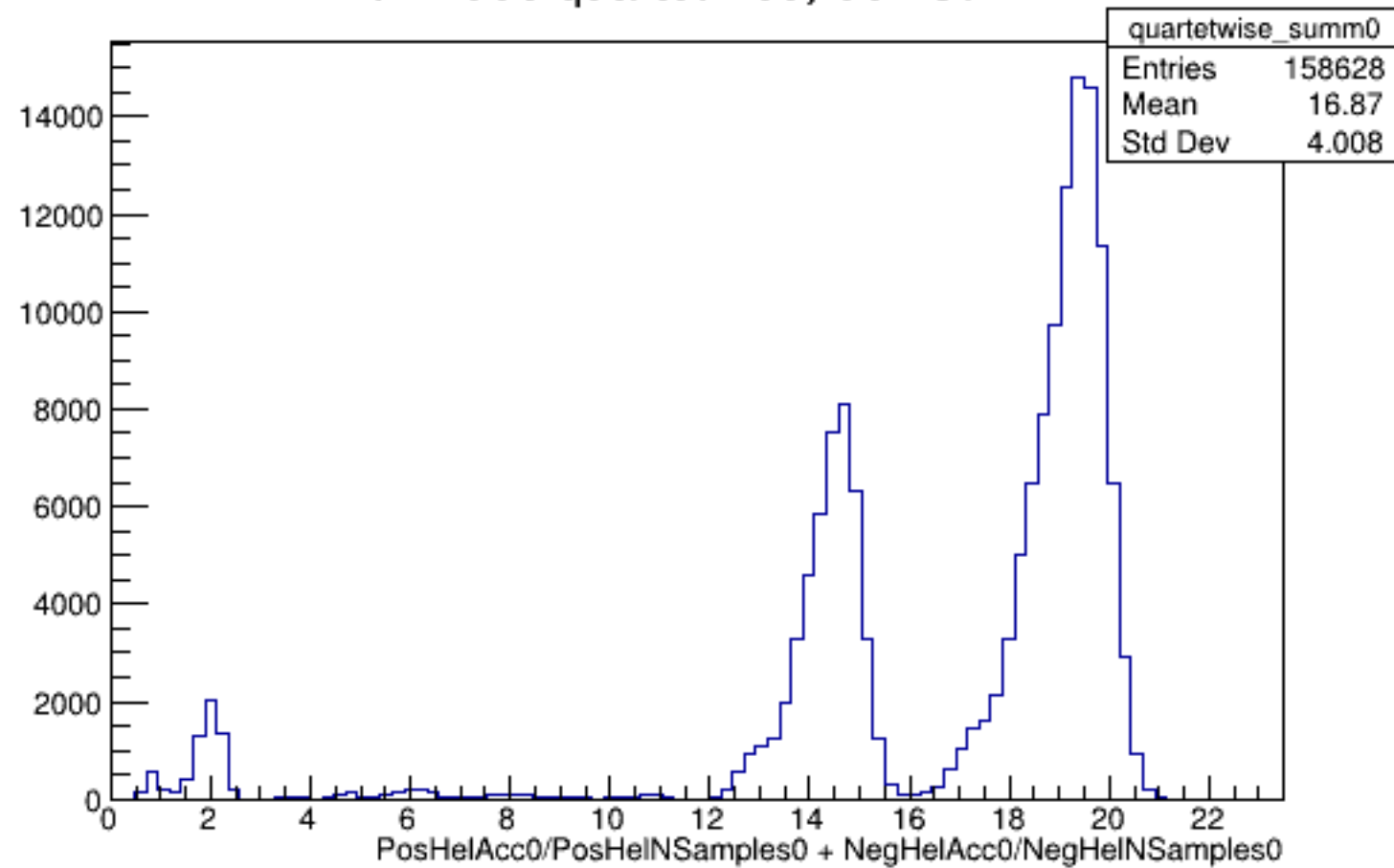
Run 4356 quartetwise, Sums0: All
