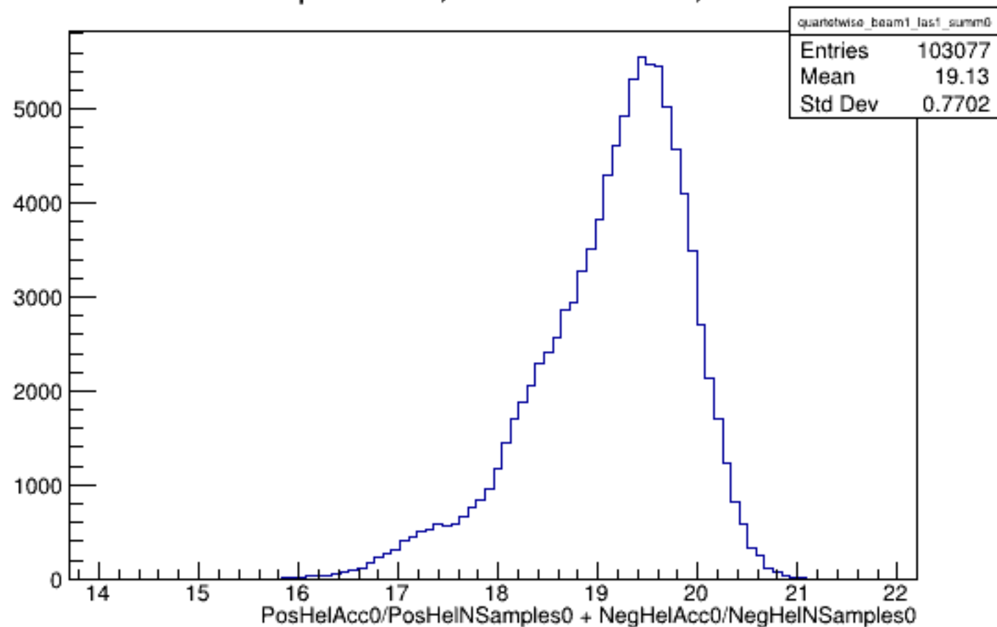
Run 4356 quartetwise, Sums0: Beam ON, Laser ON
