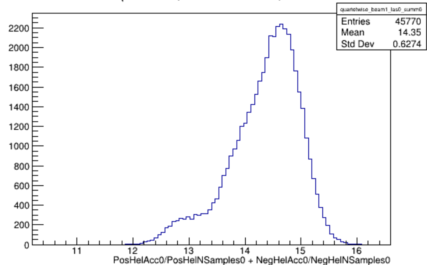
Run 4356 quartetwise, Sums0: Beam ON, Laser OFF
