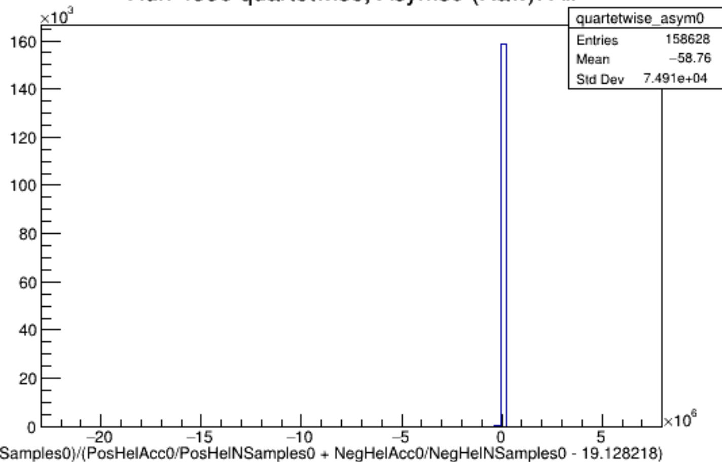
Run 4356 quartetwise, Asyms0 (Raw): All
