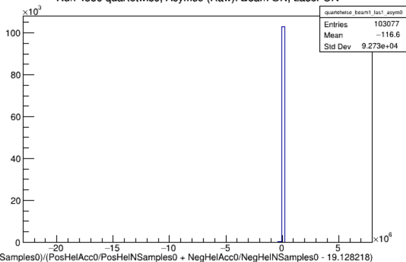
Run 4356 quartetwise, Asyms0 (Raw): Beam ON, Laser ON
