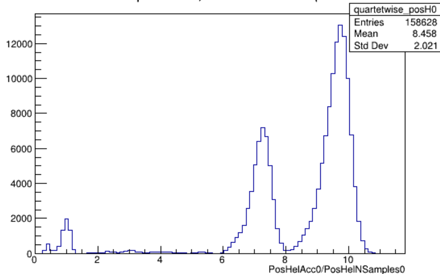
Run 4356 quartetwise, PosHelAcc0/NSamples0: All
