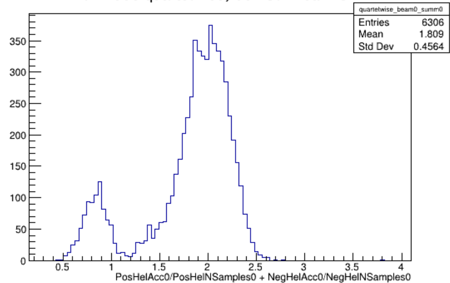
Run 4356 quartetwise, Sums0: Beam OFF
