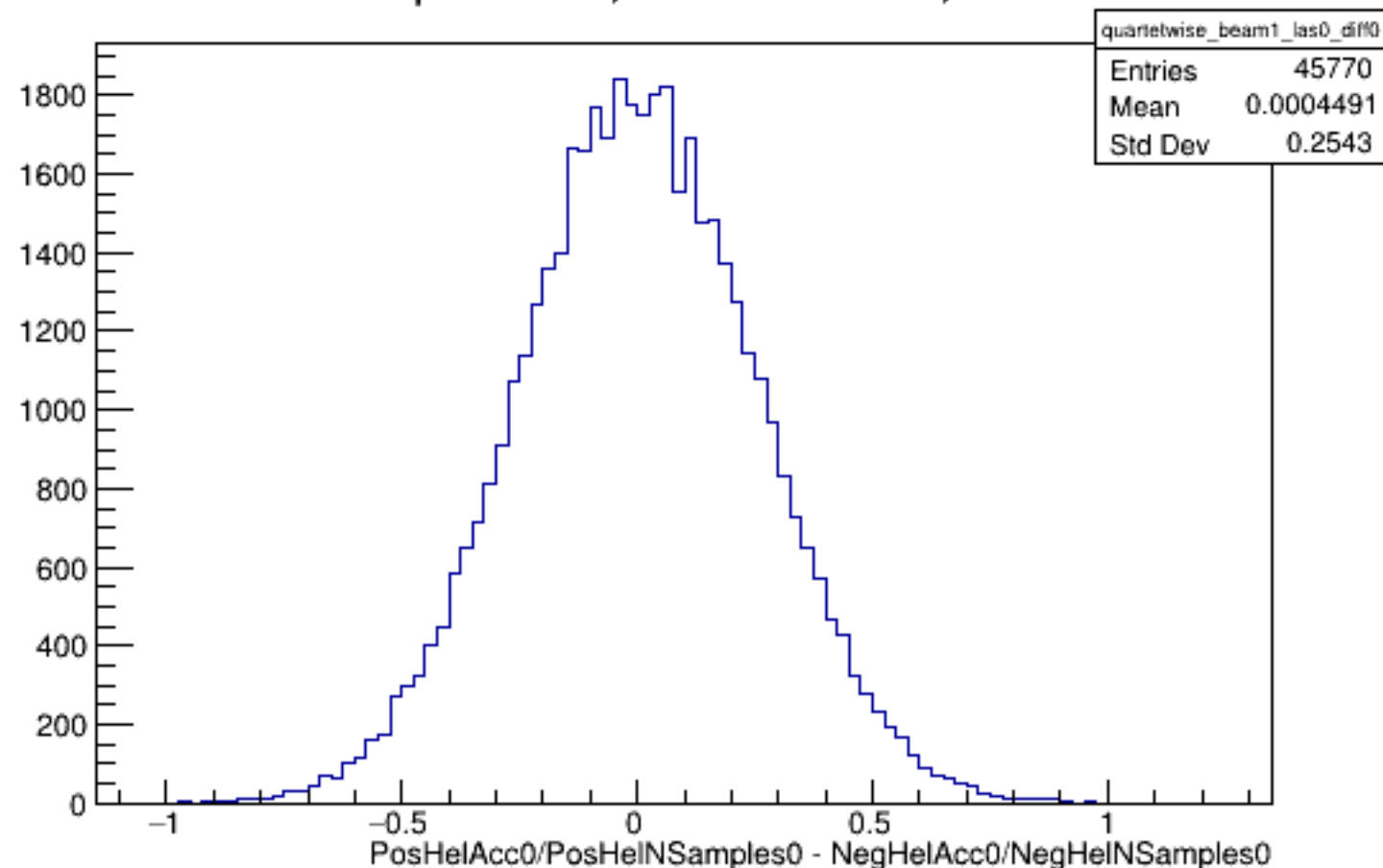
Run 4356 quartetwise, Diffs0: Beam ON, Laser OFF
