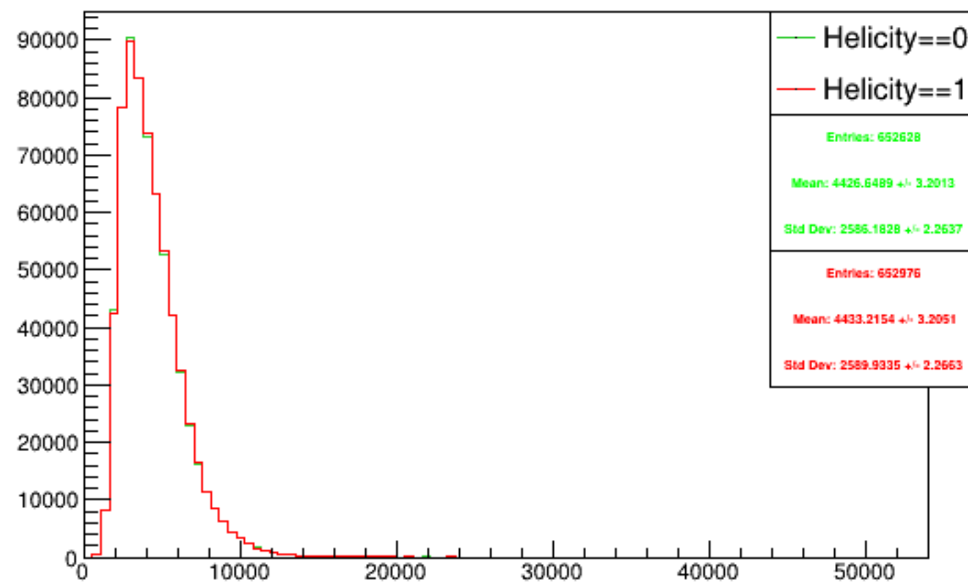
Run 4356 triggerwise, sums: Beam ON, Laser OFF
