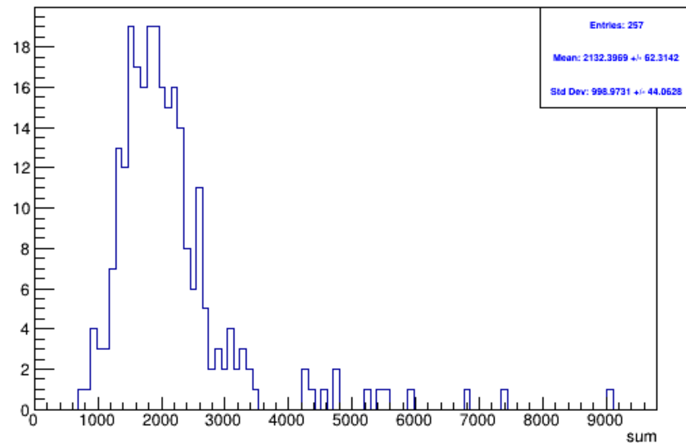
Run 4356 triggerwise, sums: Beam OFF
