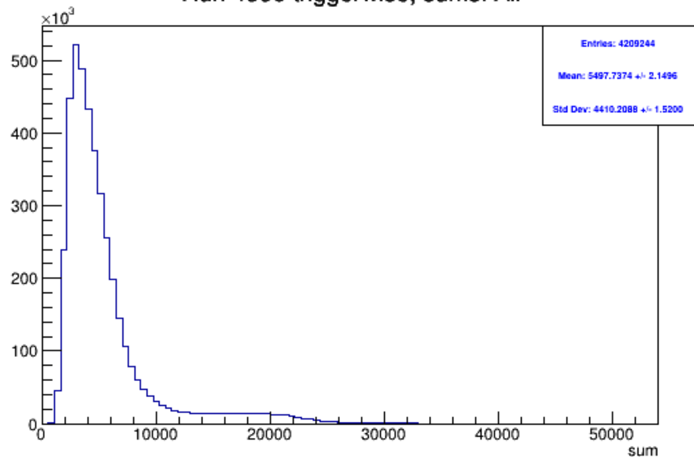
Run 4356 triggerwise, sums: All
