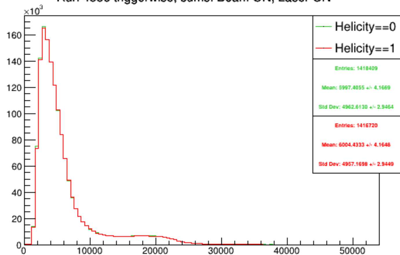
Run 4356 triggerwise, sums: Beam ON, Laser ON
