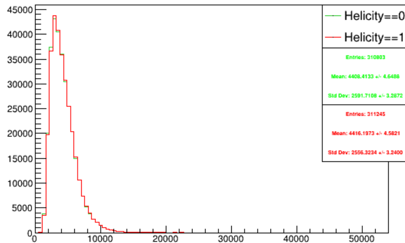
Run 4358 triggerwise, sums: Beam ON, Laser OFF
