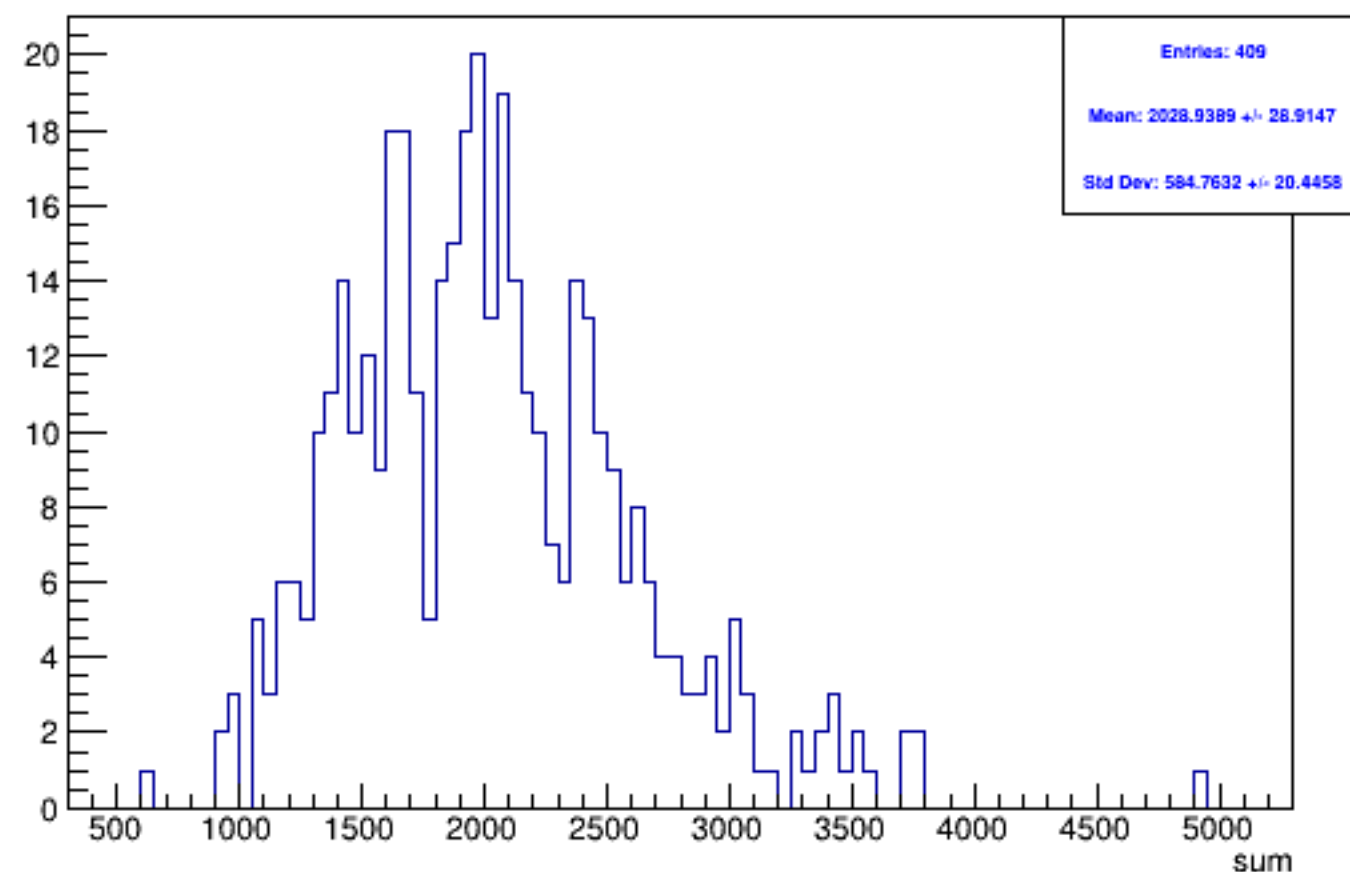
Run 4358 triggerwise, sums: Beam OFF
