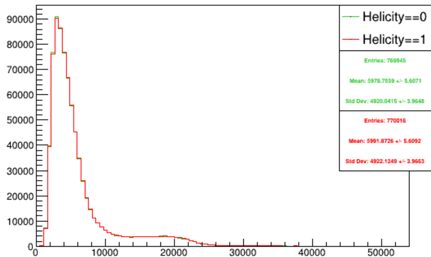
Run 4358 triggerwise, sums: Beam ON, Laser ON
