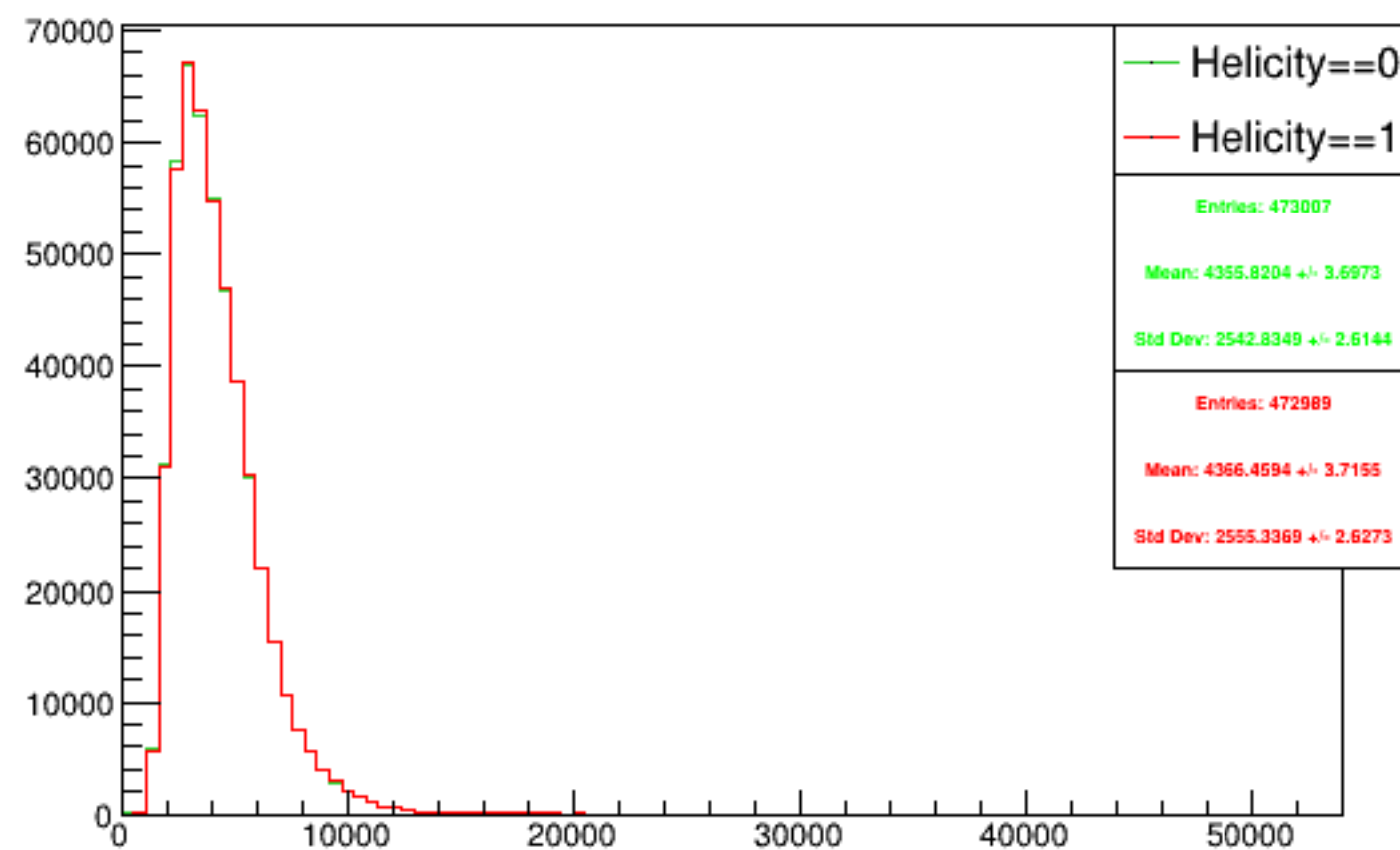
Run 4359 triggerwise, sums: Beam ON, Laser OFF
