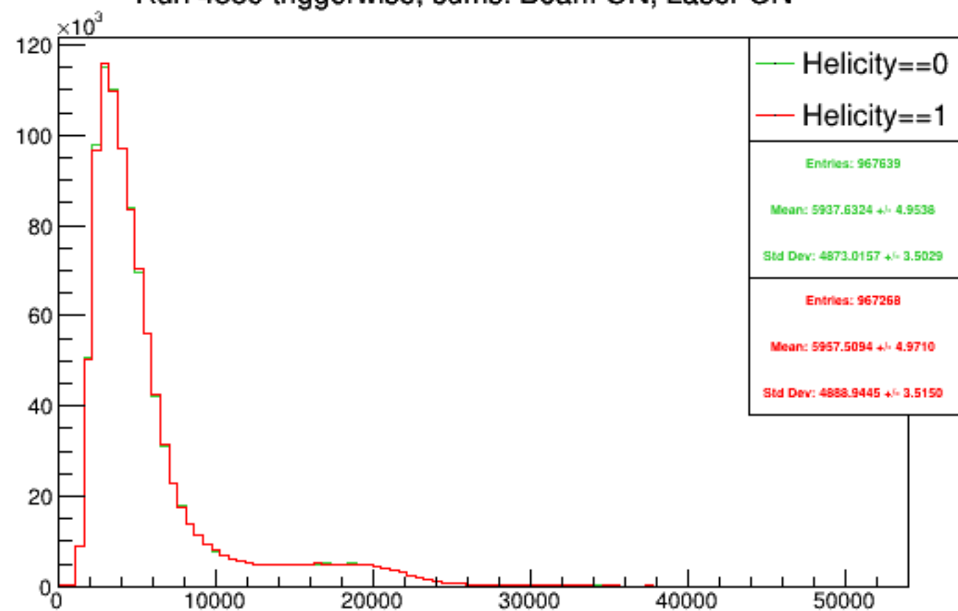
Run 4359 triggerwise, sums: Beam ON, Laser ON
