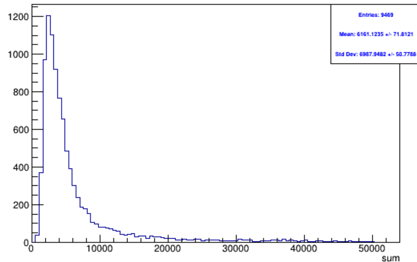
Run 4359 triggerwise, sums: Beam OFF
