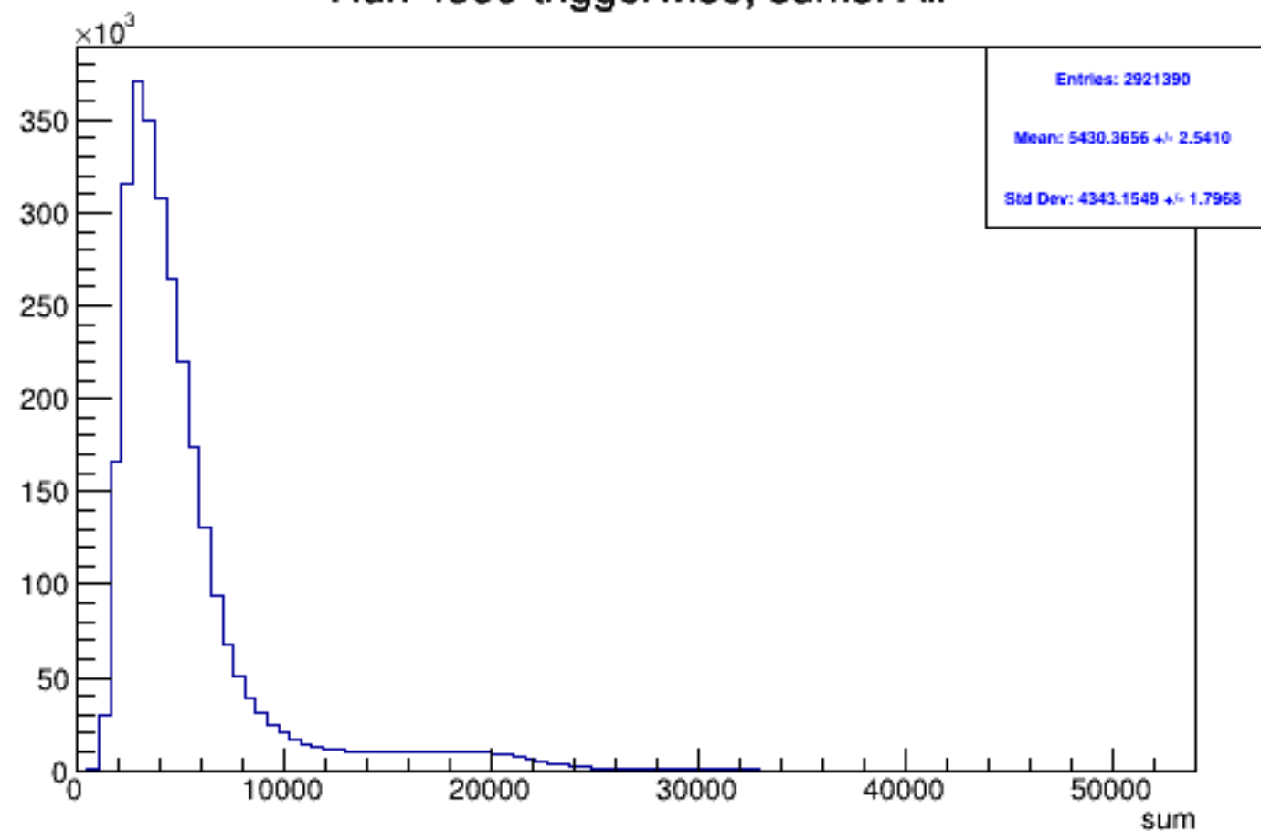
Run 4359 triggerwise, sums: All
