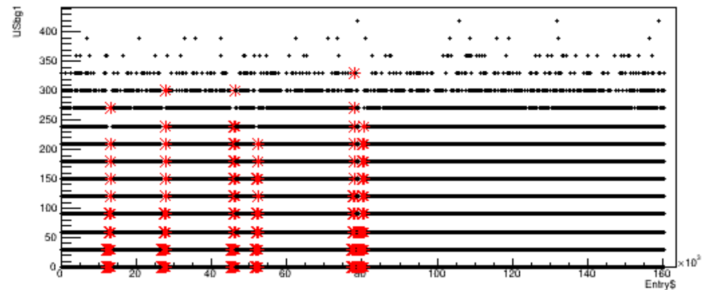
Run 4365, quartetwise: USbg1 vs time
