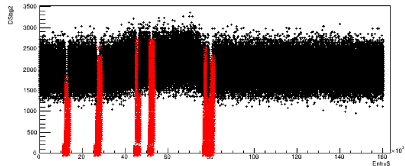
Run 4365, quartetwise: DSbg2 vs time
