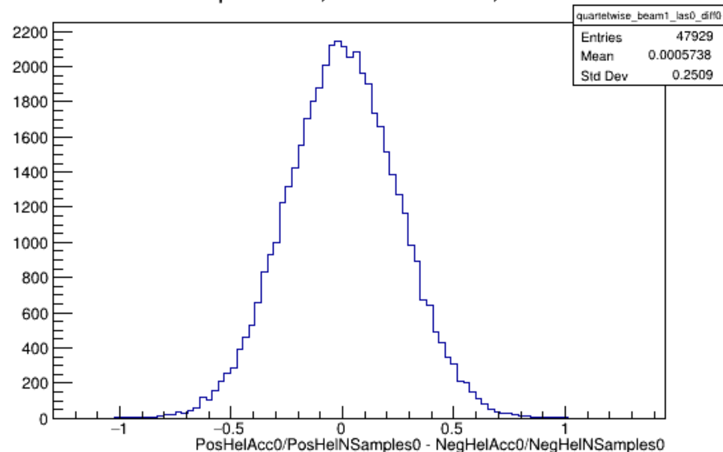
Run 4365 quartetwise, Diffs0: Beam ON, Laser OFF
