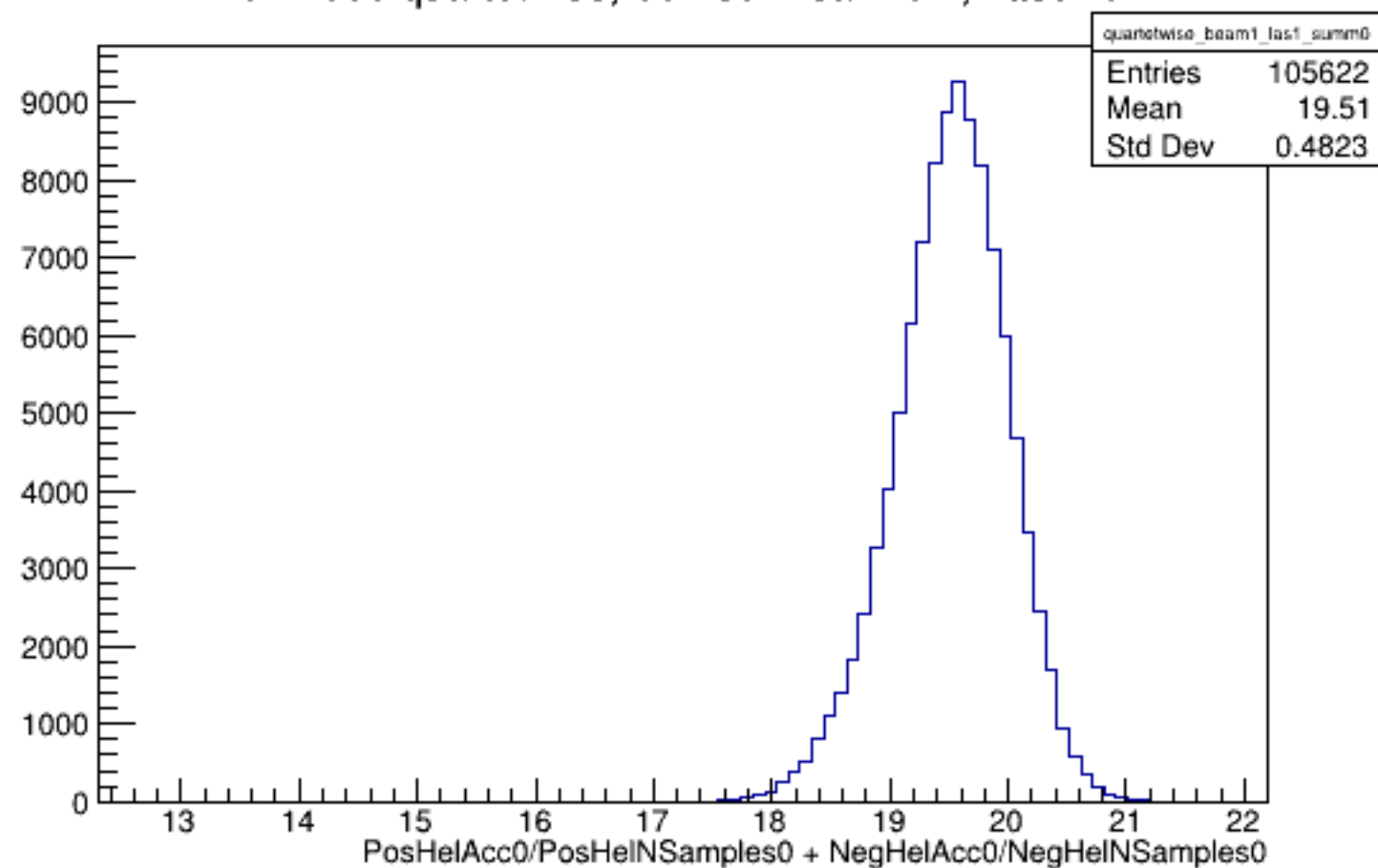
Run 4365 quartetwise, Sums0: Beam ON, Laser ON
