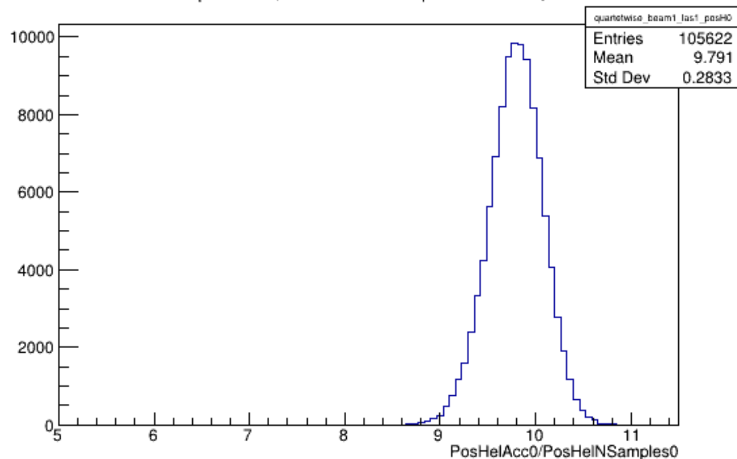
Run 4365 quartetwise, PosHelAcc0/NSamples0: Beam ON, Laser ON
