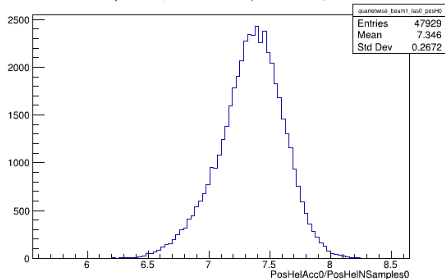
Run 4365 quartetwise, PosHelAcc0/NSamples0: Beam ON, Laser OFF
