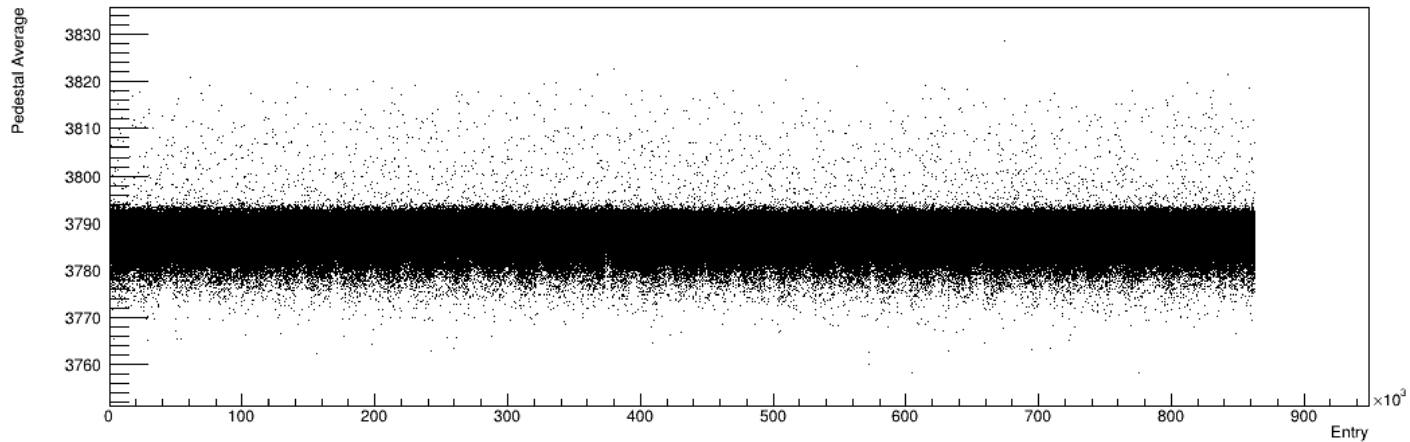
Run 4366, snapshots: Pedestal vs. Time
