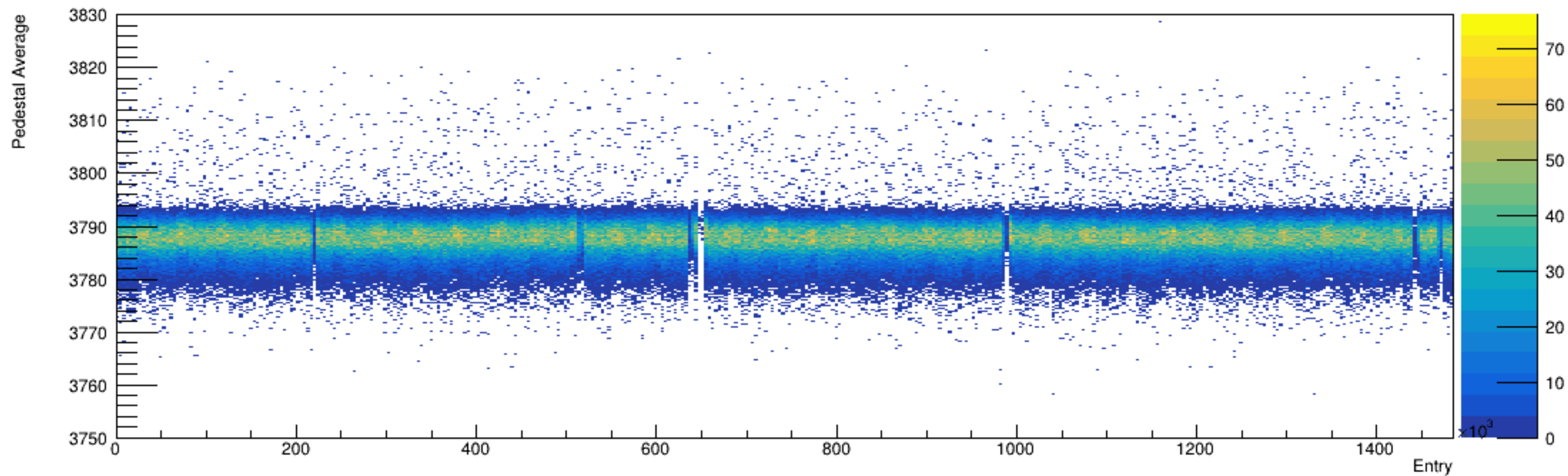
Run 4366, snapshots: Pedestal vs. Time
