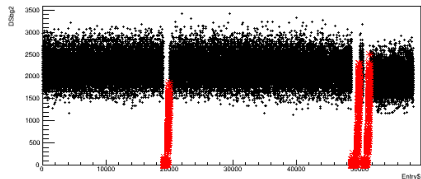
Run 4367, quartetwise: DSbg2 vs time
