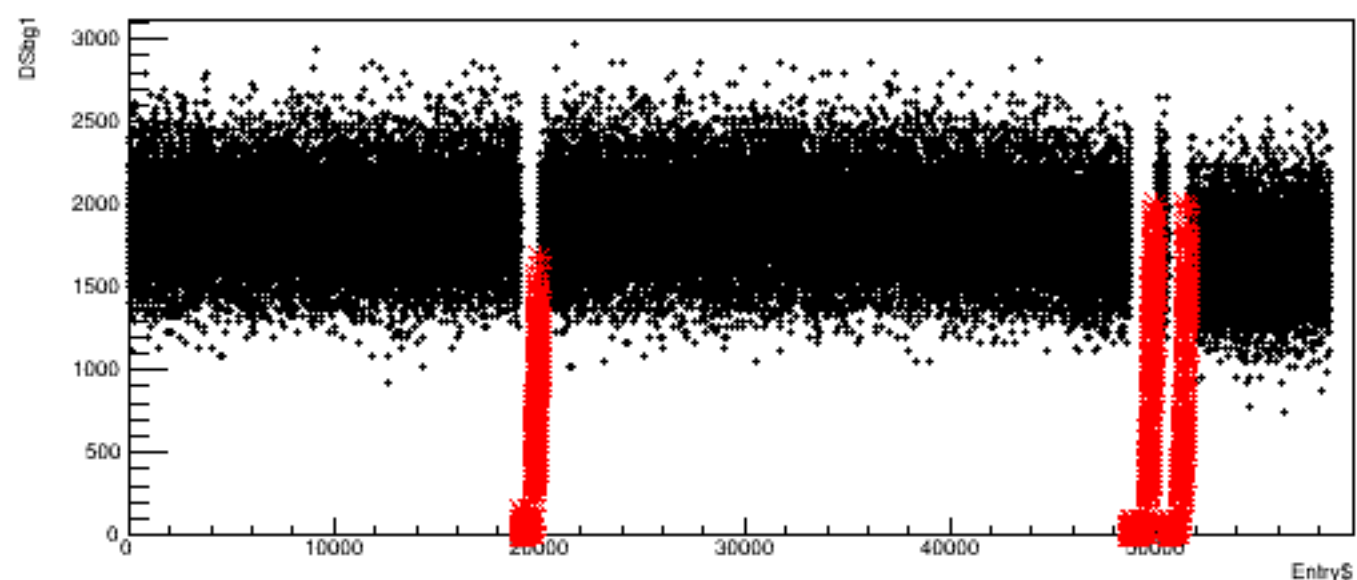
Run 4367, quartetwise: DSbg1 vs time
