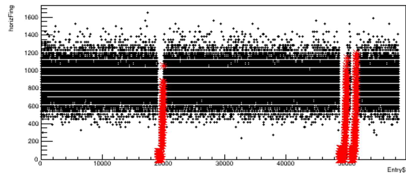
Run 4367, quartetwise: horizFing vs time
