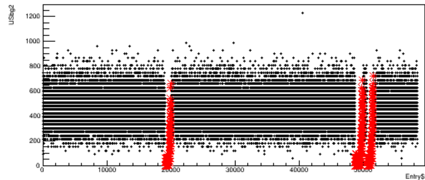
Run 4367, quartetwise: USbg2 vs time
