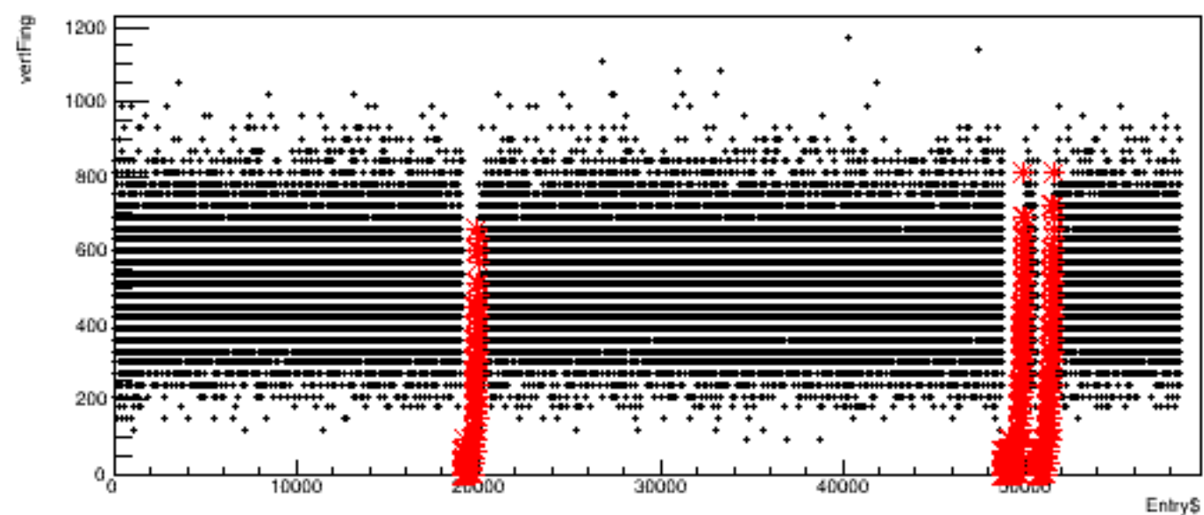
Run 4367, quartetwise: vertFing vs time
