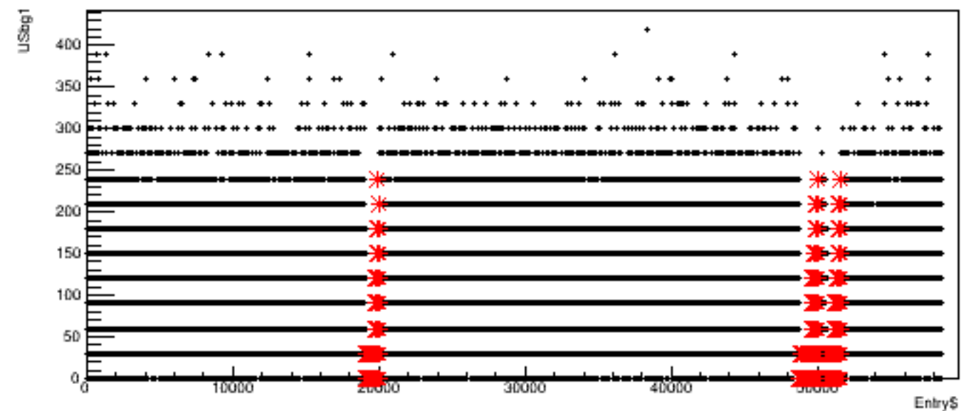
Run 4367, quartetwise: USbg1 vs time
