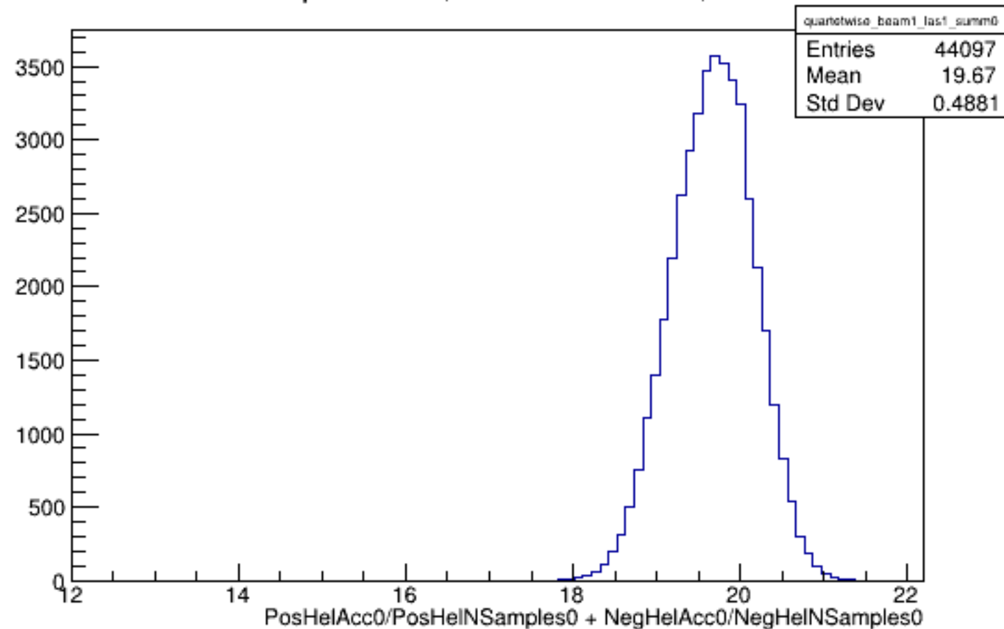
Run 4367 quartetwise, Sums0: Beam ON, Laser ON
