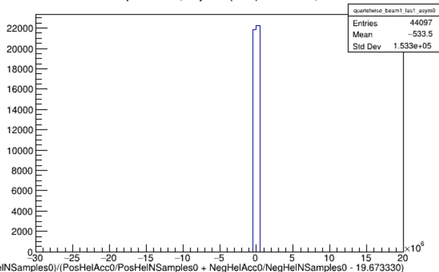
Run 4367 quartetwise, Asyms0 (Raw): Beam ON, Laser ON
