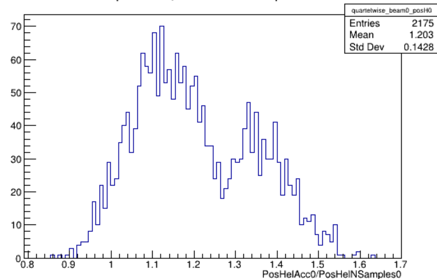
Run 4367 quartetwise, PosHelAcc0/NSamples0: Beam OFF
