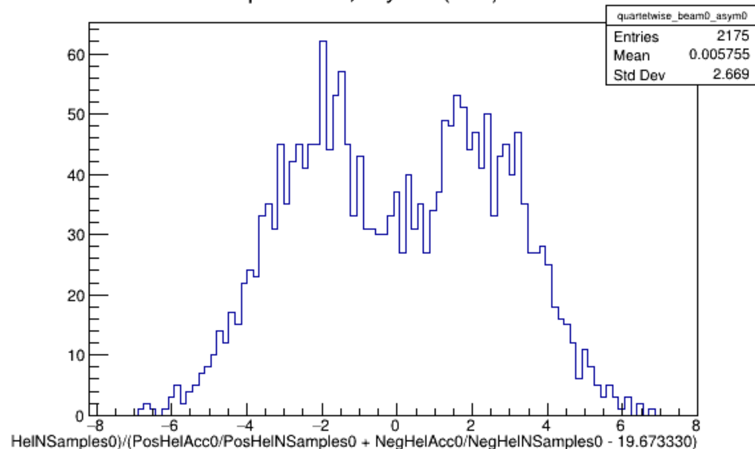
Run 4367 quartetwise, Asyms0 (Raw): Beam OFF
