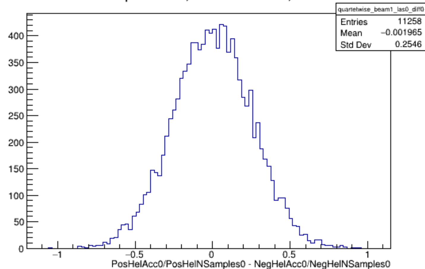
Run 4367 quartetwise, Diffs0: Beam ON, Laser OFF
