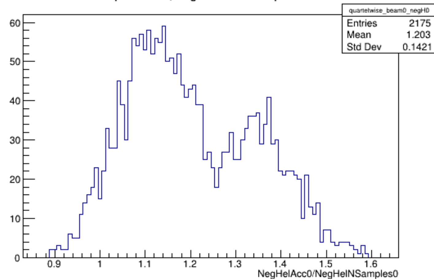
Run 4367 quartetwise, NegHelAcc0/NSamples0: Beam OFF
