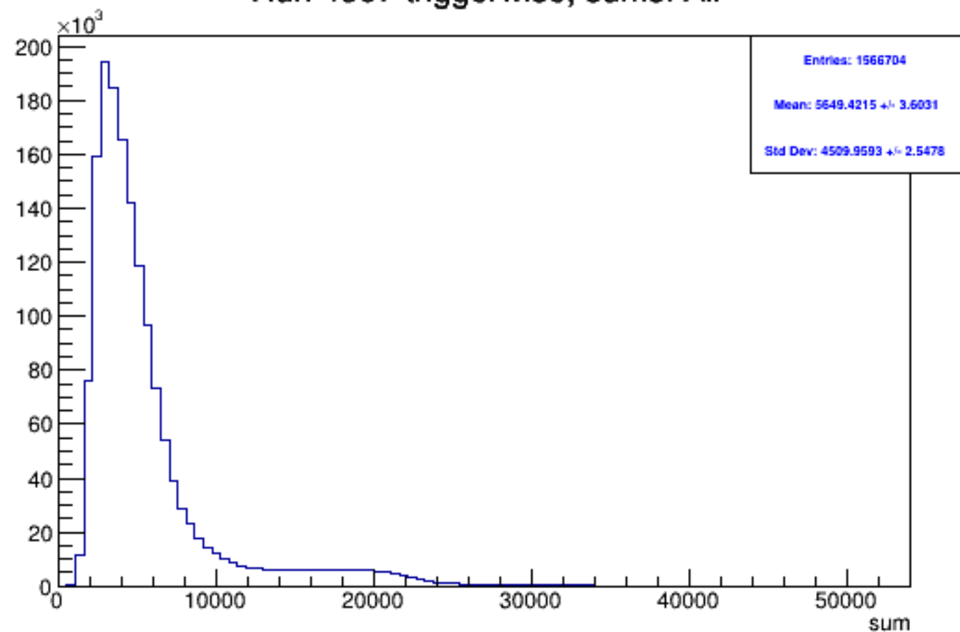
Run 4367 triggerwise, sums: All
