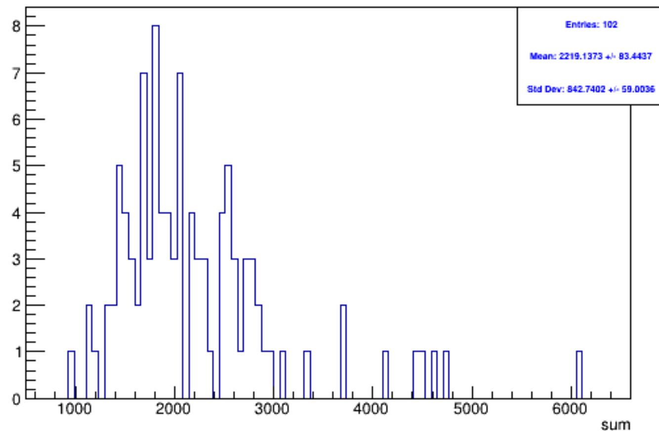
Run 4367 triggerwise, sums: Beam OFF
