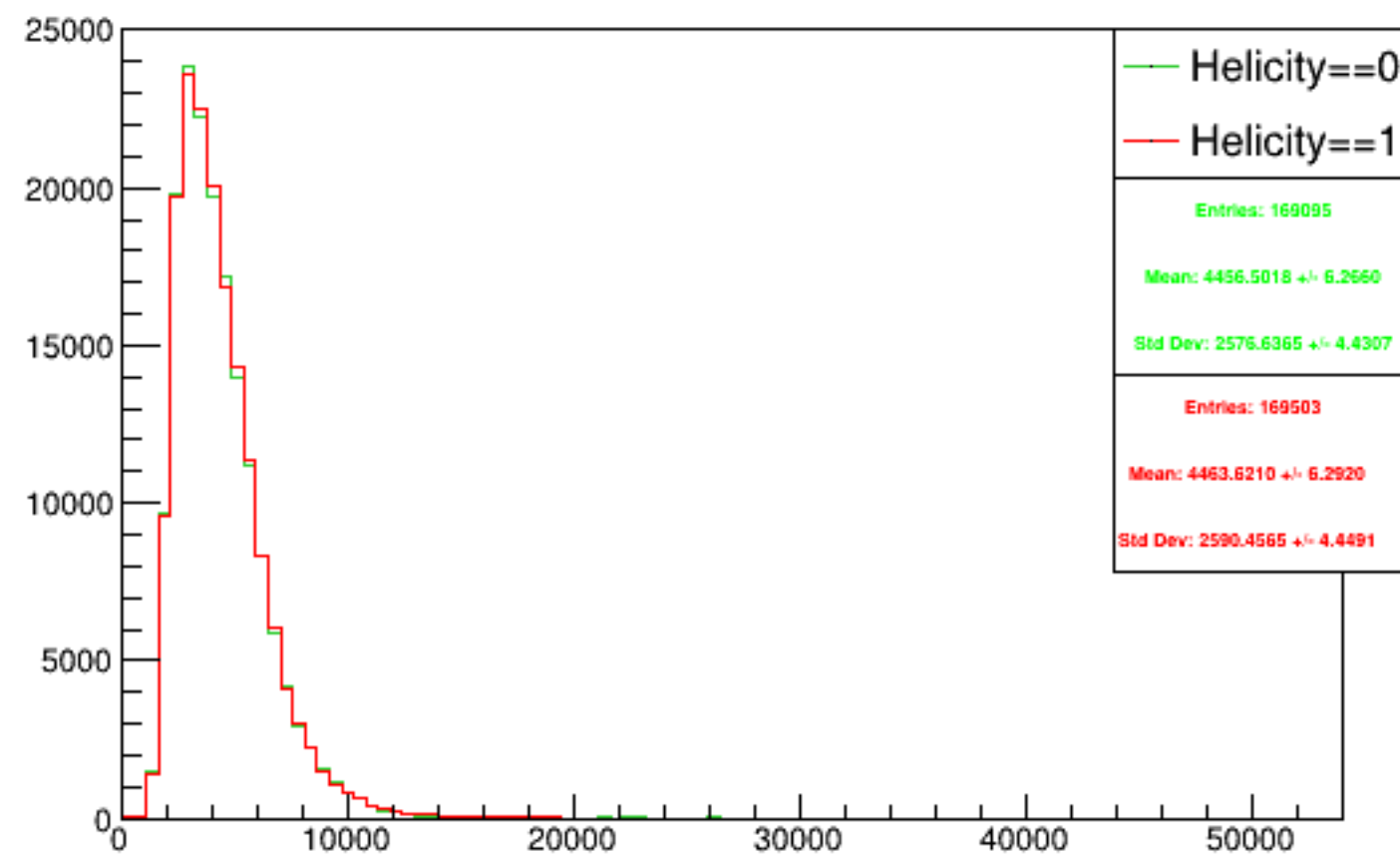
Run 4367 triggerwise, sums: Beam ON, Laser OFF
