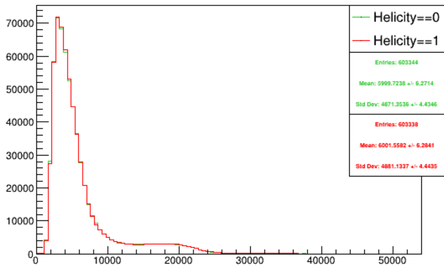
Run 4367 triggerwise, sums: Beam ON, Laser ON
