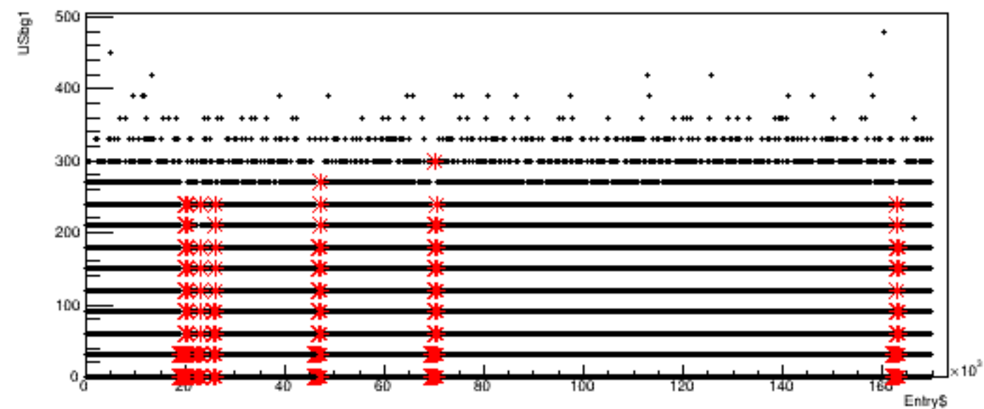
Run 4368, quartetwise: USbg1 vs time
