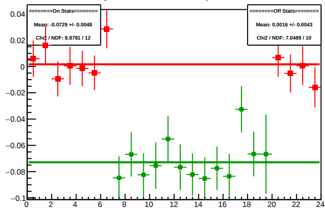
Cycle 4369.16: Multiplet Diffs
