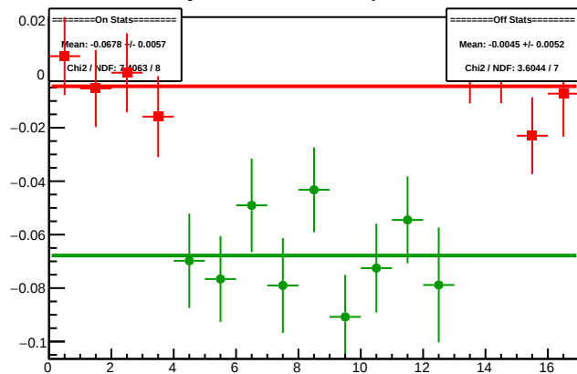
Cycle 4369.17: Multiplet Diffs
