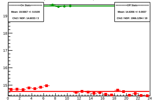
Cycle 4369.14: Multiplet Sums
