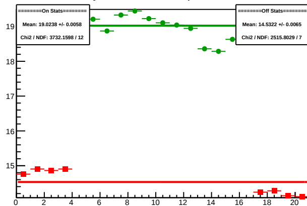
Cycle 4369.6: Multiplet Sums
