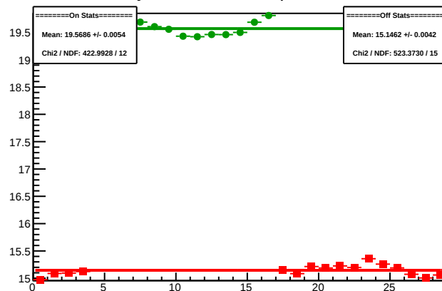
Cycle 4369.19: Multiplet Sums
