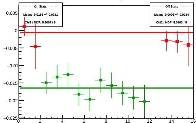
Cycle 4369.3: Multiplet Asyms
