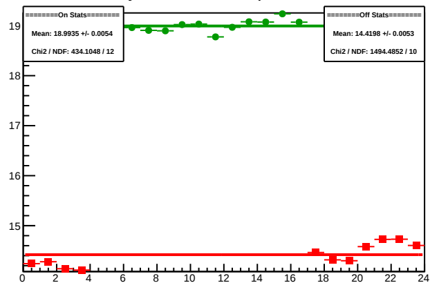
Cycle 4369.7: Multiplet Sums
