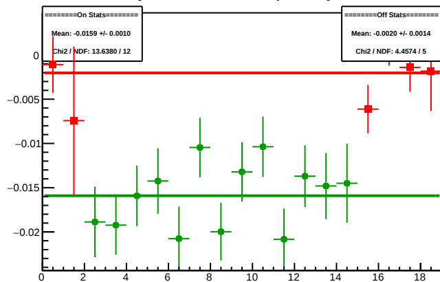
Cycle 4369.11: Multiplet Asyms
