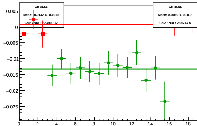
Cycle 4369.1: Multiplet Asyms
