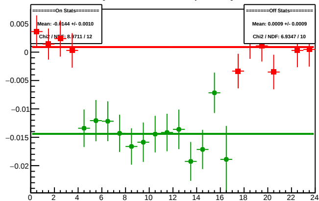
Cycle 4369.8: Multiplet Asyms
