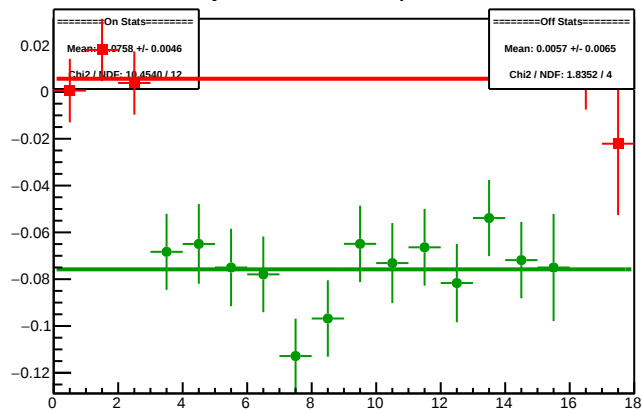
Cycle 4369.2: Multiplet Diffs
