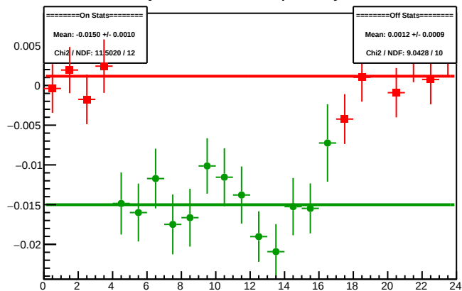
Cycle 4369.4: Multiplet Asyms
