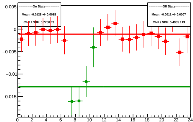
Cycle 4369.14: Multiplet Asyms
