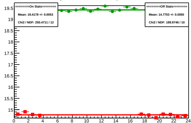
Cycle 4369.4: Multiplet Sums
