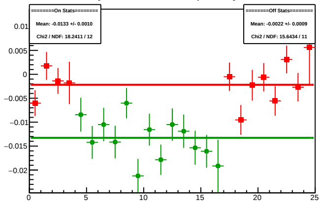
Cycle 4369.12: Multiplet Asyms
