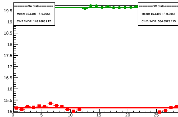
Cycle 4369.20: Multiplet Sums
