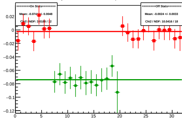
Cycle 4369.9: Multiplet Diffs
