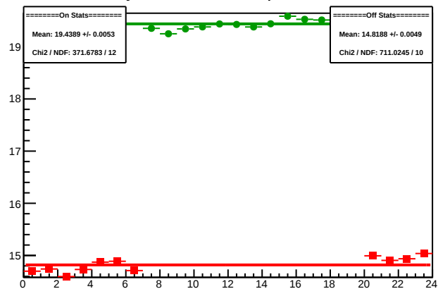
Cycle 4369.16: Multiplet Sums
