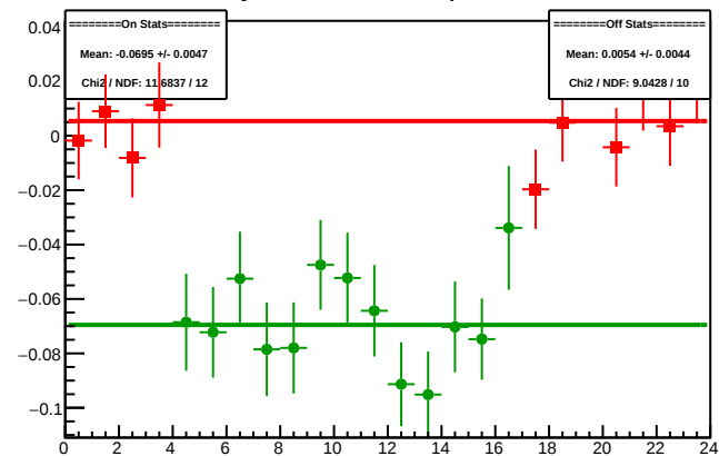
Cycle 4369.4: Multiplet Diffs
