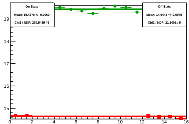
Cycle 4369.3: Multiplet Sums
