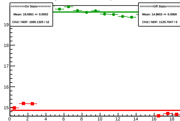
Cycle 4369.1: Multiplet Sums
