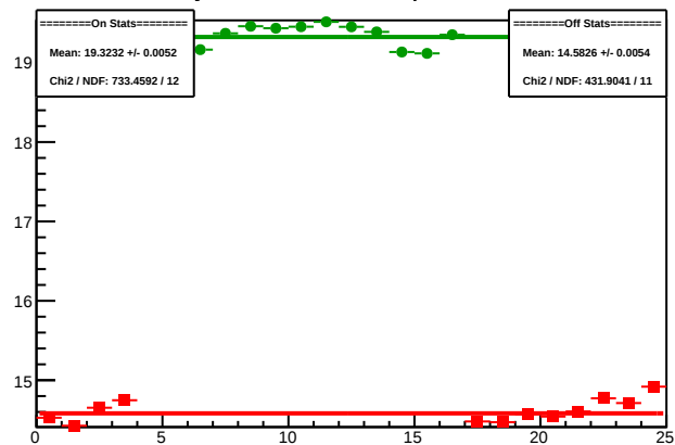
Cycle 4369.12: Multiplet Sums
