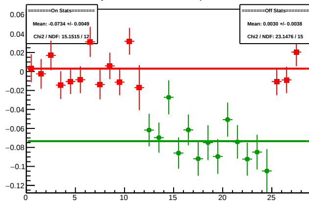
Cycle 4369.20: Multiplet Diffs
