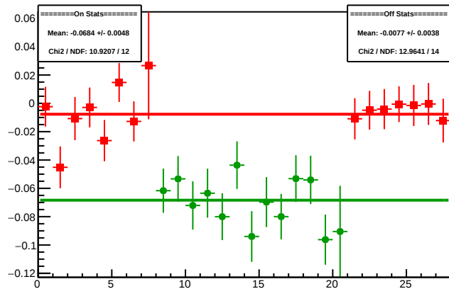
Cycle 4369.13: Multiplet Diffs
