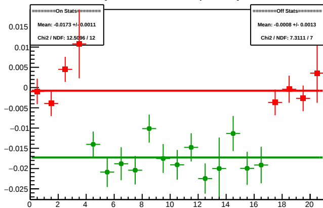
Cycle 4369.6: Multiplet Asyms
