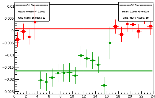
Cycle 4369.7: Multiplet Asyms
