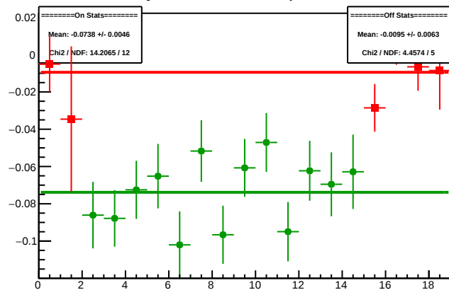
Cycle 4369.11: Multiplet Diffs
