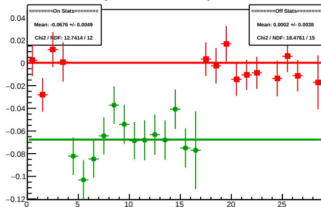
Cycle 4369.19: Multiplet Diffs
