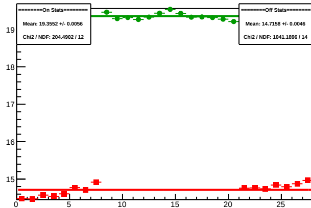
Cycle 4369.13: Multiplet Sums
