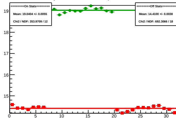
Cycle 4369.9: Multiplet Sums
