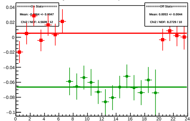
Cycle 4369.5: Multiplet Diffs
