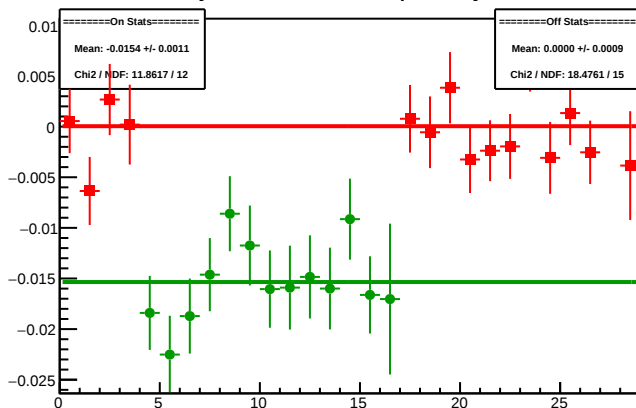
Cycle 4369.19: Multiplet Asyms
