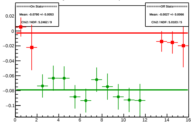
Cycle 4369.3: Multiplet Diffs
