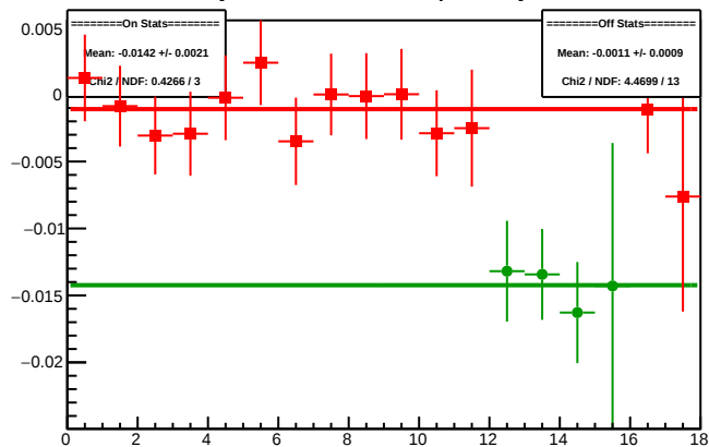
Cycle 4369.10: Multiplet Asyms
