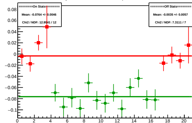
Cycle 4369.6: Multiplet Diffs
