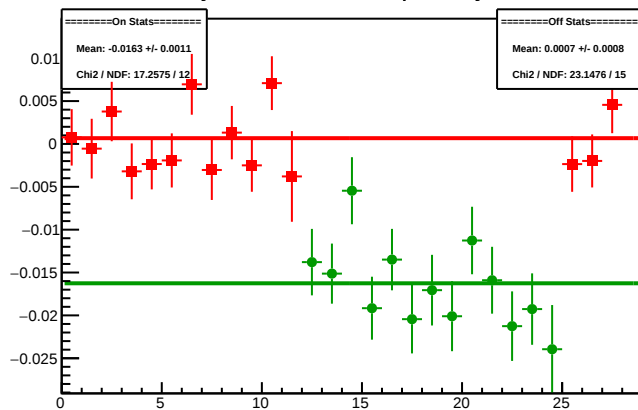
Cycle 4369.20: Multiplet Asyms
