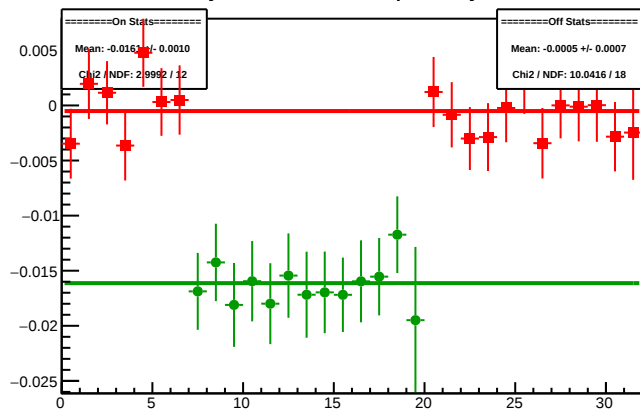
Cycle 4369.9: Multiplet Asyms
