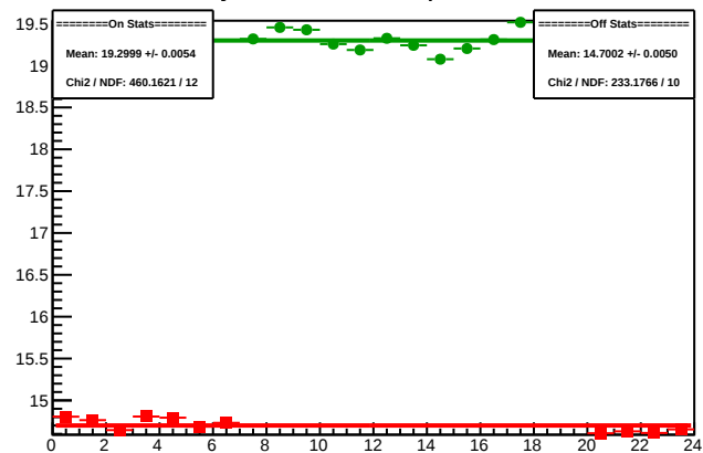
Cycle 4369.5: Multiplet Sums
