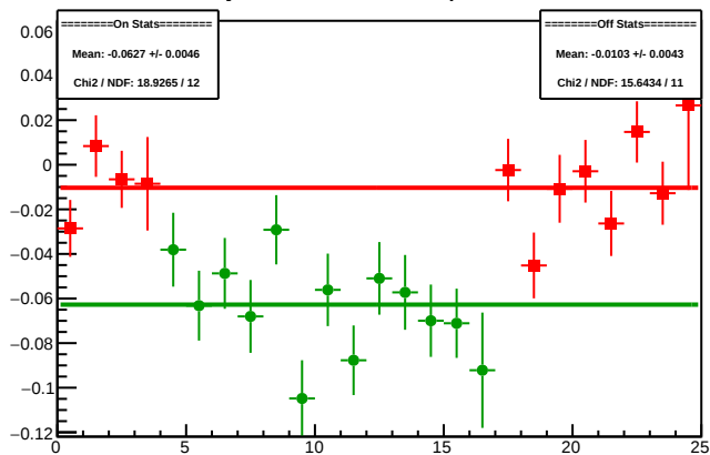
Cycle 4369.12: Multiplet Diffs
