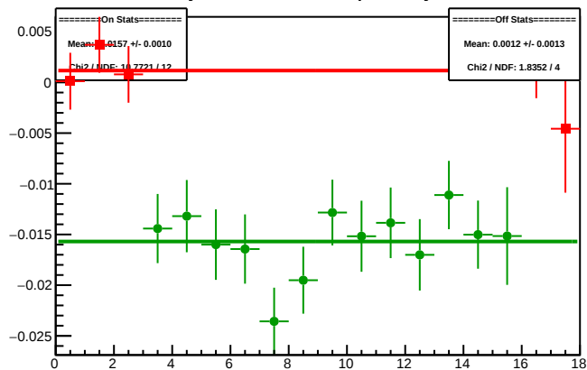
Cycle 4369.2: Multiplet Asyms
