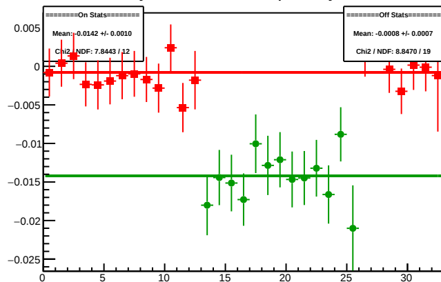
Cycle 4369.15: Multiplet Asyms
