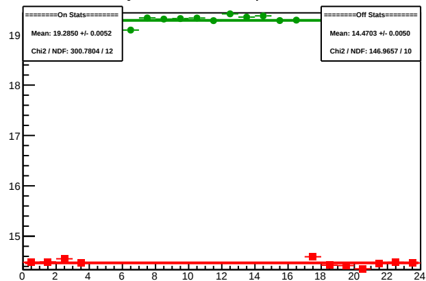
Cycle 4369.8: Multiplet Sums
