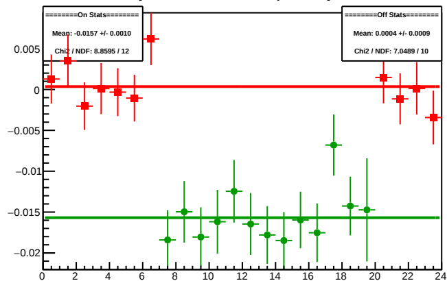
Cycle 4369.16: Multiplet Asyms
