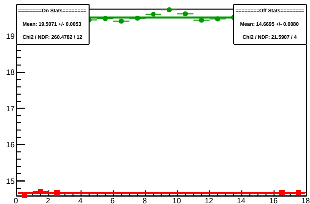
Cycle 4369.2: Multiplet Sums
