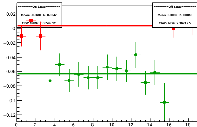
Cycle 4369.1: Multiplet Diffs
