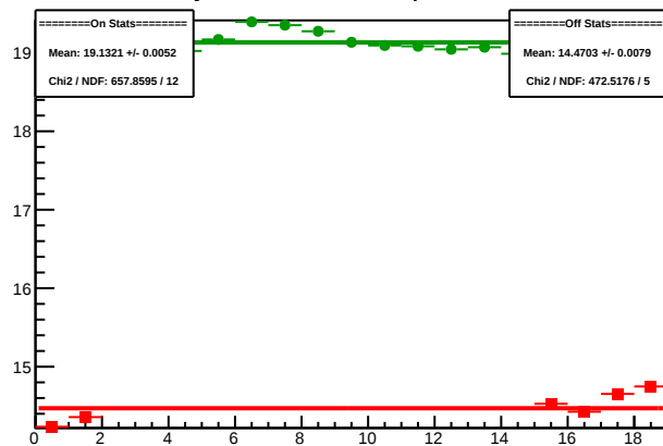
Cycle 4369.11: Multiplet Sums
