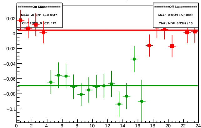
Cycle 4369.8: Multiplet Diffs
