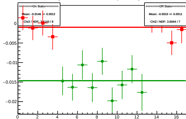
Cycle 4369.17: Multiplet Asyms
