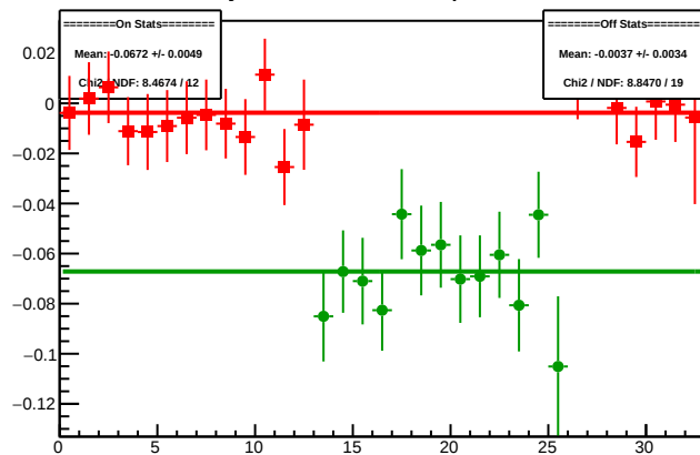
Cycle 4369.15: Multiplet Diffs
