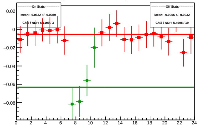
Cycle 4369.14: Multiplet Diffs
