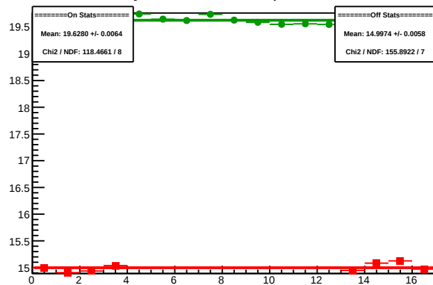
Cycle 4369.17: Multiplet Sums
