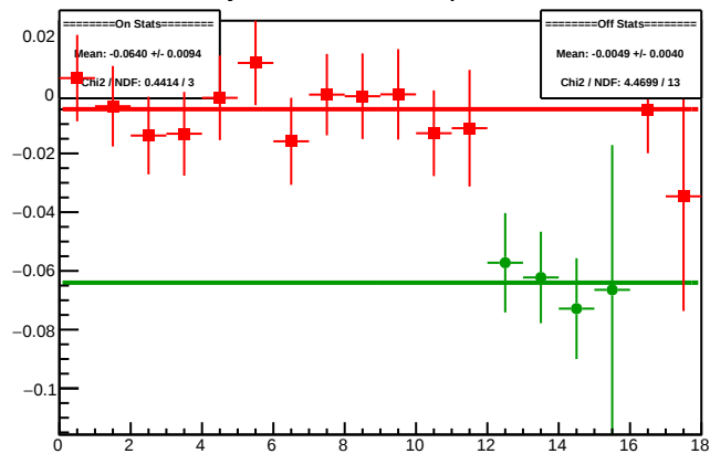
Cycle 4369.10: Multiplet Diffs
