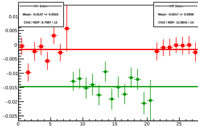
Cycle 4369.13: Multiplet Asyms
