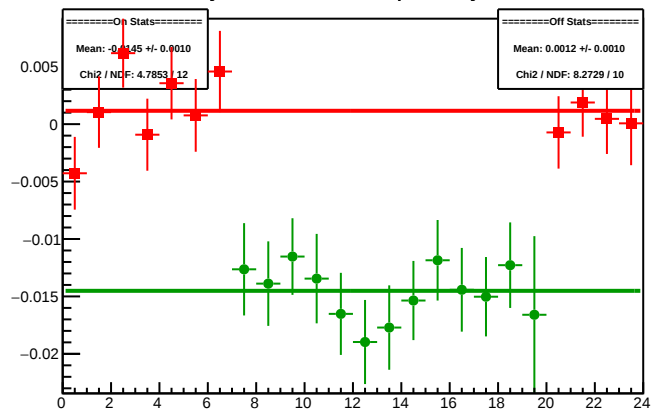
Cycle 4369.5: Multiplet Asyms
