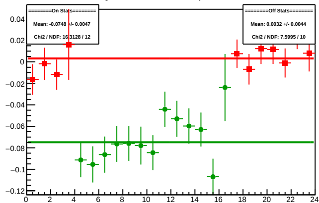
Cycle 4369.7: Multiplet Diffs
