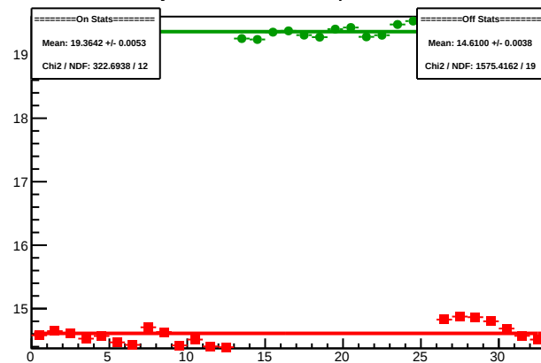
Cycle 4369.15: Multiplet Sums
