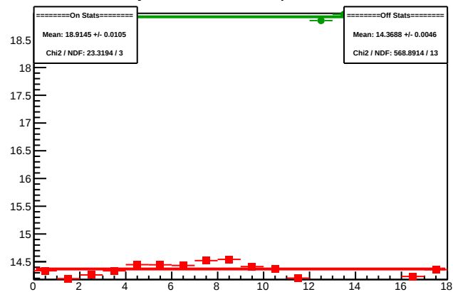
Cycle 4369.10: Multiplet Sums
