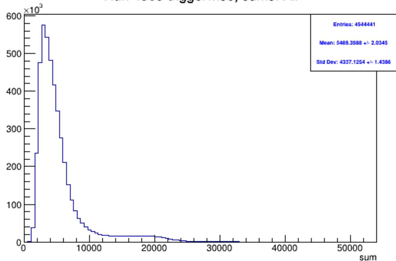
Run 4369 triggerwise, sums: All
