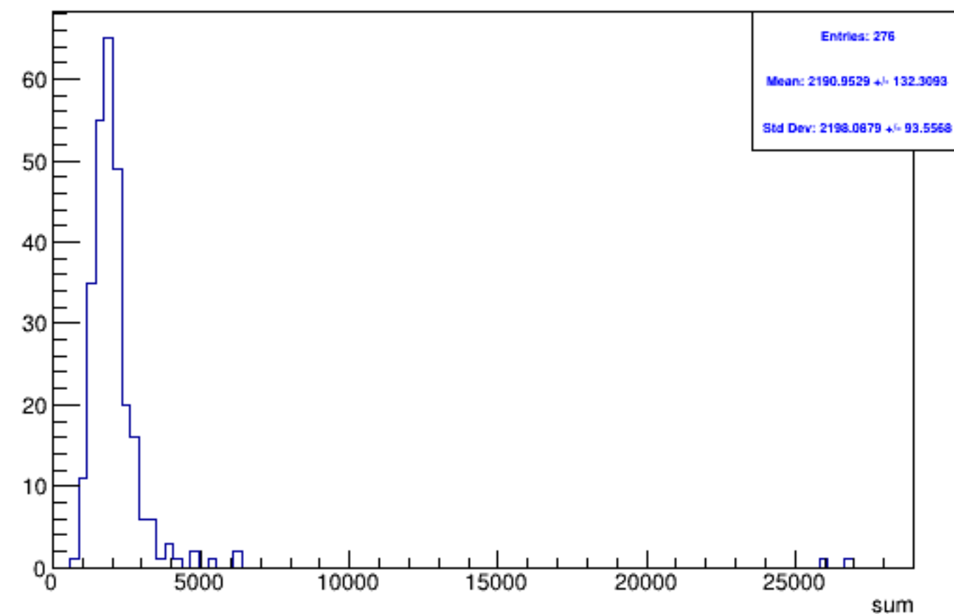
Run 4369 triggerwise, sums: Beam OFF
