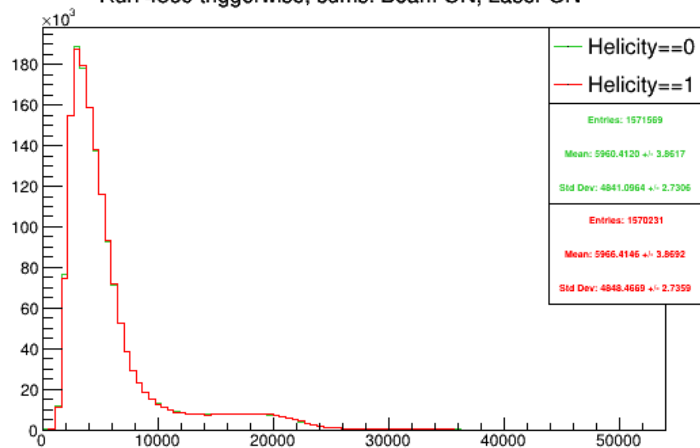
Run 4369 triggerwise, sums: Beam ON, Laser ON
