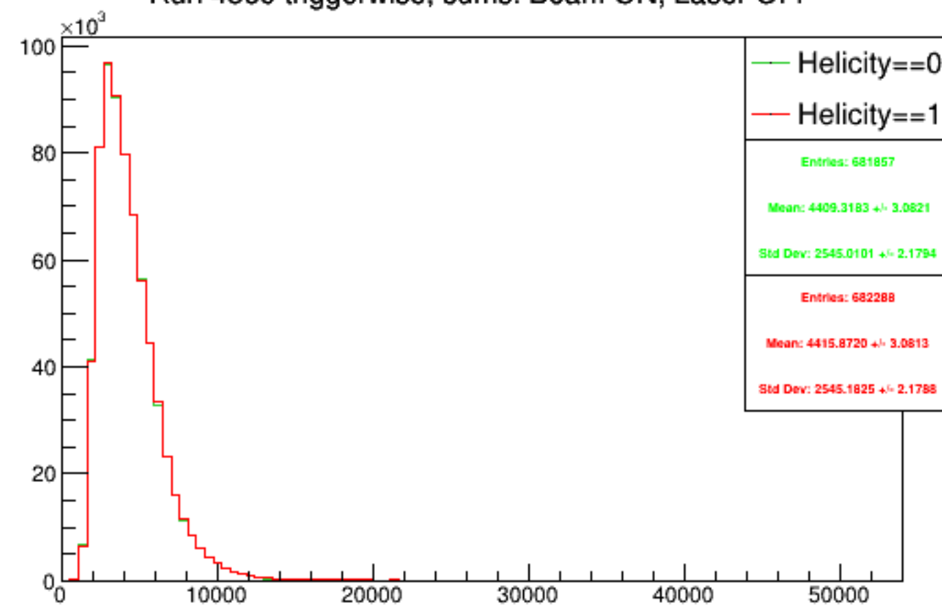
Run 4369 triggerwise, sums: Beam ON, Laser OFF
