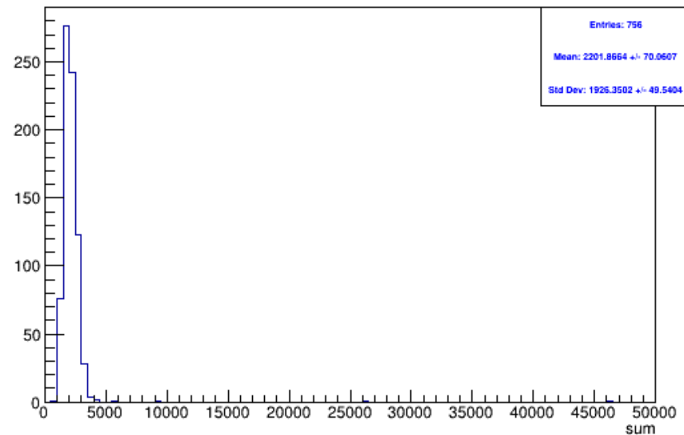
Run 4371 triggerwise, sums: Beam OFF
