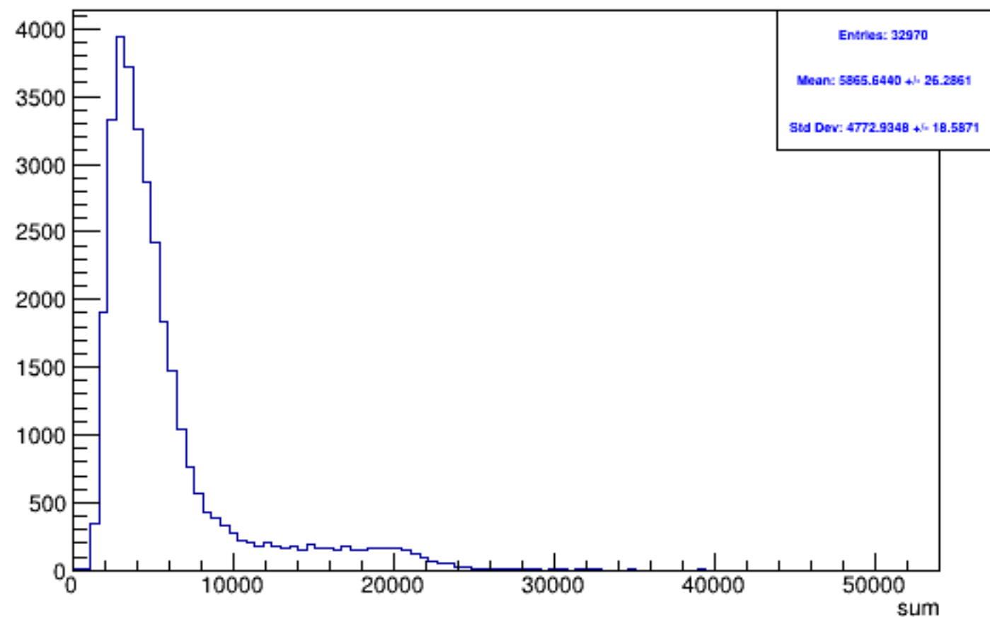
Run 4371 triggerwise, sums: All
