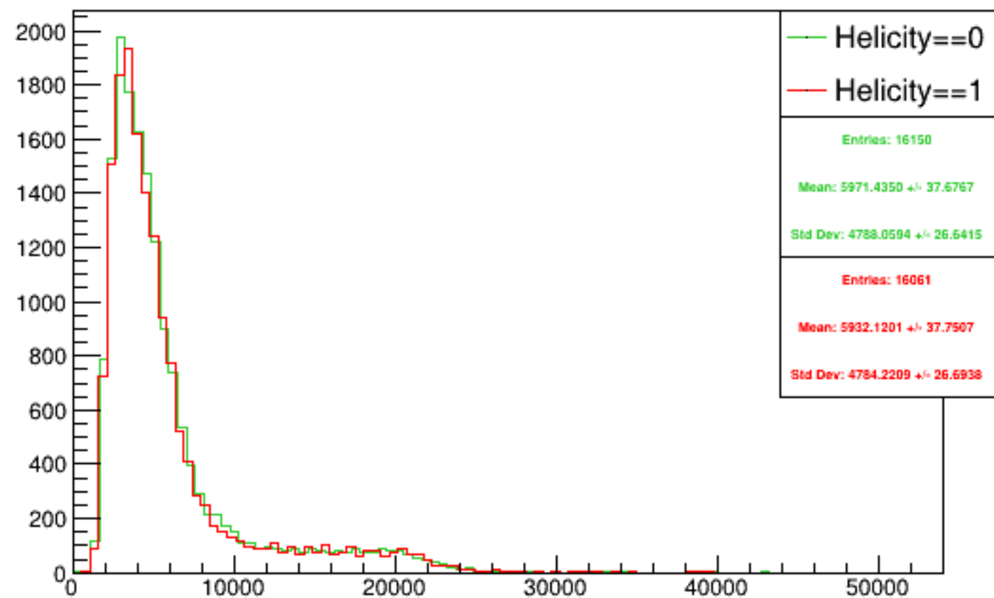
Run 4371 triggerwise, sums: Beam ON, Laser ON
