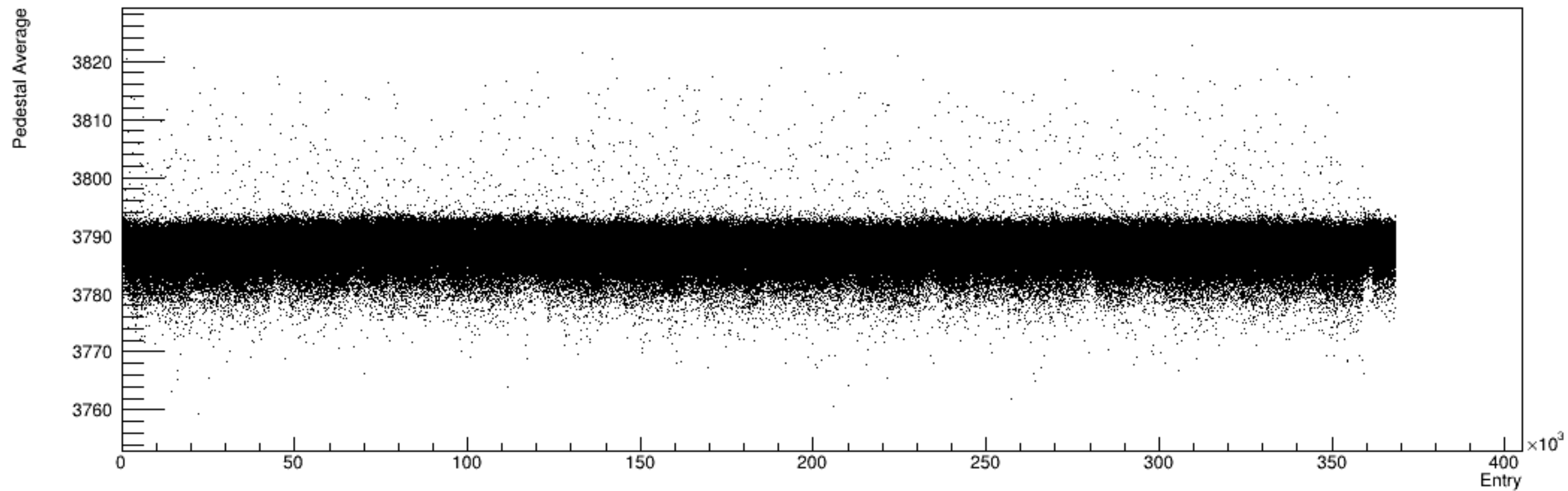
Run 4381, snapshots: Pedestal vs. Time
