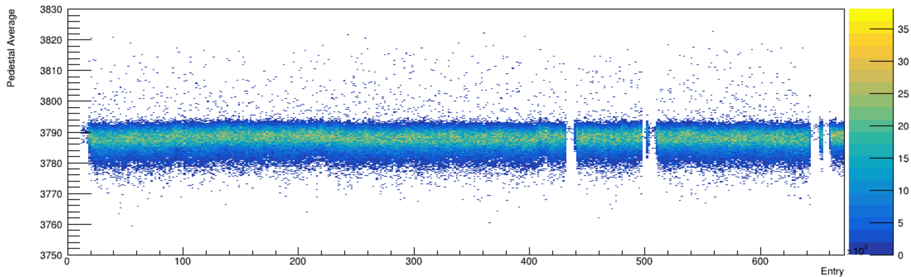
Run 4381, snapshots: Pedestal vs. Time
