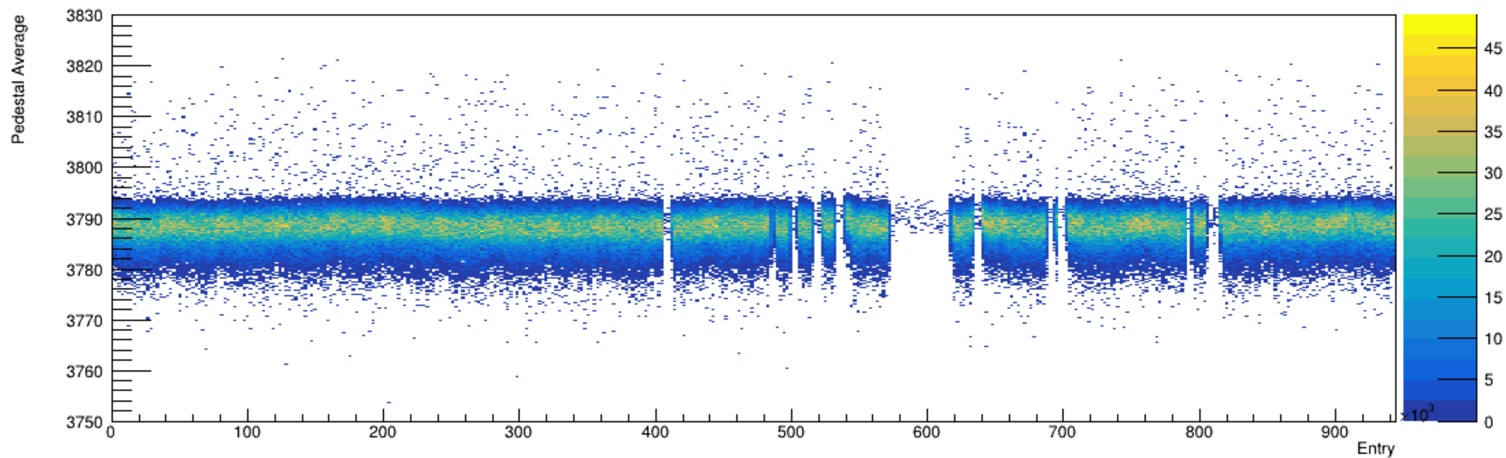
Run 4385, snapshots: Pedestal vs. Time
