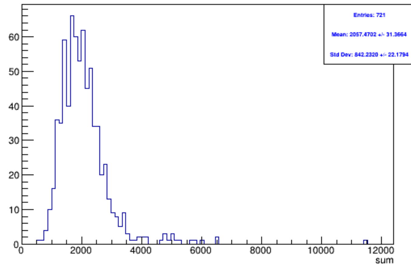
Run 4391 triggerwise, sums: Beam OFF
