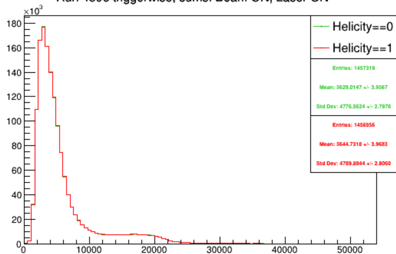
Run 4396 triggerwise, sums: Beam ON, Laser ON
