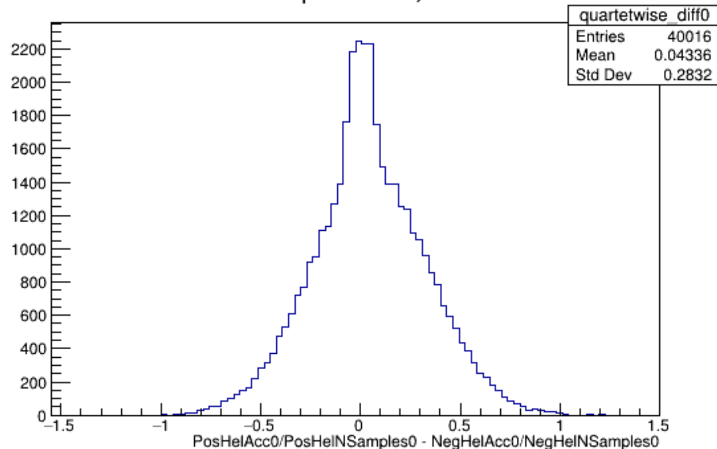
Run 4399 quartetwise, Diffs0: All
