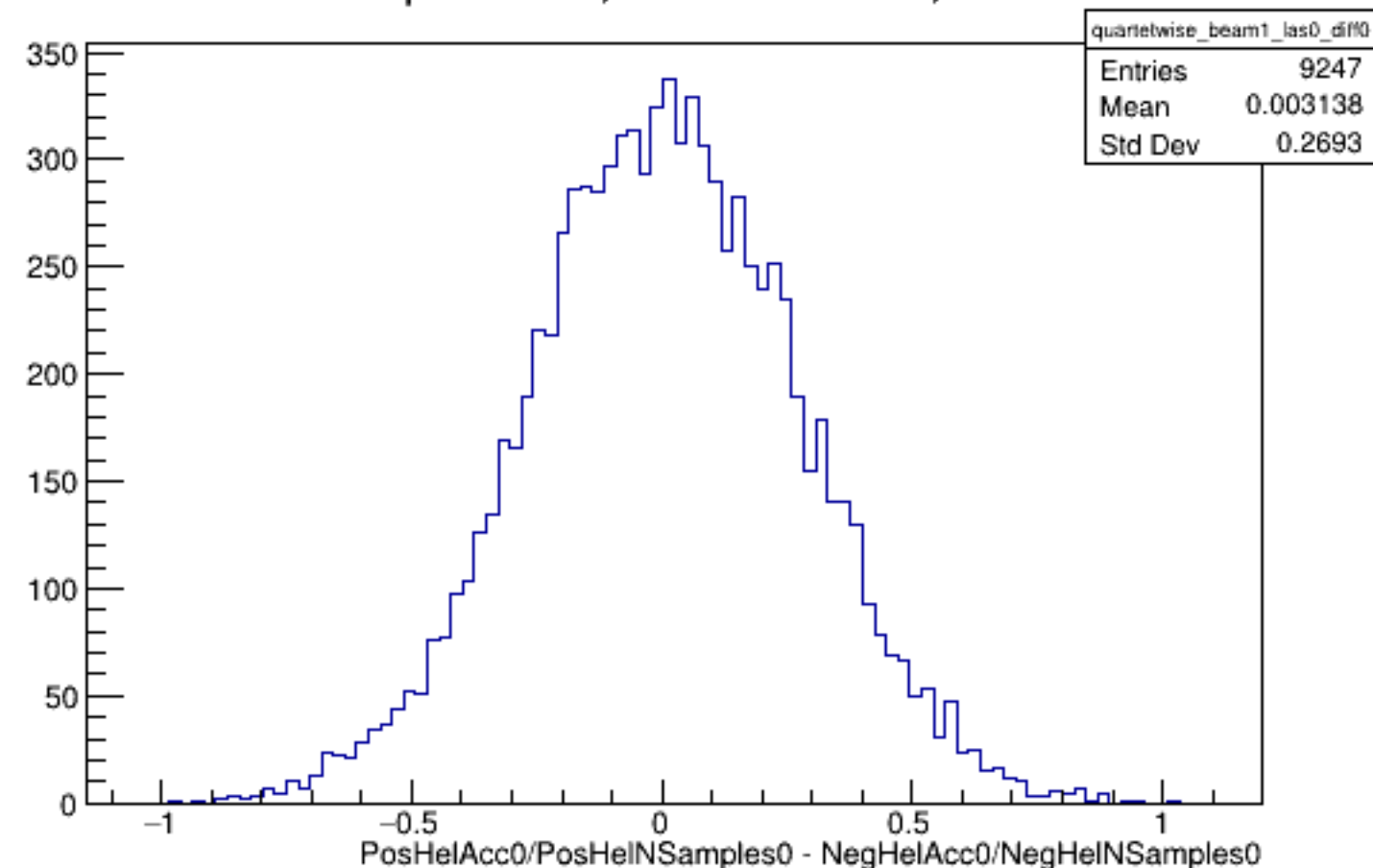
Run 4399 quartetwise, Diffs0: Beam ON, Laser OFF
