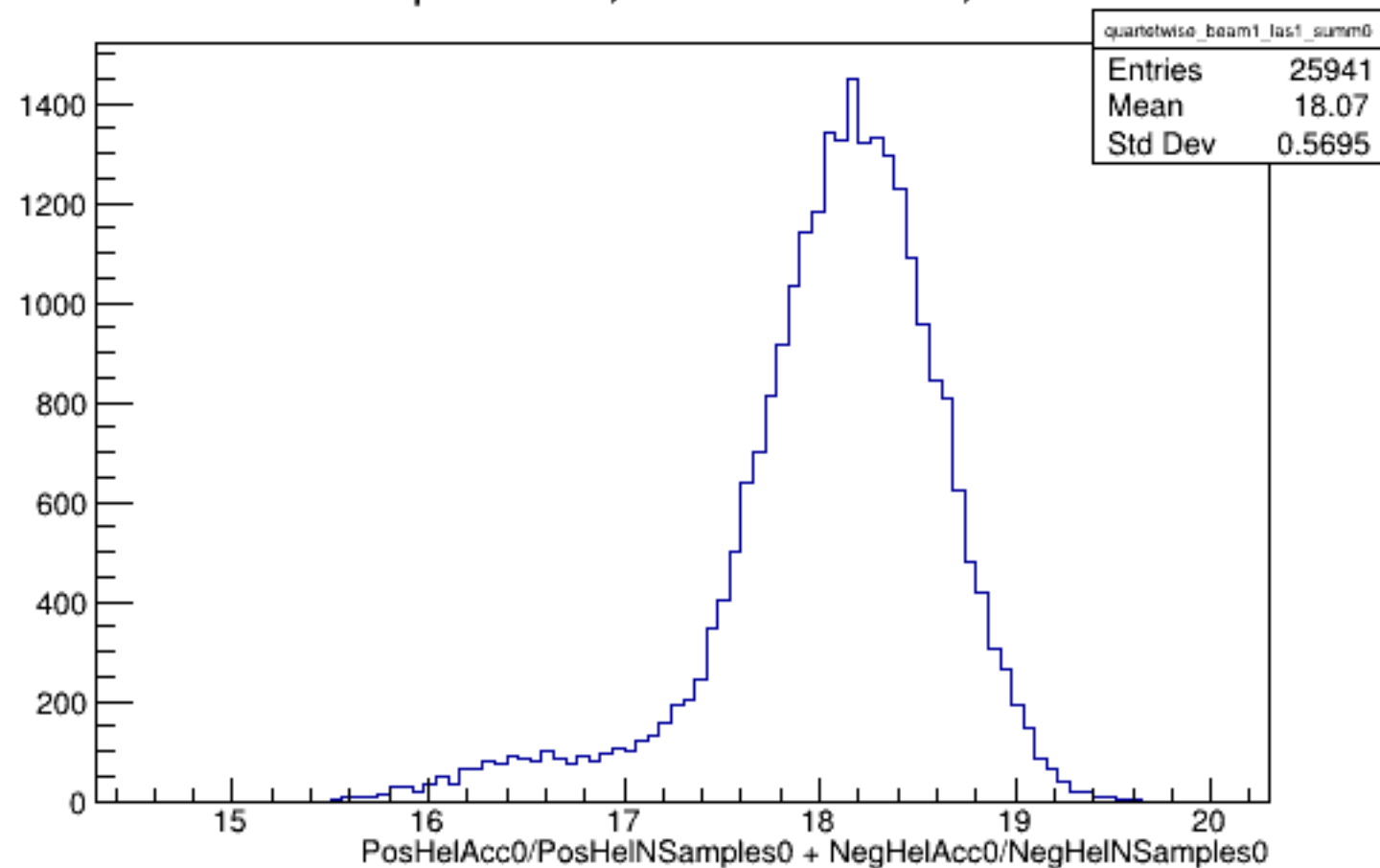
Run 4399 quartetwise, Sums0: Beam ON, Laser ON
