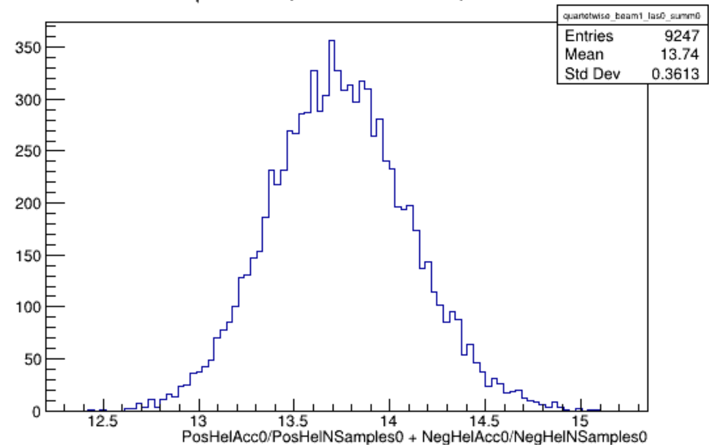
Run 4399 quartetwise, Sums0: Beam ON, Laser OFF
