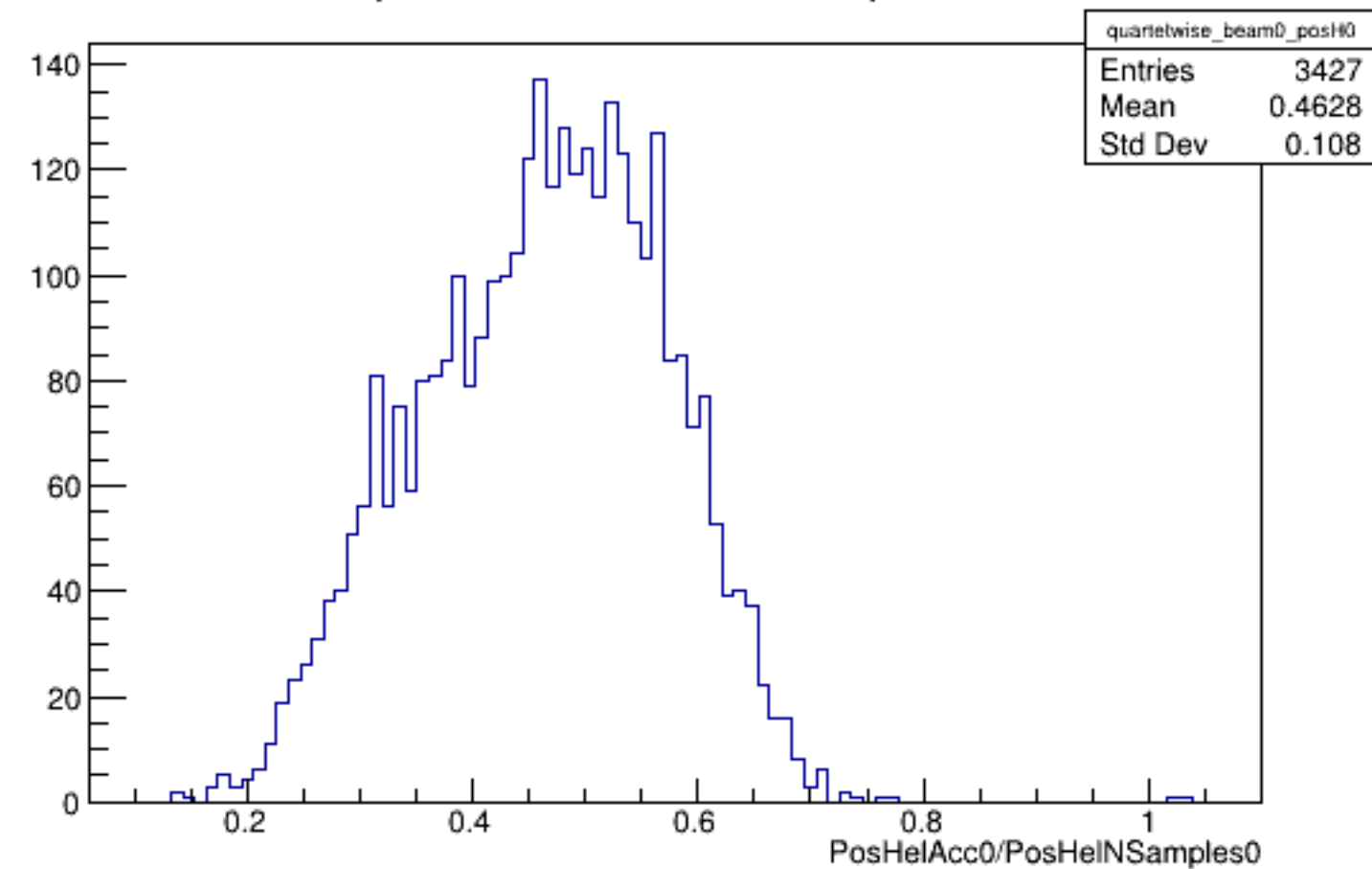
Run 4399 quartetwise, PosHelAcc0/NSamples0: Beam OFF
