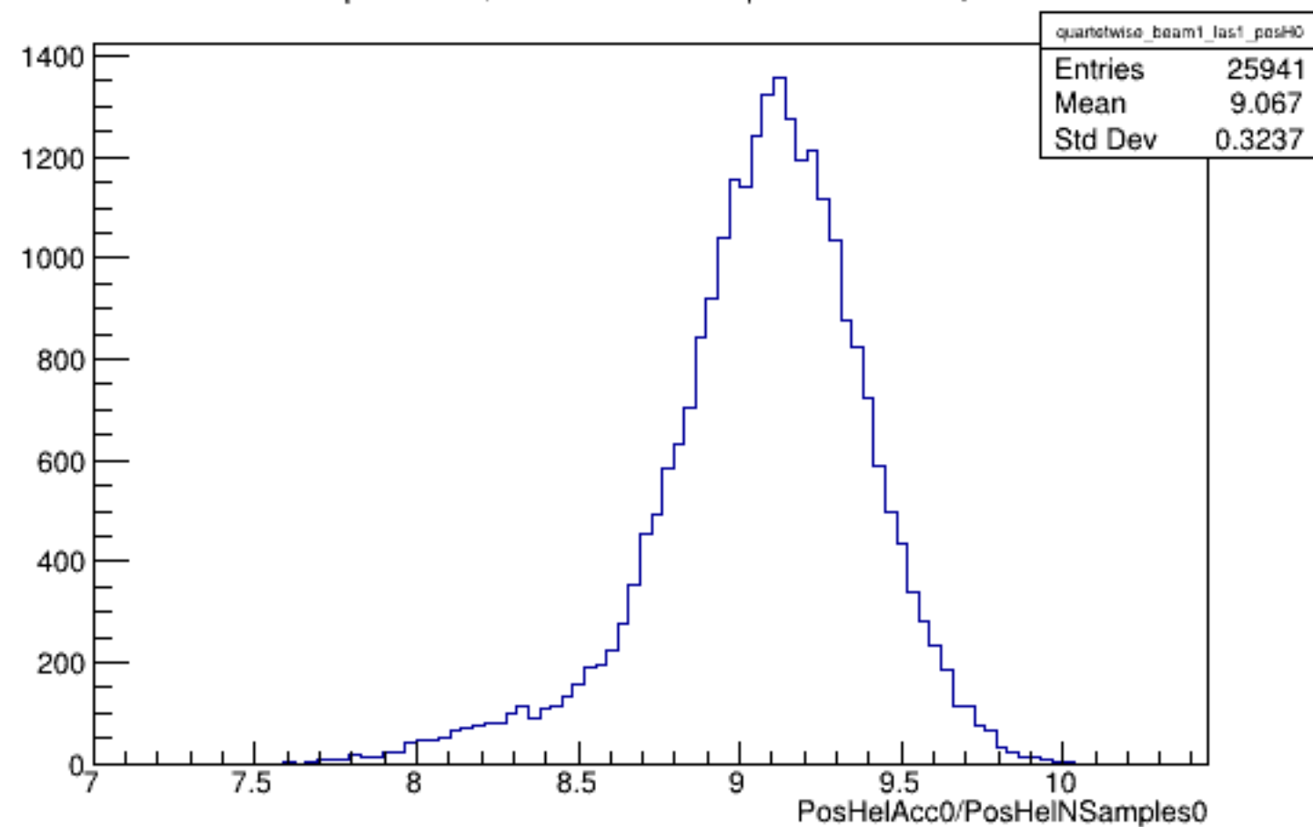
Run 4399 quartetwise, PosHelAcc0/NSamples0: Beam ON, Laser ON
