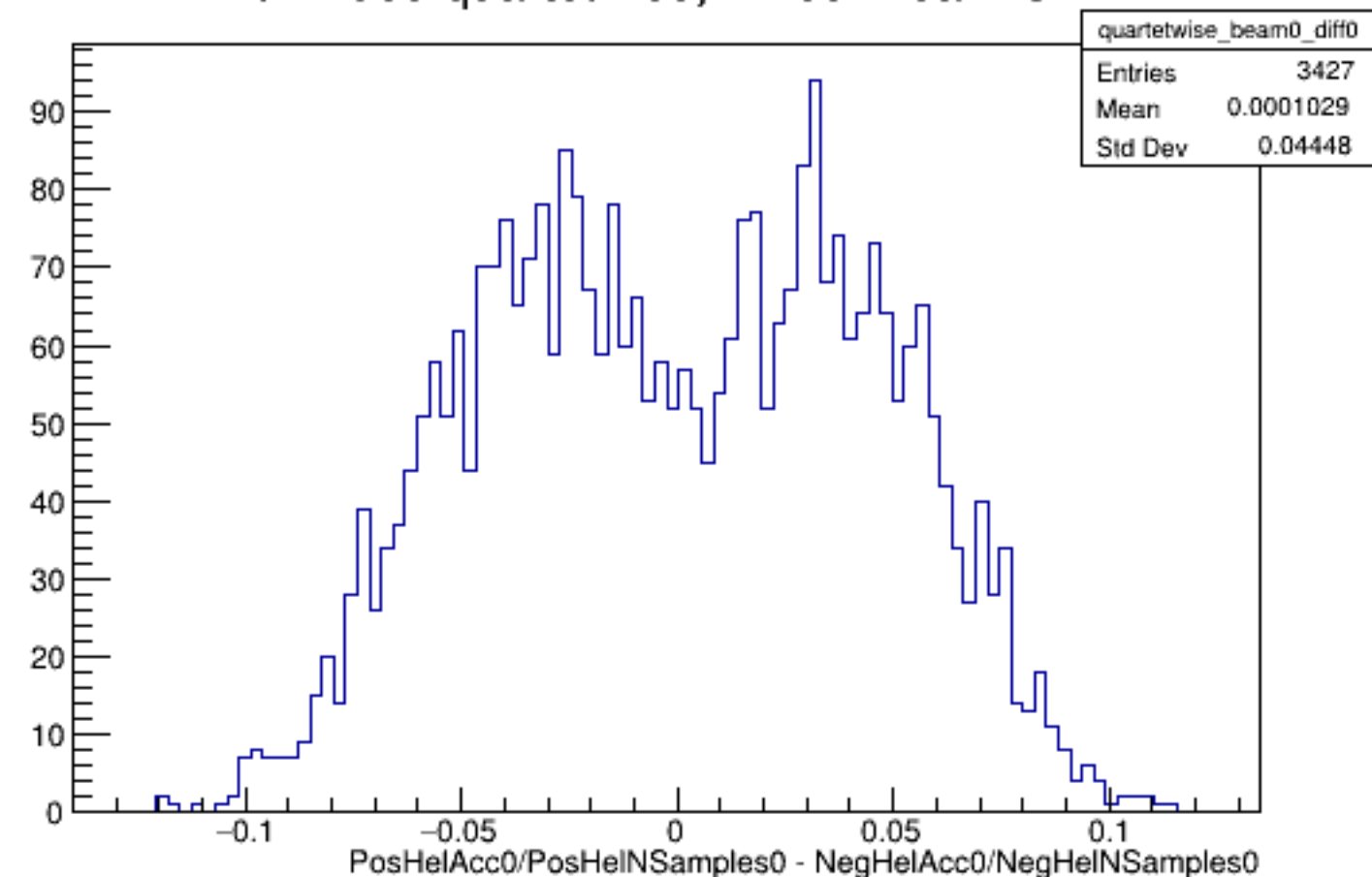
Run 4399 quartetwise, Diffs0: Beam OFF
