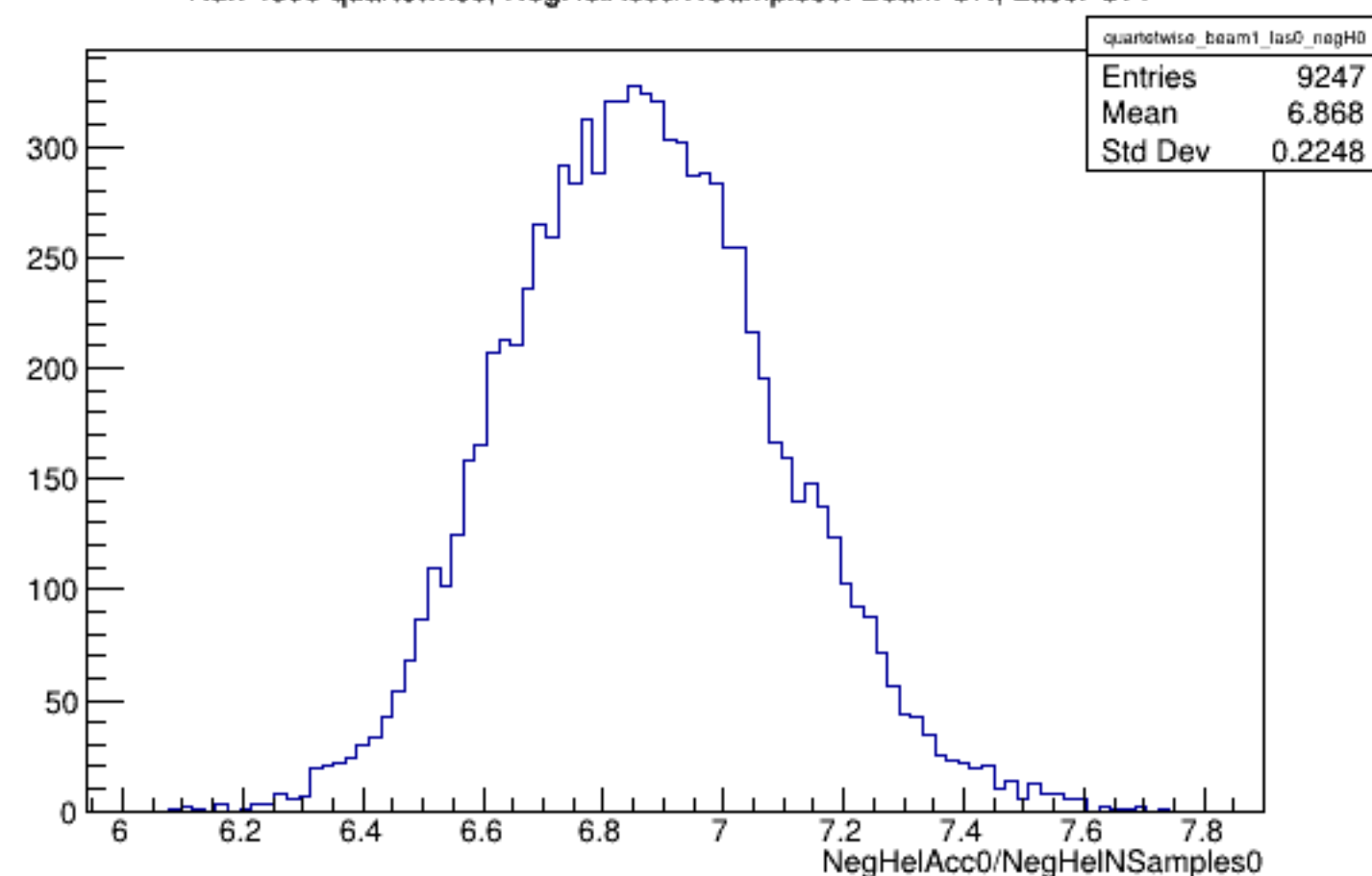
Run 4399 quartetwise, NegHelAcc0/NSamples0: Beam ON, Laser OFF
