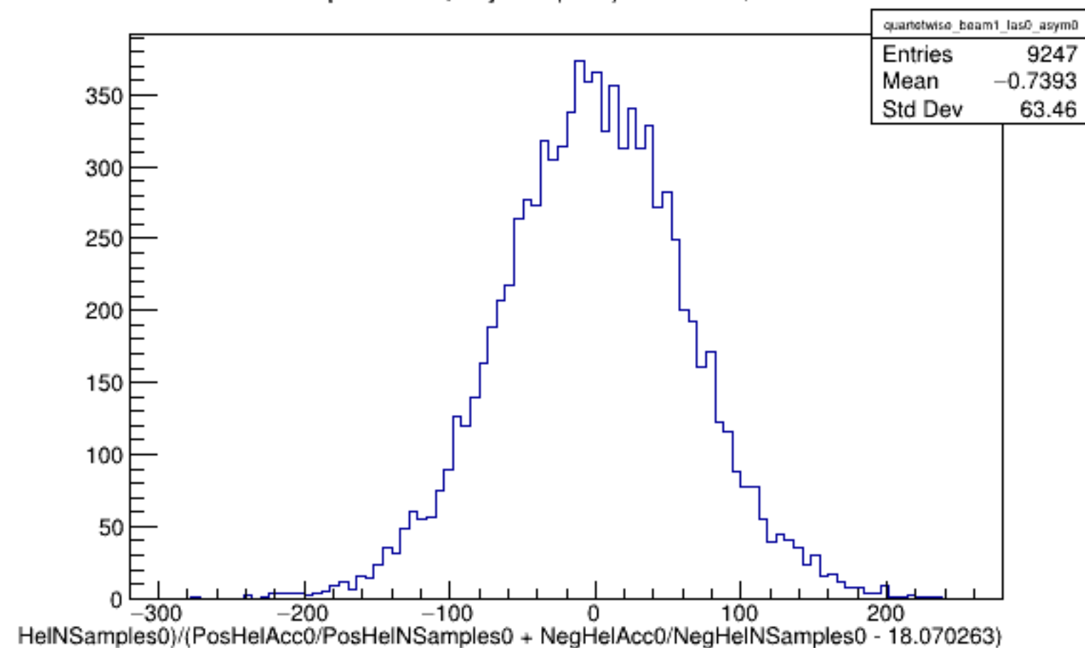
Run 4399 quartetwise, Asyms0 (Raw): Beam ON, Laser OFF
