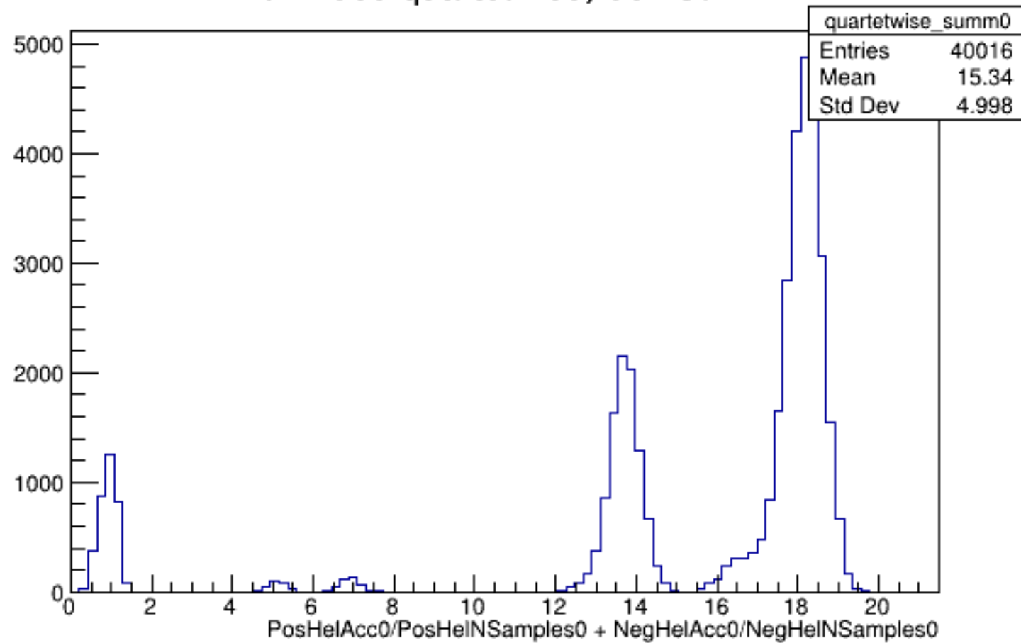
Run 4399 quartetwise, Sums0: All
