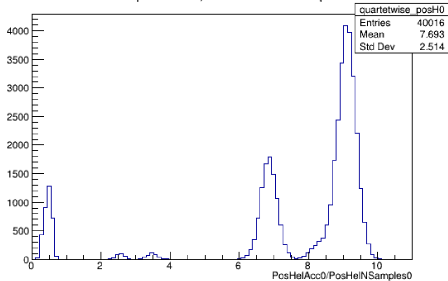
Run 4399 quartetwise, PosHelAcc0/NSamples0: All
