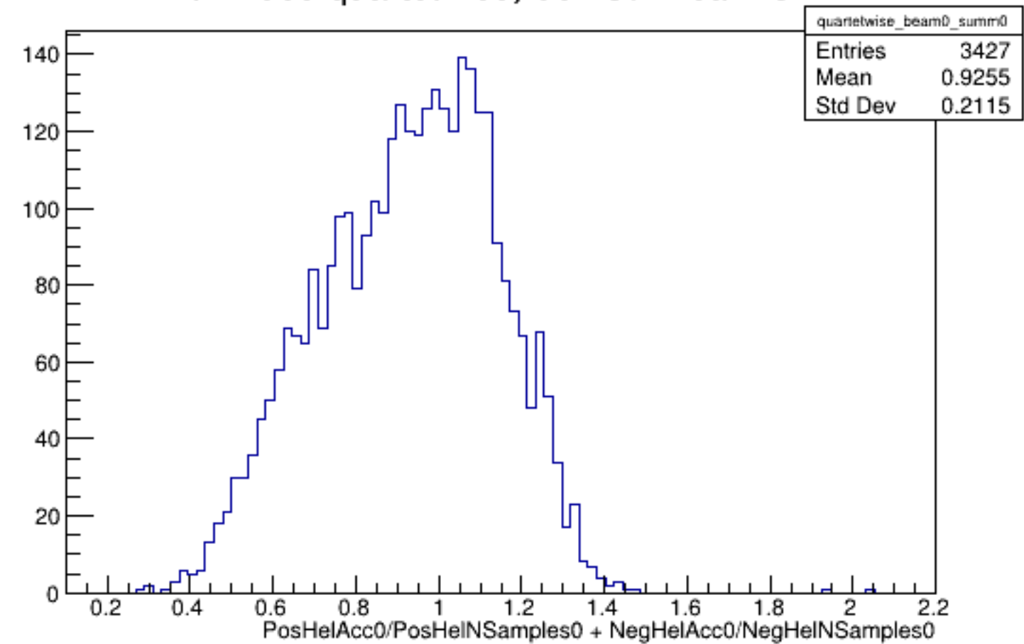
Run 4399 quartetwise, Sums0: Beam OFF
