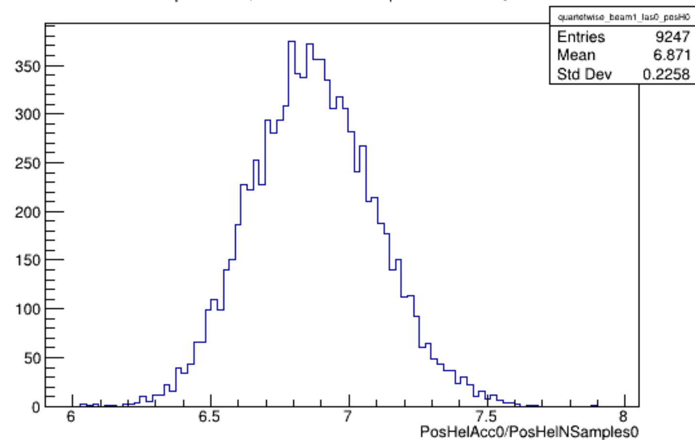
Run 4399 quartetwise, PosHelAcc0/NSamples0: Beam ON, Laser OFF
