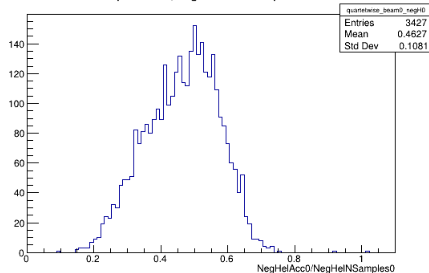
Run 4399 quartetwise, NegHelAcc0/NSamples0: Beam OFF
