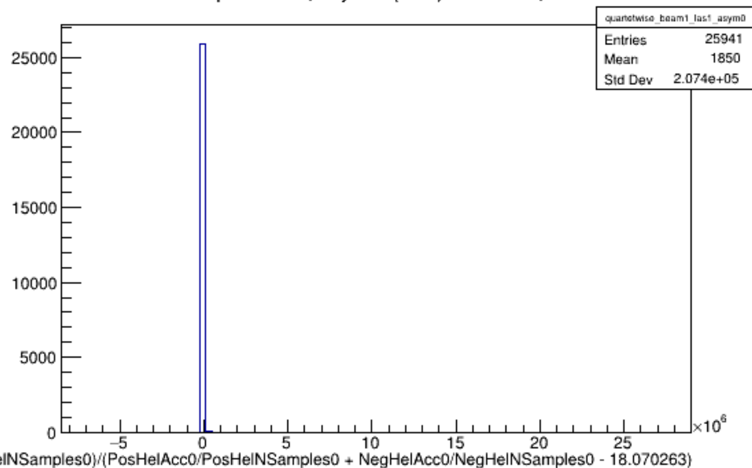
Run 4399 quartetwise, Asyms0 (Raw): Beam ON, Laser ON
