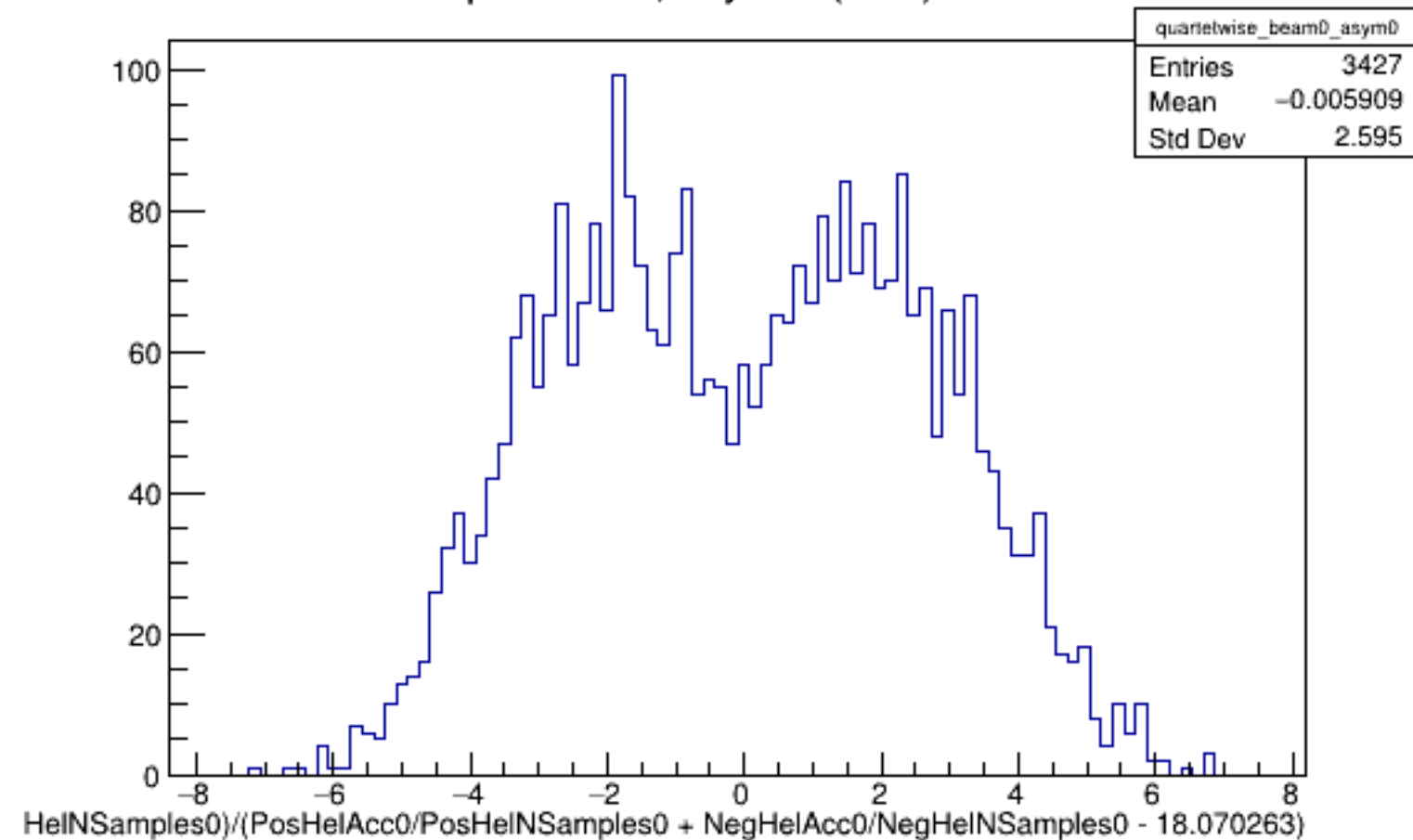
Run 4399 quartetwise, Asyms0 (Raw): Beam OFF
