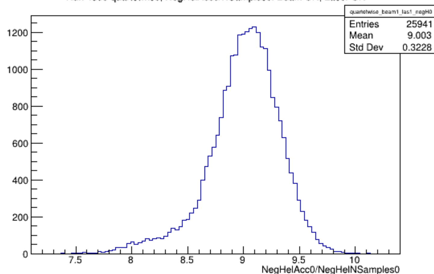
Run 4399 quartetwise, NegHelAcc0/NSamples0: Beam ON, Laser ON
