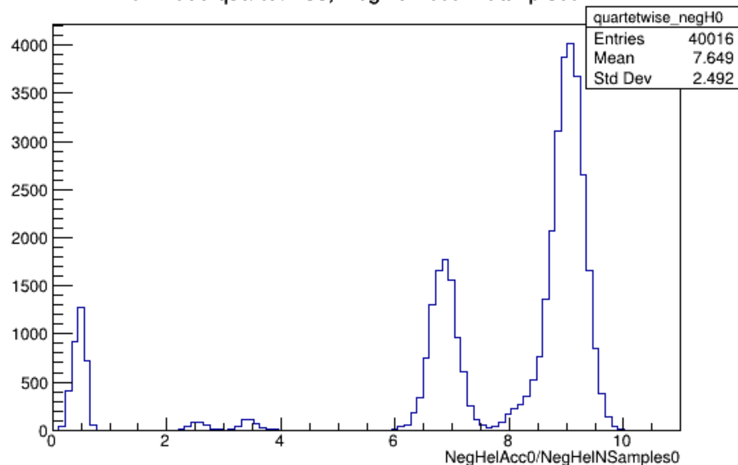
Run 4399 quartetwise, NegHelAcc0/NSamples0: All
