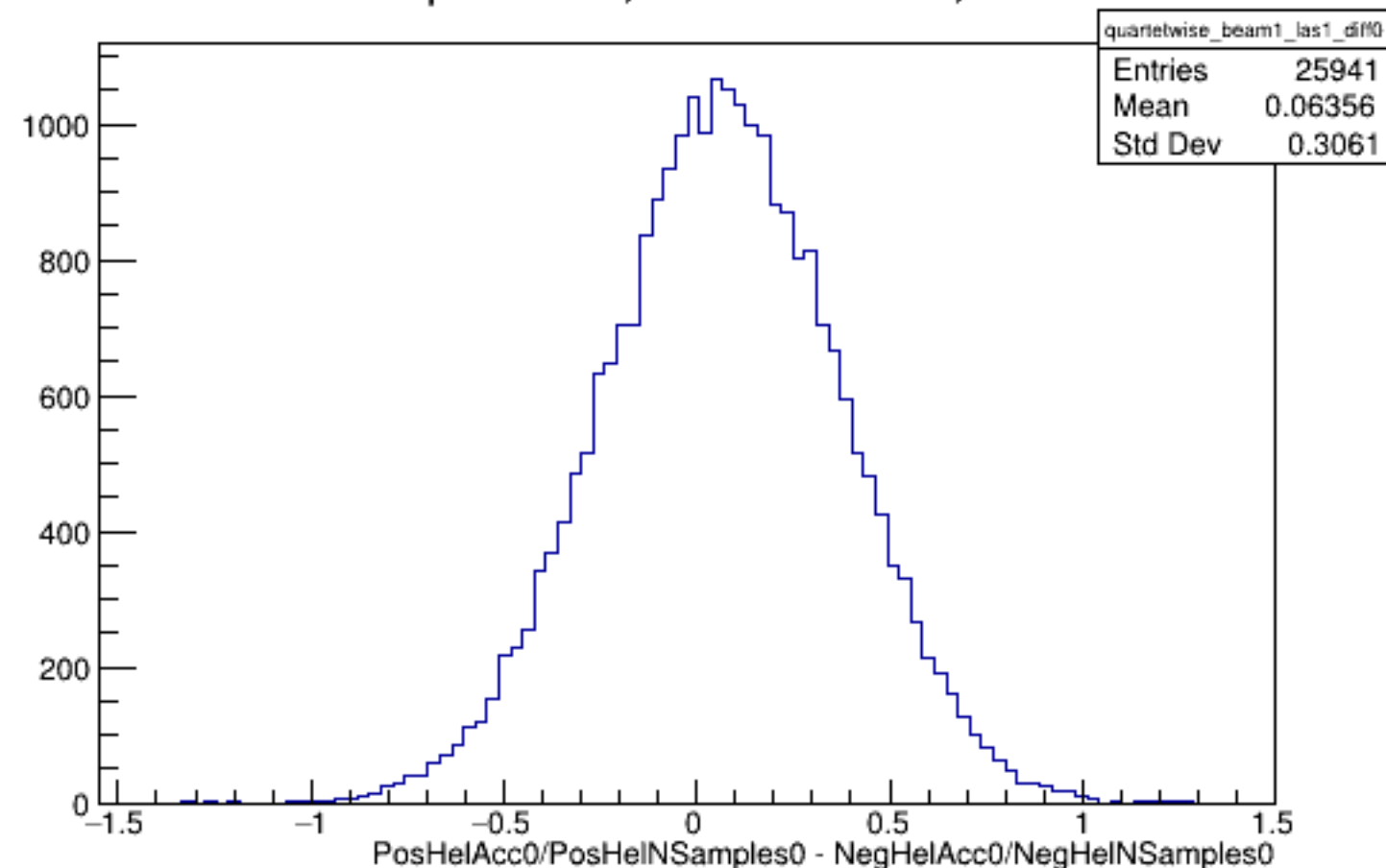
Run 4399 quartetwise, Diffs0: Beam ON, Laser ON
