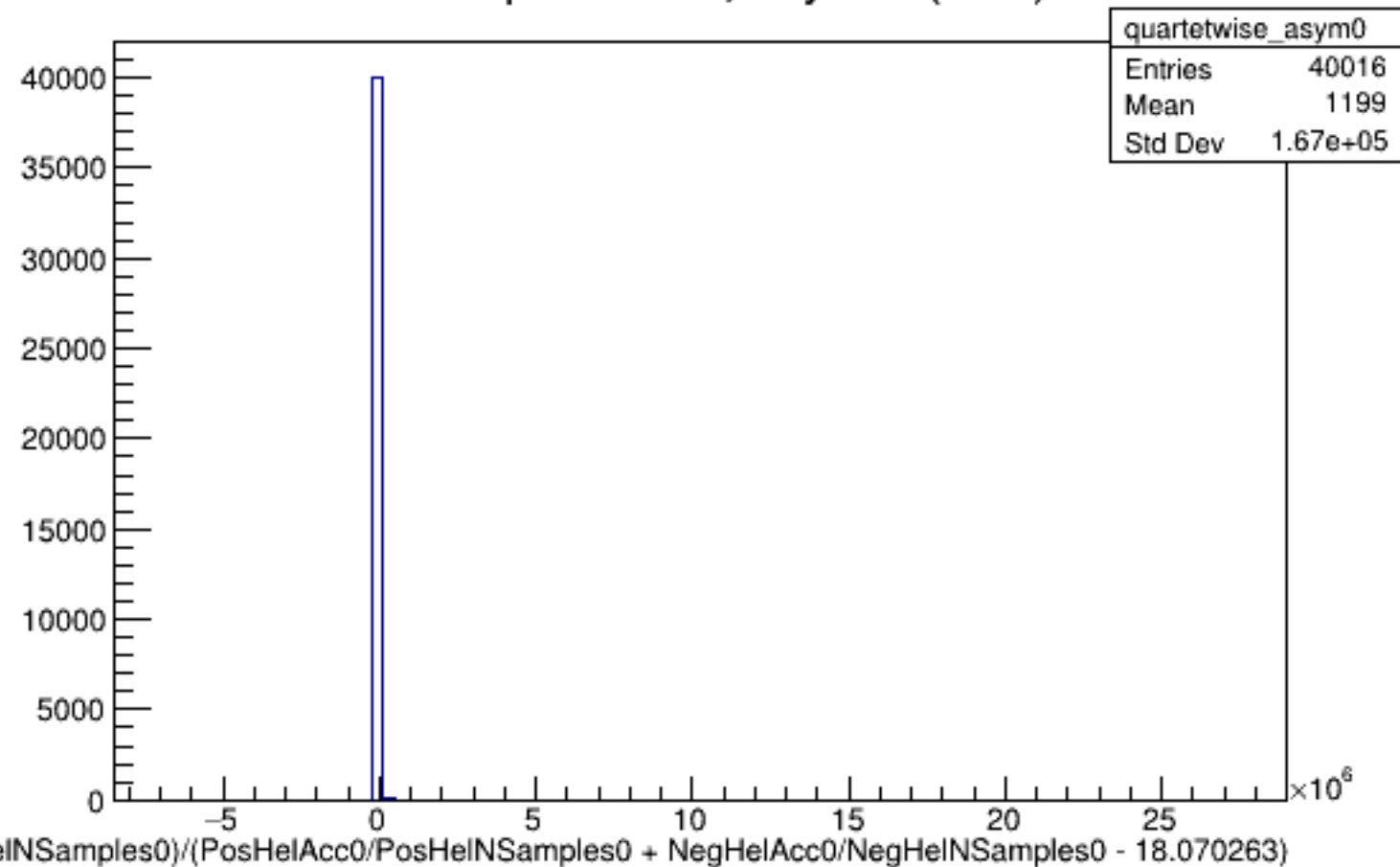
Run 4399 quartetwise, Asyms0 (Raw): All
