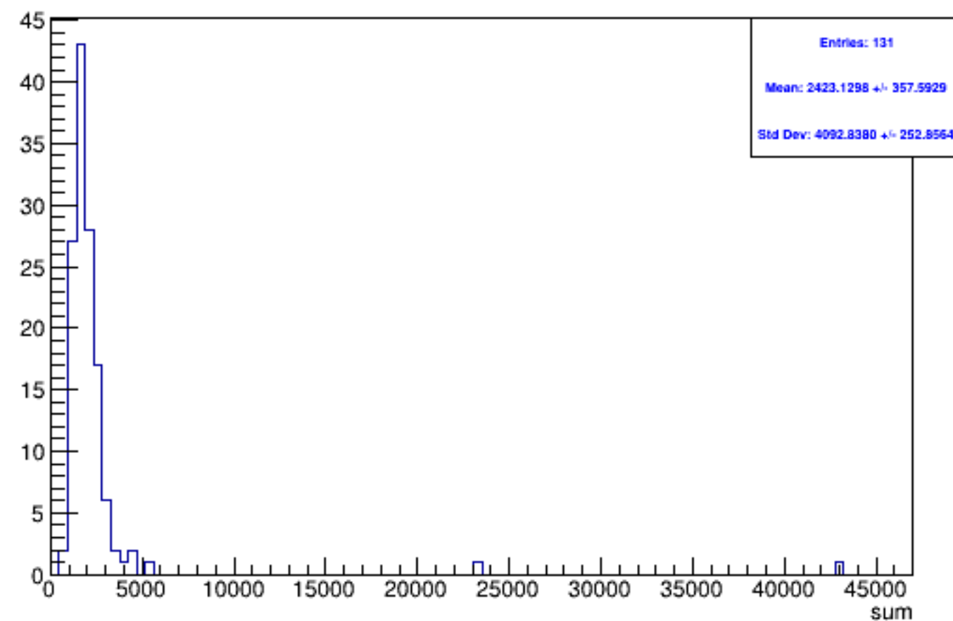
Run 4399 triggerwise, sums: Beam OFF
