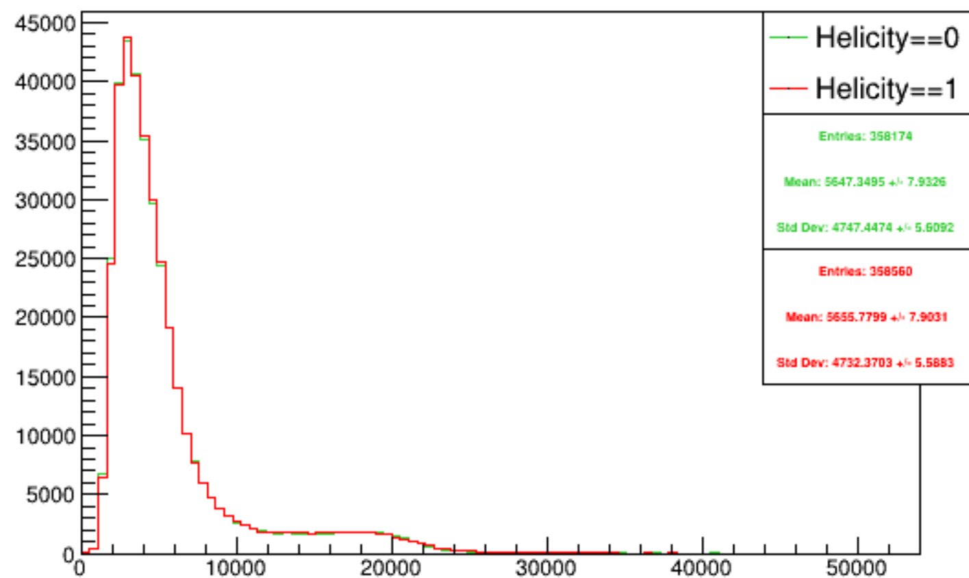
Run 4399 triggerwise, sums: Beam ON, Laser ON
