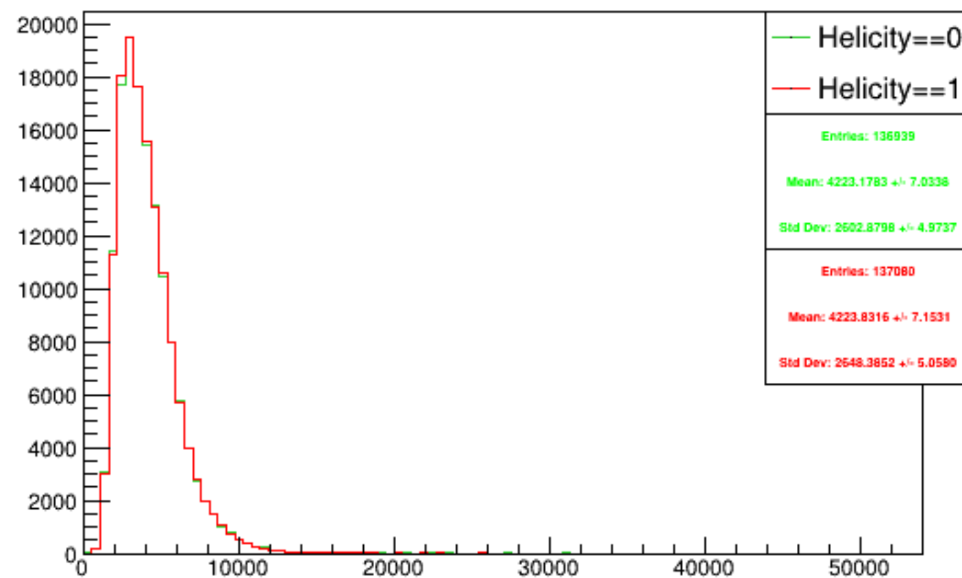
Run 4399 triggerwise, sums: Beam ON, Laser OFF
