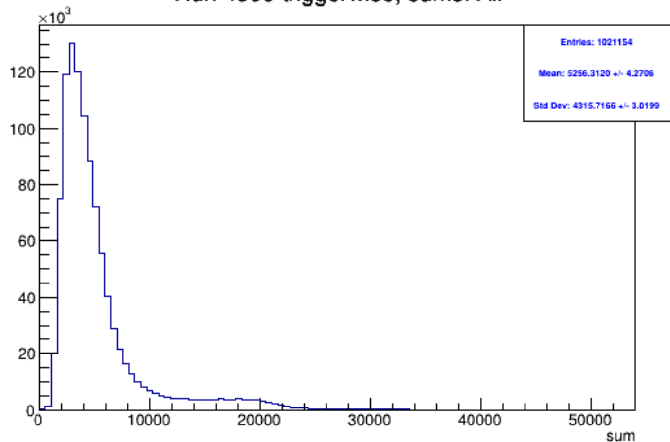
Run 4399 triggerwise, sums: All
