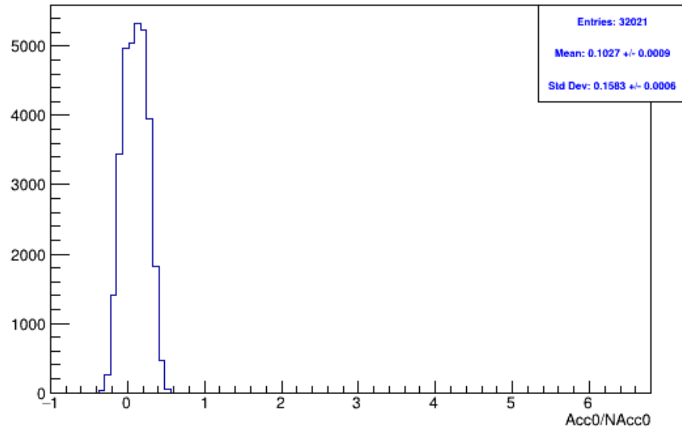
Run 4409 mpwise, acc0: All
