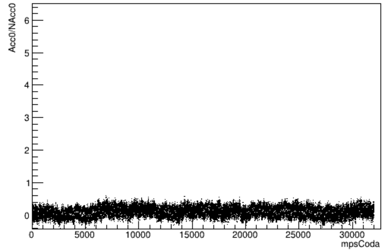
Run 4409 mpwise, Acc0/NAcc0:mpsCoda, beam OFF
