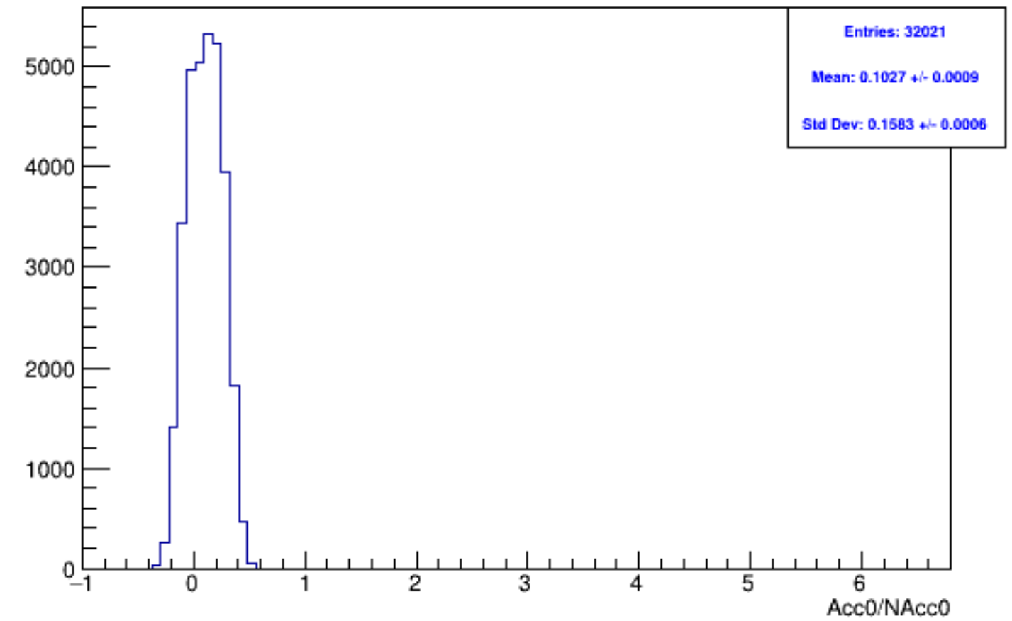
Run 4409 mpwise, acc0: Beam OFF
