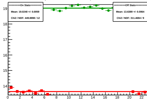
Cycle 4413.8: Multiplet Sums
