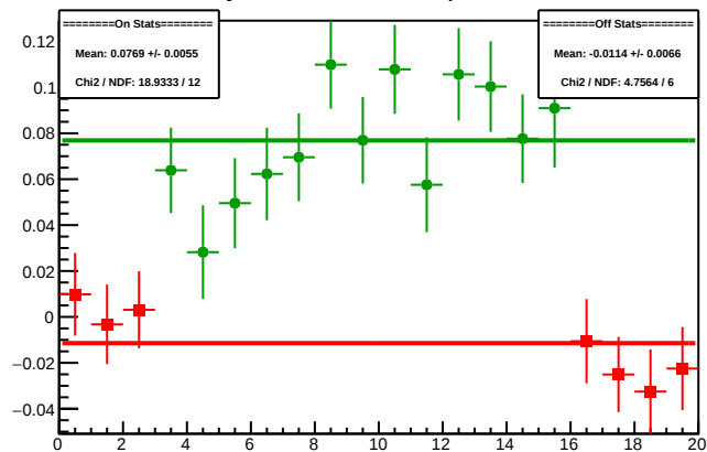
Cycle 4413.25: Multiplet Diffs
