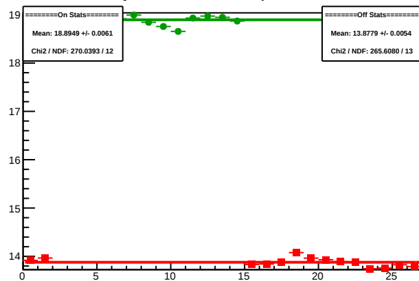
Cycle 4413.15: Multiplet Sums
