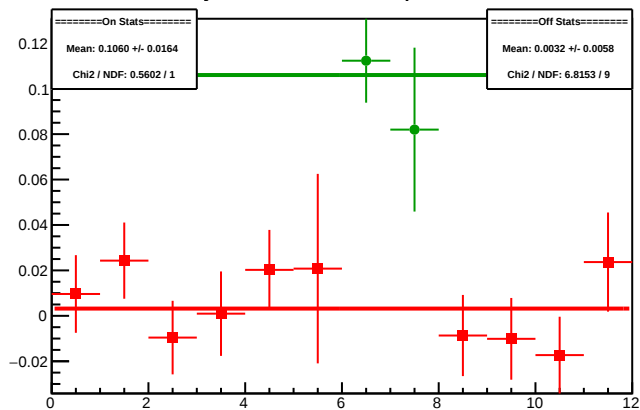
Cycle 4413.10: Multiplet Diffs
