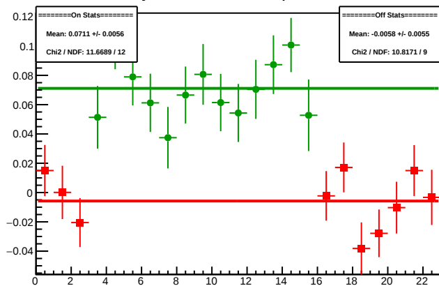
Cycle 4413.23: Multiplet Diffs
