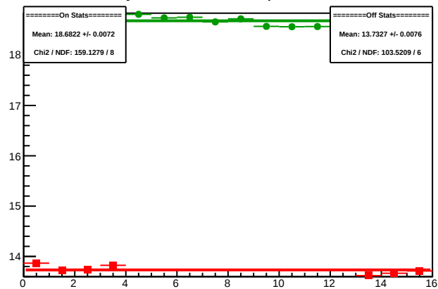
Cycle 4413.26: Multiplet Sums
