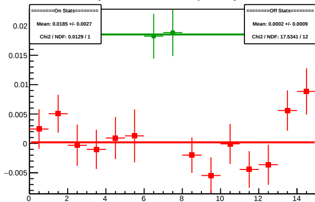
Cycle 4413.18: Multiplet Asyms
