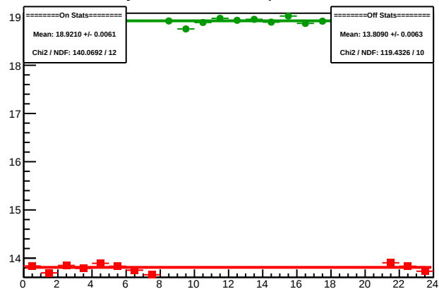
Cycle 4413.28: Multiplet Sums
