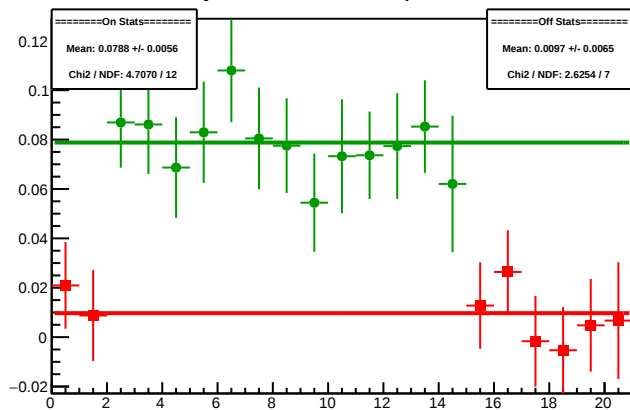
Cycle 4413.17: Multiplet Diffs
