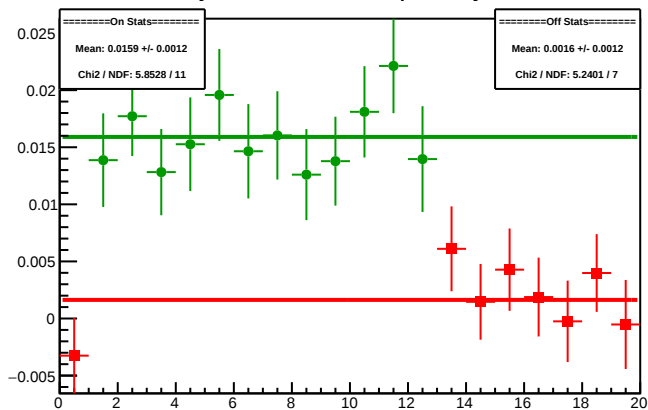
Cycle 4413.20: Multiplet Asyms
