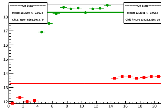
Cycle 4413.6: Multiplet Sums
