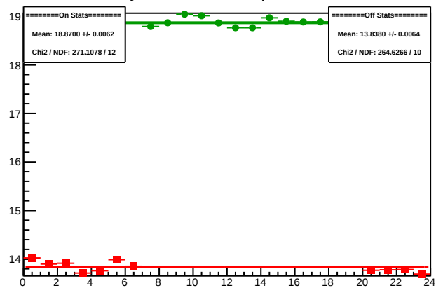
Cycle 4413.1: Multiplet Sums
