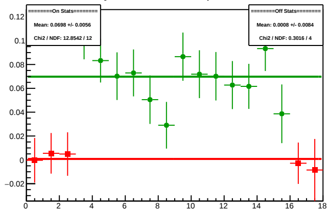
Cycle 4413.12: Multiplet Diffs
