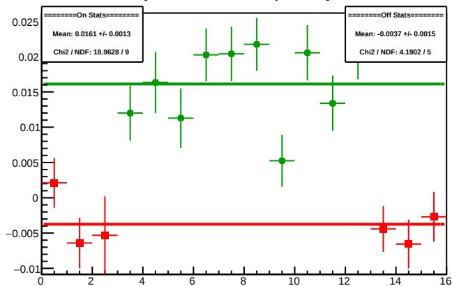
Cycle 4413.4: Multiplet Asyms
