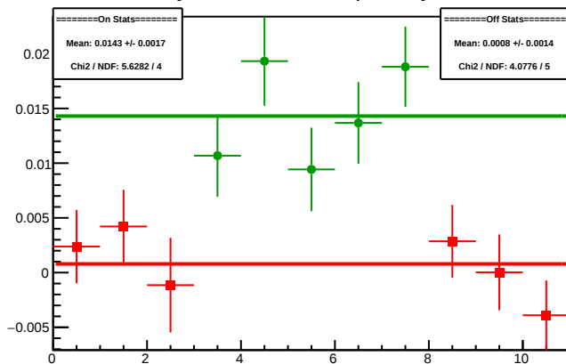
Cycle 4413.22: Multiplet Asyms
