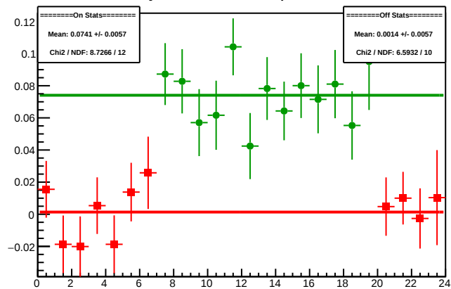
Cycle 4413.1: Multiplet Diffs
