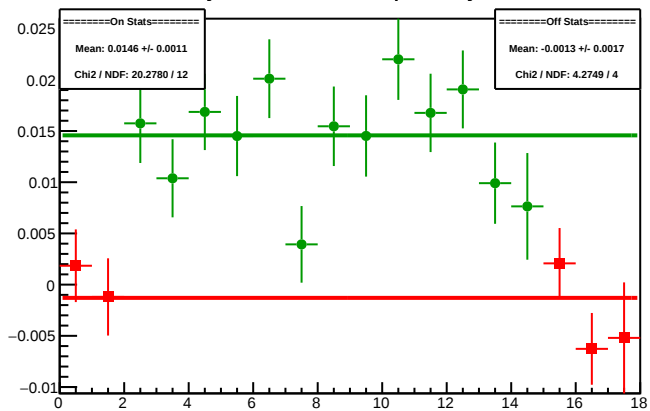
Cycle 4413.3: Multiplet Asyms
