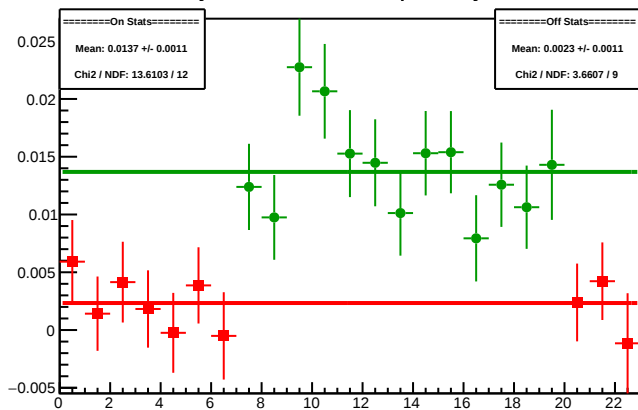
Cycle 4413.21: Multiplet Asyms
