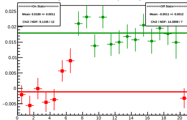
Cycle 4413.19: Multiplet Asyms
