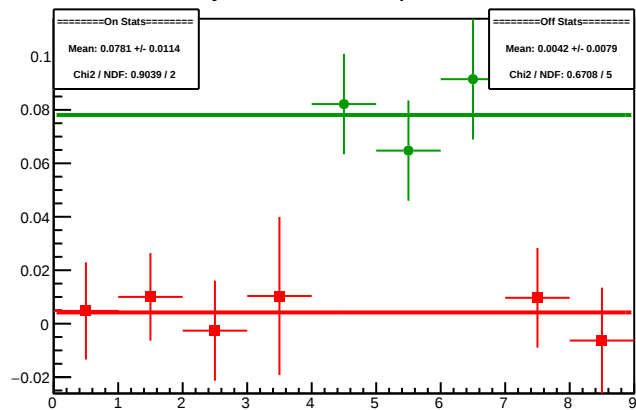
Cycle 4413.2: Multiplet Diffs
