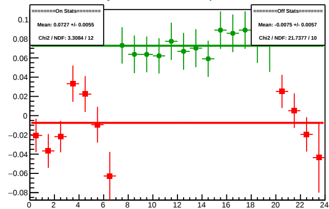
Cycle 4414.10: Multiplet Diffs
