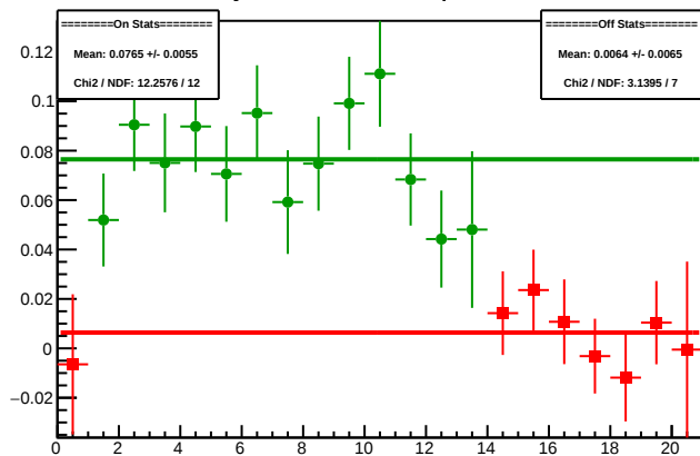
Cycle 4414.1: Multiplet Diffs
