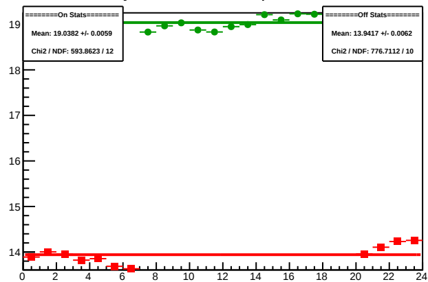
Cycle 4414.10: Multiplet Sums
