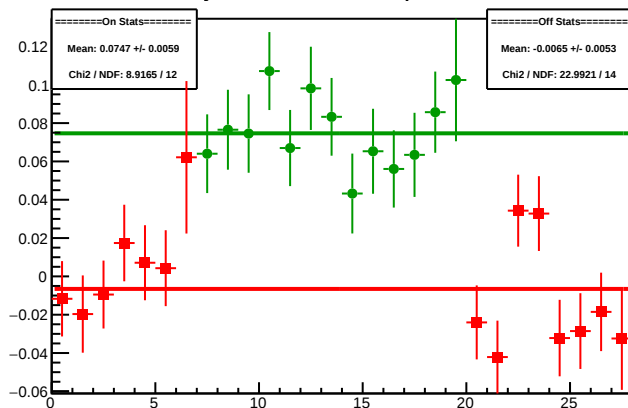
Cycle 4414.18: Multiplet Diffs
