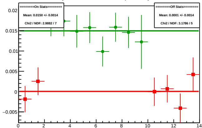
Cycle 4414.15: Multiplet Asyms
