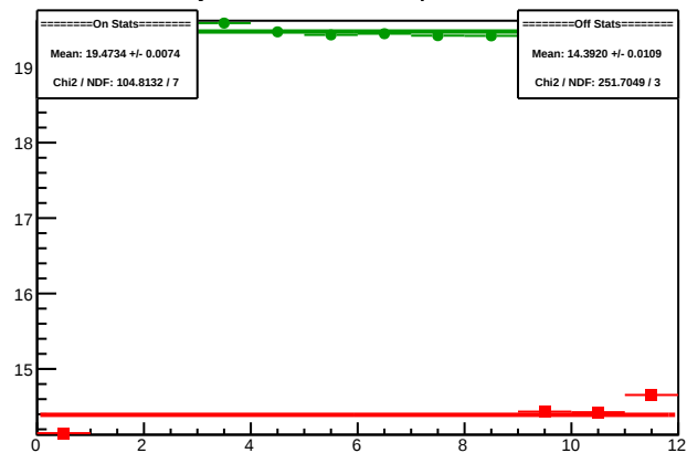
Cycle 4414.13: Multiplet Sums
