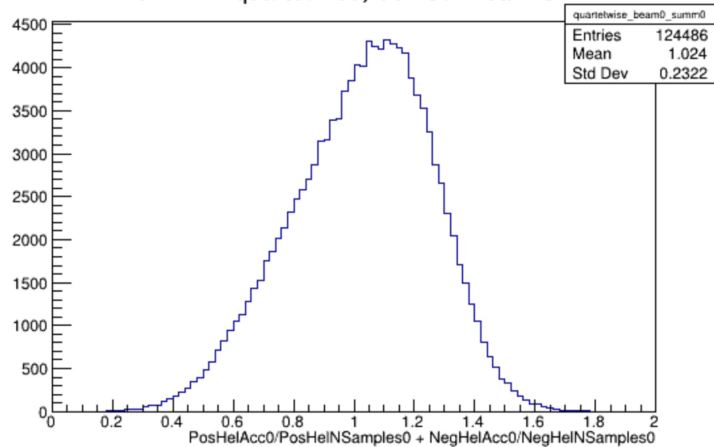
Run 4424 quartetwise, Sums0: Beam OFF
