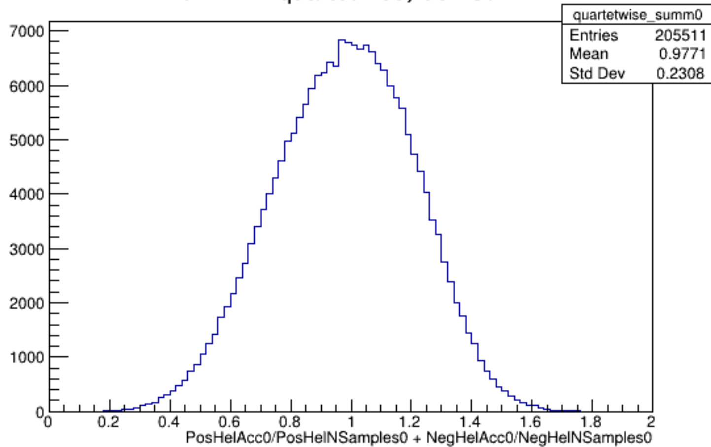
Run 4424 quartetwise, Sums0: All
